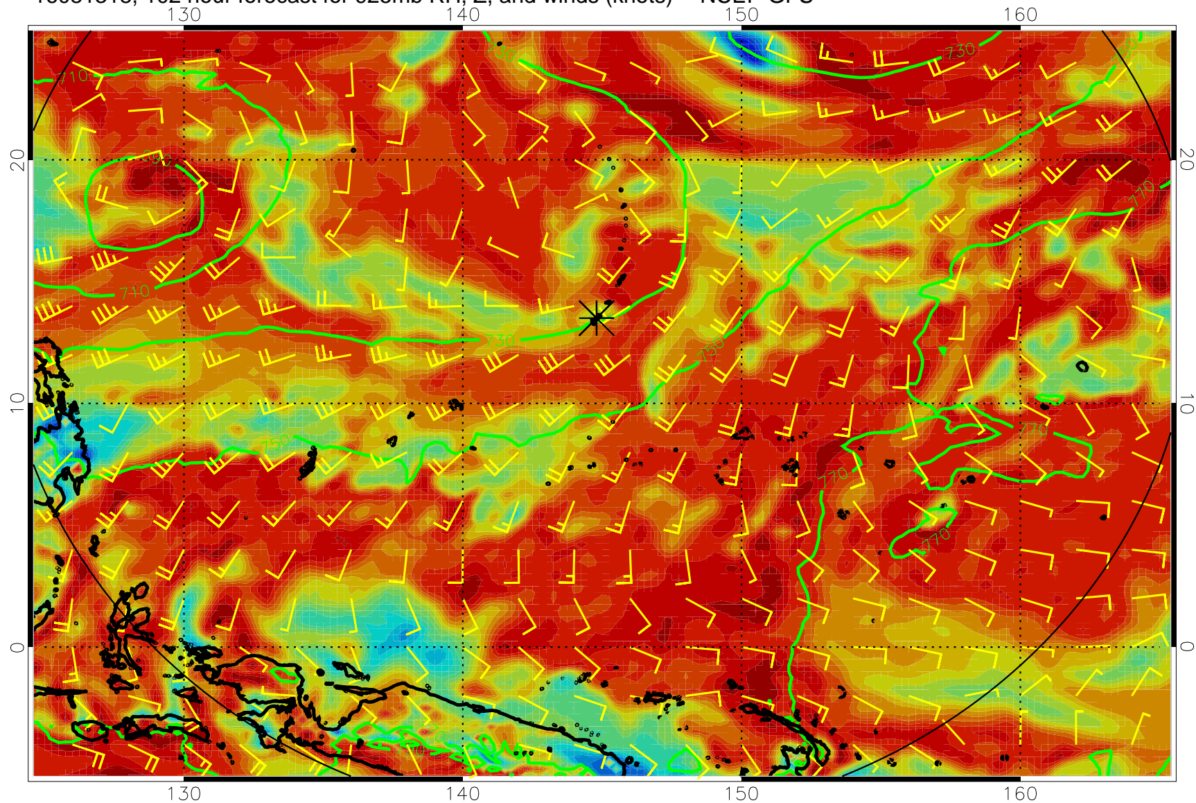
16081318, 102 hour forecast for 925mb RH, Z, and winds (knots) -- NCEP GFS
