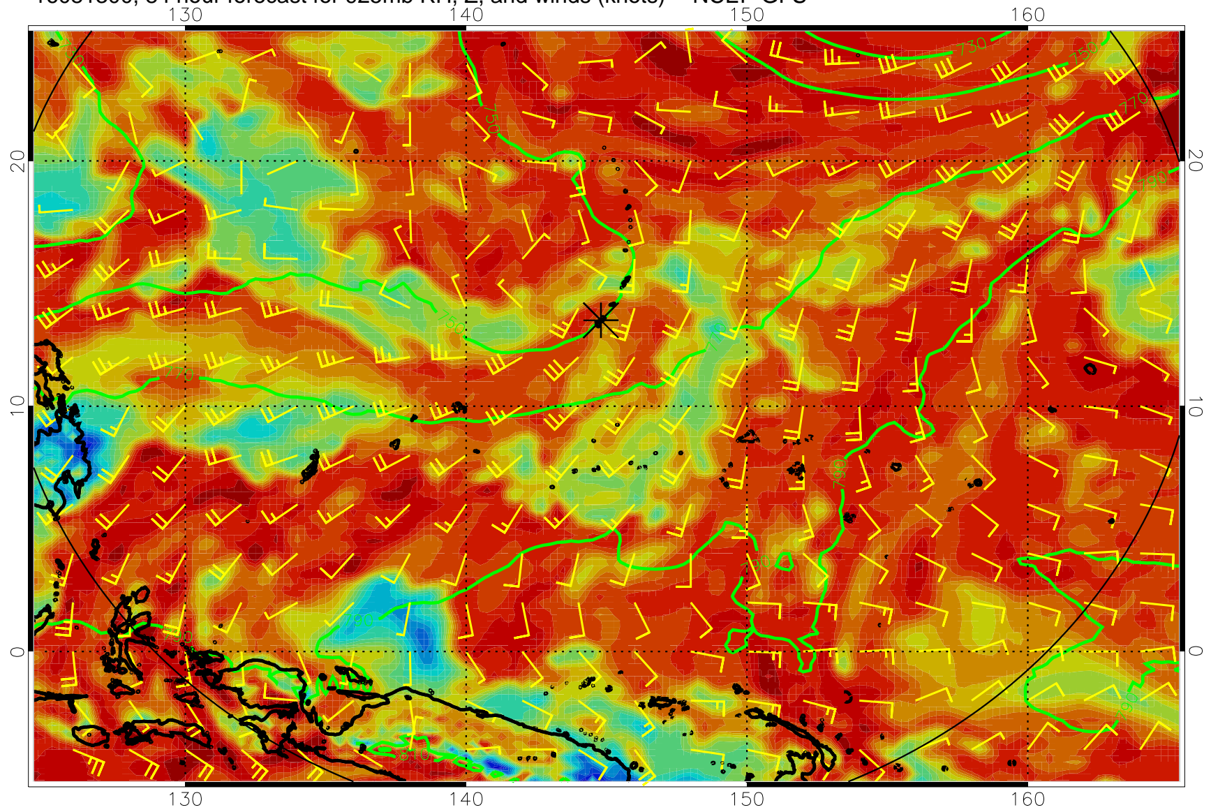
16081300, 84 hour forecast for 925mb RH, Z, and winds (knots) -- NCEP GFS
