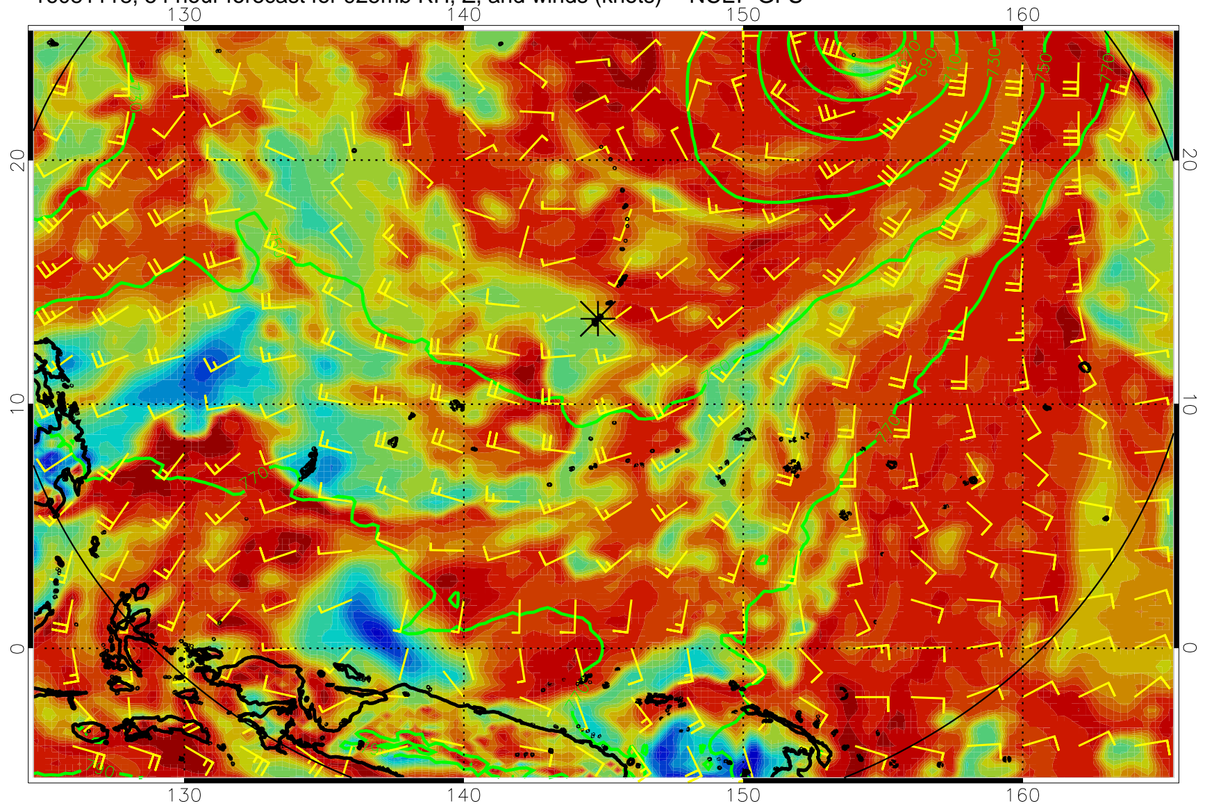
16081118, 54 hour forecast for 925mb RH, Z, and winds (knots) -- NCEP GFS
