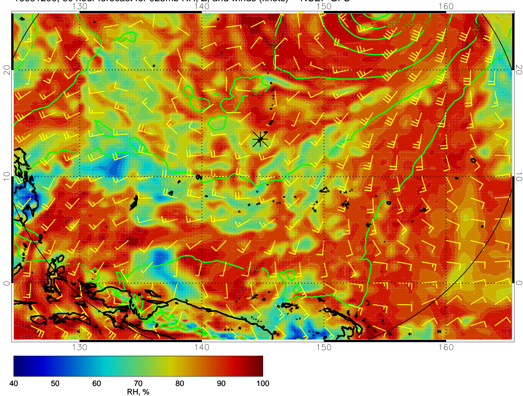
16081200, 60 hour forecast for 925mb RH, Z, and winds (knots) -- NCEP GFS
