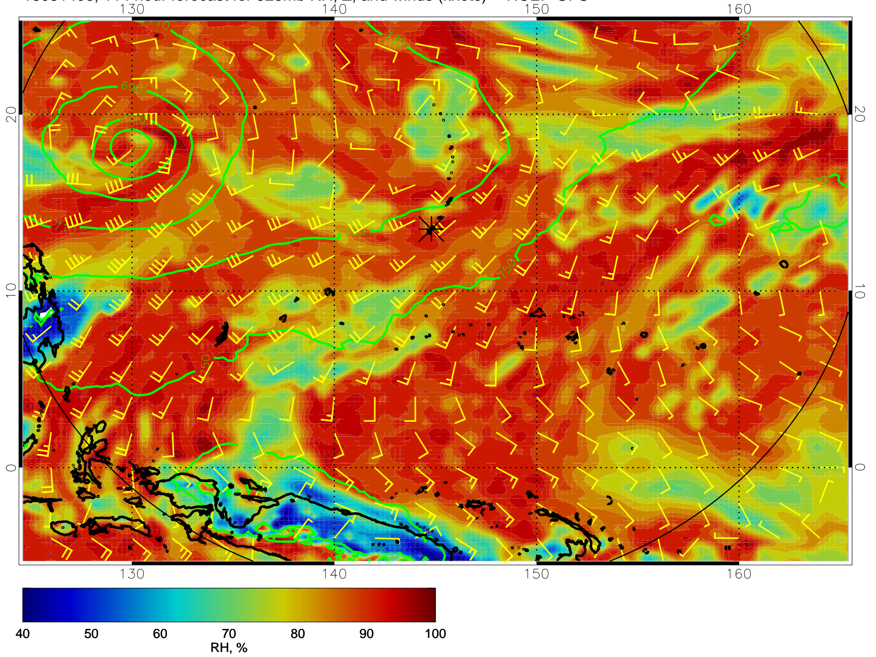
16081406, 114 hour forecast for 925mb RH, Z, and winds (knots) -- NCEP GFS
