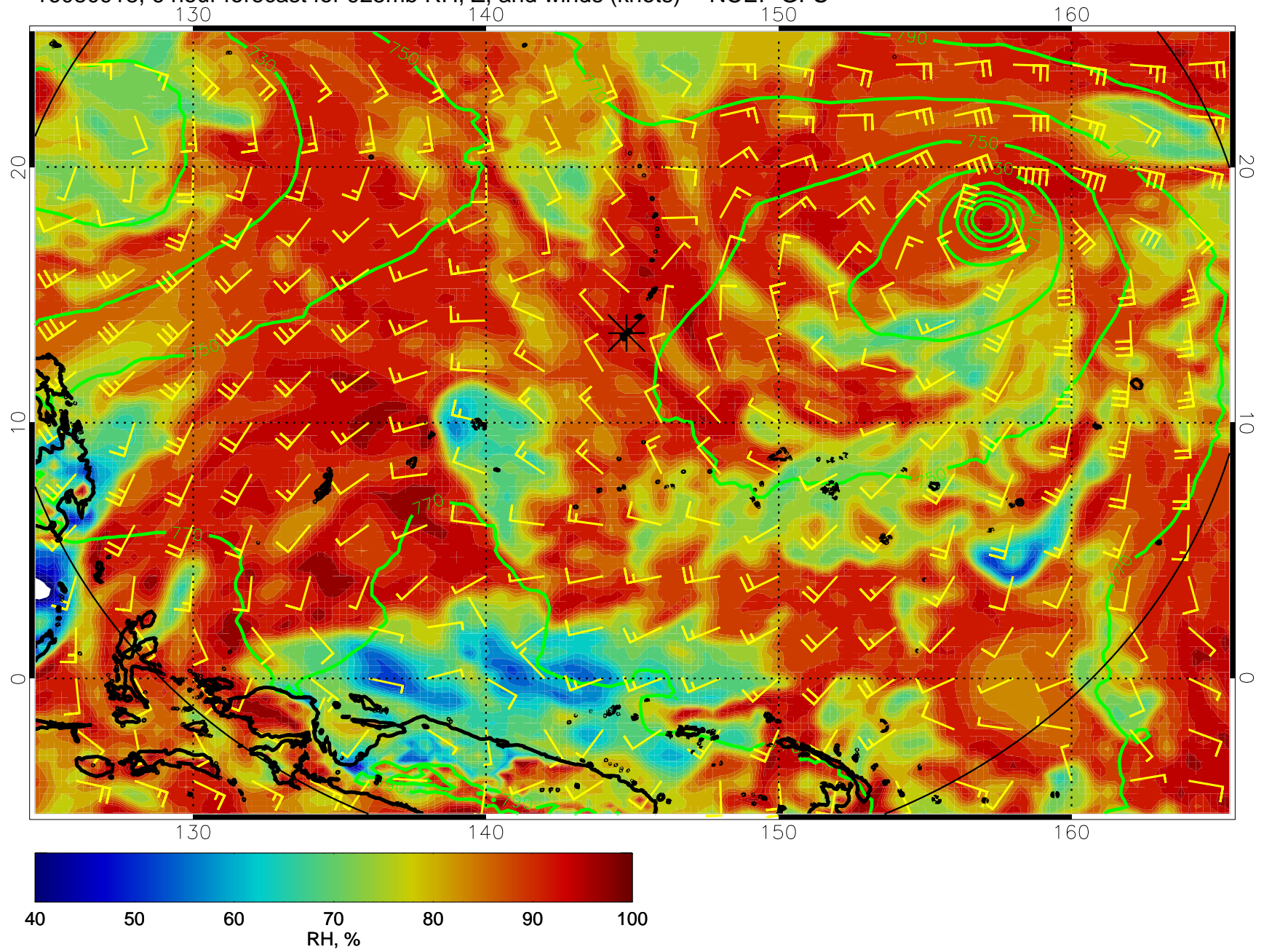
16080918, 6 hour forecast for 925mb RH, Z, and winds (knots) -- NCEP GFS
