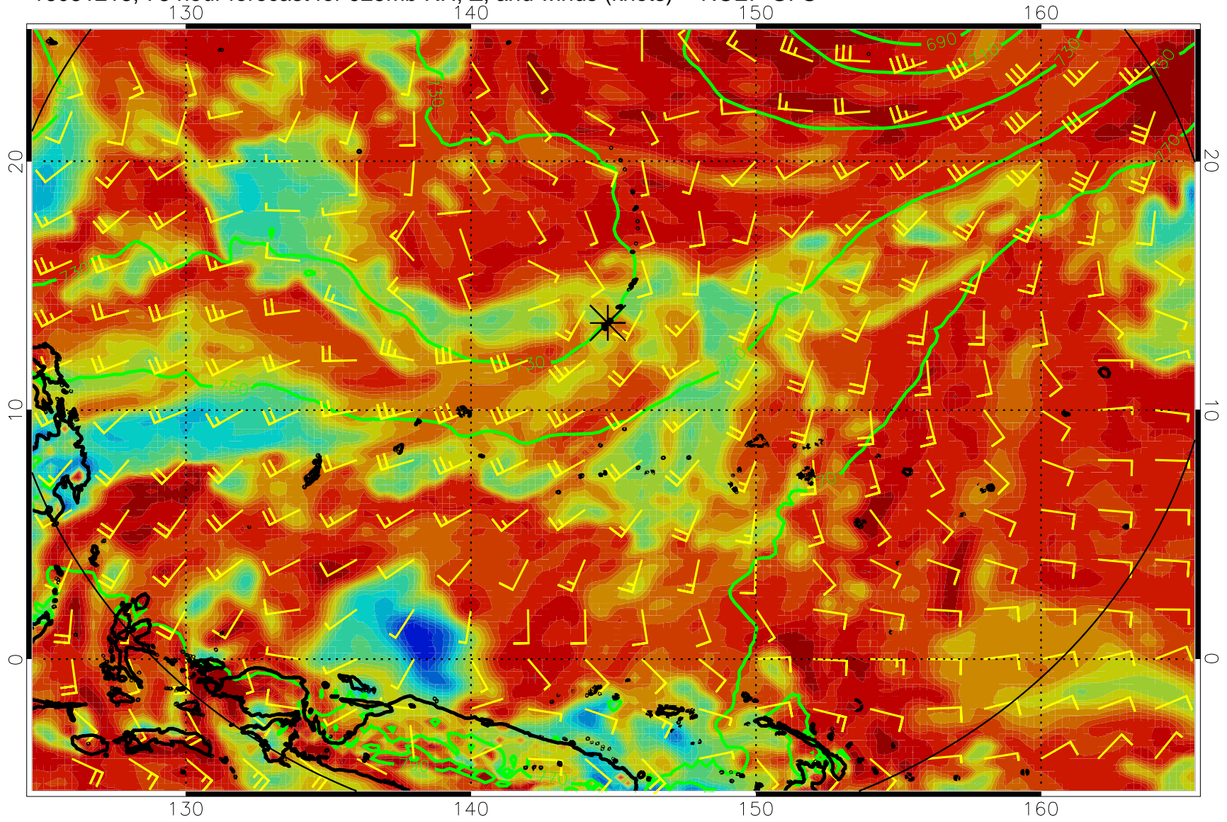
16081218, 78 hour forecast for 925mb RH, Z, and winds (knots) -- NCEP GFS
