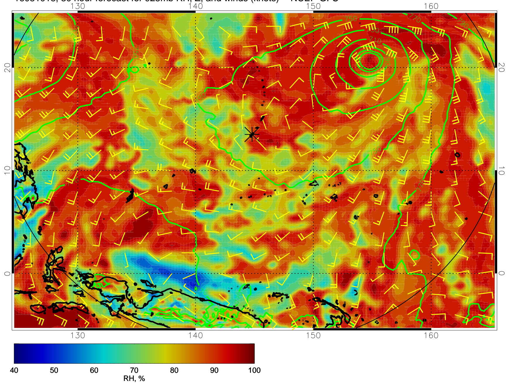
16081018, 30 hour forecast for 925mb RH, Z, and winds (knots) -- NCEP GFS
