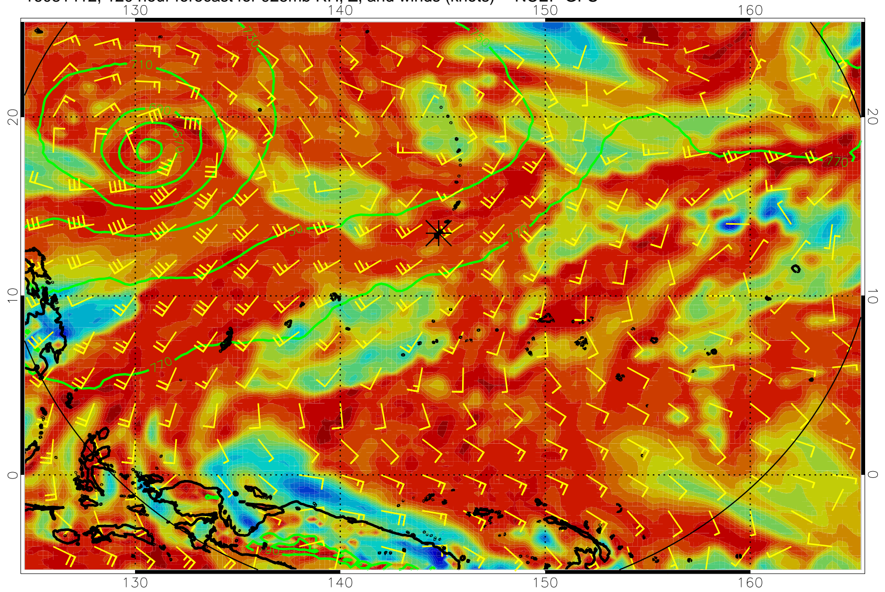
16081412, 120 hour forecast for 925mb RH, Z, and winds (knots) -- NCEP GFS
