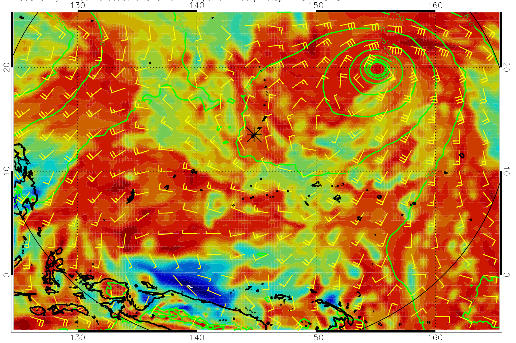
16081012, 24 hour forecast for 925mb RH, Z, and winds (knots) -- NCEP GFS
