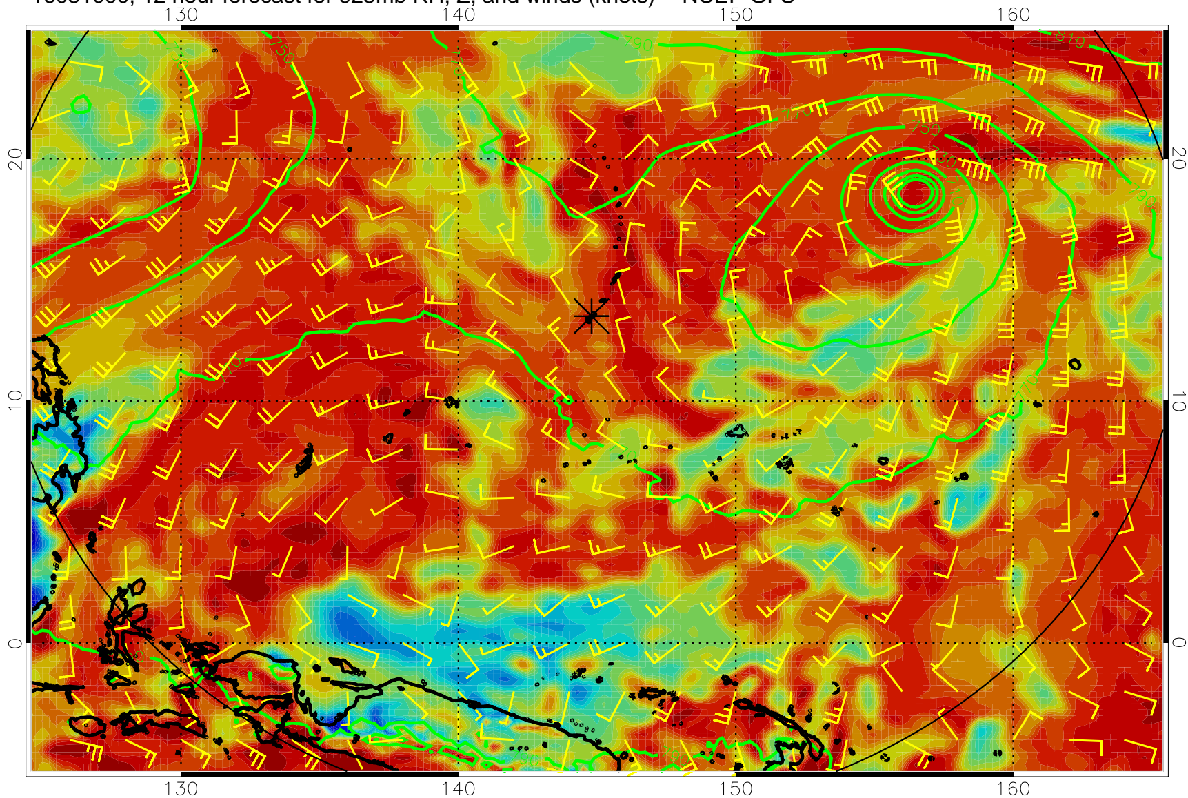
16081000, 12 hour forecast for 925mb RH, Z, and winds (knots) -- NCEP GFS
