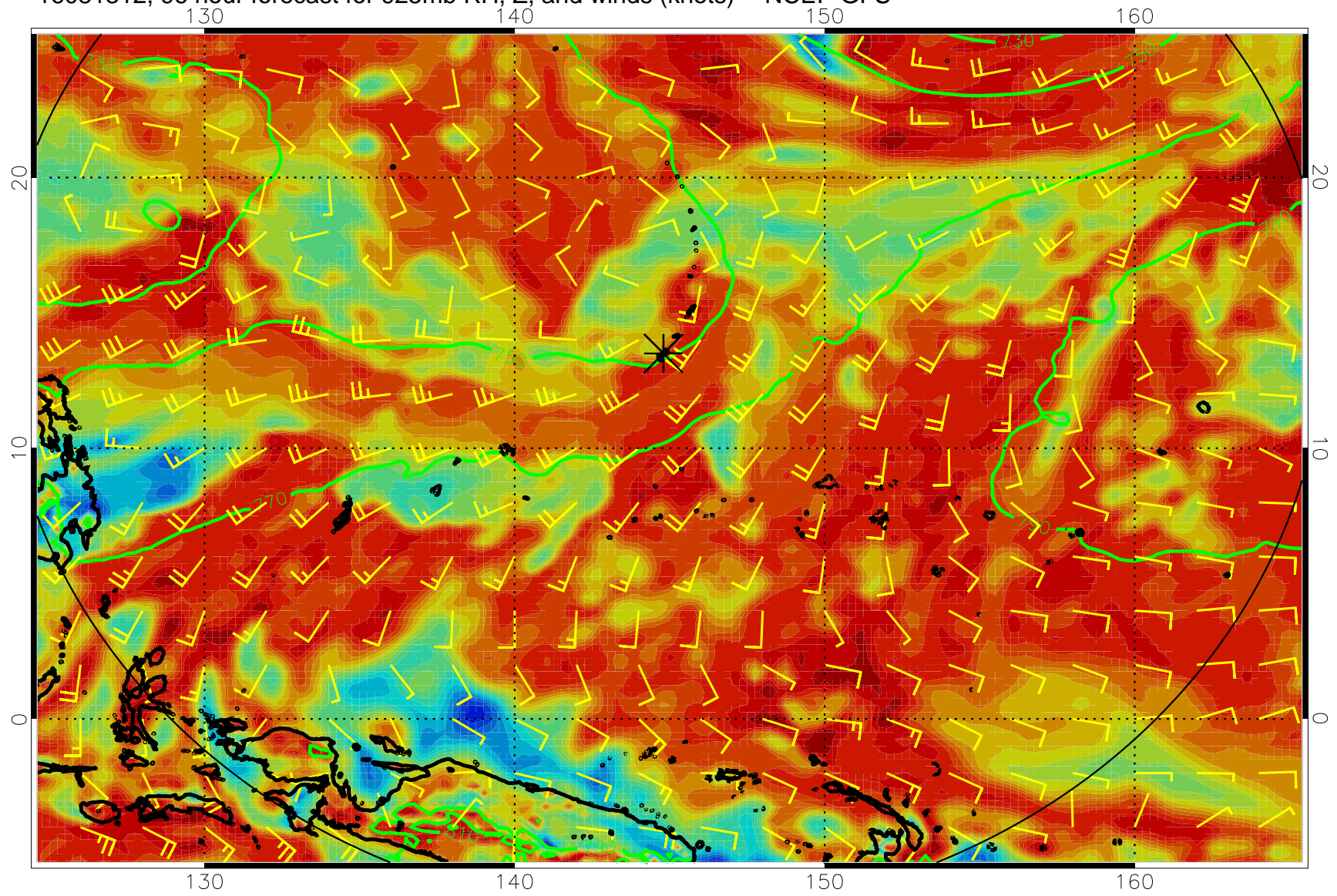
16081312, 96 hour forecast for 925mb RH, Z, and winds (knots) -- NCEP GFS
