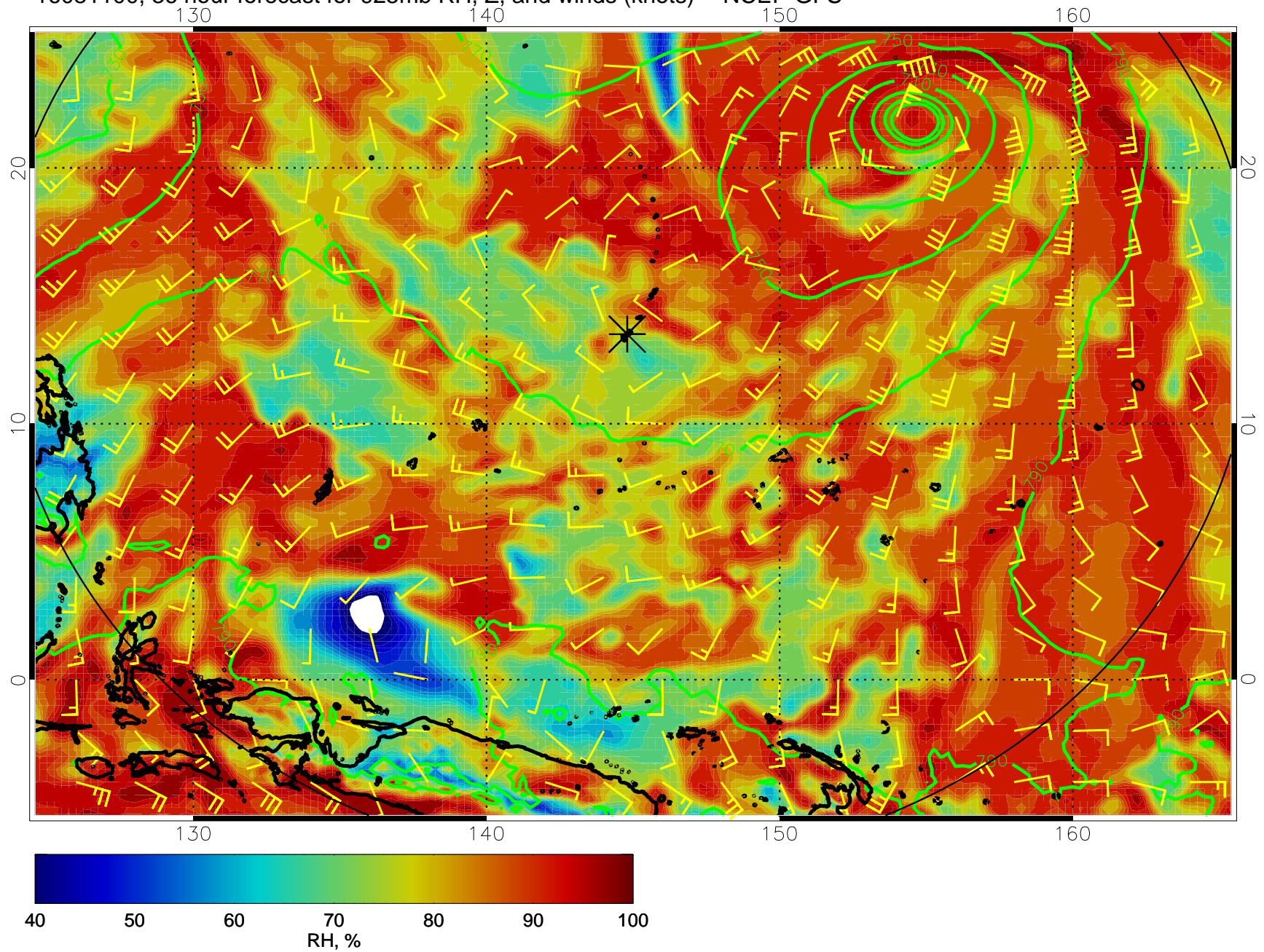
16081100, 36 hour forecast for 925mb RH, Z, and winds (knots) -- NCEP GFS
