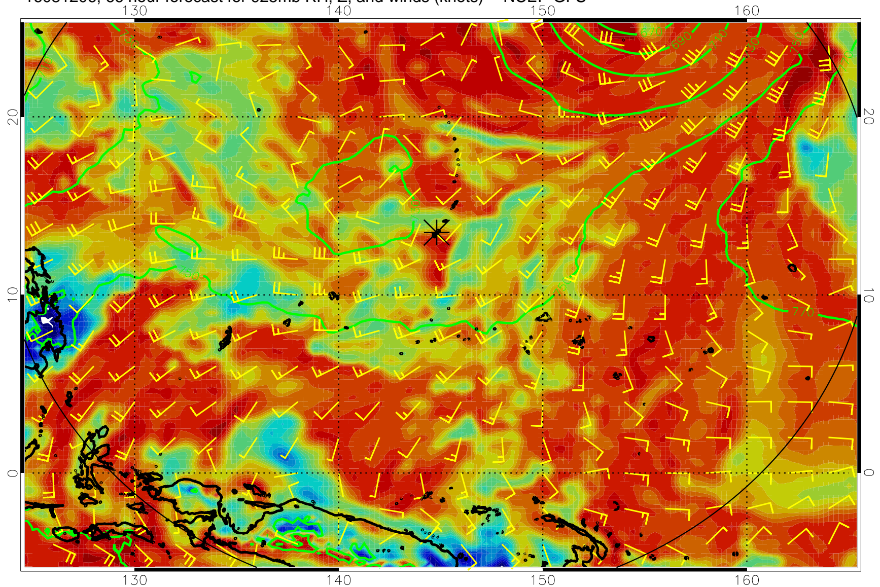
16081206, 66 hour forecast for 925mb RH, Z, and winds (knots) -- NCEP GFS
