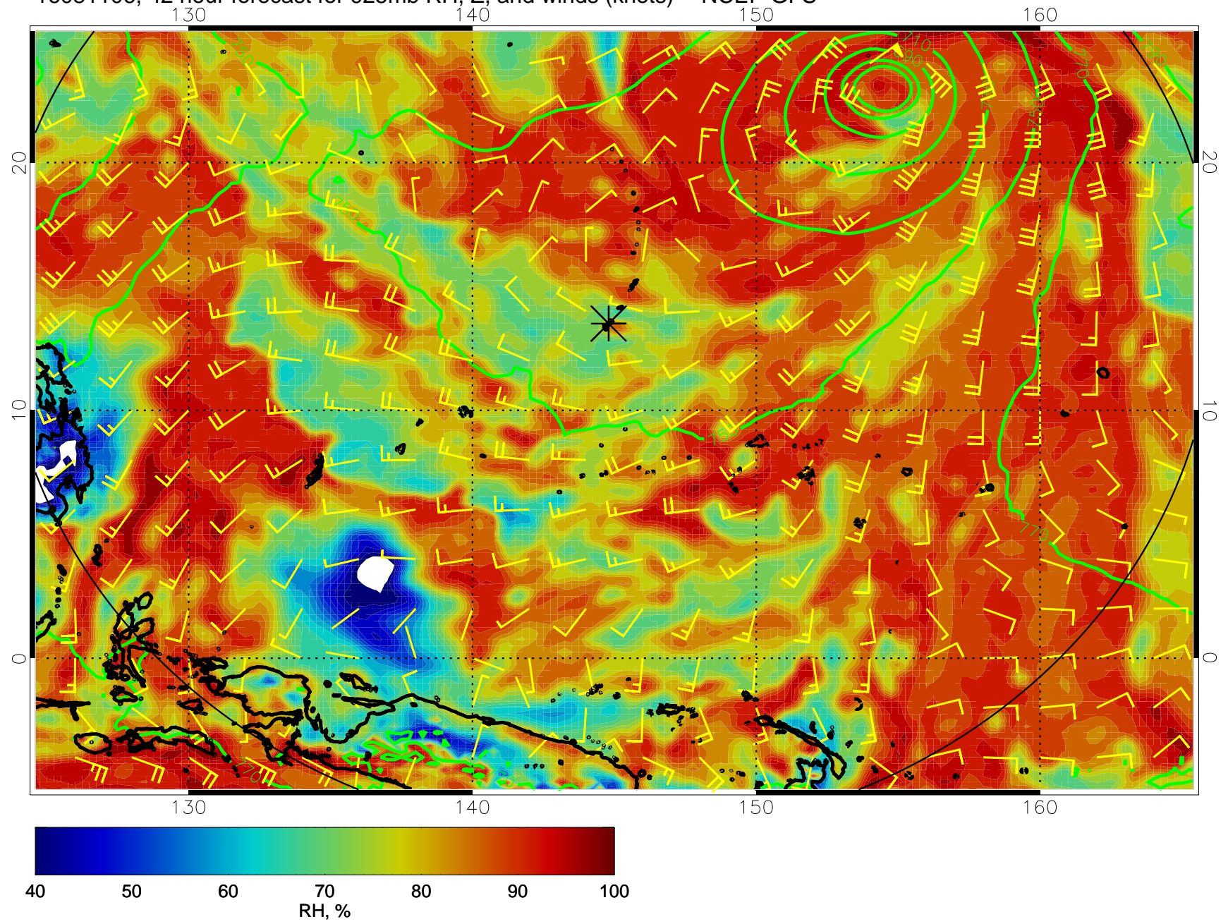
16081106, 42 hour forecast for 925mb RH, Z, and winds (knots) -- NCEP GFS
