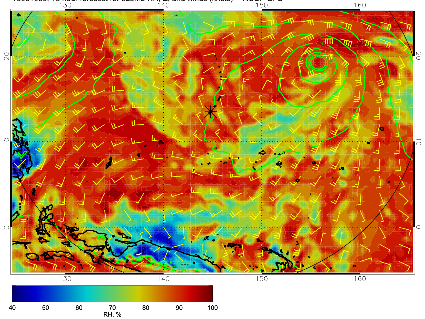
16081006, 18 hour forecast for 925mb RH, Z, and winds (knots) -- NCEP GFS
