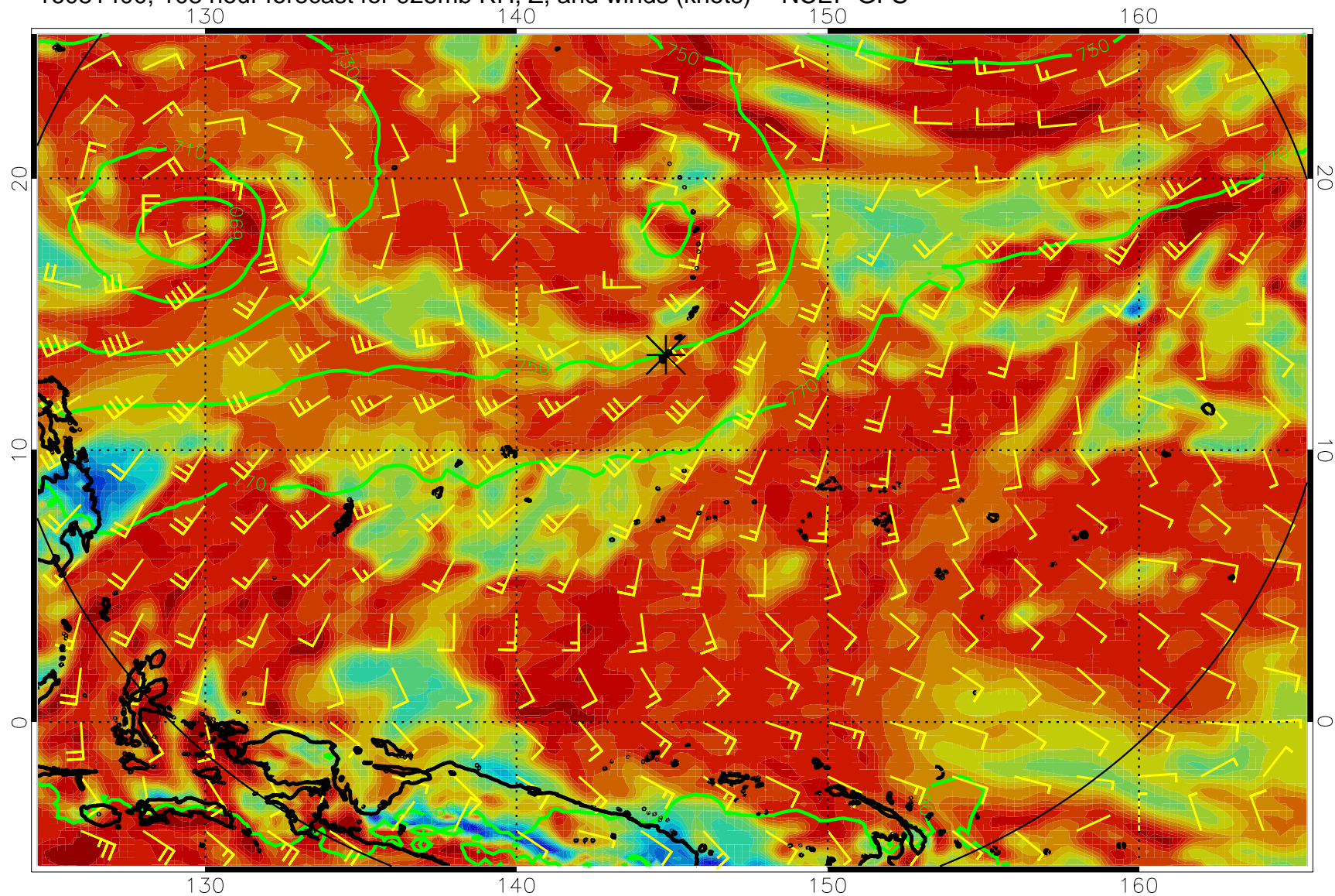
16081400, 108 hour forecast for 925mb RH, Z, and winds (knots) -- NCEP GFS
