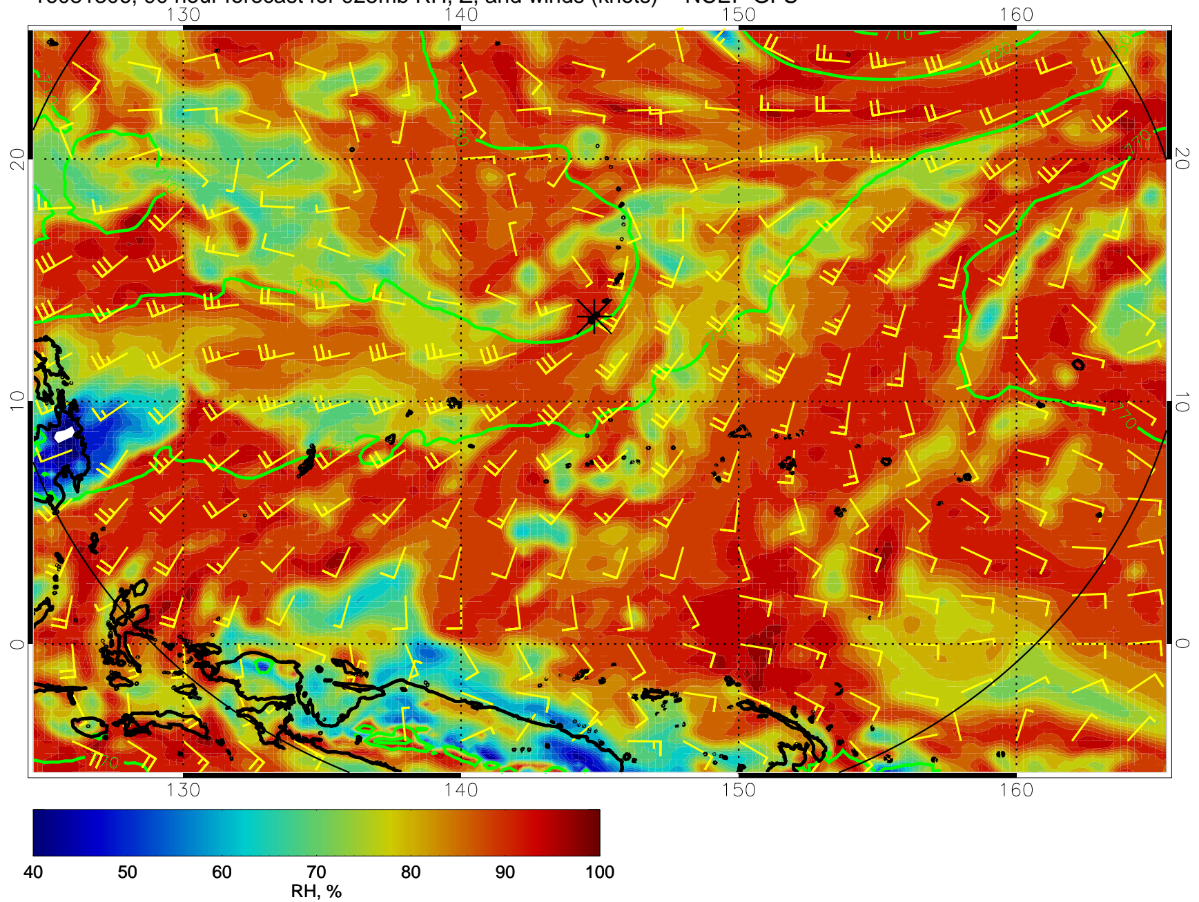
16081306, 90 hour forecast for 925mb RH, Z, and winds (knots) -- NCEP GFS
