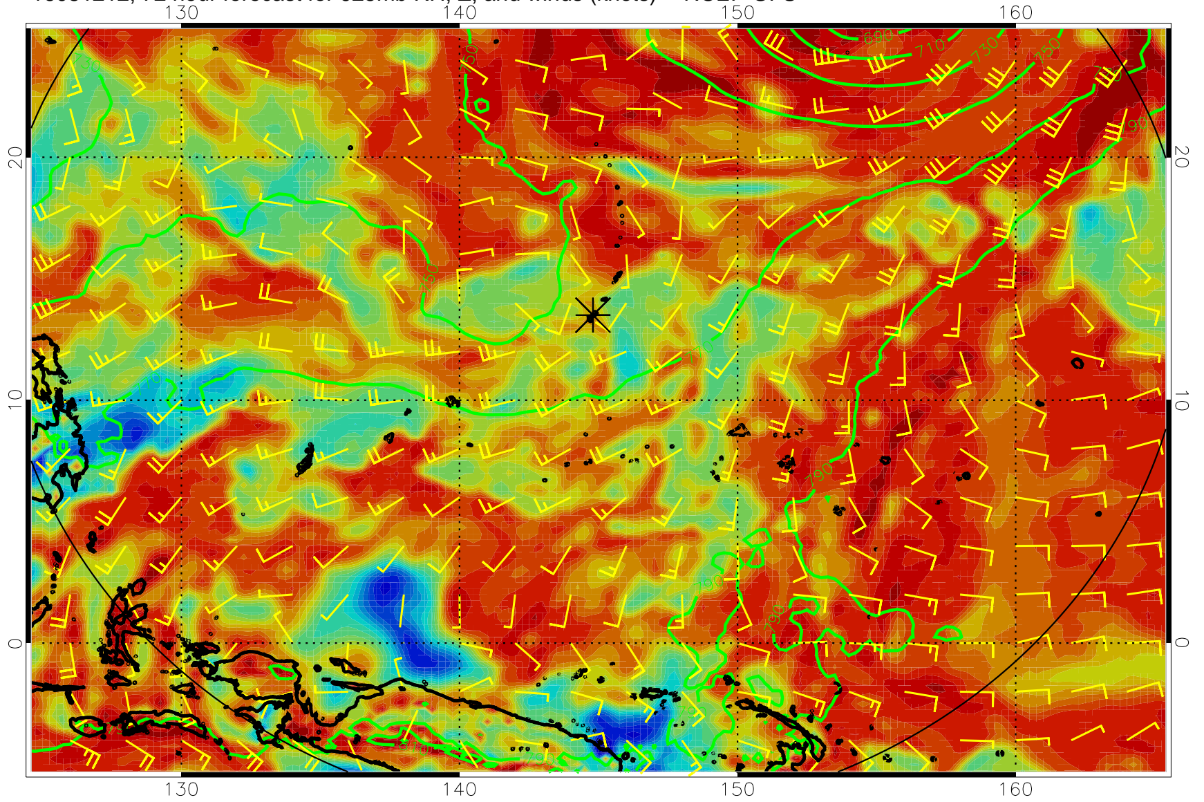
16081212, 72 hour forecast for 925mb RH, Z, and winds (knots) -- NCEP GFS
