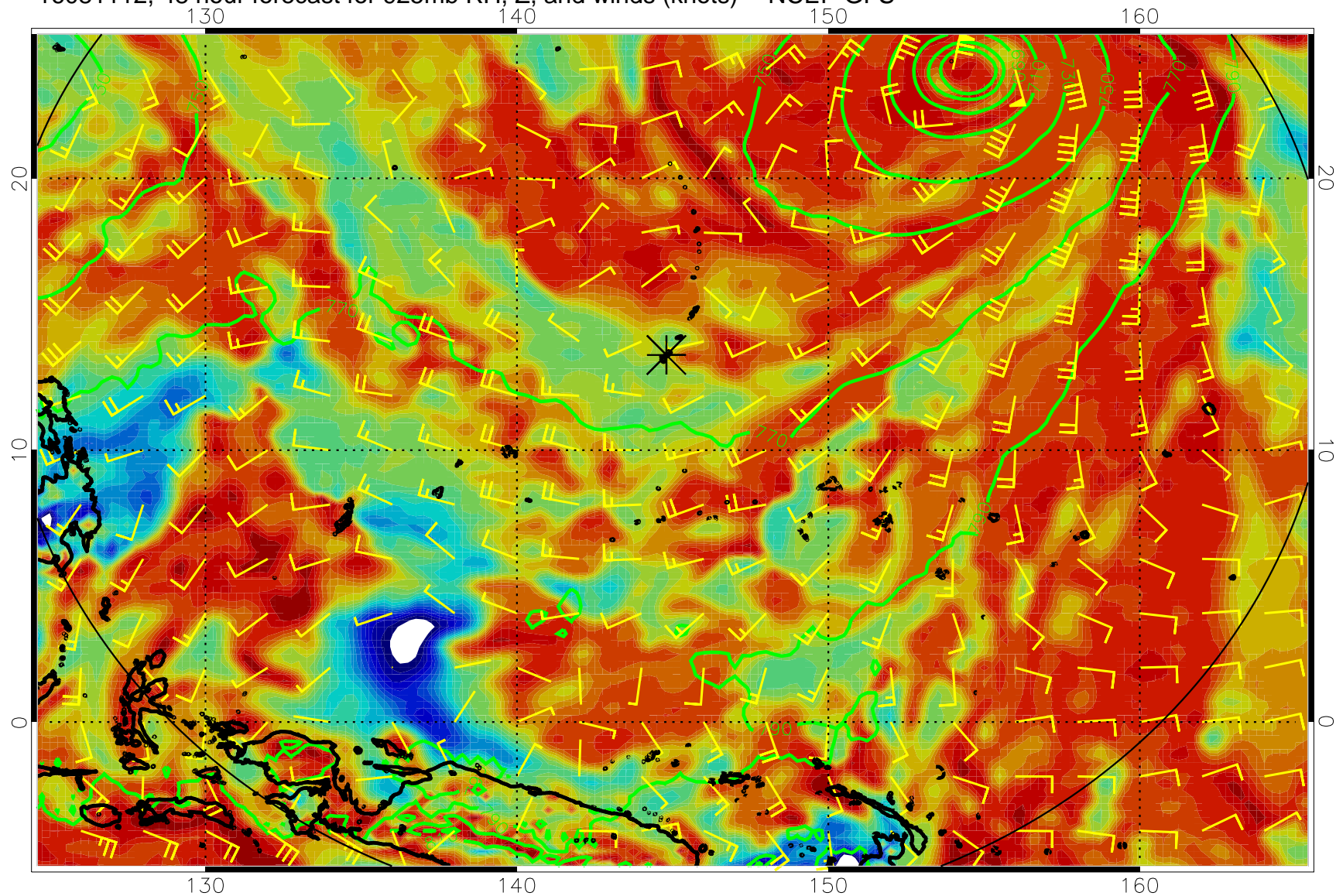
16081112, 48 hour forecast for 925mb RH, Z, and winds (knots) -- NCEP GFS
