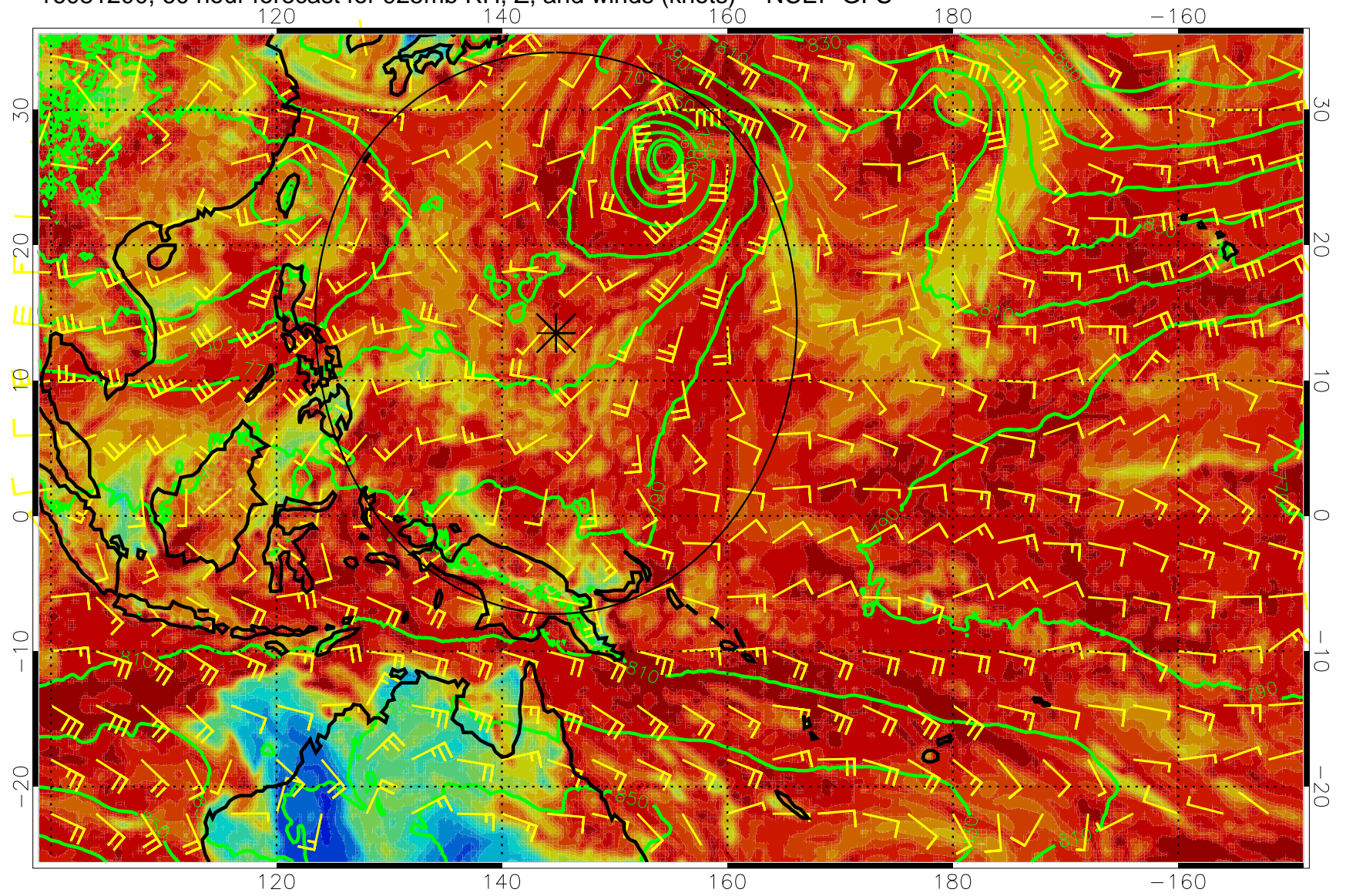
16081200, 60 hour forecast for 925mb RH, Z, and winds (knots) -- NCEP GFS
