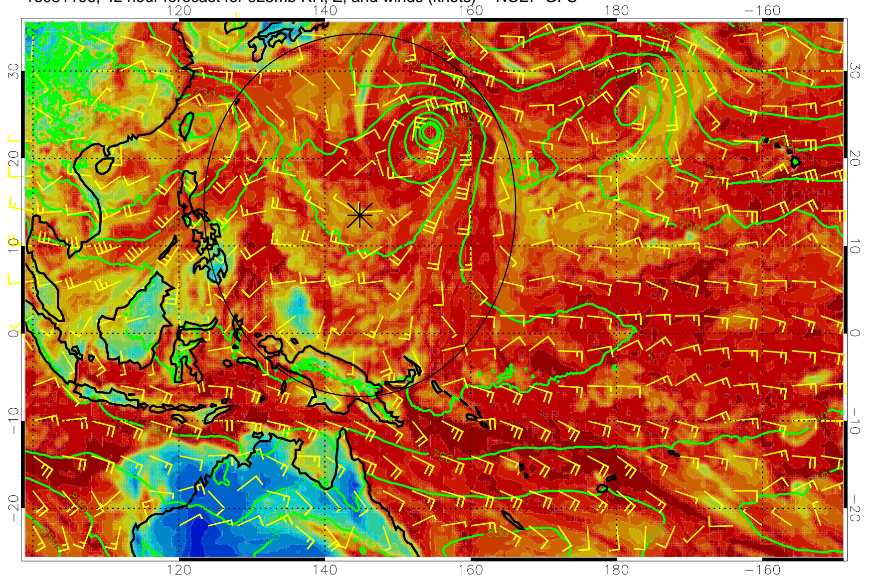
16081106, 42 hour forecast for 925mb RH, Z, and winds (knots) -- NCEP GFS
