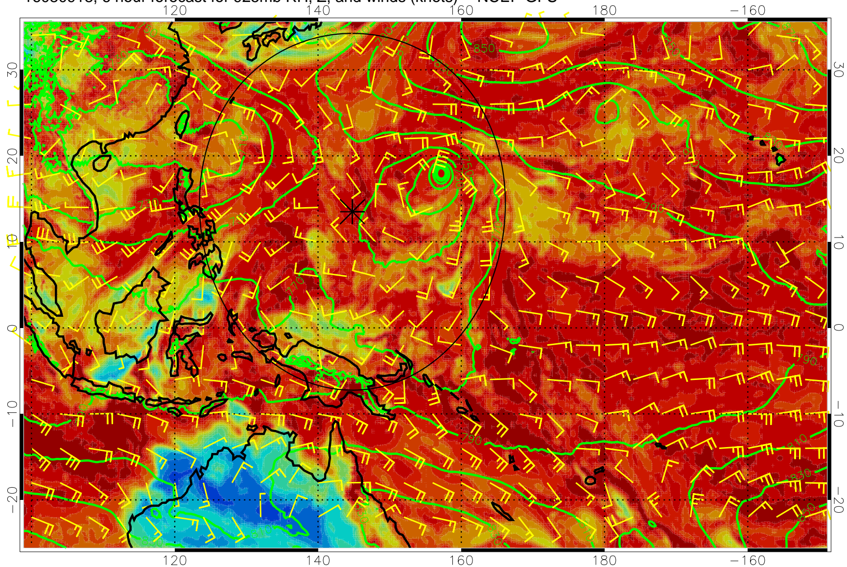
16080918, 6 hour forecast for 925mb RH, Z, and winds (knots) -- NCEP GFS
