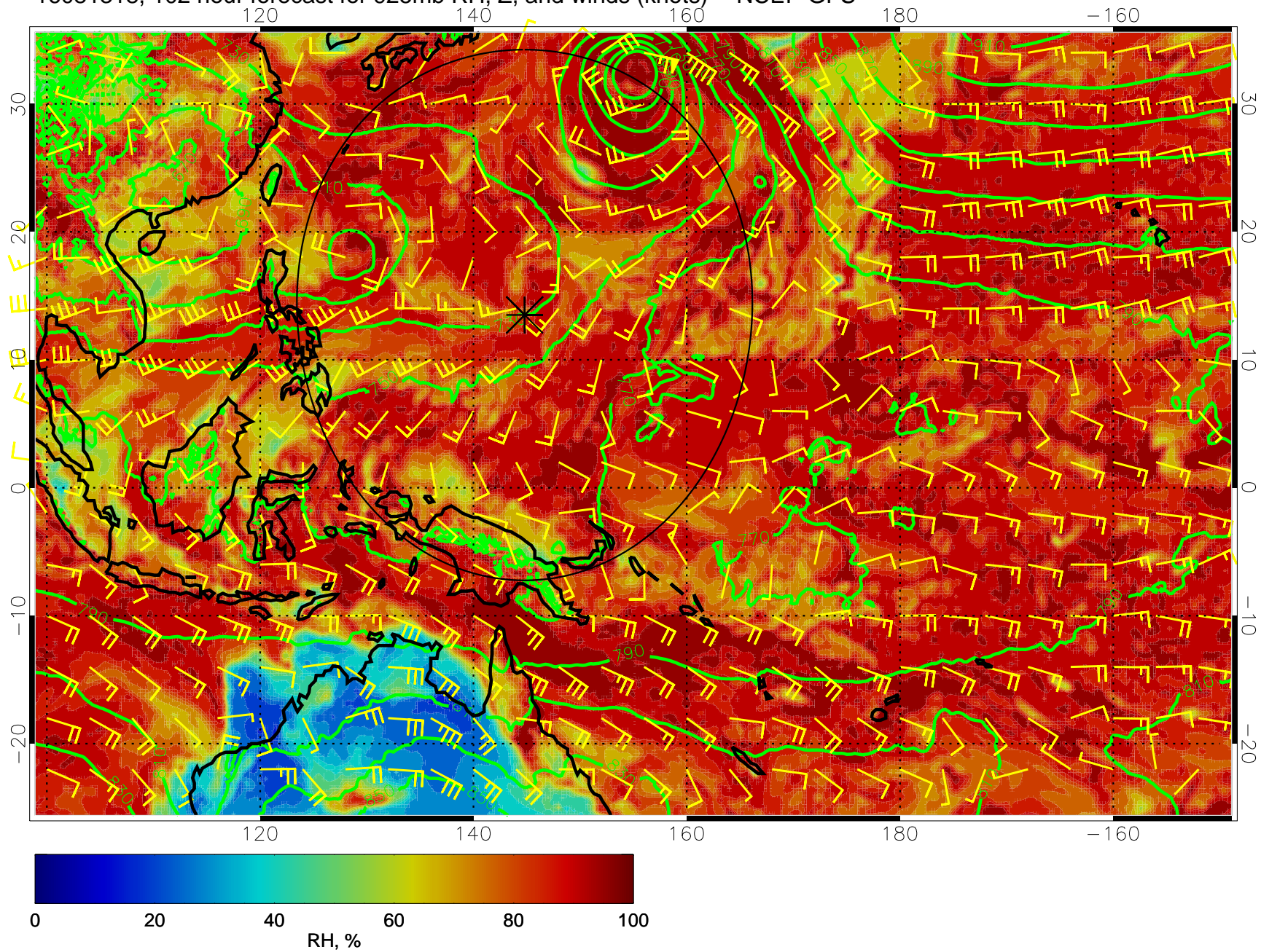
16081318, 102 hour forecast for 925mb RH, Z, and winds (knots) -- NCEP GFS
