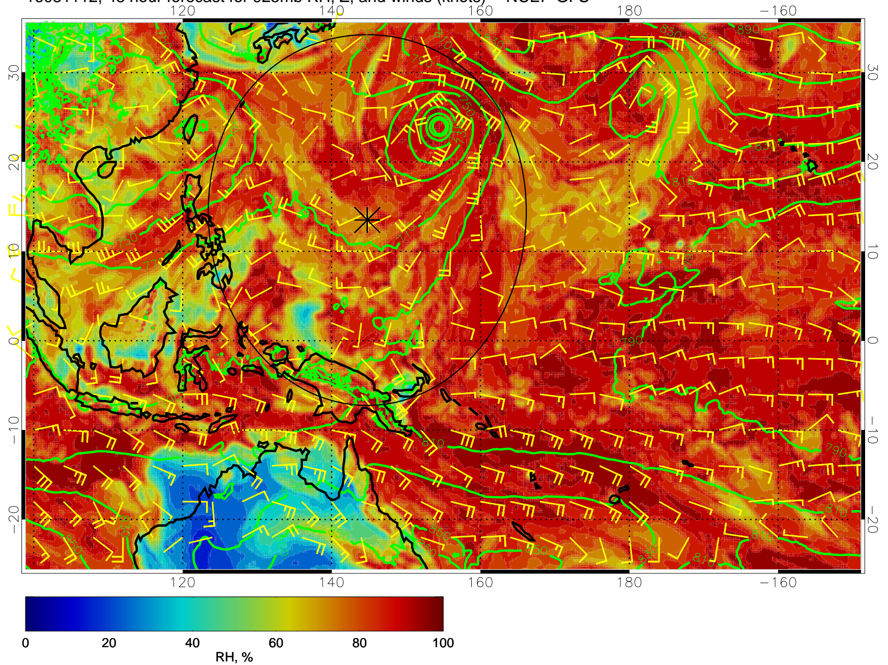
16081112, 48 hour forecast for 925mb RH, Z, and winds (knots) -- NCEP GFS
