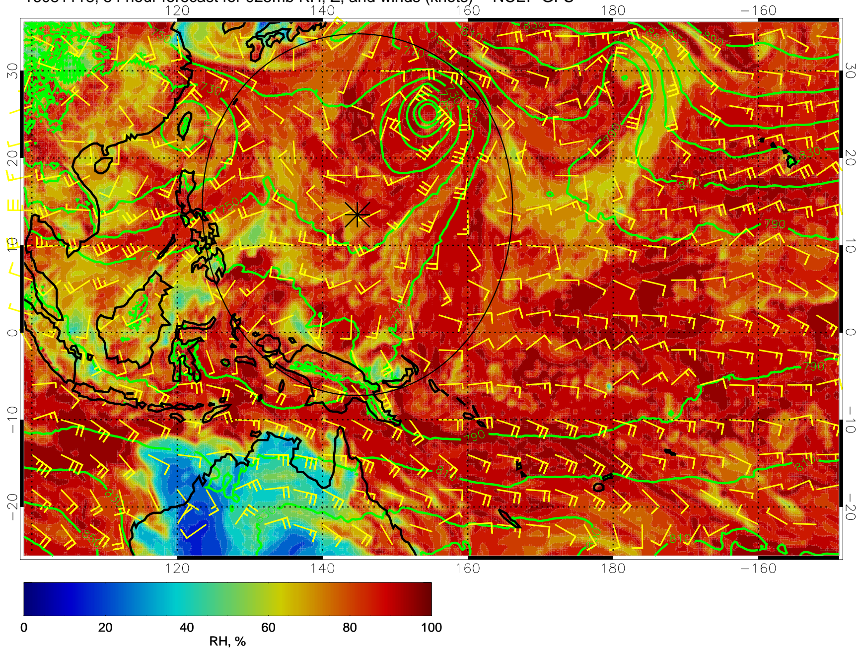
16081118, 54 hour forecast for 925mb RH, Z, and winds (knots) -- NCEP GFS
