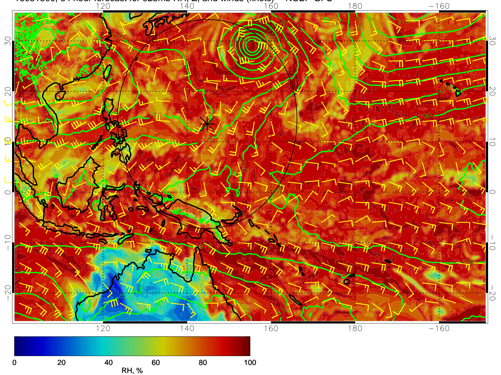
16081300, 84 hour forecast for 925mb RH, Z, and winds (knots) -- NCEP GFS
