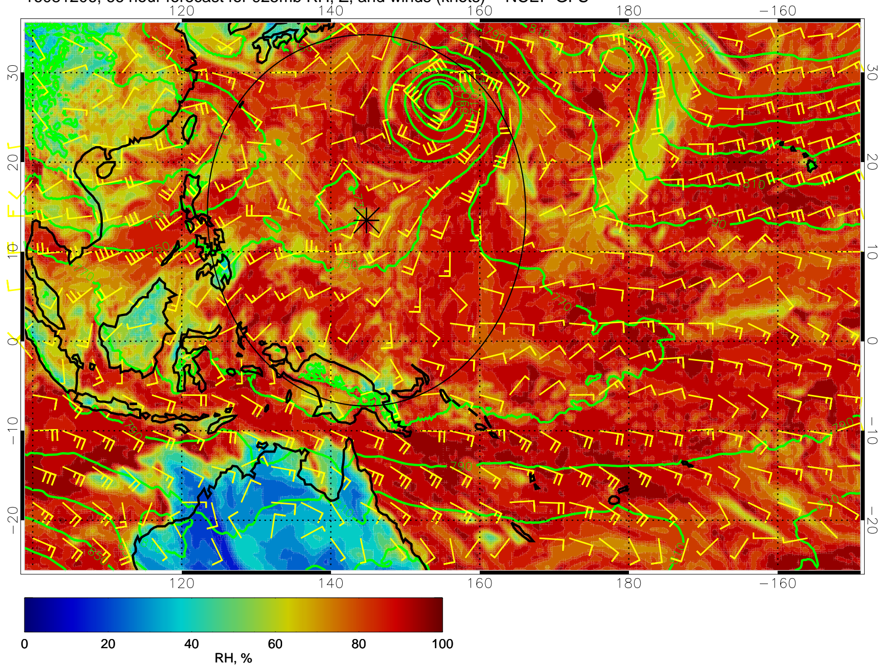
16081206, 66 hour forecast for 925mb RH, Z, and winds (knots) -- NCEP GFS
