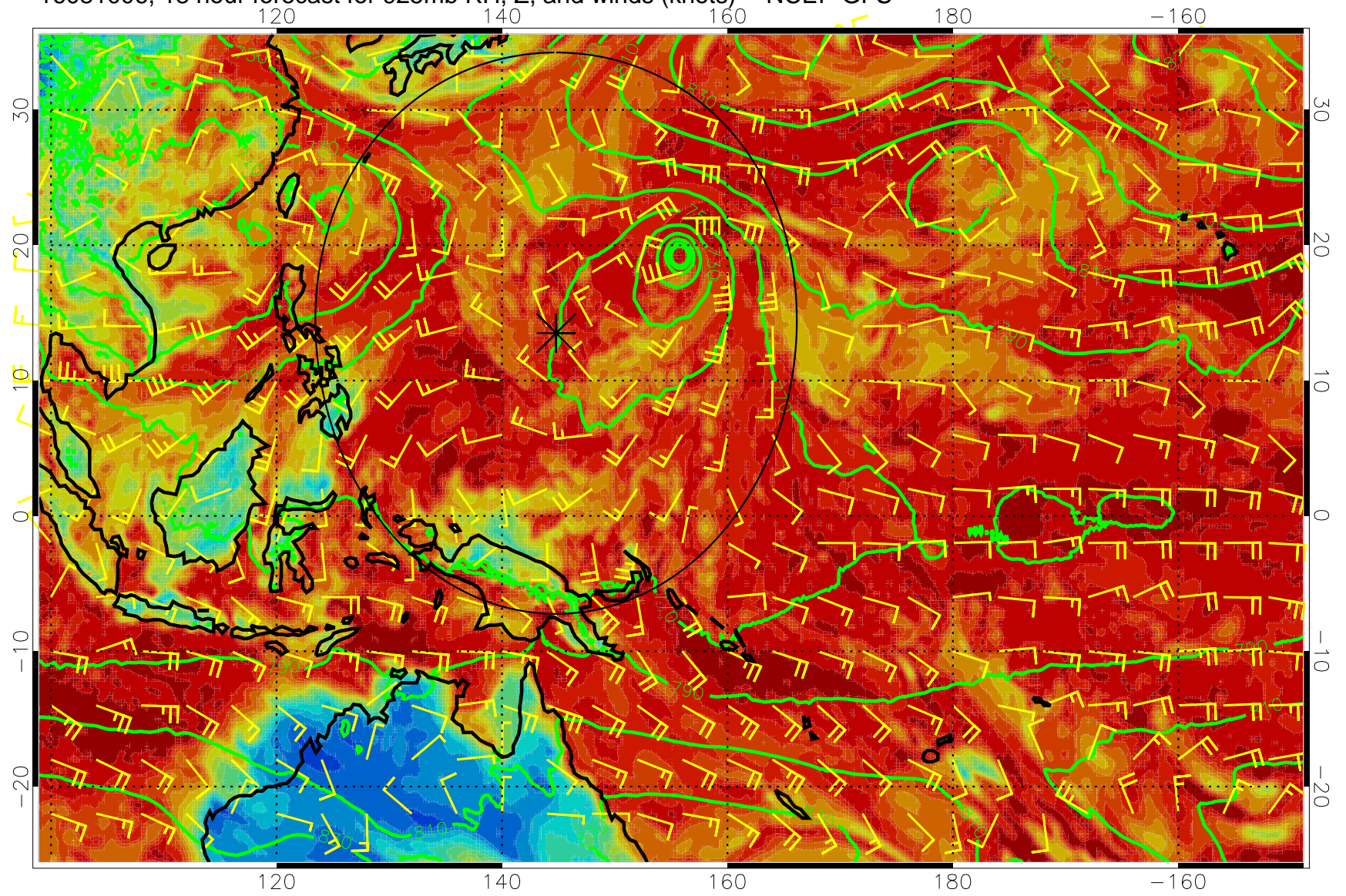
16081006, 18 hour forecast for 925mb RH, Z, and winds (knots) -- NCEP GFS
