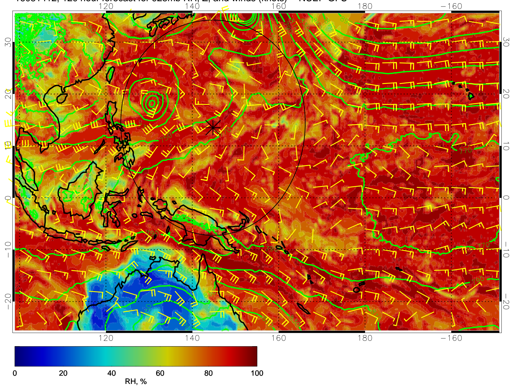
16081412, 120 hour forecast for 925mb RH, Z, and winds (knots) -- NCEP GFS
