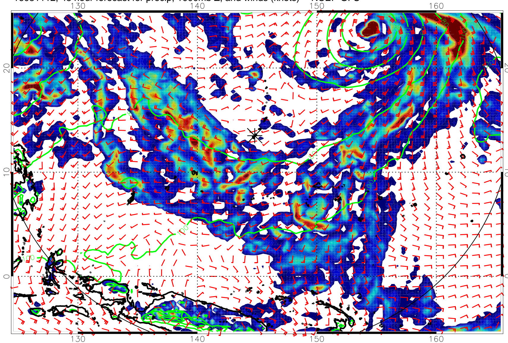
16081112, 48 hour forecast for precip, 1000mb Z, and winds (knots) -- NCEP GFS
