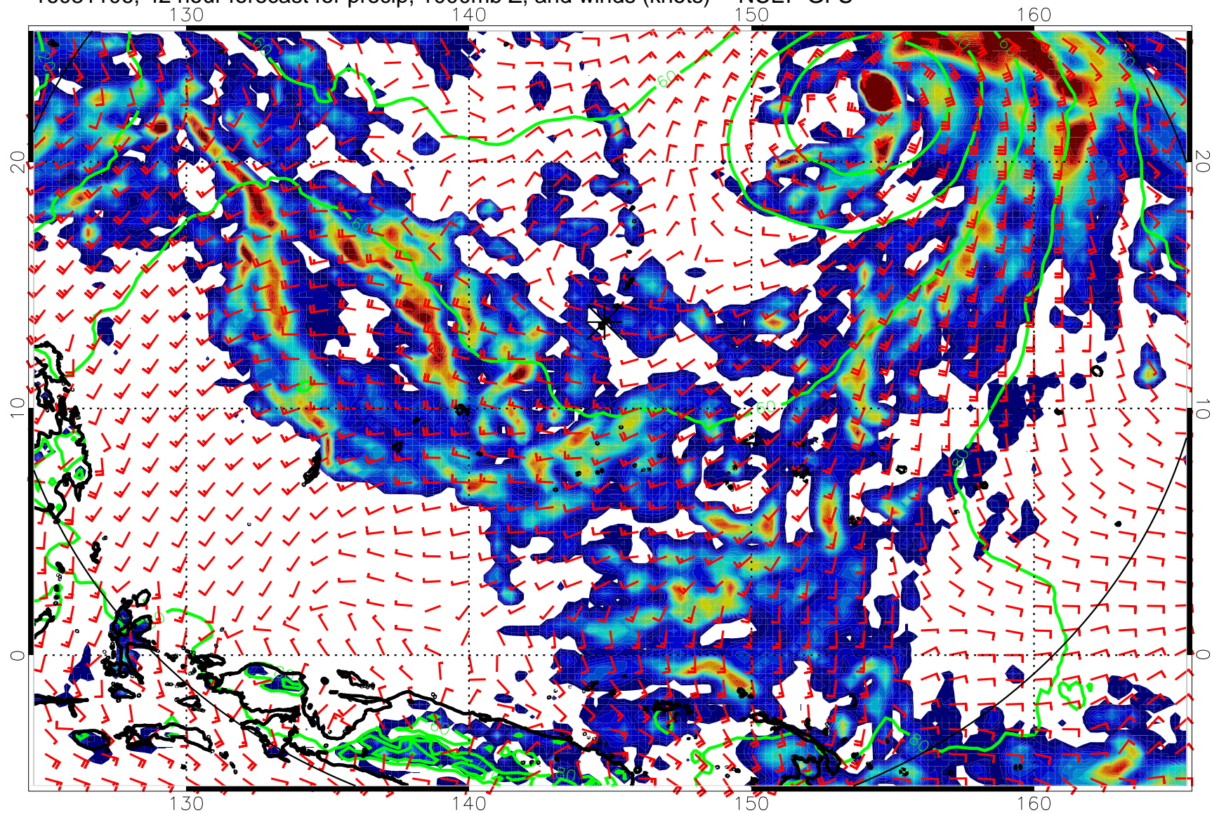
16081106, 42 hour forecast for precip, 1000mb Z, and winds (knots) -- NCEP GFS
