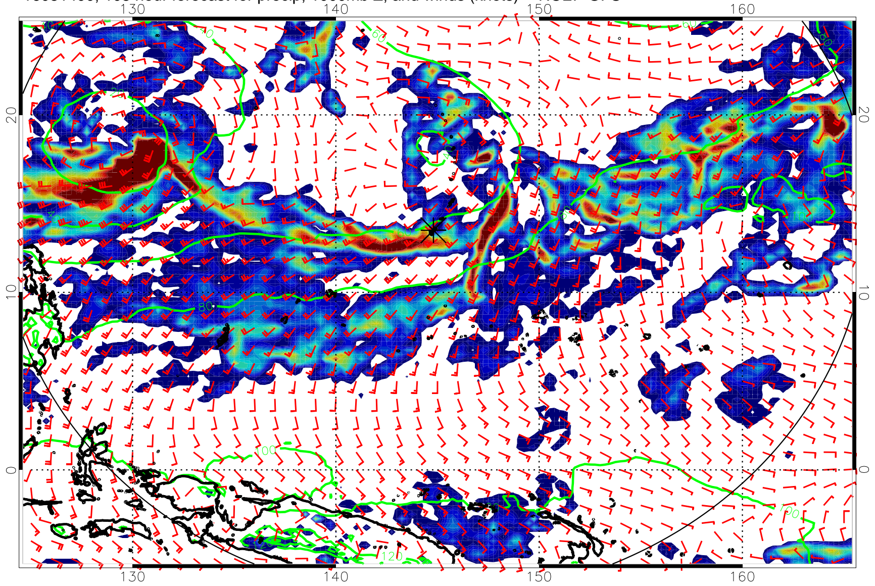
16081400, 108 hour forecast for precip, 1000mb Z, and winds (knots) -- NCEP GFS
