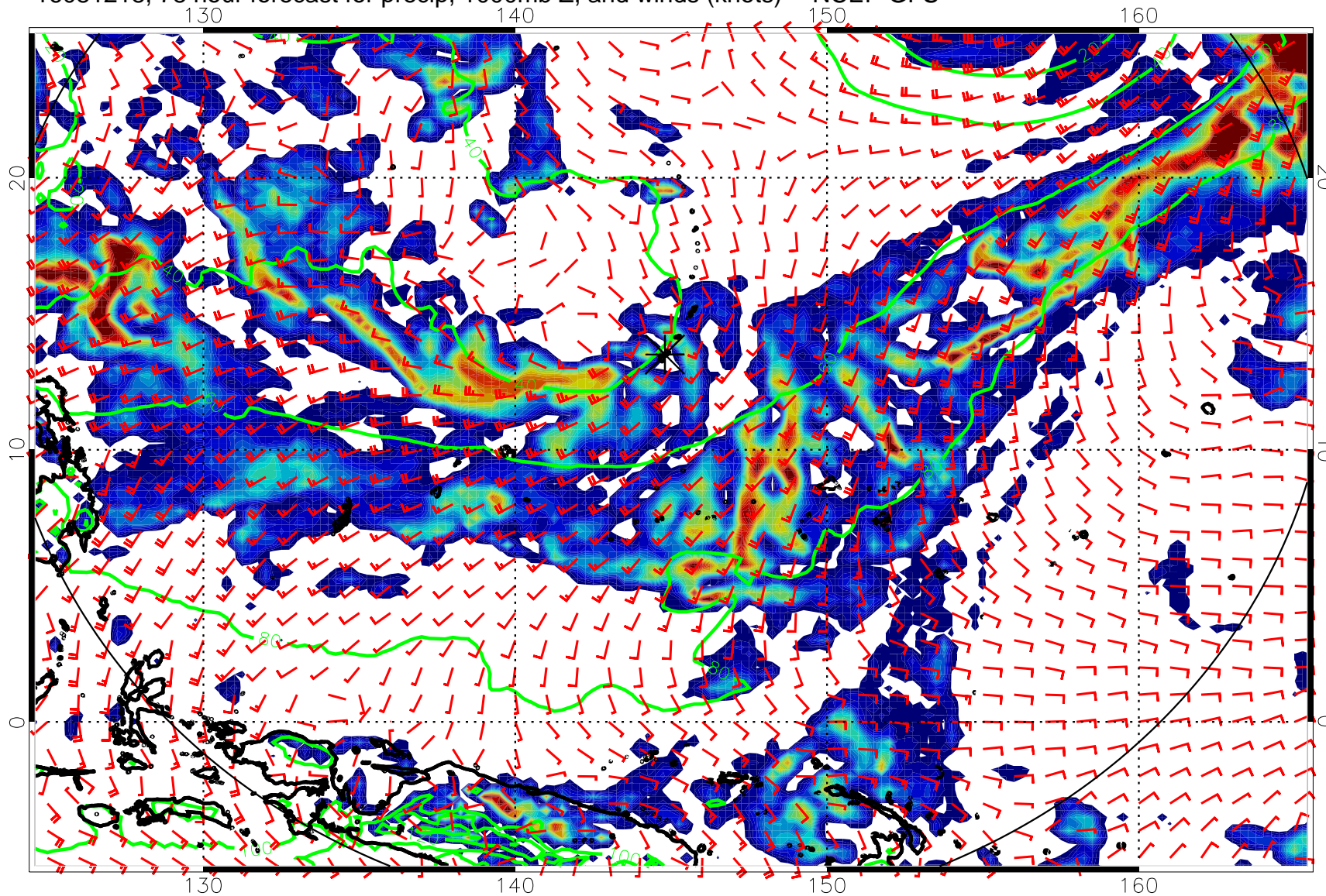
16081218, 78 hour forecast for precip, 1000mb Z, and winds (knots) -- NCEP GFS
