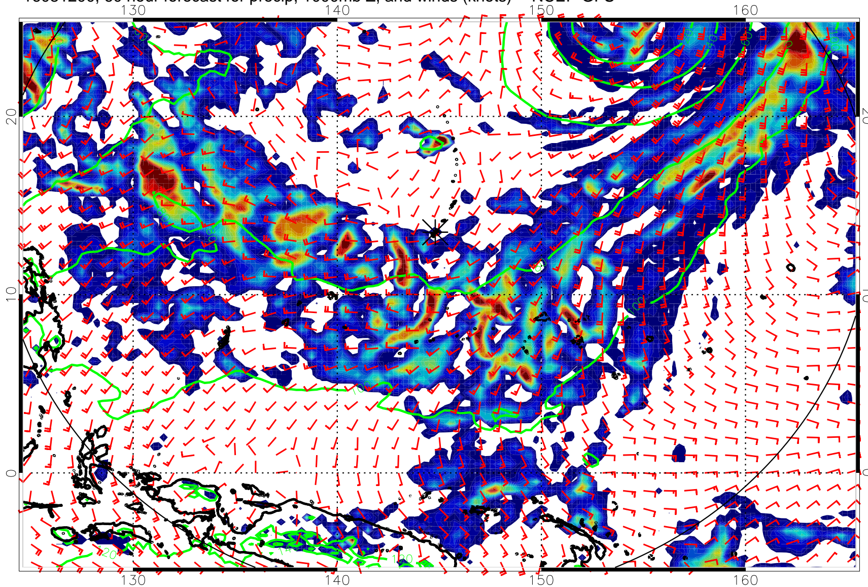
16081200, 60 hour forecast for precip, 1000mb Z, and winds (knots) -- NCEP GFS
