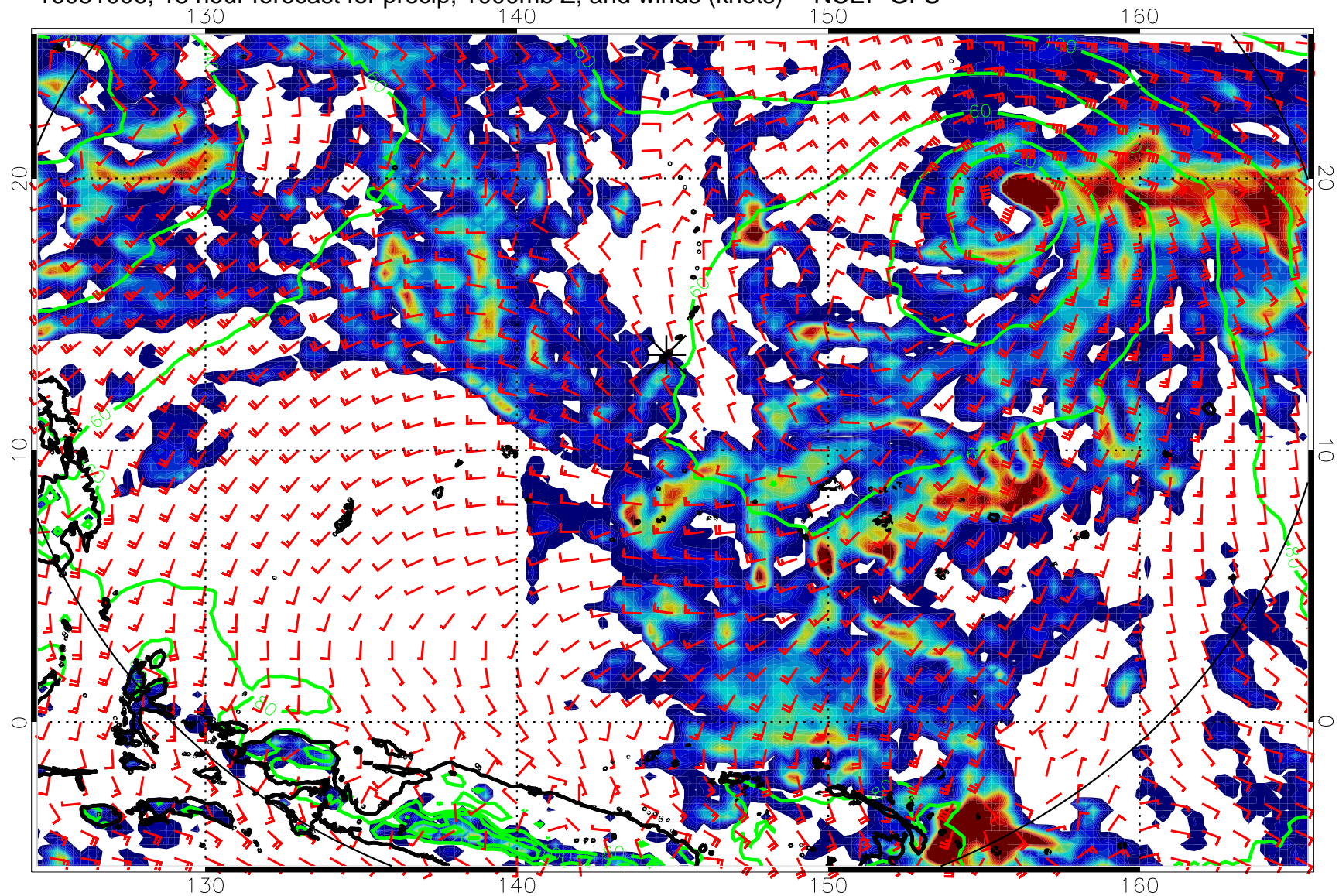
16081006, 18 hour forecast for precip, 1000mb Z, and winds (knots) -- NCEP GFS
