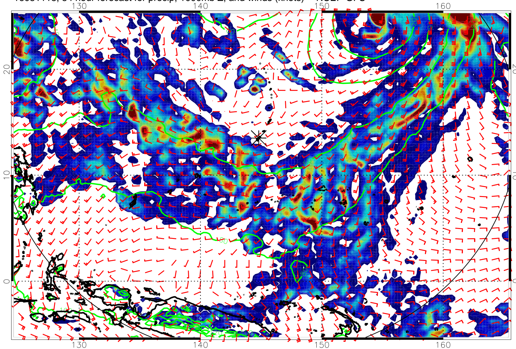
16081118, 54 hour forecast for precip, 1000mb Z, and winds (knots) -- NCEP GFS
