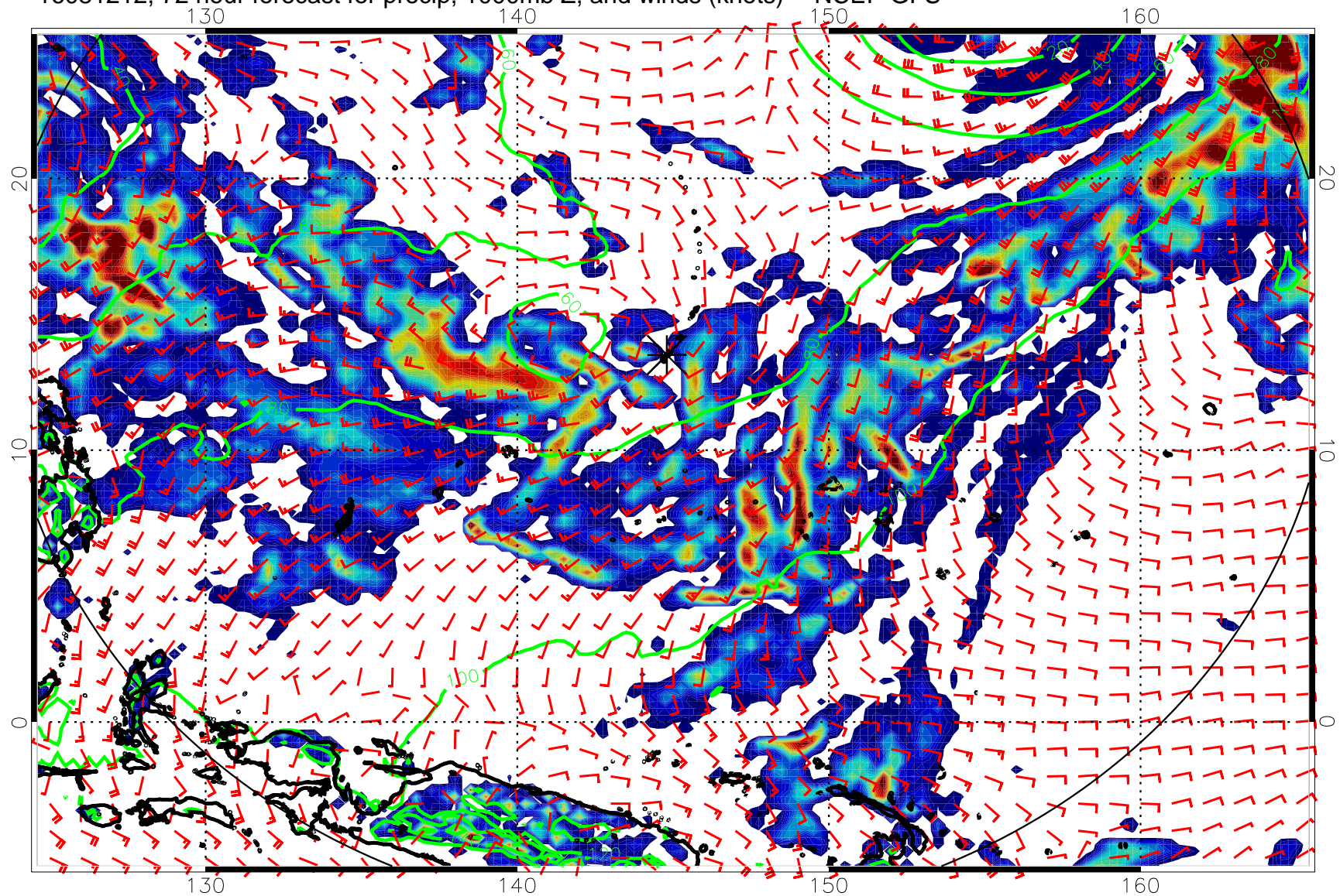
16081212, 72 hour forecast for precip, 1000mb Z, and winds (knots) -- NCEP GFS
