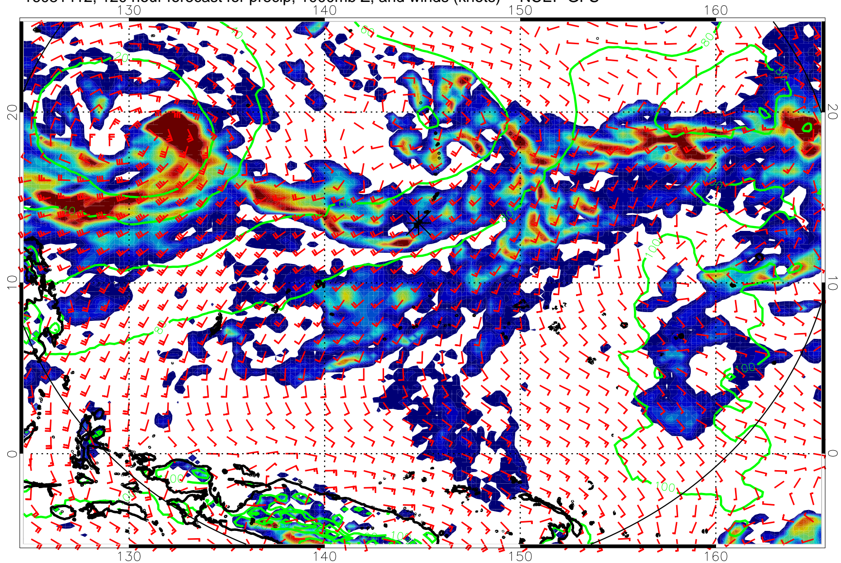
16081412, 120 hour forecast for precip, 1000mb Z, and winds (knots) -- NCEP GFS
