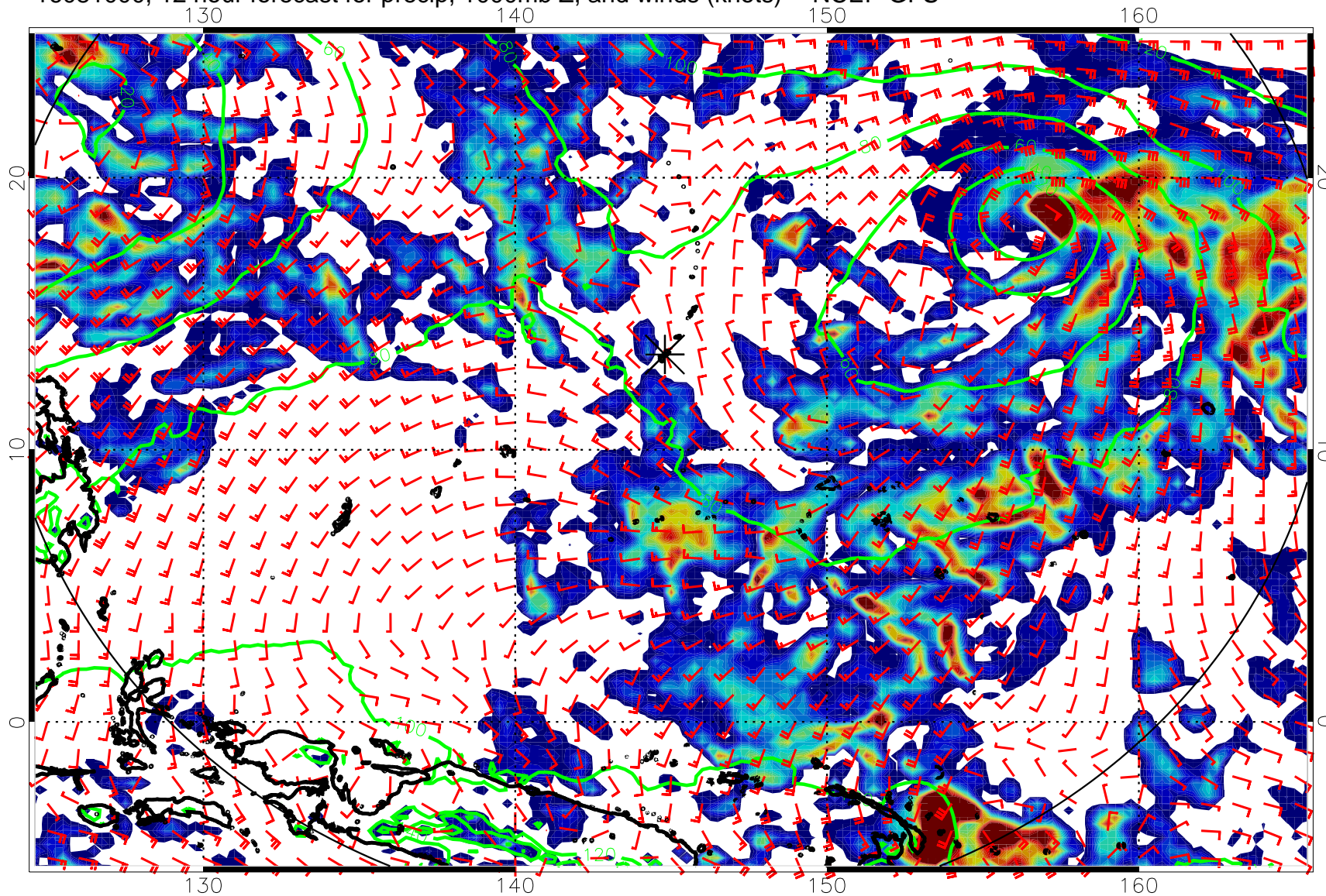
16081000, 12 hour forecast for precip, 1000mb Z, and winds (knots) -- NCEP GFS
