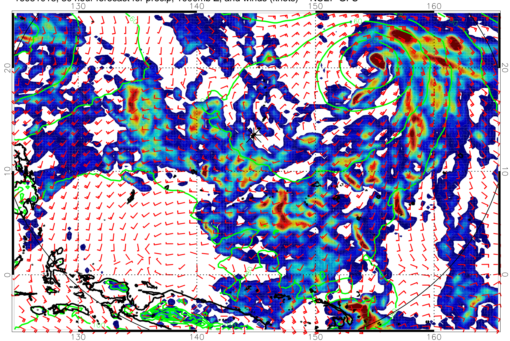
16081018, 30 hour forecast for precip, 1000mb Z, and winds (knots) -- NCEP GFS
