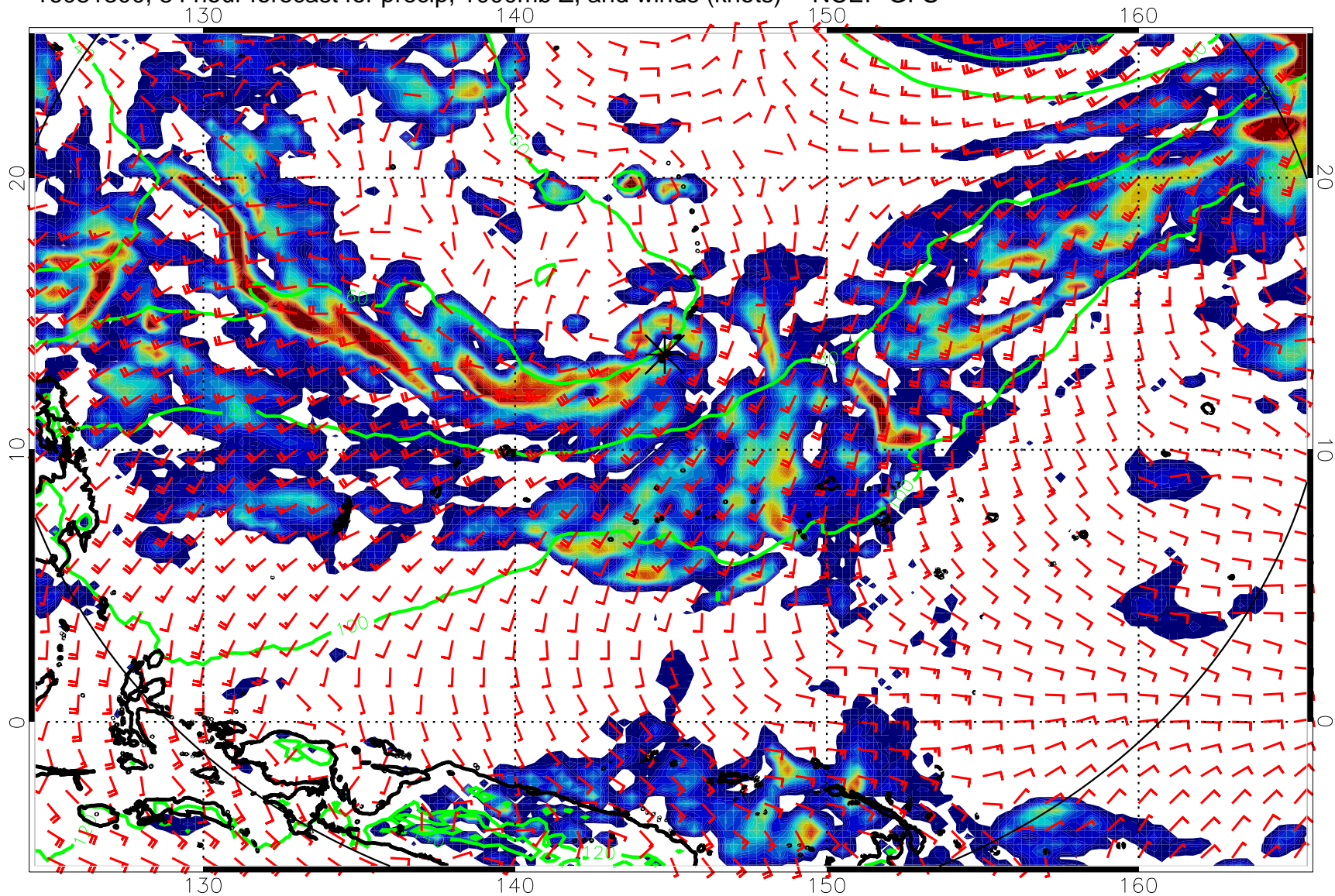
16081300, 84 hour forecast for precip, 1000mb Z, and winds (knots) -- NCEP GFS
