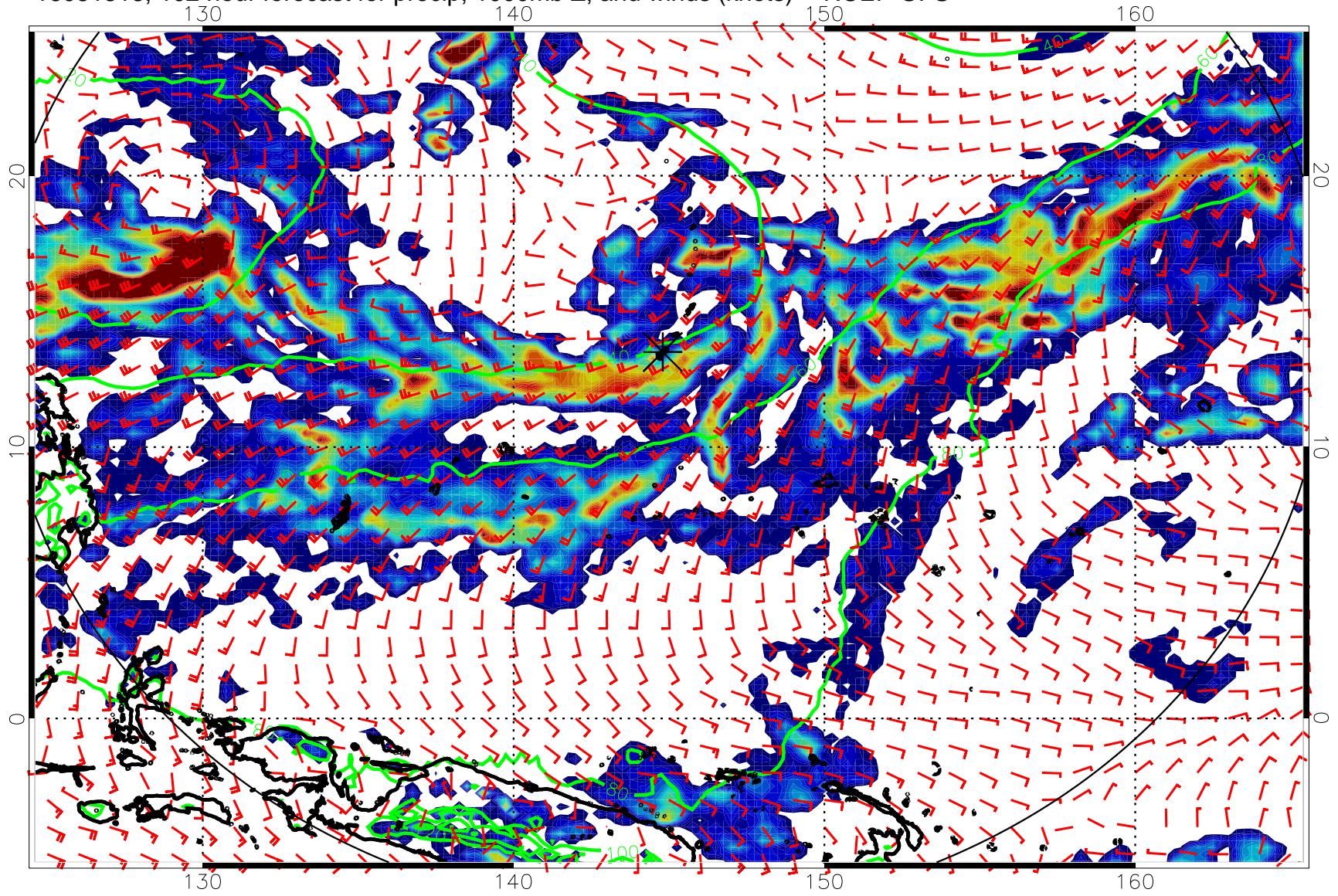
16081318, 102 hour forecast for precip, 1000mb Z, and winds (knots) -- NCEP GFS
