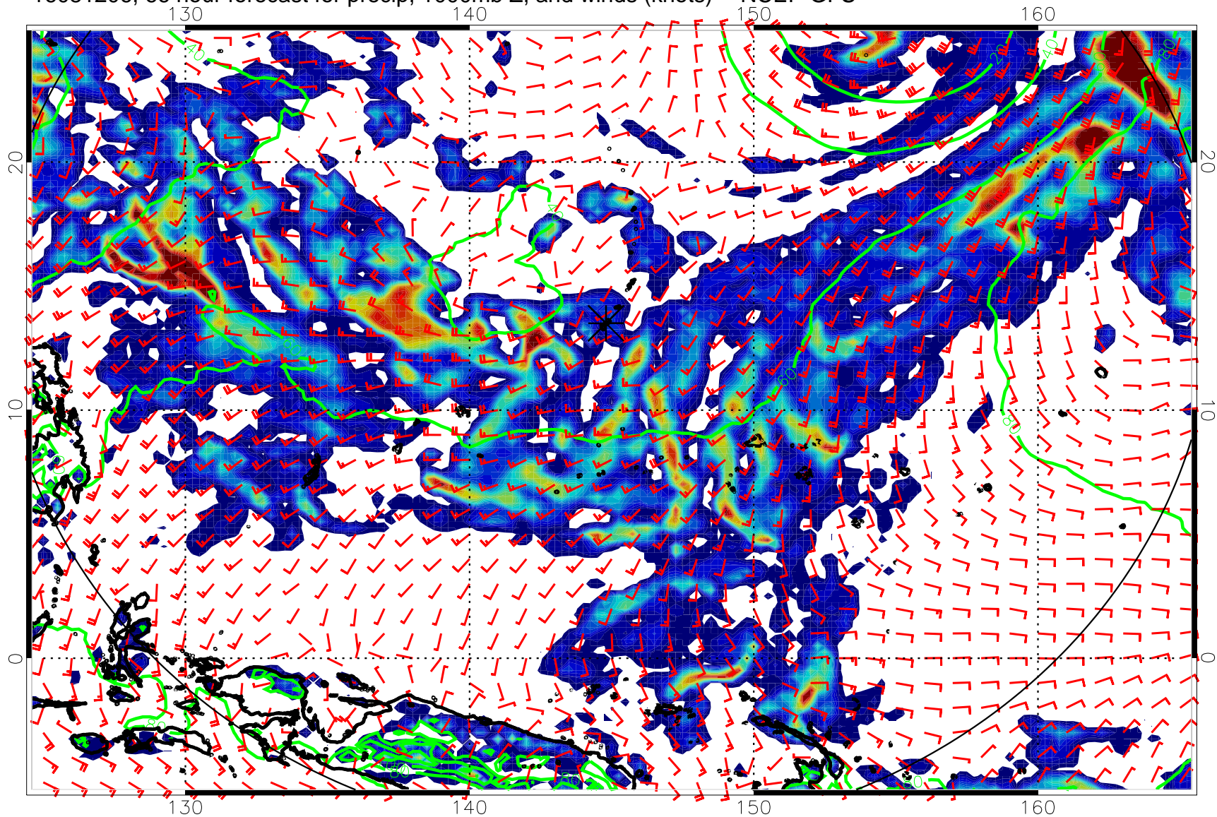
16081206, 66 hour forecast for precip, 1000mb Z, and winds (knots) -- NCEP GFS
