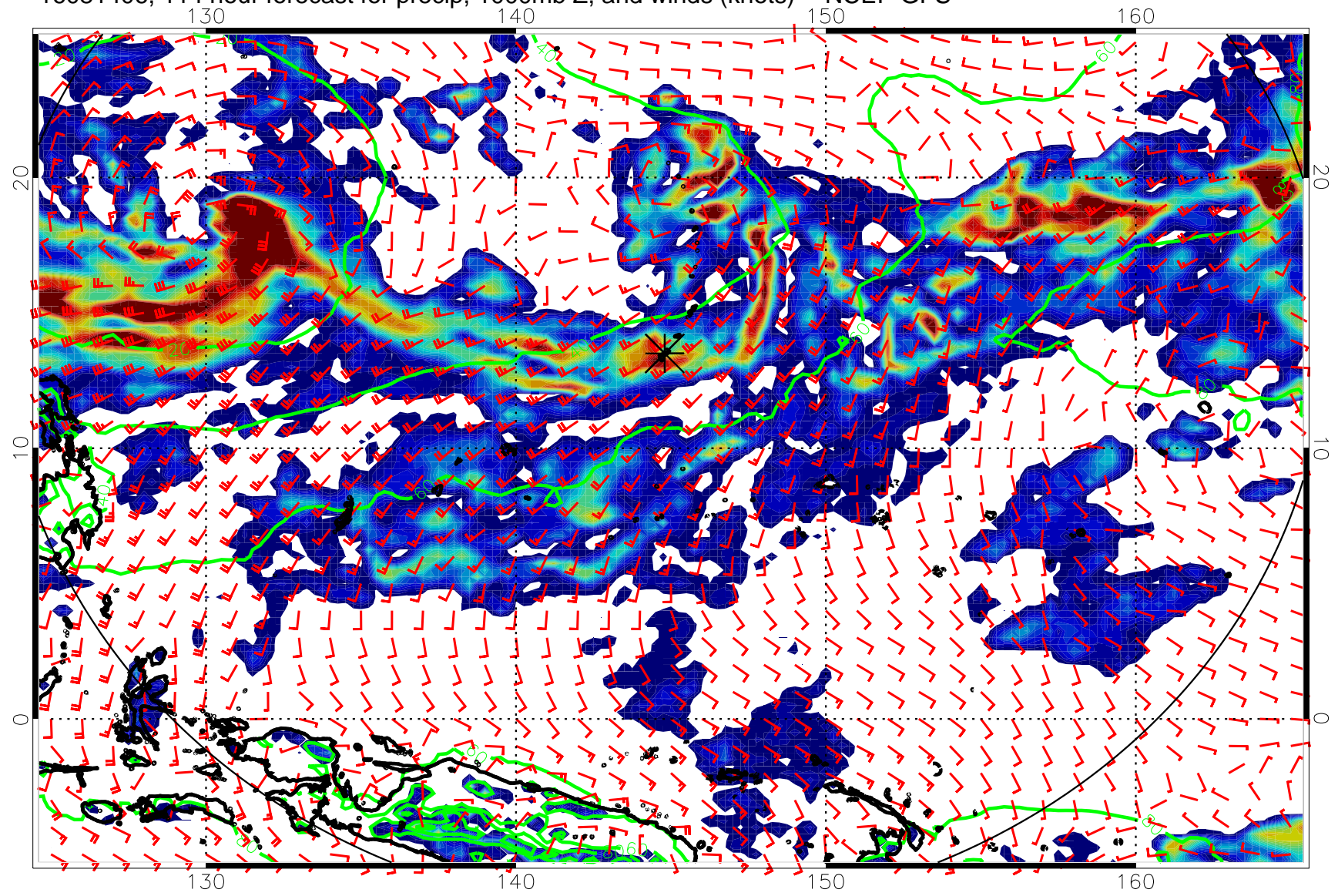
16081406, 114 hour forecast for precip, 1000mb Z, and winds (knots) -- NCEP GFS
