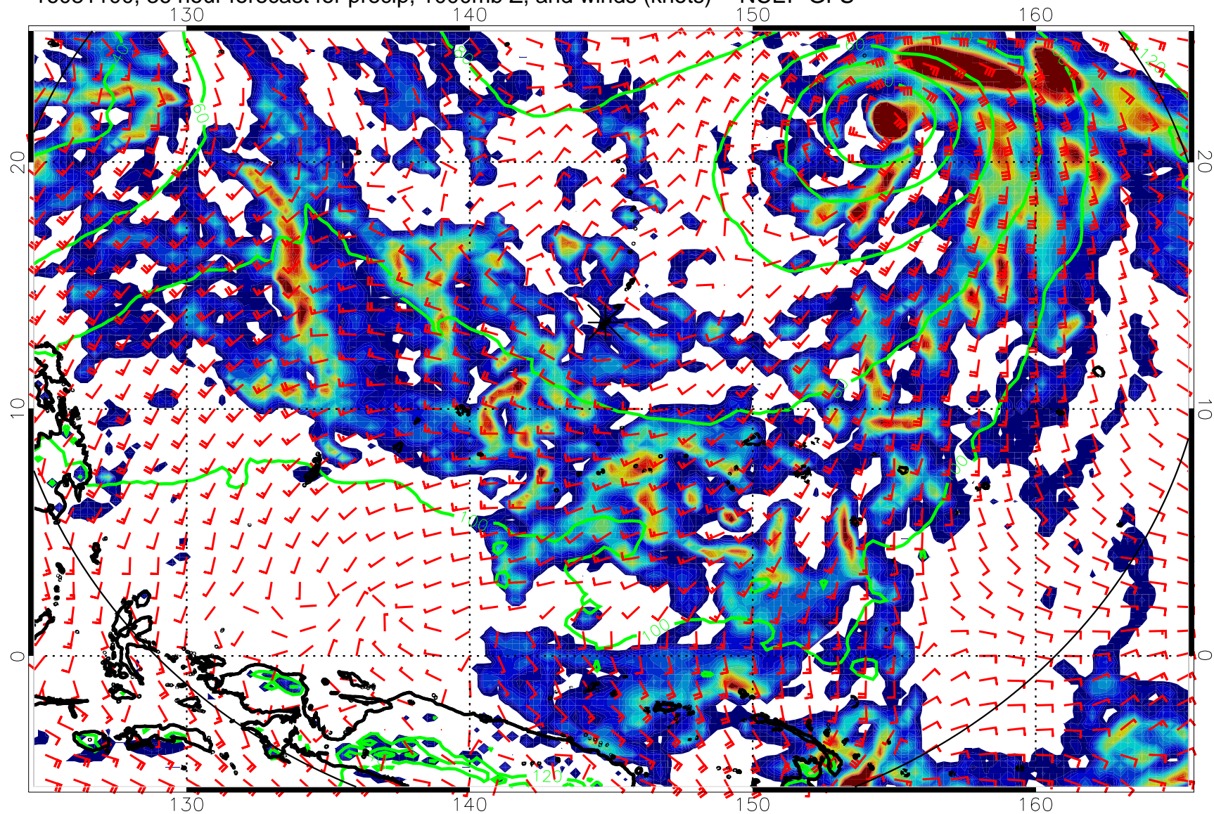
16081100, 36 hour forecast for precip, 1000mb Z, and winds (knots) -- NCEP GFS
