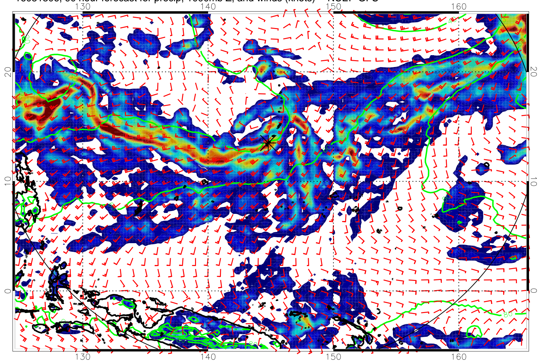
16081306, 90 hour forecast for precip, 1000mb Z, and winds (knots) -- NCEP GFS
