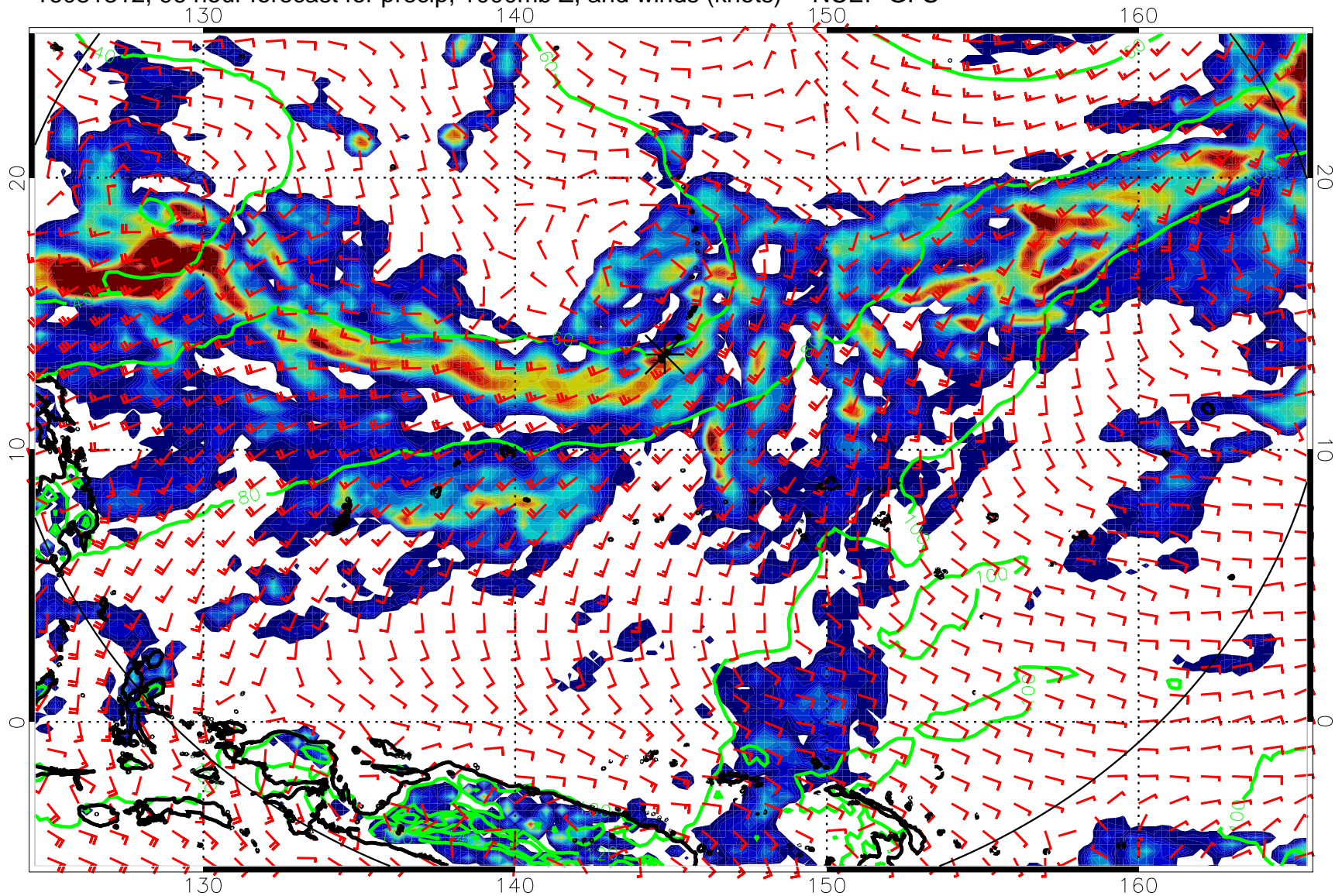
16081312, 96 hour forecast for precip, 1000mb Z, and winds (knots) -- NCEP GFS
