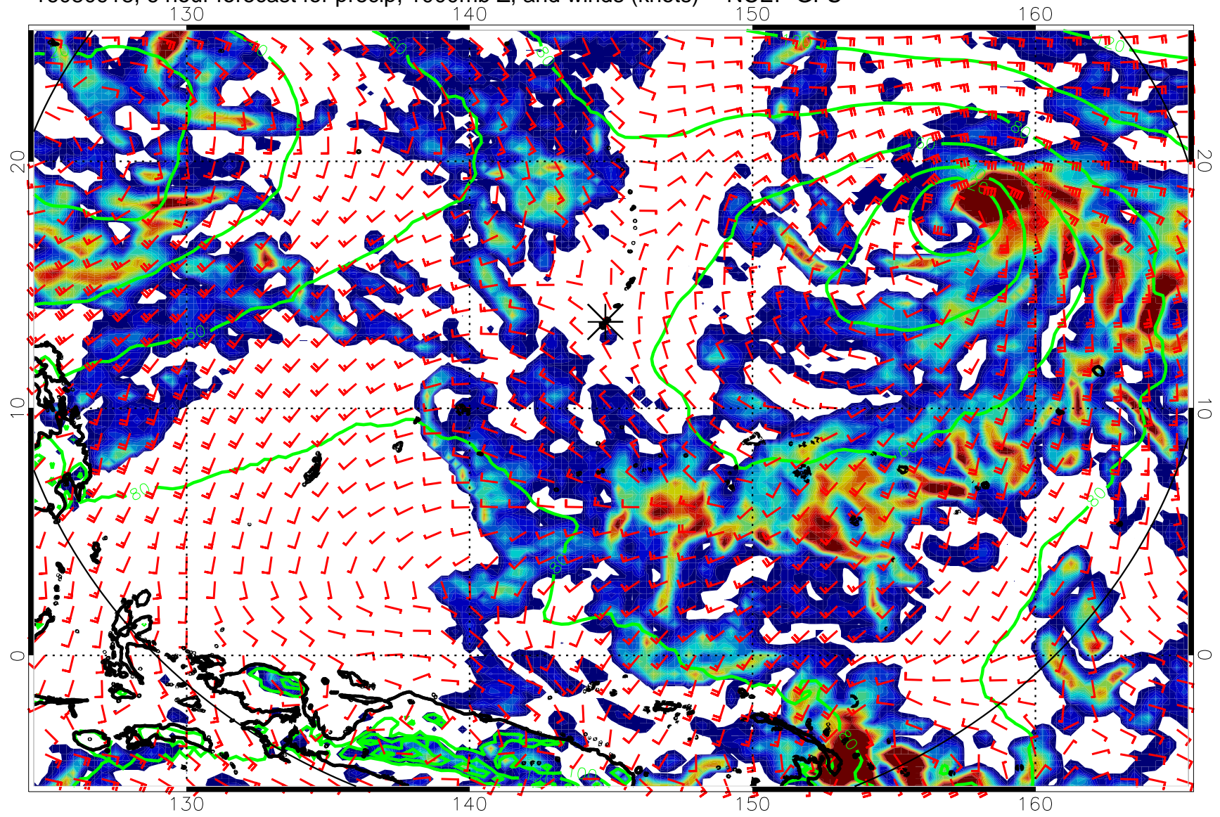
16080918, 6 hour forecast for precip, 1000mb Z, and winds (knots) -- NCEP GFS
