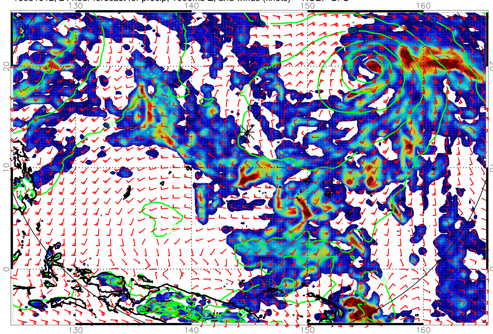
16081012, 24 hour forecast for precip, 1000mb Z, and winds (knots) -- NCEP GFS
