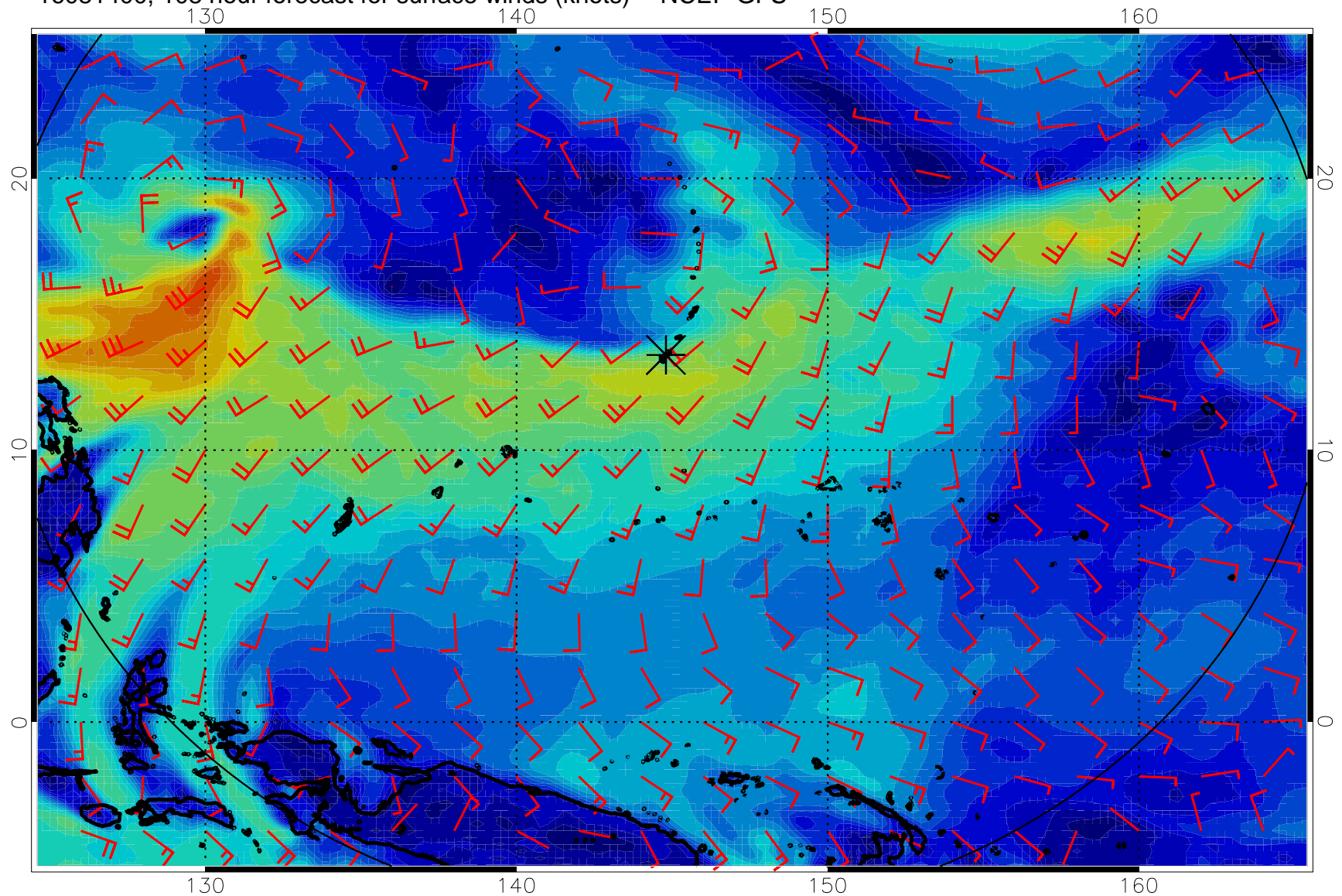
16081400, 108 hour forecast for surface winds (knots) -- NCEP GFS
