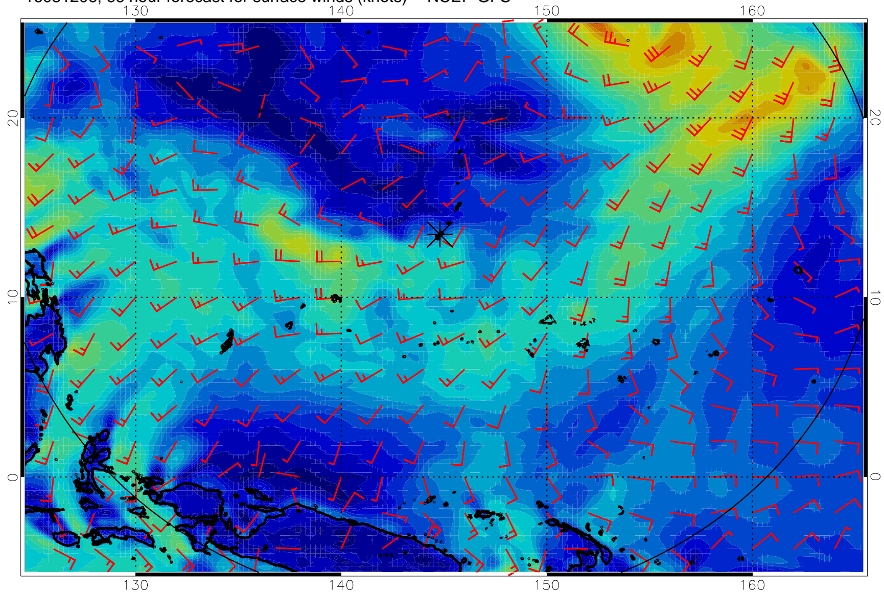
16081206, 66 hour forecast for surface winds (knots) -- NCEP GFS
