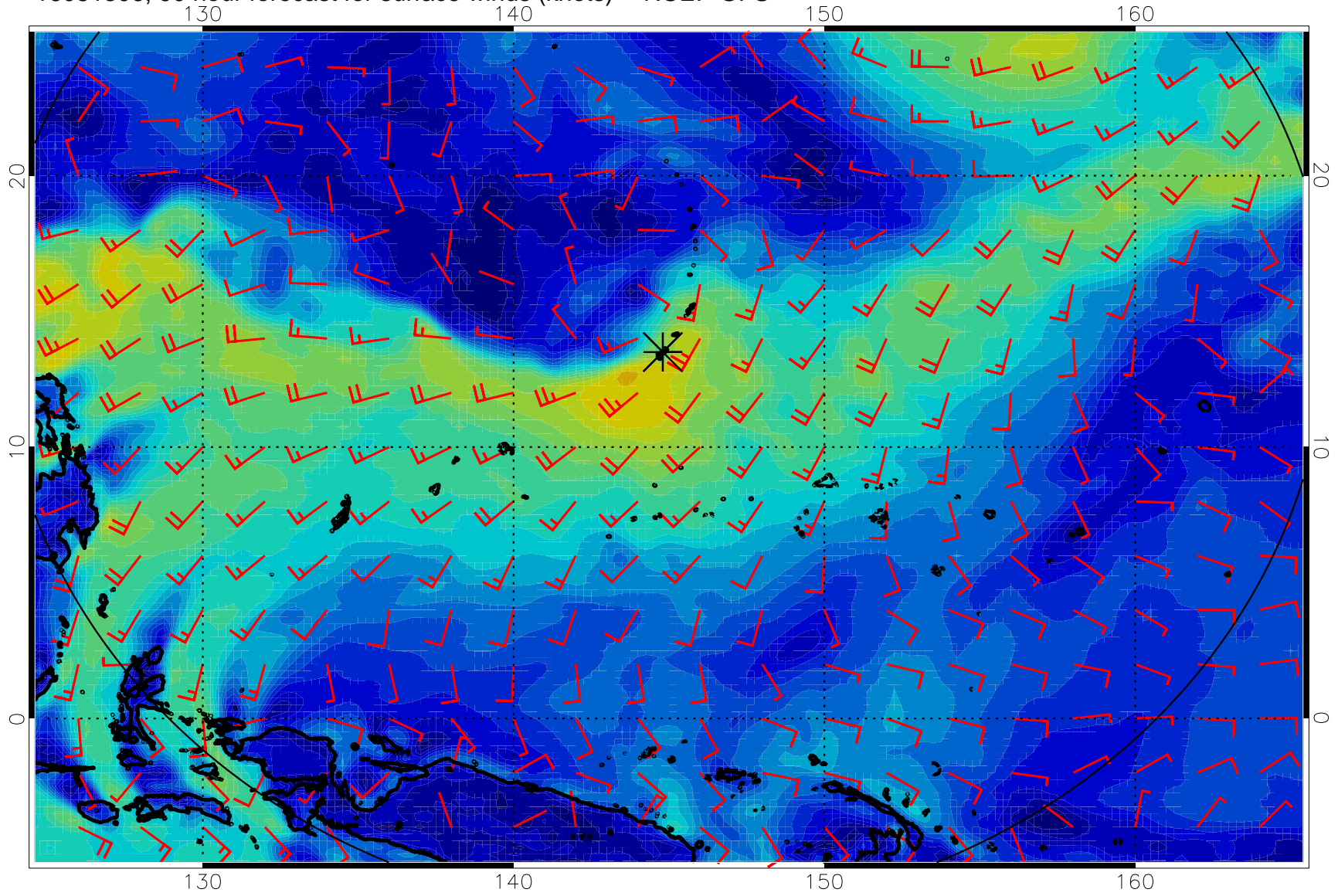
16081306, 90 hour forecast for surface winds (knots) -- NCEP GFS
