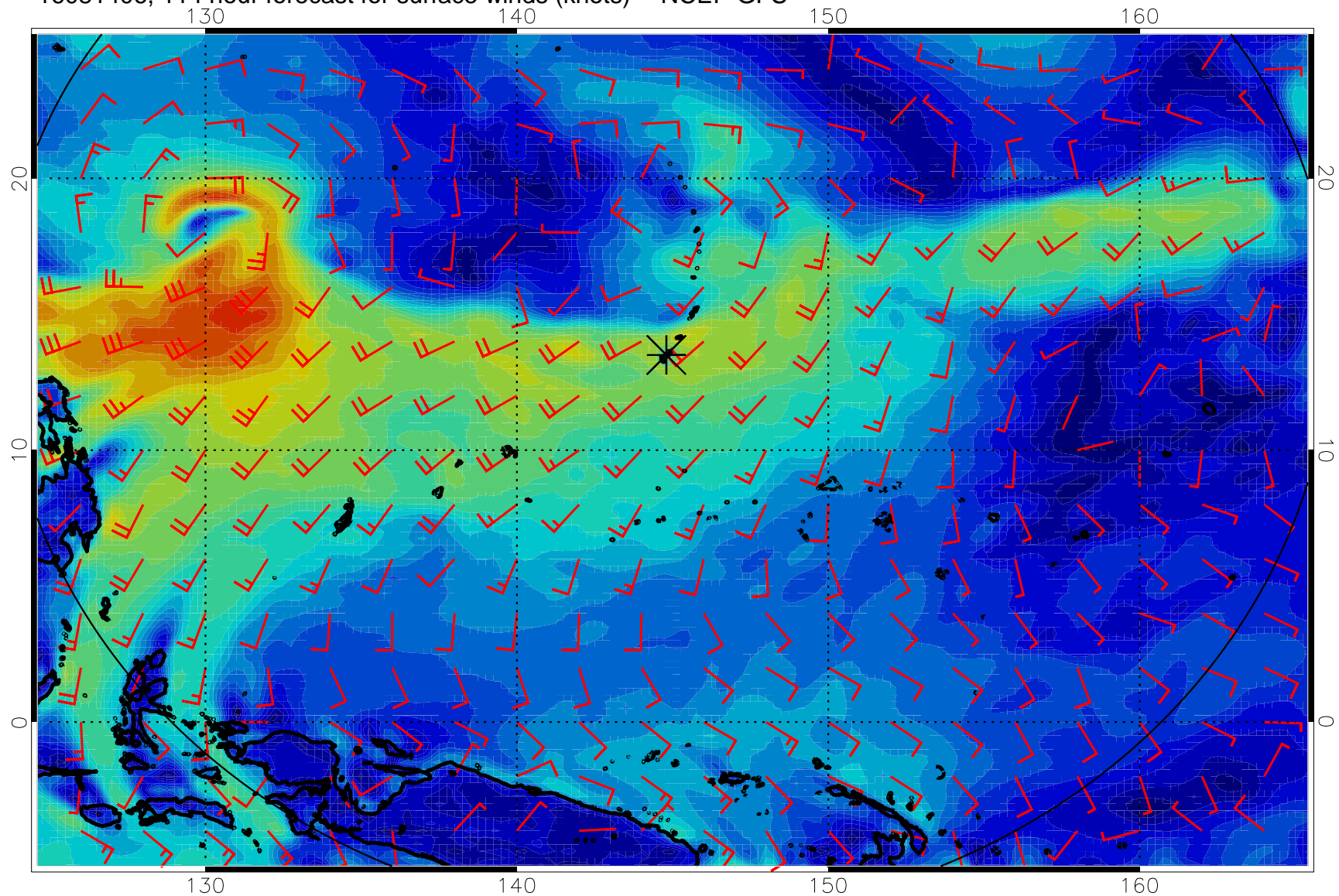
16081406, 114 hour forecast for surface winds (knots) -- NCEP GFS
