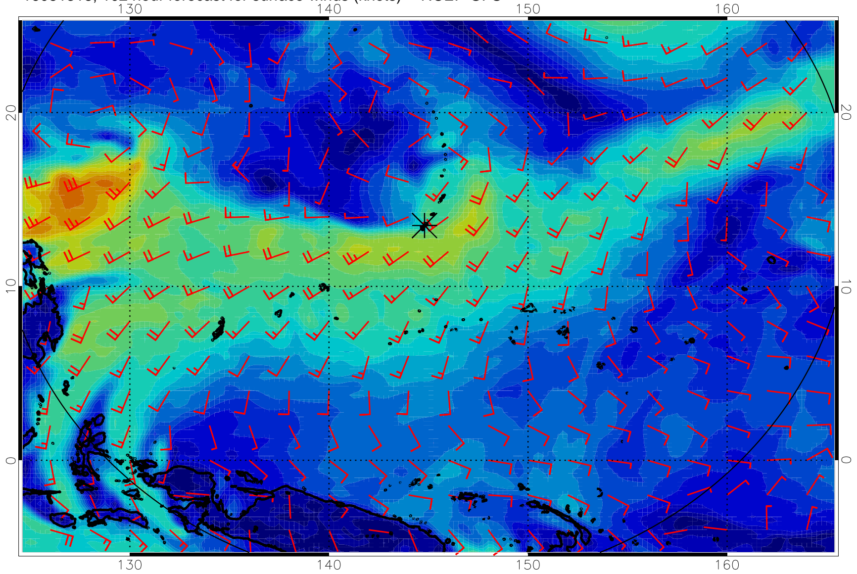
16081318, 102 hour forecast for surface winds (knots) -- NCEP GFS
