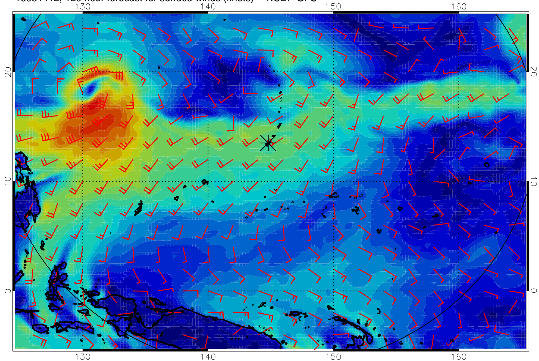
16081412, 120 hour forecast for surface winds (knots) -- NCEP GFS
