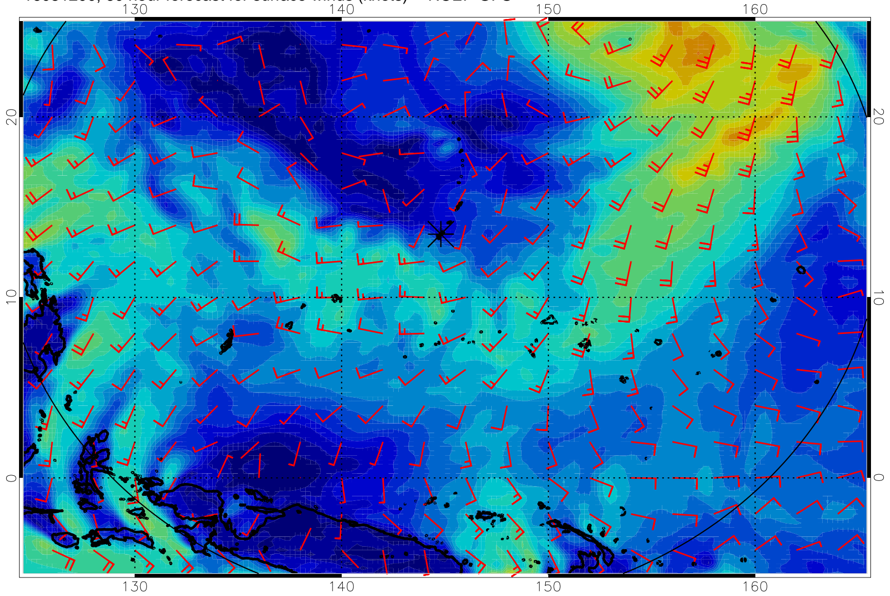
16081200, 60 hour forecast for surface winds (knots) -- NCEP GFS
