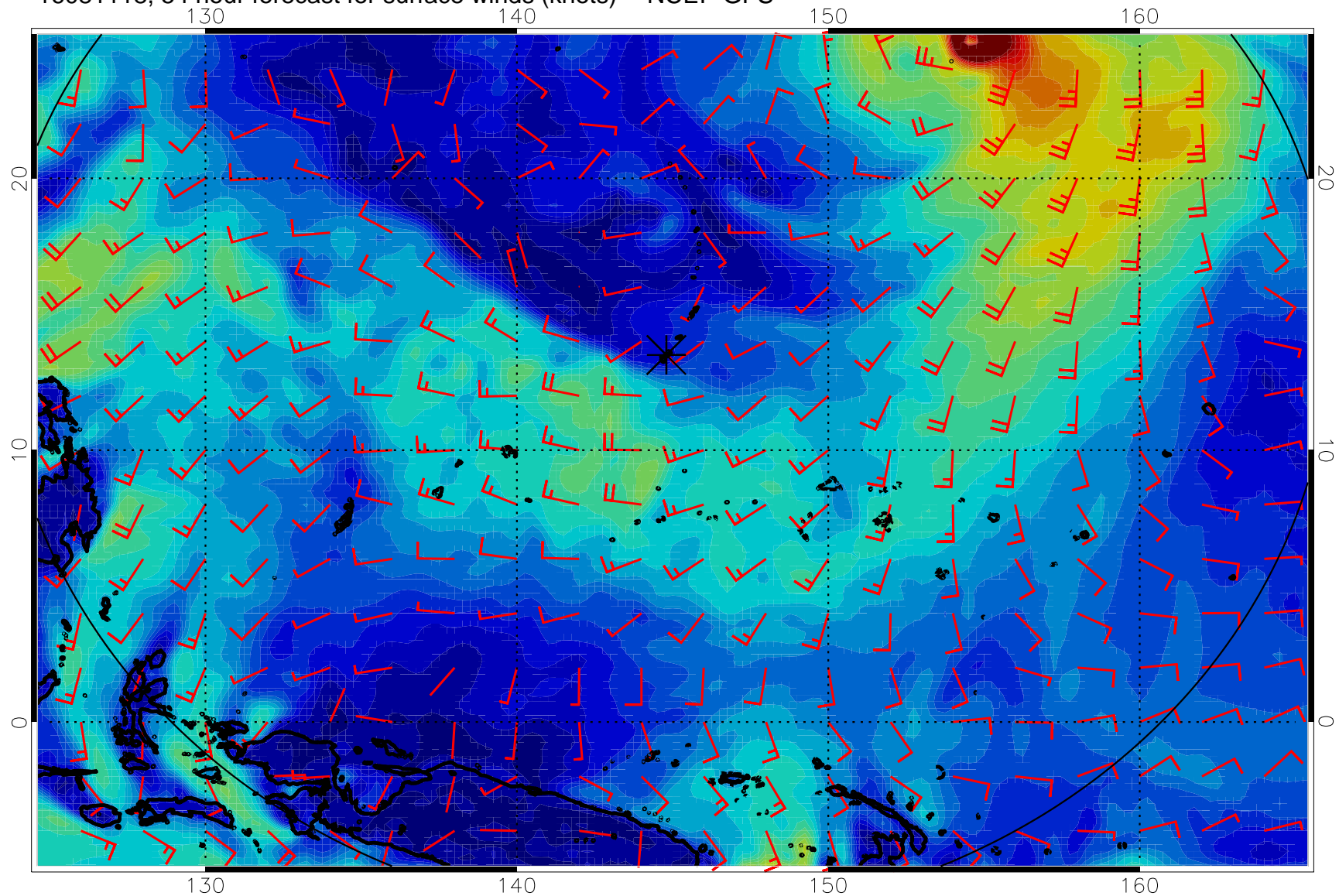
16081118, 54 hour forecast for surface winds (knots) -- NCEP GFS
