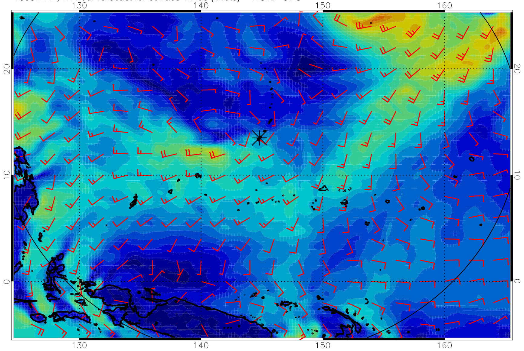
16081212, 72 hour forecast for surface winds (knots) -- NCEP GFS
