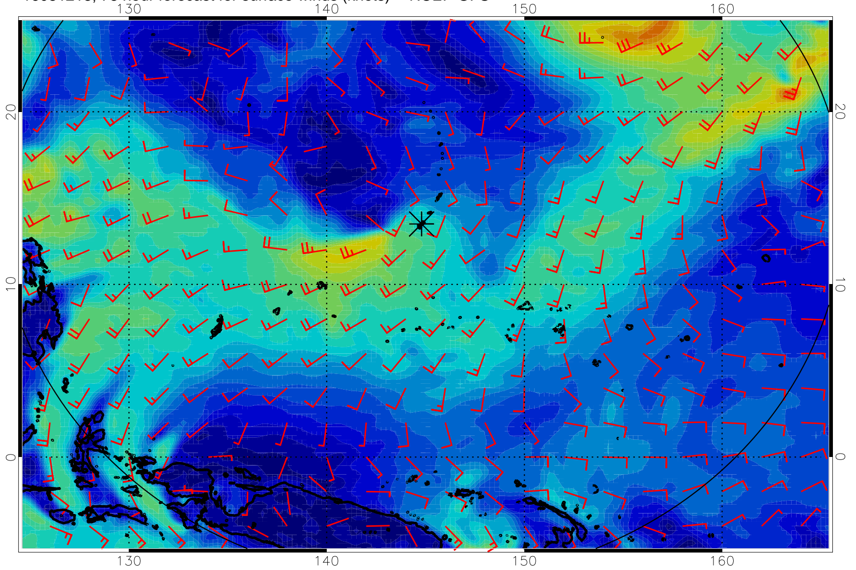
16081218, 78 hour forecast for surface winds (knots) -- NCEP GFS
