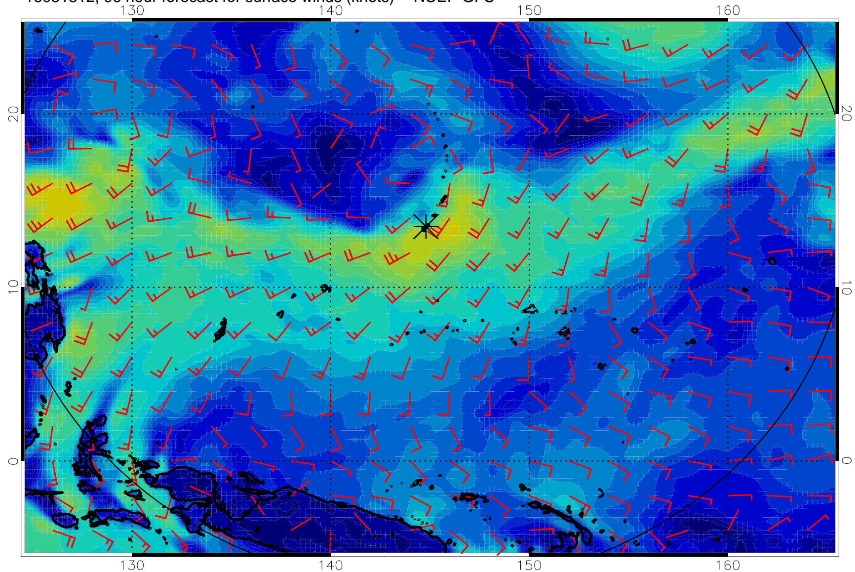
16081312, 96 hour forecast for surface winds (knots) -- NCEP GFS
