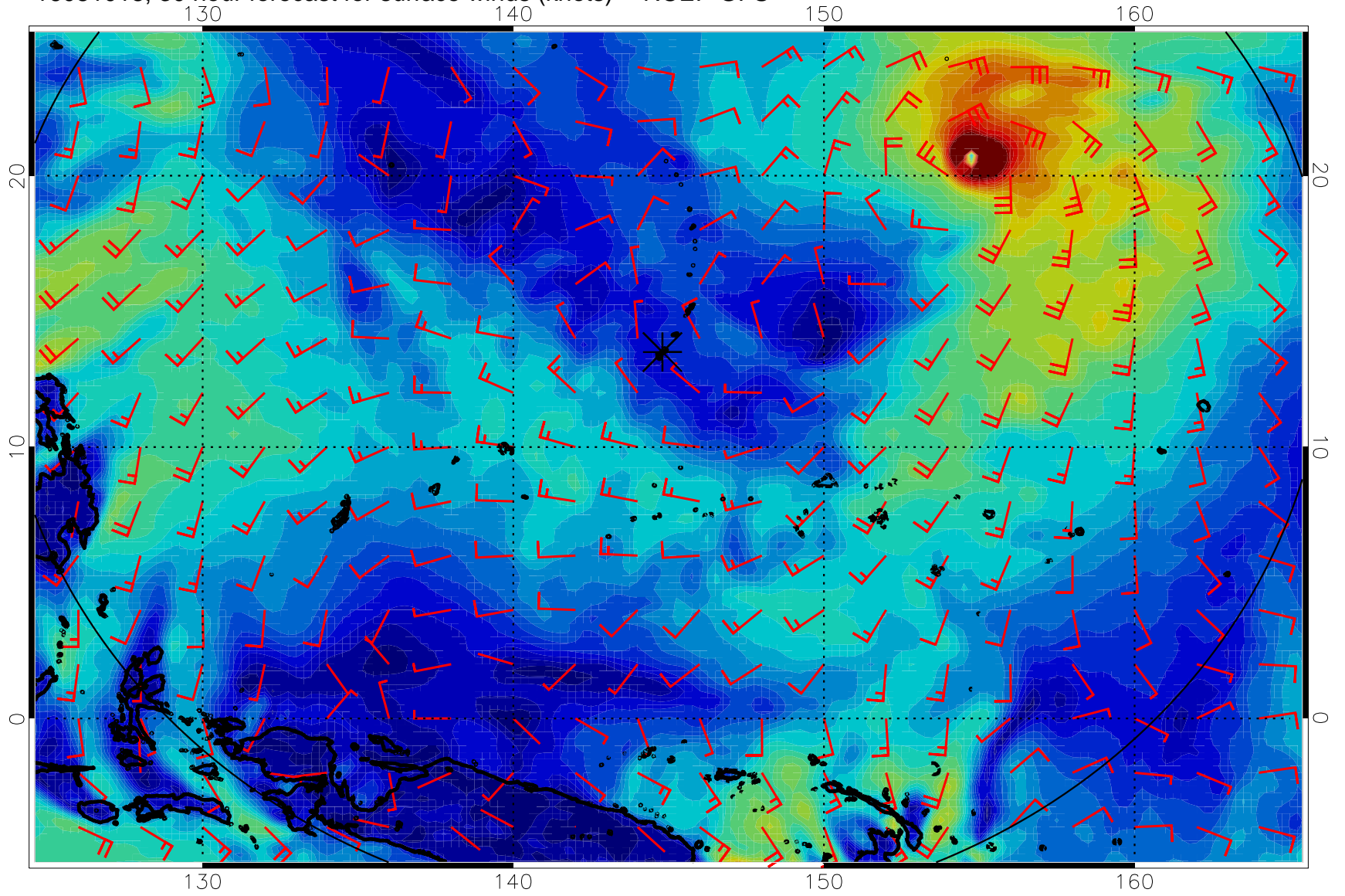
16081018, 30 hour forecast for surface winds (knots) -- NCEP GFS
