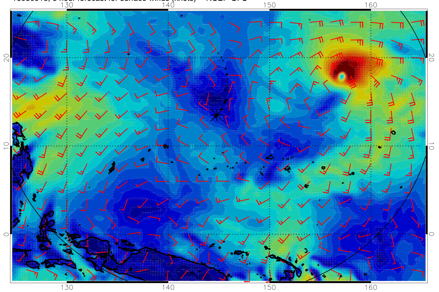
16080918, 6 hour forecast for surface winds (knots) -- NCEP GFS
