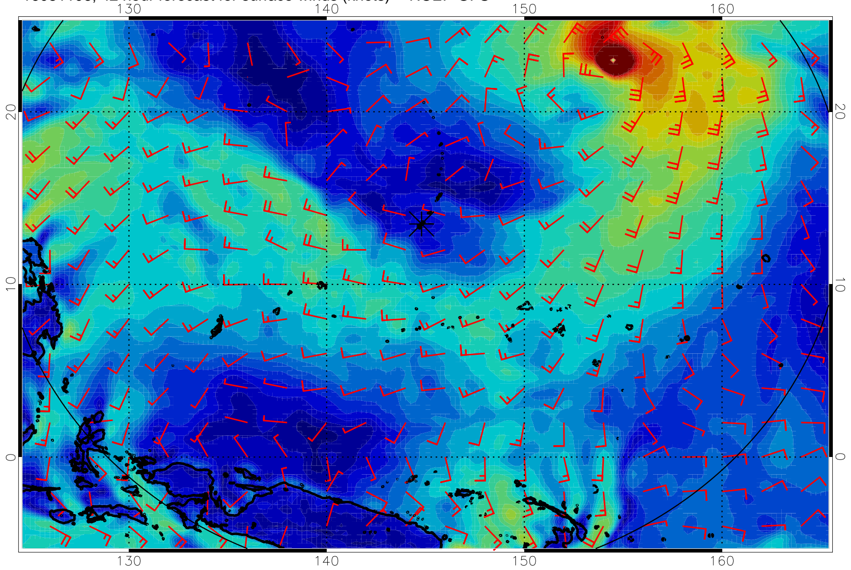
16081106, 42 hour forecast for surface winds (knots) -- NCEP GFS
