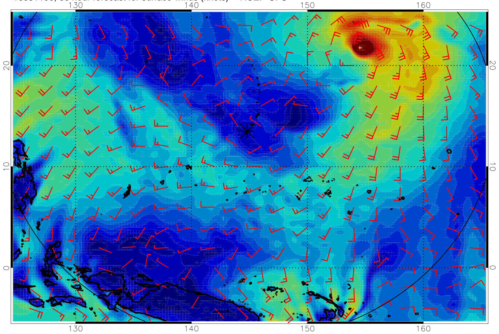
16081100, 36 hour forecast for surface winds (knots) -- NCEP GFS
