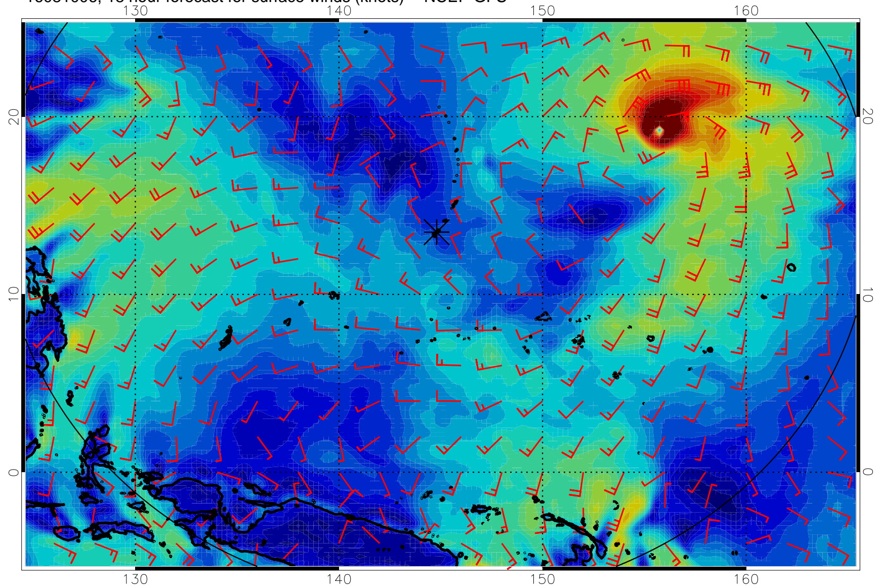
16081006, 18 hour forecast for surface winds (knots) -- NCEP GFS
