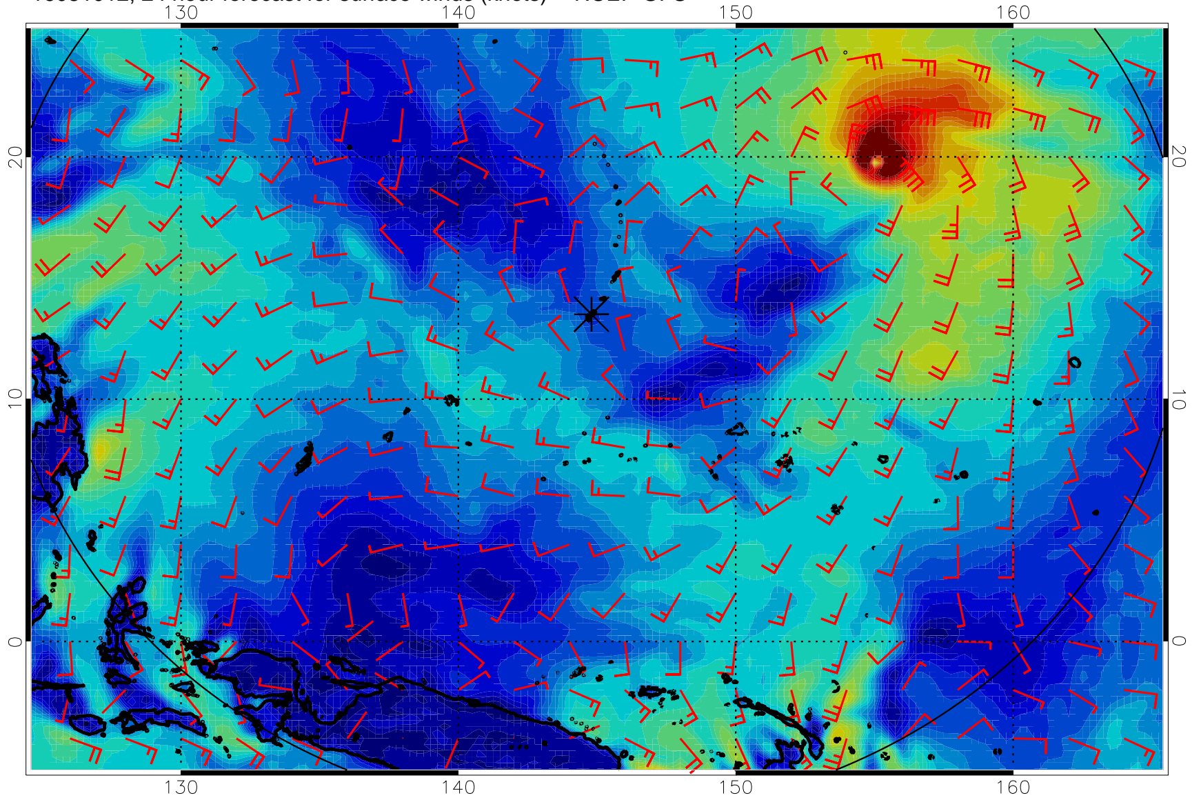
16081012, 24 hour forecast for surface winds (knots) -- NCEP GFS
