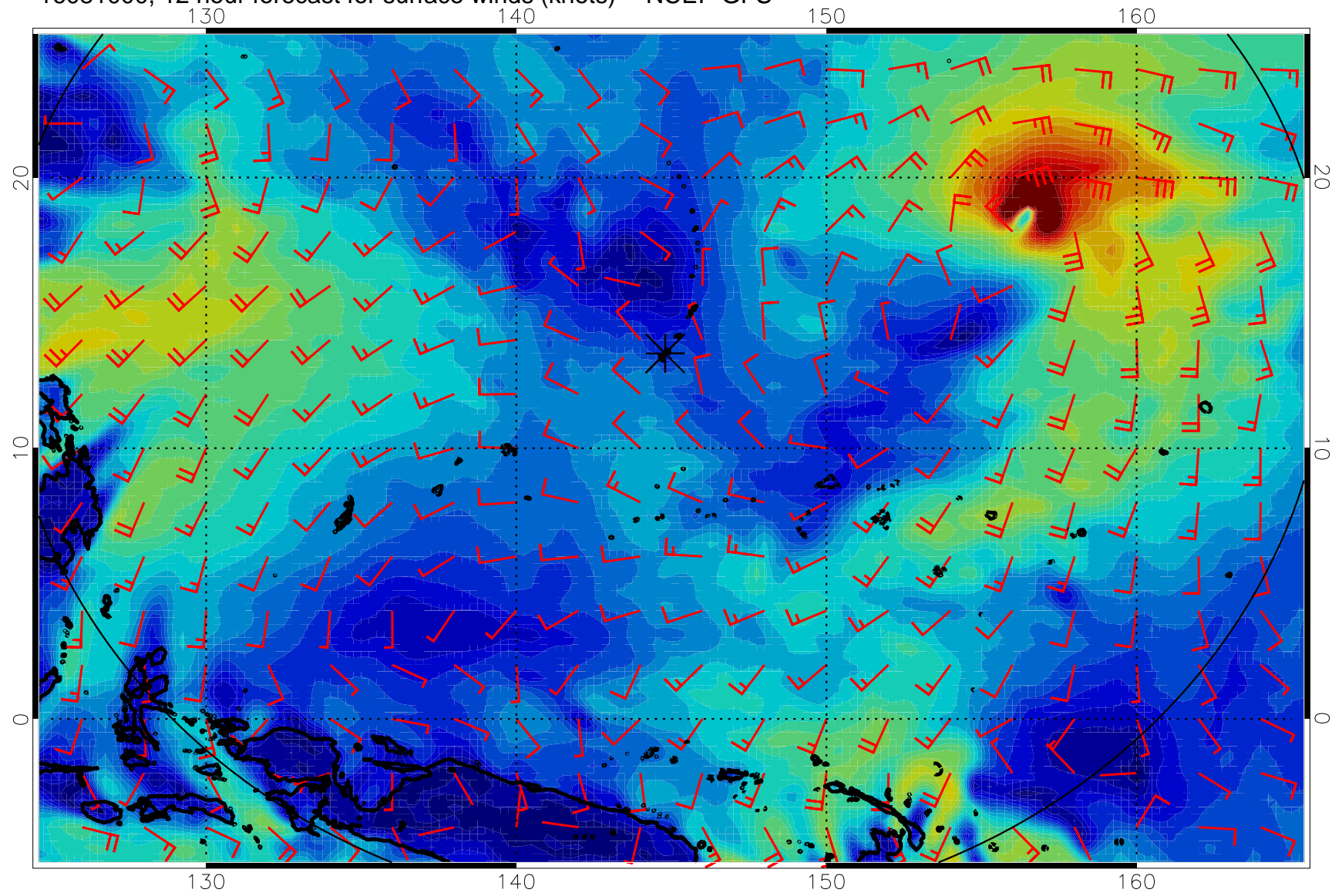
16081000, 12 hour forecast for surface winds (knots) -- NCEP GFS
