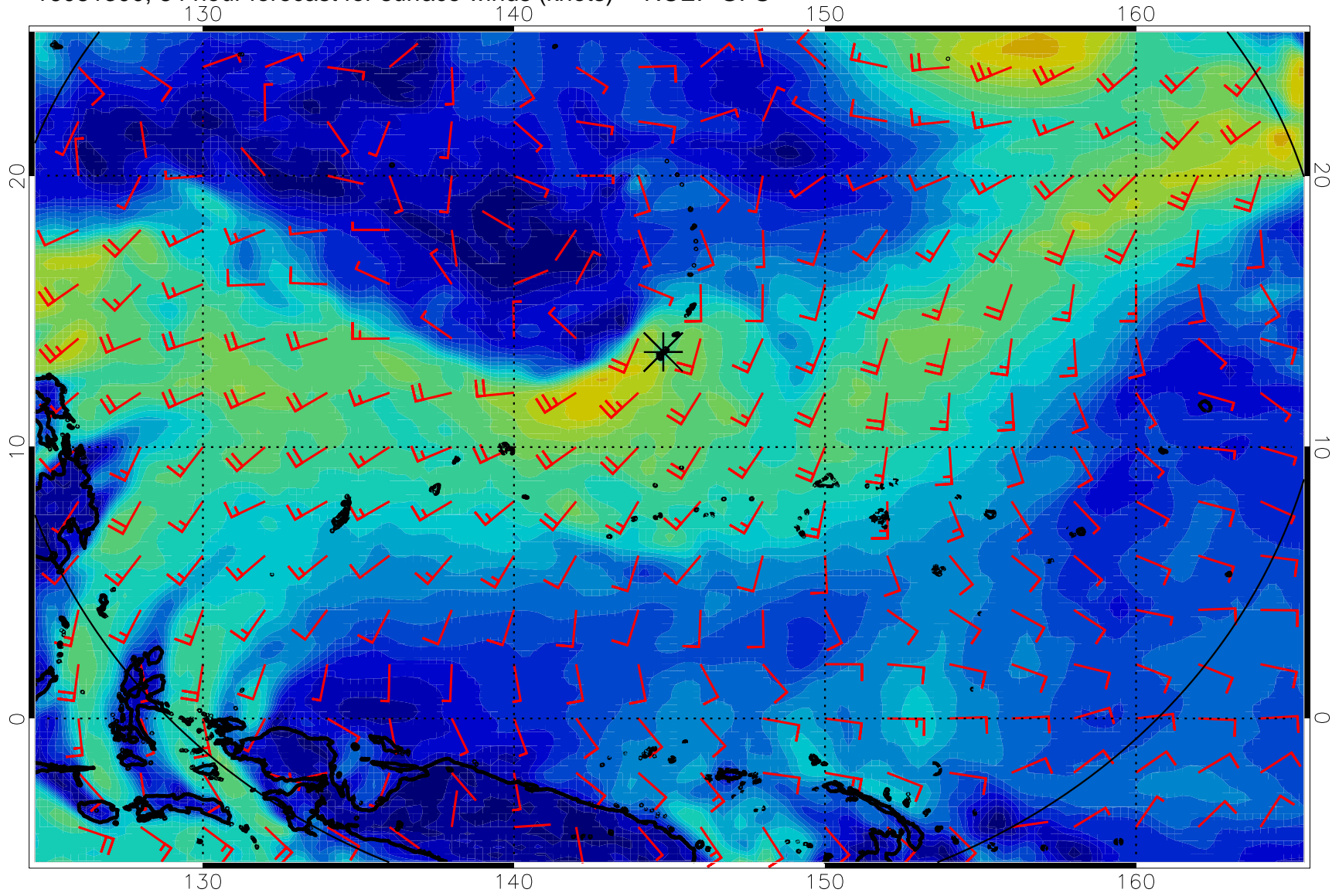
16081300, 84 hour forecast for surface winds (knots) -- NCEP GFS
