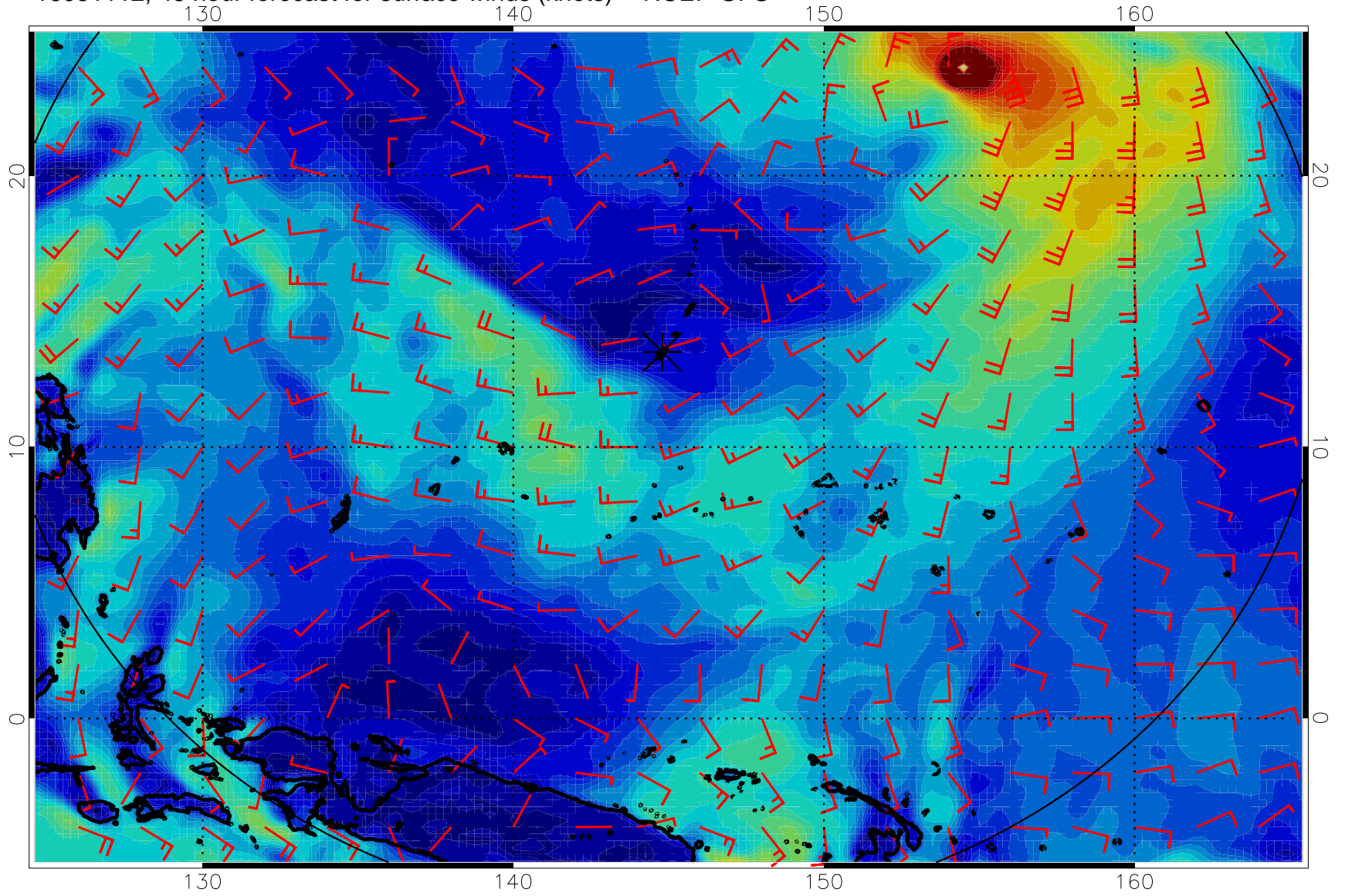
16081112, 48 hour forecast for surface winds (knots) -- NCEP GFS
