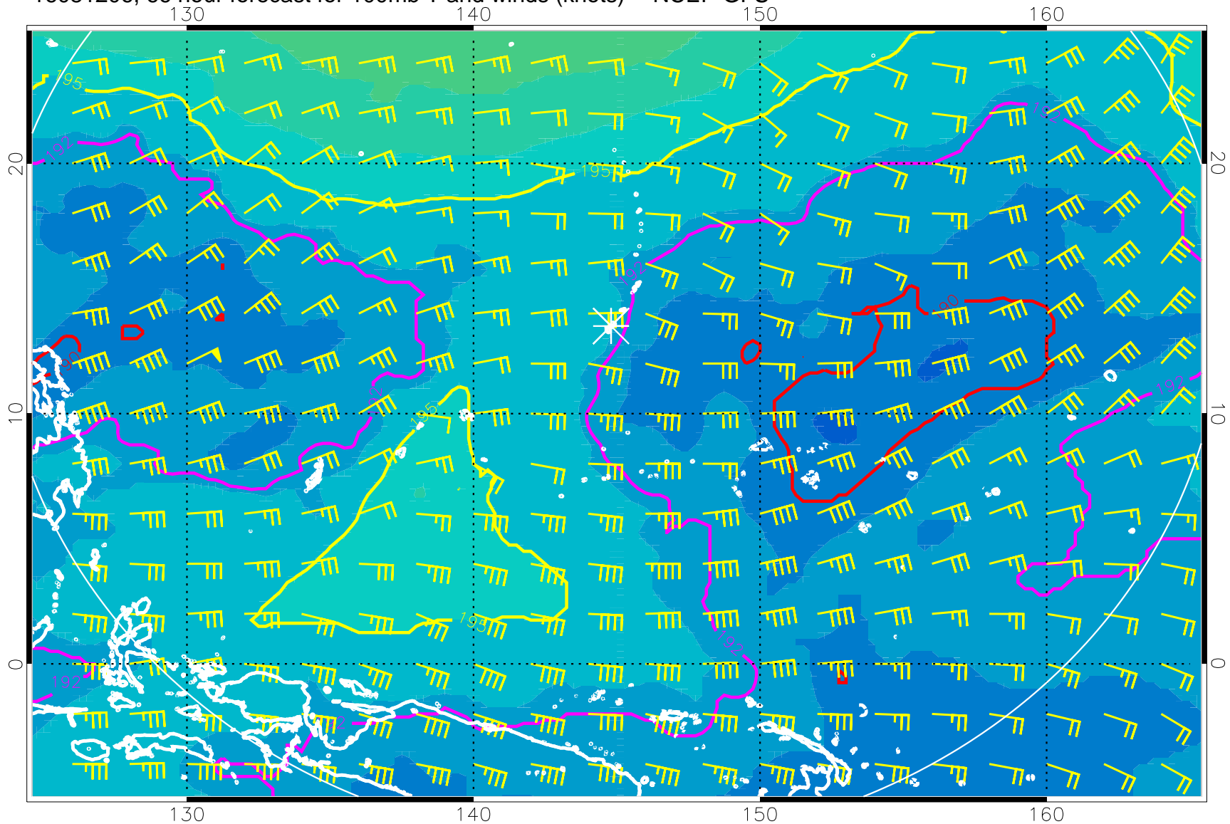
16081206, 66 hour forecast for 100mb T and winds (knots) -- NCEP GFS
