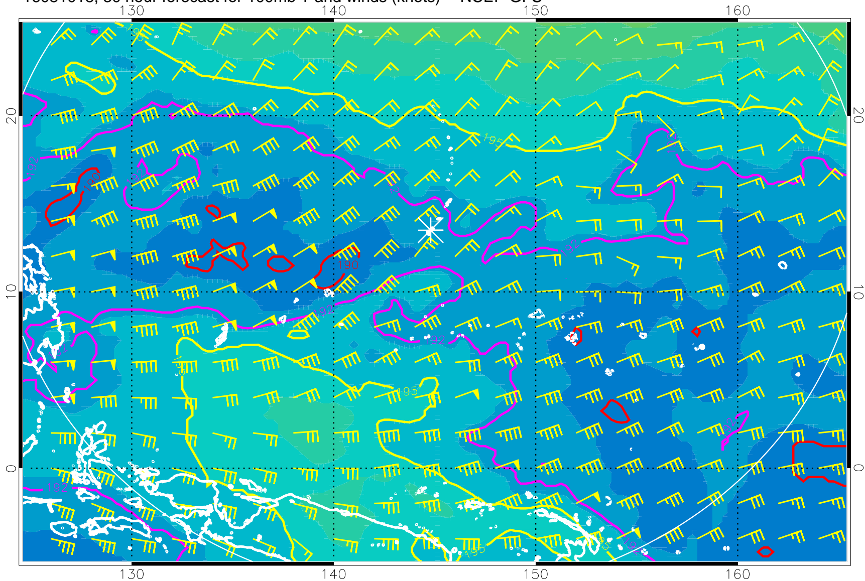
16081018, 30 hour forecast for 100mb T and winds (knots) -- NCEP GFS
