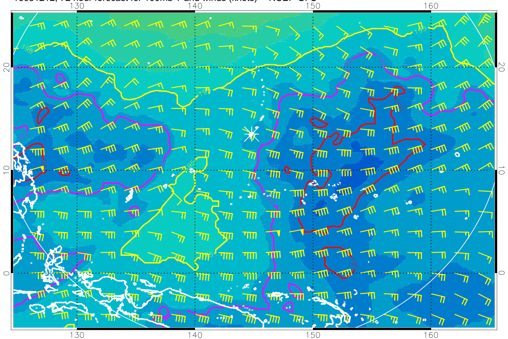
16081212, 72 hour forecast for 100mb T and winds (knots) -- NCEP GFS
