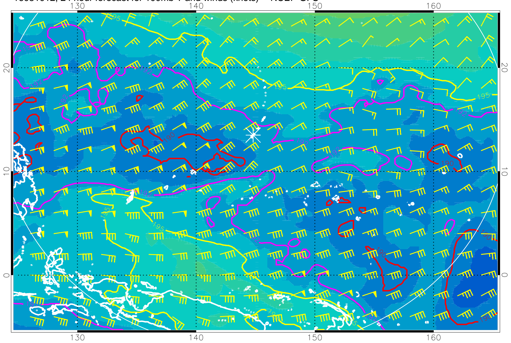
16081012, 24 hour forecast for 100mb T and winds (knots) -- NCEP GFS
