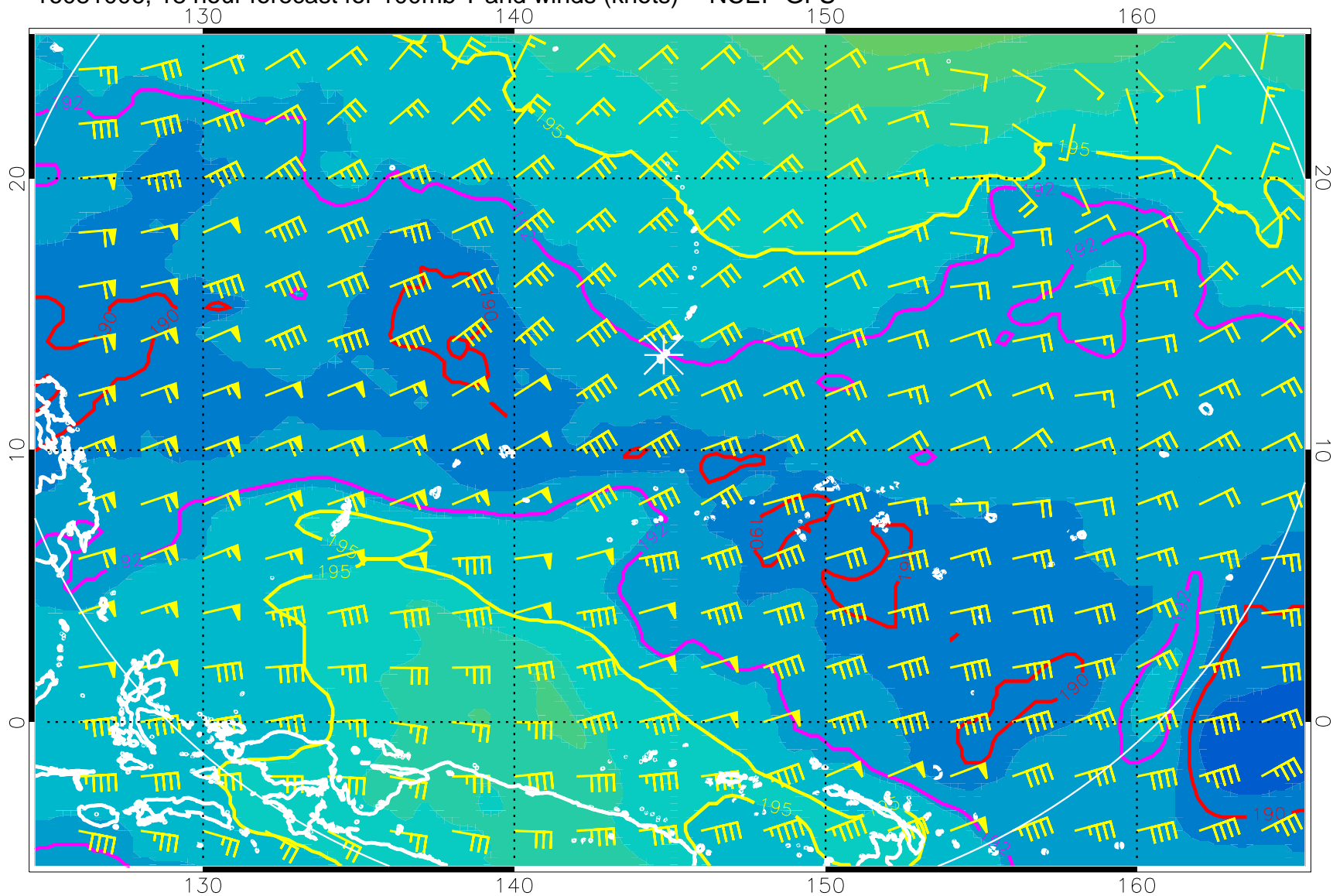
16081006, 18 hour forecast for 100mb T and winds (knots) -- NCEP GFS
