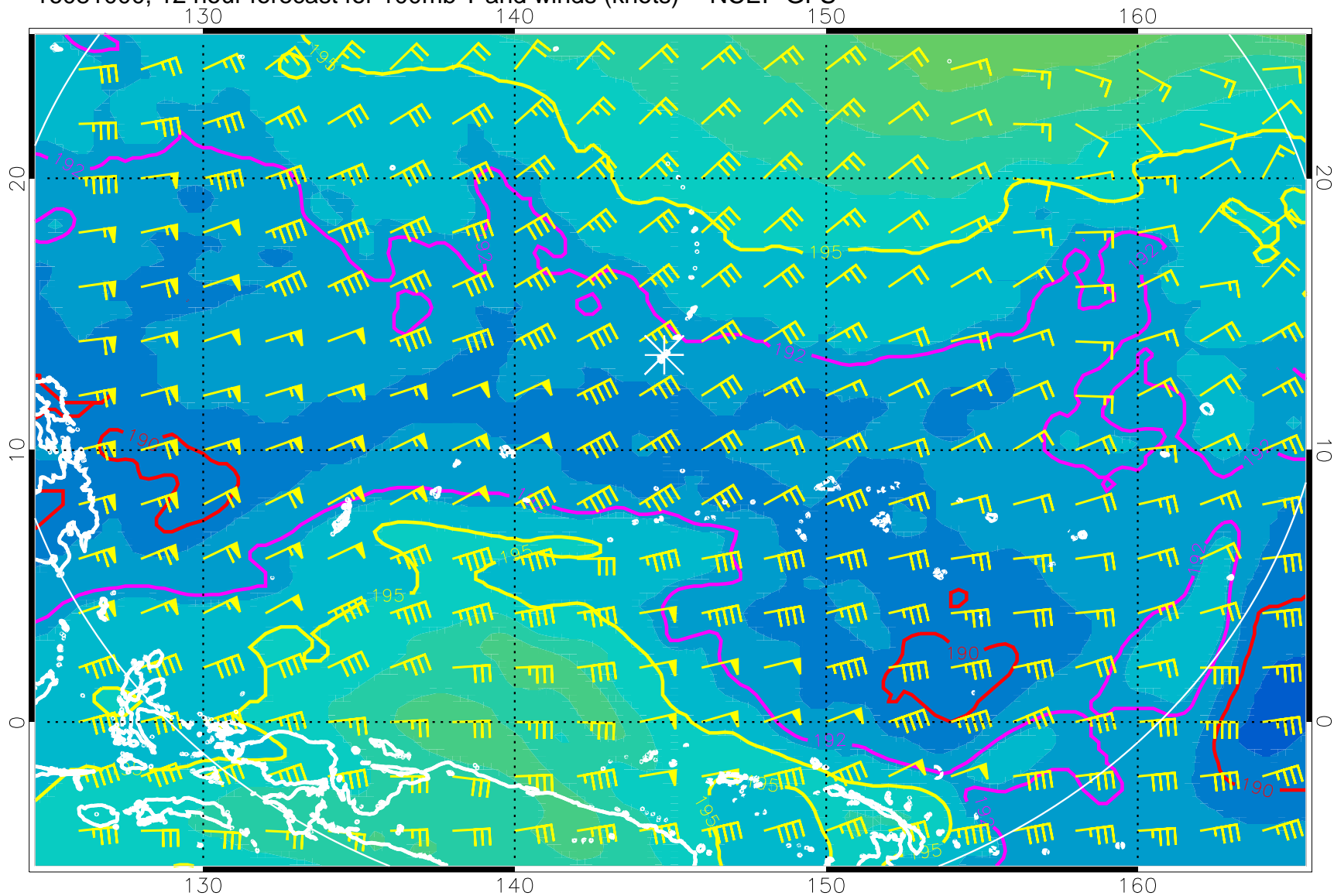
16081000, 12 hour forecast for 100mb T and winds (knots) -- NCEP GFS
