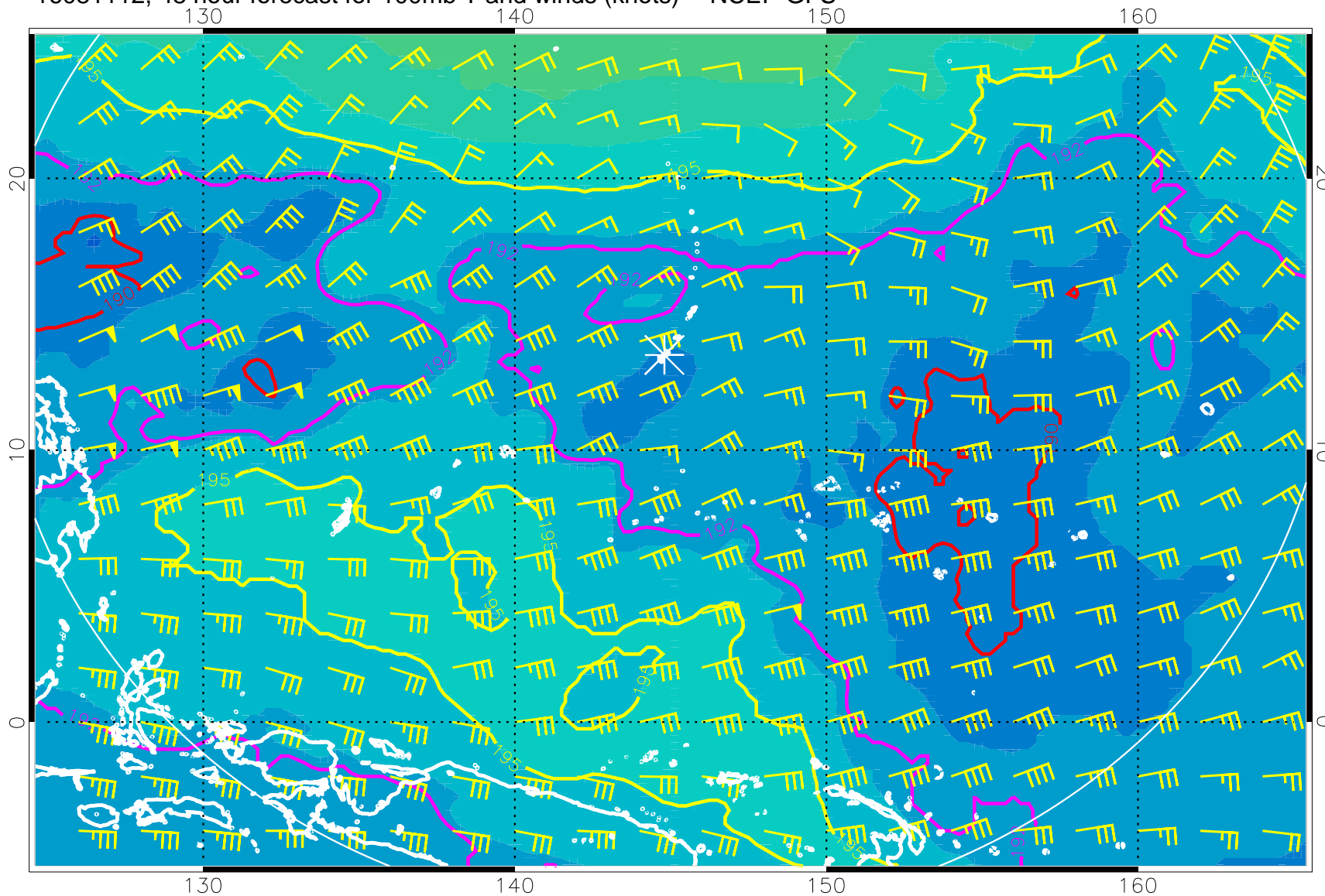
16081112, 48 hour forecast for 100mb T and winds (knots) -- NCEP GFS
