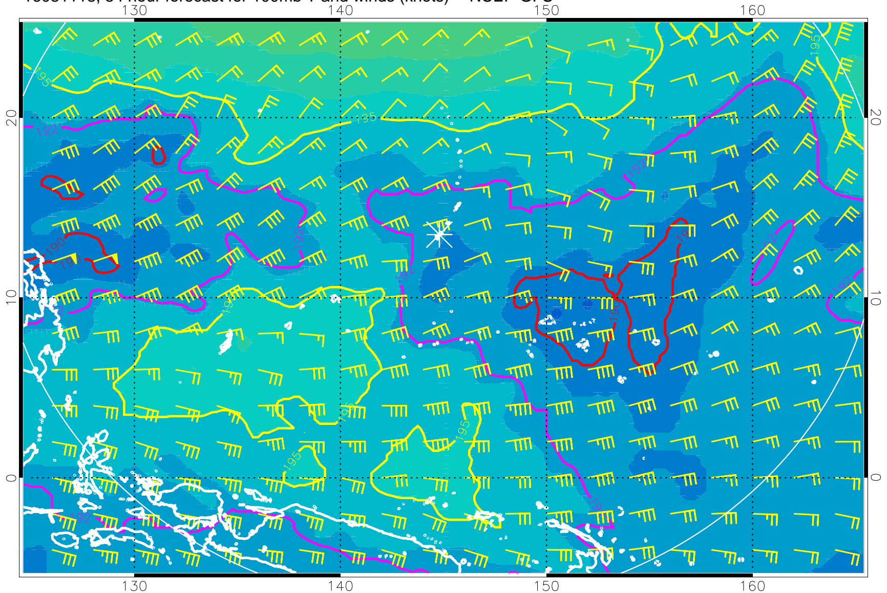
16081118, 54 hour forecast for 100mb T and winds (knots) -- NCEP GFS
