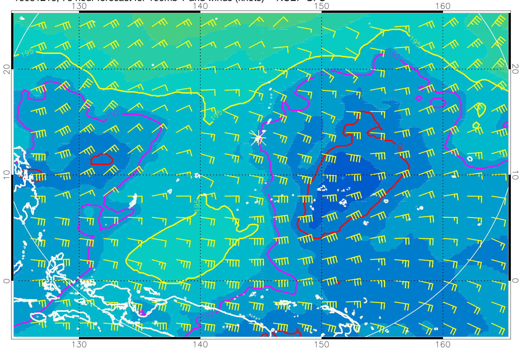
16081218, 78 hour forecast for 100mb T and winds (knots) -- NCEP GFS
