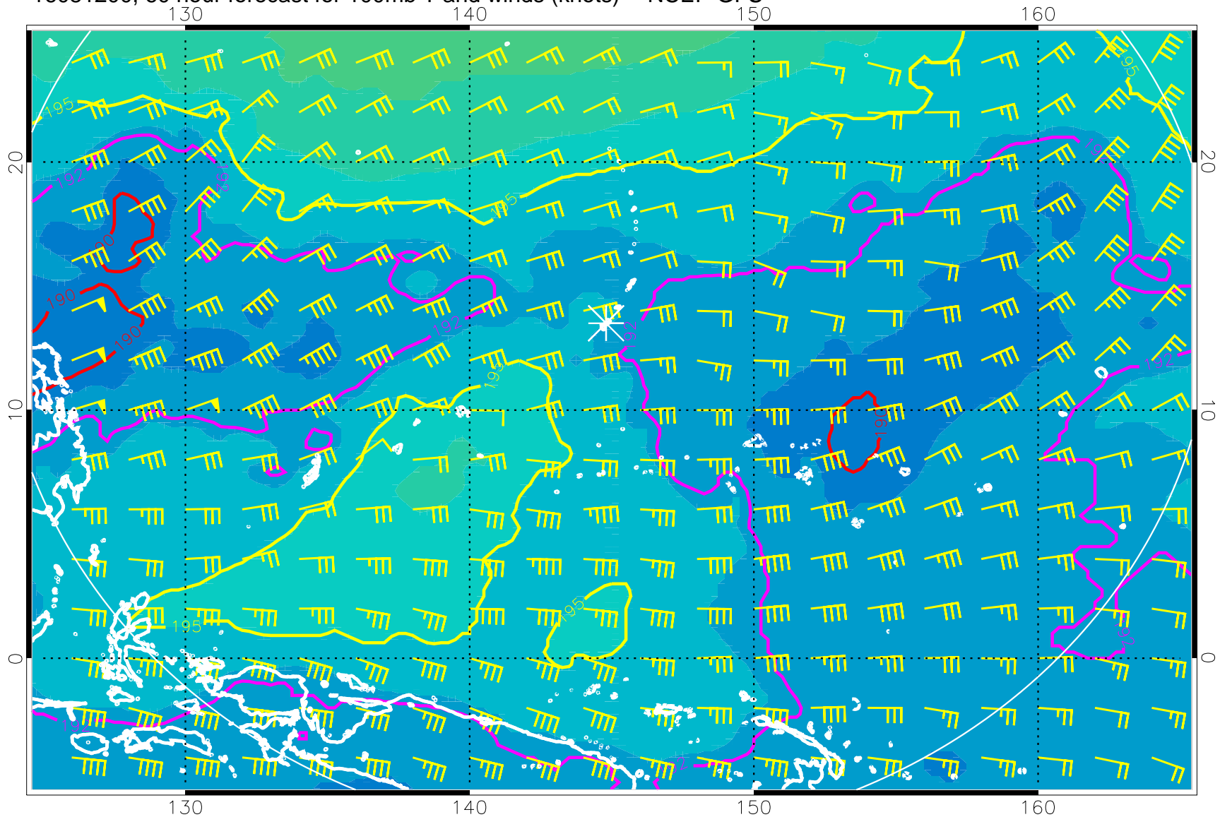
16081200, 60 hour forecast for 100mb T and winds (knots) -- NCEP GFS
