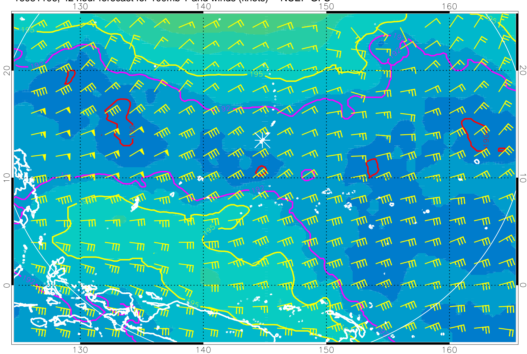
16081106, 42 hour forecast for 100mb T and winds (knots) -- NCEP GFS
