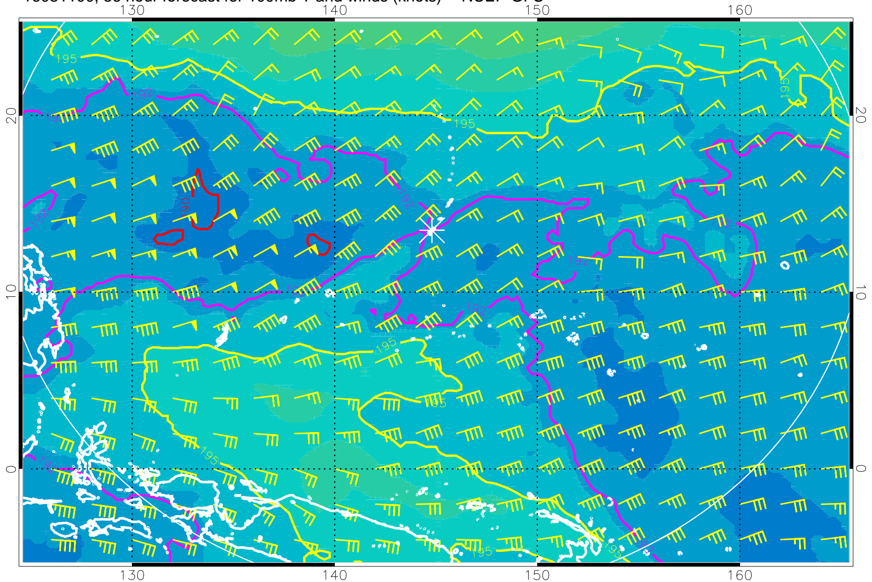
16081100, 36 hour forecast for 100mb T and winds (knots) -- NCEP GFS
