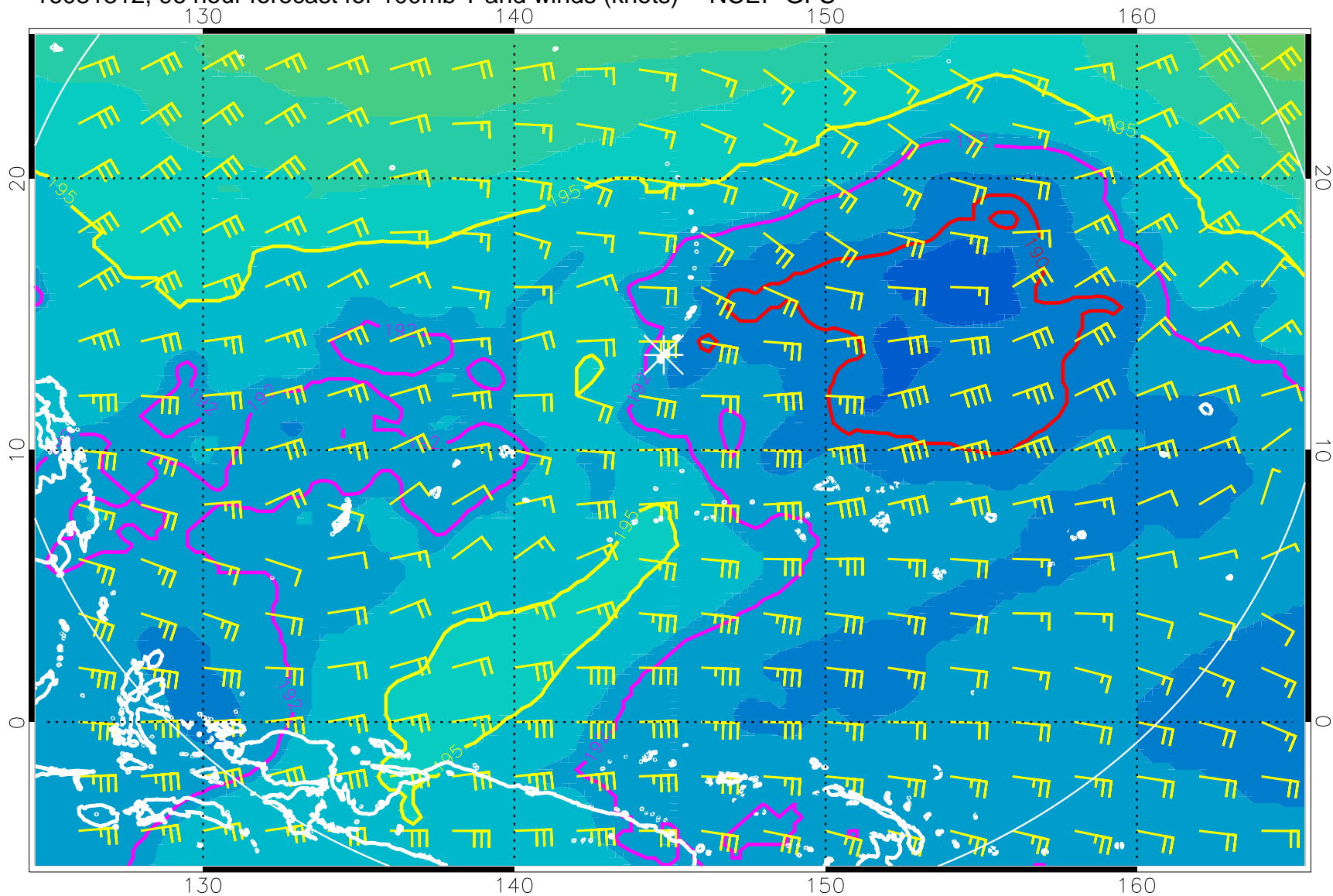
16081312, 96 hour forecast for 100mb T and winds (knots) -- NCEP GFS
