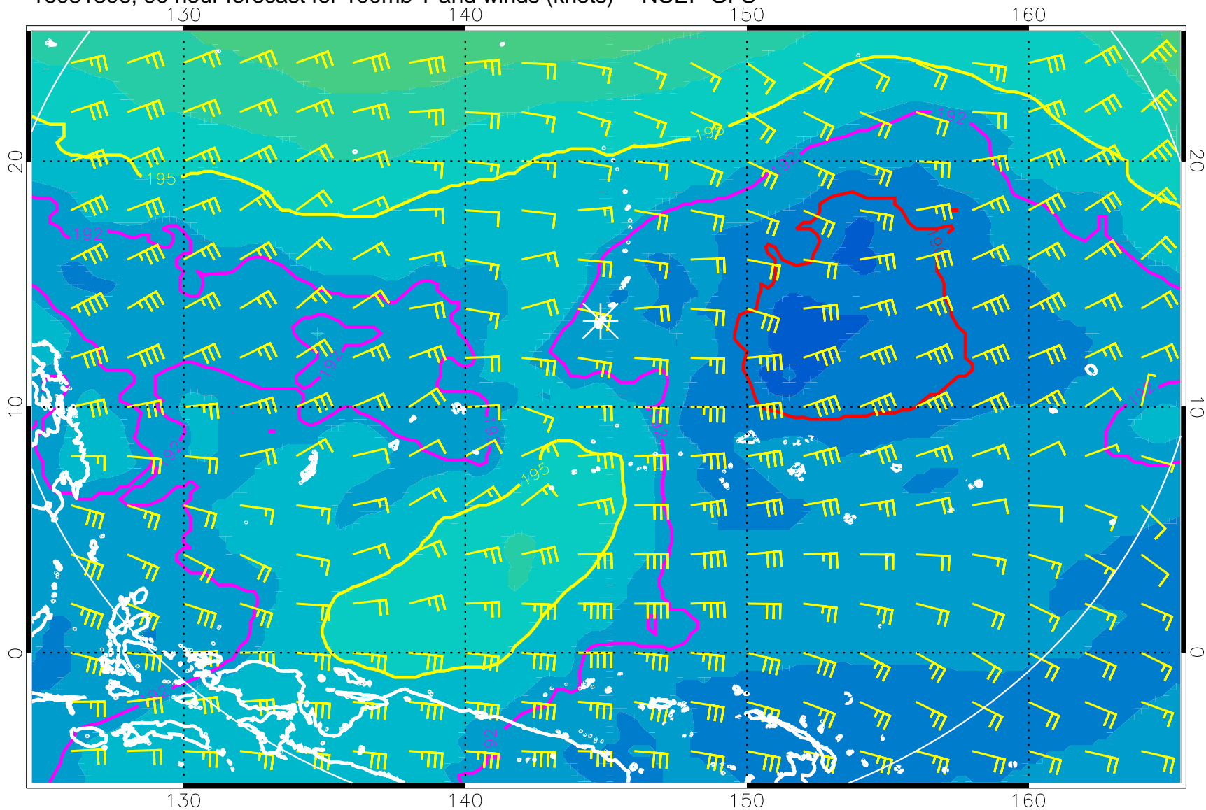
16081306, 90 hour forecast for 100mb T and winds (knots) -- NCEP GFS
