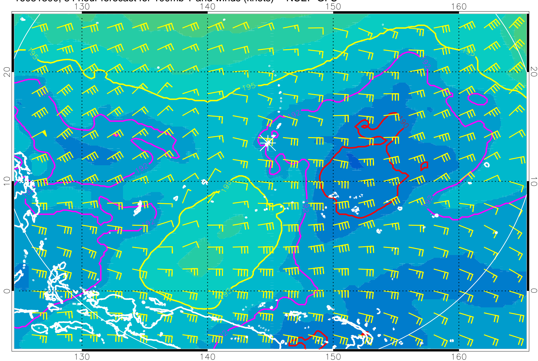
16081300, 84 hour forecast for 100mb T and winds (knots) -- NCEP GFS
