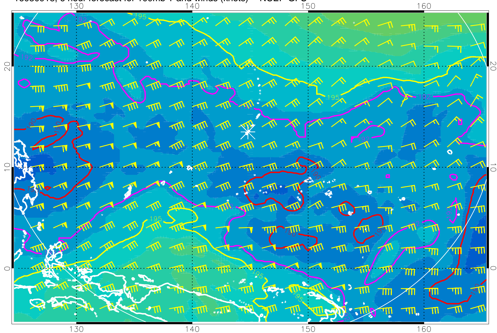
16080918, 6 hour forecast for 100mb T and winds (knots) -- NCEP GFS
