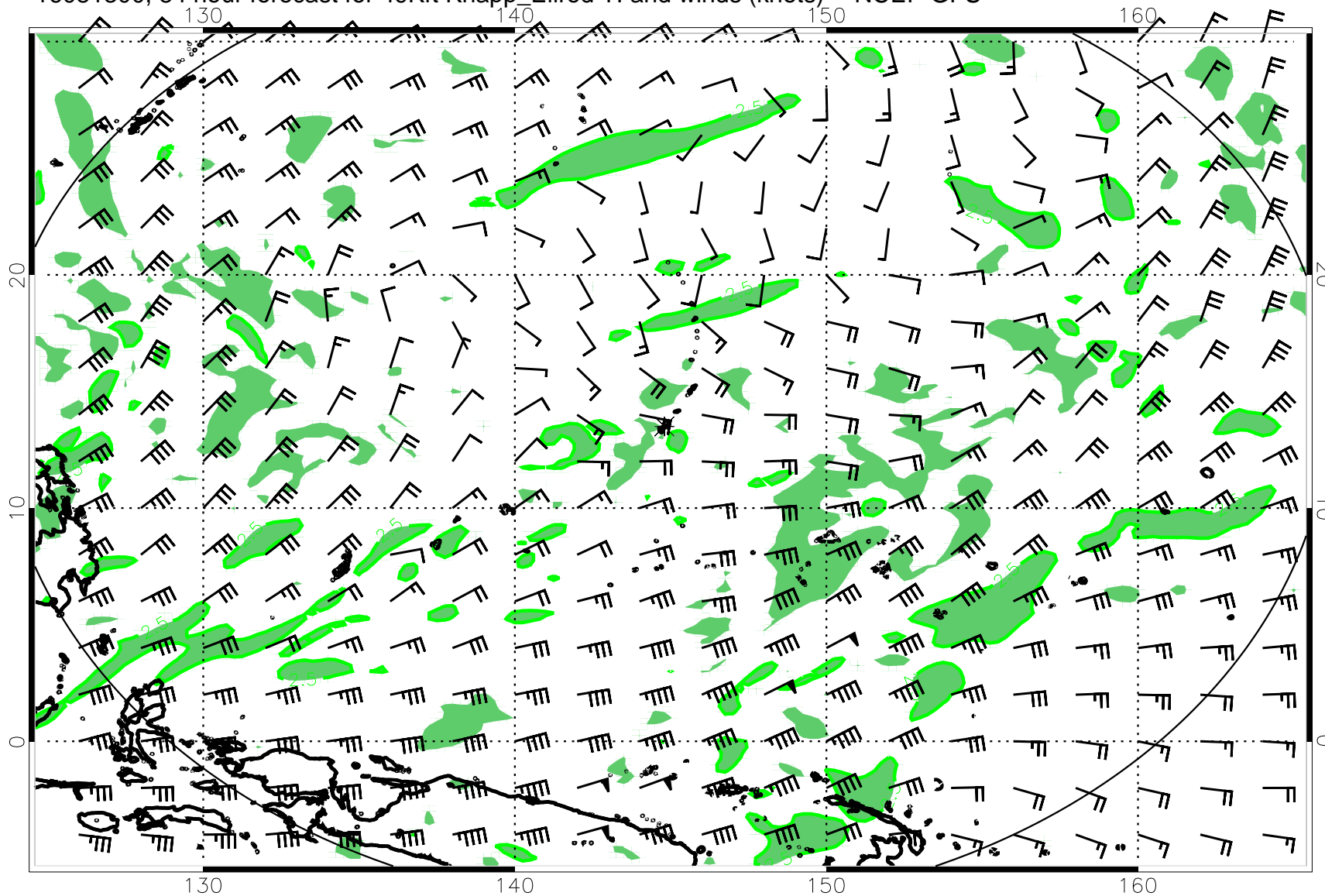
16081300, 84 hour forecast for 49Kft Knapp_Ellrod TI and winds (knots) -- NCEP GFS
