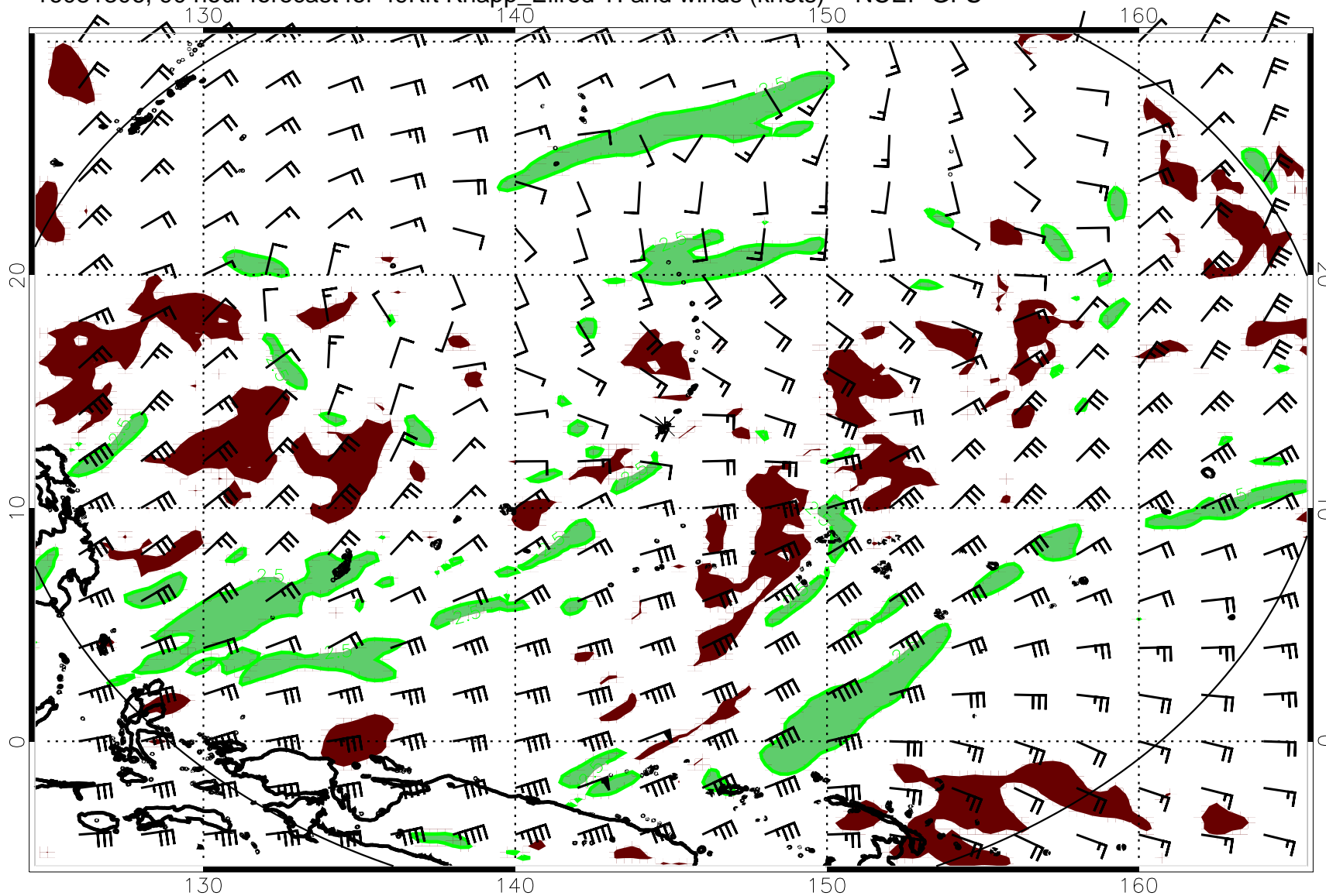
16081306, 90 hour forecast for 49Kft Knapp_Ellrod TI and winds (knots) -- NCEP GFS
