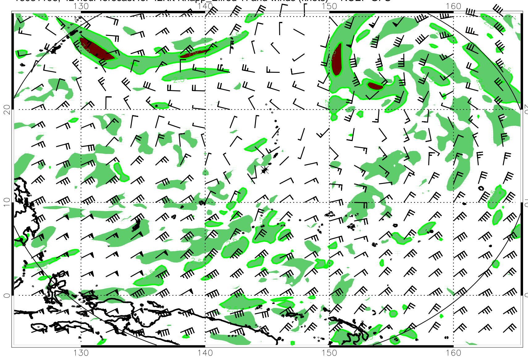
16081106, 42 hour forecast for 42Kft Knapp_Ellrod TI and winds (knots) -- NCEP GFS
