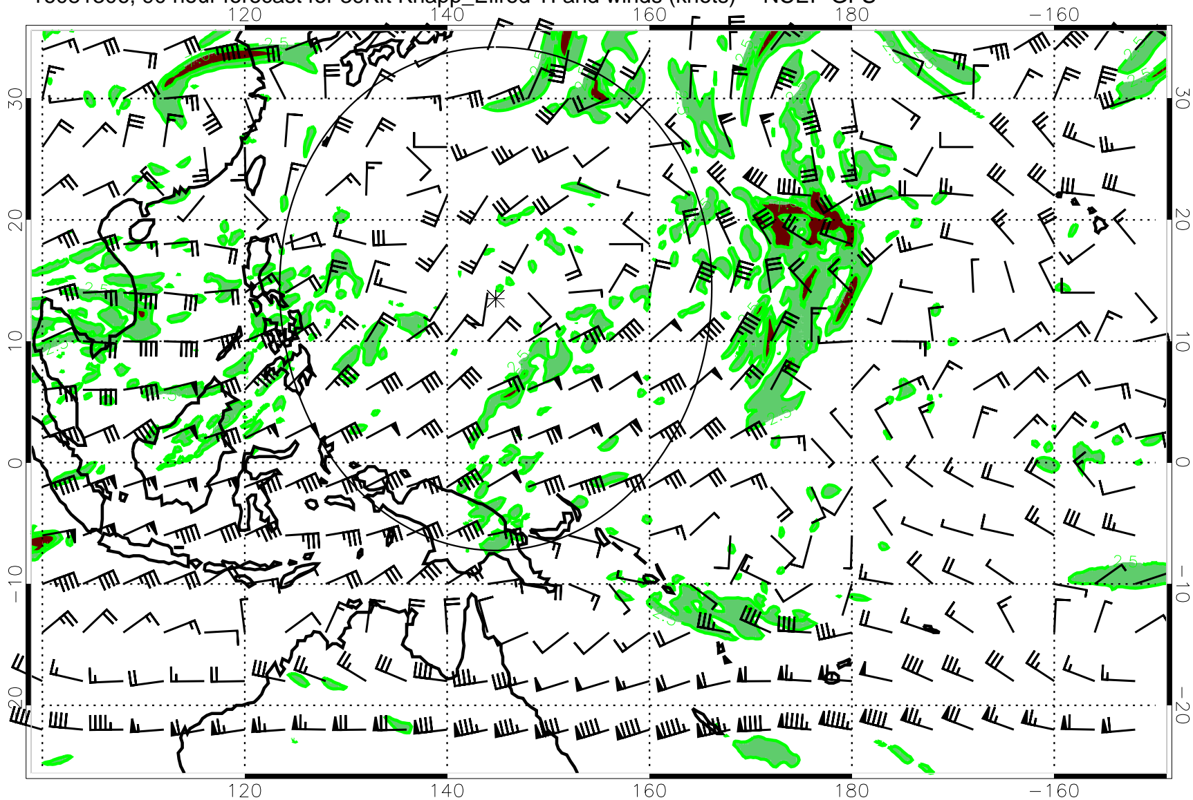
16081306, 90 hour forecast for 39Kft Knapp_Ellrod TI and winds (knots) -- NCEP GFS
