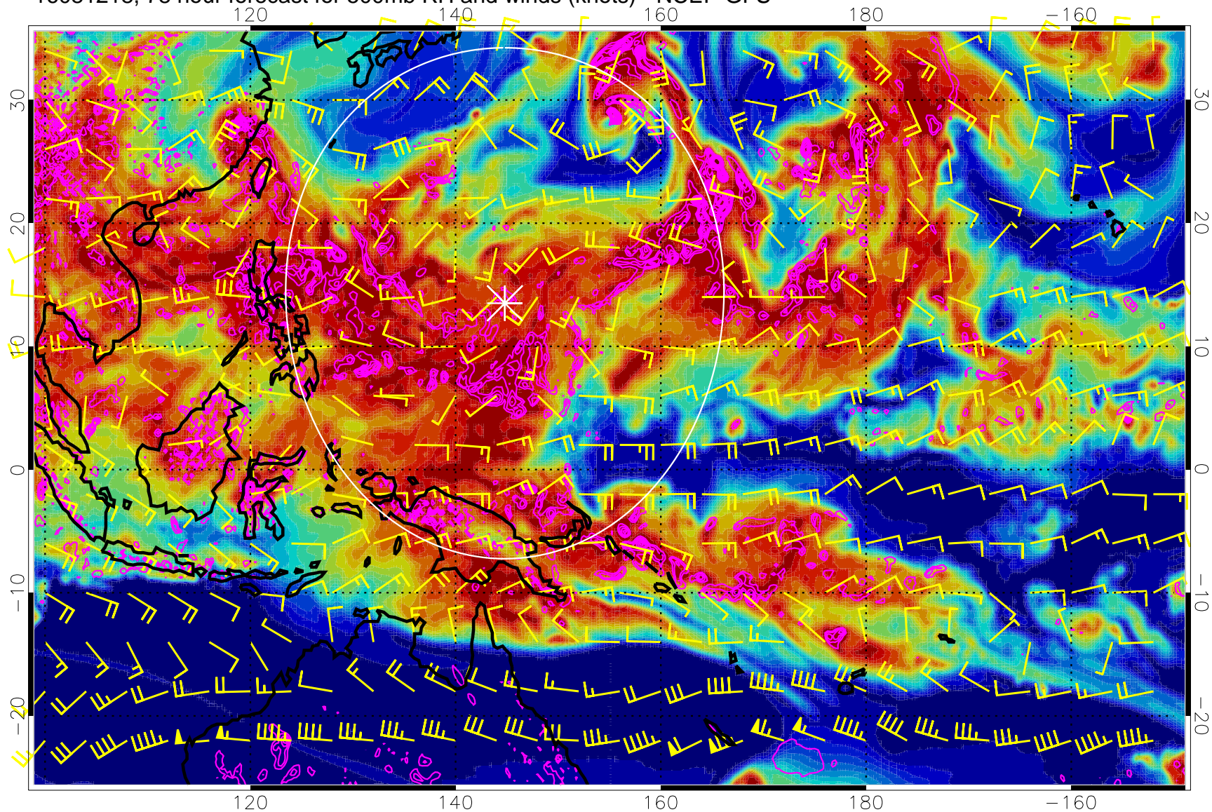
16081218, 78 hour forecast for 500mb RH and winds (knots) - NCEP GFS
