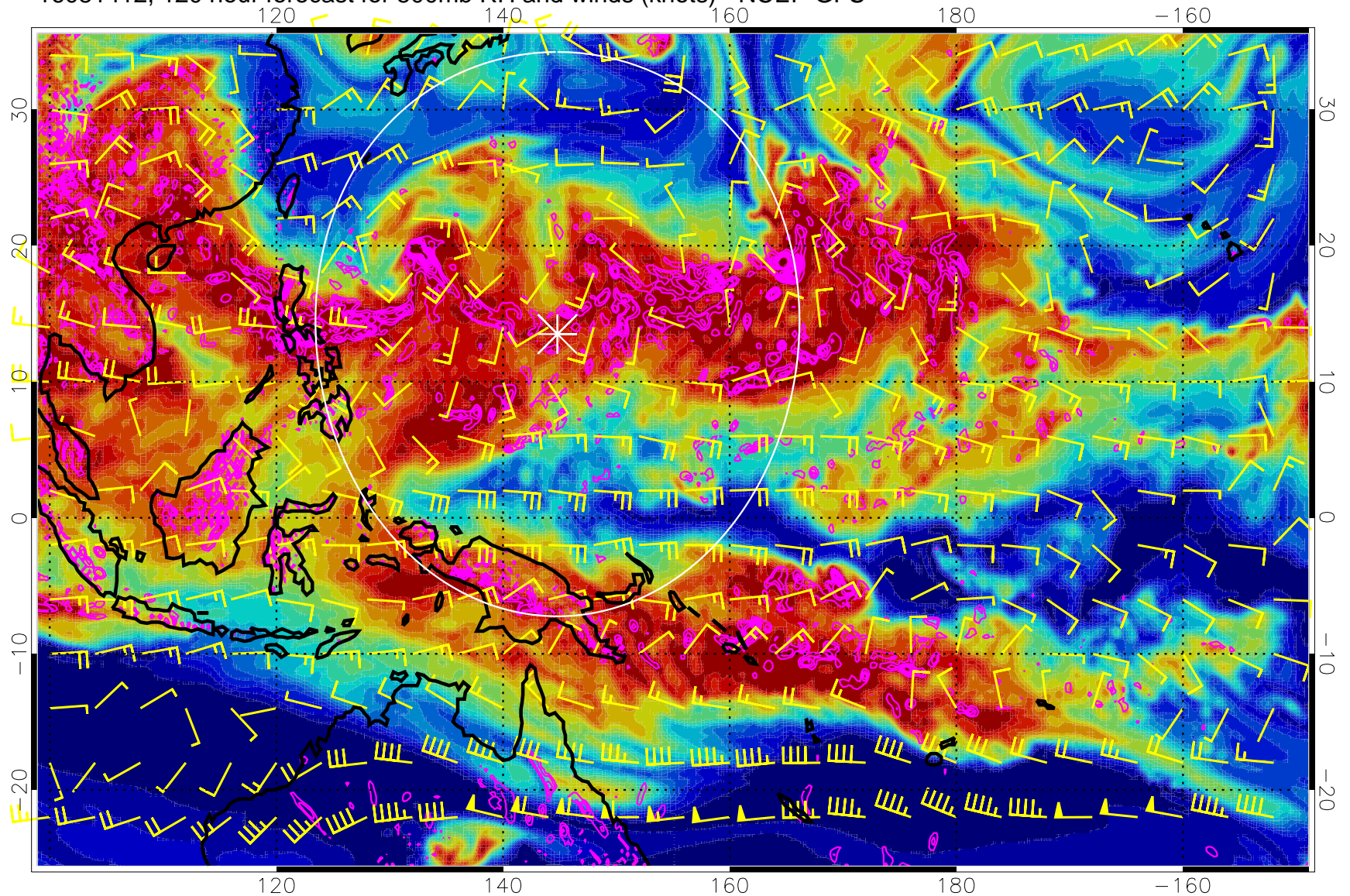
16081412, 120 hour forecast for 500mb RH and winds (knots) - NCEP GFS
