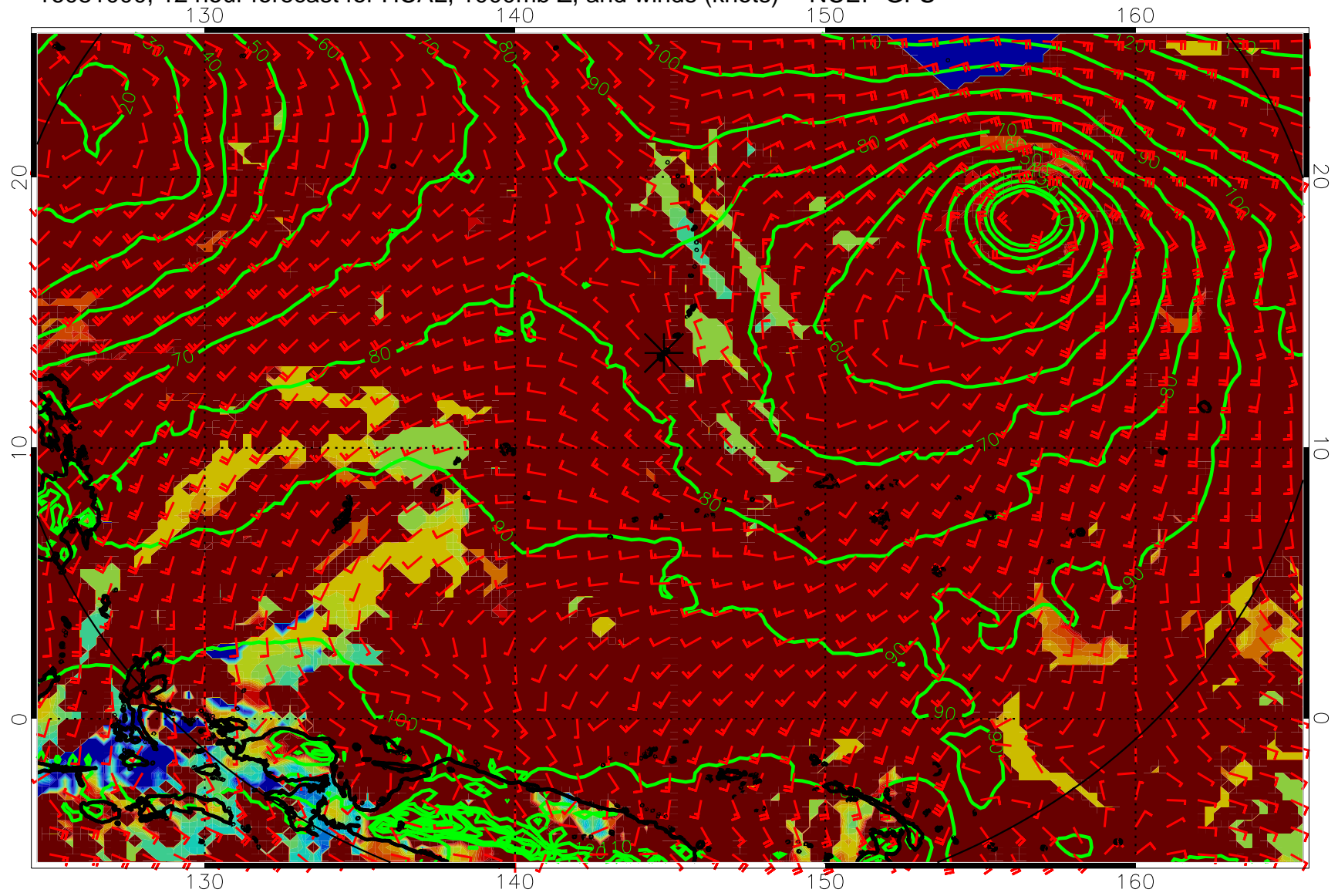
16081000, 12 hour forecast for HCAL, 1000mb Z, and winds (knots) -- NCEP GFS
