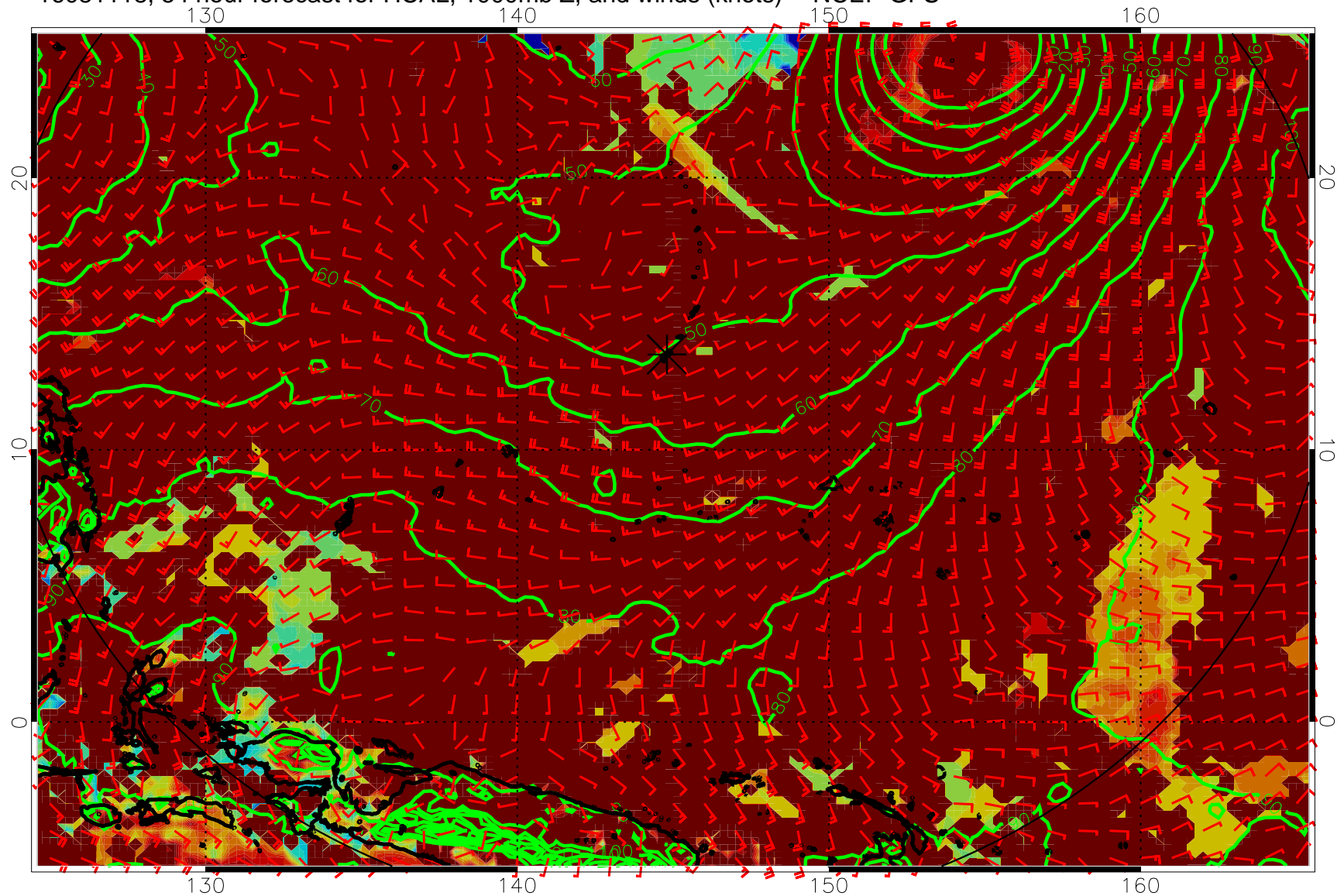
16081118, 54 hour forecast for HCAL, 1000mb Z, and winds (knots) -- NCEP GFS
