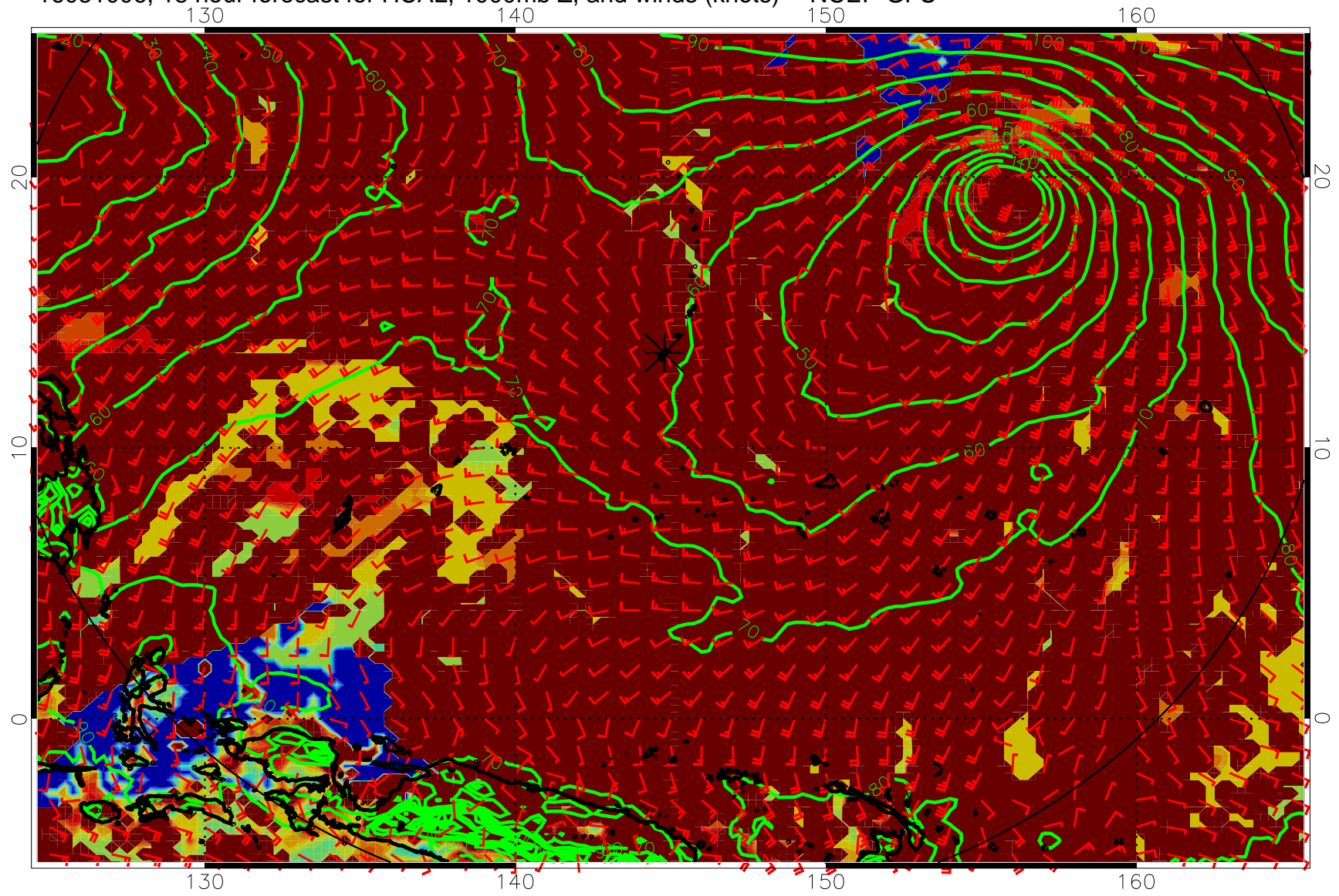
16081006, 18 hour forecast for HCAL, 1000mb Z, and winds (knots) -- NCEP GFS
