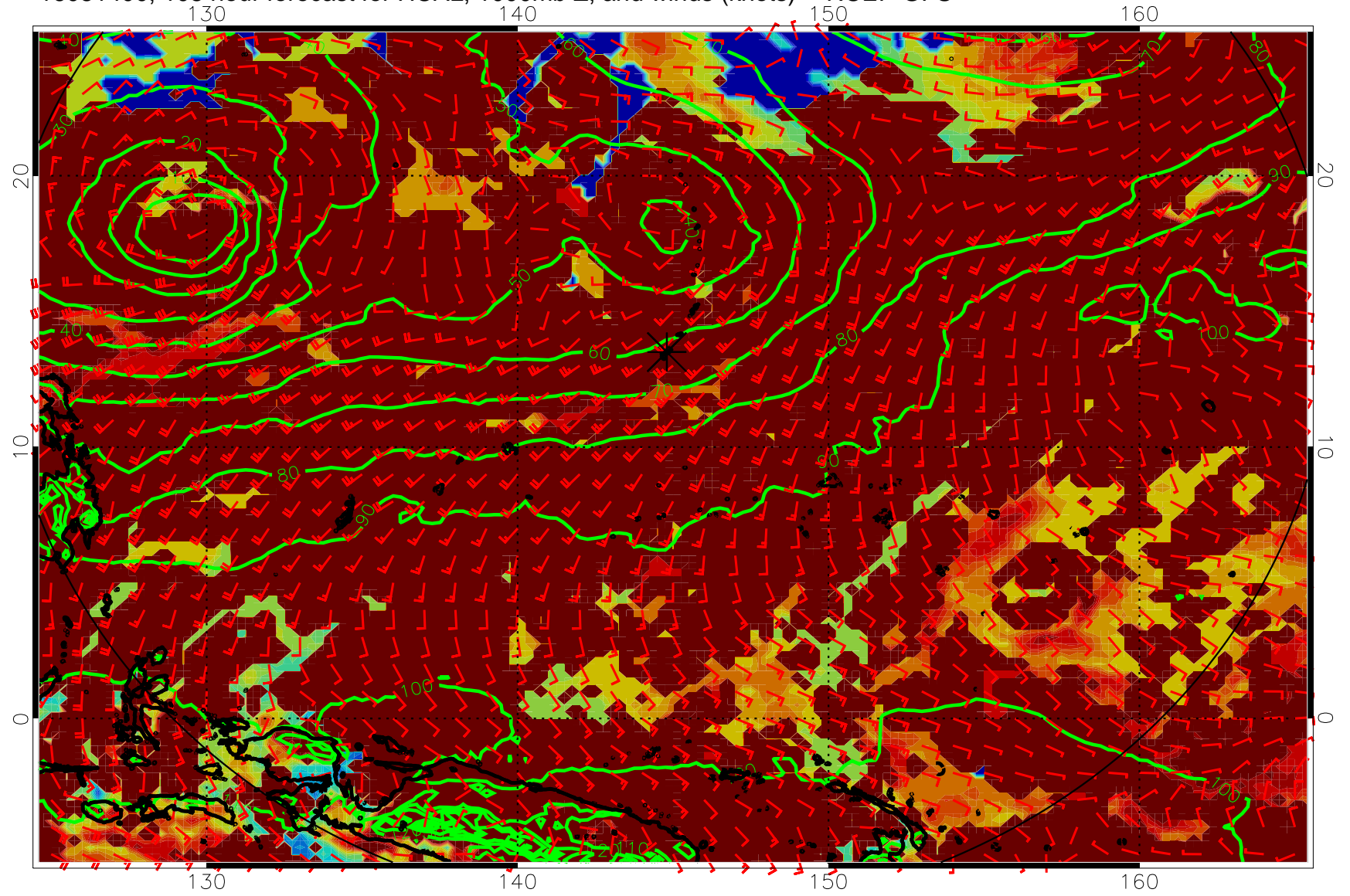
16081400, 108 hour forecast for HCAL, 1000mb Z, and winds (knots) -- NCEP GFS
