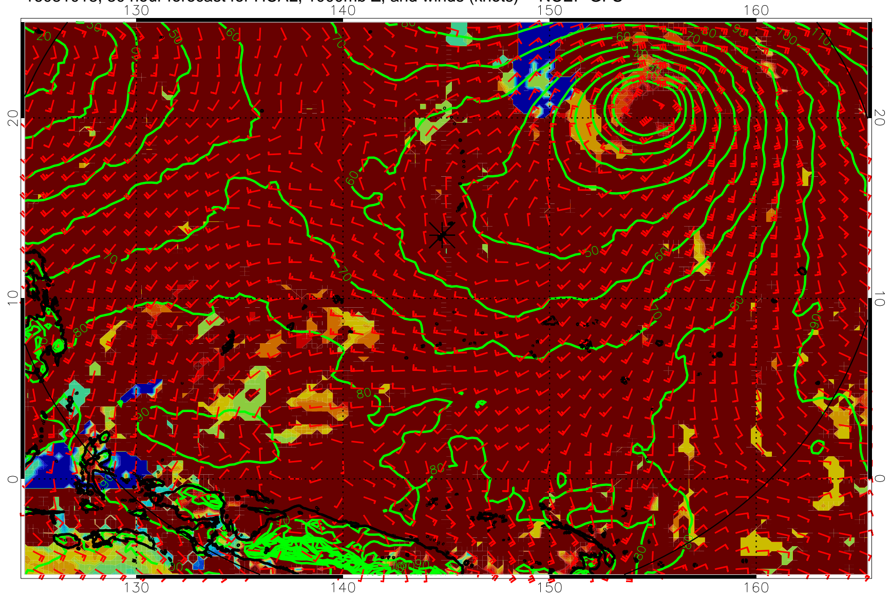
16081018, 30 hour forecast for HCAL, 1000mb Z, and winds (knots) -- NCEP GFS
