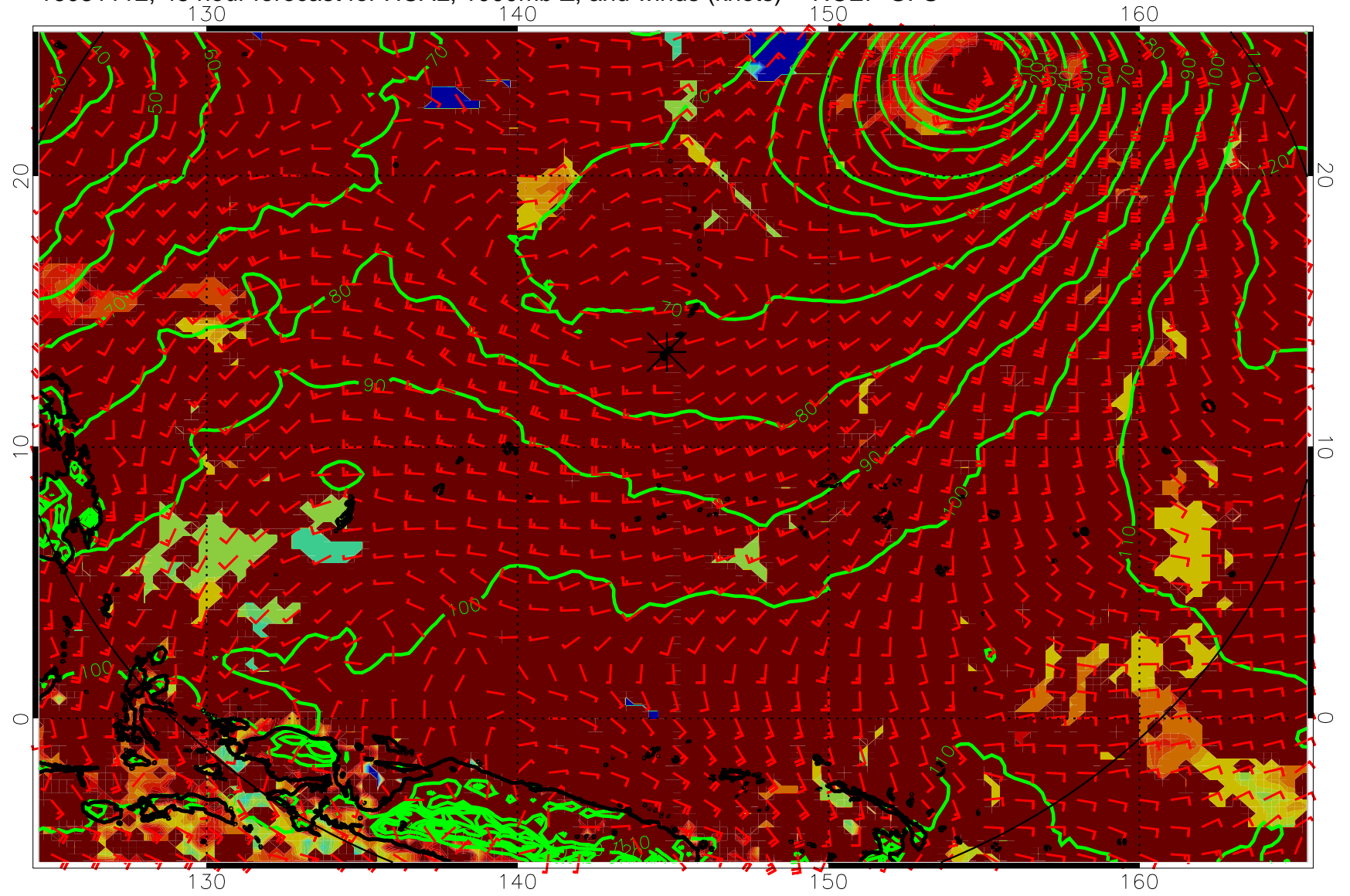
16081112, 48 hour forecast for HCAL, 1000mb Z, and winds (knots) -- NCEP GFS
