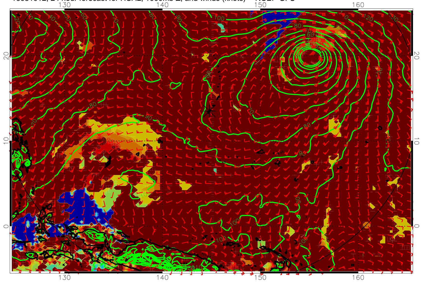
16081012, 24 hour forecast for HCAL, 1000mb Z, and winds (knots) -- NCEP GFS
