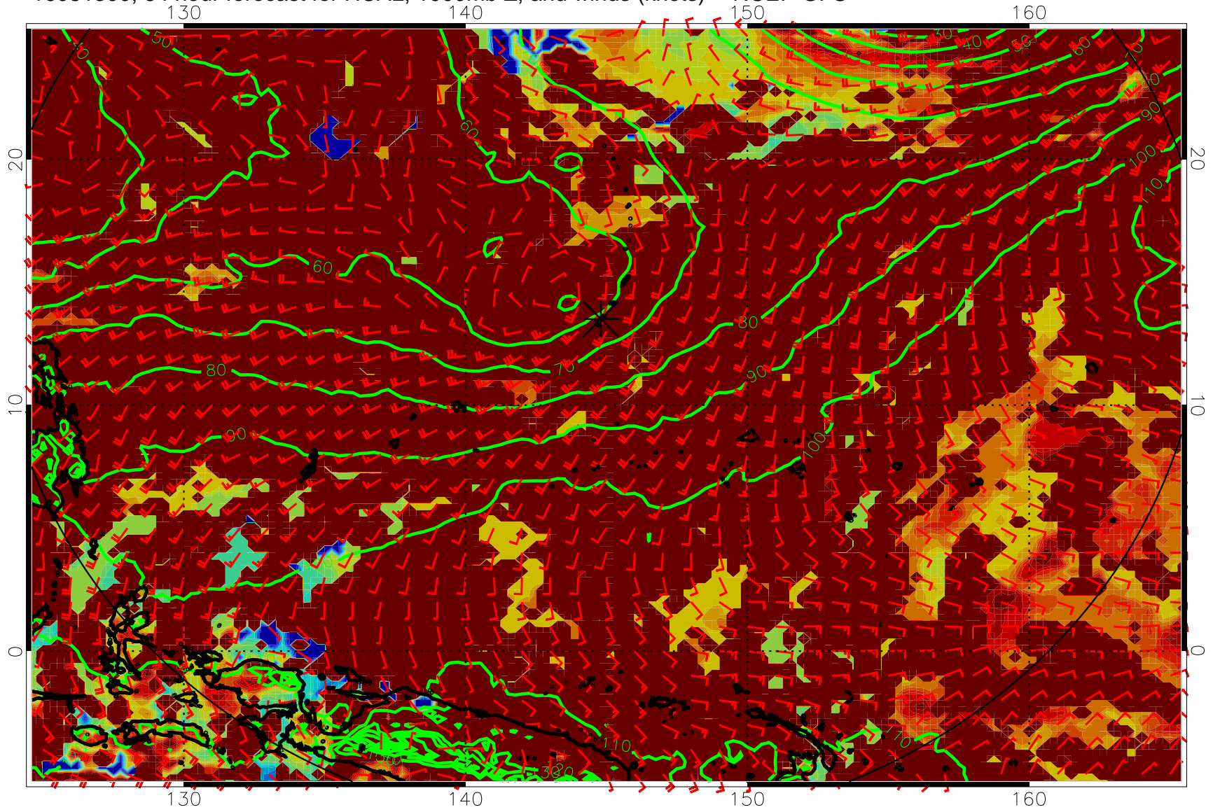
16081300, 84 hour forecast for HCAL, 1000mb Z, and winds (knots) -- NCEP GFS
