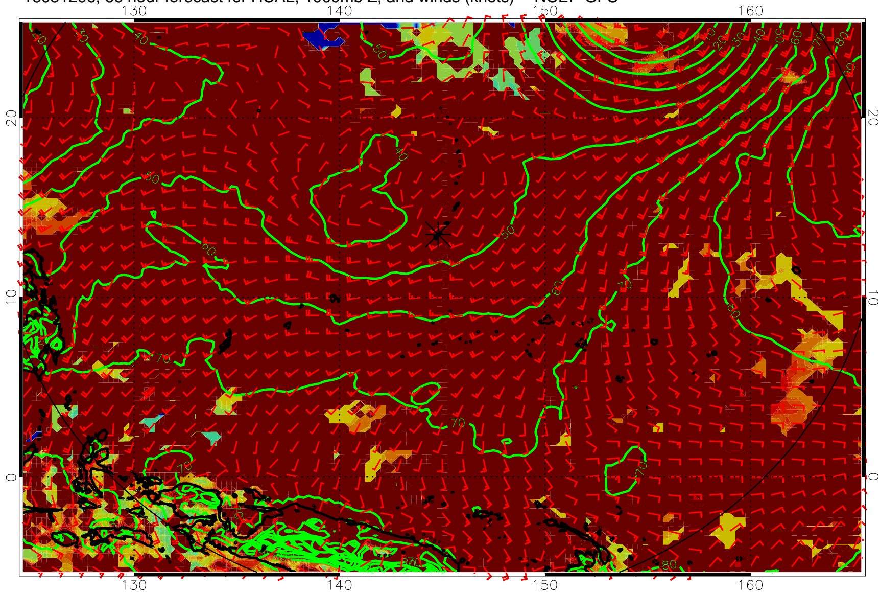
16081206, 66 hour forecast for HCAL, 1000mb Z, and winds (knots) -- NCEP GFS
