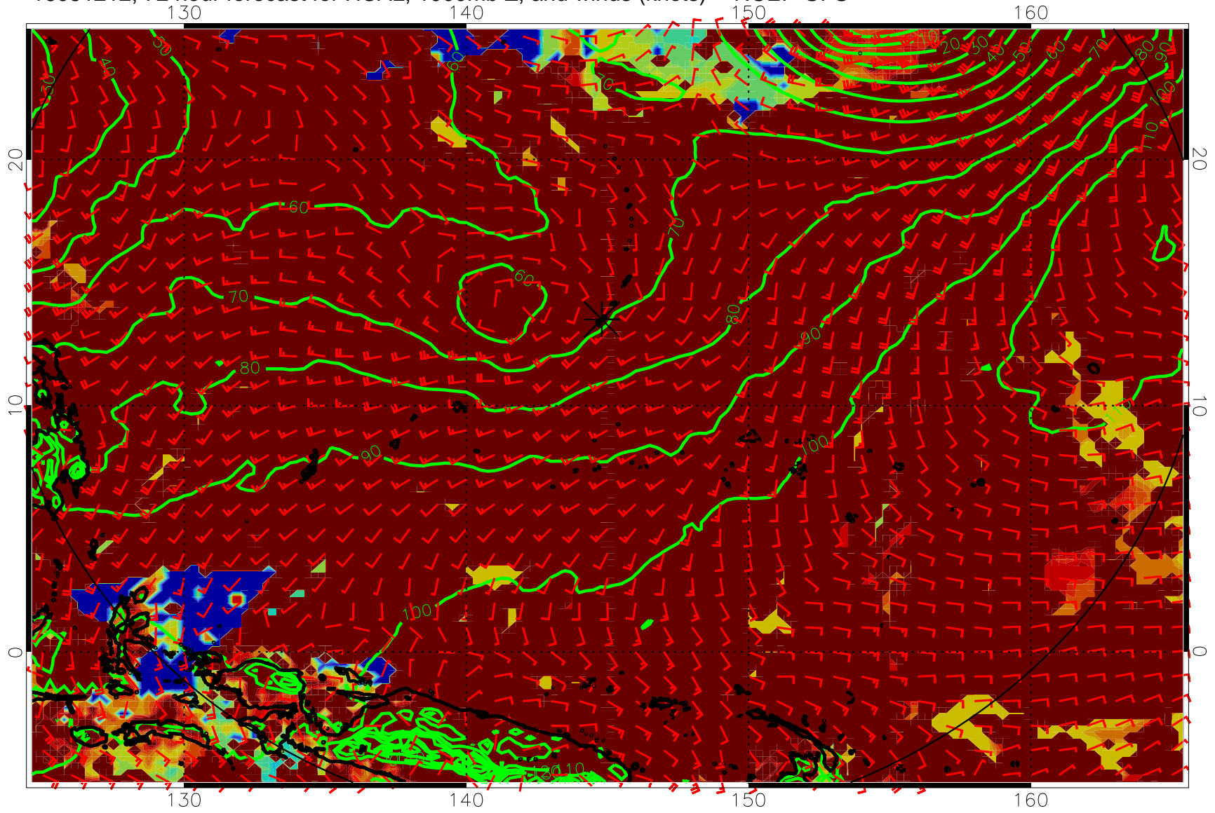
16081212, 72 hour forecast for HCAL, 1000mb Z, and winds (knots) -- NCEP GFS
