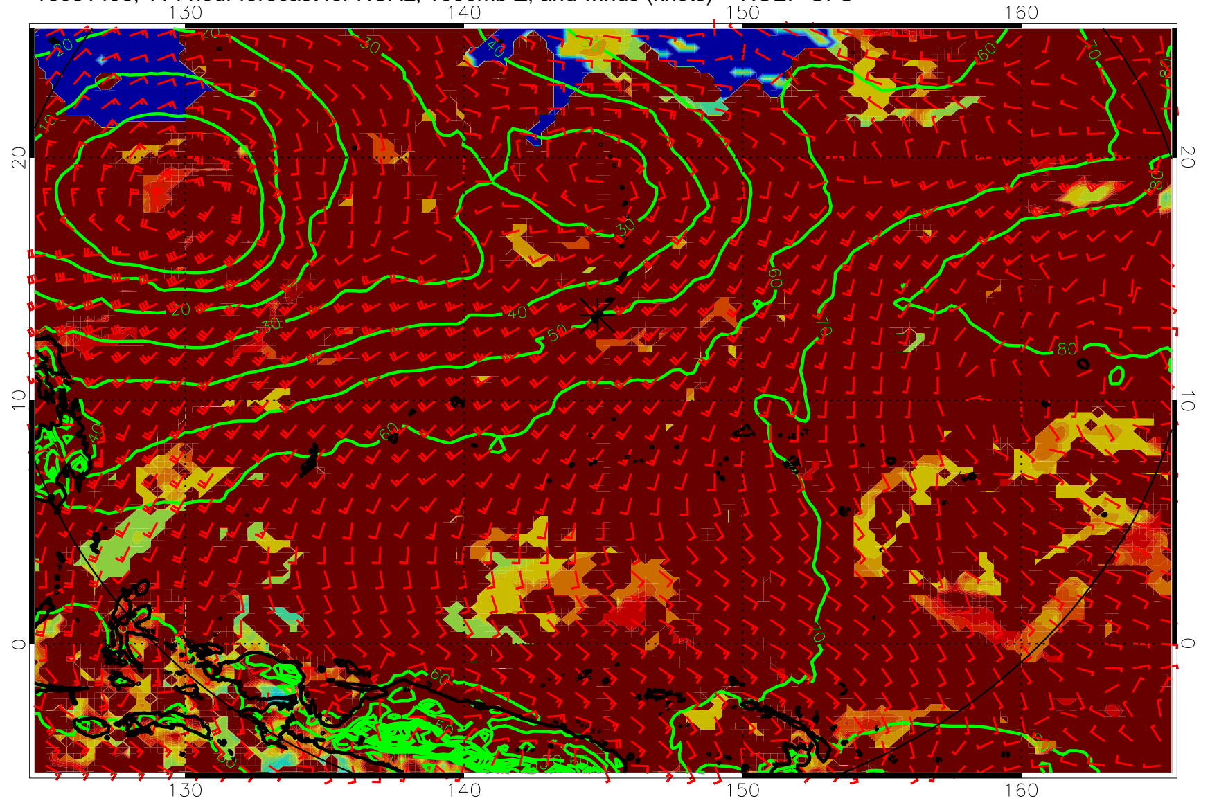
16081406, 114 hour forecast for HCAL, 1000mb Z, and winds (knots) -- NCEP GFS
