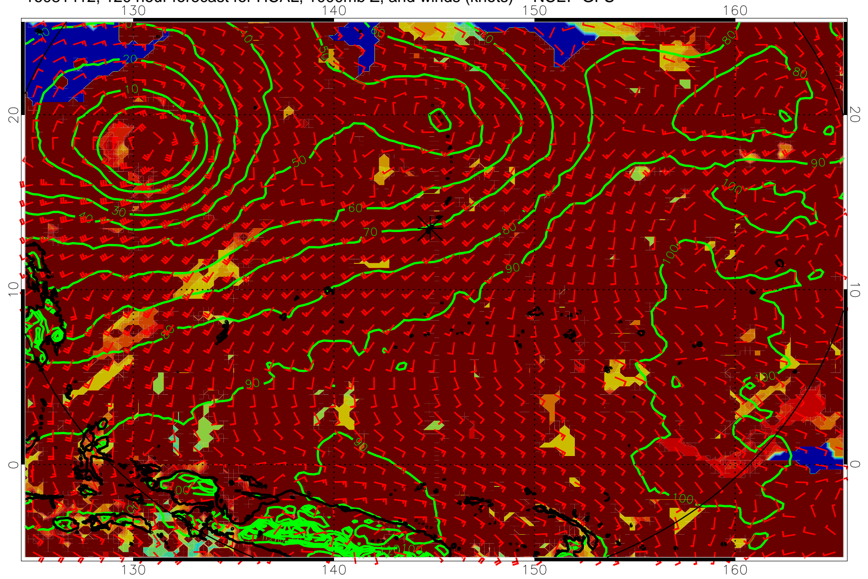
16081412, 120 hour forecast for HCAL, 1000mb Z, and winds (knots) -- NCEP GFS
