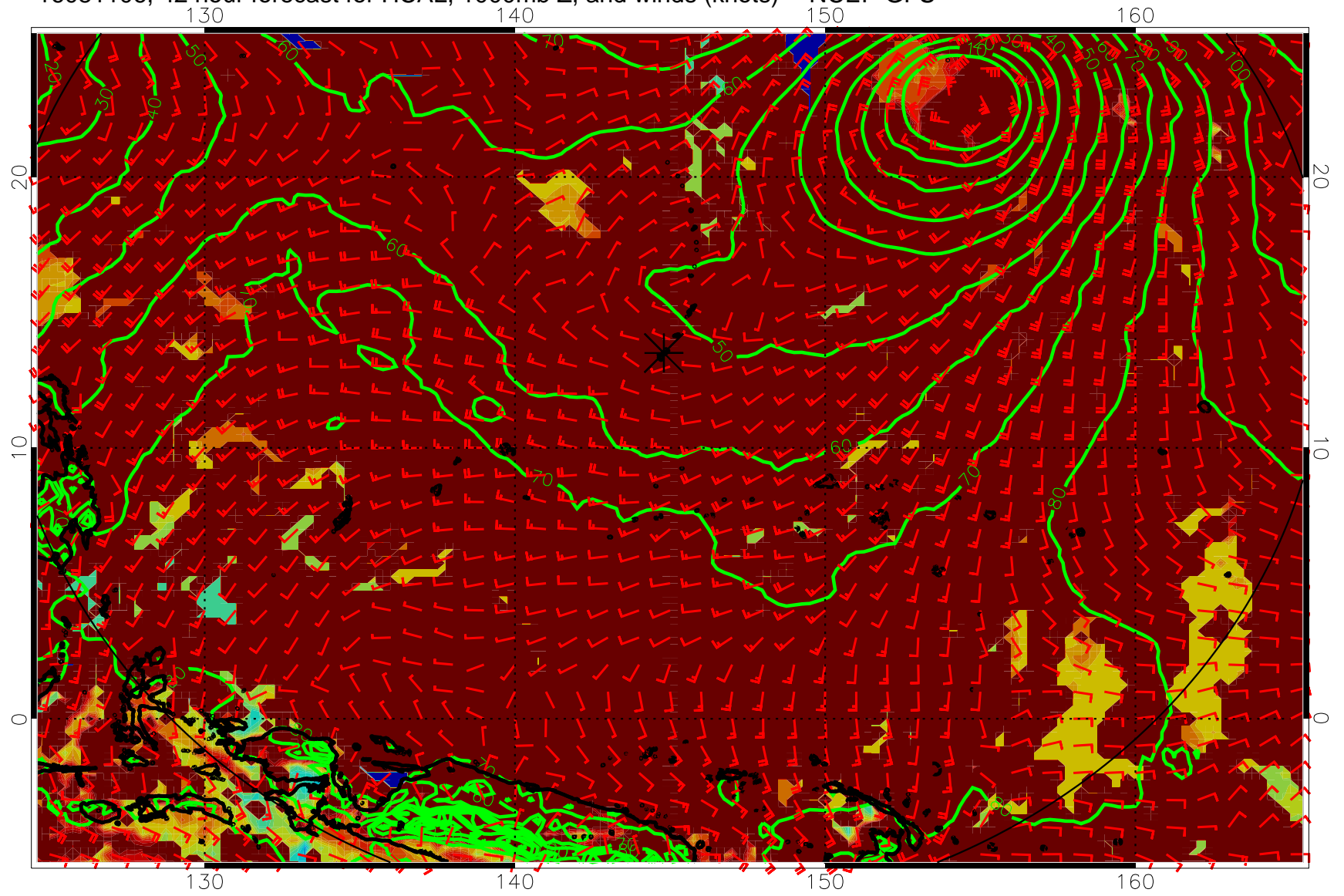
16081106, 42 hour forecast for HCAL, 1000mb Z, and winds (knots) -- NCEP GFS
