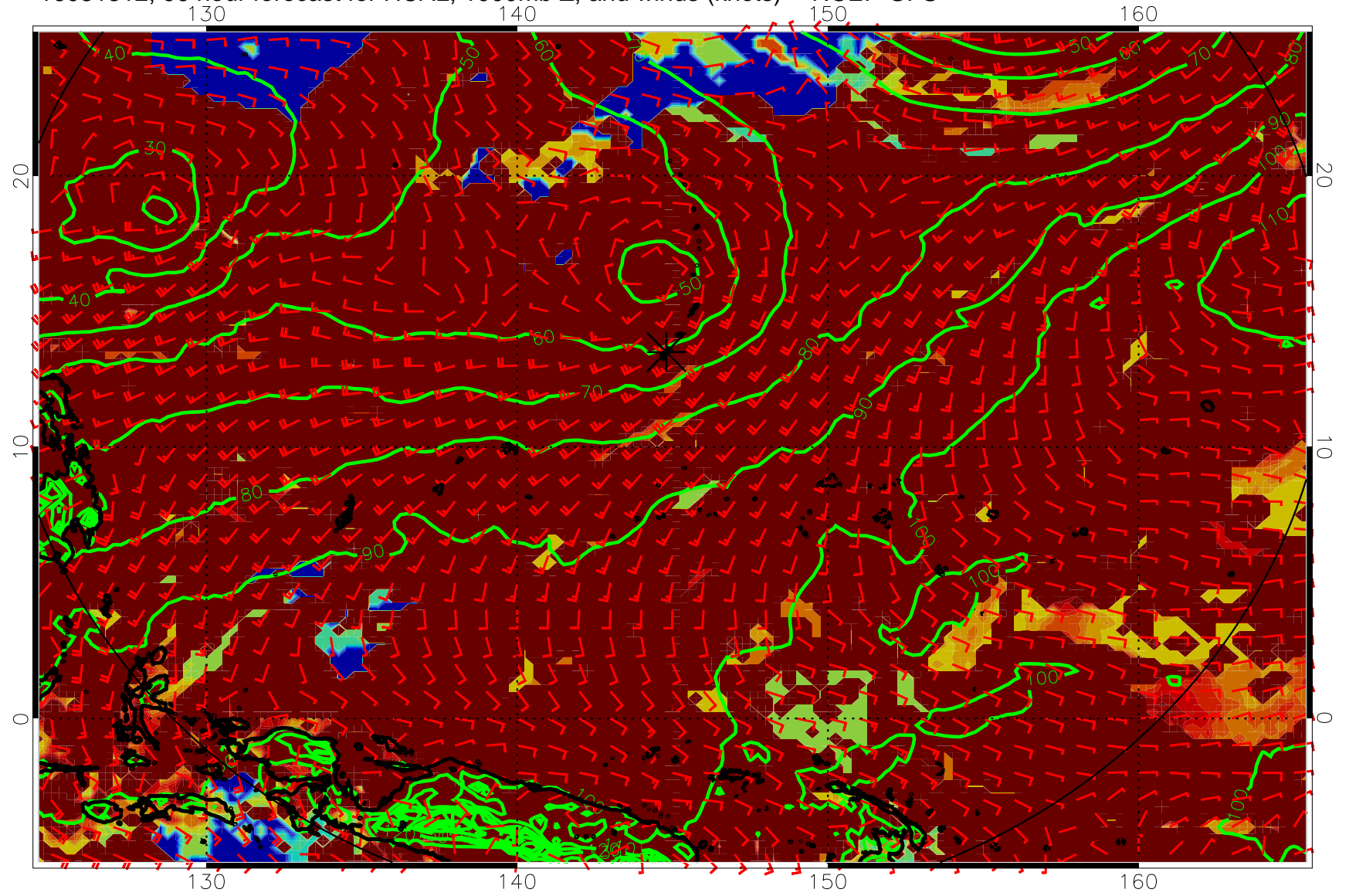
16081312, 96 hour forecast for HCAL, 1000mb Z, and winds (knots) -- NCEP GFS
