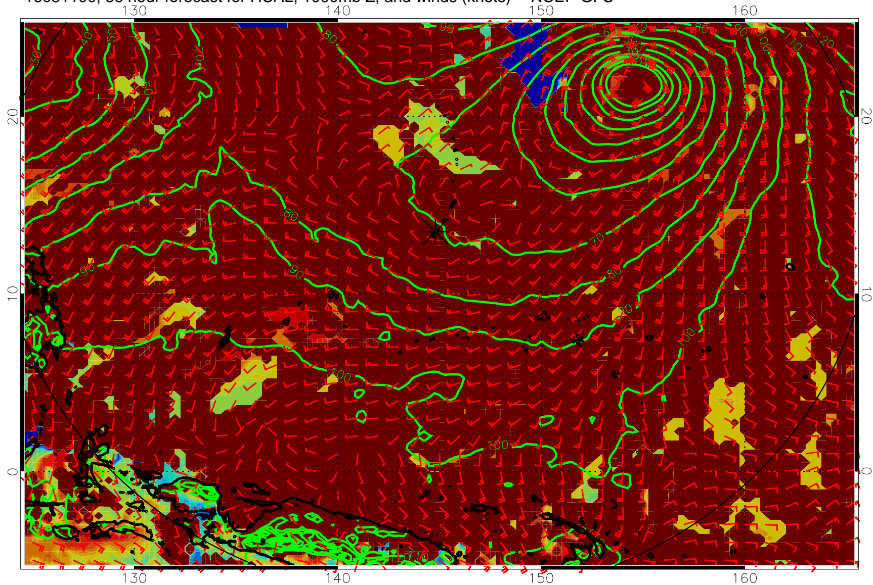
16081100, 36 hour forecast for HCAL, 1000mb Z, and winds (knots) -- NCEP GFS
