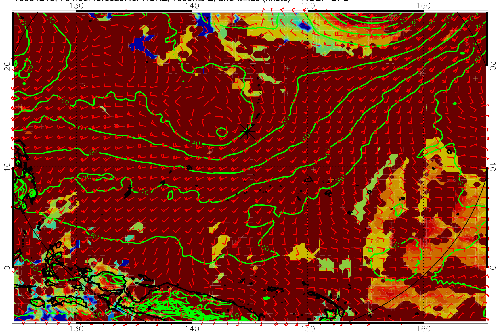
16081218, 78 hour forecast for HCAL, 1000mb Z, and winds (knots) -- NCEP GFS
