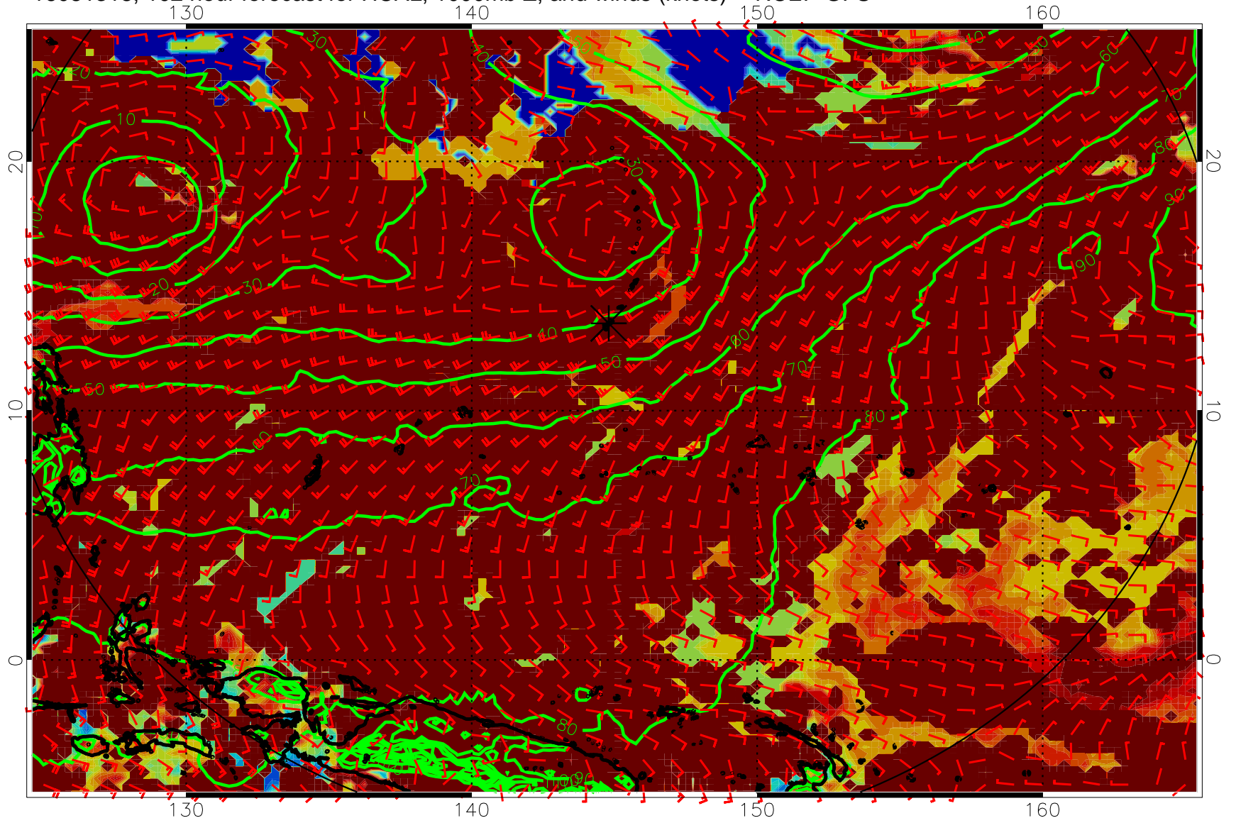
16081318, 102 hour forecast for HCAL, 1000mb Z, and winds (knots) -- NCEP GFS
