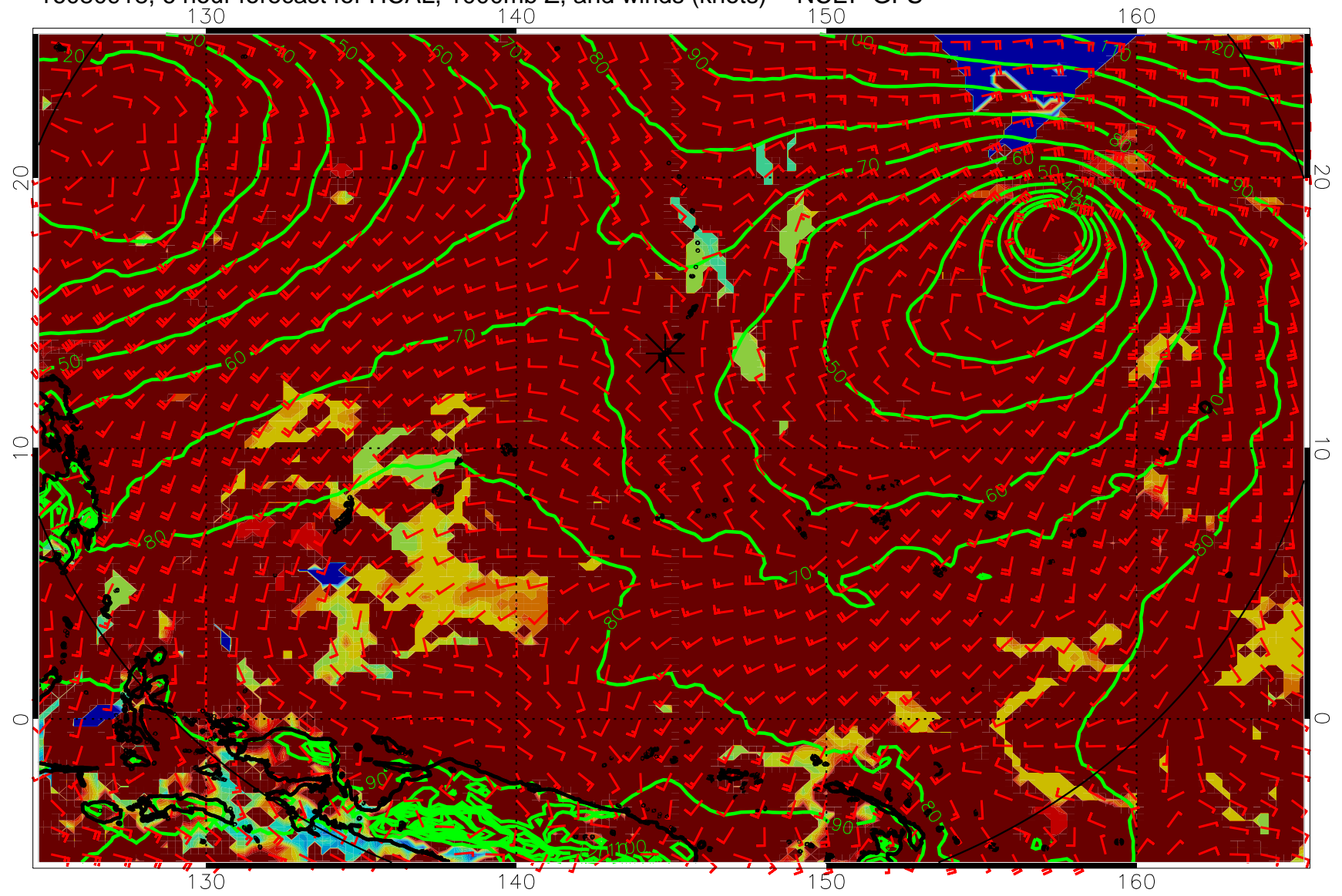
16080918, 6 hour forecast for HCAL, 1000mb Z, and winds (knots) -- NCEP GFS
