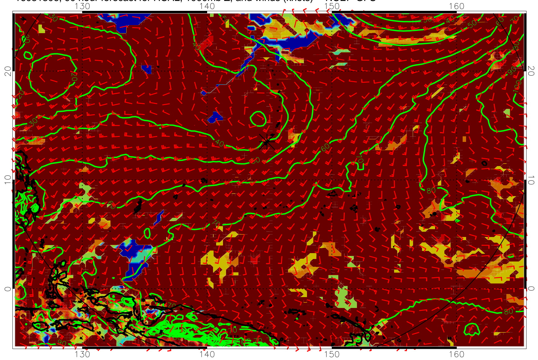
16081306, 90 hour forecast for HCAL, 1000mb Z, and winds (knots) -- NCEP GFS
