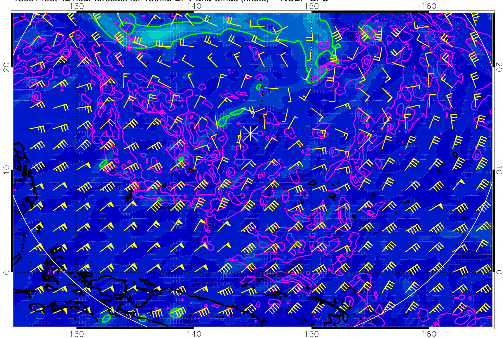
16081106, 42 hour forecast for 150mb EPV and winds (knots) -- NCEP GFS
