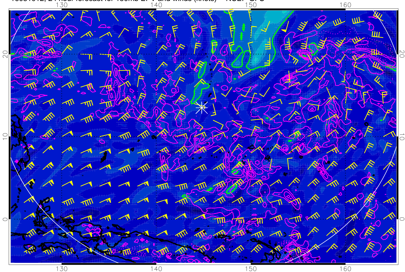
16081012, 24 hour forecast for 150mb EPV and winds (knots) -- NCEP GFS
