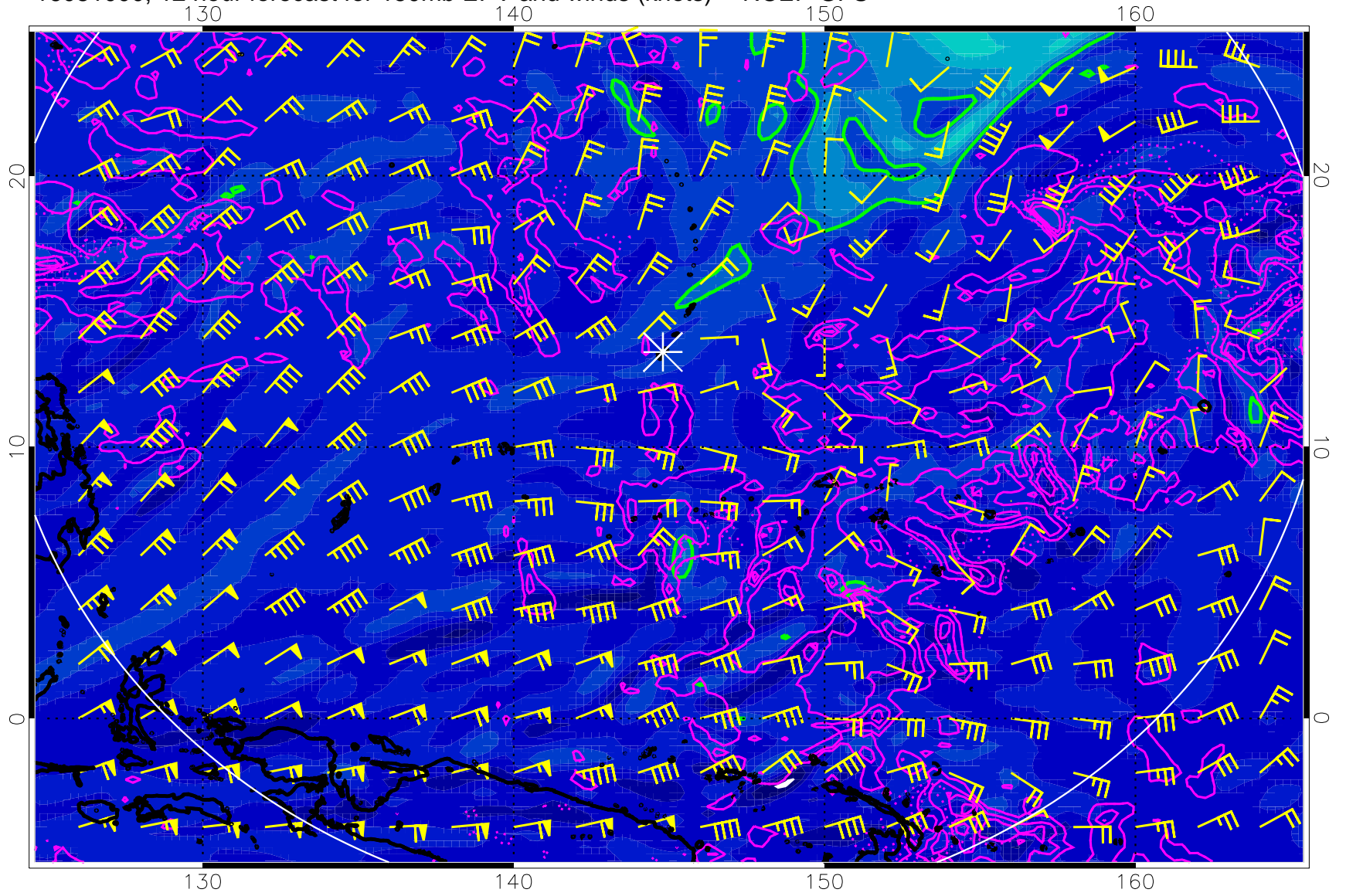
16081000, 12 hour forecast for 150mb EPV and winds (knots) -- NCEP GFS
