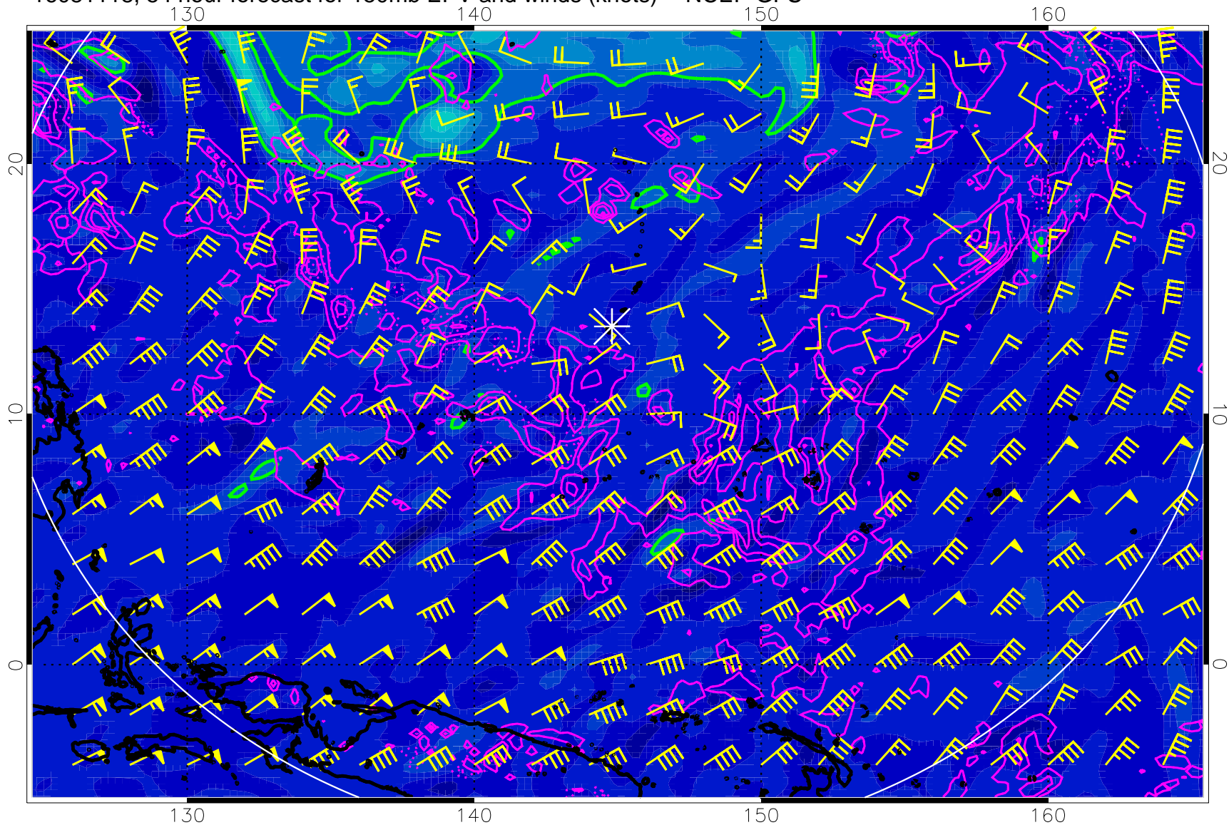
16081118, 54 hour forecast for 150mb EPV and winds (knots) -- NCEP GFS
