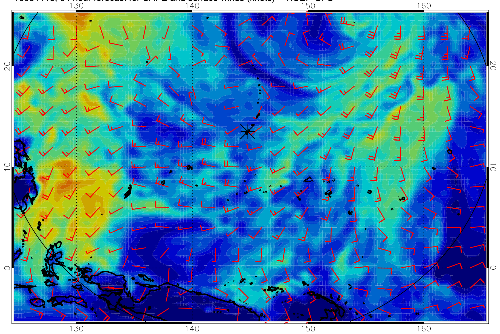
16081118, 54 hour forecast for CAPE and surface winds (knots) -- NCEP GFS
