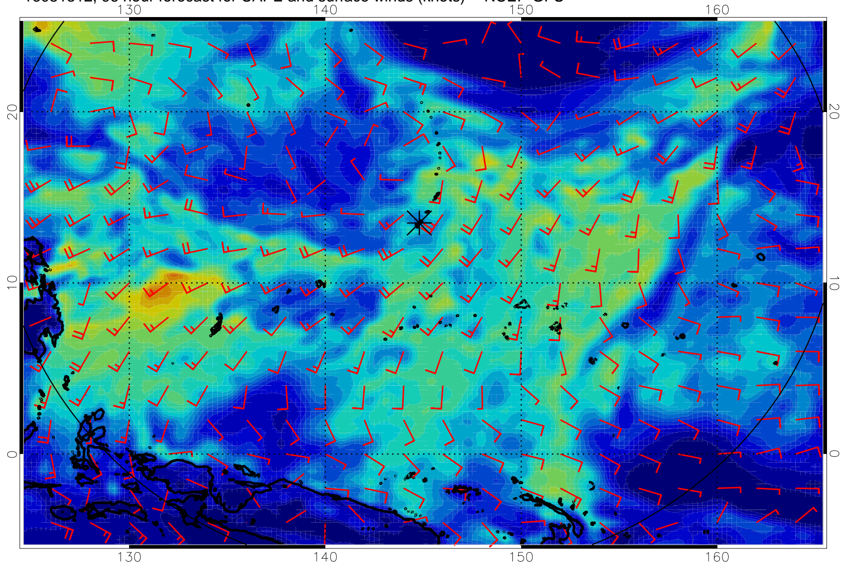
16081312, 96 hour forecast for CAPE and surface winds (knots) -- NCEP GFS
