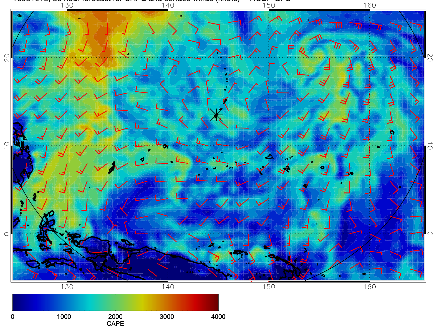
16081018, 30 hour forecast for CAPE and surface winds (knots) -- NCEP GFS
