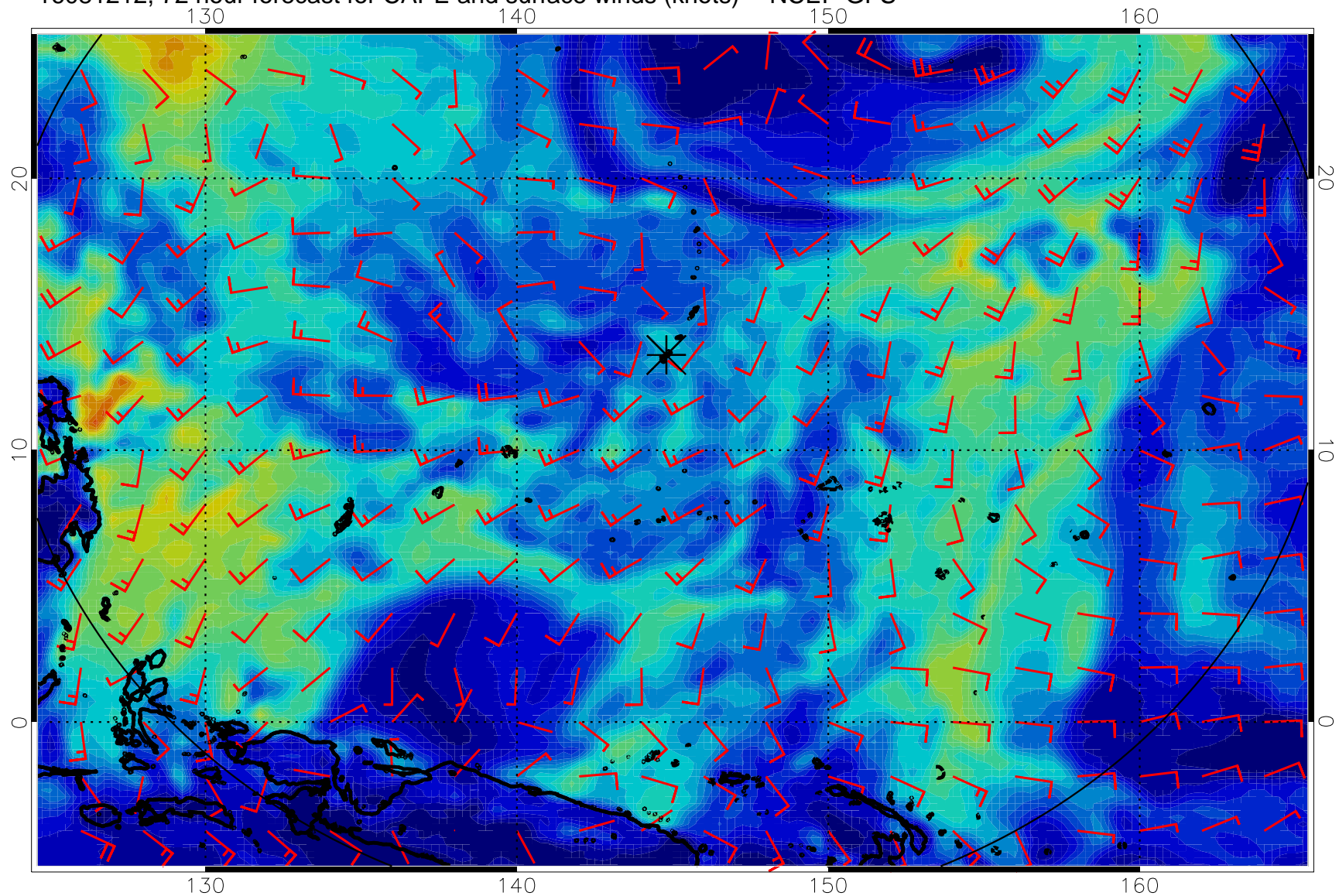
16081212, 72 hour forecast for CAPE and surface winds (knots) -- NCEP GFS
