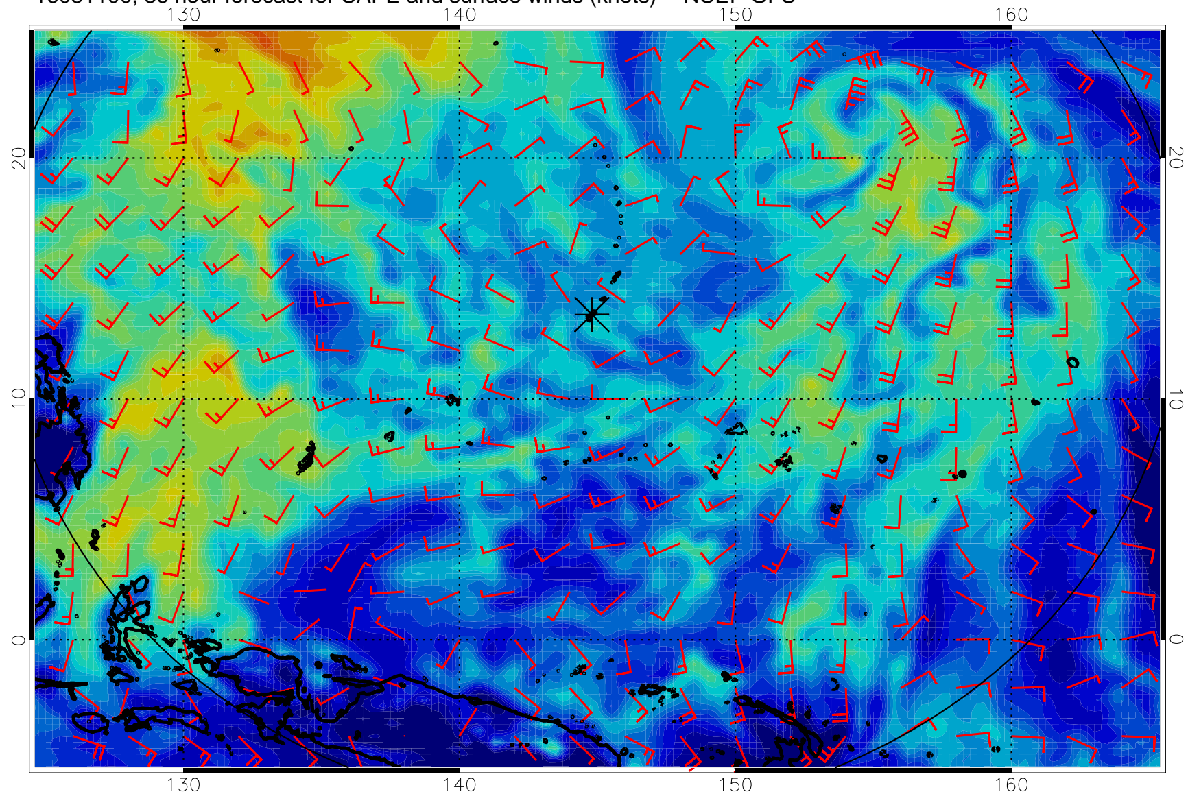
16081100, 36 hour forecast for CAPE and surface winds (knots) -- NCEP GFS
