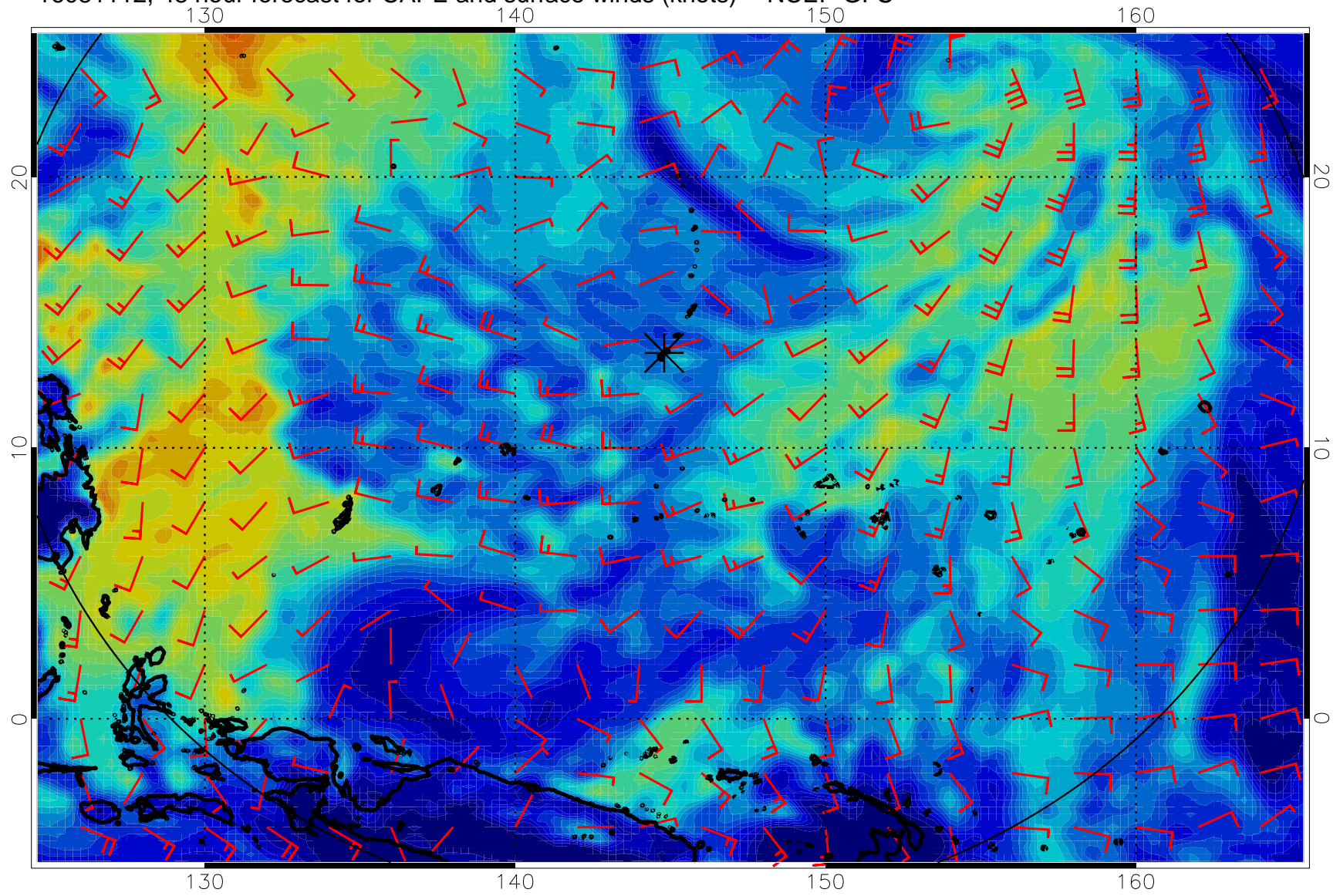
16081112, 48 hour forecast for CAPE and surface winds (knots) -- NCEP GFS
