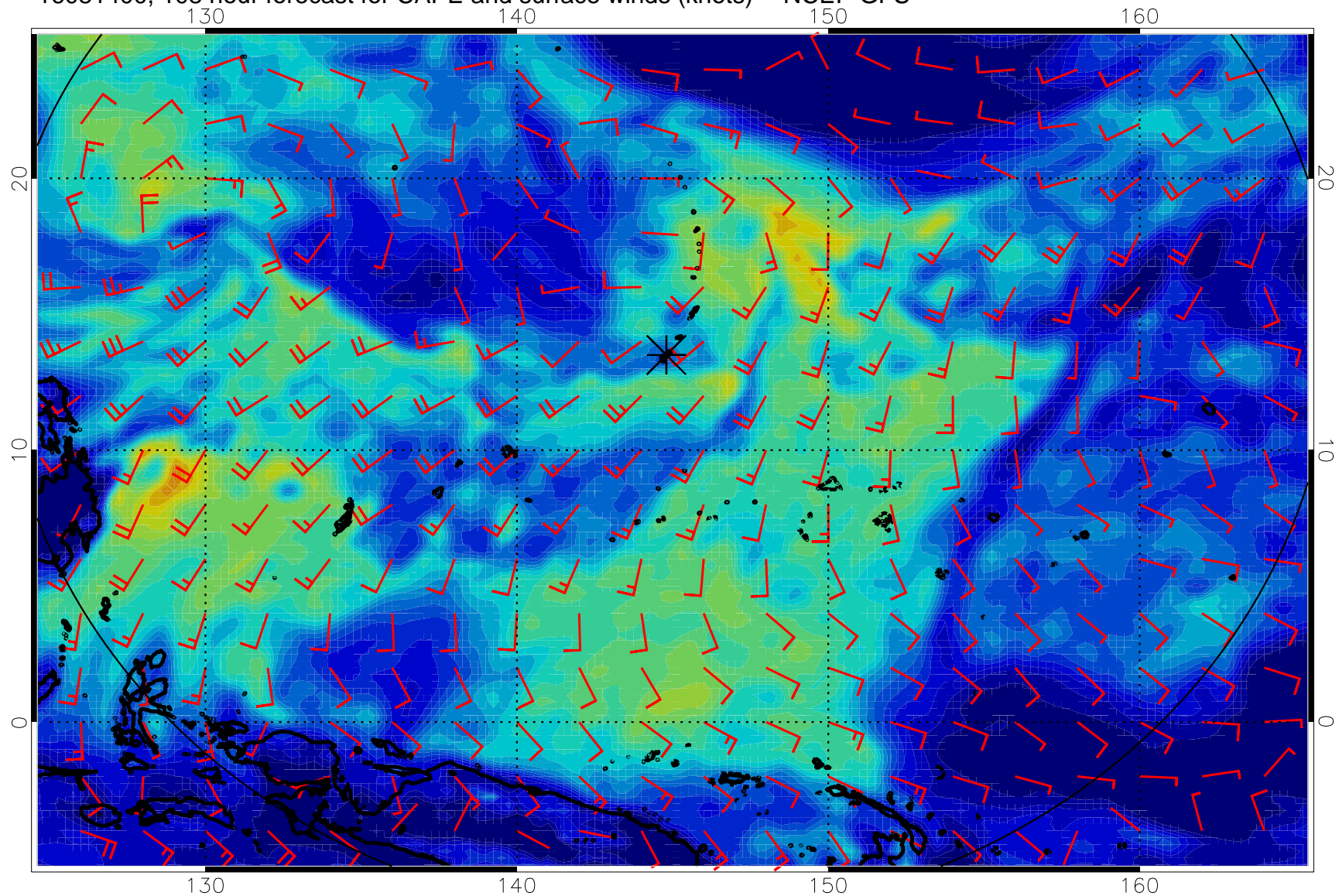
16081400, 108 hour forecast for CAPE and surface winds (knots) -- NCEP GFS
