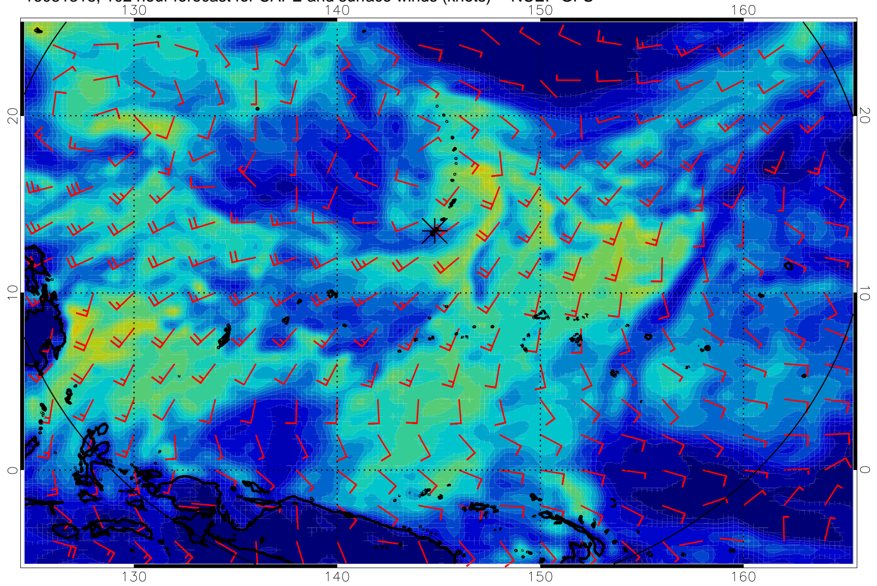
16081318, 102 hour forecast for CAPE and surface winds (knots) -- NCEP GFS
