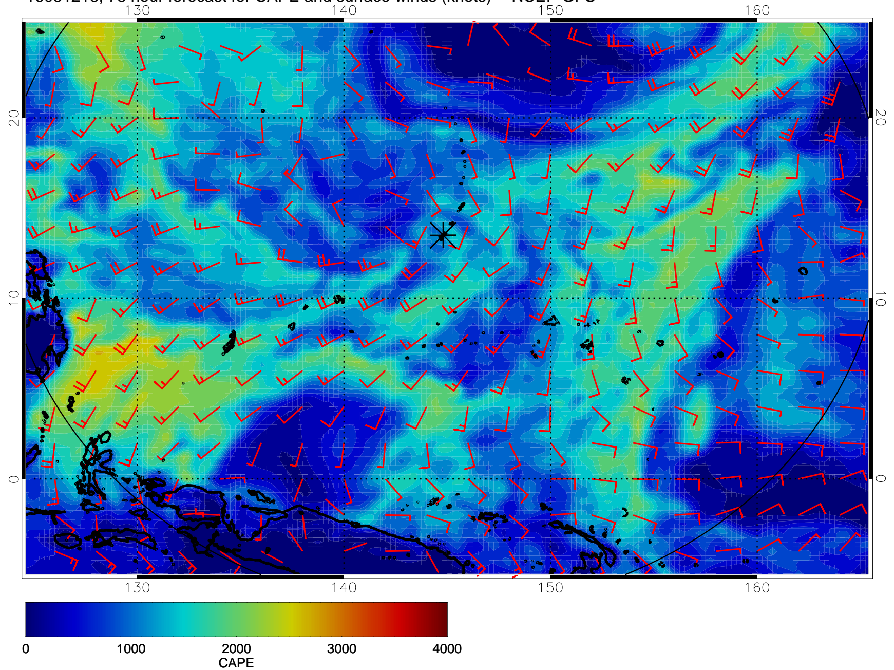
16081218, 78 hour forecast for CAPE and surface winds (knots) -- NCEP GFS
