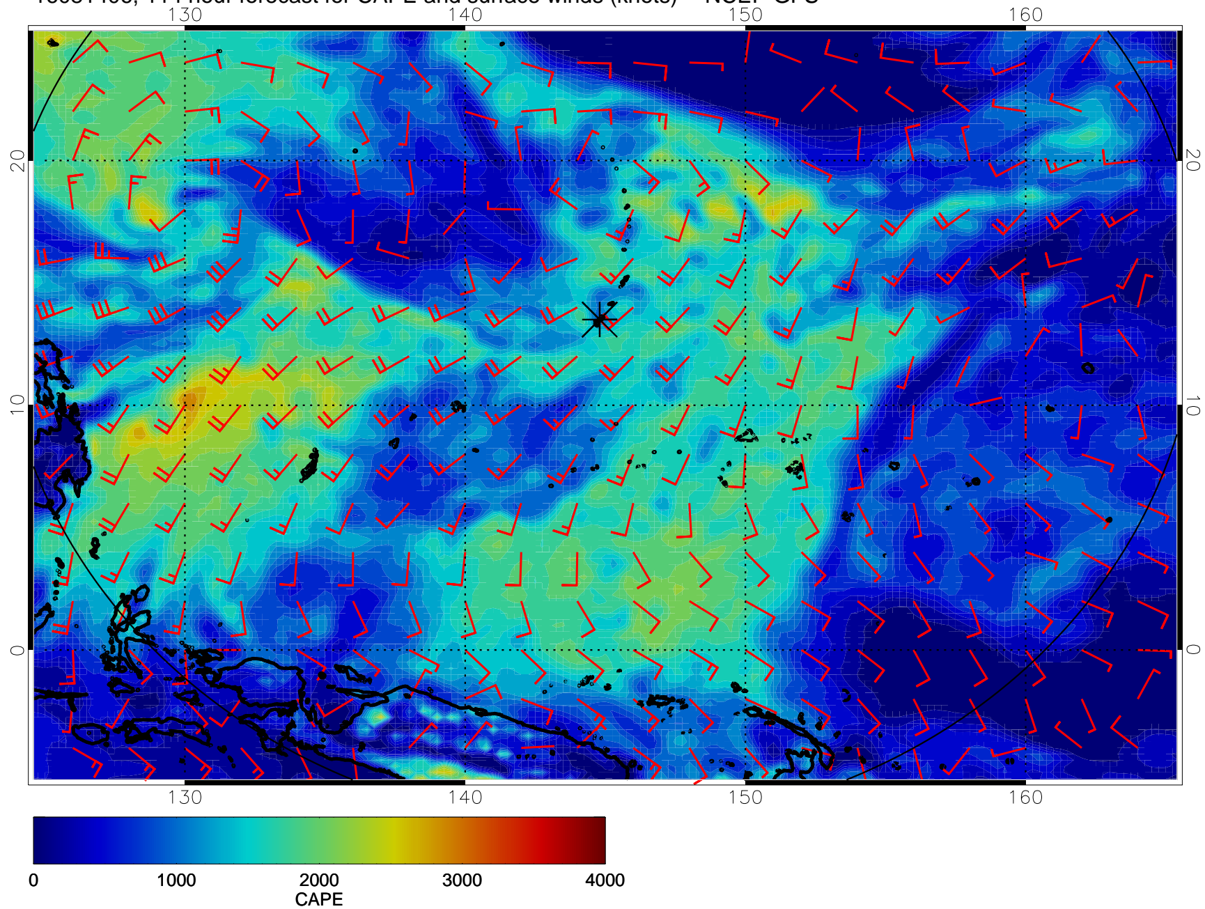
16081406, 114 hour forecast for CAPE and surface winds (knots) -- NCEP GFS
