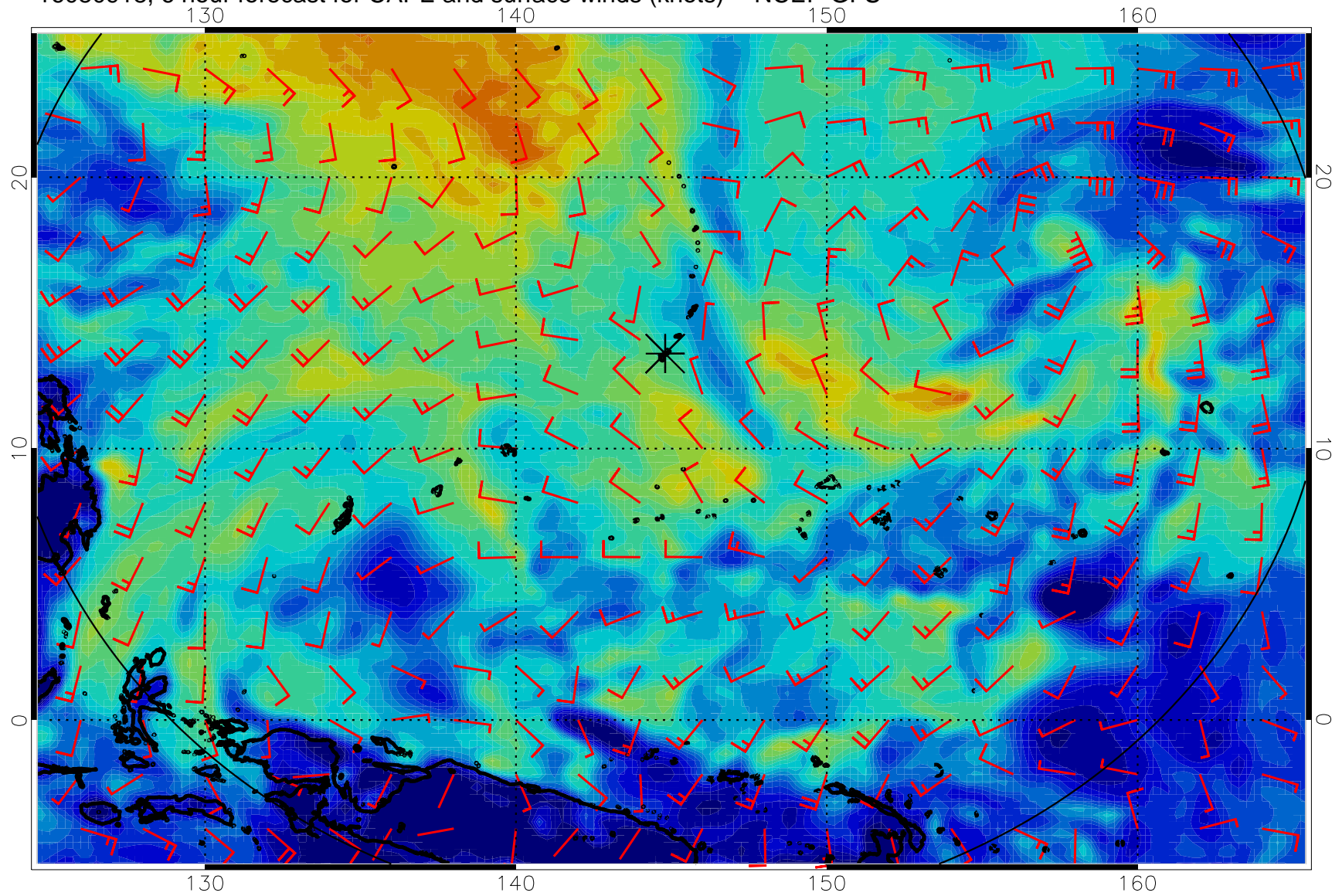
16080918, 6 hour forecast for CAPE and surface winds (knots) -- NCEP GFS
