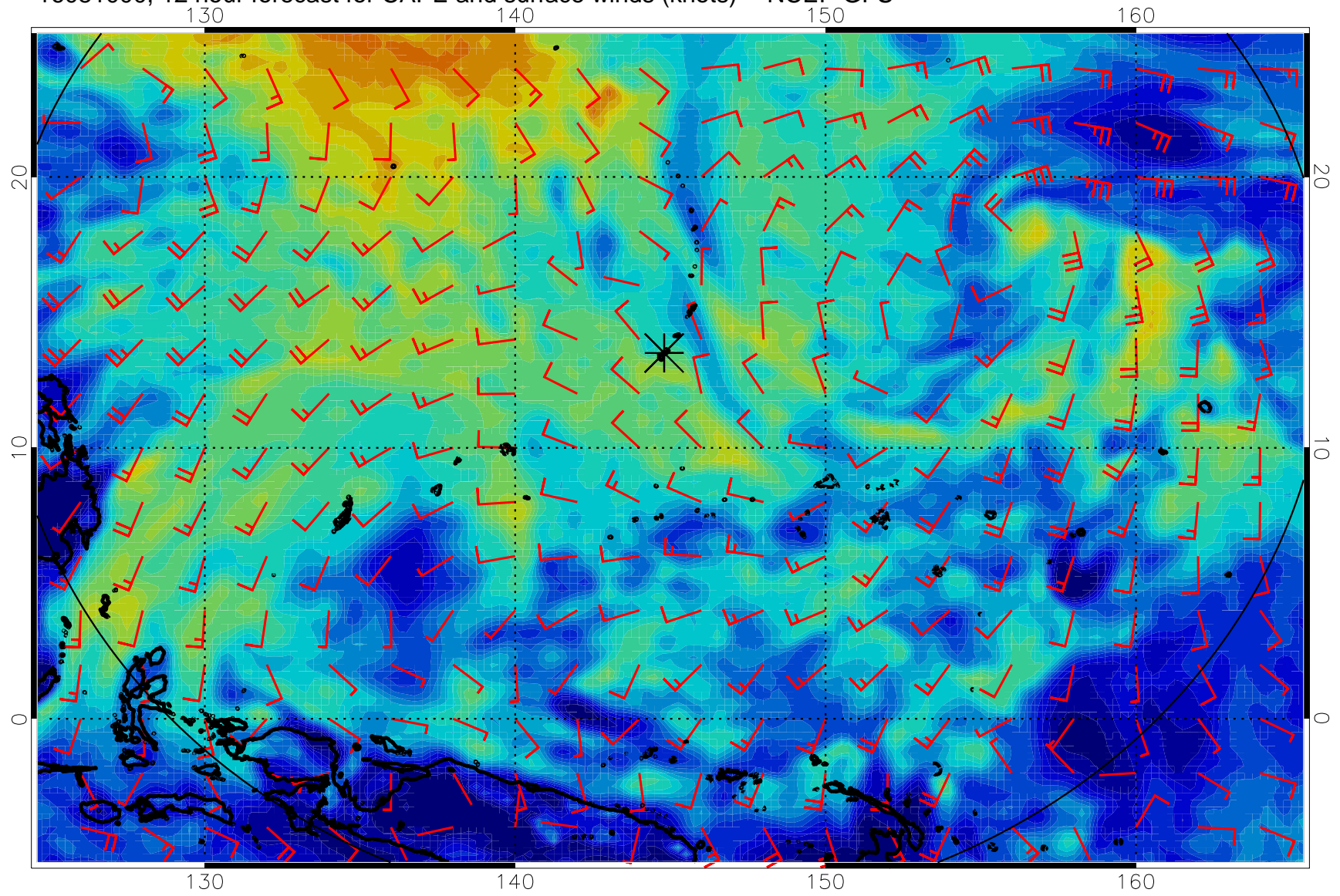
16081000, 12 hour forecast for CAPE and surface winds (knots) -- NCEP GFS
