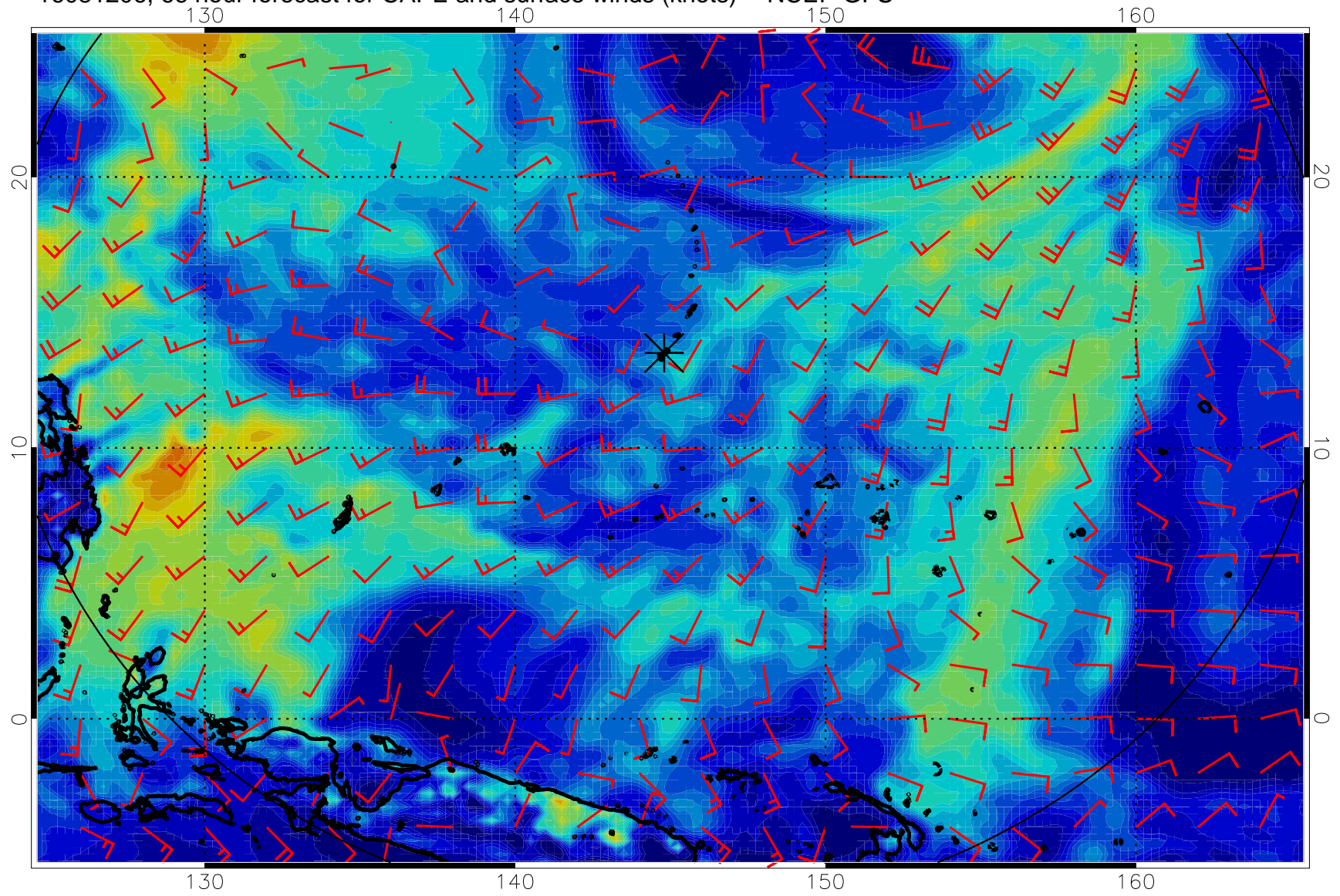
16081206, 66 hour forecast for CAPE and surface winds (knots) -- NCEP GFS
