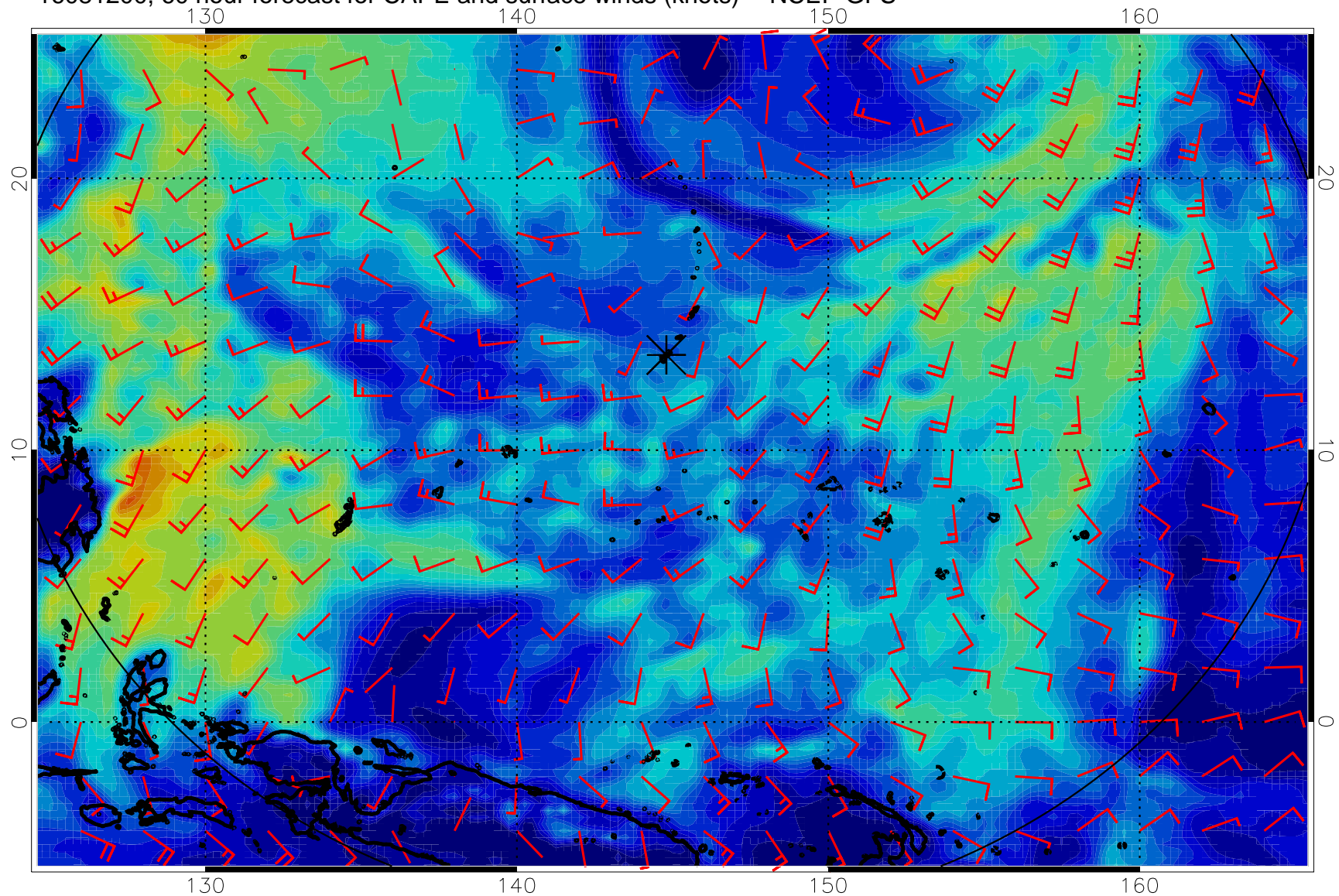
16081200, 60 hour forecast for CAPE and surface winds (knots) -- NCEP GFS
