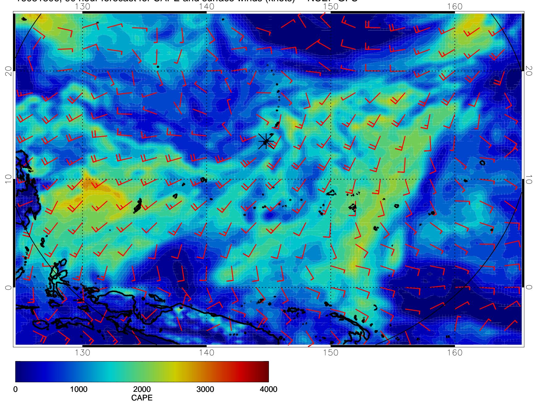
16081306, 90 hour forecast for CAPE and surface winds (knots) -- NCEP GFS
