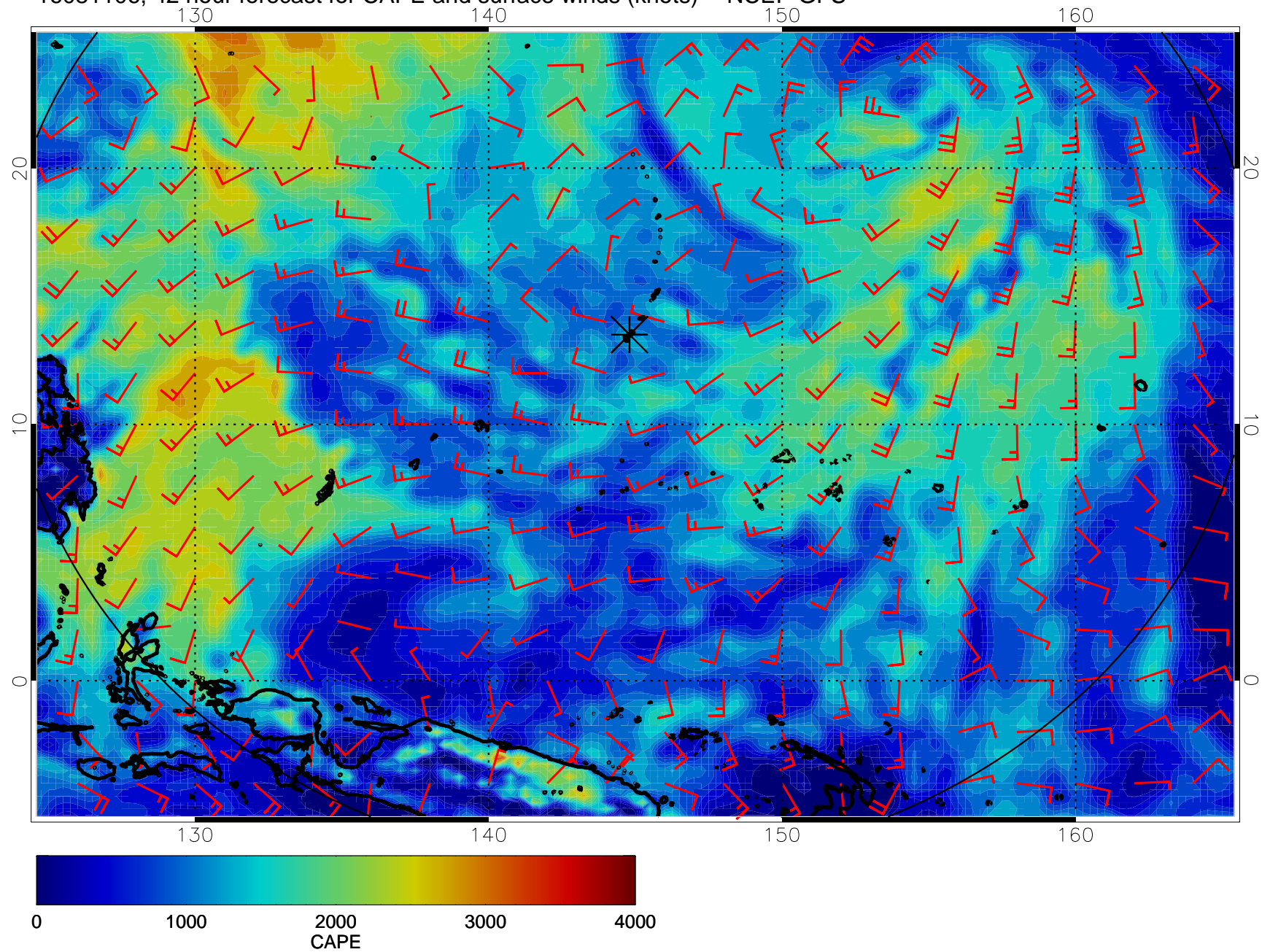
16081106, 42 hour forecast for CAPE and surface winds (knots) -- NCEP GFS
