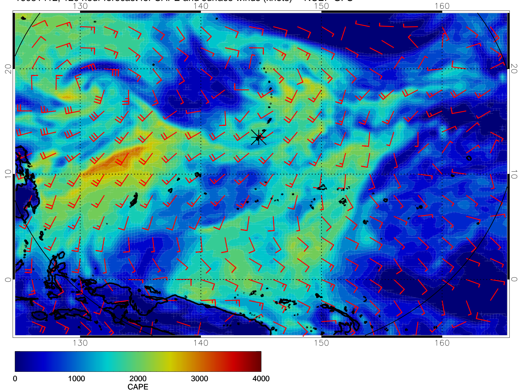
16081412, 120 hour forecast for CAPE and surface winds (knots) -- NCEP GFS
