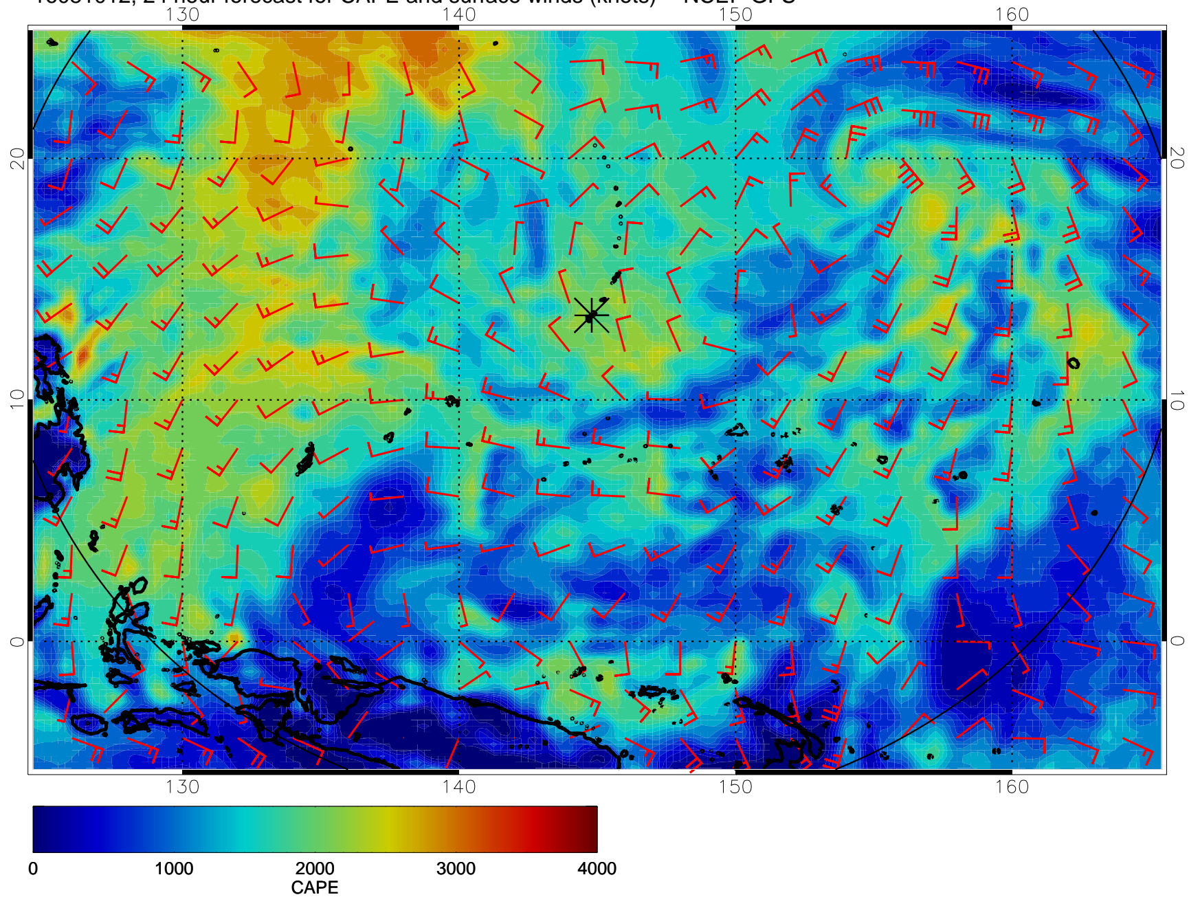
16081012, 24 hour forecast for CAPE and surface winds (knots) -- NCEP GFS
