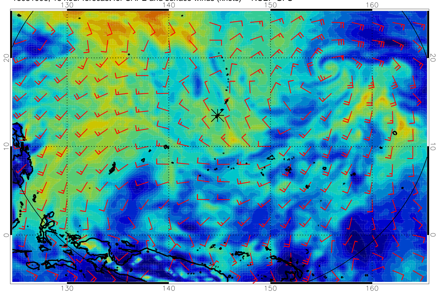
16081006, 18 hour forecast for CAPE and surface winds (knots) -- NCEP GFS
