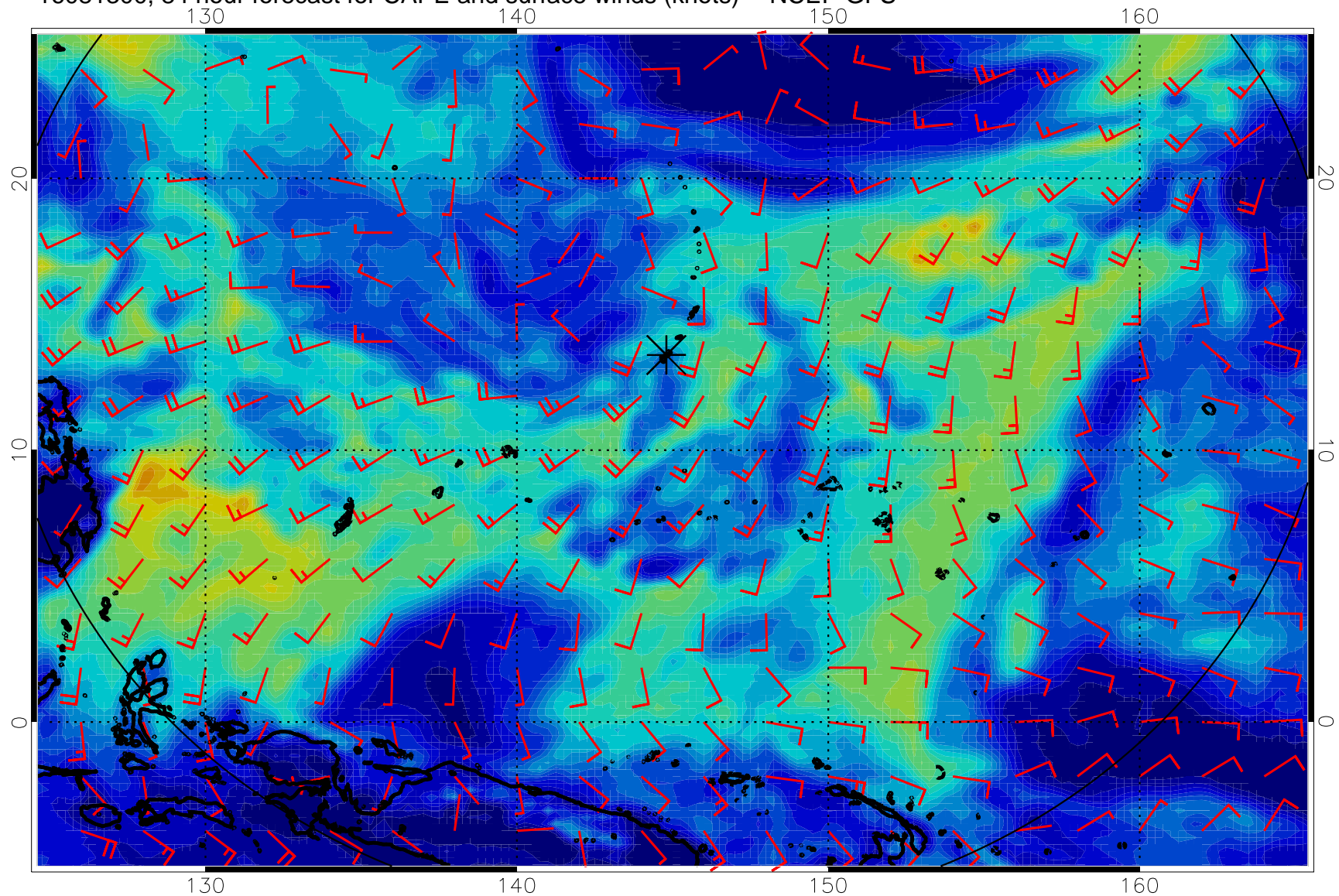
16081300, 84 hour forecast for CAPE and surface winds (knots) -- NCEP GFS
