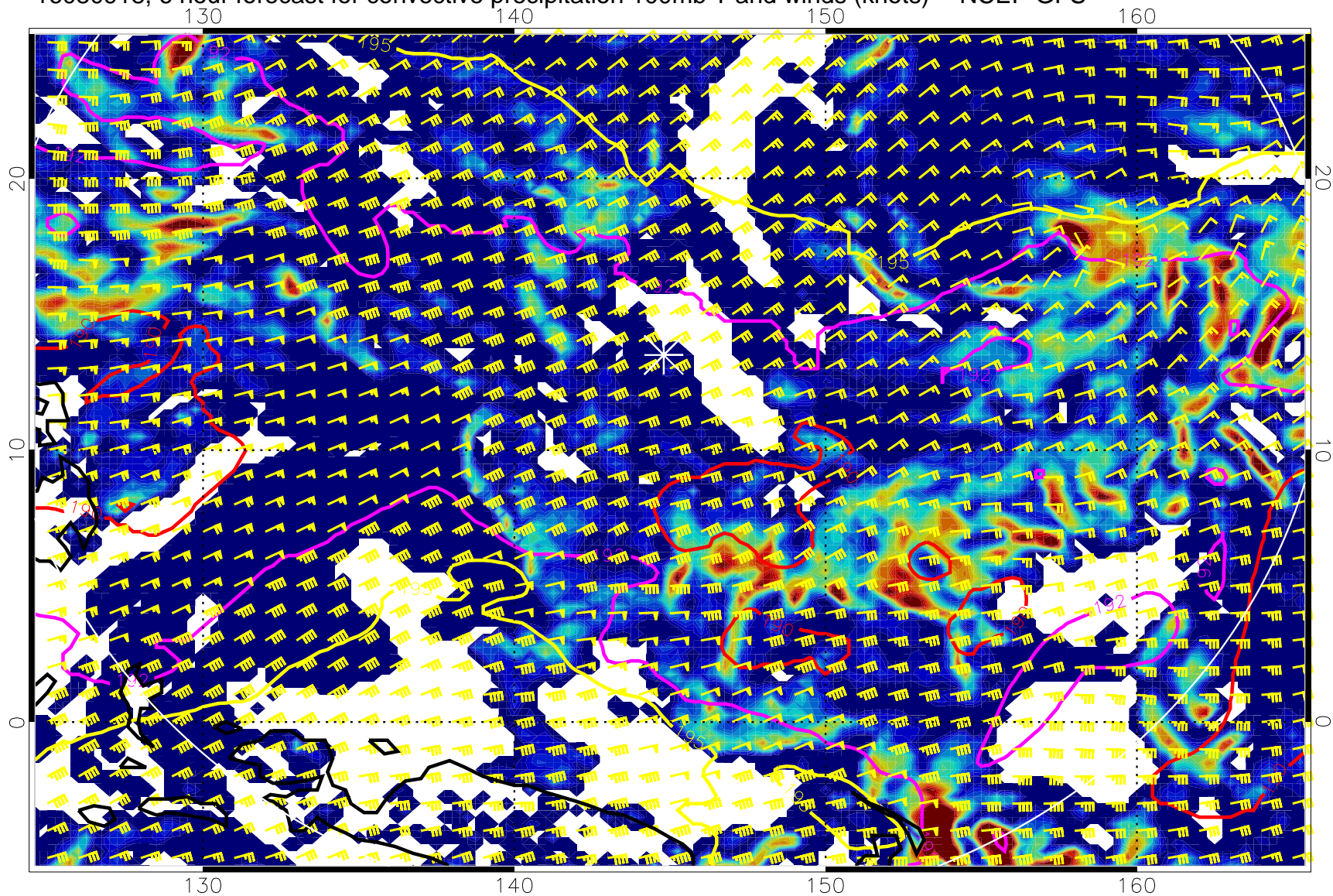
16080918, 6 hour forecast for convective precipitation 100mb T and winds (knots) -- NCEP GFS
