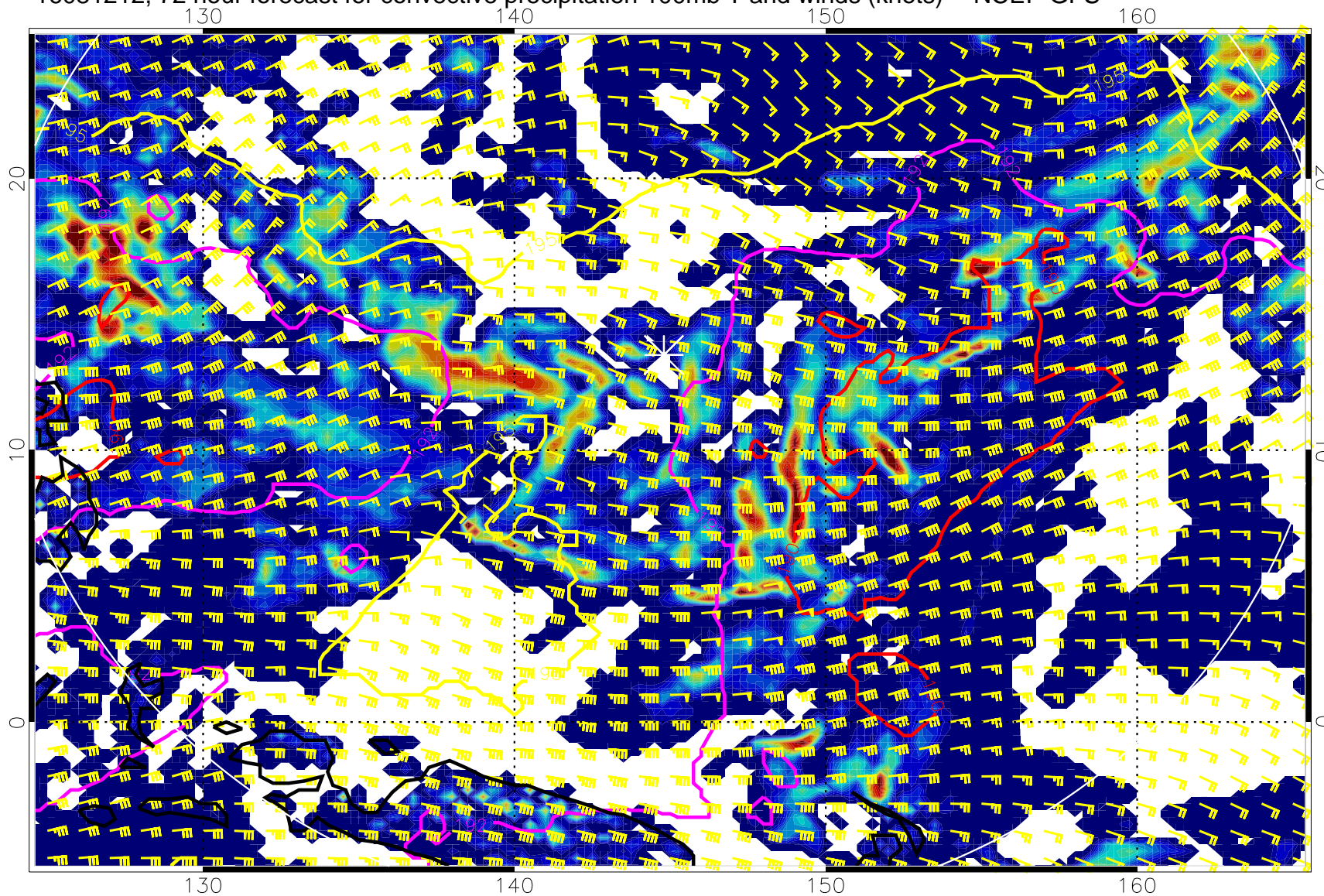
16081212, 72 hour forecast for convective precipitation 100mb T and winds (knots) -- NCEP GFS
