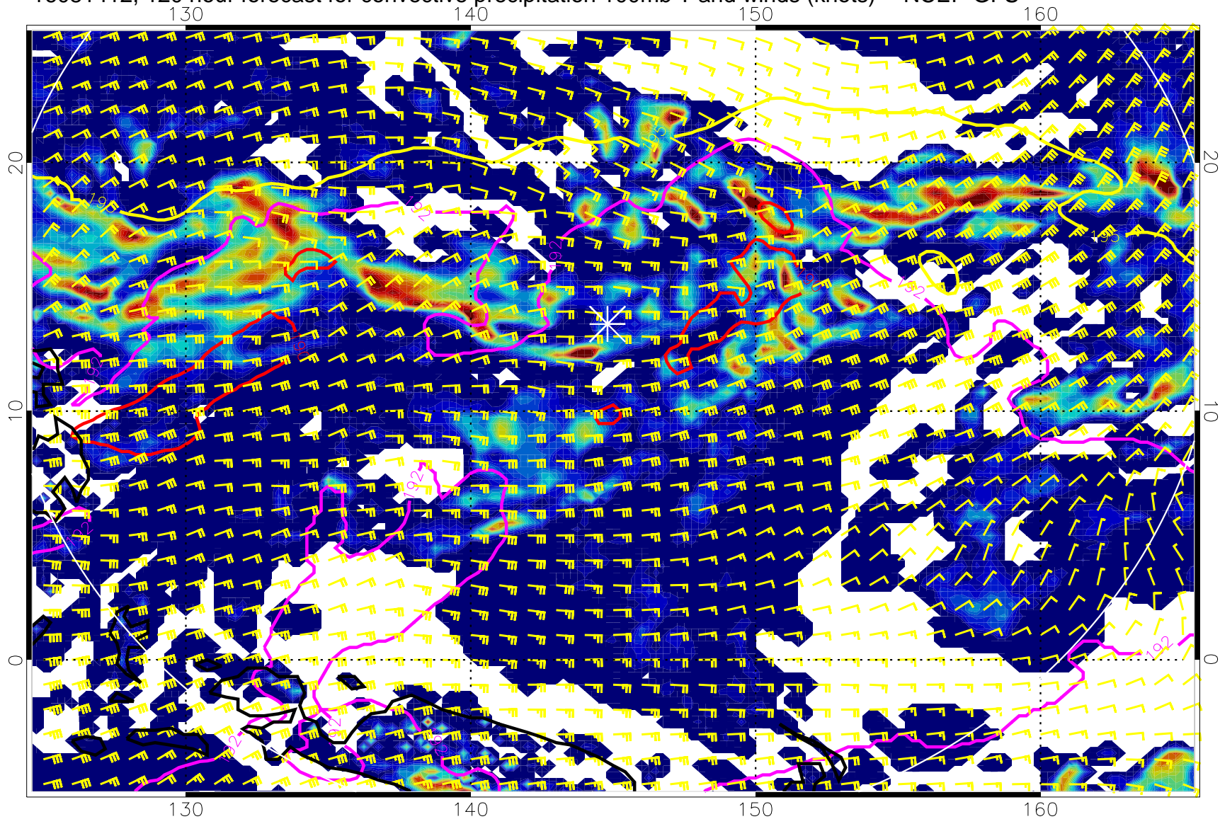
16081412, 120 hour forecast for convective precipitation 100mb T and winds (knots) -- NCEP GFS
