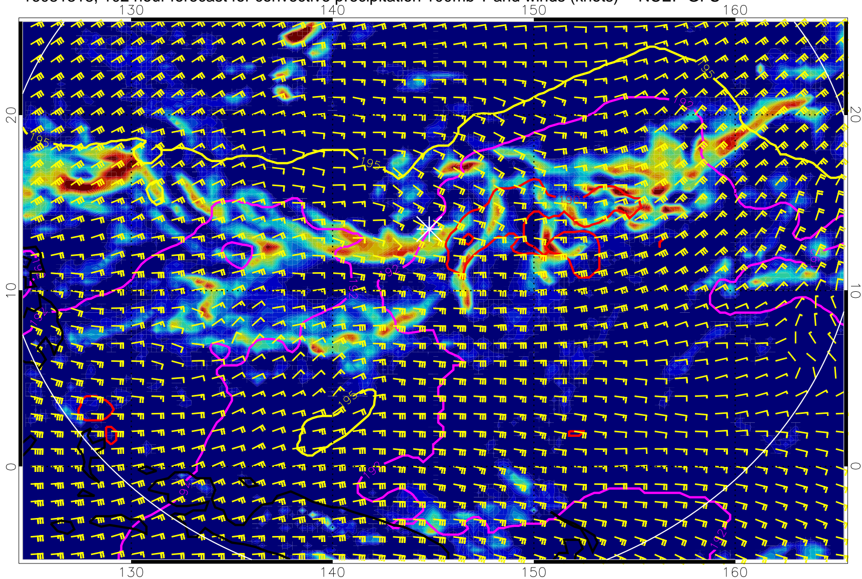
16081318, 102 hour forecast for convective precipitation 100mb T and winds (knots) -- NCEP GFS
