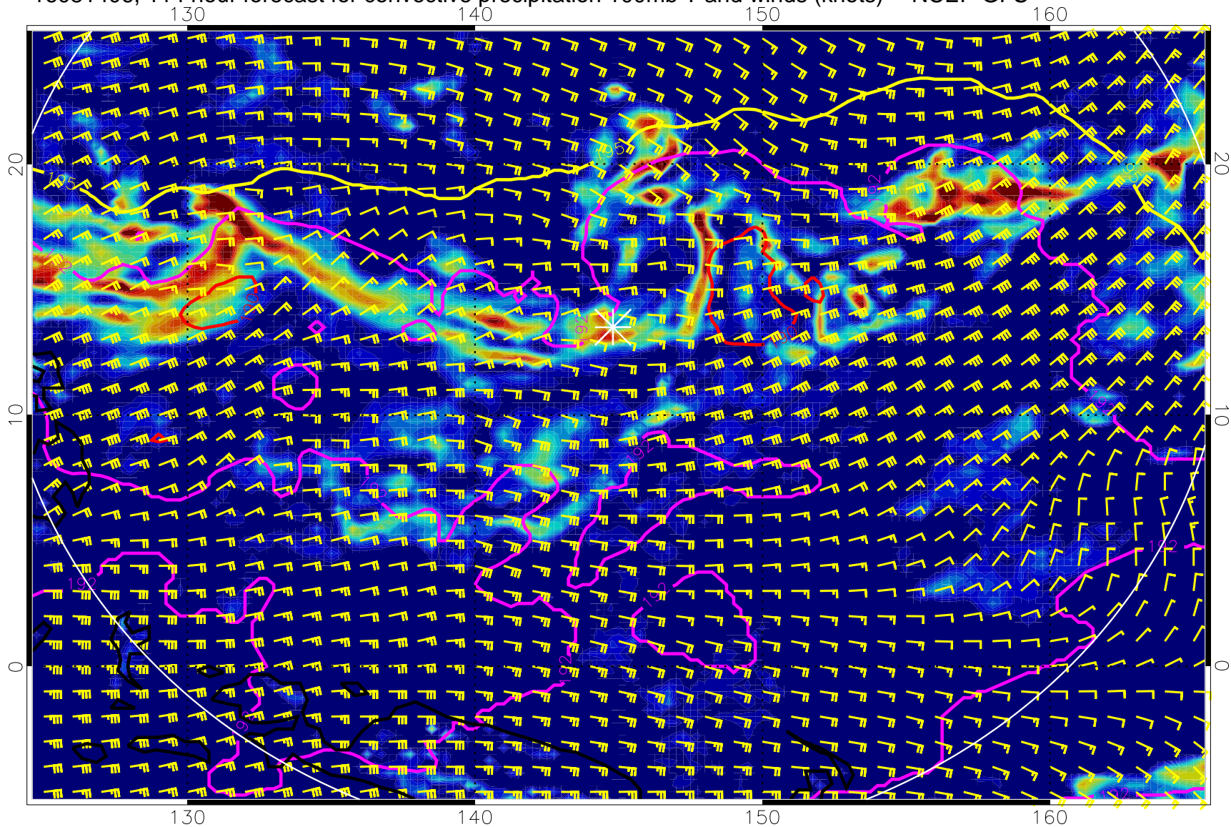
16081406, 114 hour forecast for convective precipitation 100mb T and winds (knots) -- NCEP GFS
