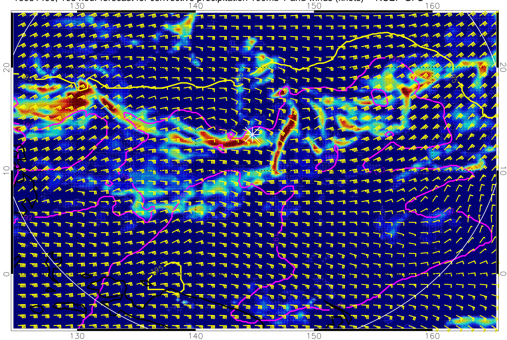
16081400, 108 hour forecast for convective precipitation 100mb T and winds (knots) -- NCEP GFS
