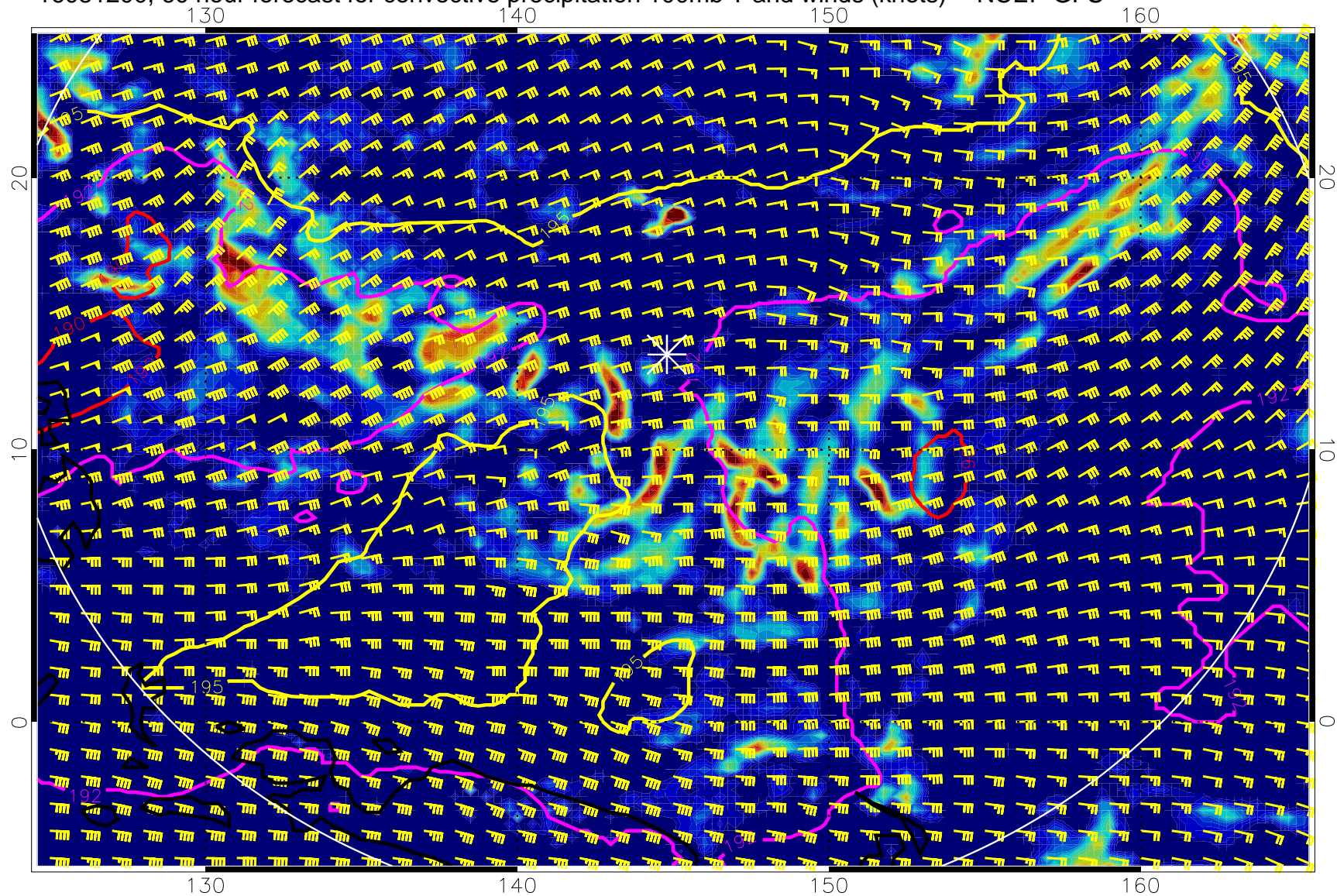
16081200, 60 hour forecast for convective precipitation 100mb T and winds (knots) -- NCEP GFS
