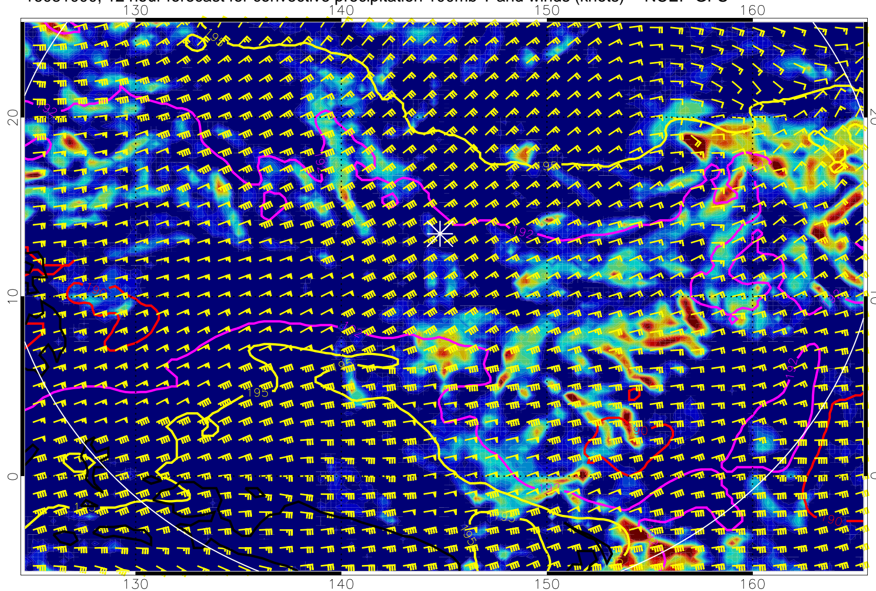
16081000, 12 hour forecast for convective precipitation 100mb T and winds (knots) -- NCEP GFS
