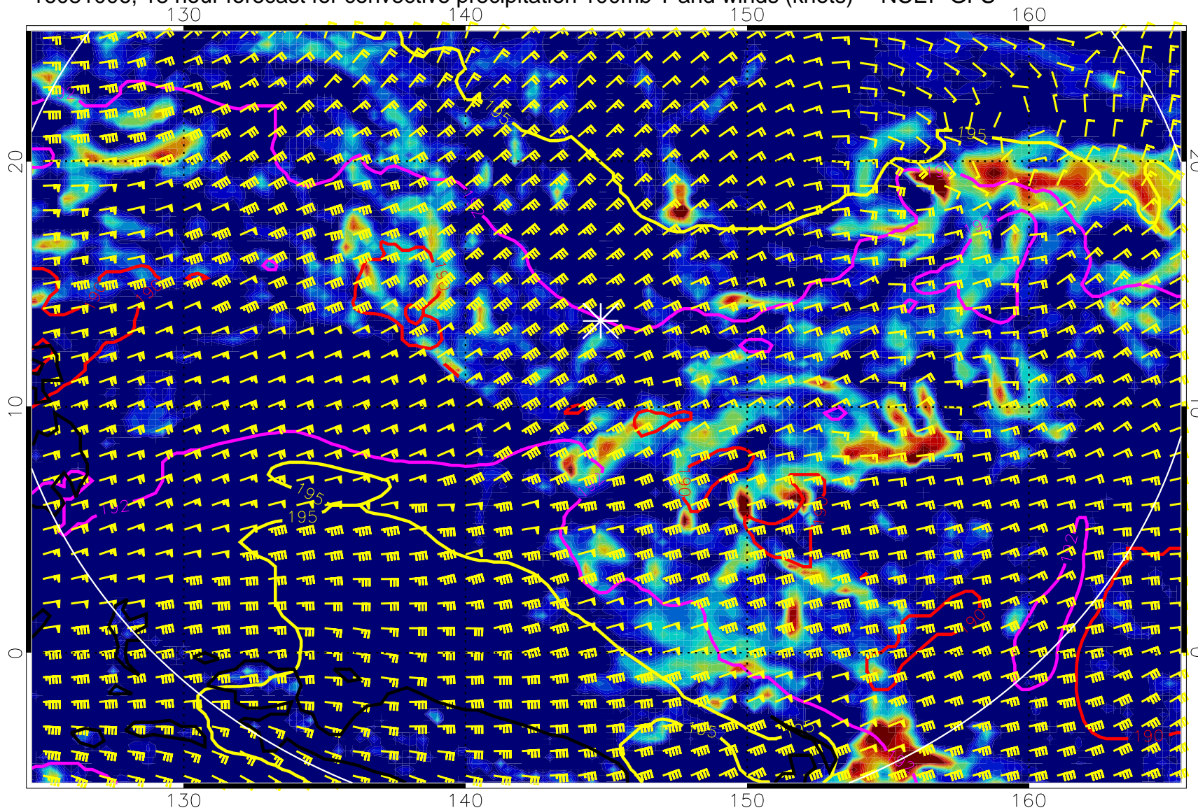
16081006, 18 hour forecast for convective precipitation 100mb T and winds (knots) -- NCEP GFS
