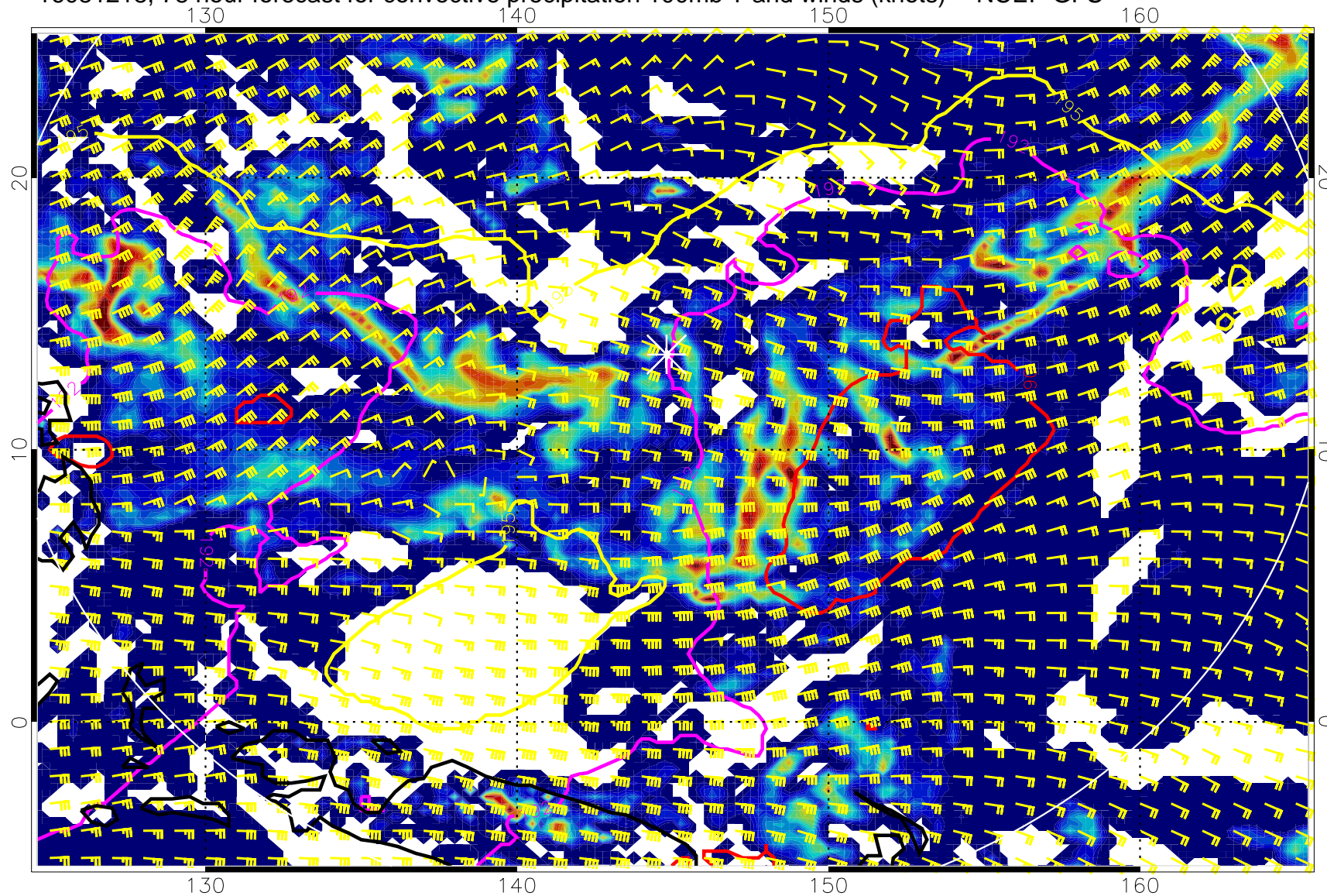
16081218, 78 hour forecast for convective precipitation 100mb T and winds (knots) -- NCEP GFS
