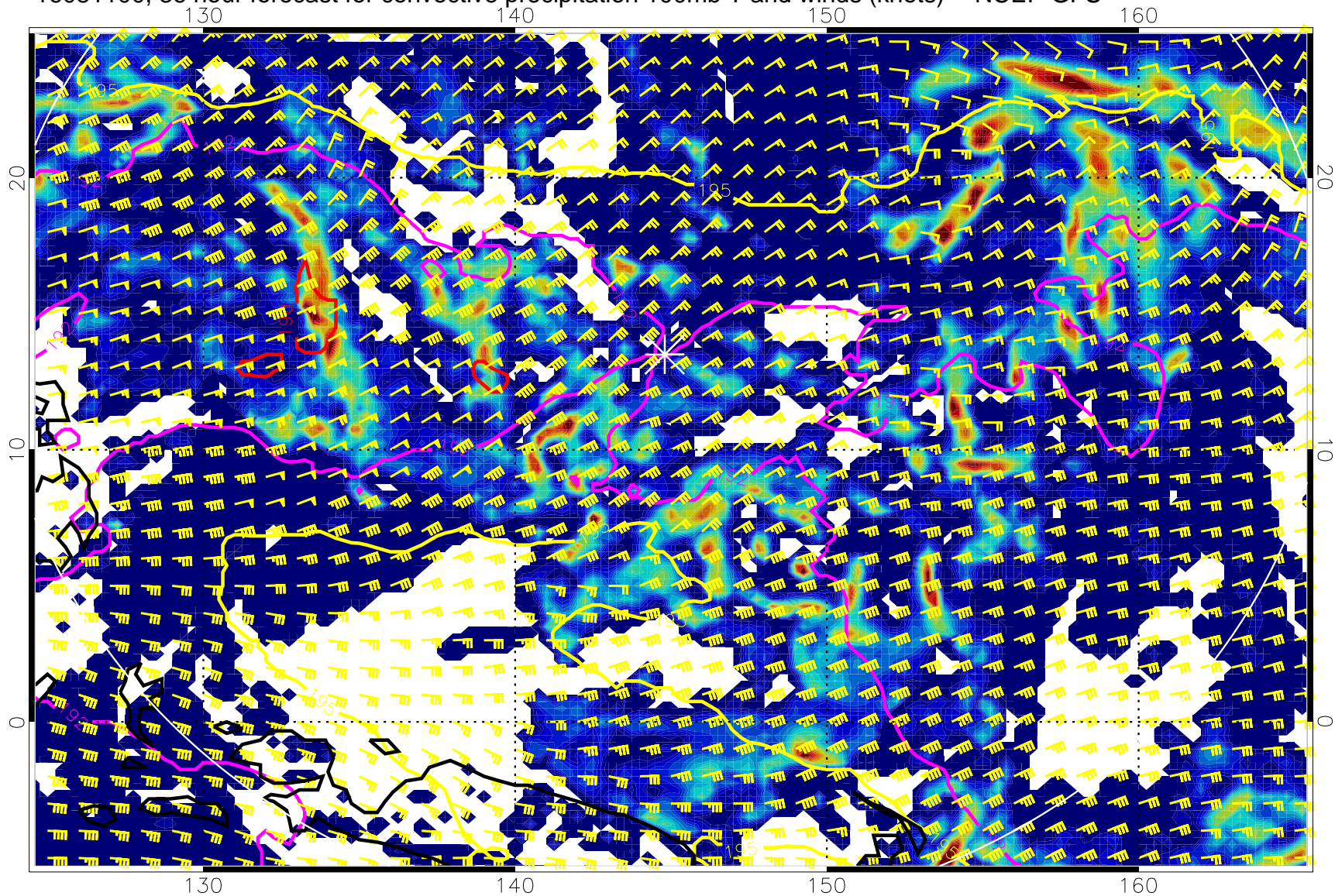
16081100, 36 hour forecast for convective precipitation 100mb T and winds (knots) -- NCEP GFS
