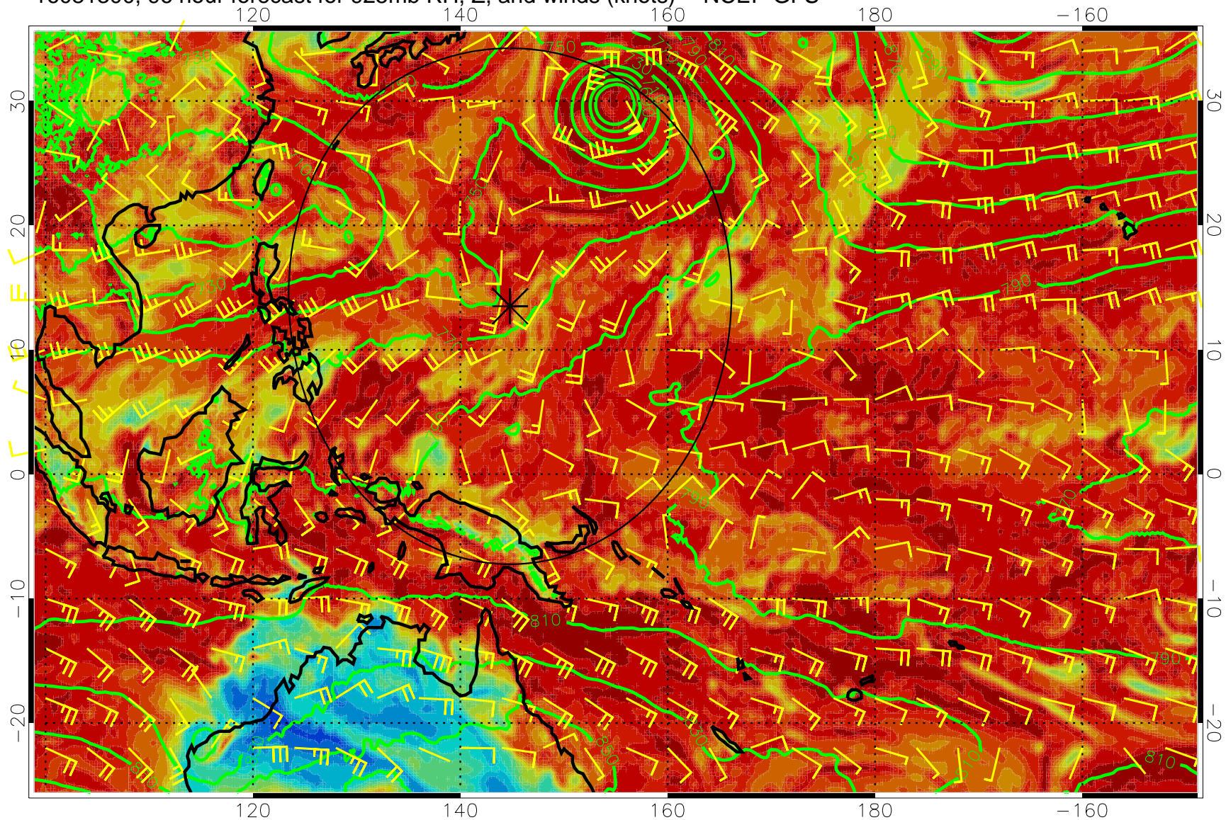
16081300, 96 hour forecast for 925mb RH, Z, and winds (knots) -- NCEP GFS
