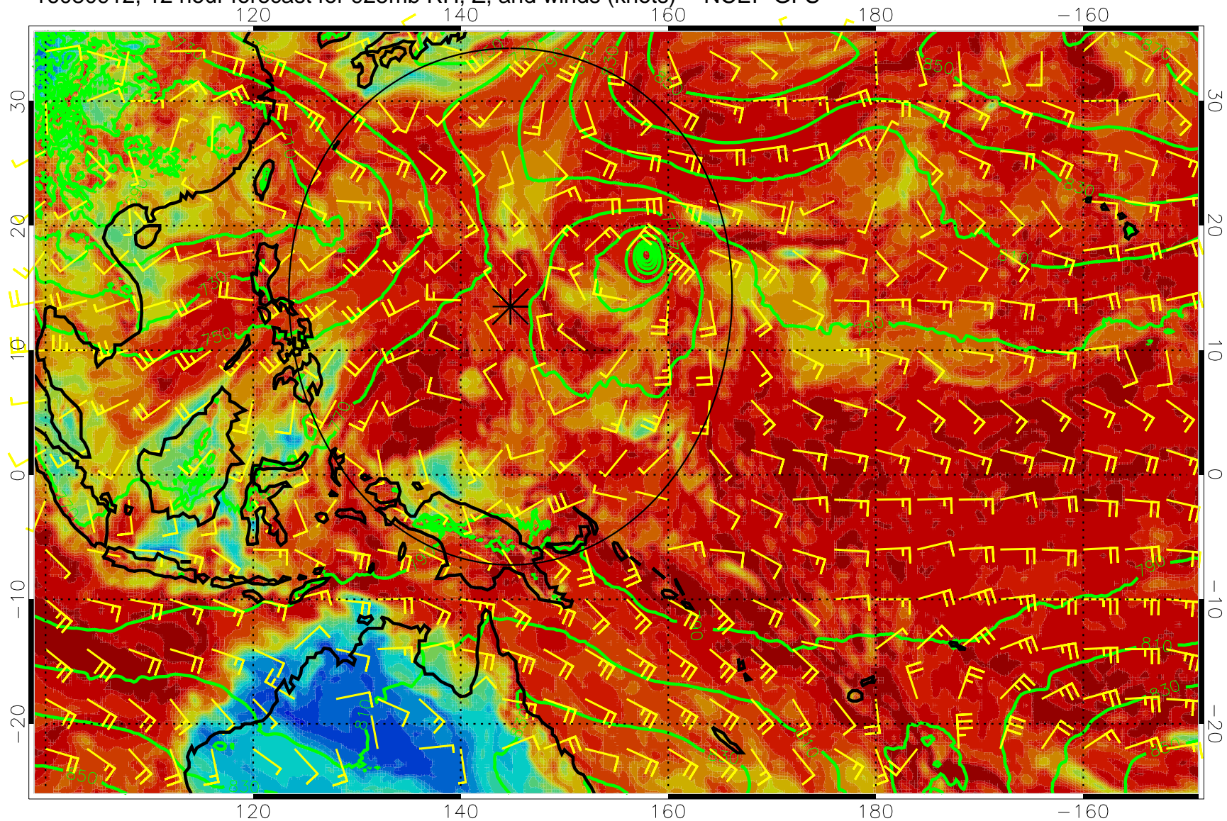
16080912, 12 hour forecast for 925mb RH, Z, and winds (knots) -- NCEP GFS
