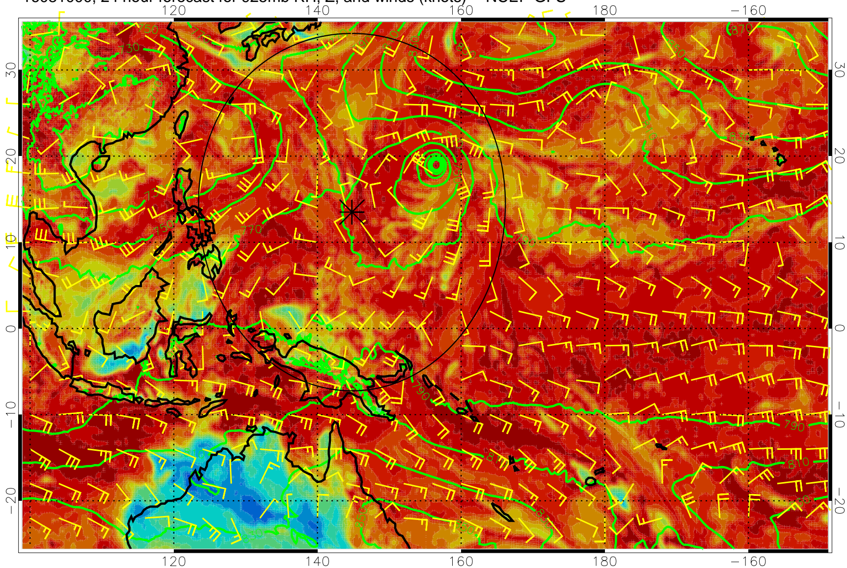
16081000, 24 hour forecast for 925mb RH, Z, and winds (knots) -- NCEP GFS
