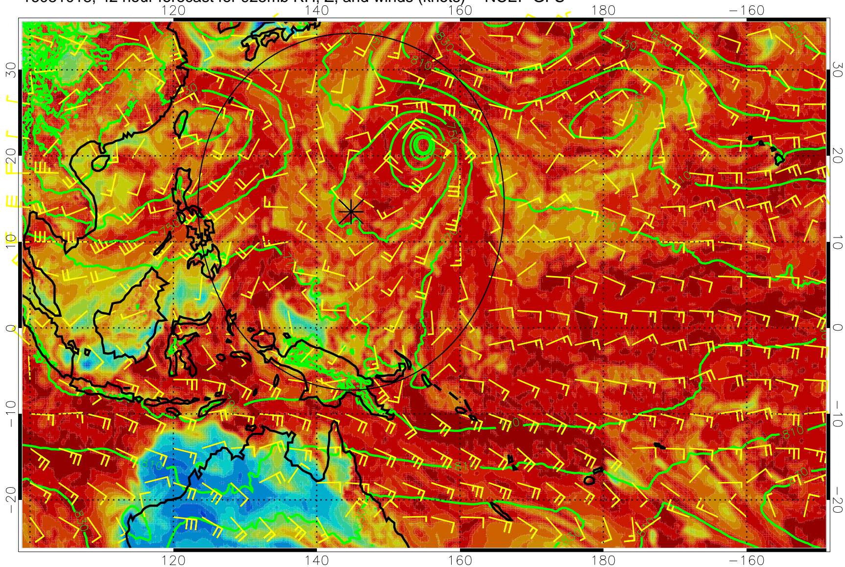
16081018, 42 hour forecast for 925mb RH, Z, and winds (knots) -- NCEP GFS
