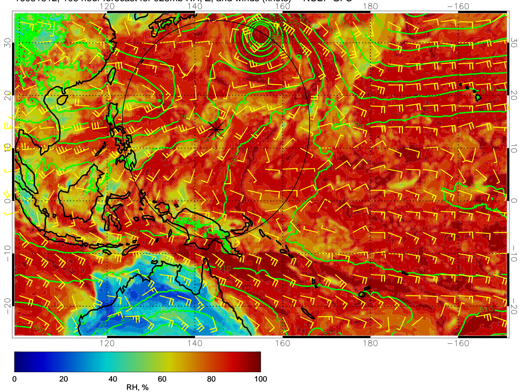
16081312, 108 hour forecast for 925mb RH, Z, and winds (knots) -- NCEP GFS
