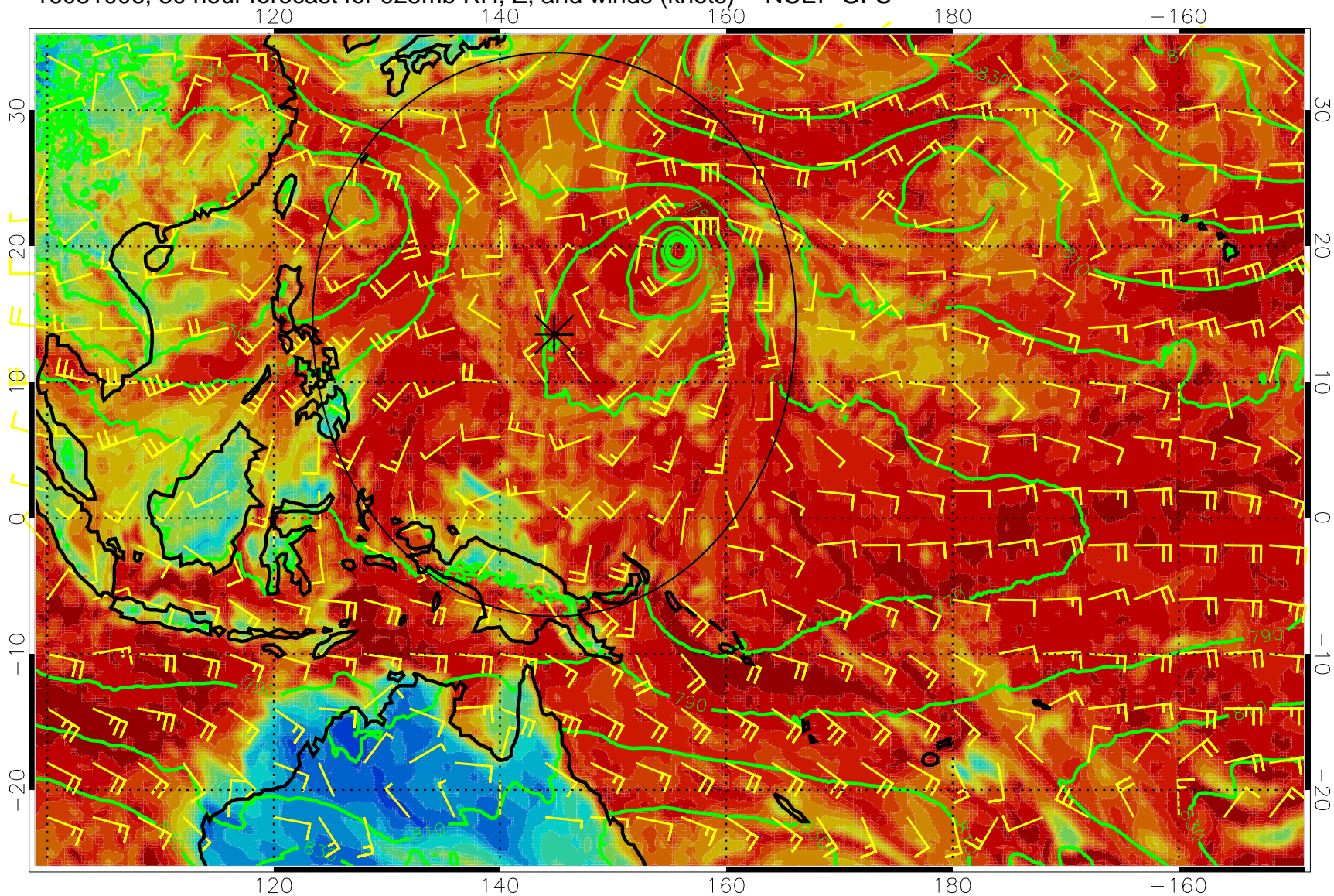
16081006, 30 hour forecast for 925mb RH, Z, and winds (knots) -- NCEP GFS
