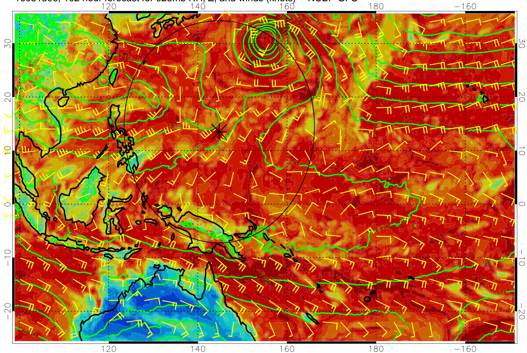
16081306, 102 hour forecast for 925mb RH, Z, and winds (knots) -- NCEP GFS
