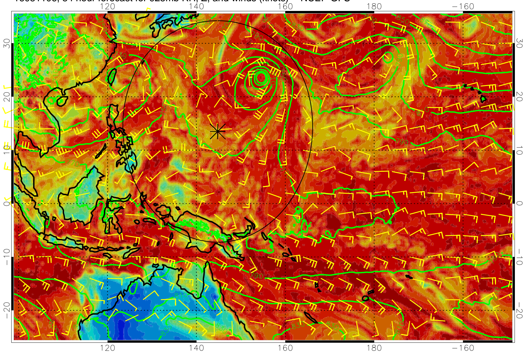
16081106, 54 hour forecast for 925mb RH, Z, and winds (knots) -- NCEP GFS
