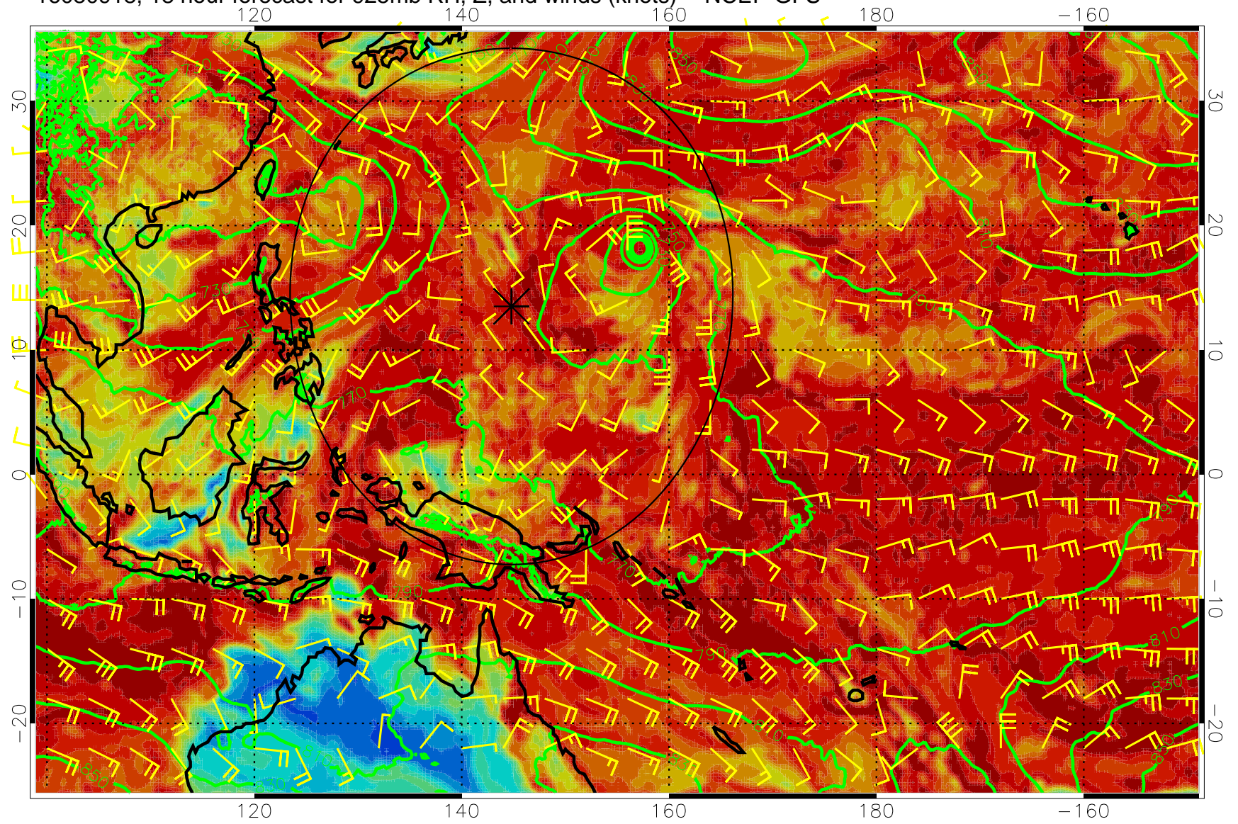
16080918, 18 hour forecast for 925mb RH, Z, and winds (knots) -- NCEP GFS
