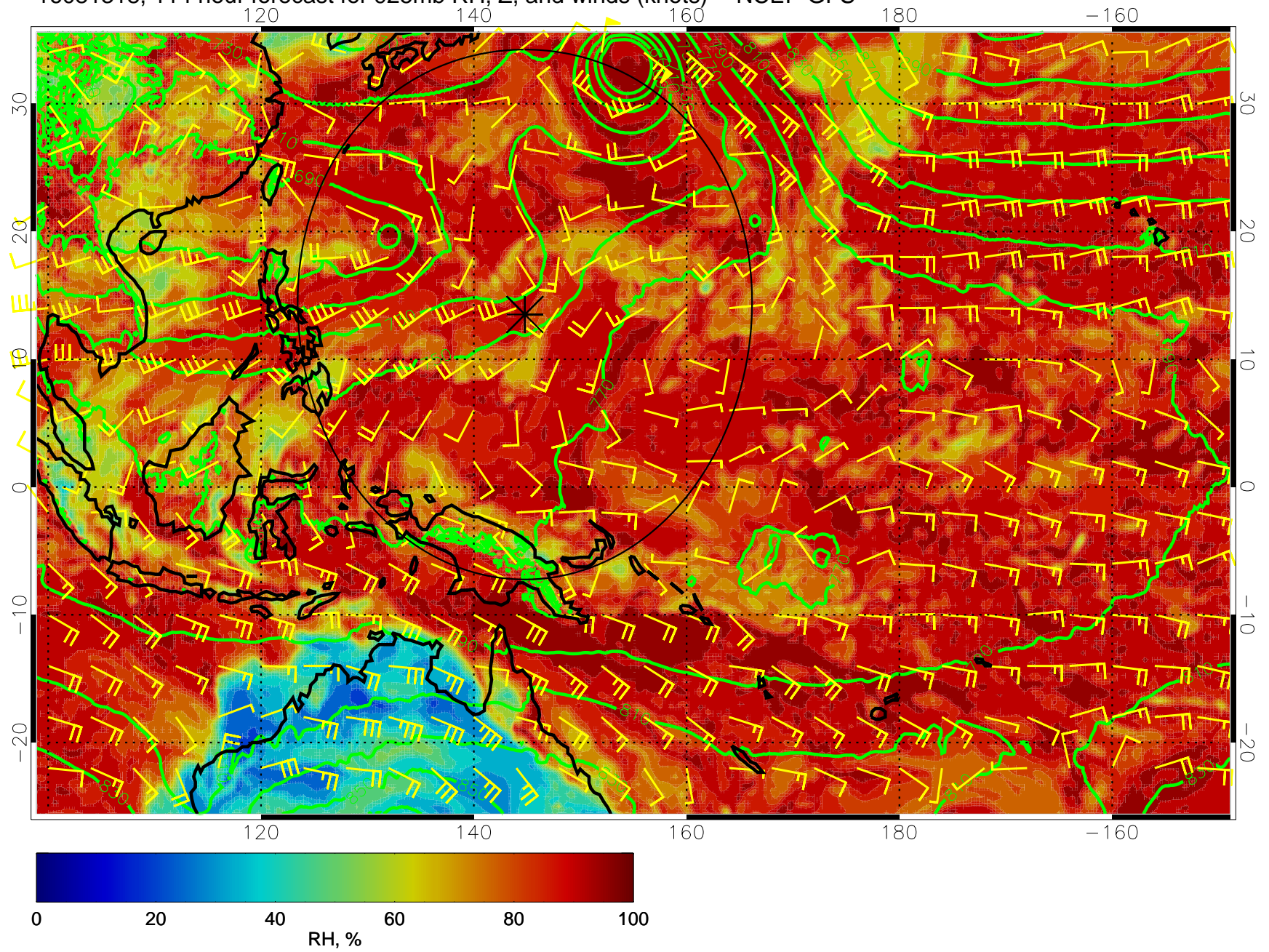
16081318, 114 hour forecast for 925mb RH, Z, and winds (knots) -- NCEP GFS
