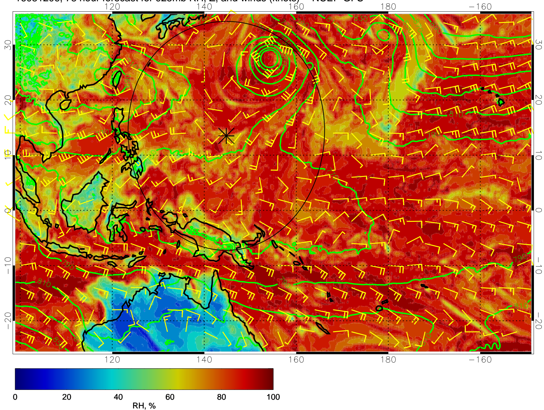
16081206, 78 hour forecast for 925mb RH, Z, and winds (knots) -- NCEP GFS
