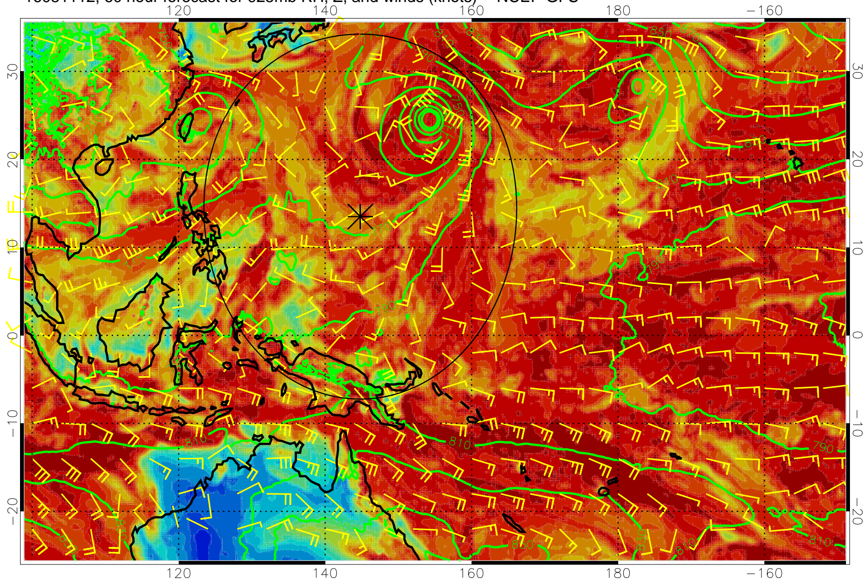
16081112, 60 hour forecast for 925mb RH, Z, and winds (knots) -- NCEP GFS
