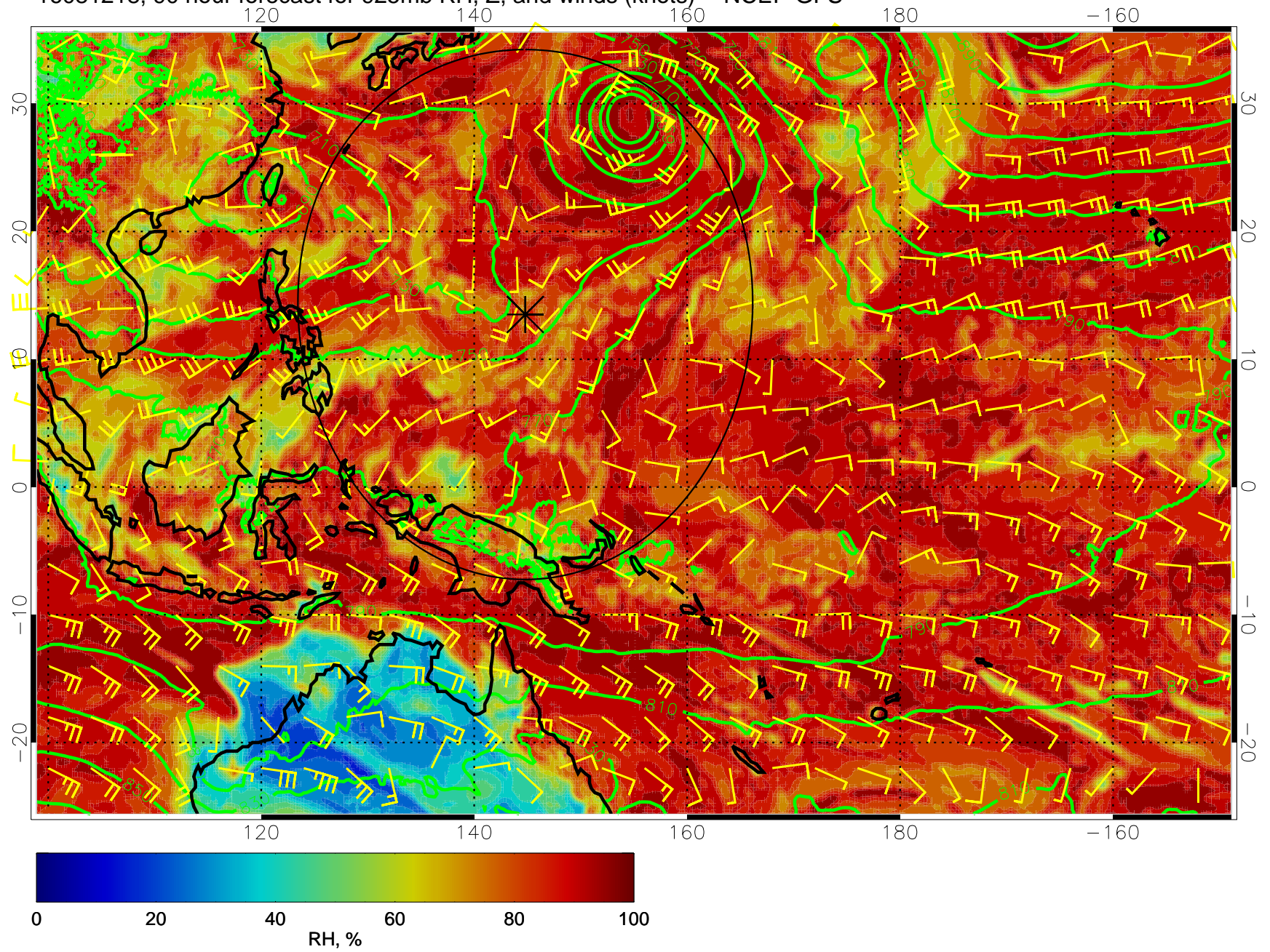
16081218, 90 hour forecast for 925mb RH, Z, and winds (knots) -- NCEP GFS
