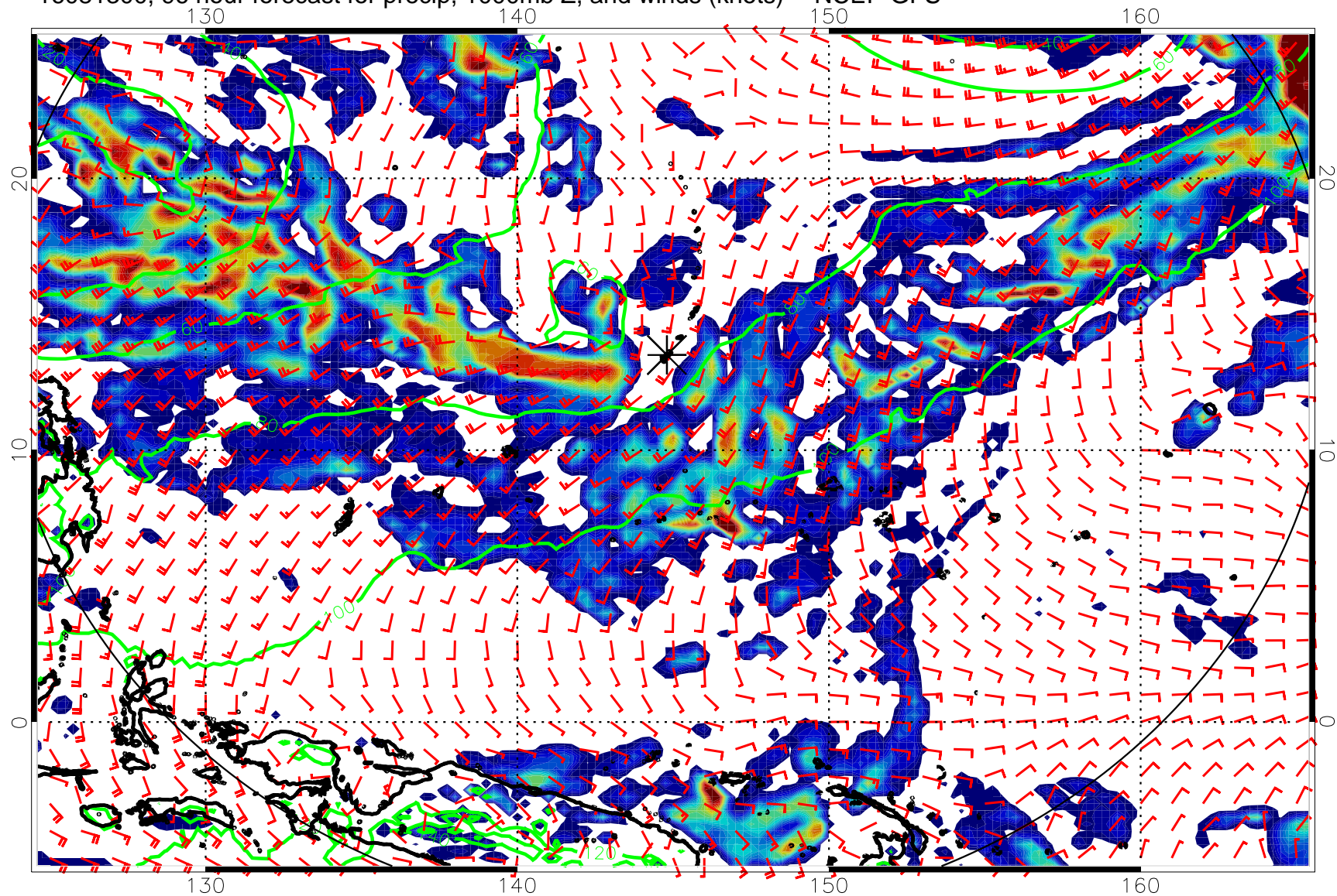
16081300, 96 hour forecast for precip, 1000mb Z, and winds (knots) -- NCEP GFS
