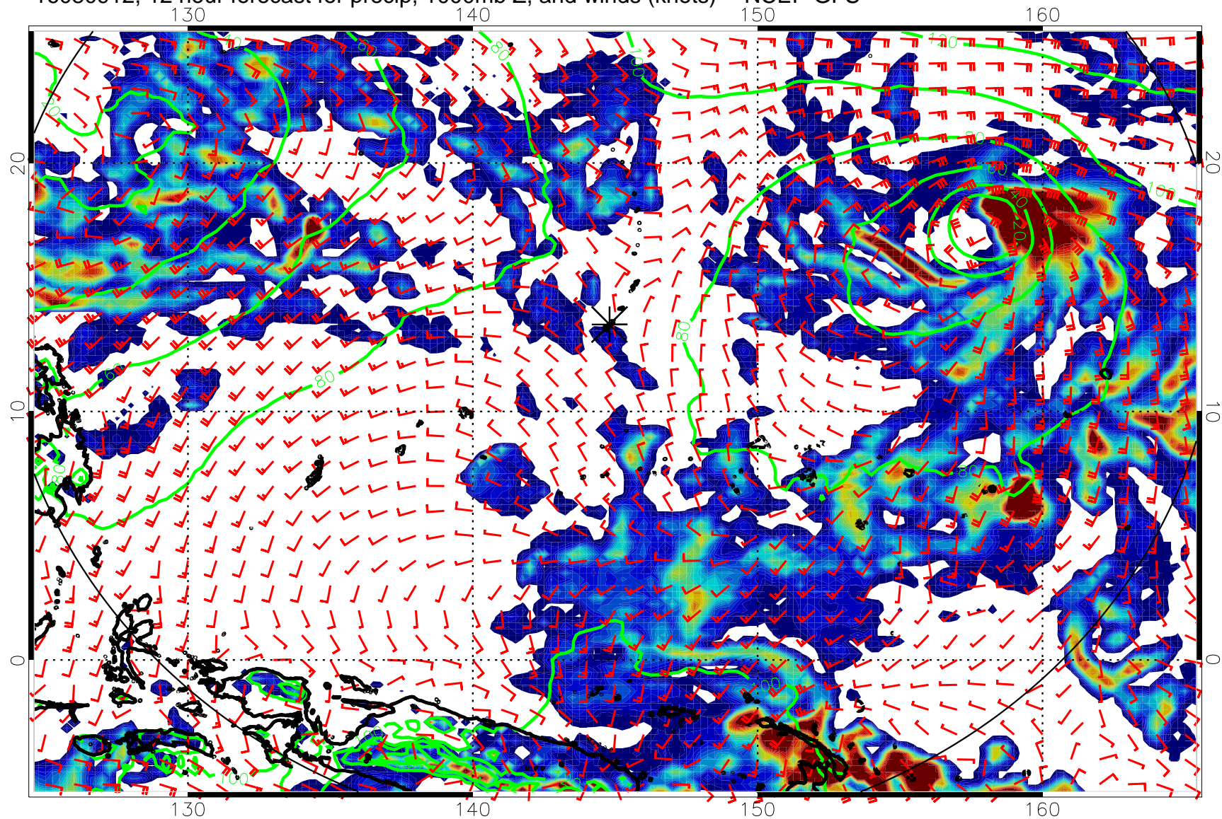
16080912, 12 hour forecast for precip, 1000mb Z, and winds (knots) -- NCEP GFS
