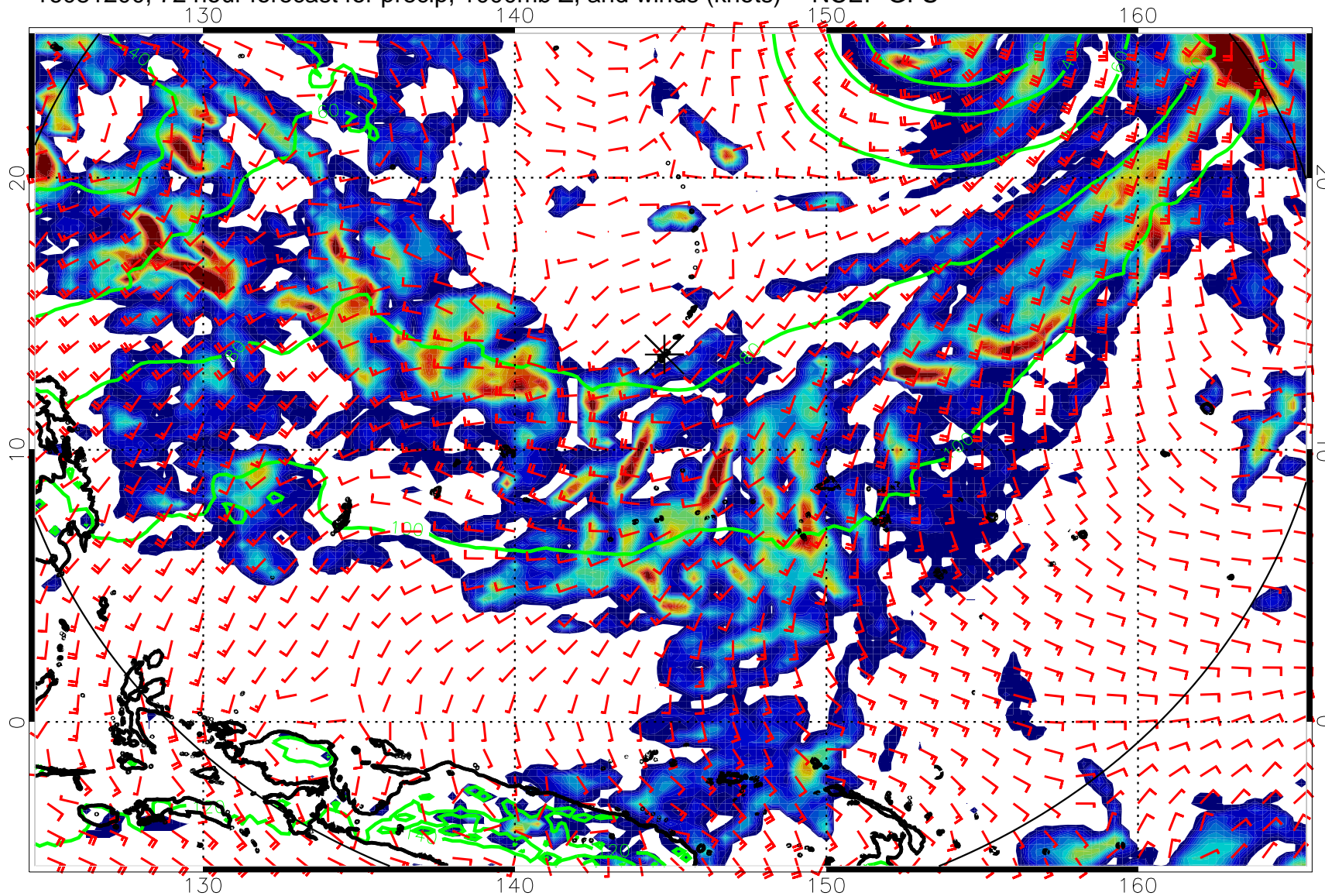
16081200, 72 hour forecast for precip, 1000mb Z, and winds (knots) -- NCEP GFS
