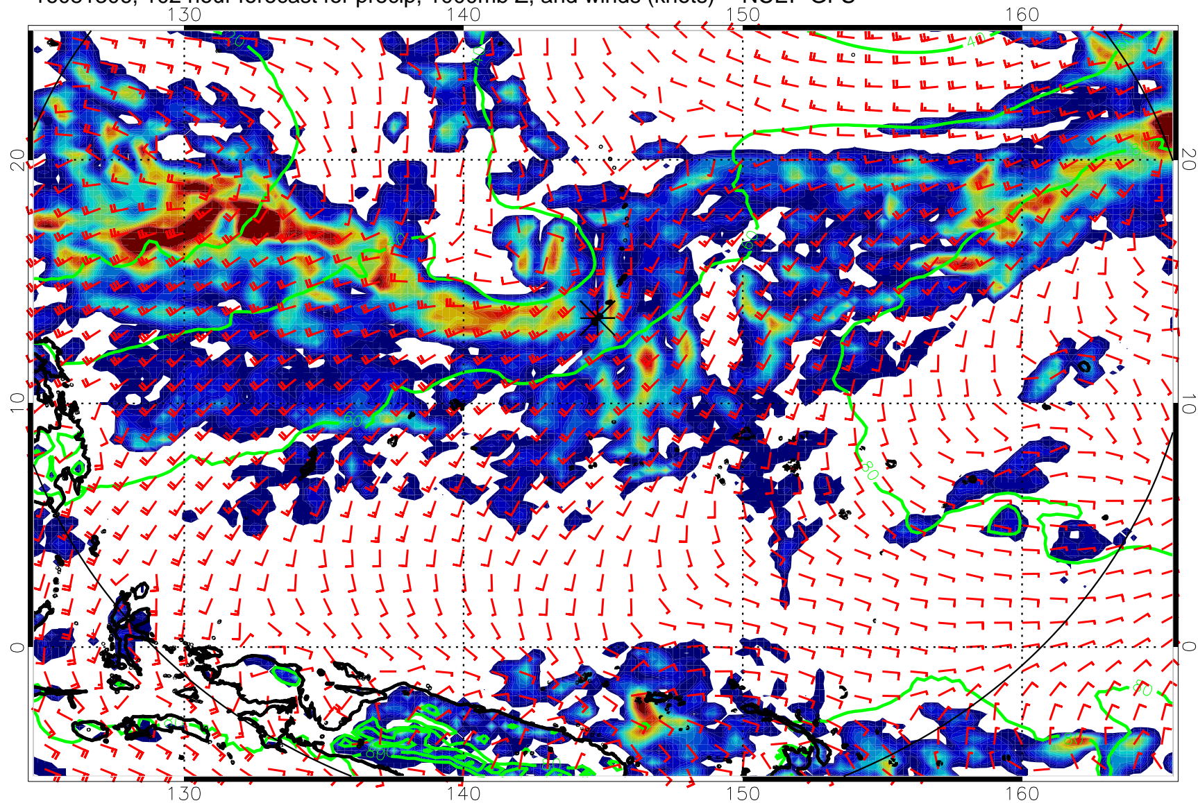
16081306, 102 hour forecast for precip, 1000mb Z, and winds (knots) -- NCEP GFS
