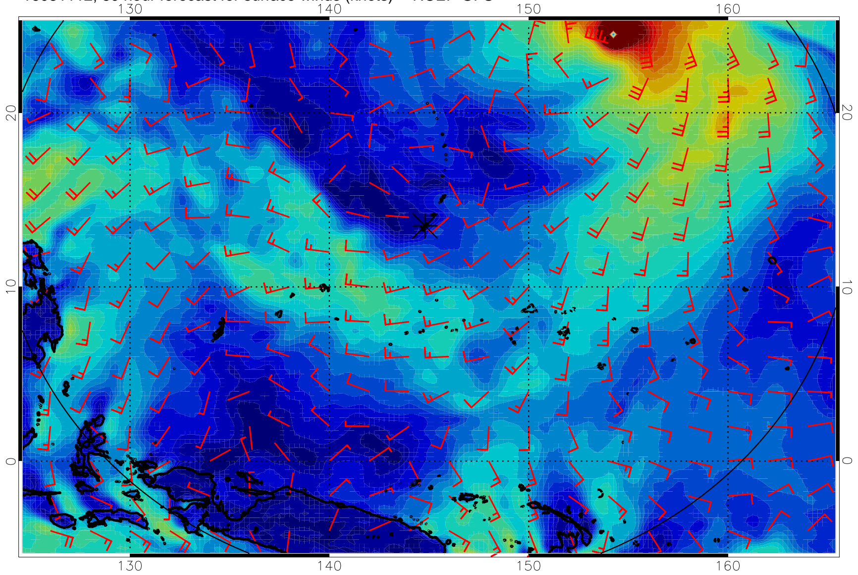
16081112, 60 hour forecast for surface winds (knots) -- NCEP GFS
