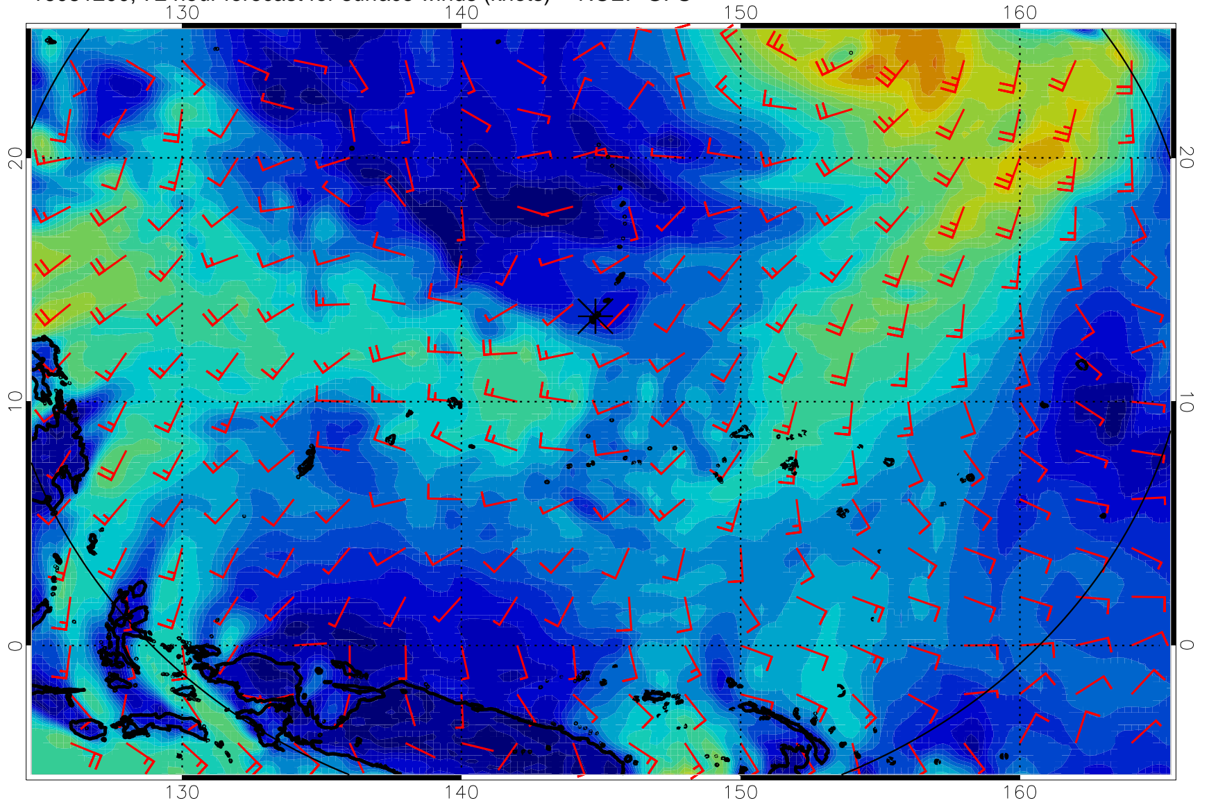
16081200, 72 hour forecast for surface winds (knots) -- NCEP GFS
