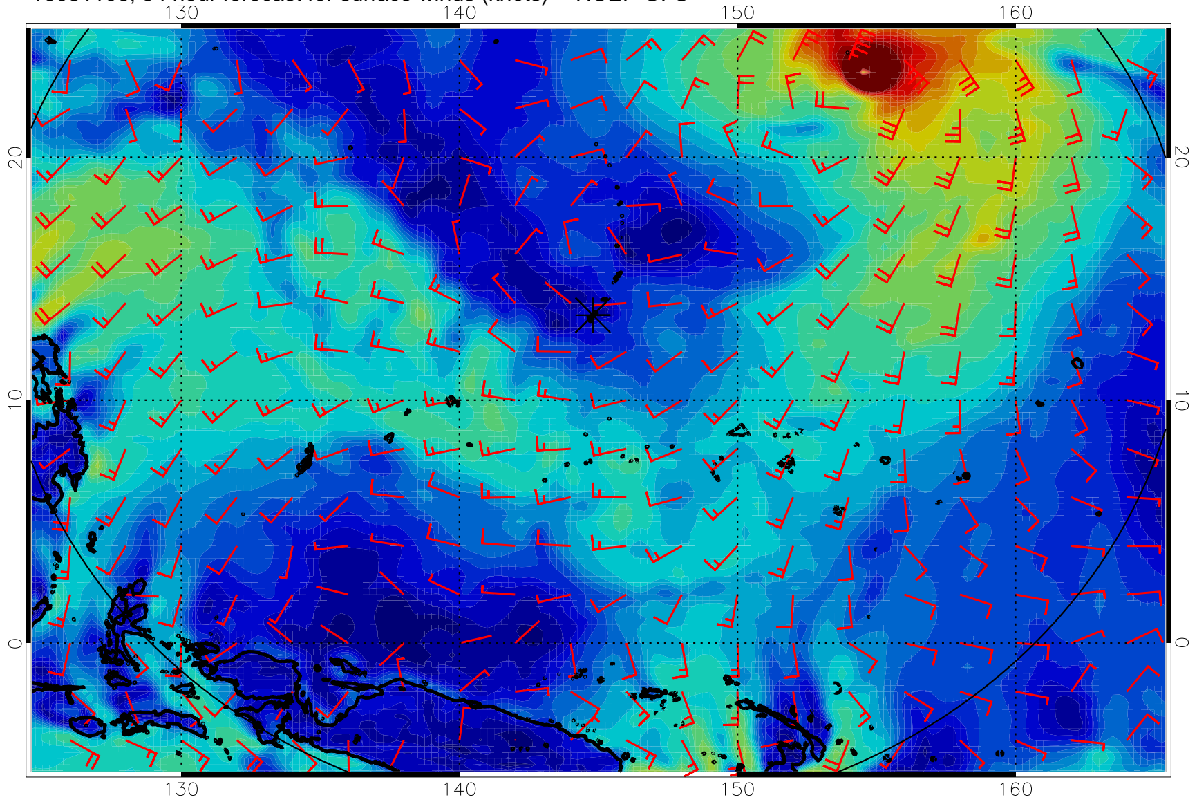
16081106, 54 hour forecast for surface winds (knots) -- NCEP GFS
