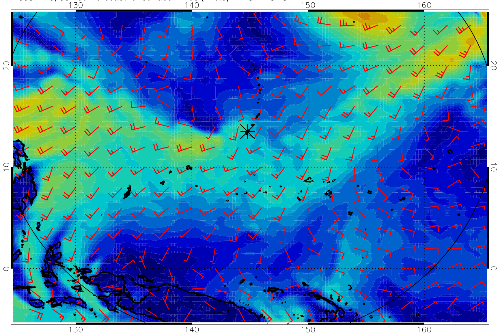
16081218, 90 hour forecast for surface winds (knots) -- NCEP GFS
