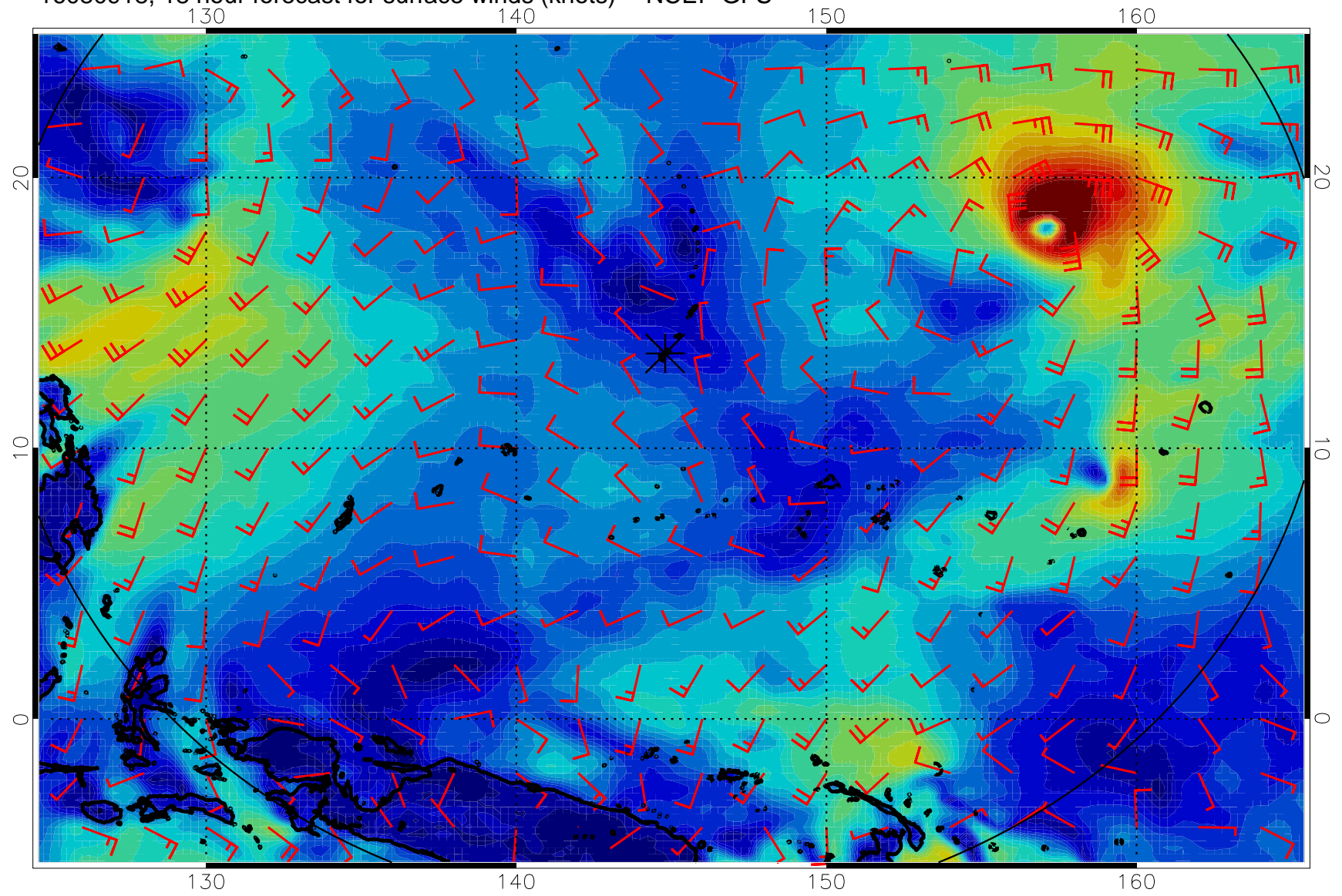
16080918, 18 hour forecast for surface winds (knots) -- NCEP GFS
