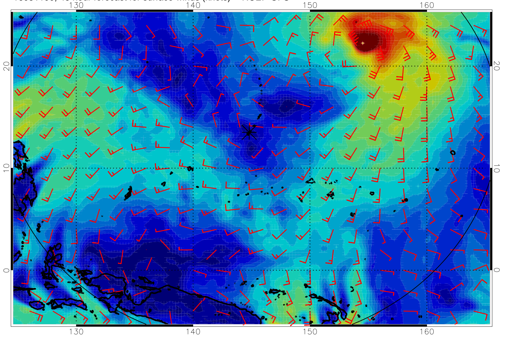
16081100, 48 hour forecast for surface winds (knots) -- NCEP GFS
