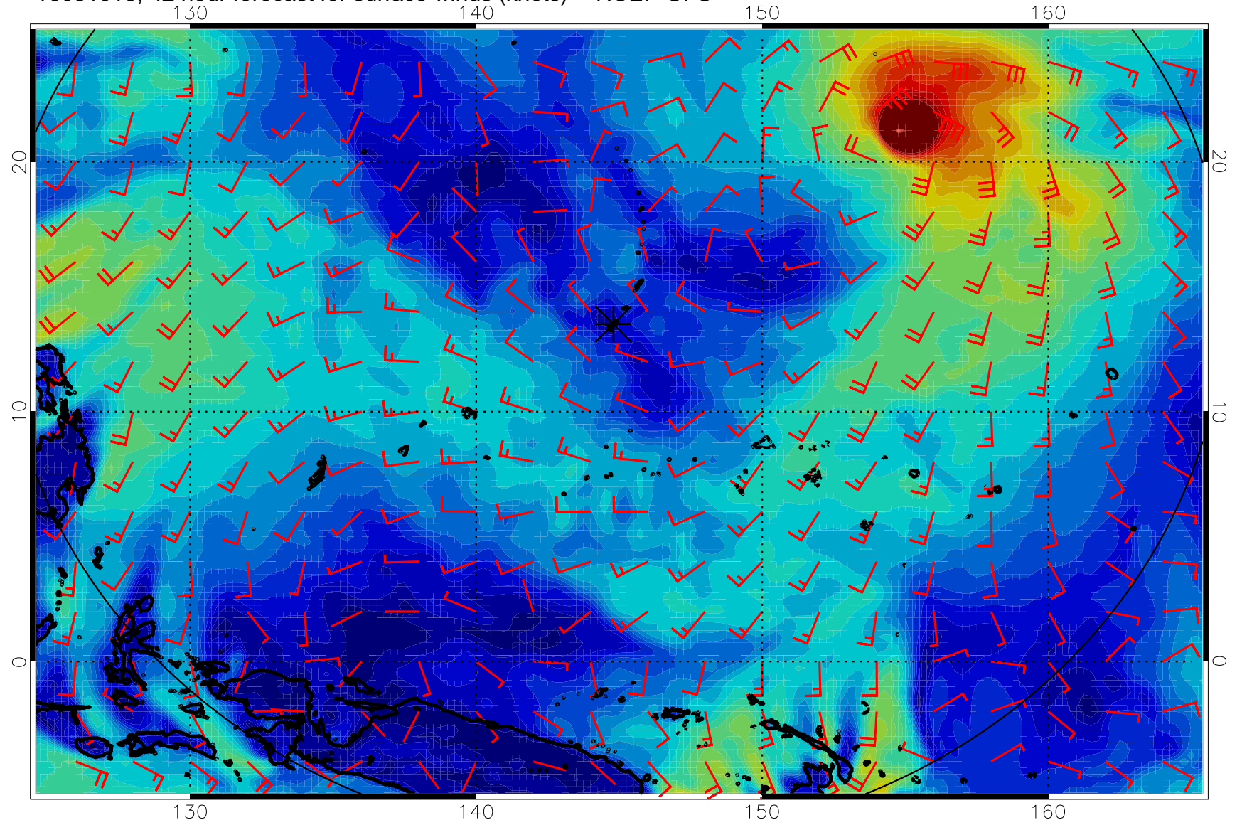
16081018, 42 hour forecast for surface winds (knots) -- NCEP GFS
