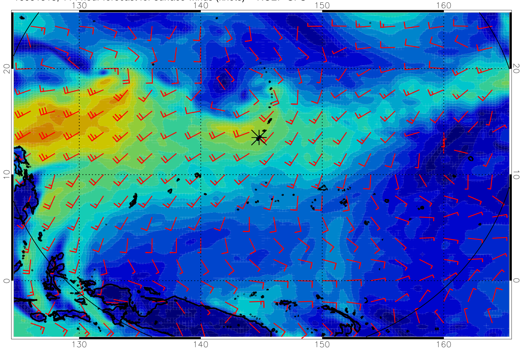
16081318, 114 hour forecast for surface winds (knots) -- NCEP GFS
