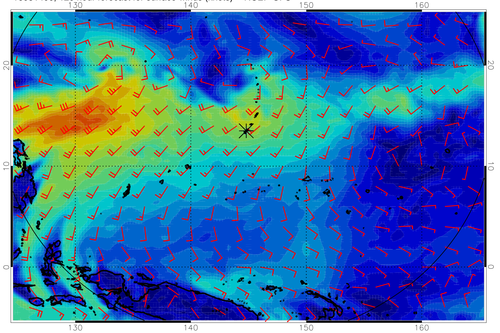
16081400, 120 hour forecast for surface winds (knots) -- NCEP GFS
