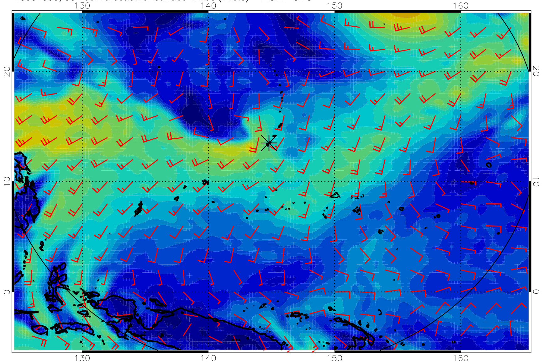
16081300, 96 hour forecast for surface winds (knots) -- NCEP GFS
