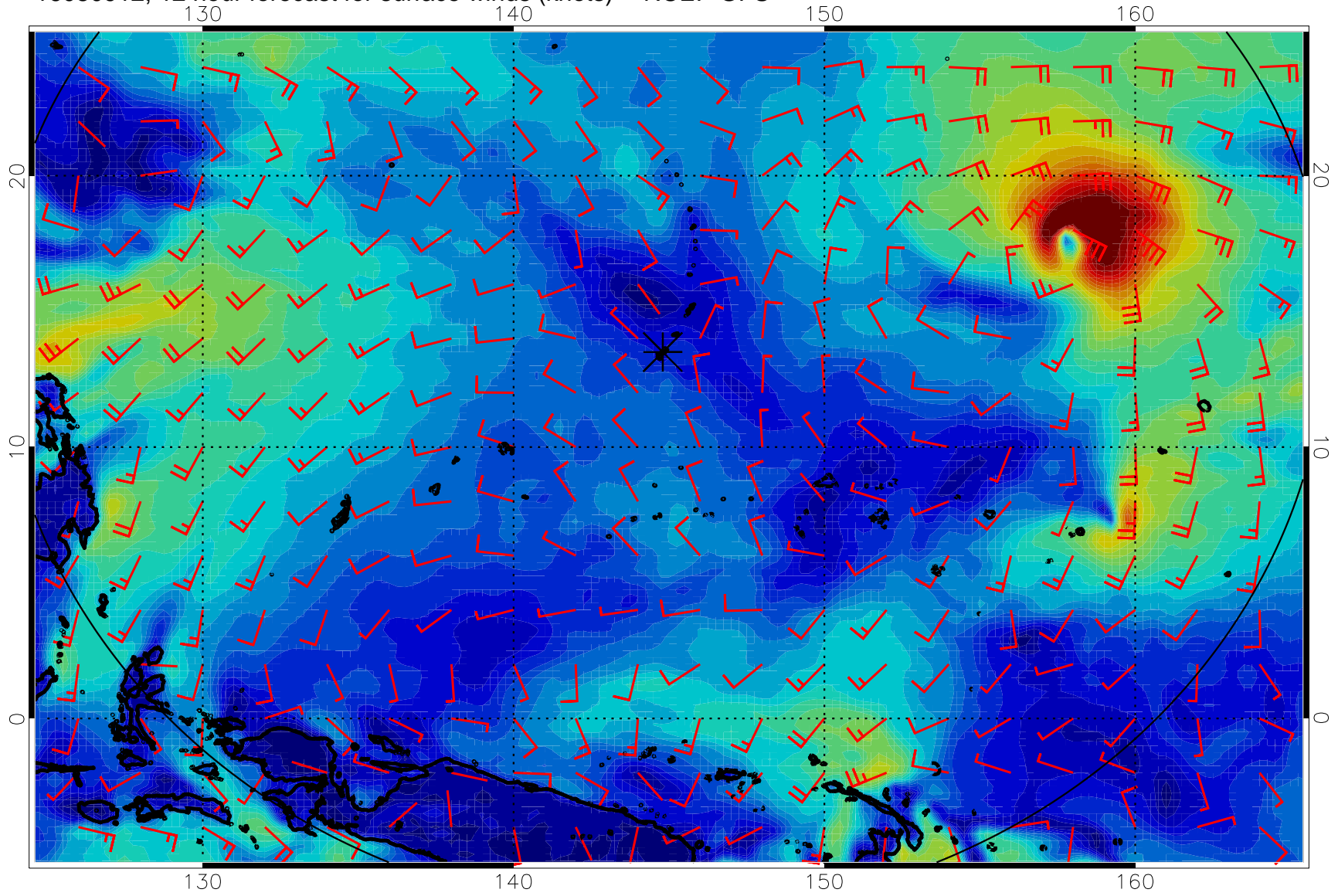
16080912, 12 hour forecast for surface winds (knots) -- NCEP GFS
