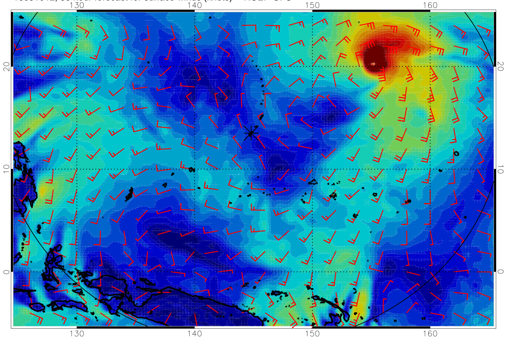
16081012, 36 hour forecast for surface winds (knots) -- NCEP GFS
