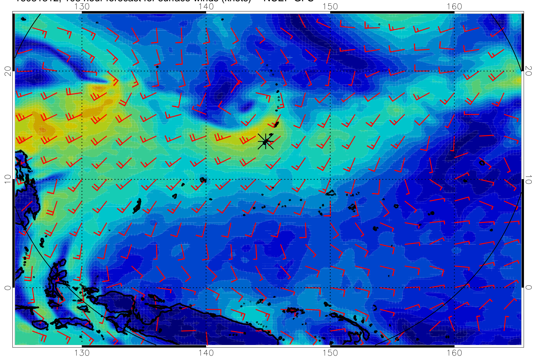
16081312, 108 hour forecast for surface winds (knots) -- NCEP GFS
