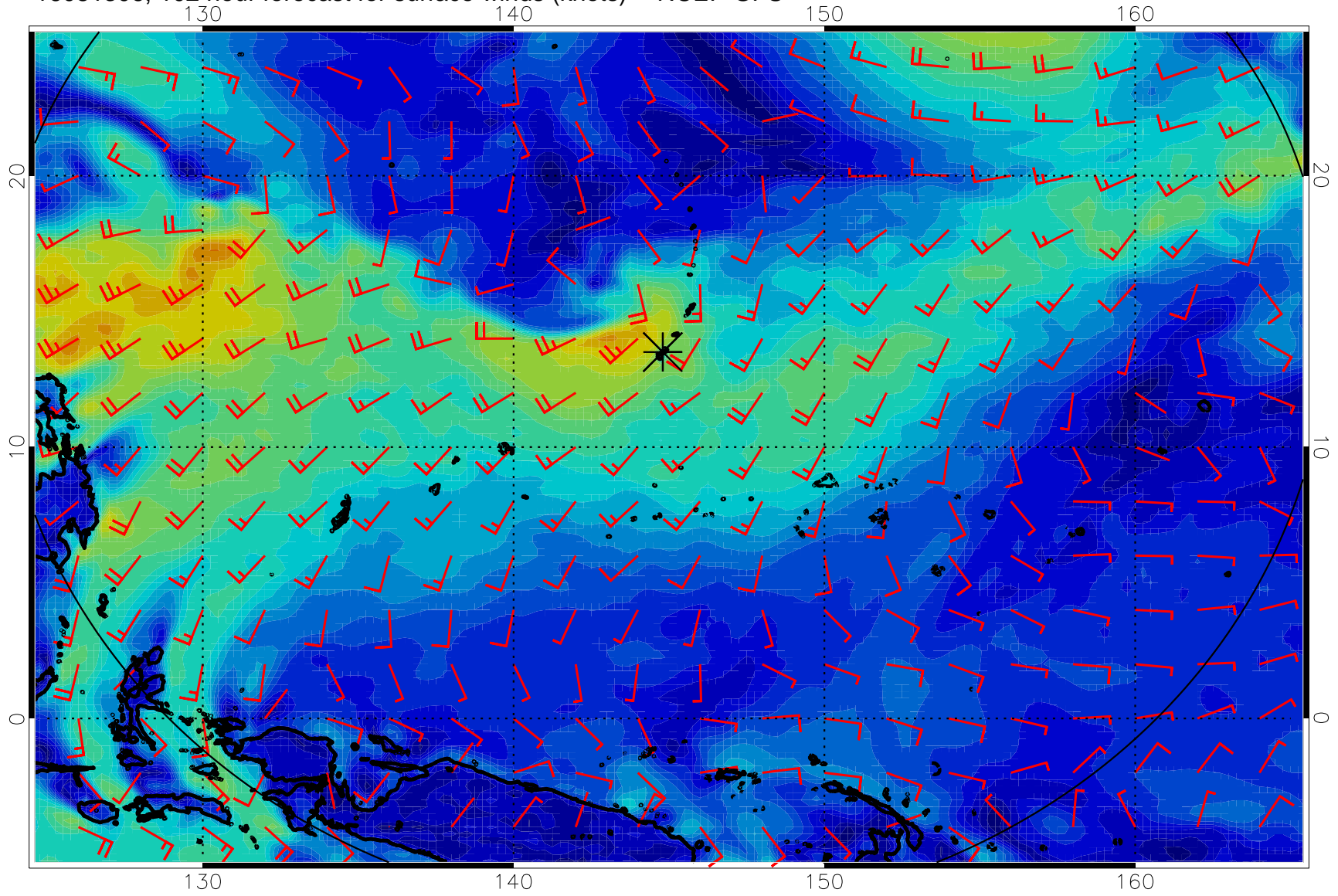
16081306, 102 hour forecast for surface winds (knots) -- NCEP GFS
