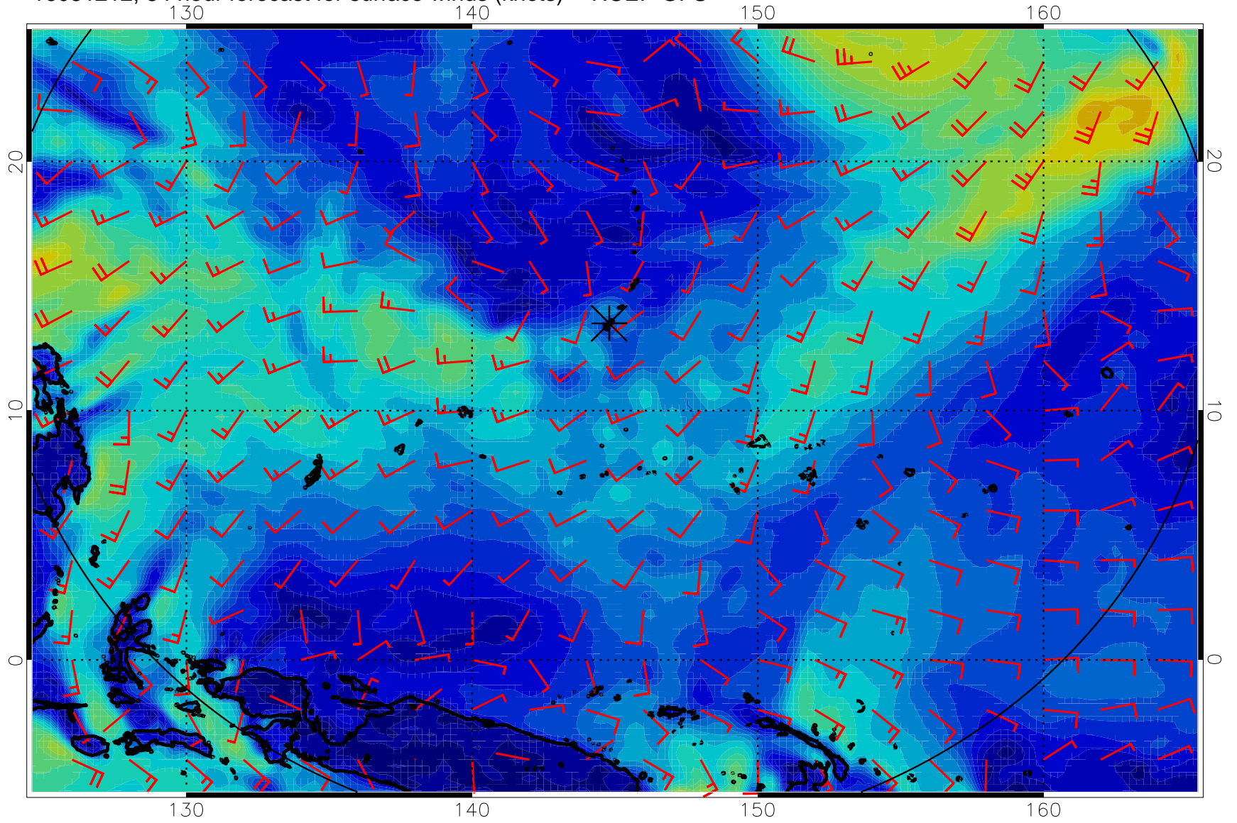
16081212, 84 hour forecast for surface winds (knots) -- NCEP GFS
