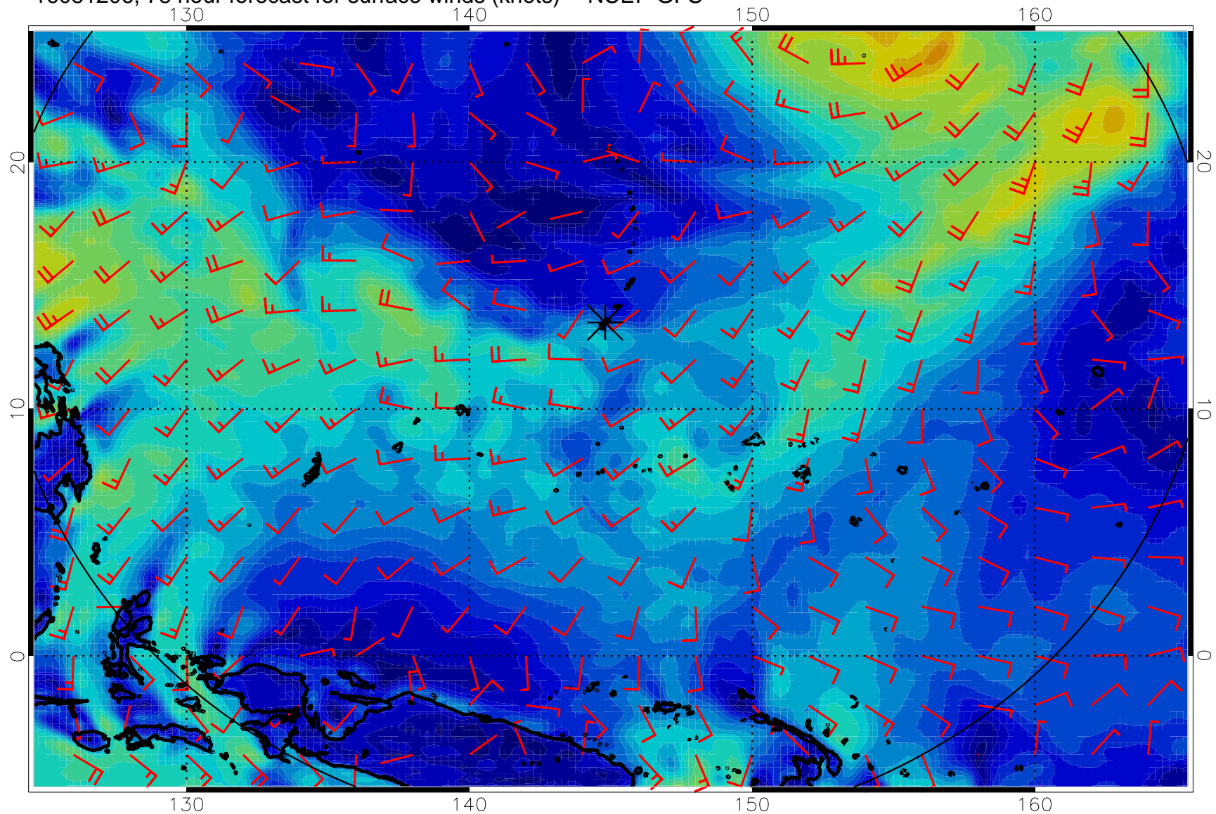
16081206, 78 hour forecast for surface winds (knots) -- NCEP GFS
