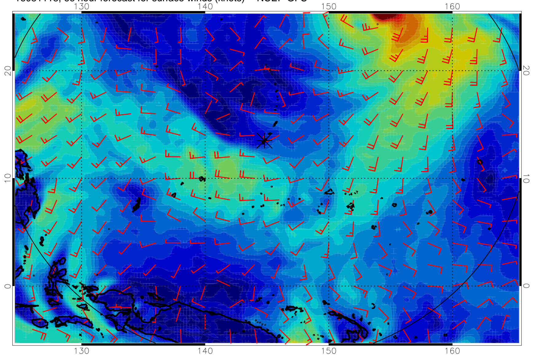
16081118, 66 hour forecast for surface winds (knots) -- NCEP GFS
