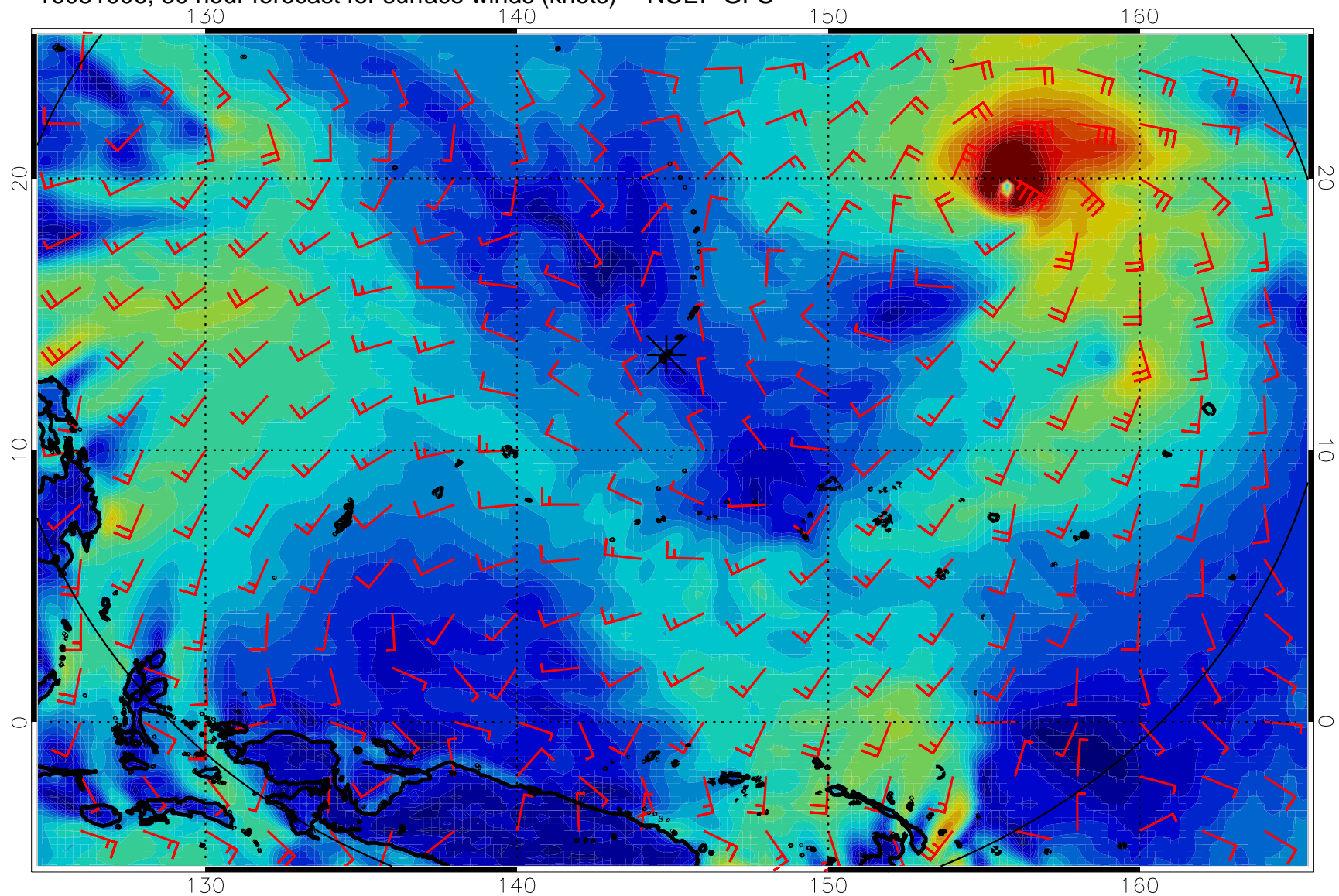
16081006, 30 hour forecast for surface winds (knots) -- NCEP GFS
