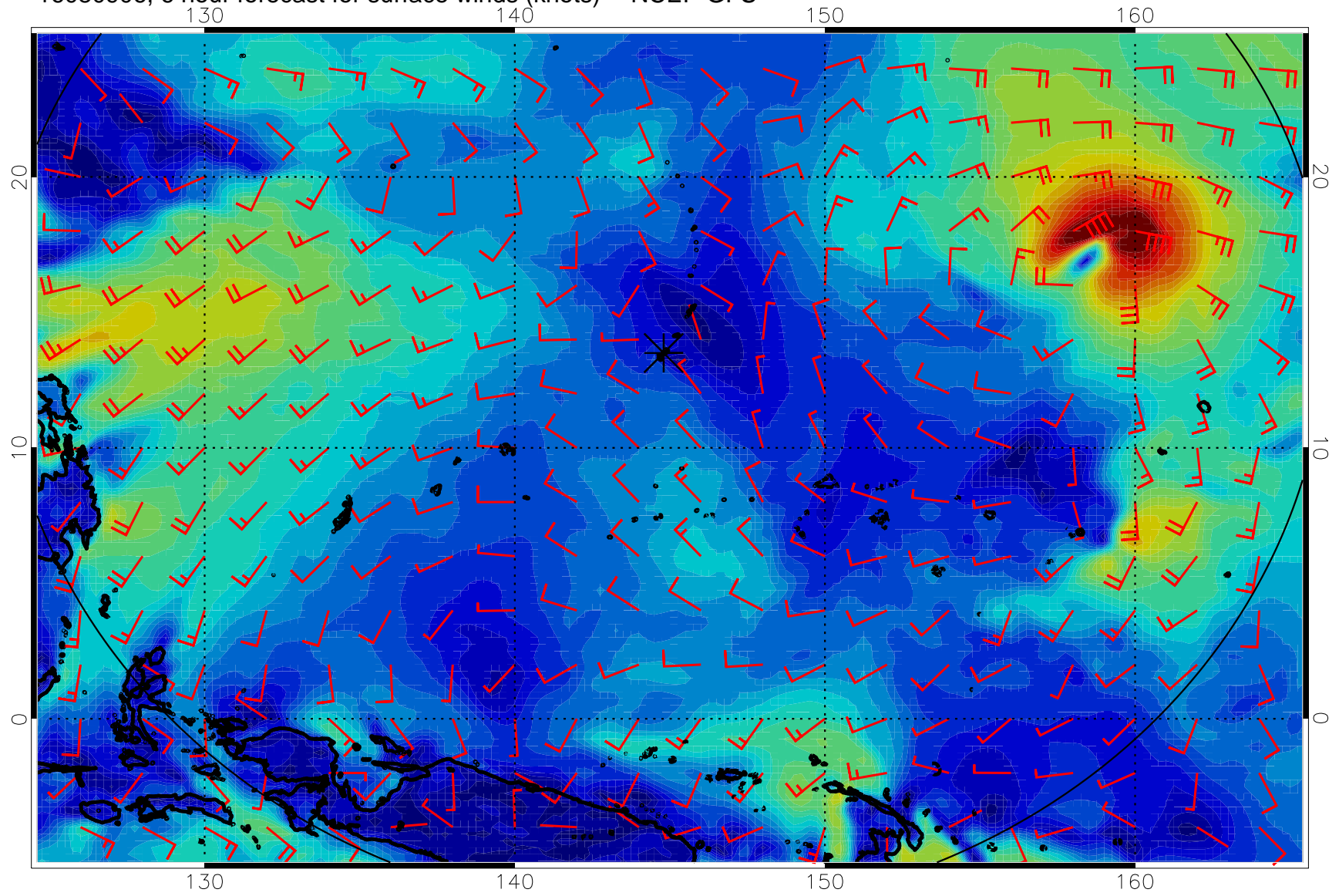
16080906, 6 hour forecast for surface winds (knots) -- NCEP GFS
