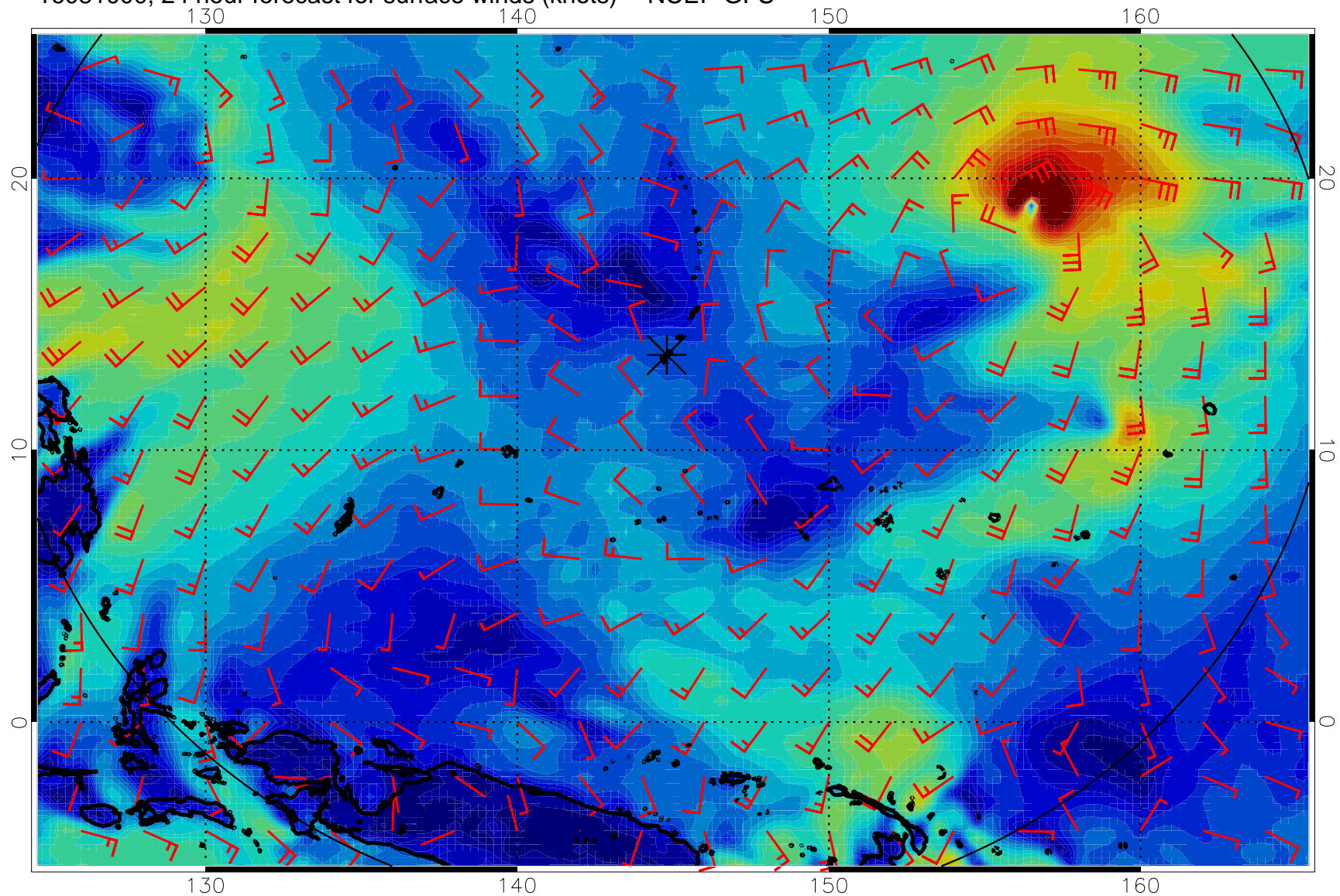
16081000, 24 hour forecast for surface winds (knots) -- NCEP GFS
