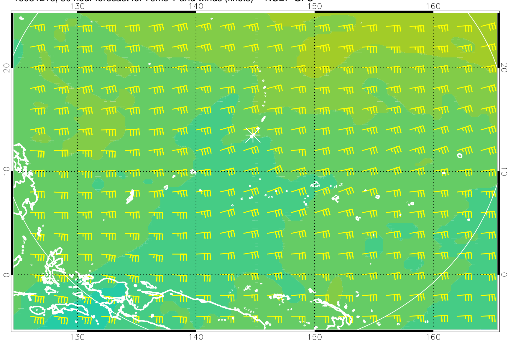
16081218, 90 hour forecast for 70mb T and winds (knots) -- NCEP GFS
