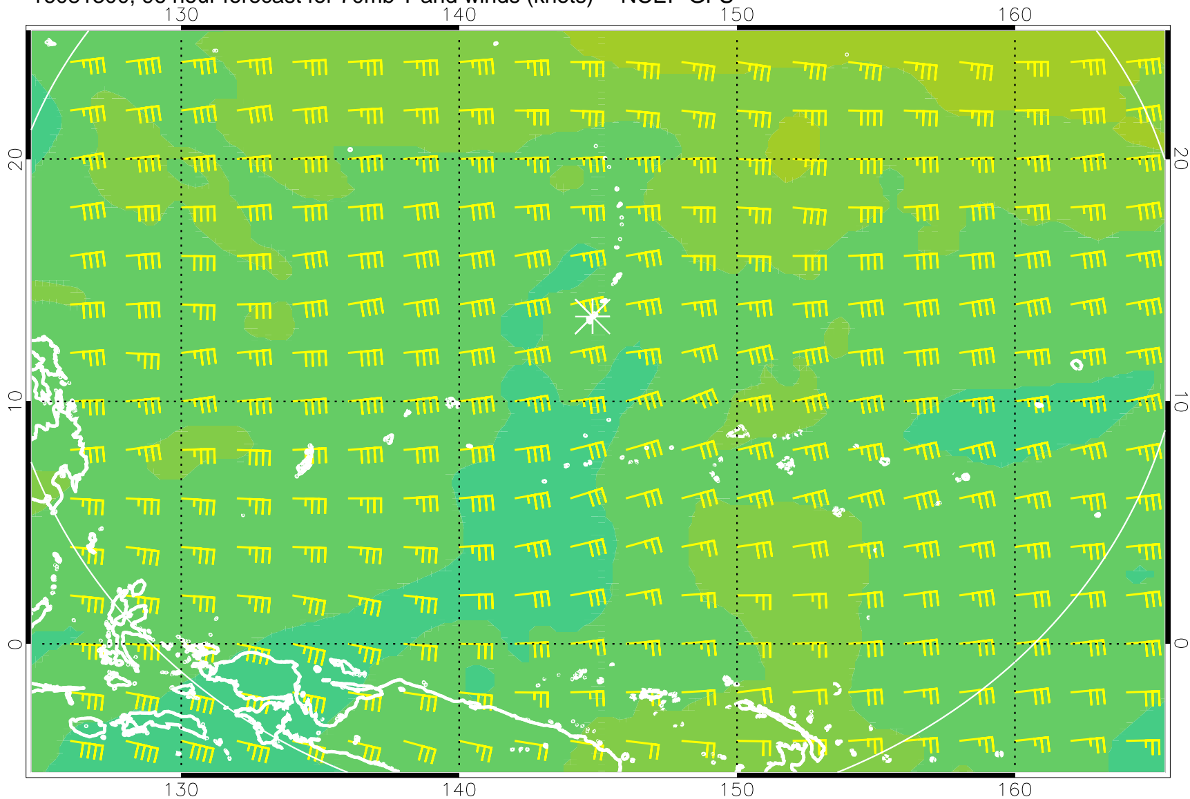
16081300, 96 hour forecast for 70mb T and winds (knots) -- NCEP GFS
