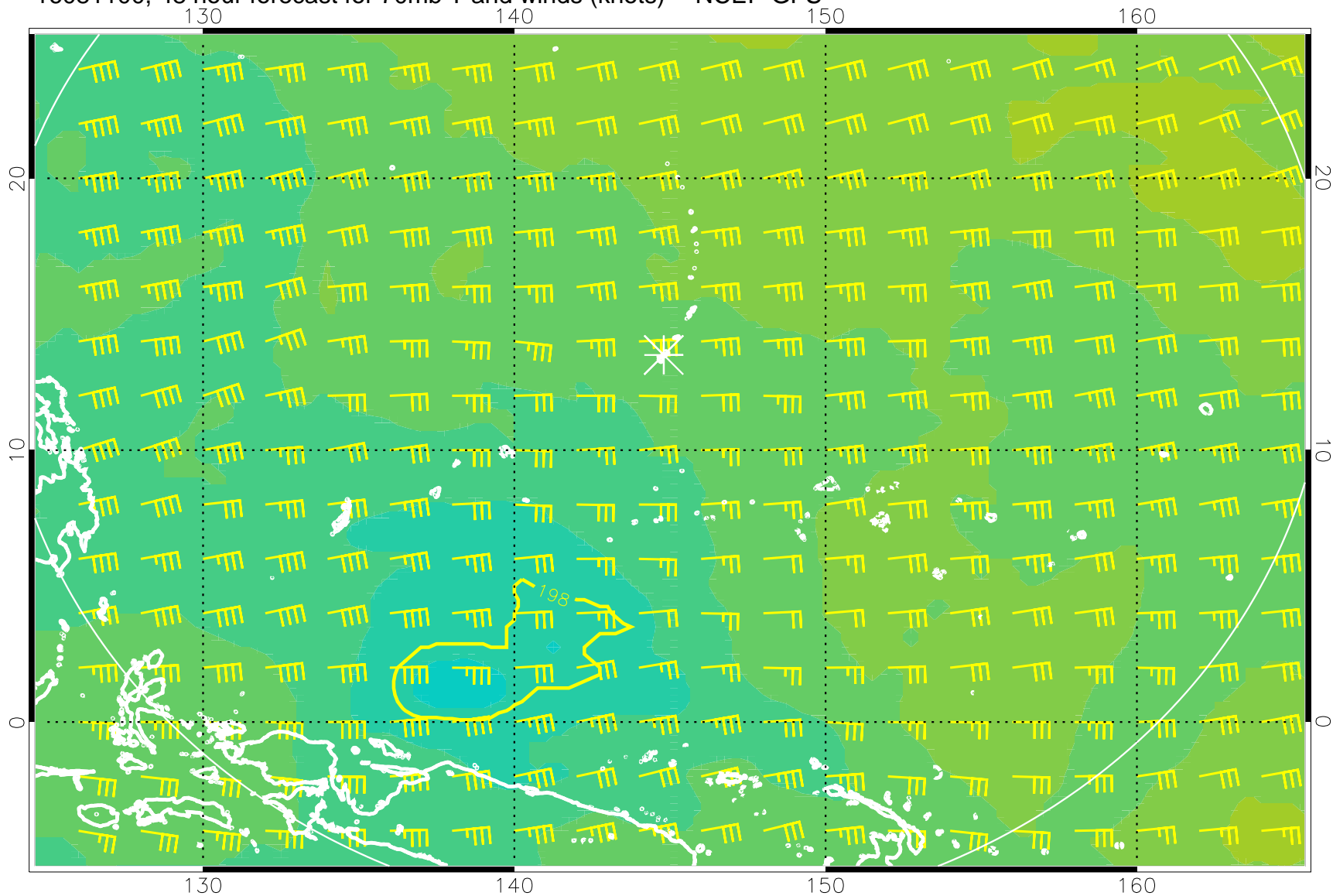
16081100, 48 hour forecast for 70mb T and winds (knots) -- NCEP GFS
