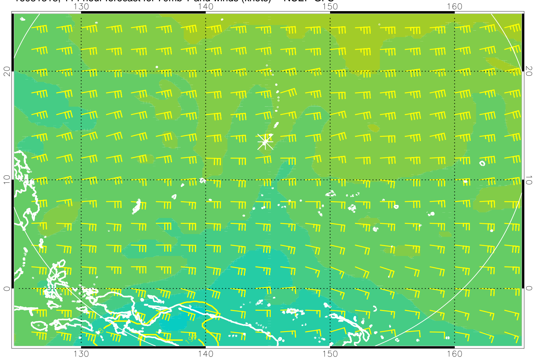
16081318, 114 hour forecast for 70mb T and winds (knots) -- NCEP GFS
