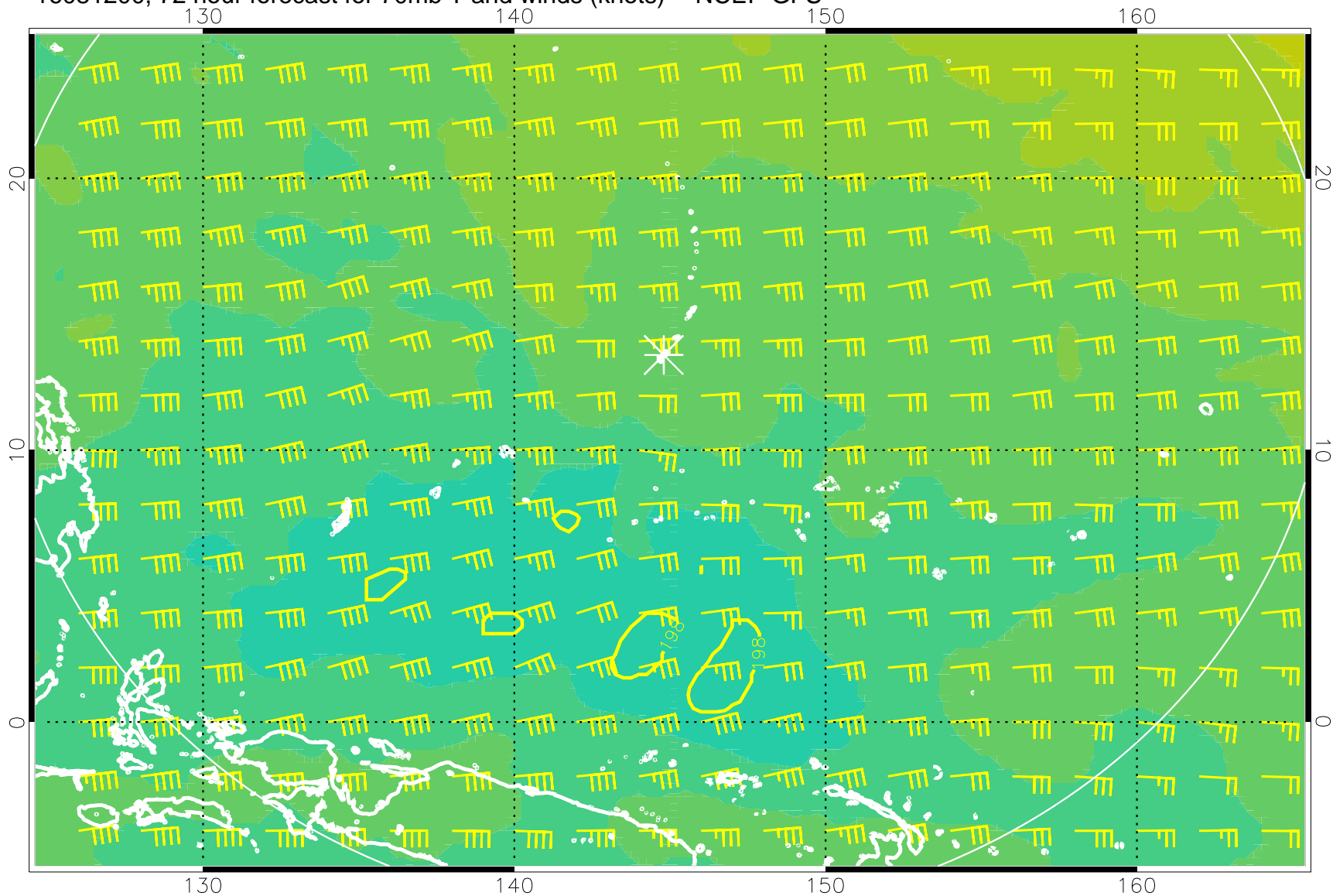
16081200, 72 hour forecast for 70mb T and winds (knots) -- NCEP GFS
