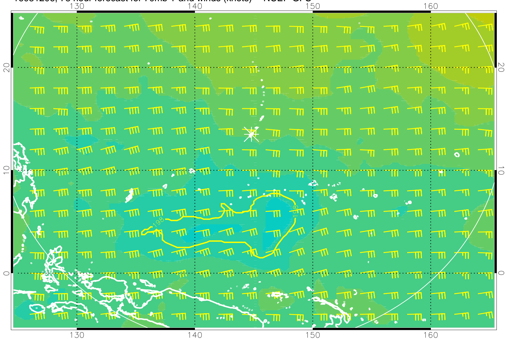
16081206, 78 hour forecast for 70mb T and winds (knots) -- NCEP GFS
