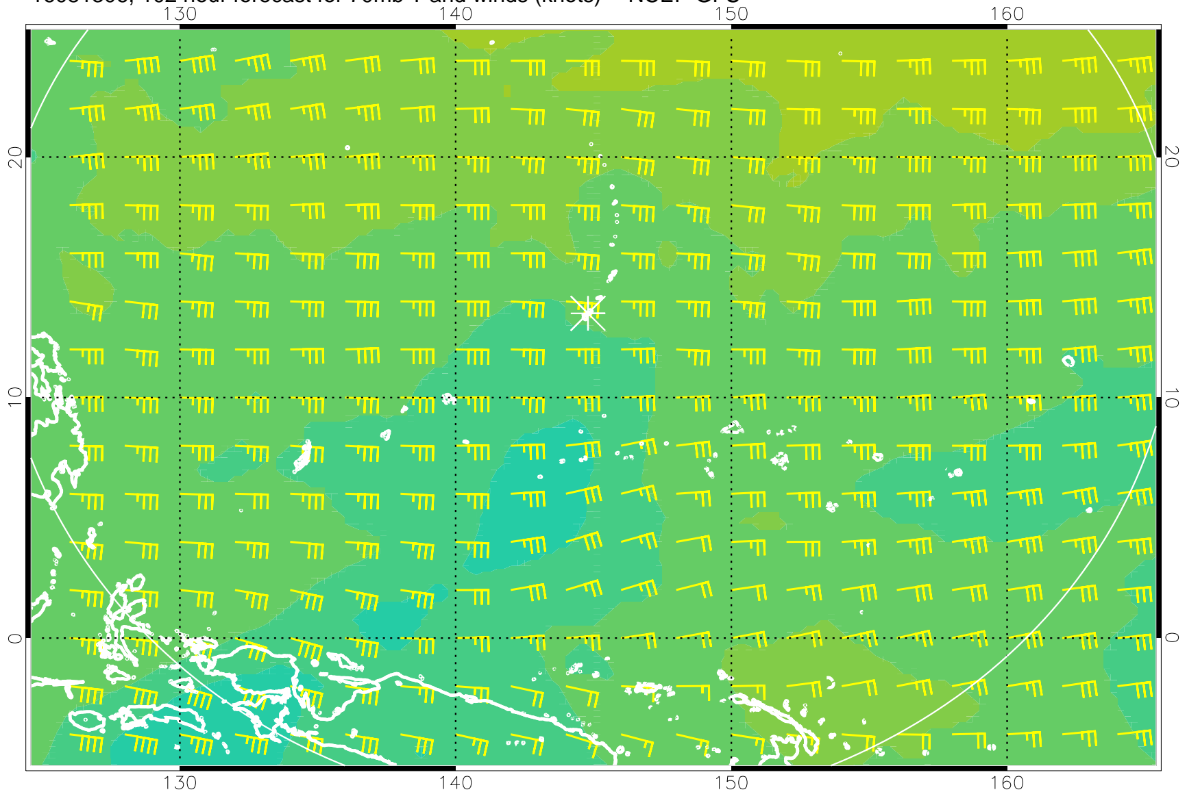
16081306, 102 hour forecast for 70mb T and winds (knots) -- NCEP GFS
