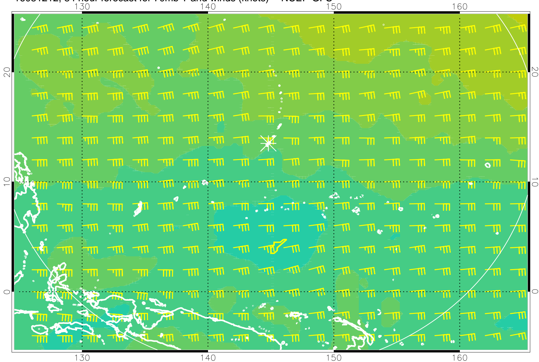
16081212, 84 hour forecast for 70mb T and winds (knots) -- NCEP GFS
