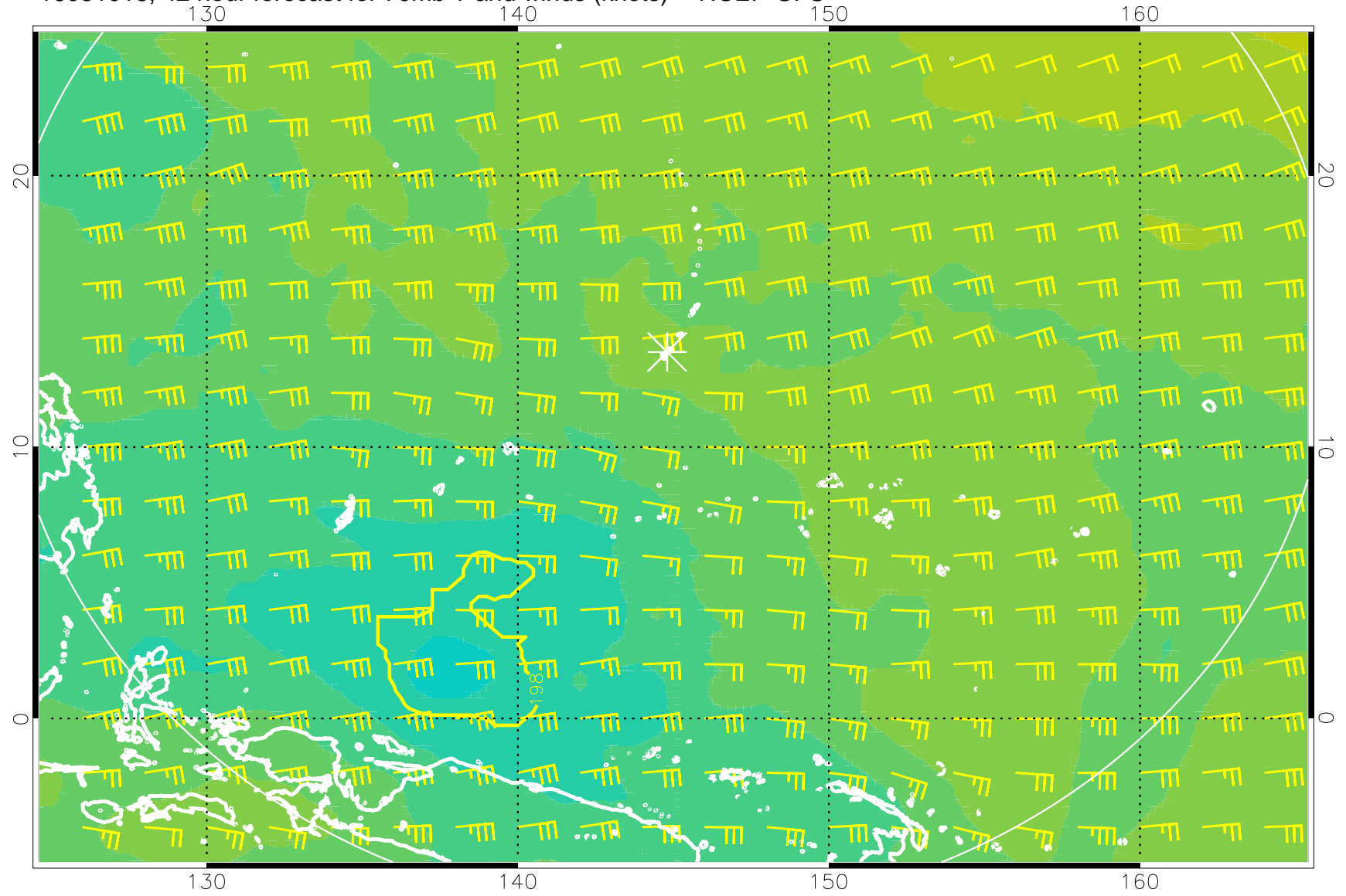
16081018, 42 hour forecast for 70mb T and winds (knots) -- NCEP GFS
