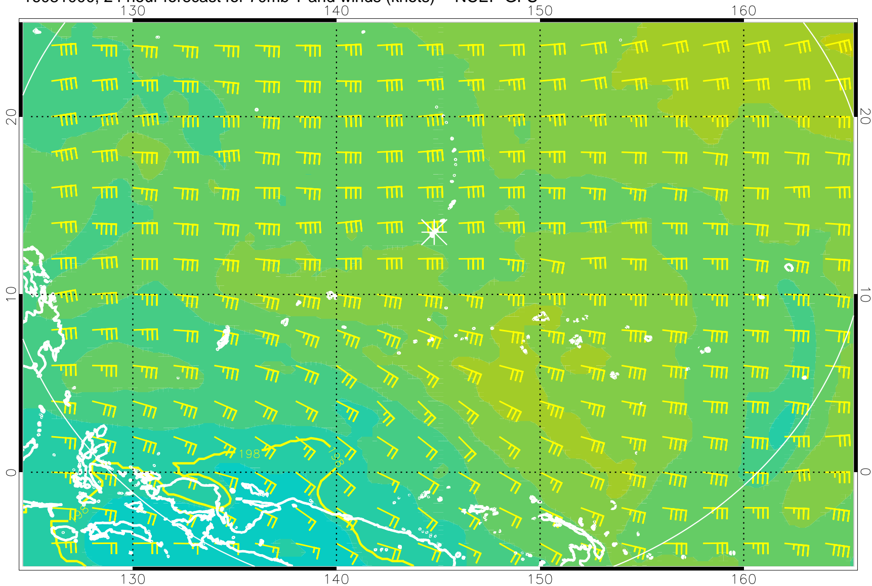
16081000, 24 hour forecast for 70mb T and winds (knots) -- NCEP GFS
