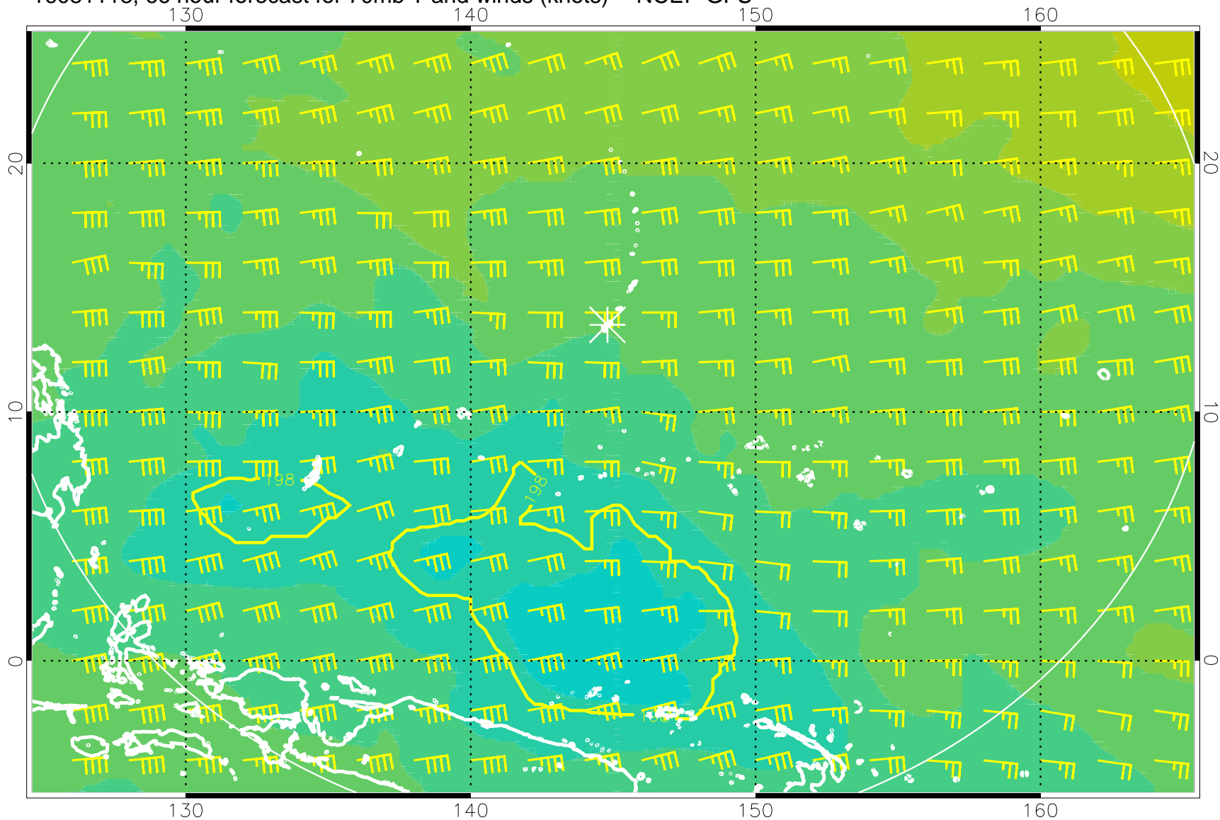
16081118, 66 hour forecast for 70mb T and winds (knots) -- NCEP GFS
