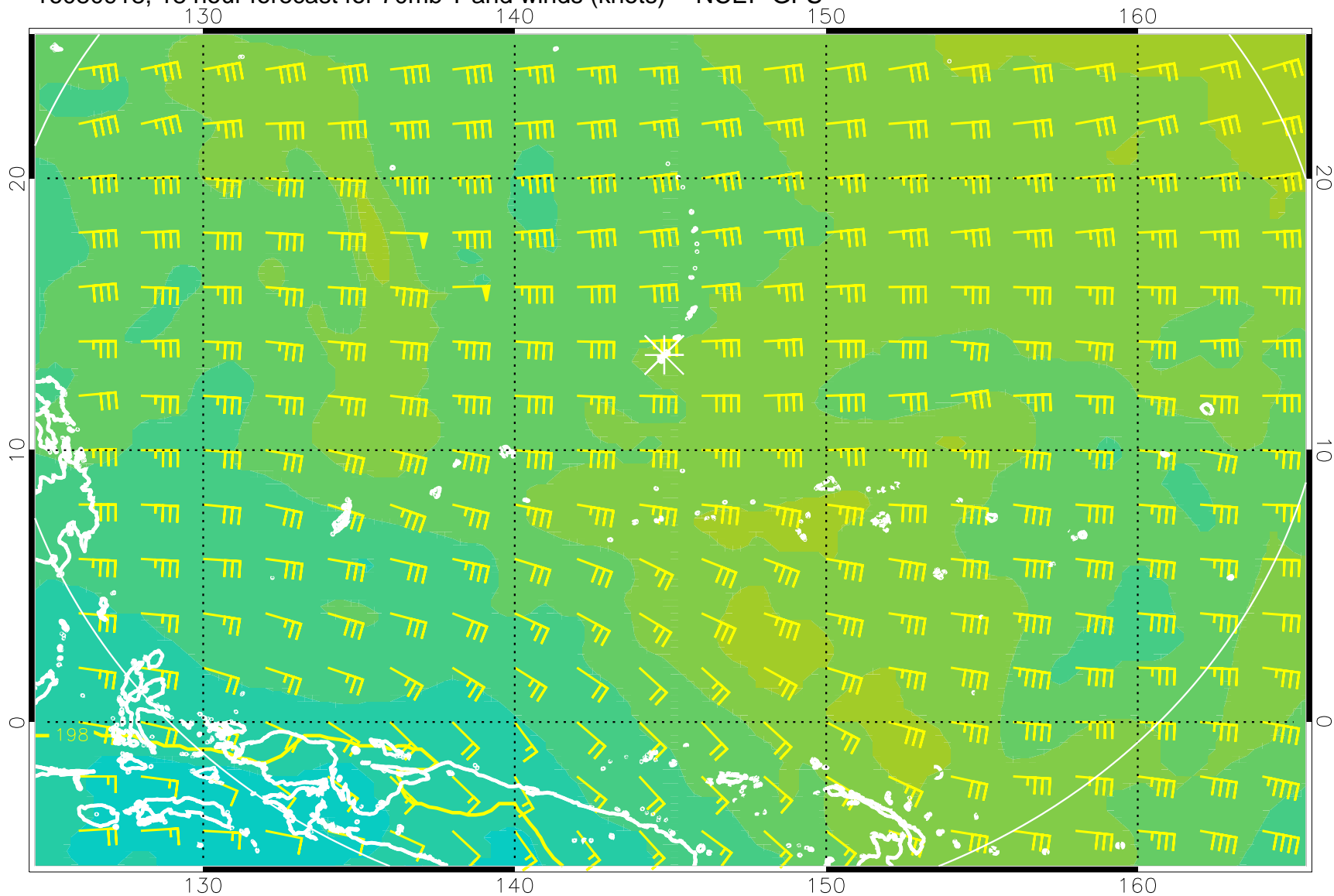
16080918, 18 hour forecast for 70mb T and winds (knots) -- NCEP GFS
