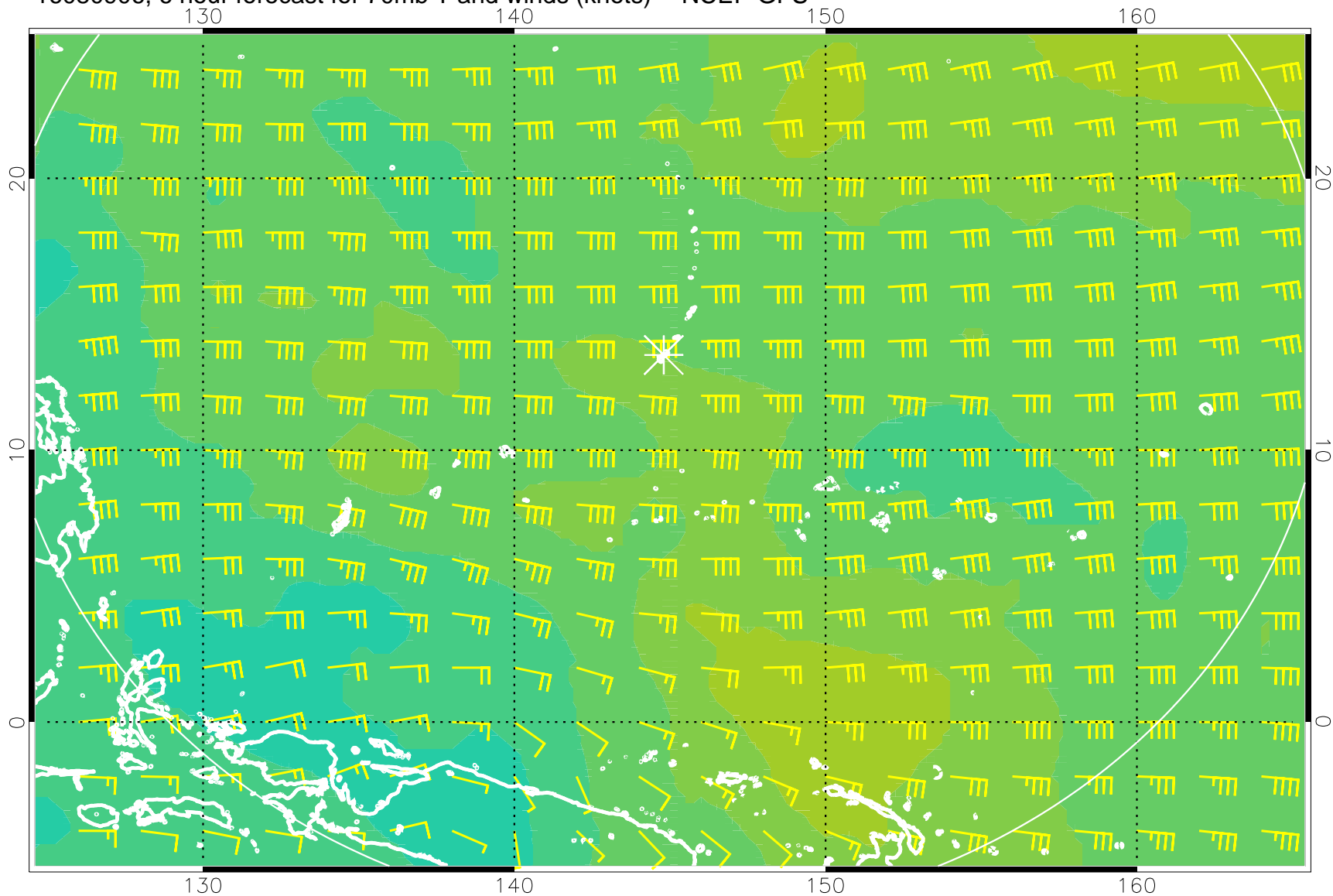
16080906, 6 hour forecast for 70mb T and winds (knots) -- NCEP GFS
