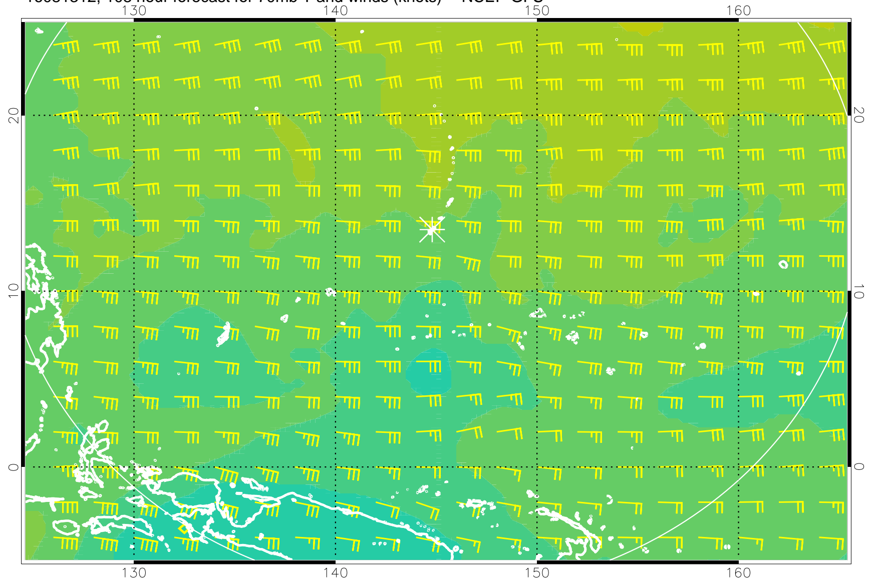
16081312, 108 hour forecast for 70mb T and winds (knots) -- NCEP GFS
