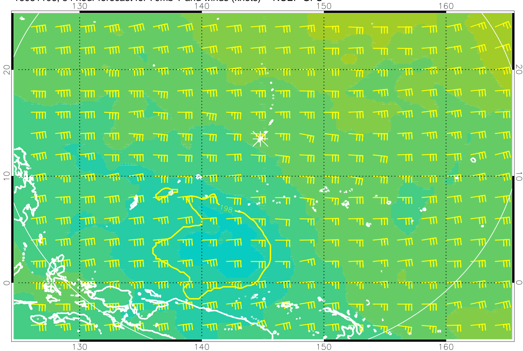
16081106, 54 hour forecast for 70mb T and winds (knots) -- NCEP GFS
