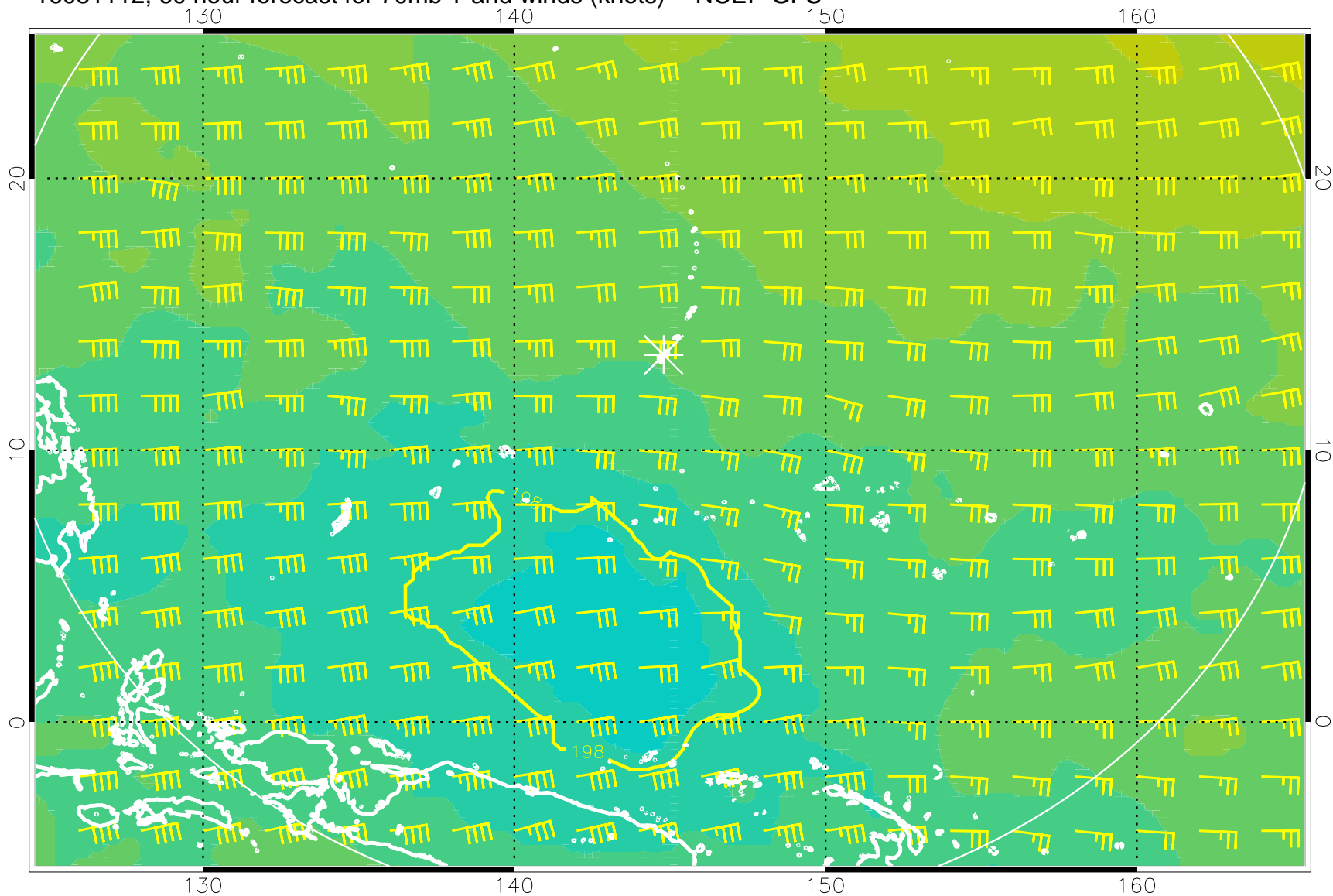
16081112, 60 hour forecast for 70mb T and winds (knots) -- NCEP GFS
