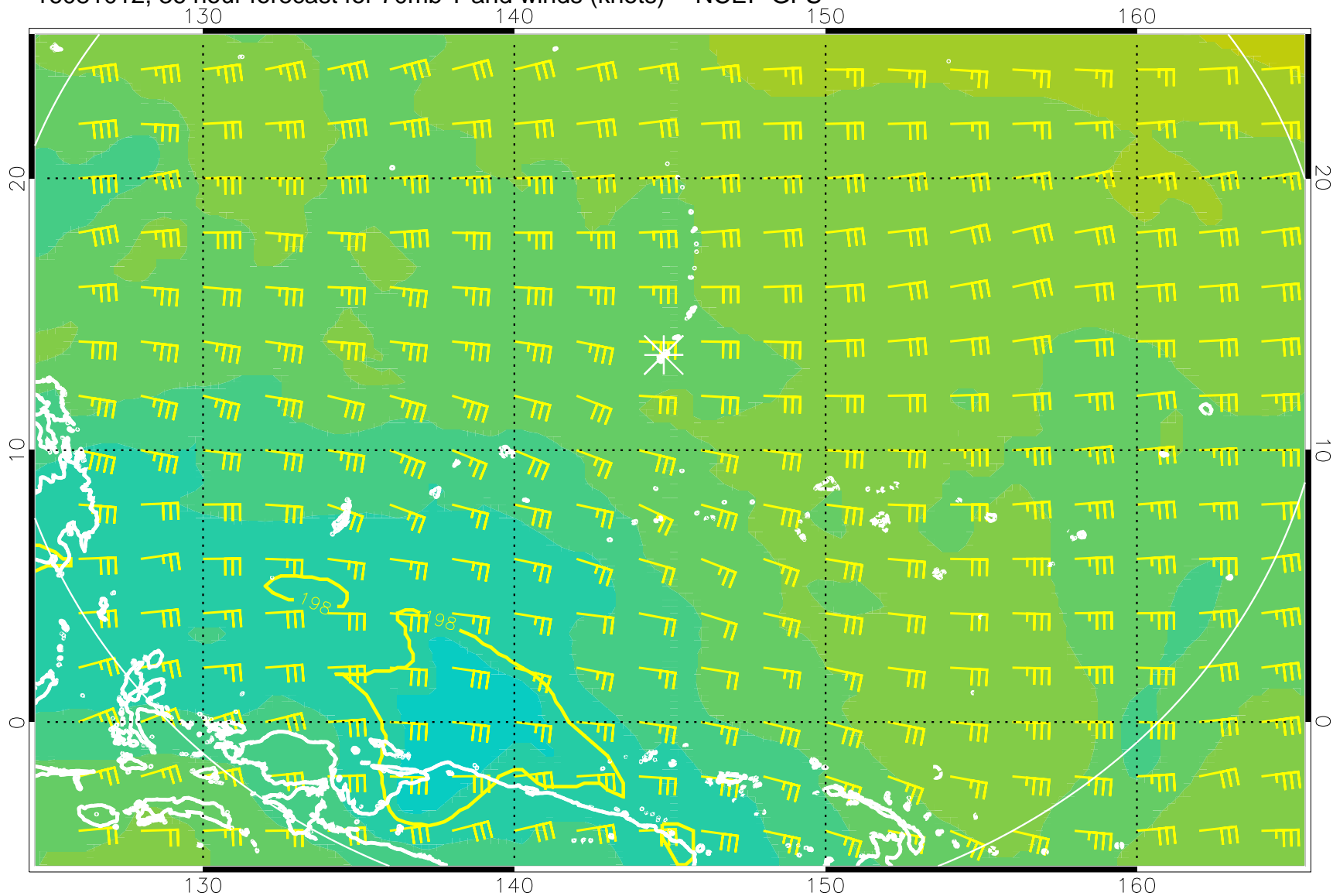
16081012, 36 hour forecast for 70mb T and winds (knots) -- NCEP GFS
