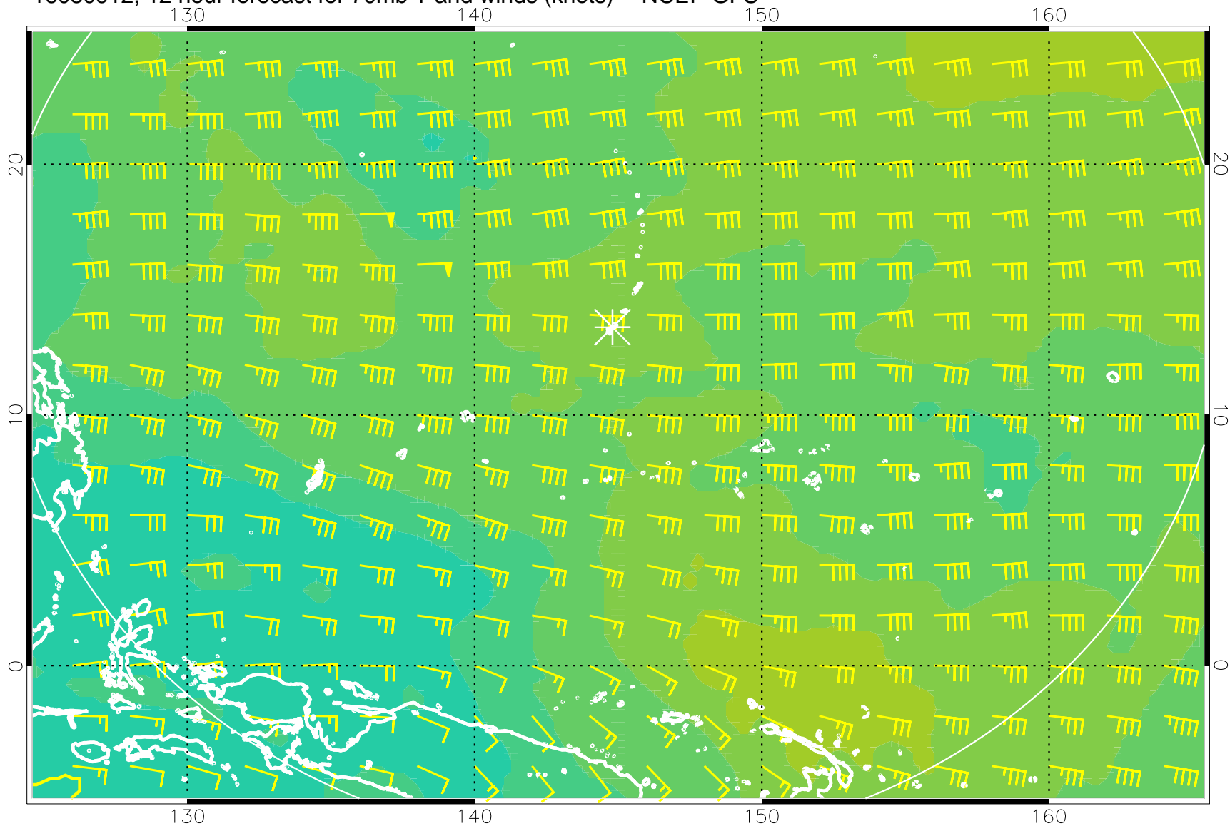
16080912, 12 hour forecast for 70mb T and winds (knots) -- NCEP GFS
