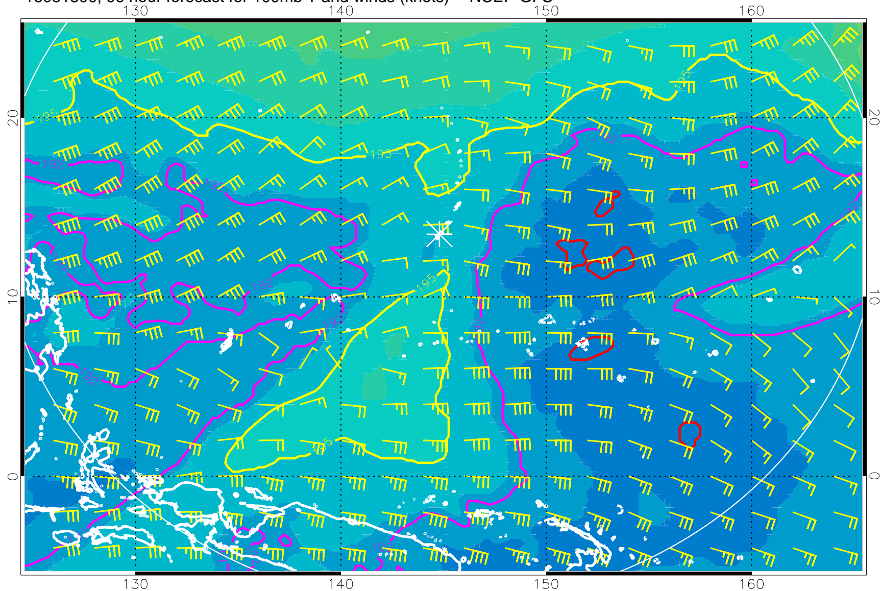
16081300, 96 hour forecast for 100mb T and winds (knots) -- NCEP GFS
