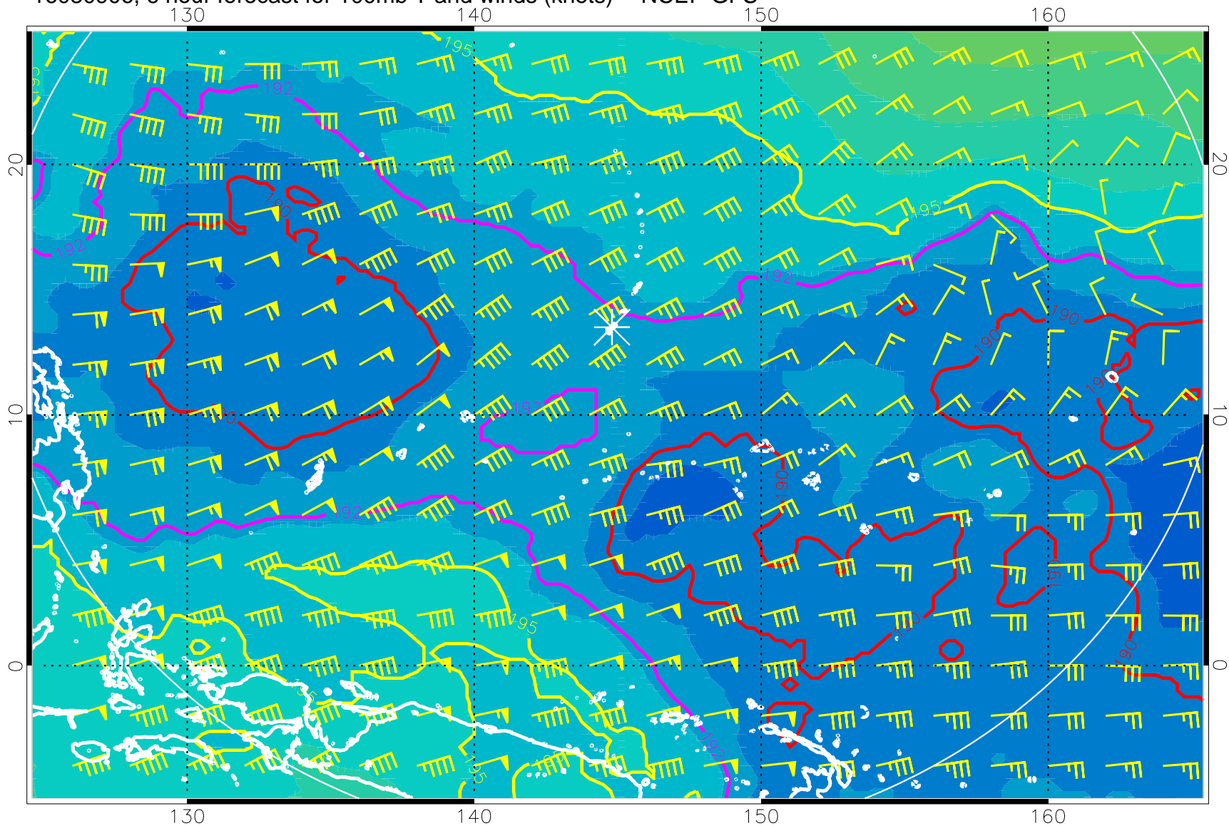
16080906, 6 hour forecast for 100mb T and winds (knots) -- NCEP GFS
