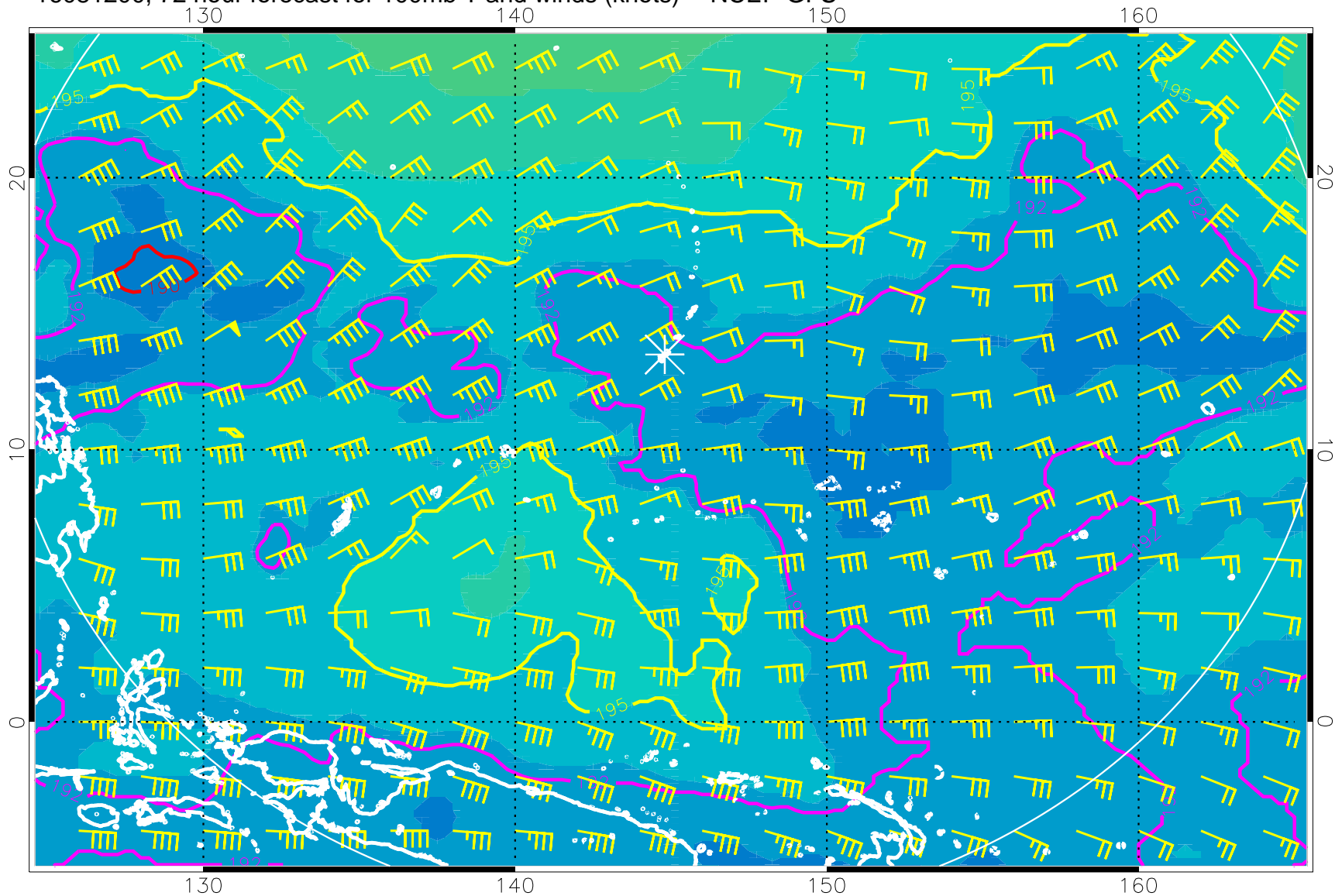
16081200, 72 hour forecast for 100mb T and winds (knots) -- NCEP GFS
