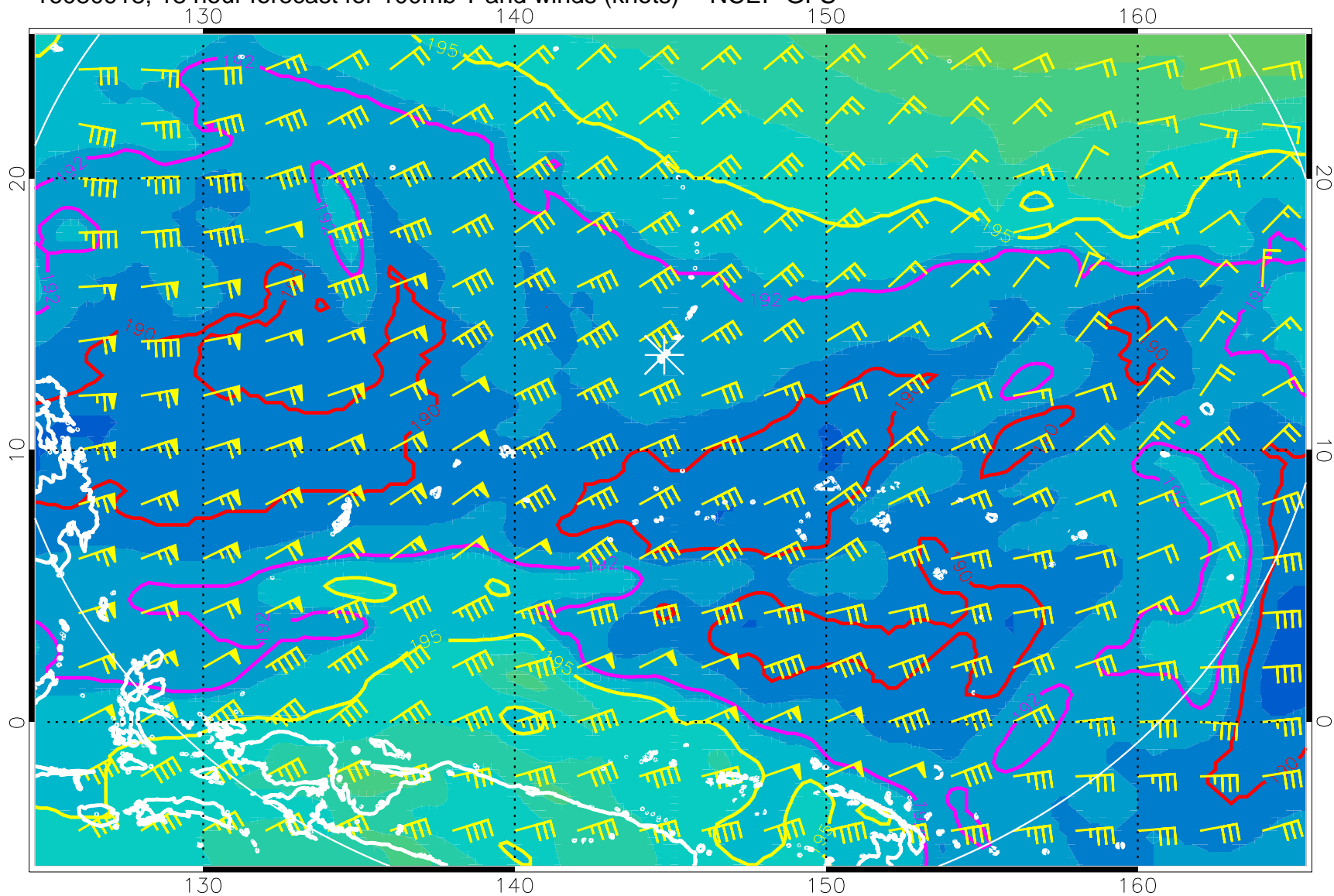
16080918, 18 hour forecast for 100mb T and winds (knots) -- NCEP GFS
