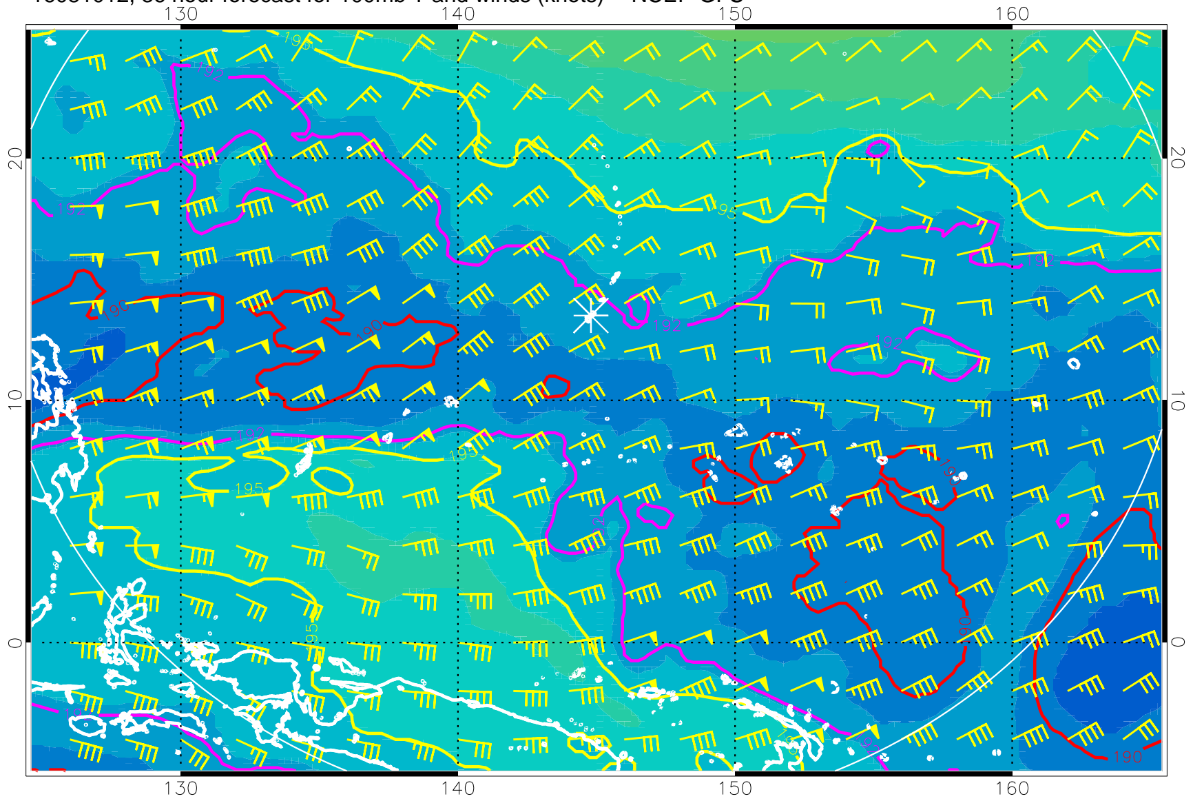
16081012, 36 hour forecast for 100mb T and winds (knots) -- NCEP GFS
