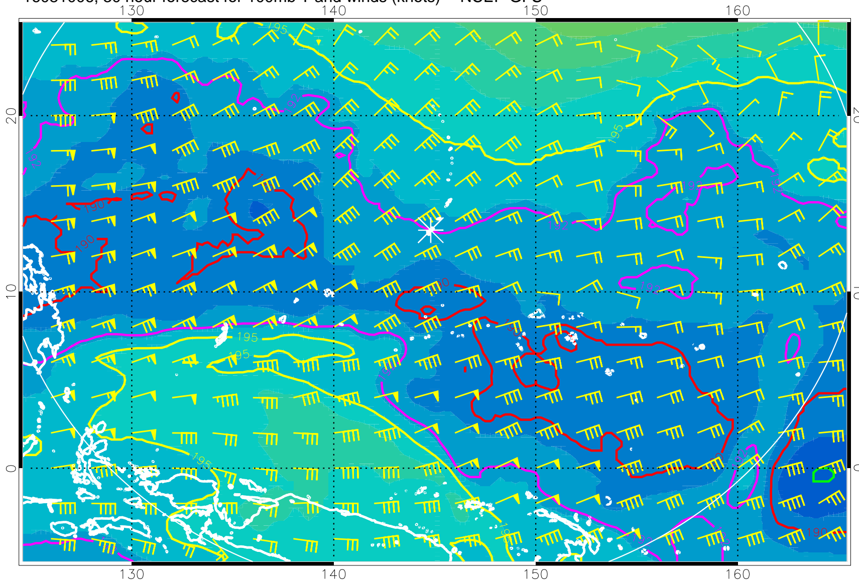
16081006, 30 hour forecast for 100mb T and winds (knots) -- NCEP GFS
