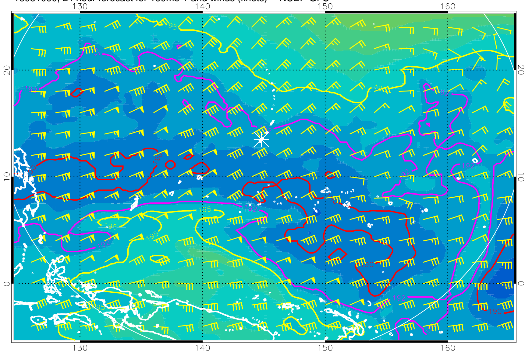
16081000, 24 hour forecast for 100mb T and winds (knots) -- NCEP GFS
