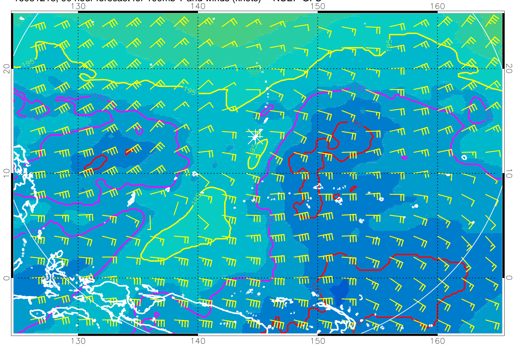
16081218, 90 hour forecast for 100mb T and winds (knots) -- NCEP GFS
