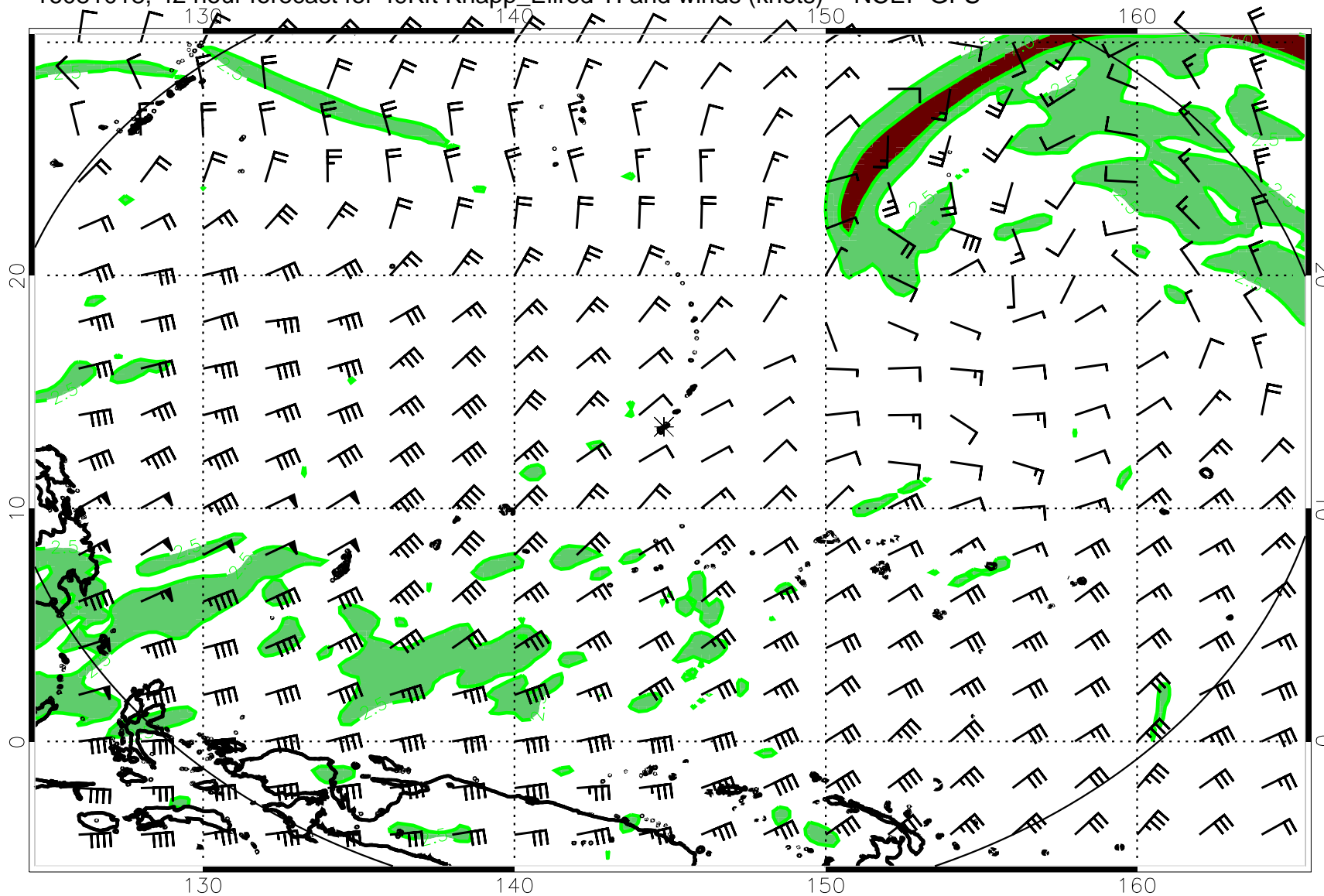
16081018, 42 hour forecast for 49Kft Knapp_Ellrod TI and winds (knots) -- NCEP GFS
