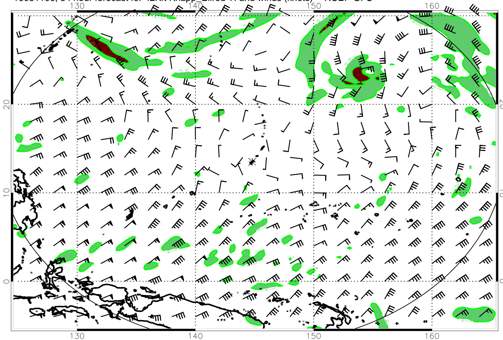
16081106, 54 hour forecast for 42Kft Knapp_Ellrod TI and winds (knots) -- NCEP GFS
