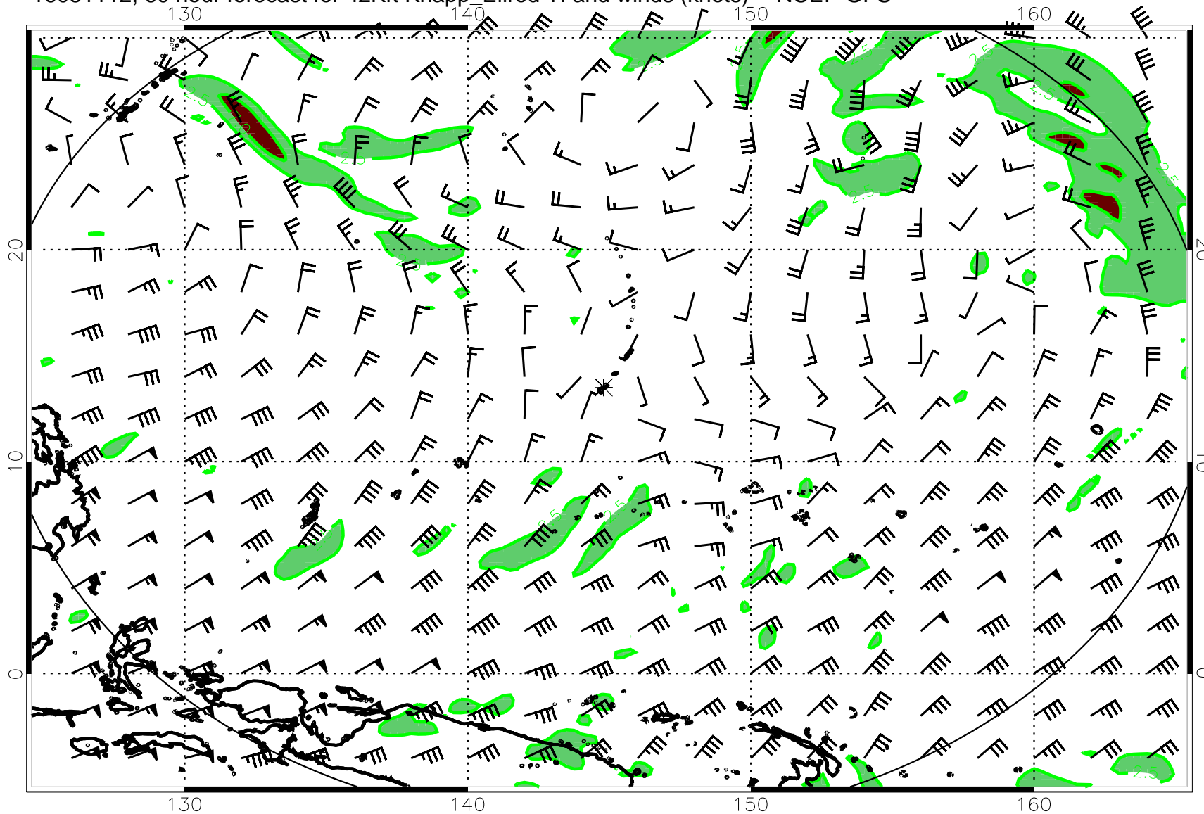
16081112, 60 hour forecast for 42Kft Knapp_Ellrod TI and winds (knots) -- NCEP GFS
