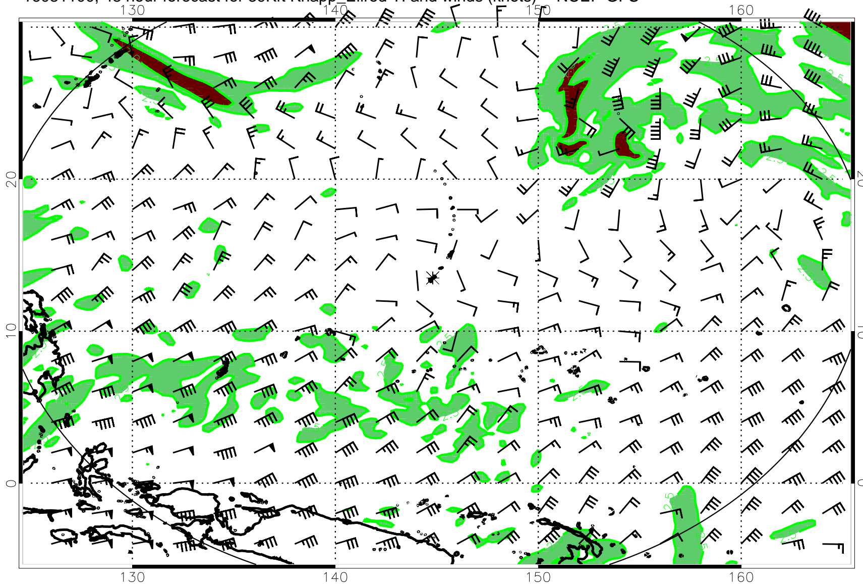
16081100, 48 hour forecast for 39Kft Knapp_Ellrod TI and winds (knots) -- NCEP GFS
