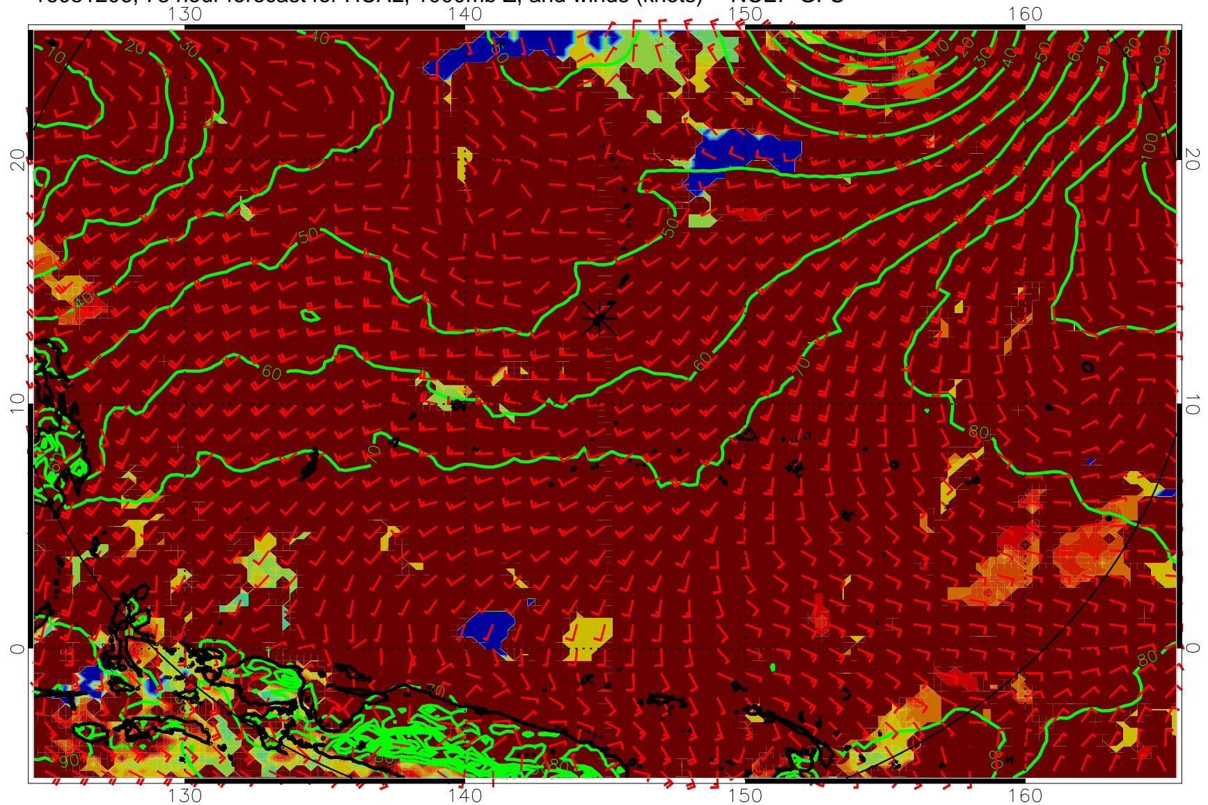
16081206, 78 hour forecast for HCAL, 1000mb Z, and winds (knots) -- NCEP GFS
