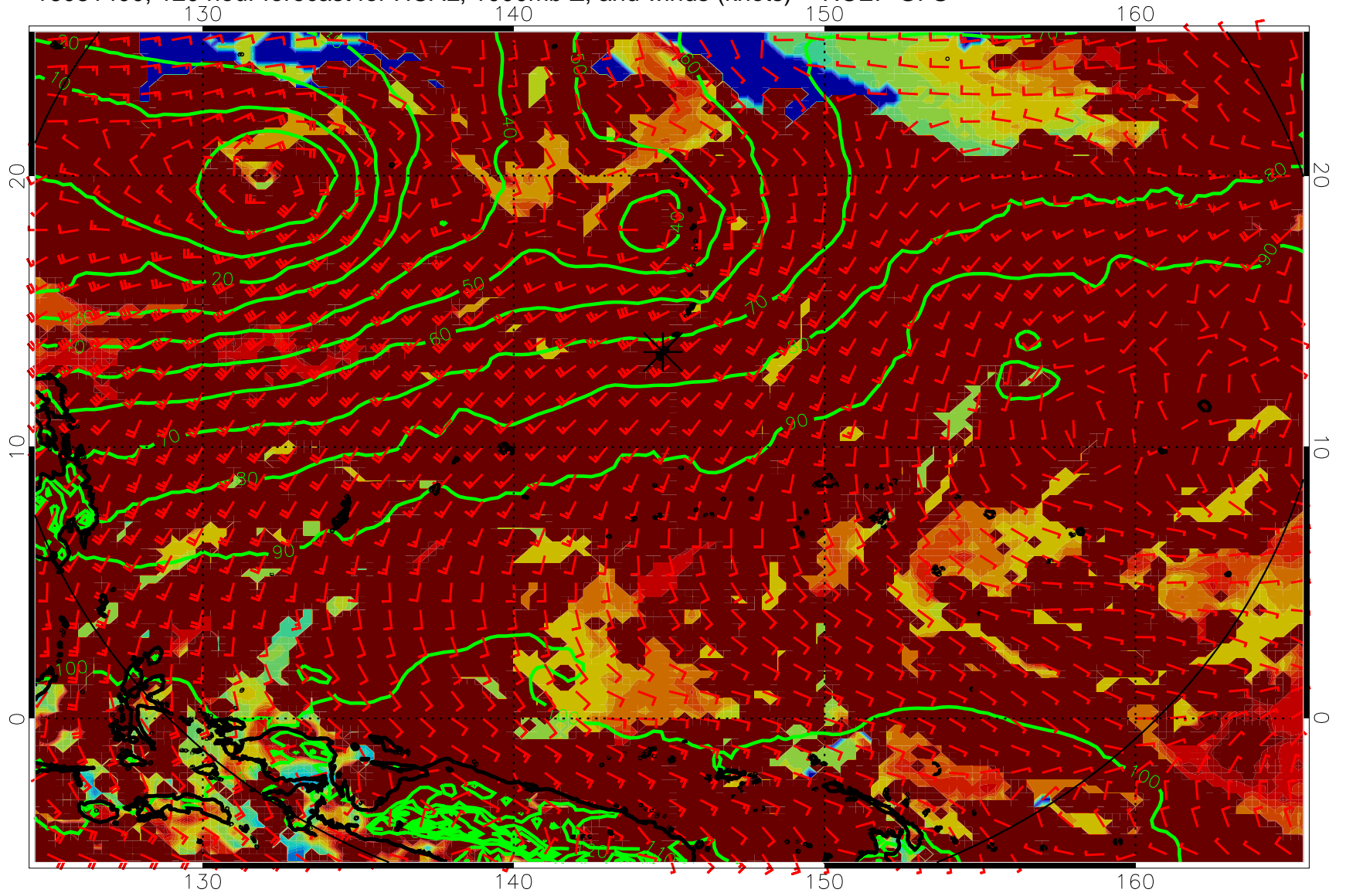
16081400, 120 hour forecast for HCAL, 1000mb Z, and winds (knots) -- NCEP GFS
