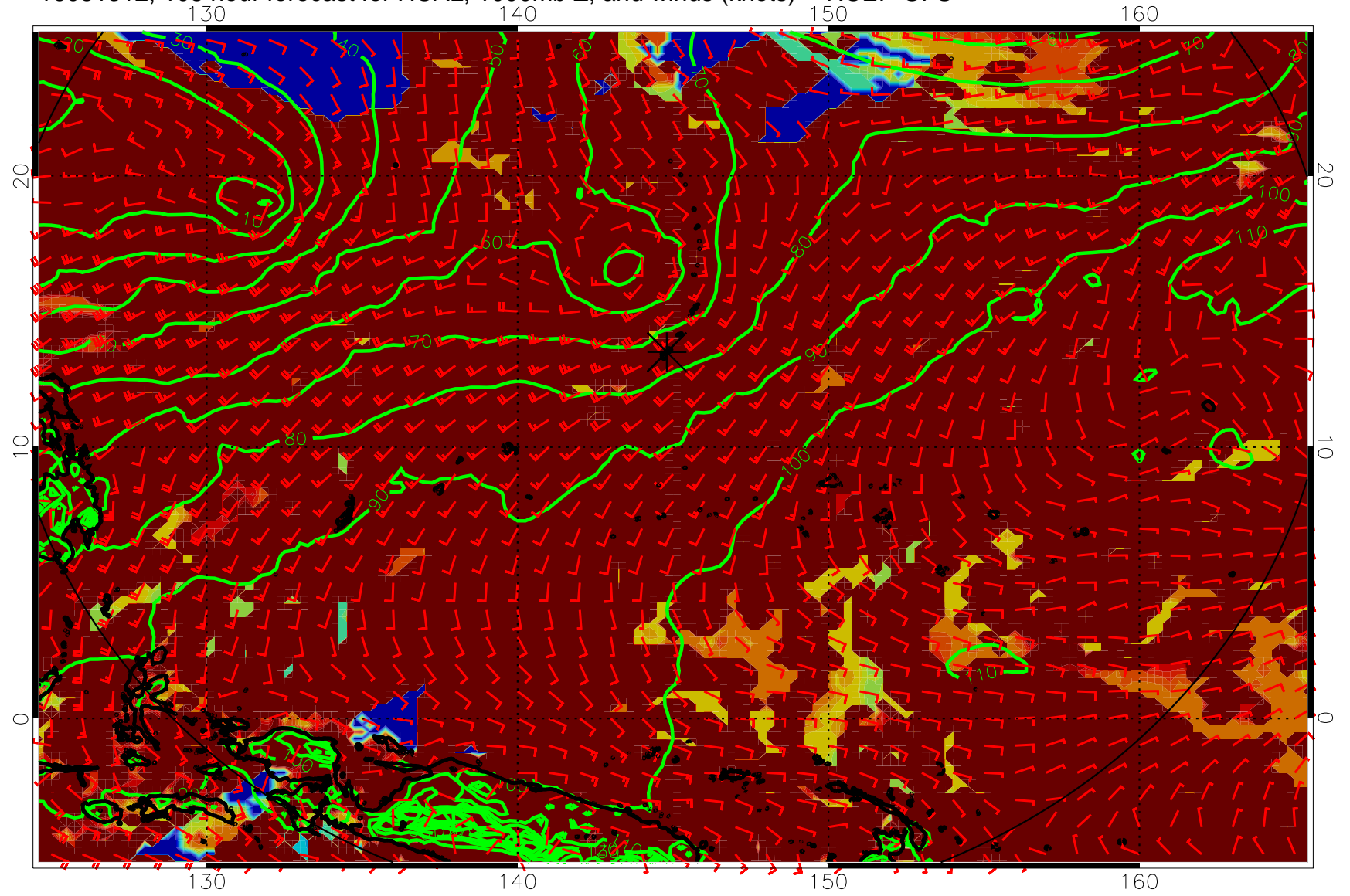
16081312, 108 hour forecast for HCAL, 1000mb Z, and winds (knots) -- NCEP GFS
