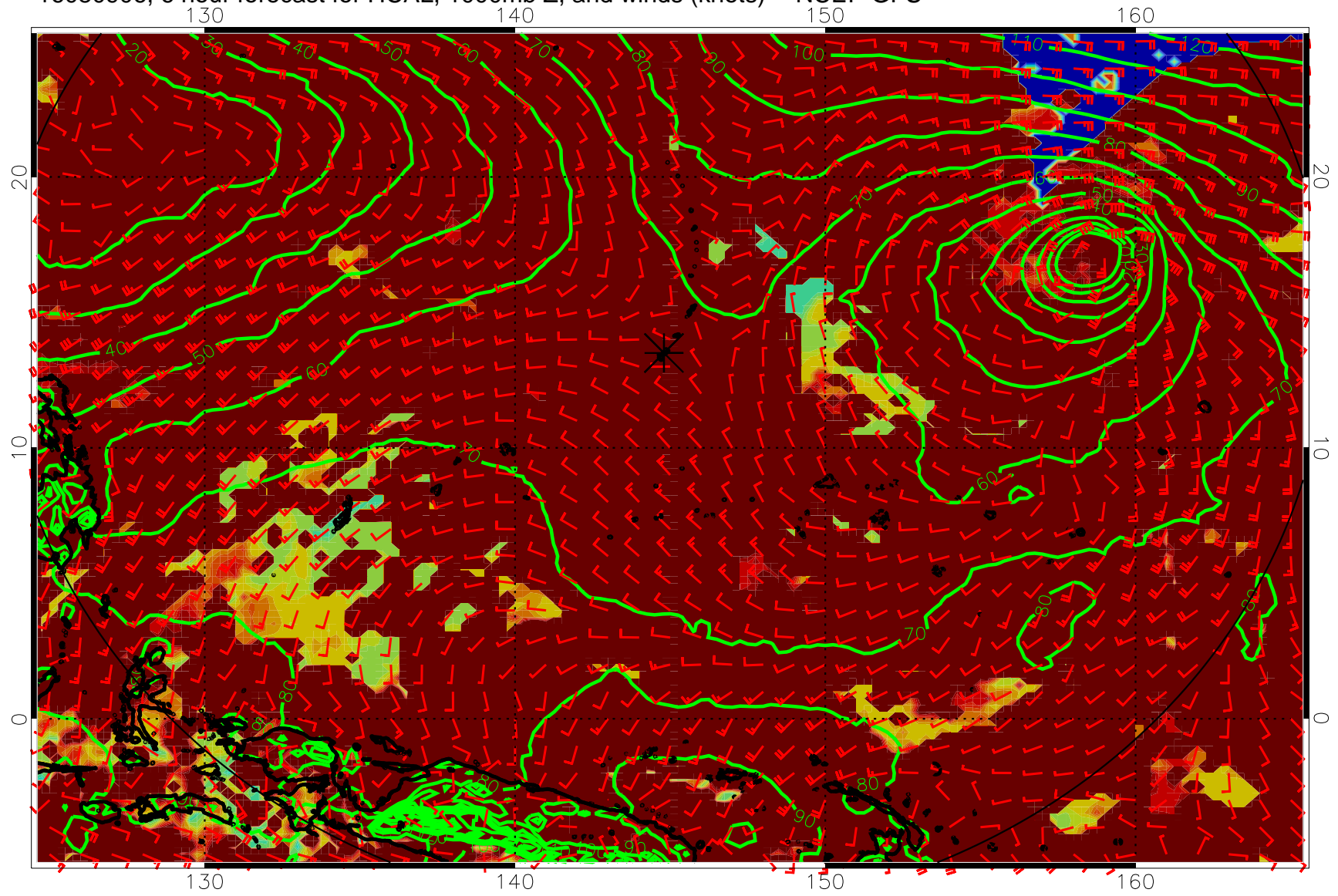
16080906, 6 hour forecast for HCAL, 1000mb Z, and winds (knots) -- NCEP GFS
