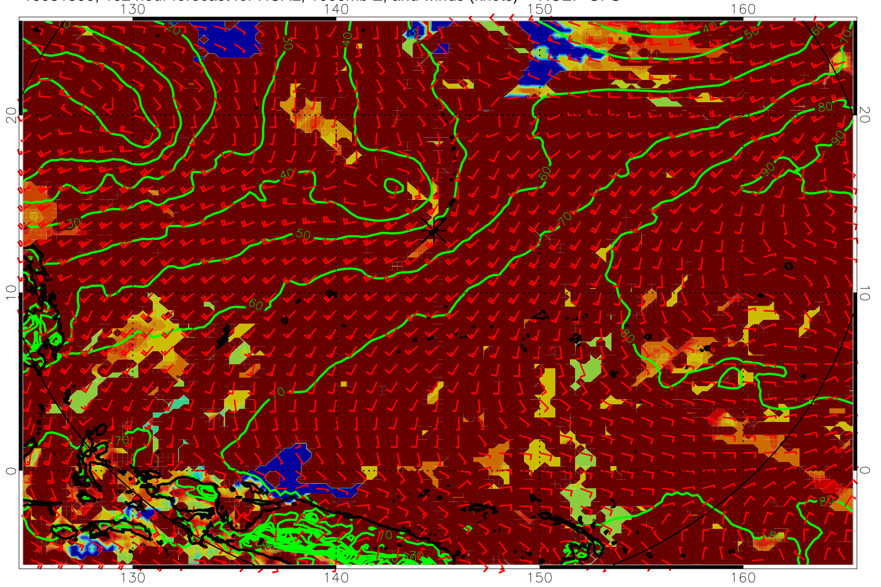
16081306, 102 hour forecast for HCAL, 1000mb Z, and winds (knots) -- NCEP GFS
