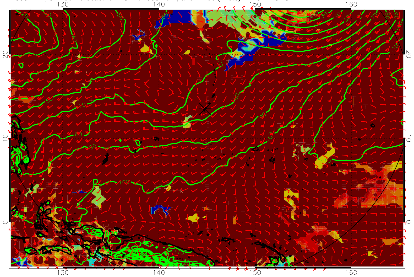
16081212, 84 hour forecast for HCAL, 1000mb Z, and winds (knots) -- NCEP GFS
