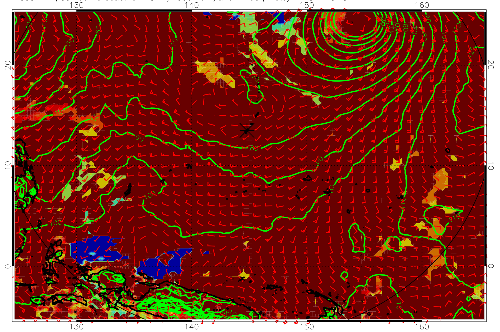
16081112, 60 hour forecast for HCAL, 1000mb Z, and winds (knots) -- NCEP GFS
