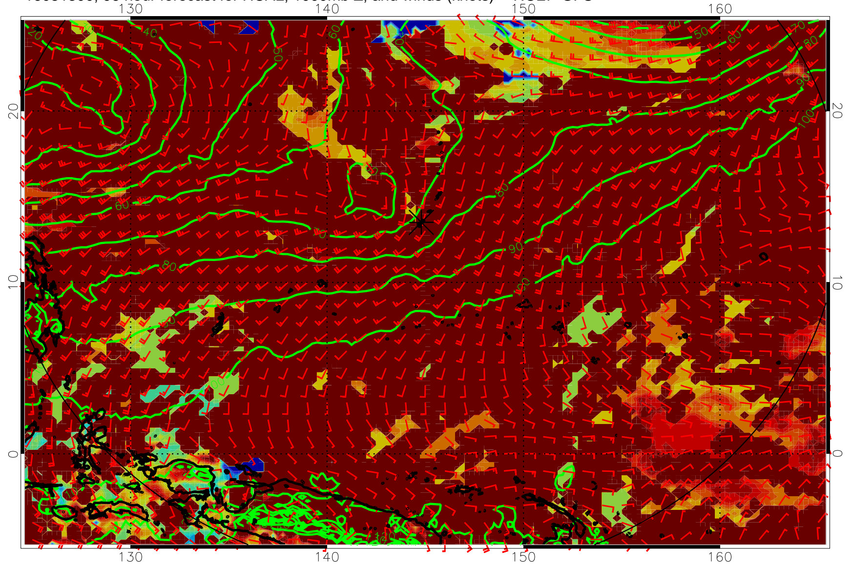
16081300, 96 hour forecast for HCAL, 1000mb Z, and winds (knots) -- NCEP GFS
