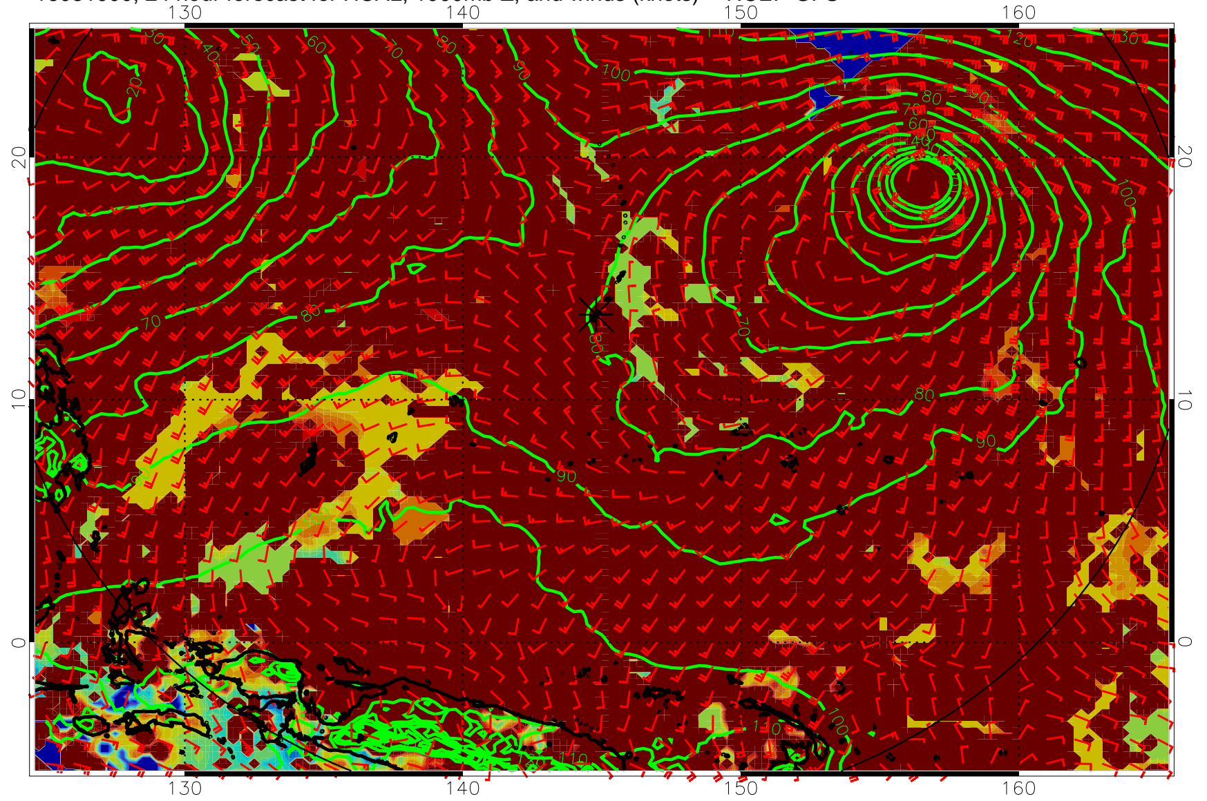
16081000, 24 hour forecast for HCAL, 1000mb Z, and winds (knots) -- NCEP GFS
