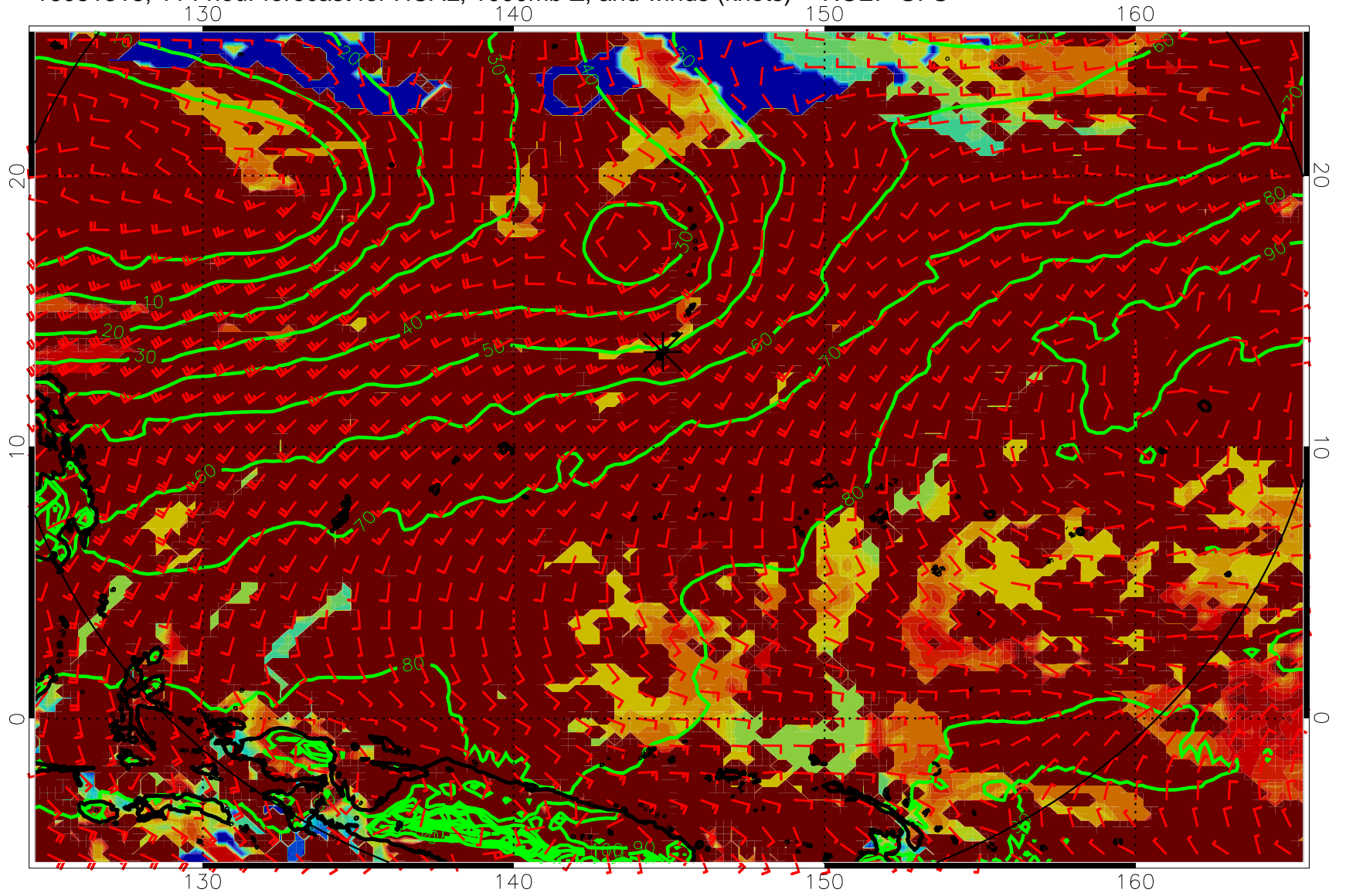
16081318, 114 hour forecast for HCAL, 1000mb Z, and winds (knots) -- NCEP GFS
