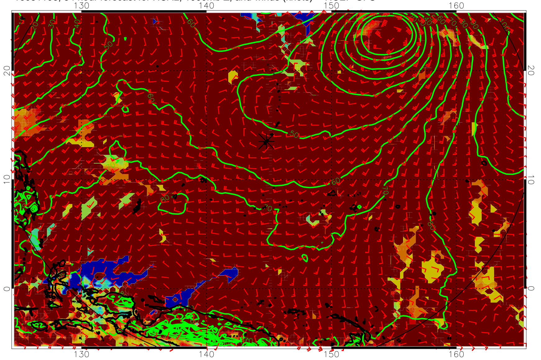
16081106, 54 hour forecast for HCAL, 1000mb Z, and winds (knots) -- NCEP GFS
