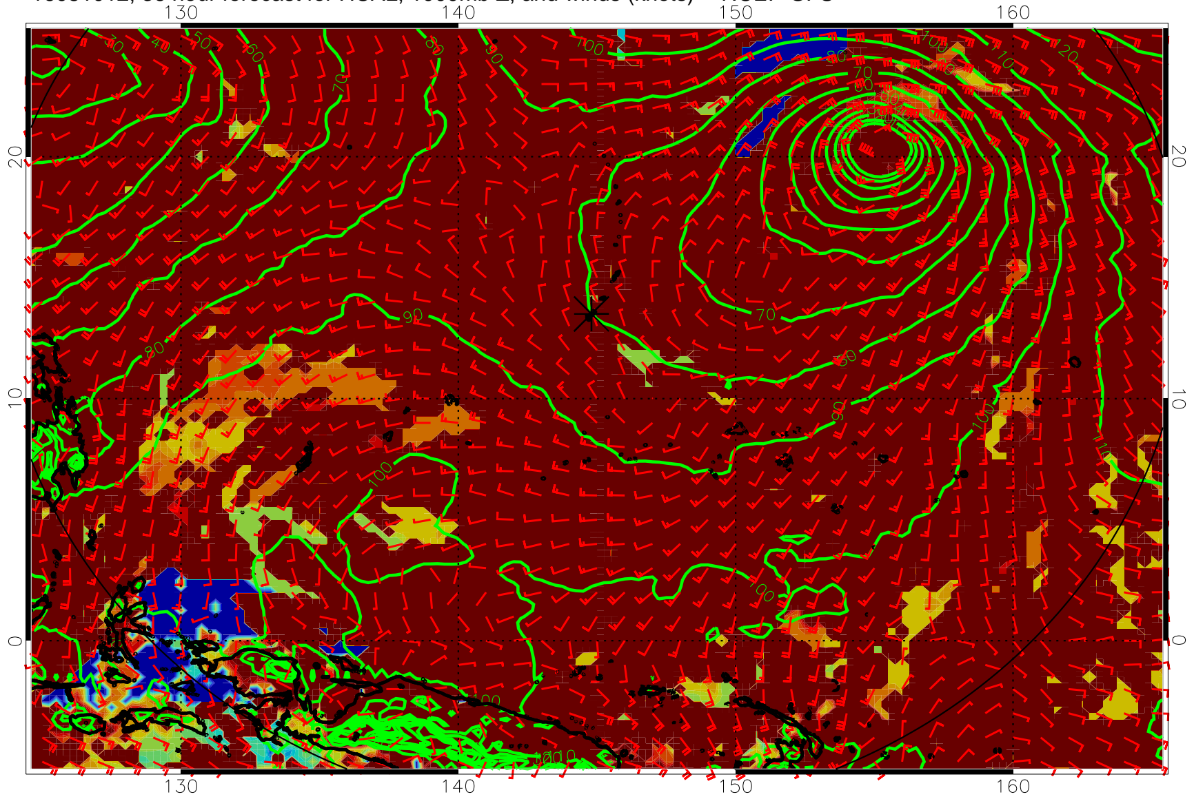
16081012, 36 hour forecast for HCAL, 1000mb Z, and winds (knots) -- NCEP GFS
