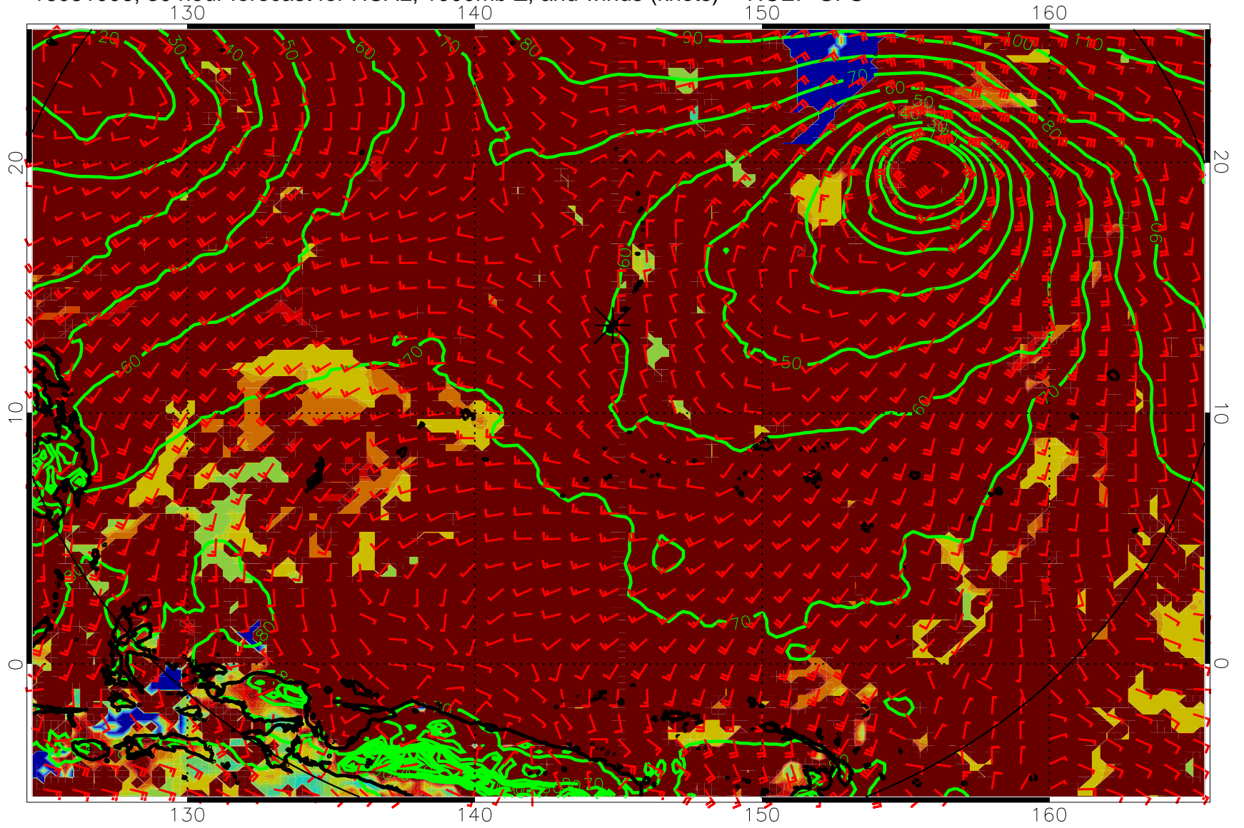
16081006, 30 hour forecast for HCAL, 1000mb Z, and winds (knots) -- NCEP GFS
