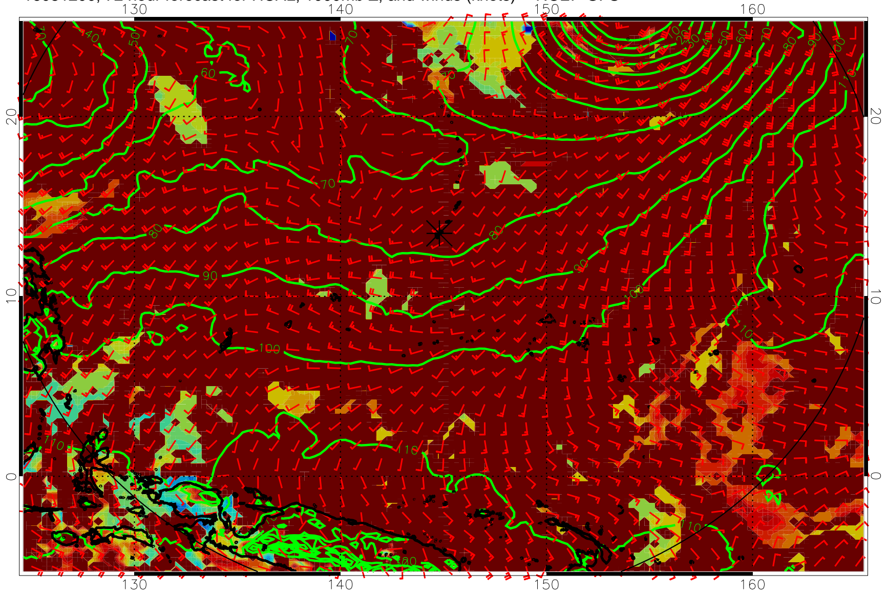
16081200, 72 hour forecast for HCAL, 1000mb Z, and winds (knots) -- NCEP GFS
