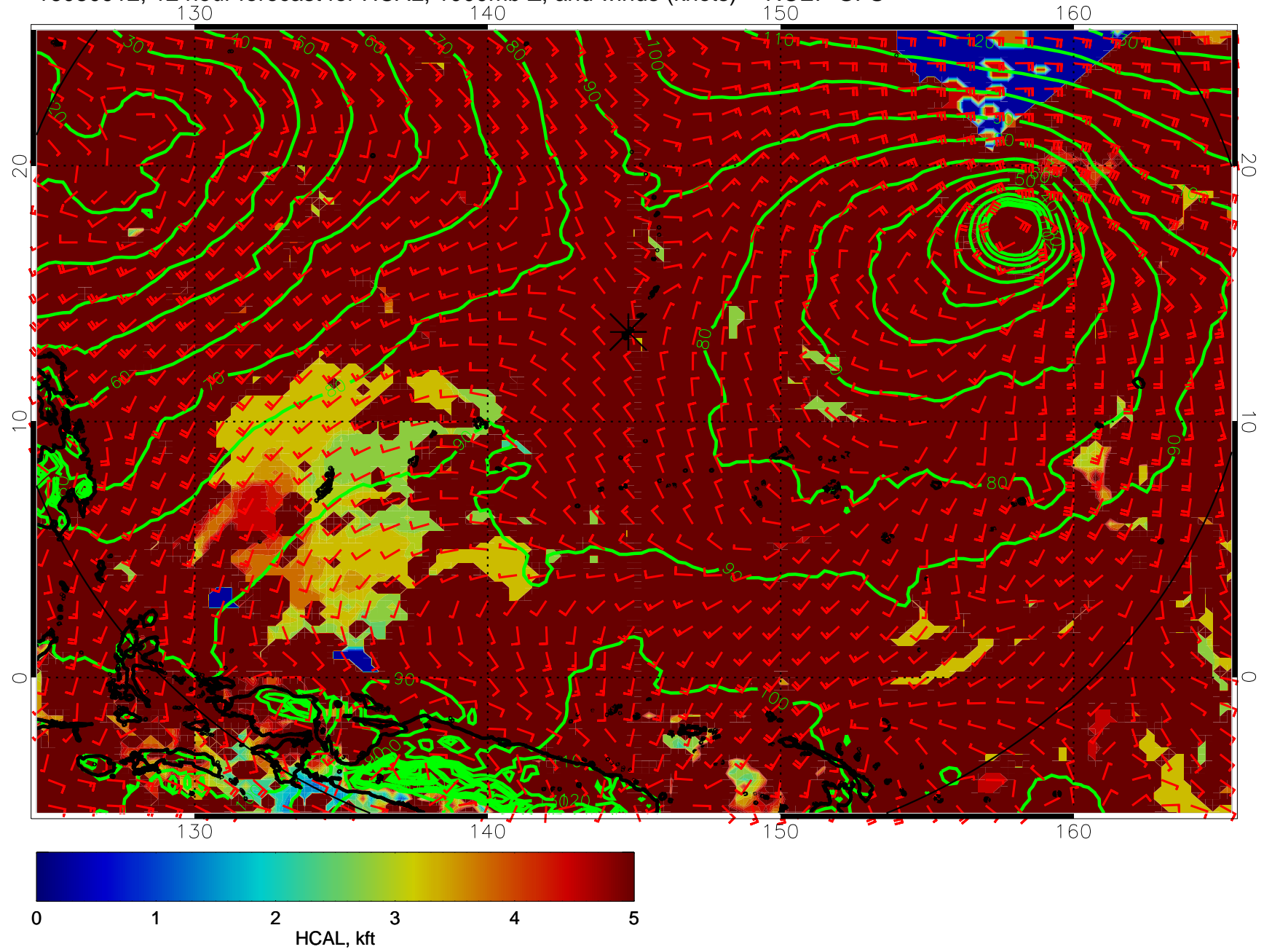
16080912, 12 hour forecast for HCAL, 1000mb Z, and winds (knots) -- NCEP GFS
