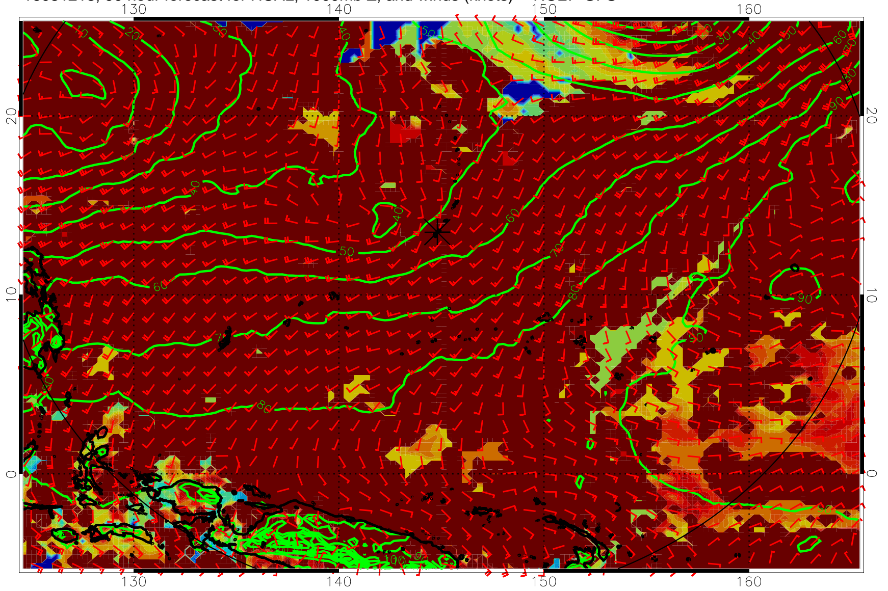
16081218, 90 hour forecast for HCAL, 1000mb Z, and winds (knots) -- NCEP GFS
