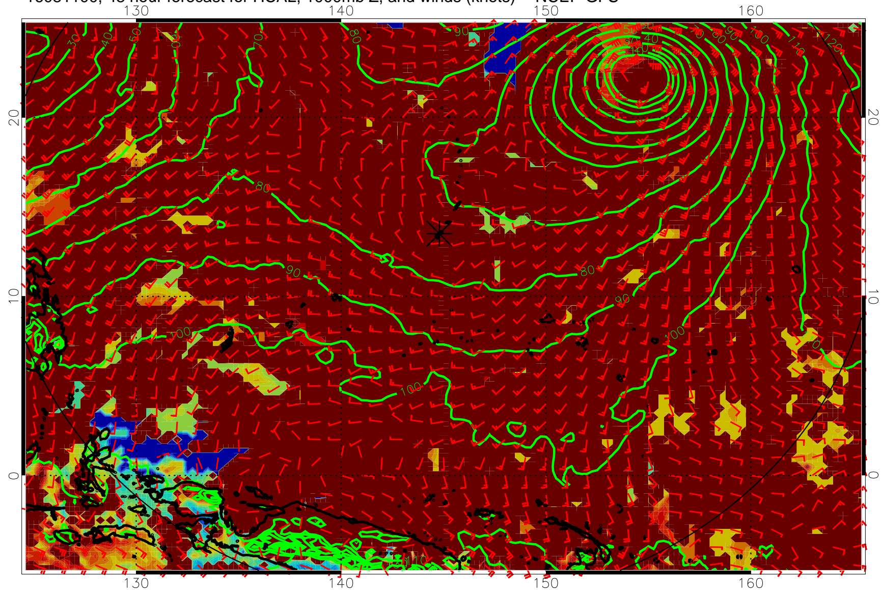
16081100, 48 hour forecast for HCAL, 1000mb Z, and winds (knots) -- NCEP GFS
