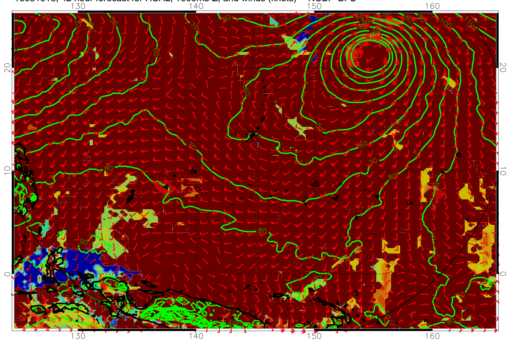
16081018, 42 hour forecast for HCAL, 1000mb Z, and winds (knots) -- NCEP GFS
