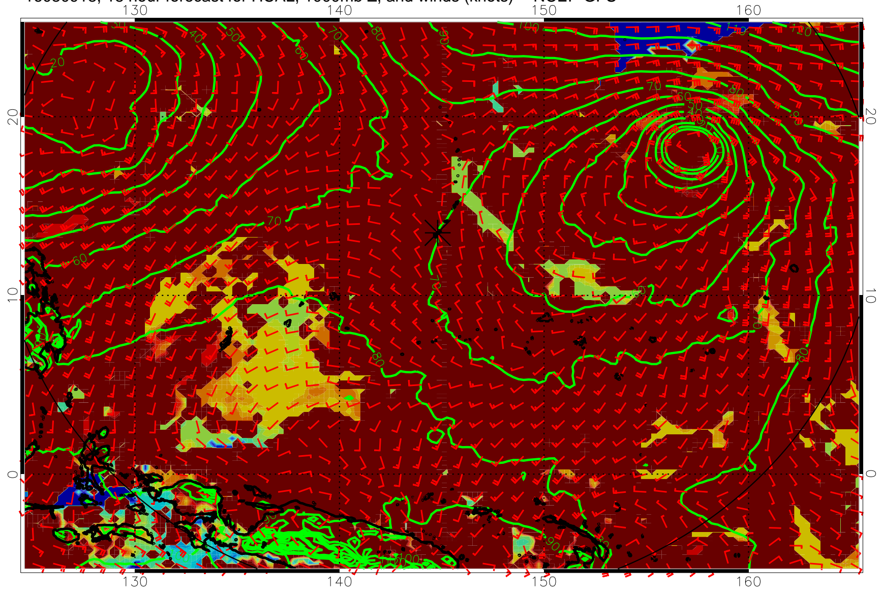
16080918, 18 hour forecast for HCAL, 1000mb Z, and winds (knots) -- NCEP GFS
