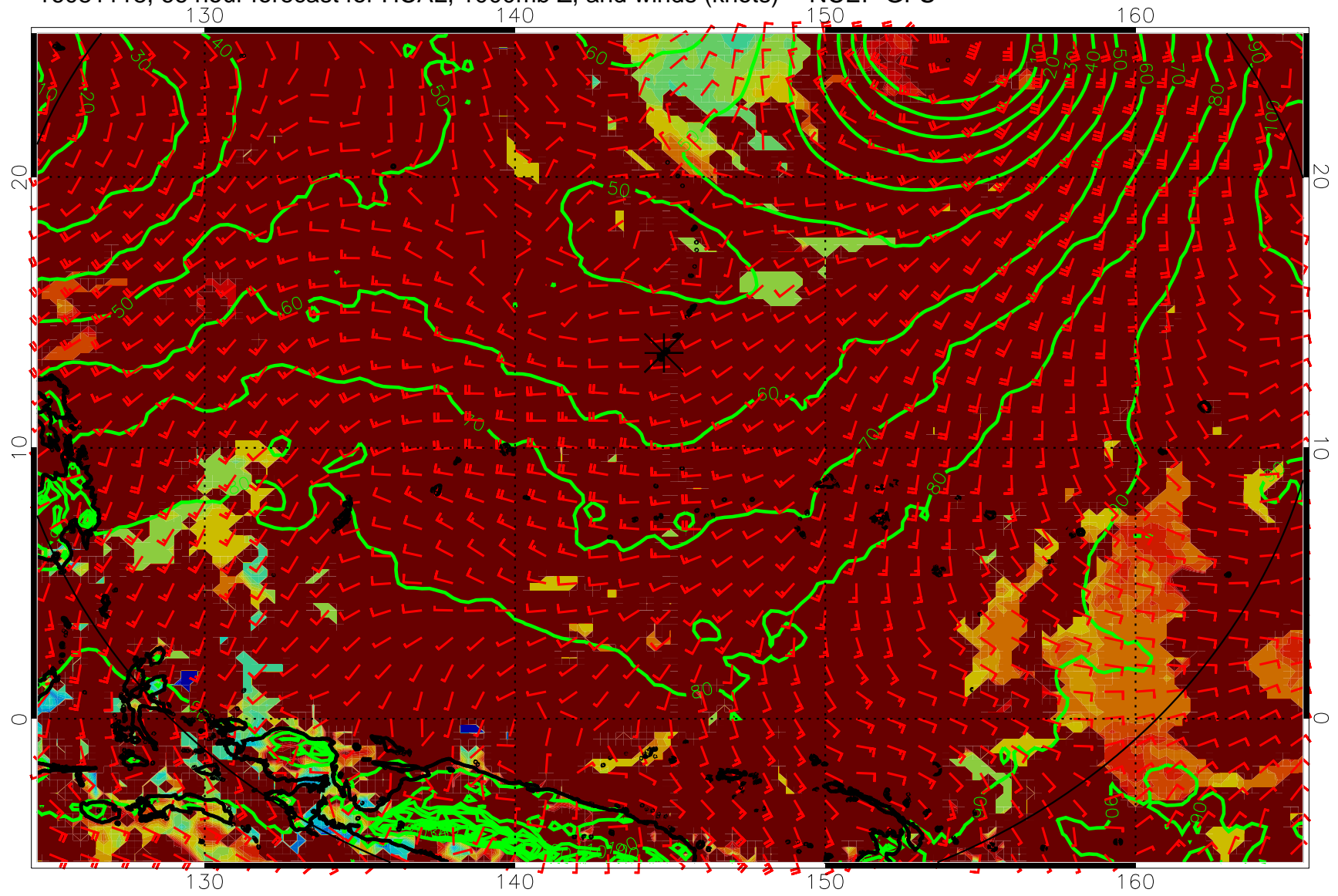
16081118, 66 hour forecast for HCAL, 1000mb Z, and winds (knots) -- NCEP GFS
