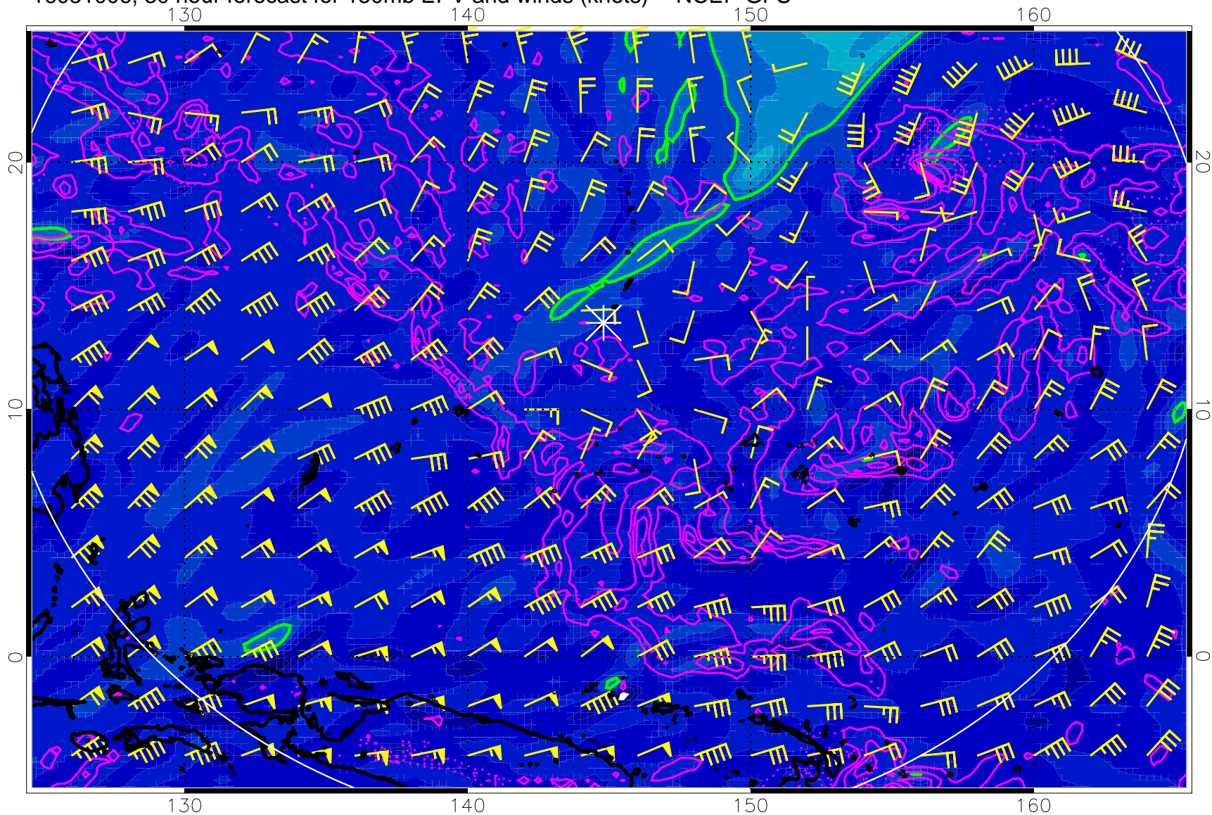
16081006, 30 hour forecast for 150mb EPV and winds (knots) -- NCEP GFS
