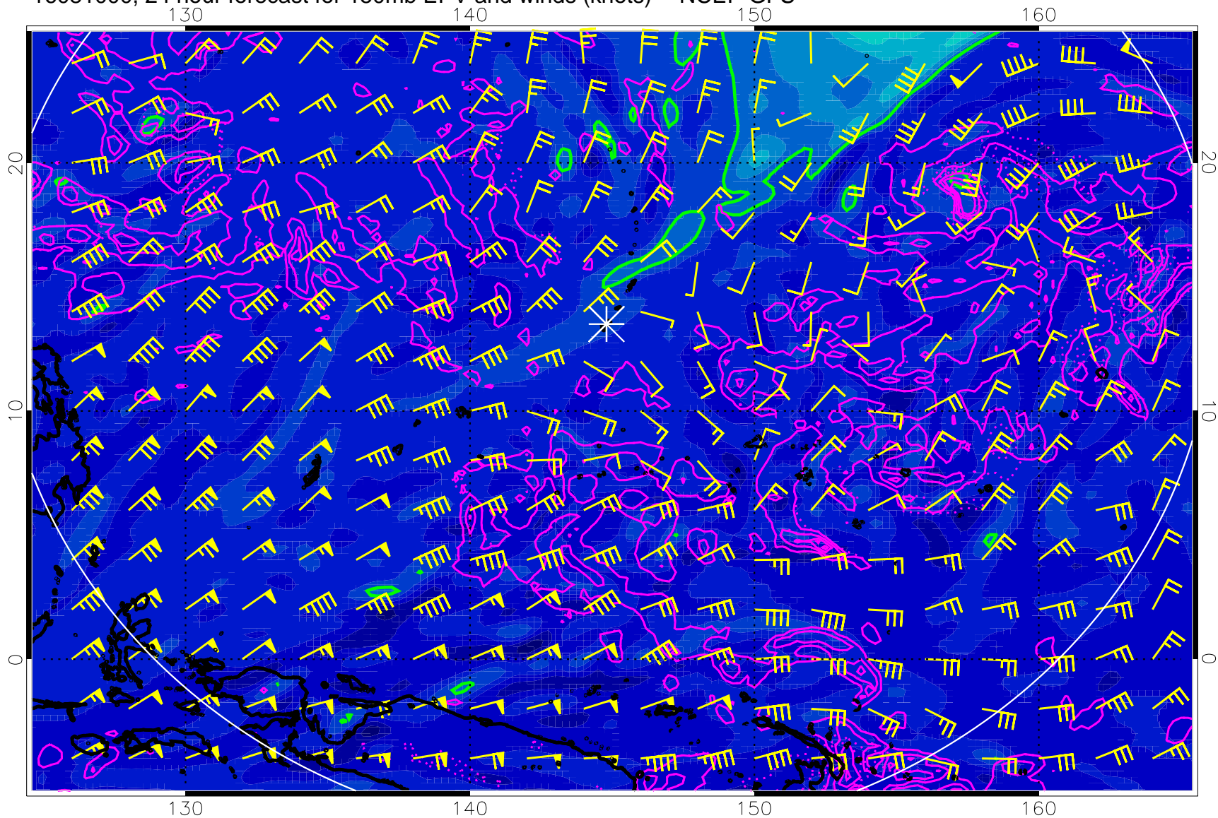
16081000, 24 hour forecast for 150mb EPV and winds (knots) -- NCEP GFS
