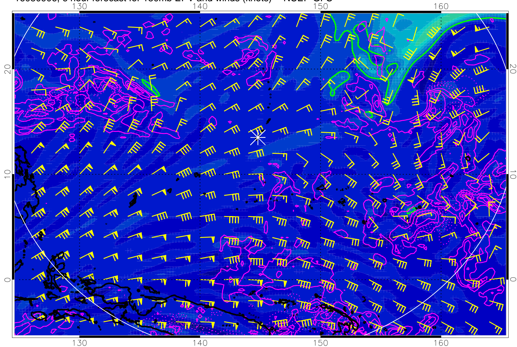
16080906, 6 hour forecast for 150mb EPV and winds (knots) -- NCEP GFS
