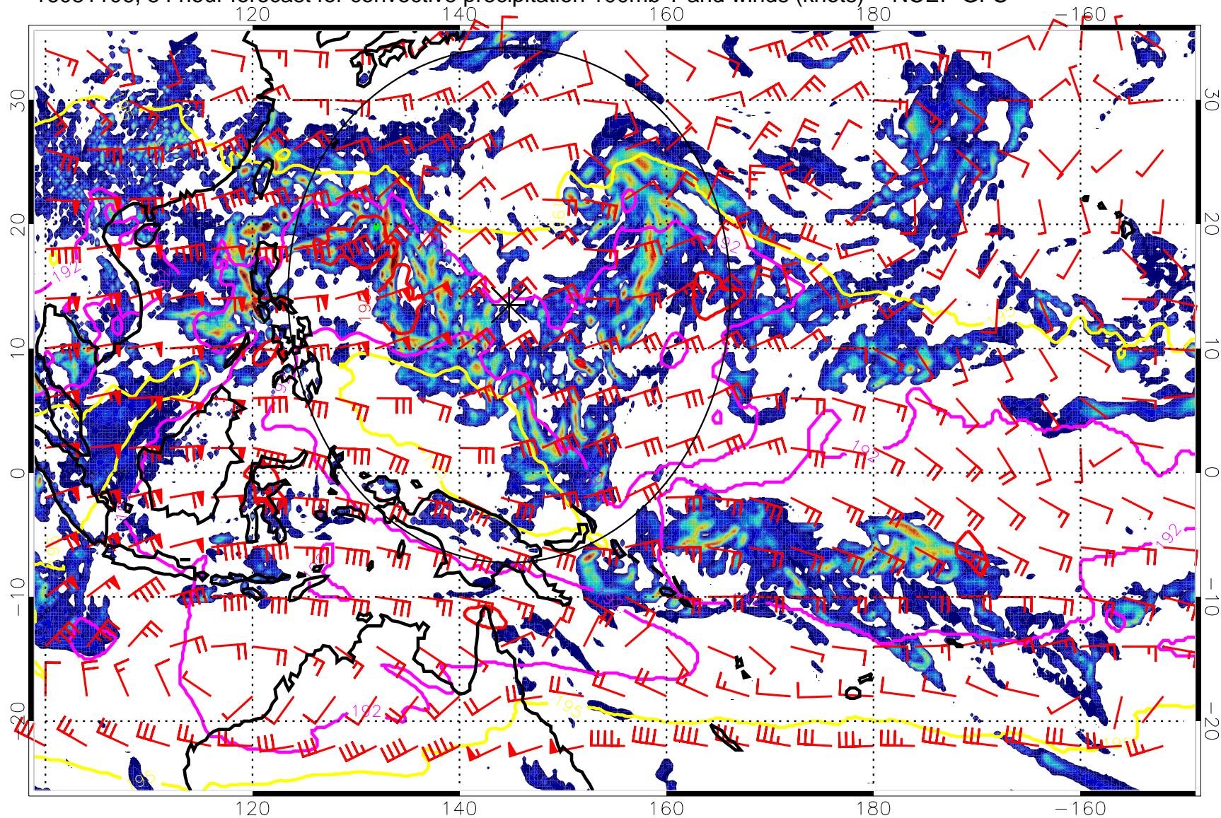
16081106, 54 hour forecast for convective precipitation 100mb T and winds (knots) -- NCEP GFS
