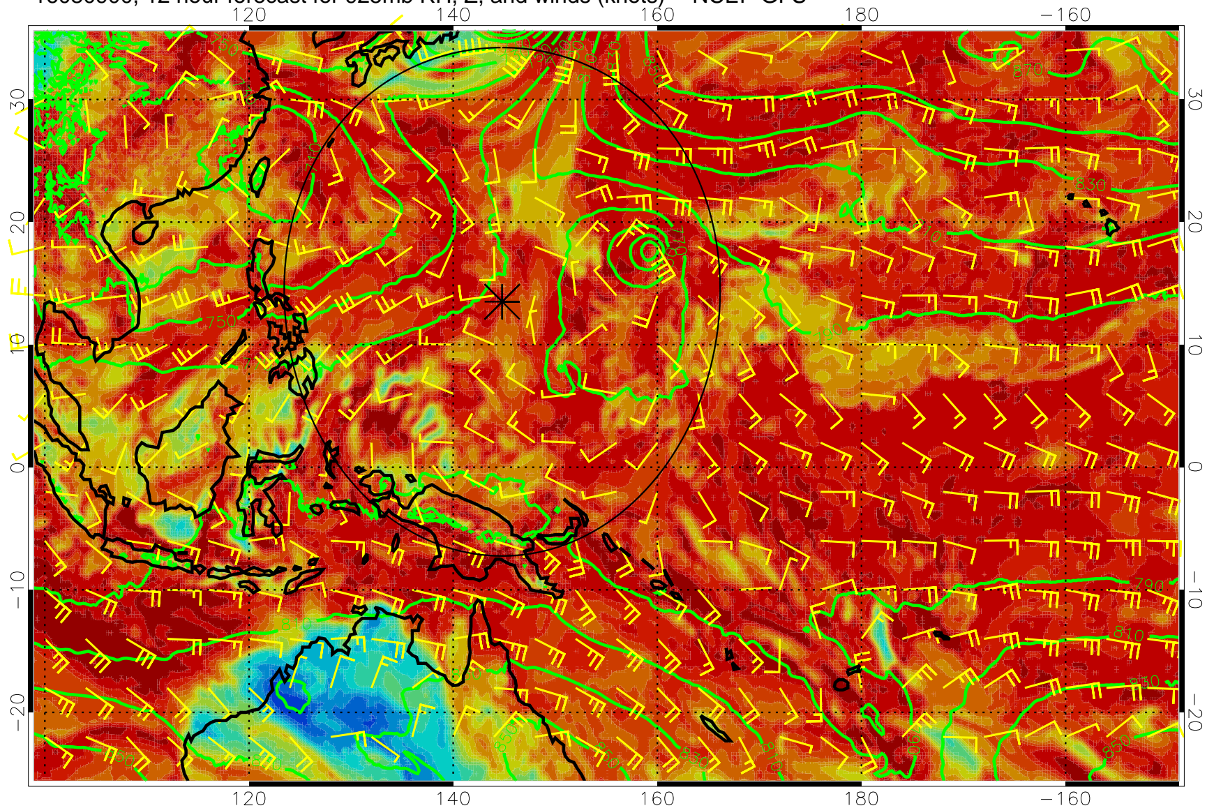
16080900, 12 hour forecast for 925mb RH, Z, and winds (knots) -- NCEP GFS
