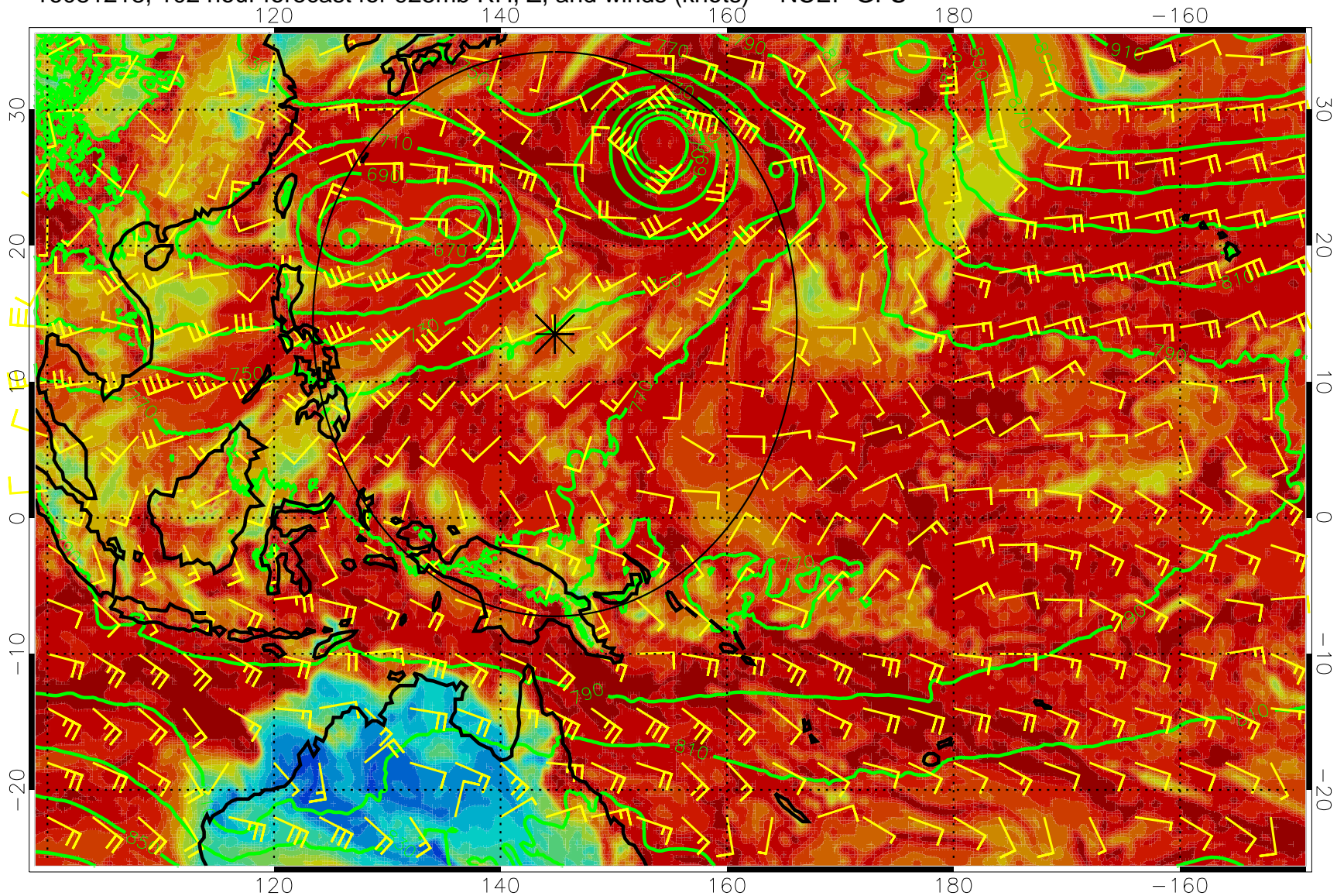
16081218, 102 hour forecast for 925mb RH, Z, and winds (knots) -- NCEP GFS
