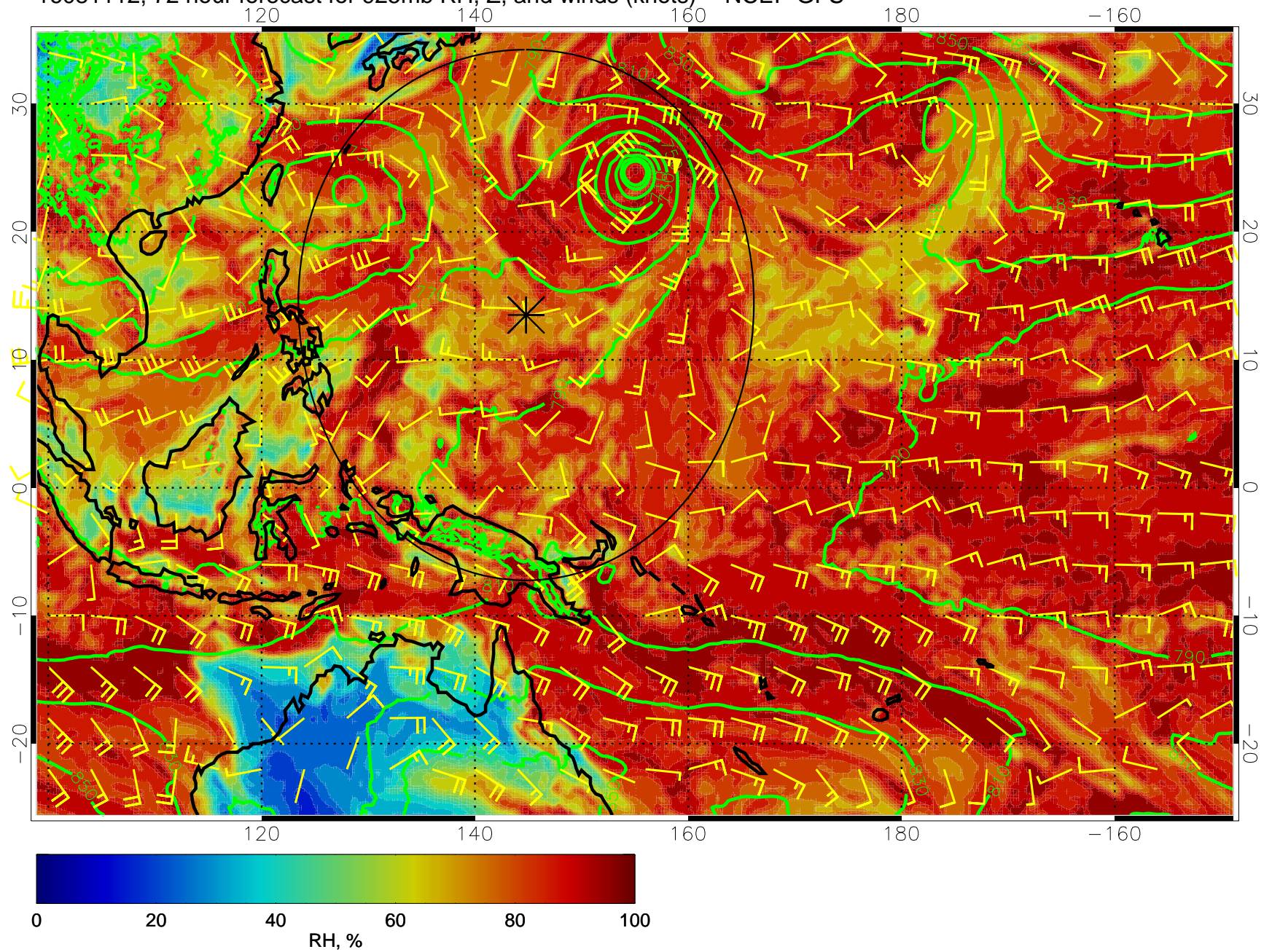
16081112, 72 hour forecast for 925mb RH, Z, and winds (knots) -- NCEP GFS
