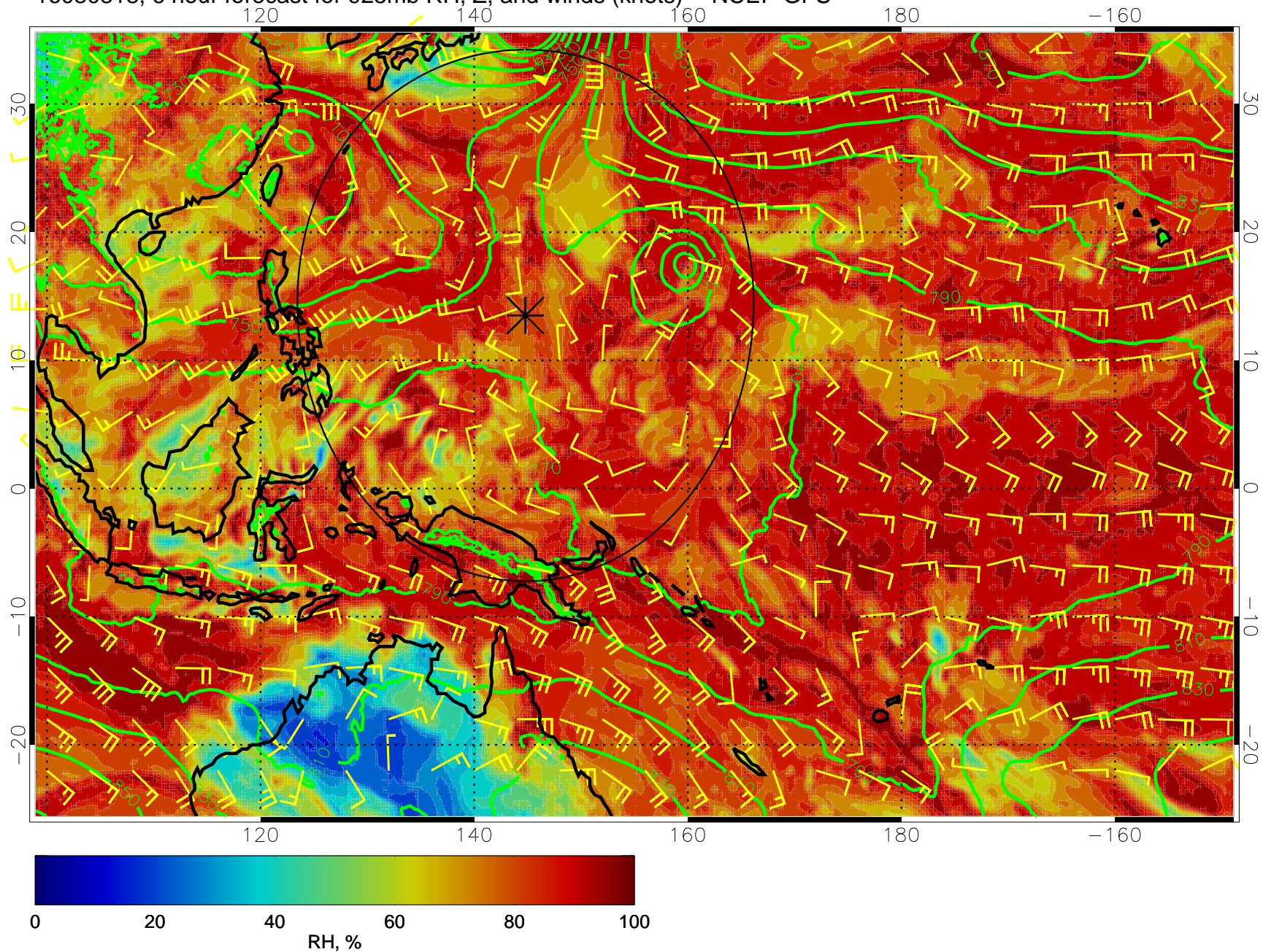
16080818, 6 hour forecast for 925mb RH, Z, and winds (knots) -- NCEP GFS
