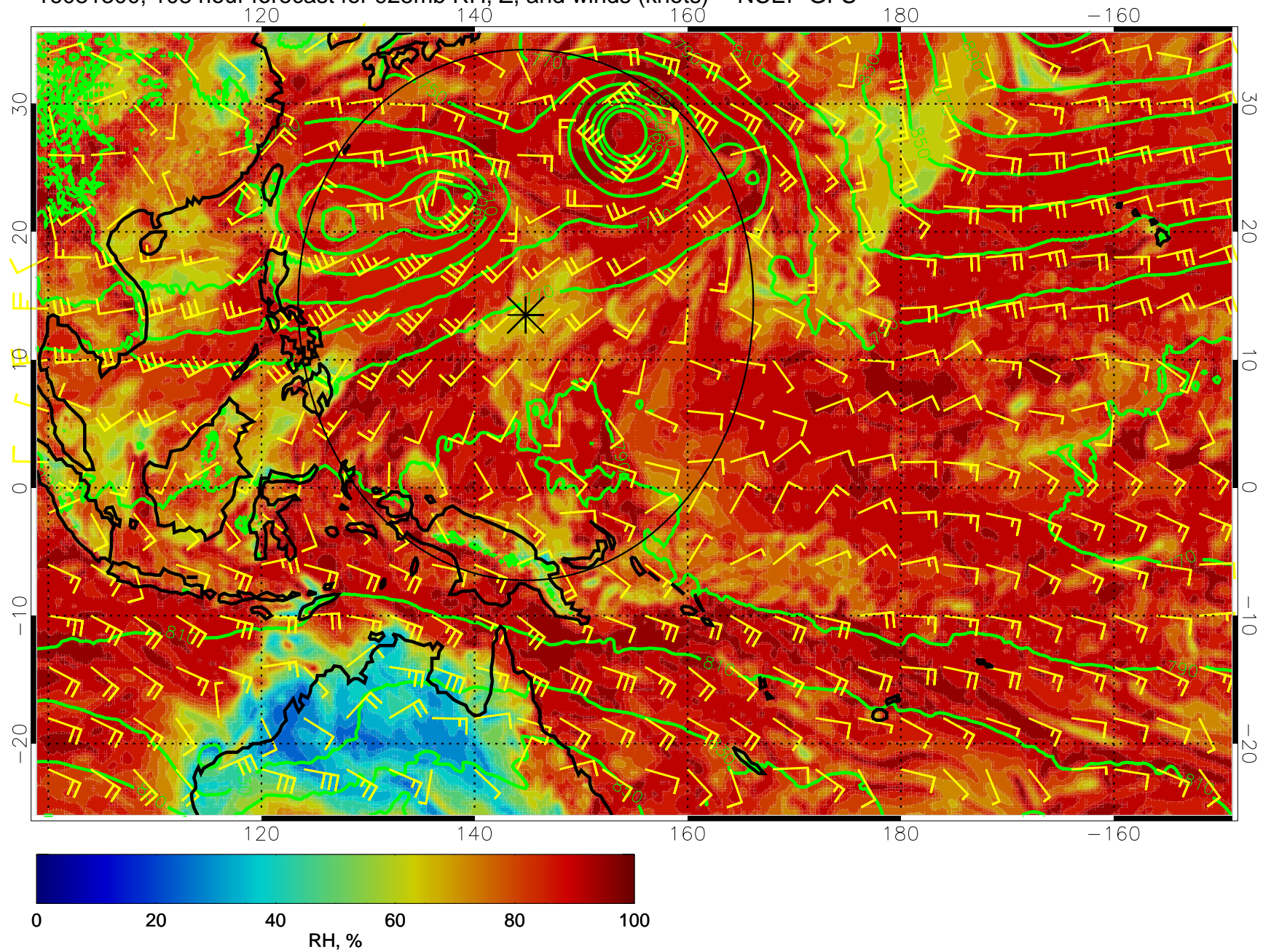
16081300, 108 hour forecast for 925mb RH, Z, and winds (knots) -- NCEP GFS
