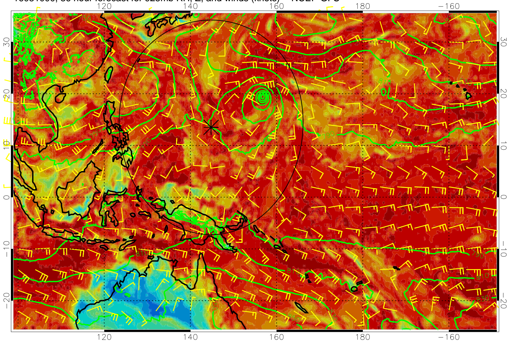
16081000, 36 hour forecast for 925mb RH, Z, and winds (knots) -- NCEP GFS
