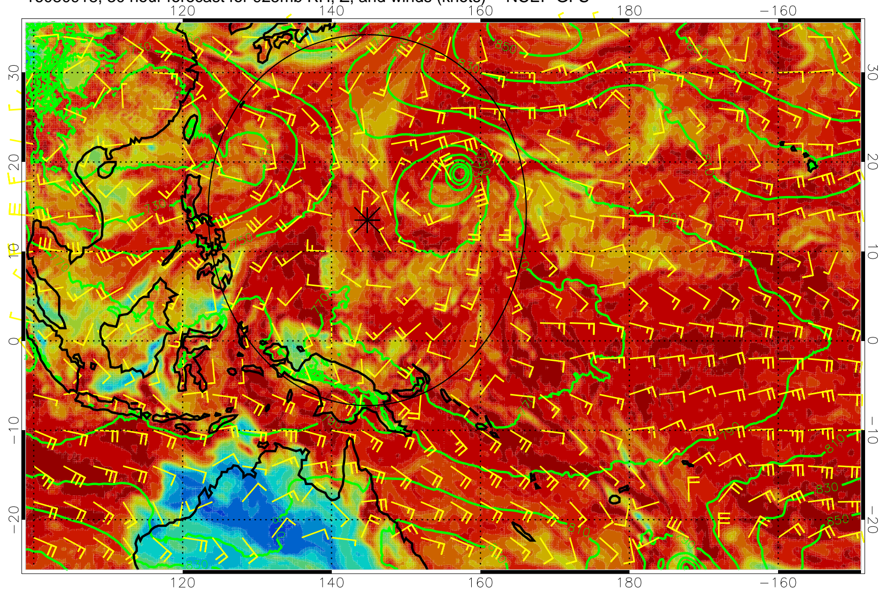
16080918, 30 hour forecast for 925mb RH, Z, and winds (knots) -- NCEP GFS
