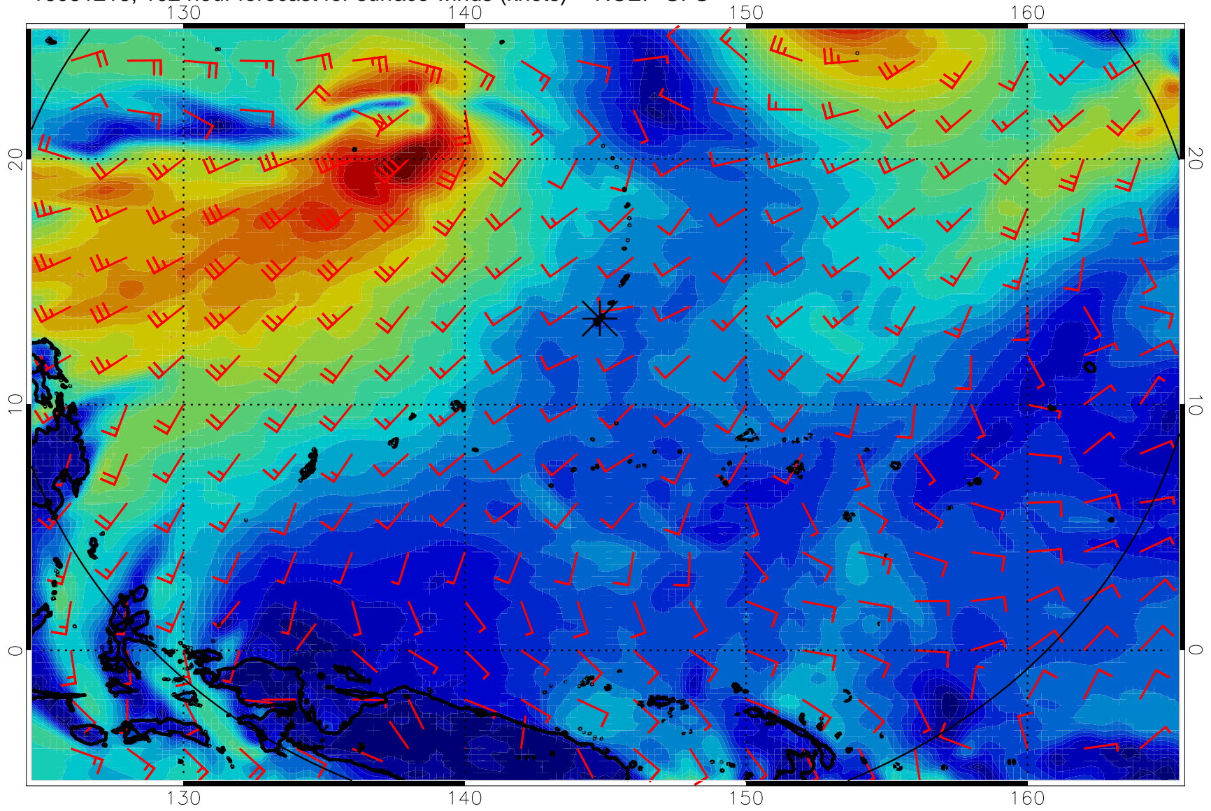
16081218, 102 hour forecast for surface winds (knots) -- NCEP GFS
