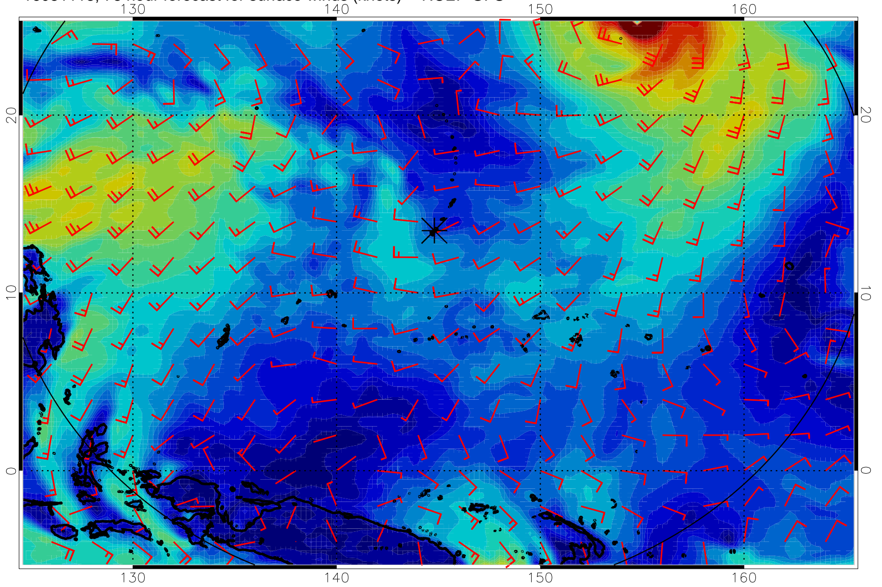
16081118, 78 hour forecast for surface winds (knots) -- NCEP GFS
