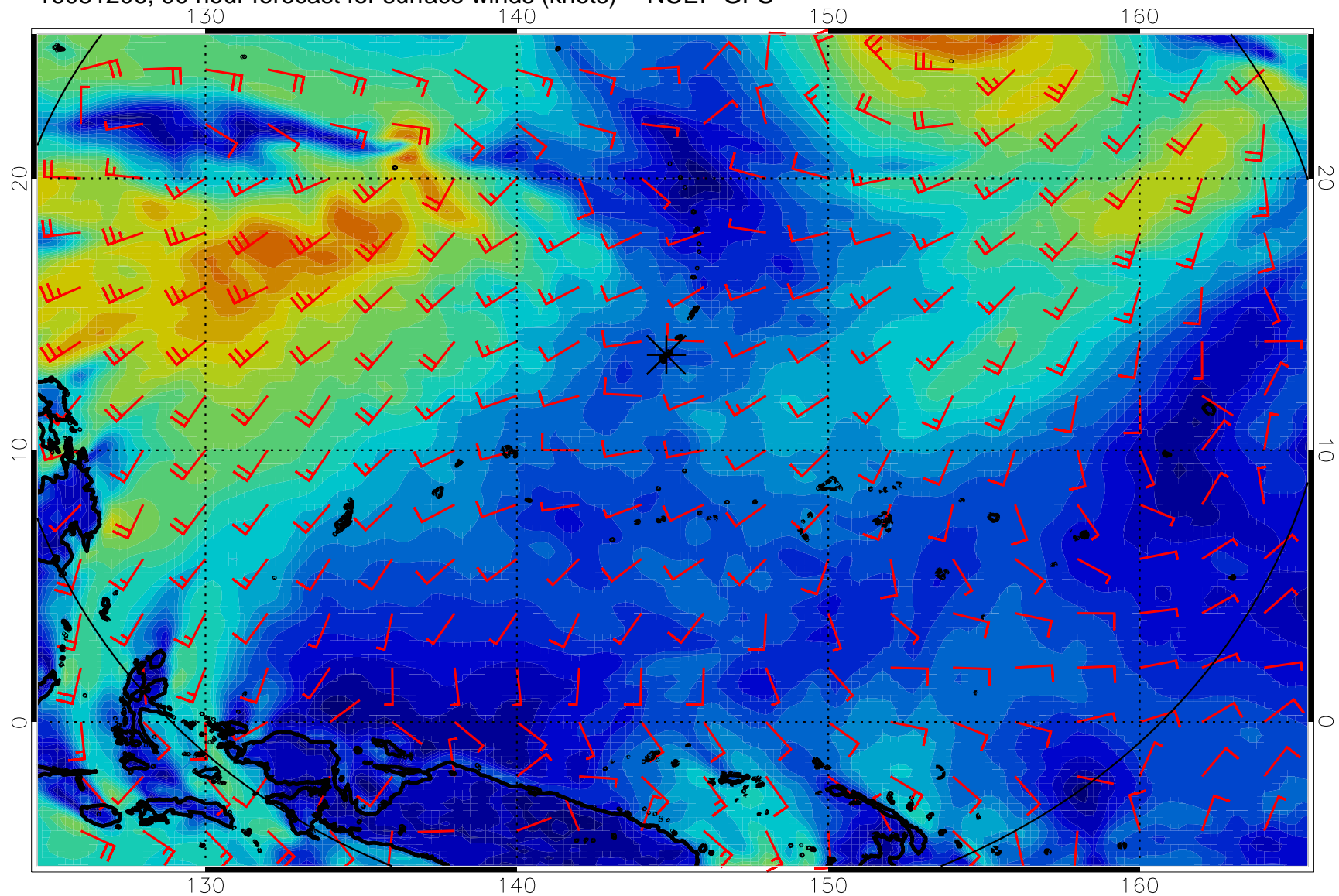
16081206, 90 hour forecast for surface winds (knots) -- NCEP GFS
