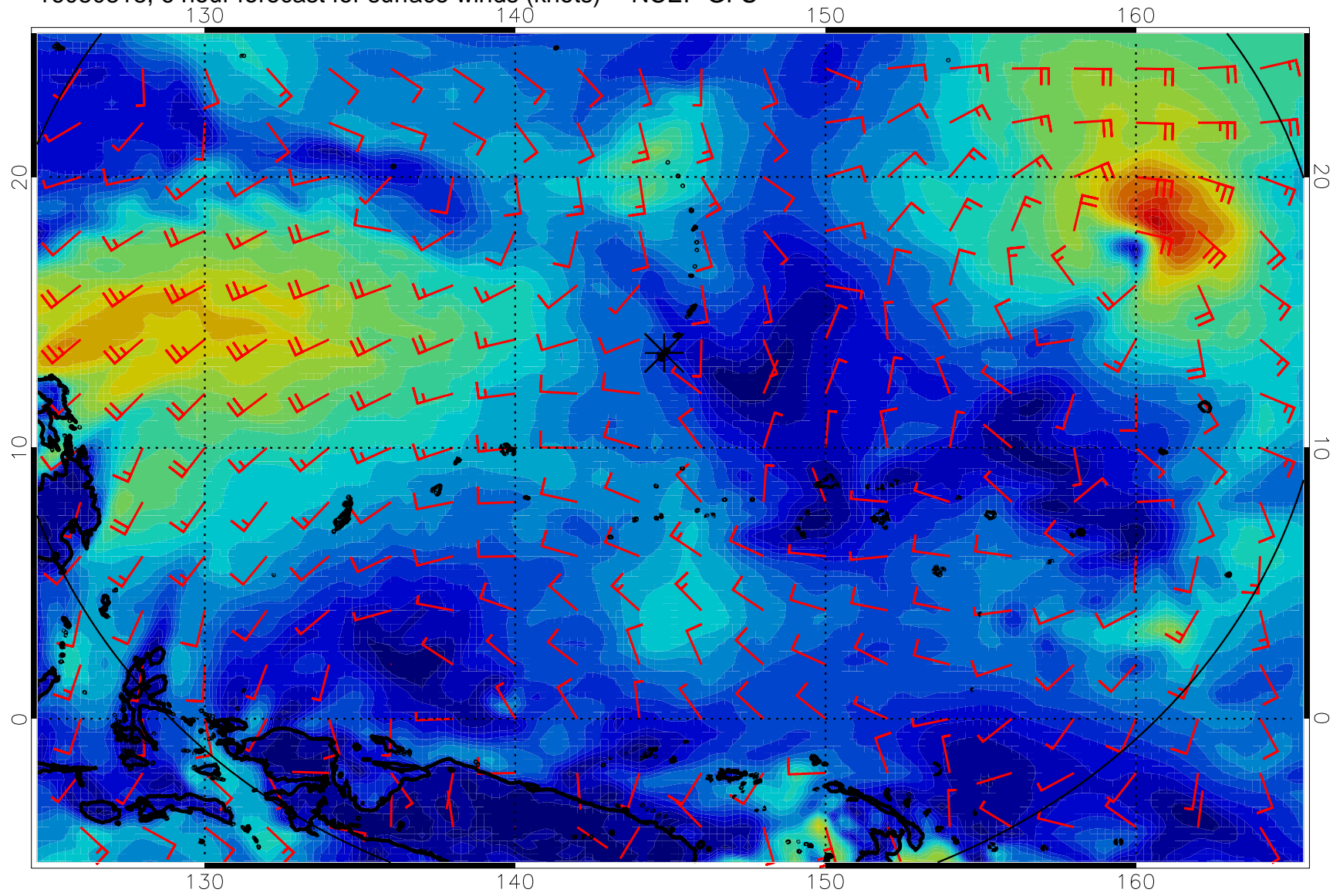
16080818, 6 hour forecast for surface winds (knots) -- NCEP GFS
