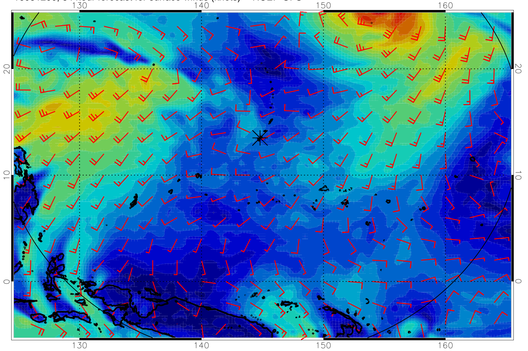
16081200, 84 hour forecast for surface winds (knots) -- NCEP GFS
