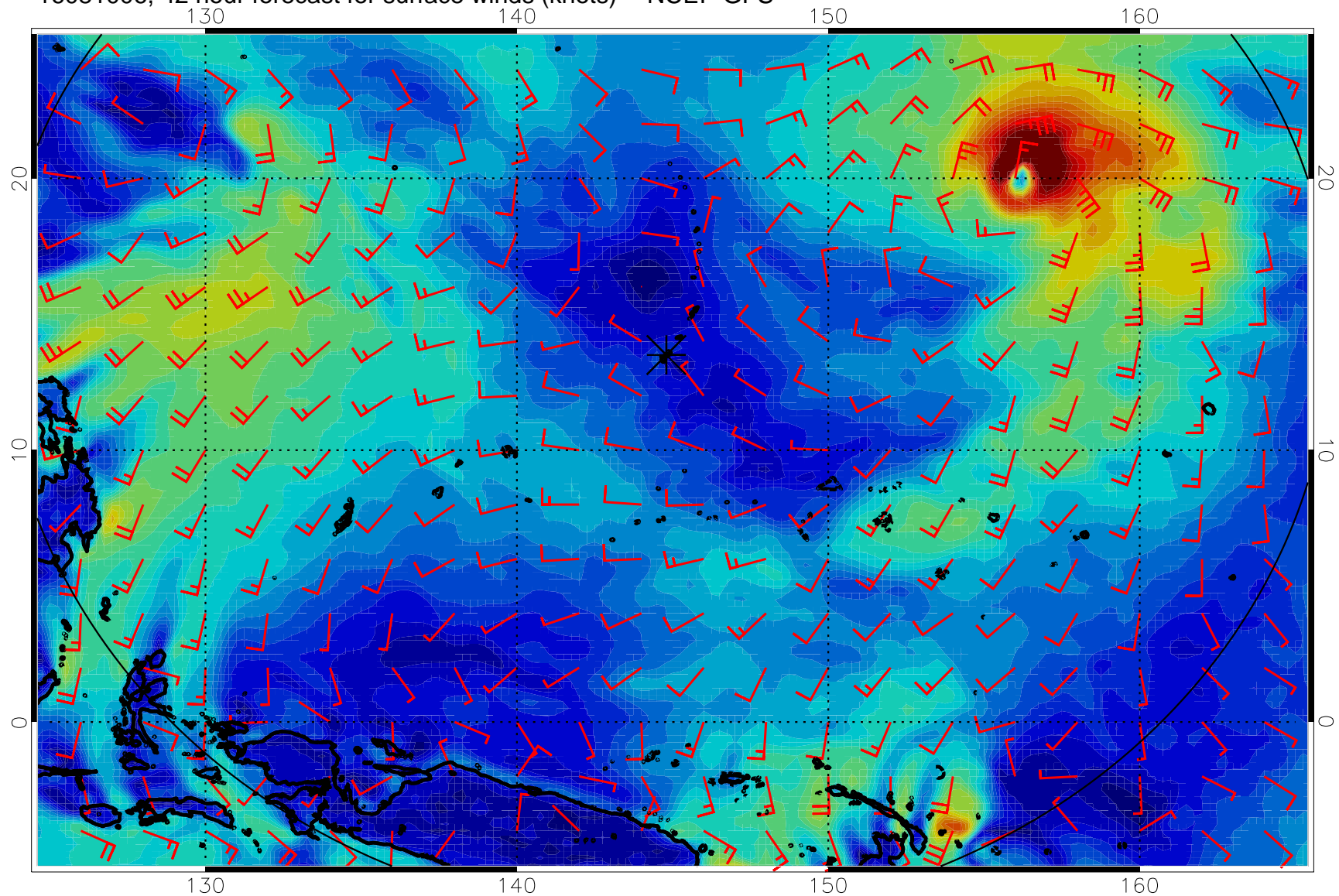
16081006, 42 hour forecast for surface winds (knots) -- NCEP GFS
