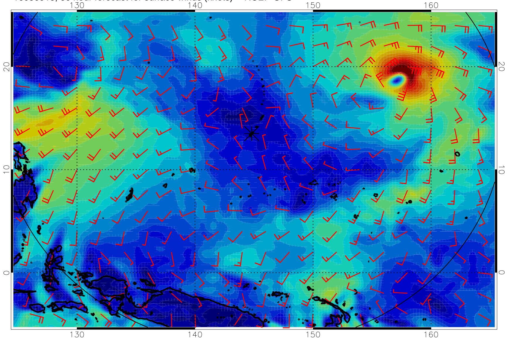
16080918, 30 hour forecast for surface winds (knots) -- NCEP GFS
