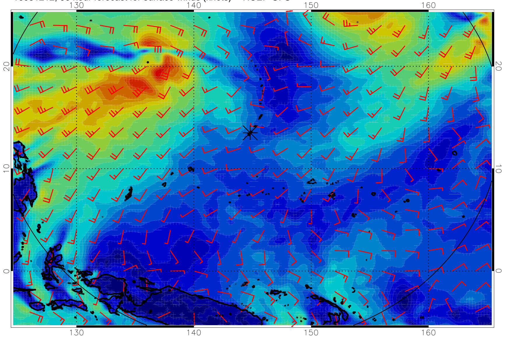
16081212, 96 hour forecast for surface winds (knots) -- NCEP GFS
