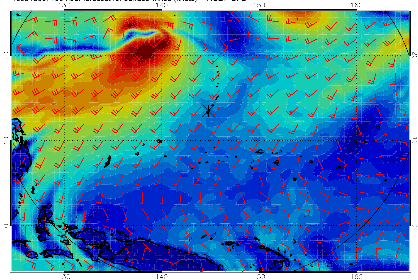
16081300, 108 hour forecast for surface winds (knots) -- NCEP GFS
