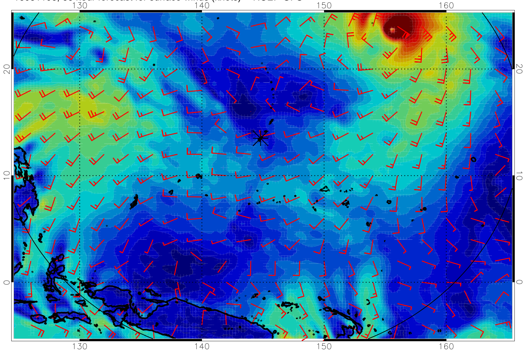
16081106, 66 hour forecast for surface winds (knots) -- NCEP GFS
