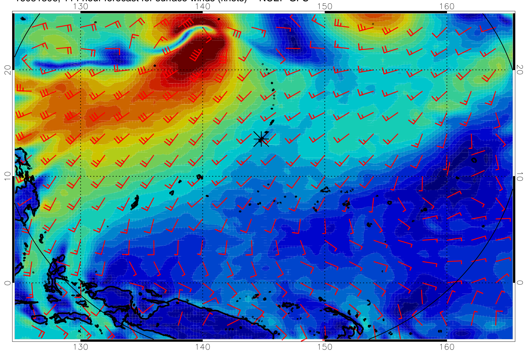
16081306, 114 hour forecast for surface winds (knots) -- NCEP GFS
