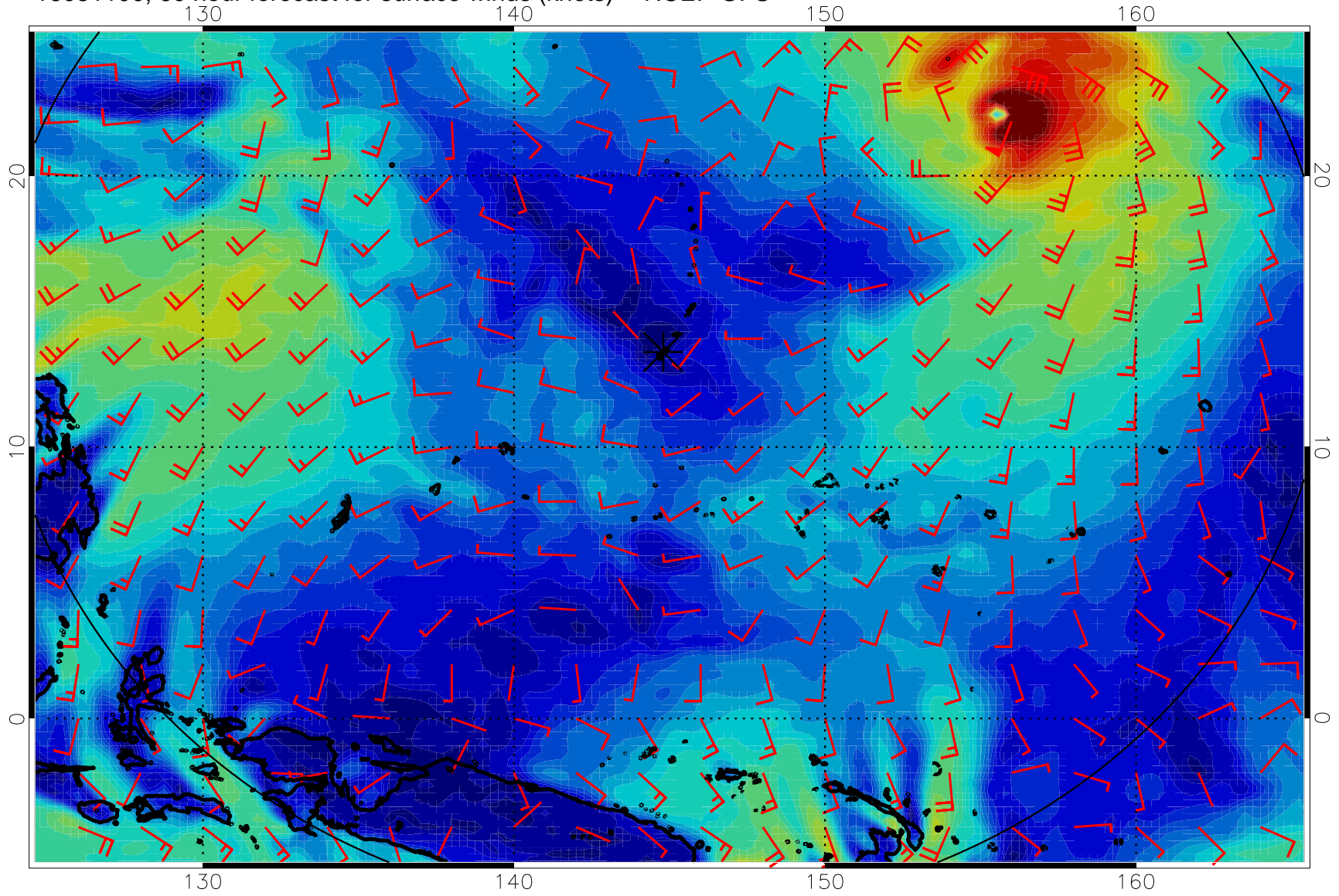
16081100, 60 hour forecast for surface winds (knots) -- NCEP GFS
