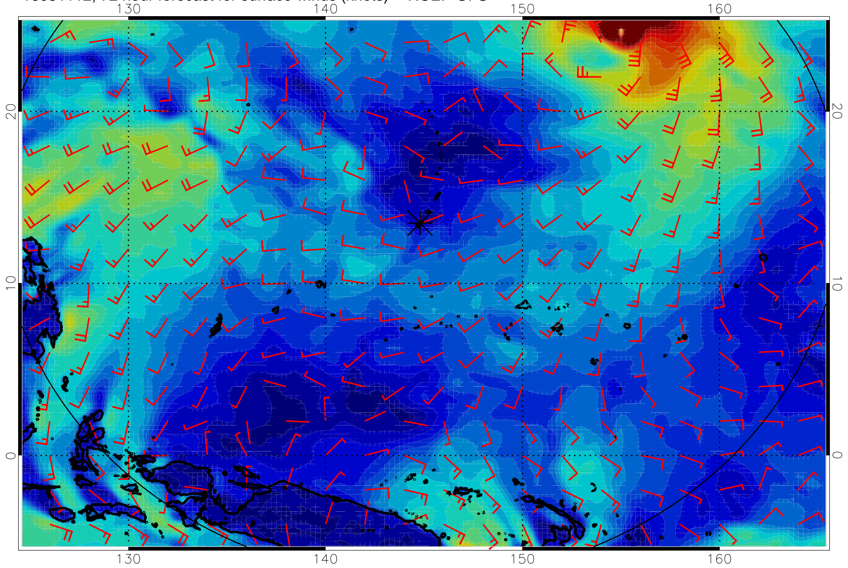
16081112, 72 hour forecast for surface winds (knots) -- NCEP GFS
