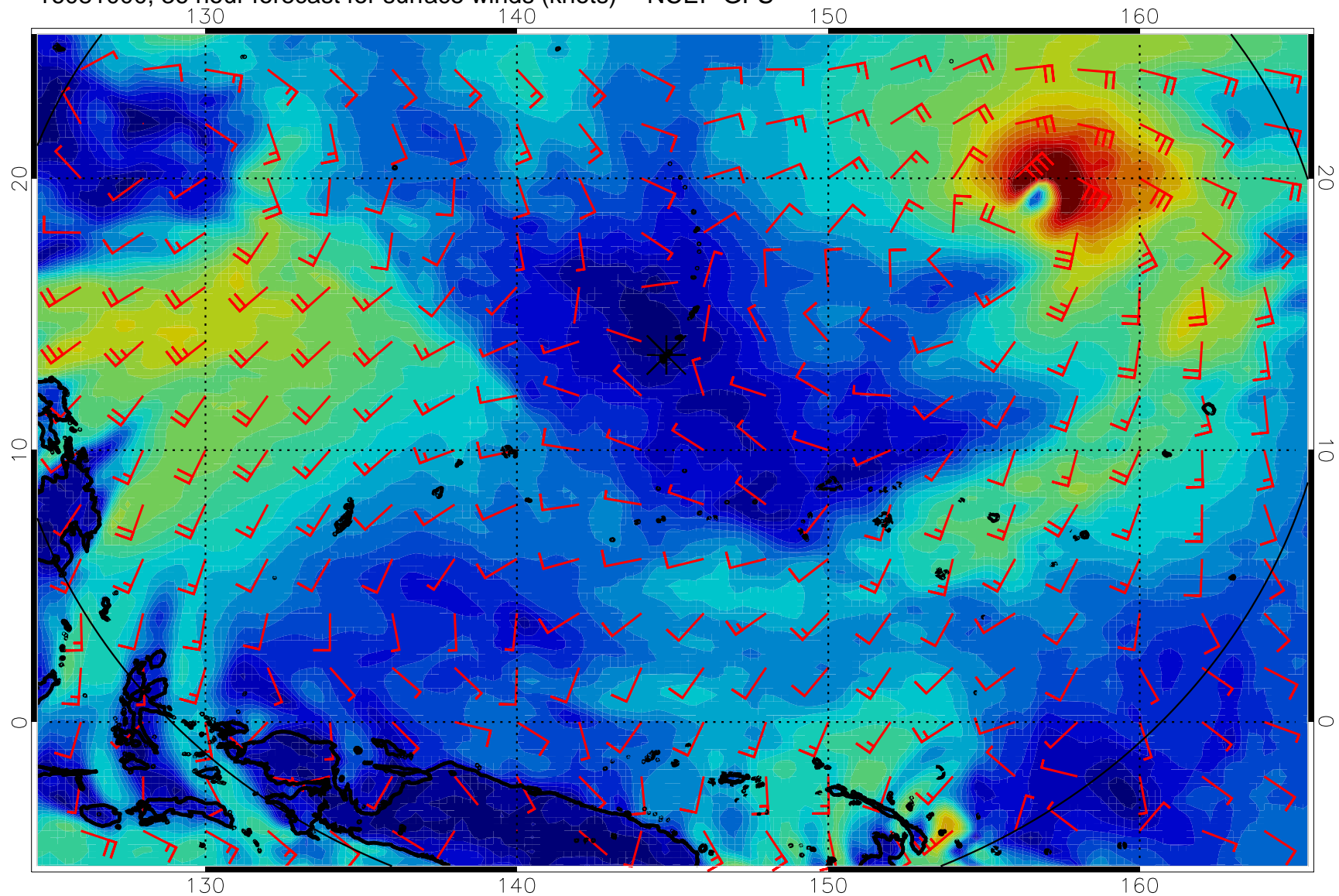
16081000, 36 hour forecast for surface winds (knots) -- NCEP GFS
