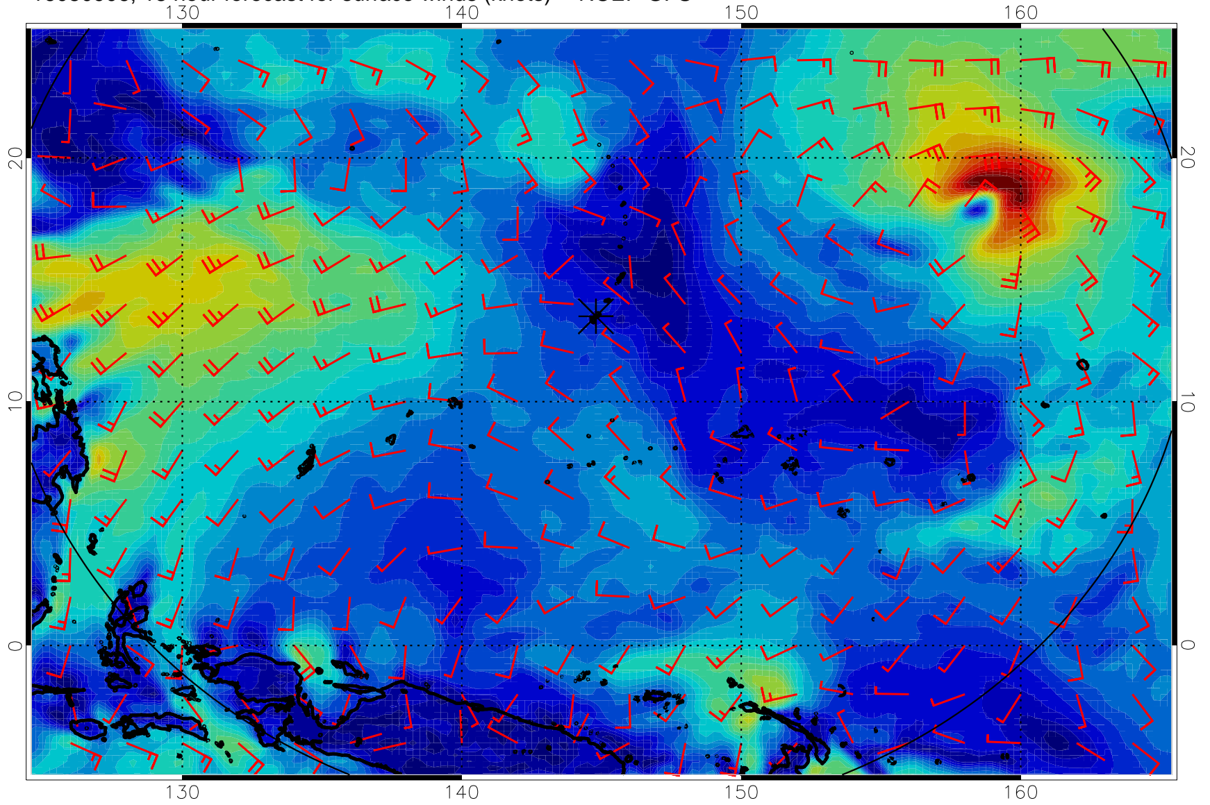
16080906, 18 hour forecast for surface winds (knots) -- NCEP GFS
