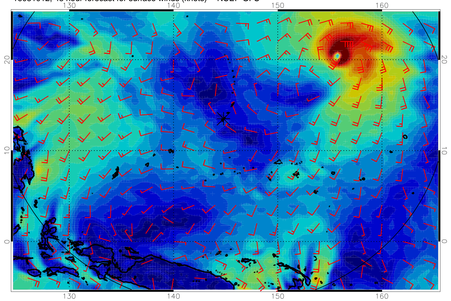
16081012, 48 hour forecast for surface winds (knots) -- NCEP GFS
