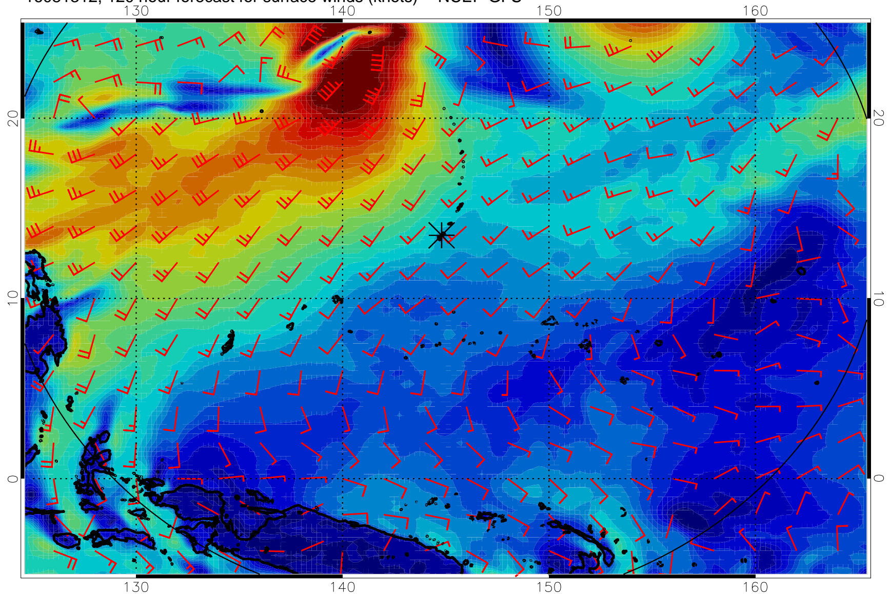
16081312, 120 hour forecast for surface winds (knots) -- NCEP GFS
