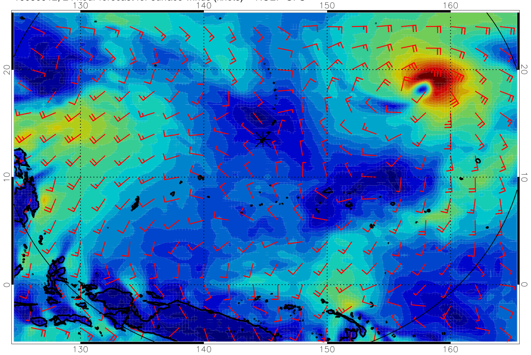
16080912, 24 hour forecast for surface winds (knots) -- NCEP GFS
