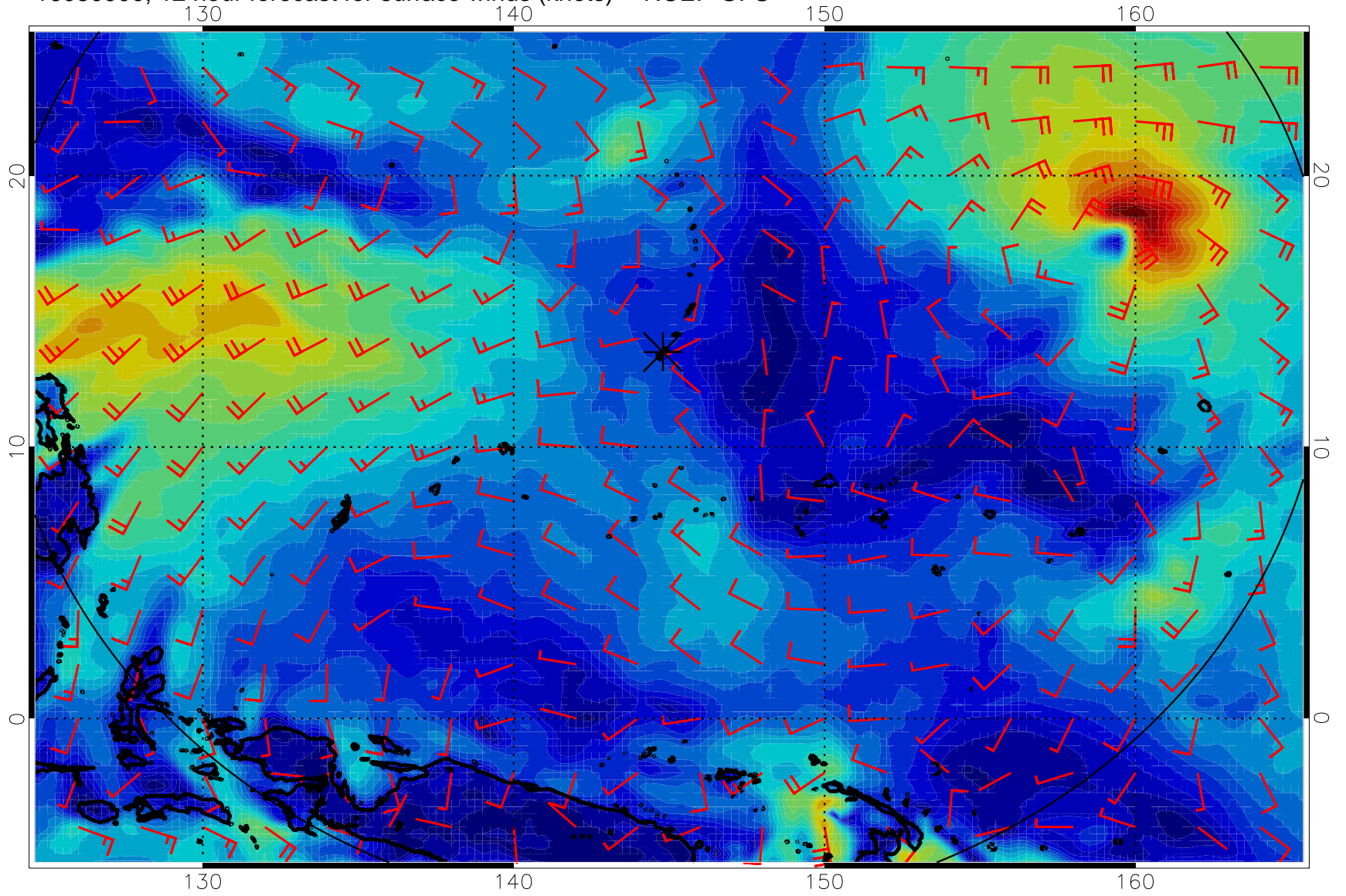
16080900, 12 hour forecast for surface winds (knots) -- NCEP GFS
