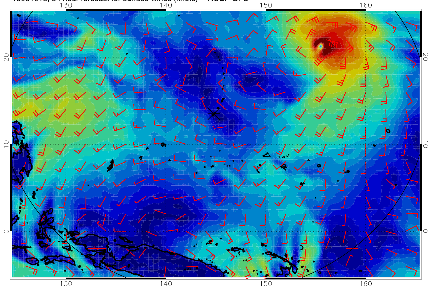
16081018, 54 hour forecast for surface winds (knots) -- NCEP GFS
