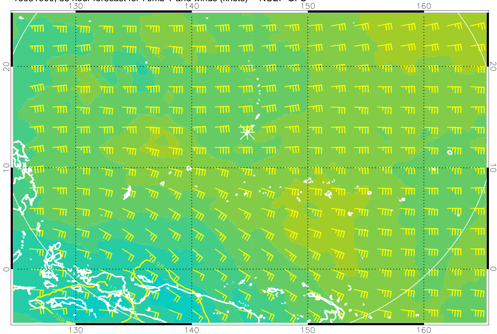
16081000, 36 hour forecast for 70mb T and winds (knots) -- NCEP GFS
