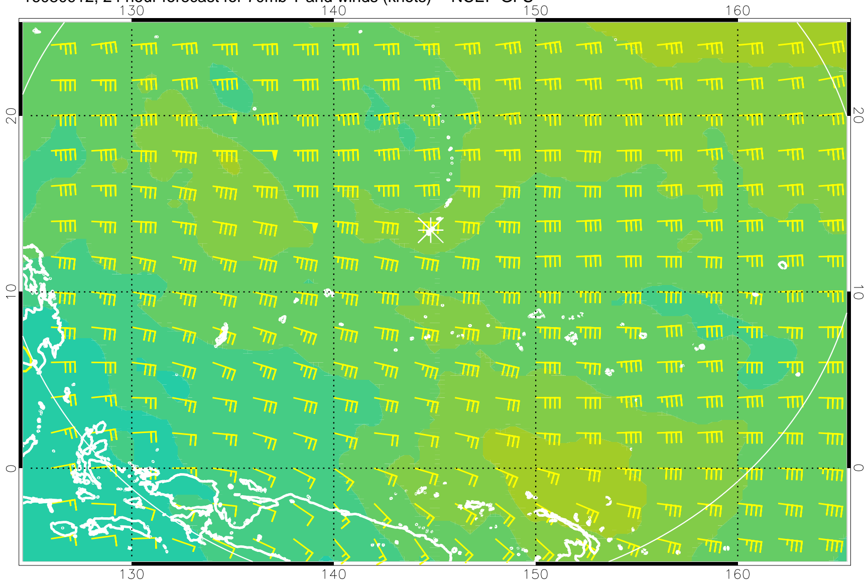
16080912, 24 hour forecast for 70mb T and winds (knots) -- NCEP GFS
