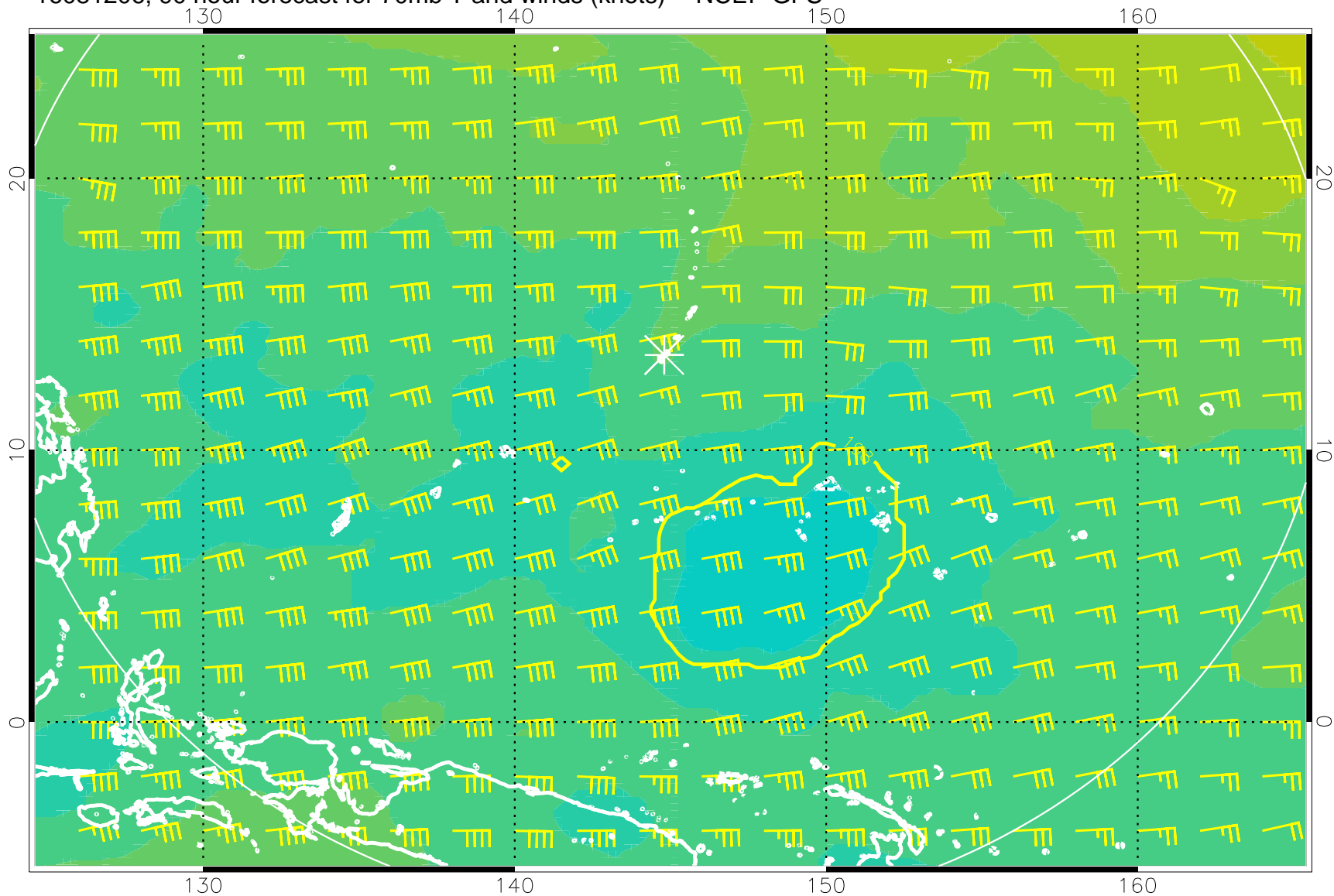
16081206, 90 hour forecast for 70mb T and winds (knots) -- NCEP GFS
