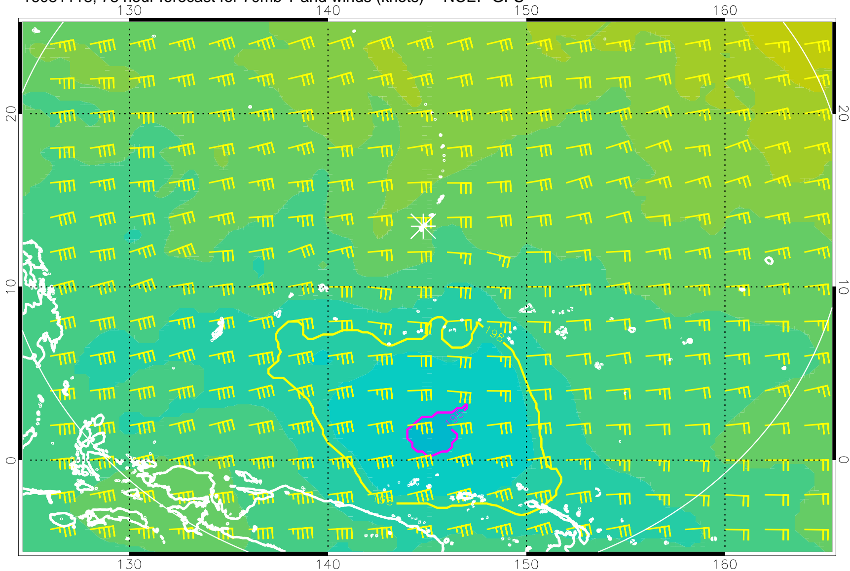
16081118, 78 hour forecast for 70mb T and winds (knots) -- NCEP GFS
