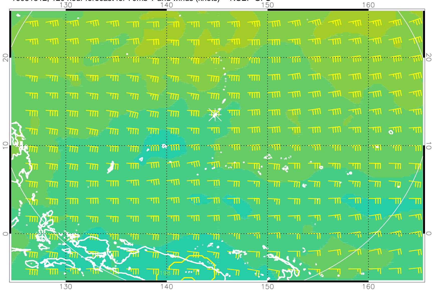
16081312, 120 hour forecast for 70mb T and winds (knots) -- NCEP GFS
