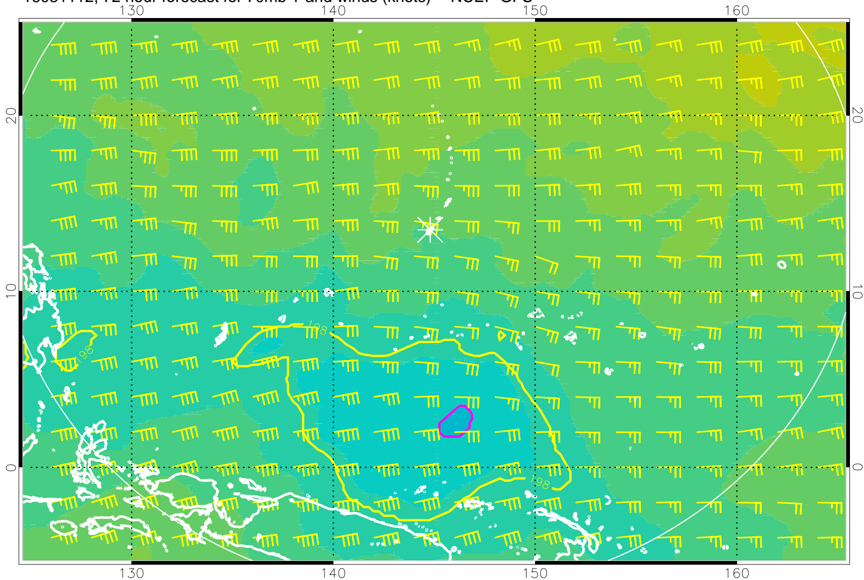
16081112, 72 hour forecast for 70mb T and winds (knots) -- NCEP GFS
