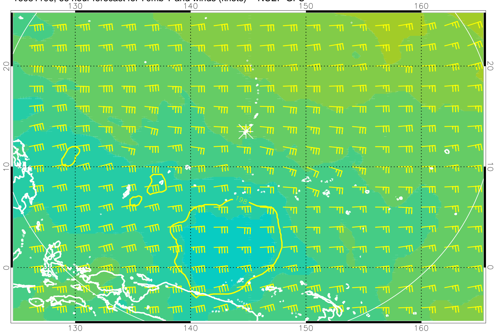
16081106, 66 hour forecast for 70mb T and winds (knots) -- NCEP GFS
