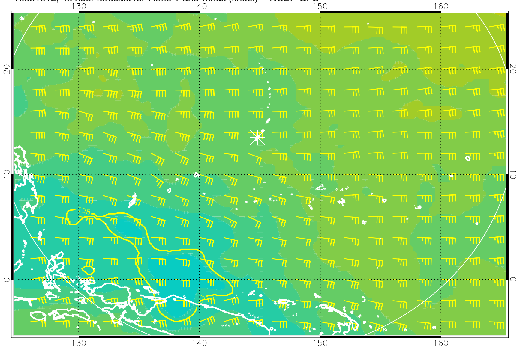
16081012, 48 hour forecast for 70mb T and winds (knots) -- NCEP GFS
