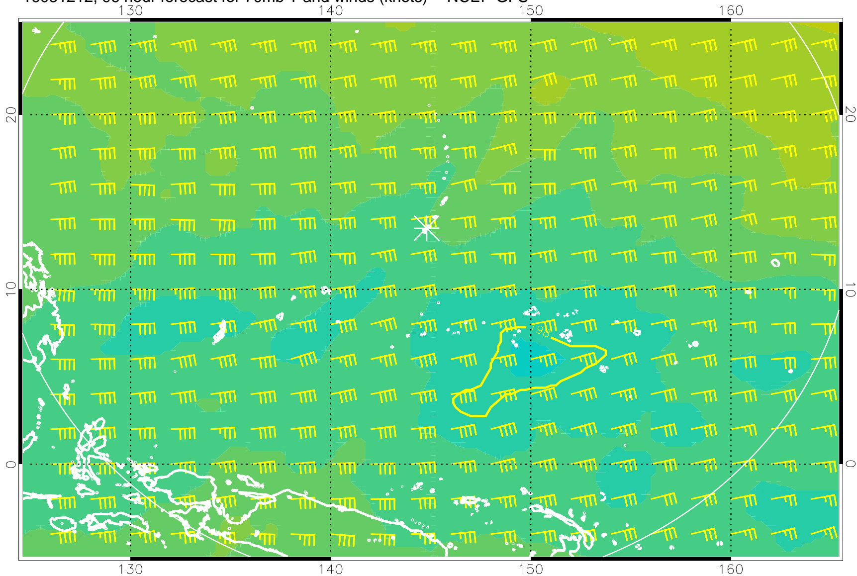
16081212, 96 hour forecast for 70mb T and winds (knots) -- NCEP GFS
