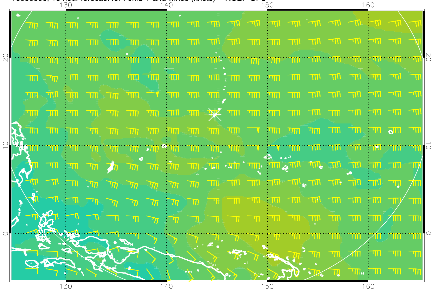
16080906, 18 hour forecast for 70mb T and winds (knots) -- NCEP GFS
