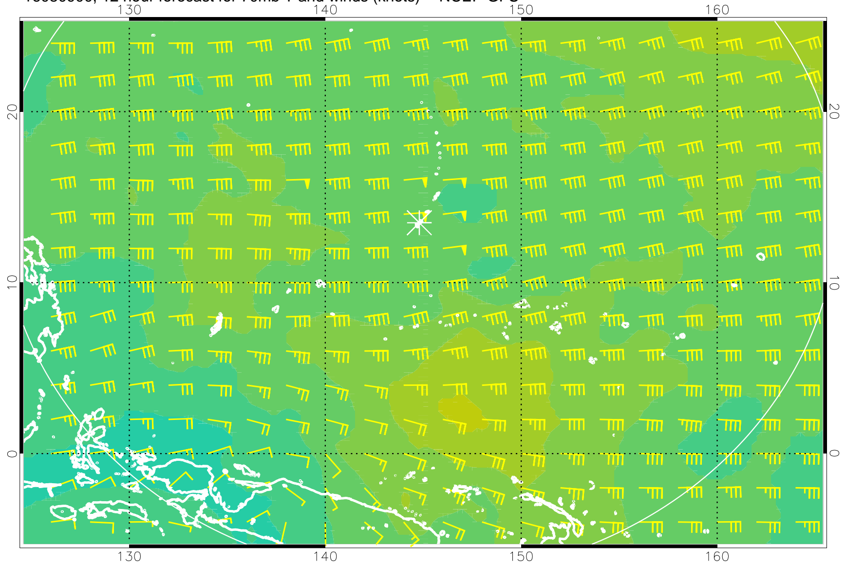
16080900, 12 hour forecast for 70mb T and winds (knots) -- NCEP GFS
