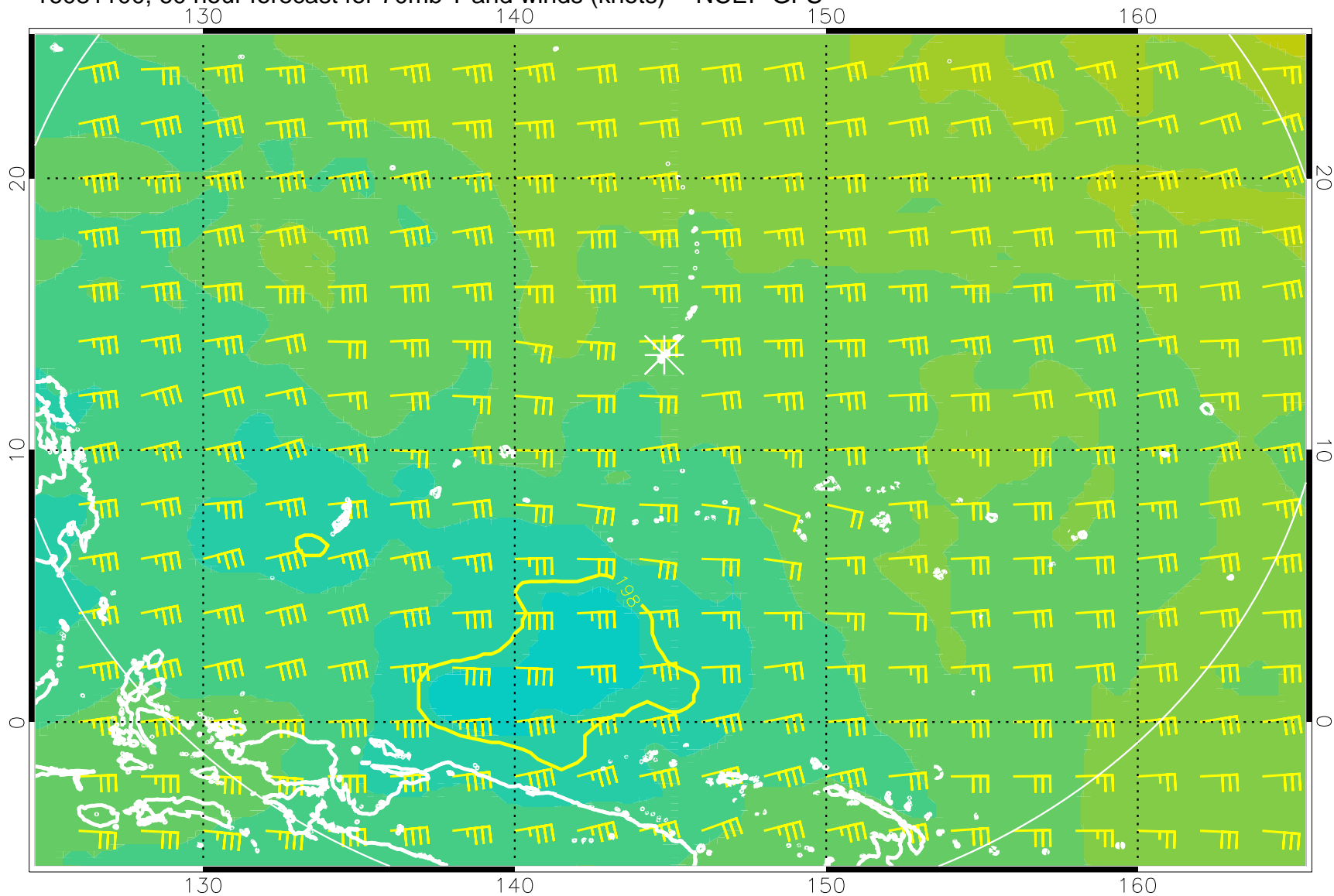
16081100, 60 hour forecast for 70mb T and winds (knots) -- NCEP GFS
