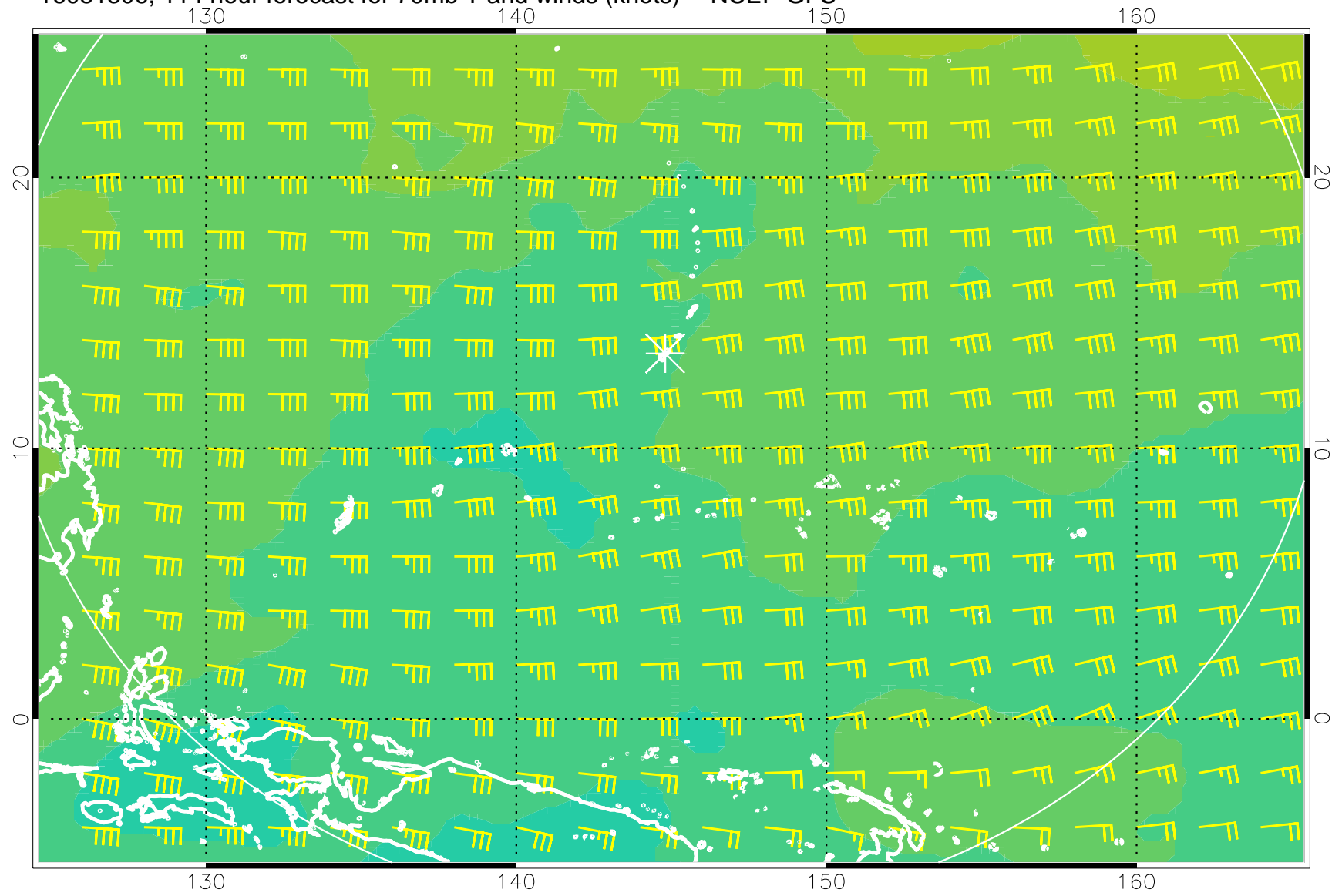
16081306, 114 hour forecast for 70mb T and winds (knots) -- NCEP GFS
