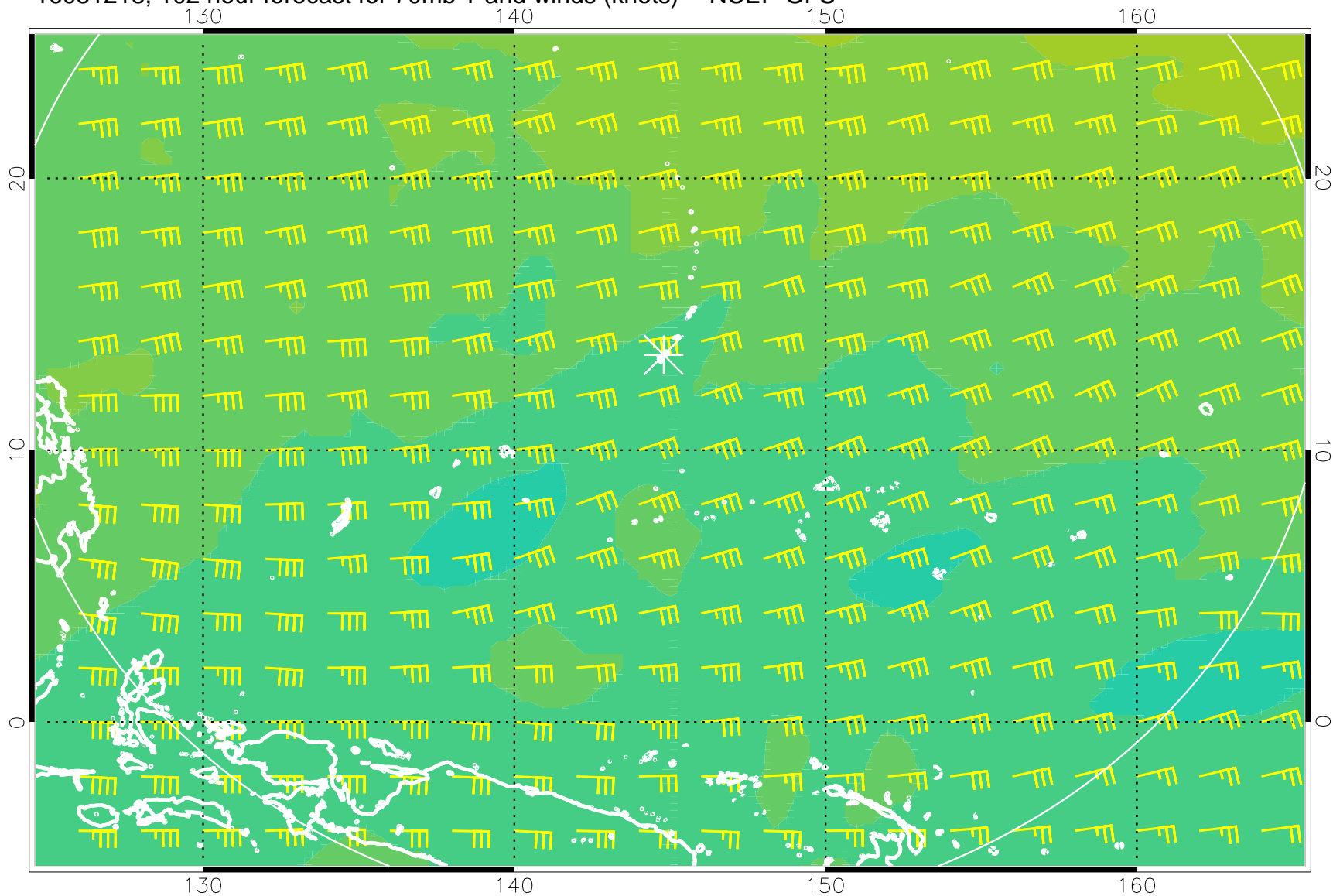
16081218, 102 hour forecast for 70mb T and winds (knots) -- NCEP GFS
