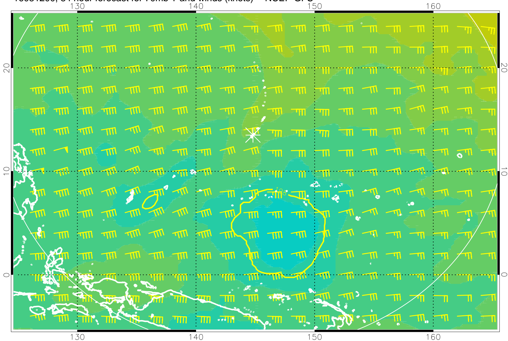
16081200, 84 hour forecast for 70mb T and winds (knots) -- NCEP GFS
