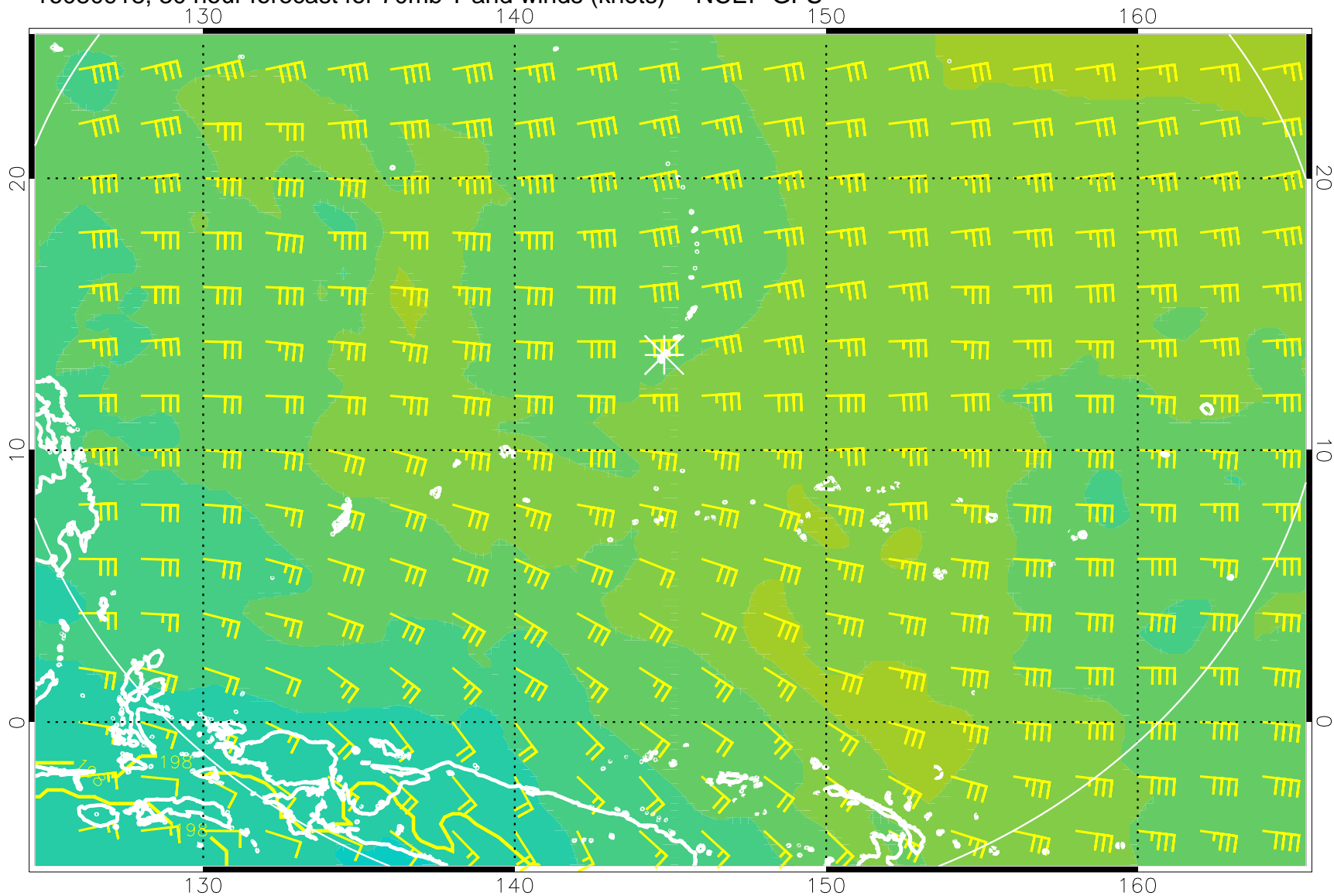
16080918, 30 hour forecast for 70mb T and winds (knots) -- NCEP GFS
