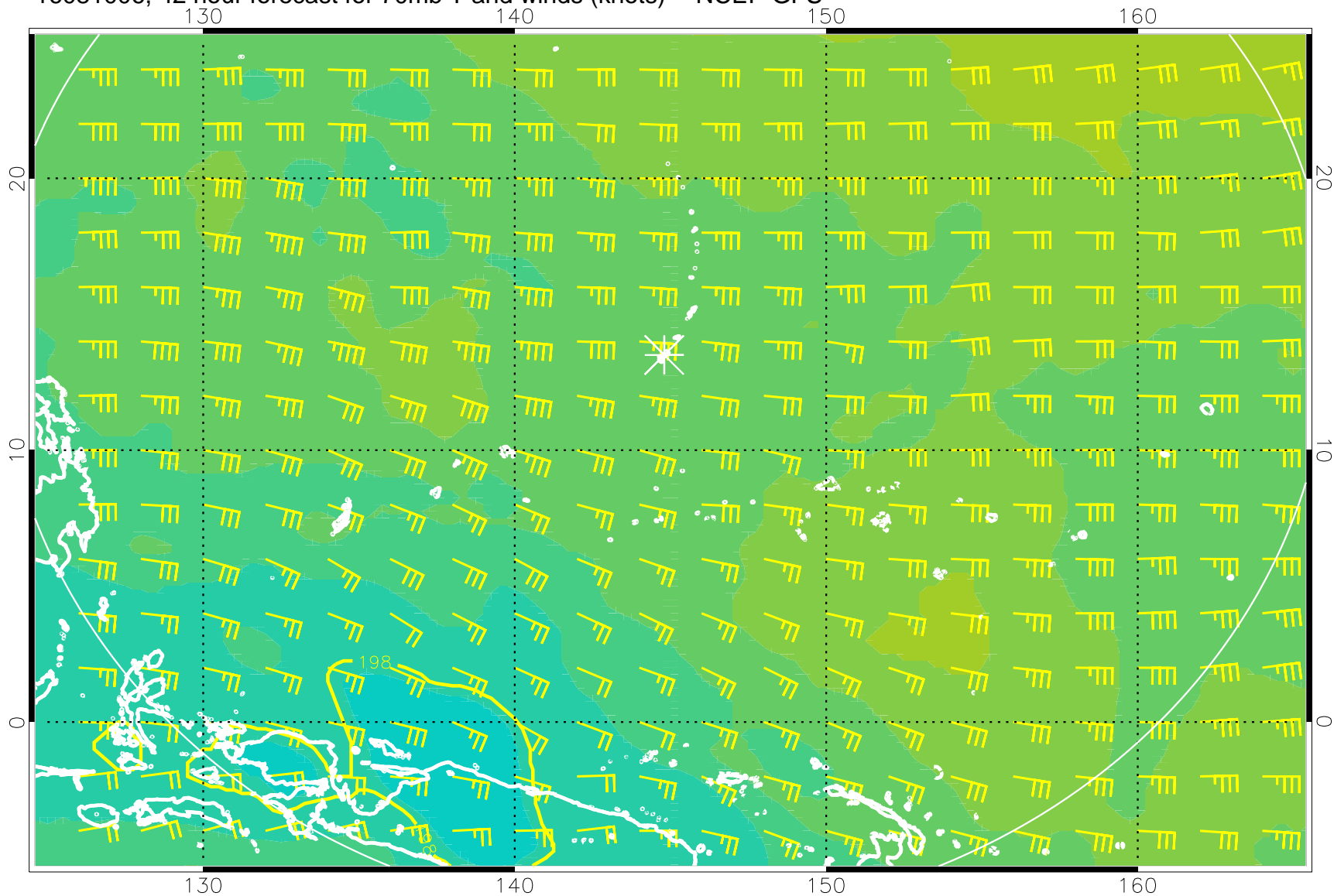
16081006, 42 hour forecast for 70mb T and winds (knots) -- NCEP GFS
