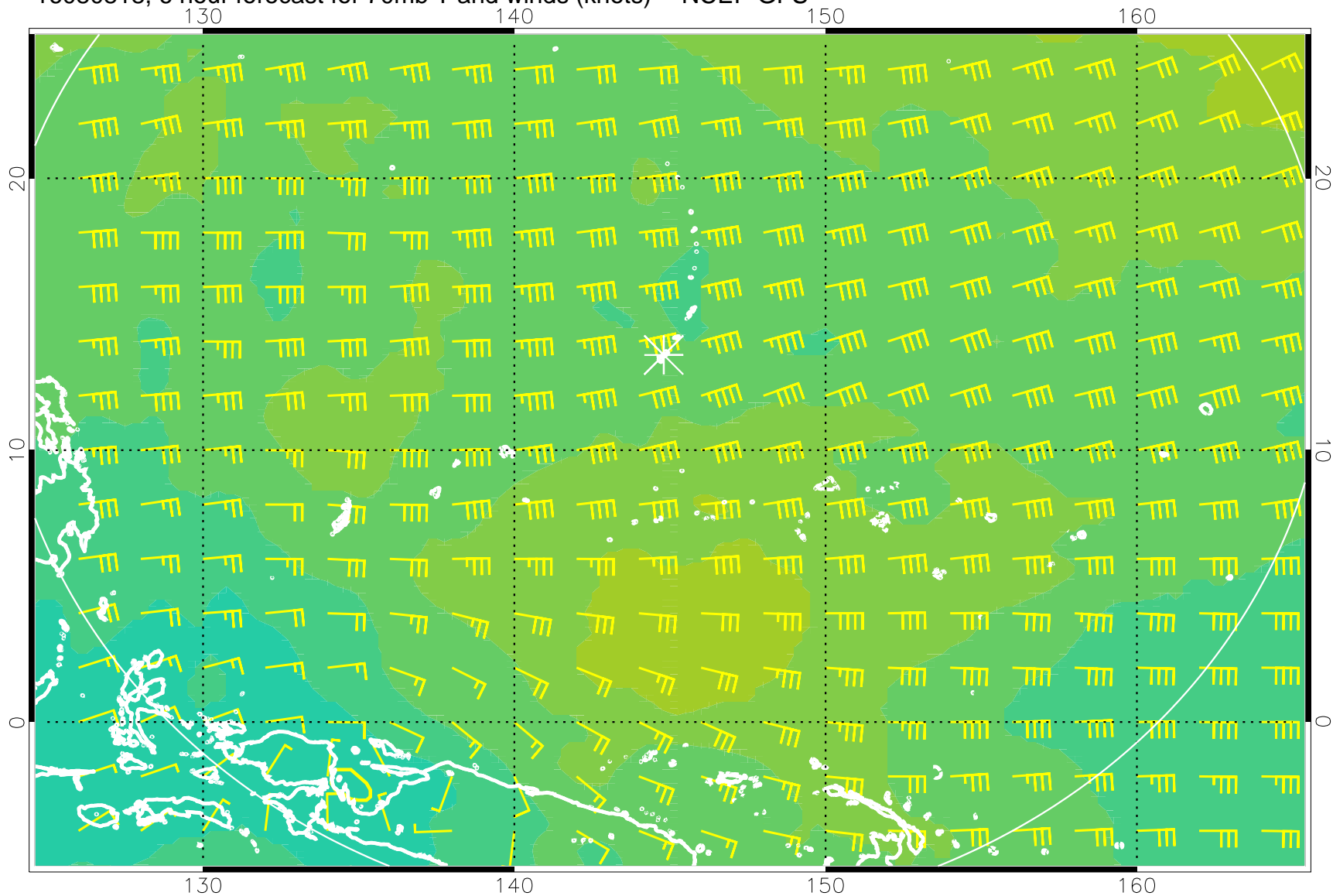
16080818, 6 hour forecast for 70mb T and winds (knots) -- NCEP GFS
