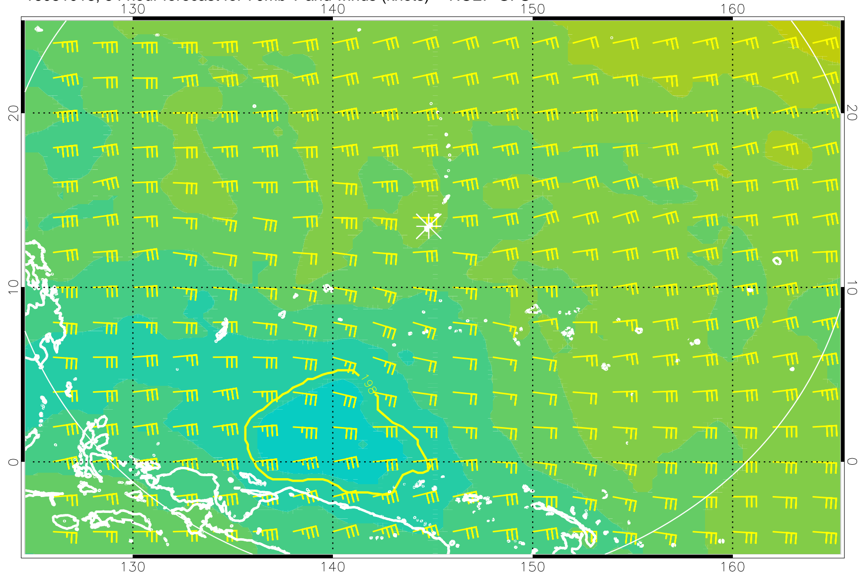
16081018, 54 hour forecast for 70mb T and winds (knots) -- NCEP GFS
