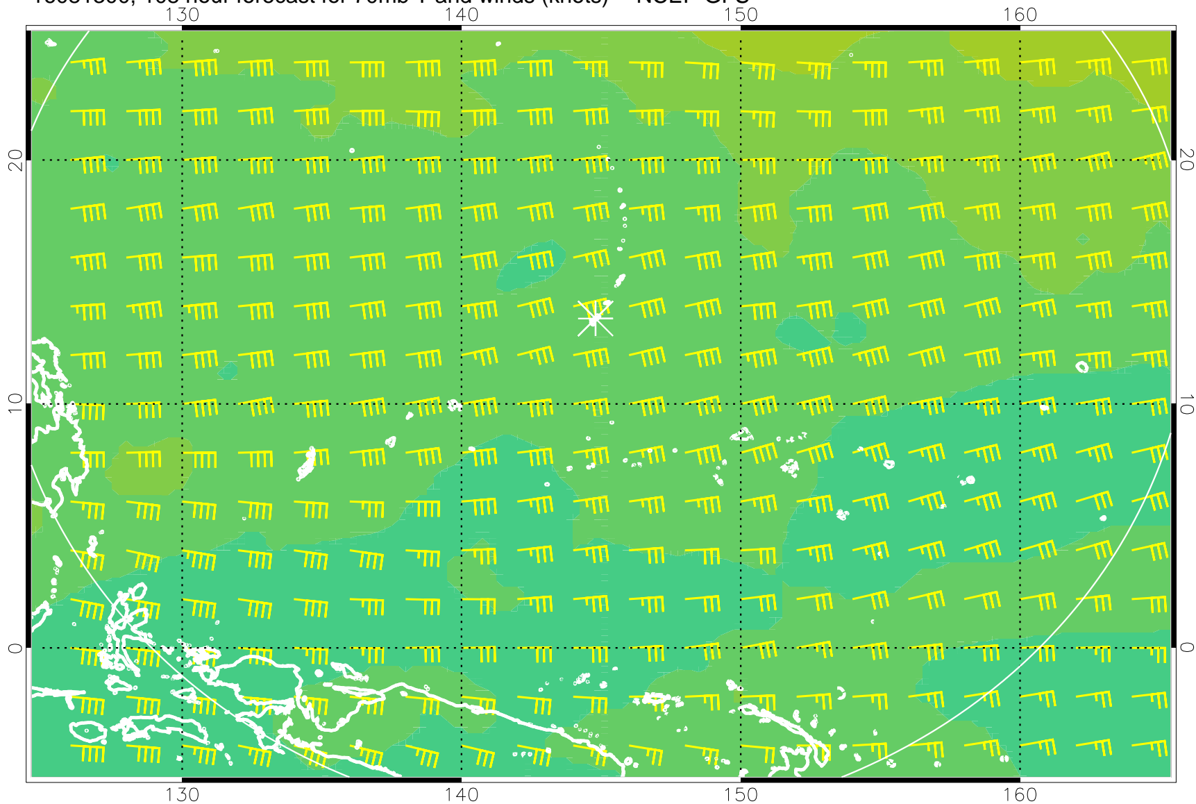
16081300, 108 hour forecast for 70mb T and winds (knots) -- NCEP GFS
