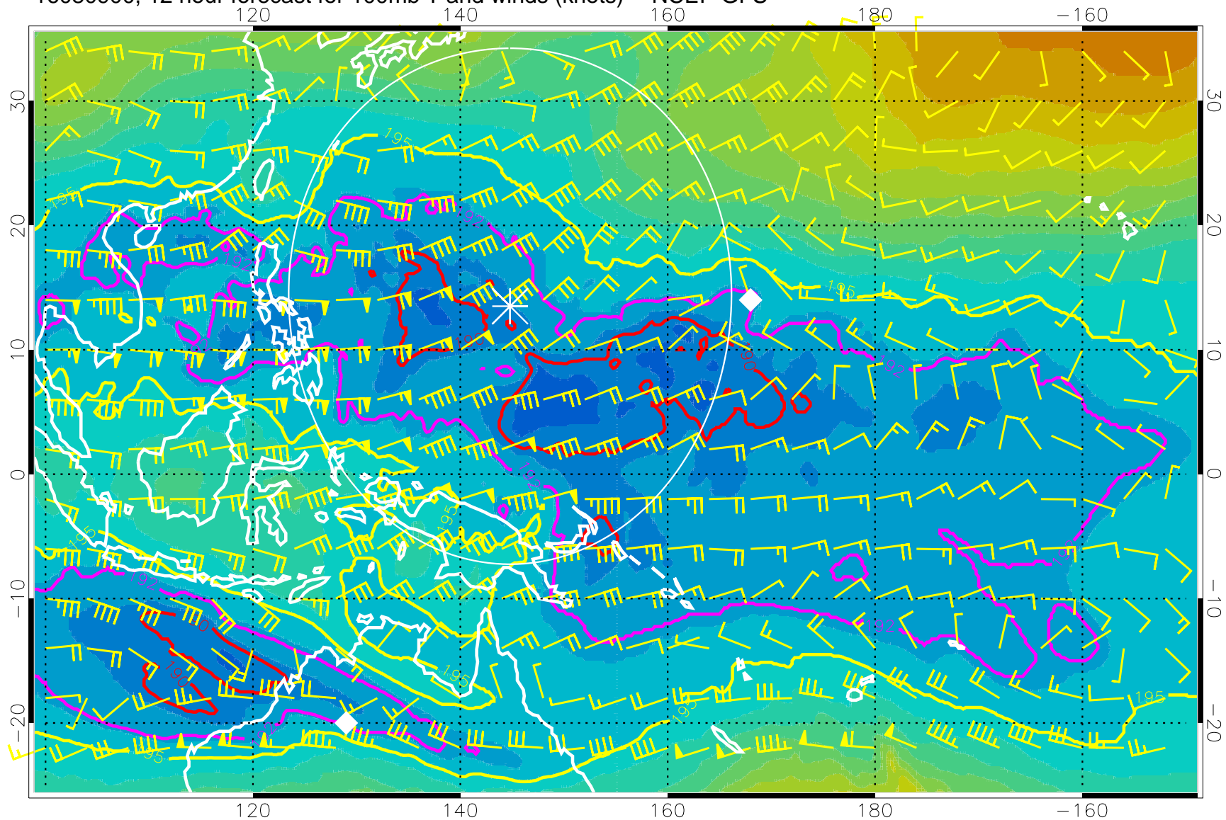
16080900, 12 hour forecast for 100mb T and winds (knots) -- NCEP GFS
