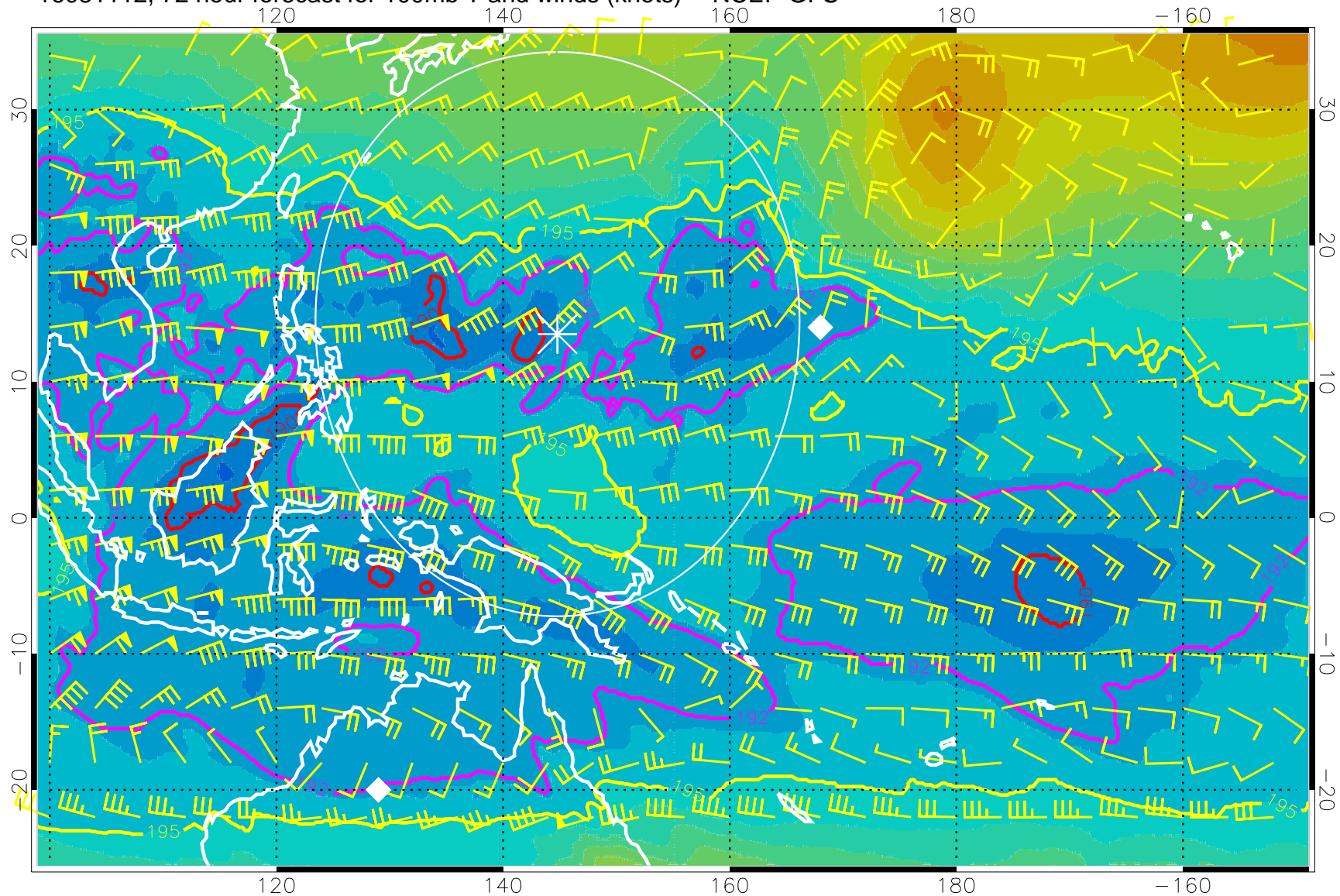
16081112, 72 hour forecast for 100mb T and winds (knots) -- NCEP GFS
