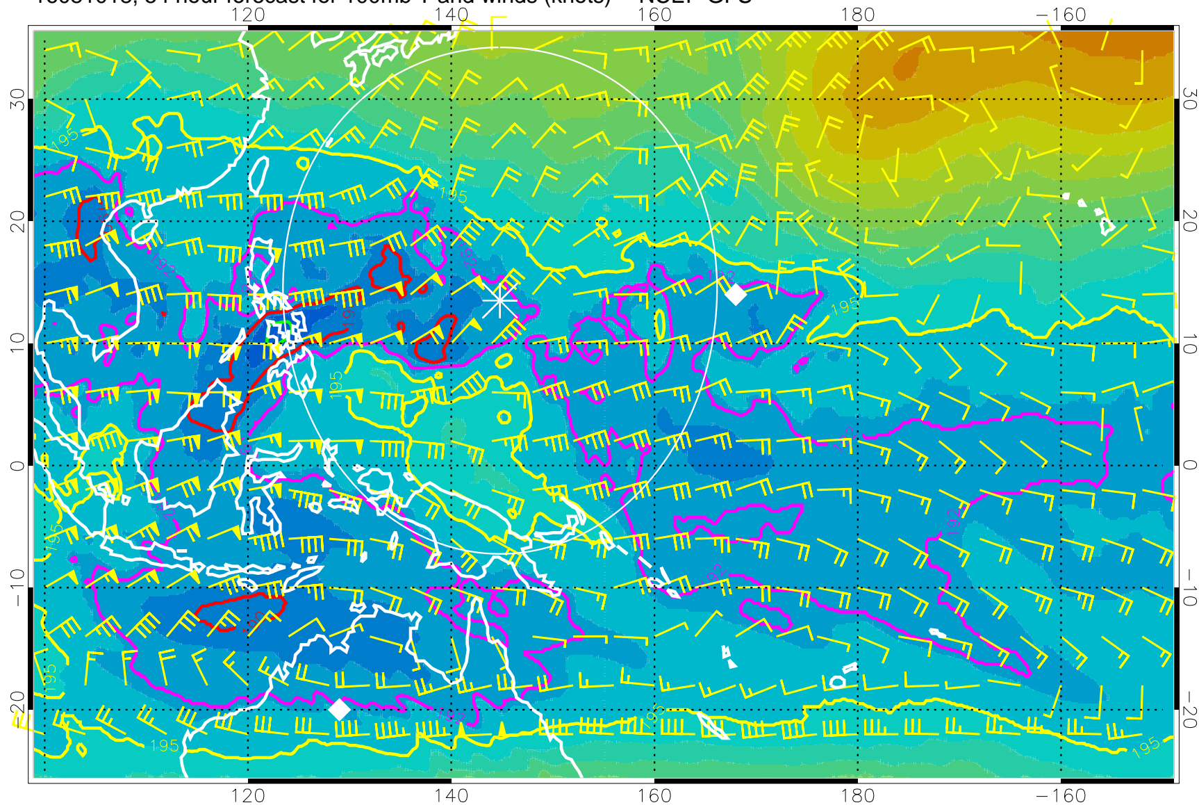
16081018, 54 hour forecast for 100mb T and winds (knots) -- NCEP GFS
