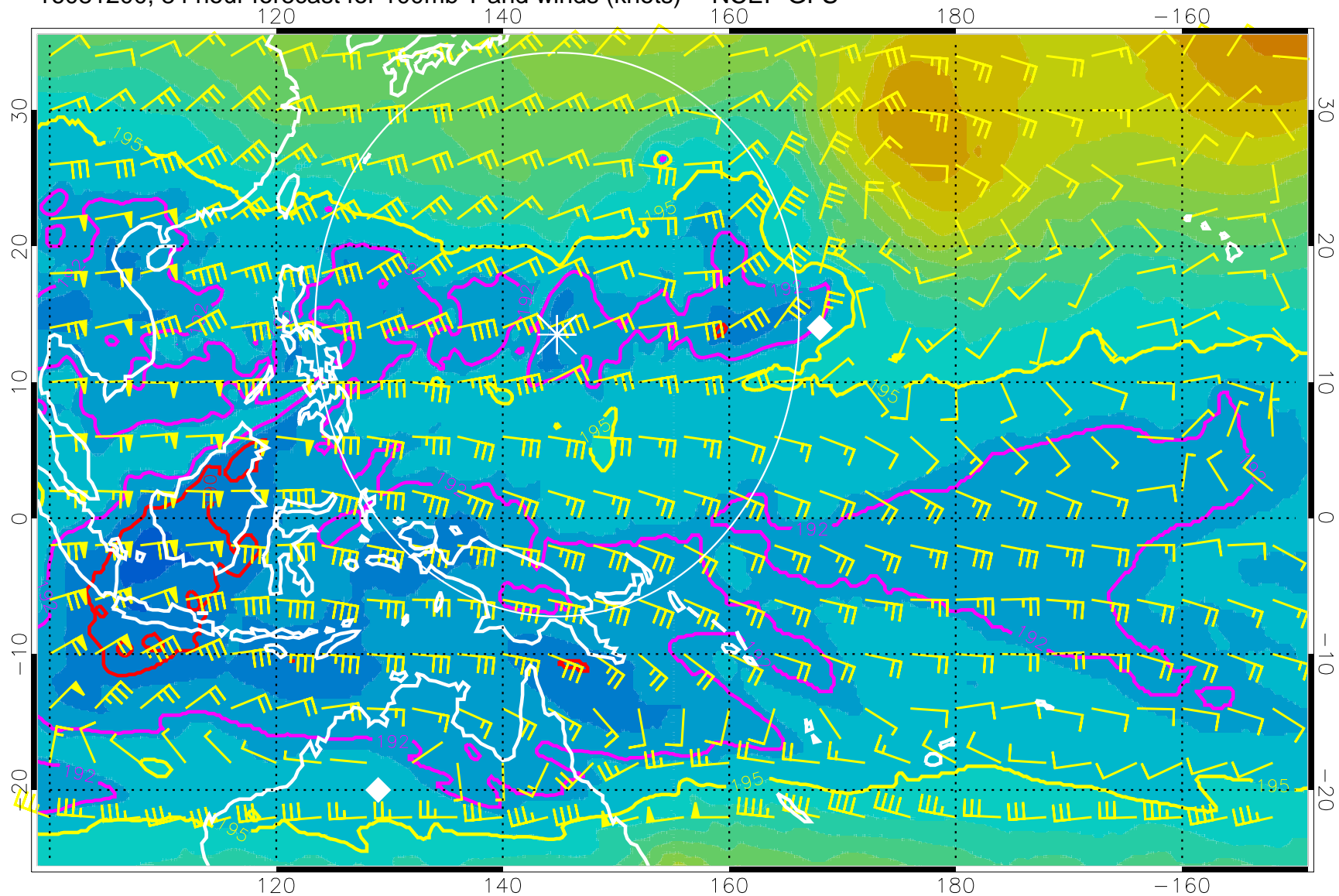
16081200, 84 hour forecast for 100mb T and winds (knots) -- NCEP GFS
