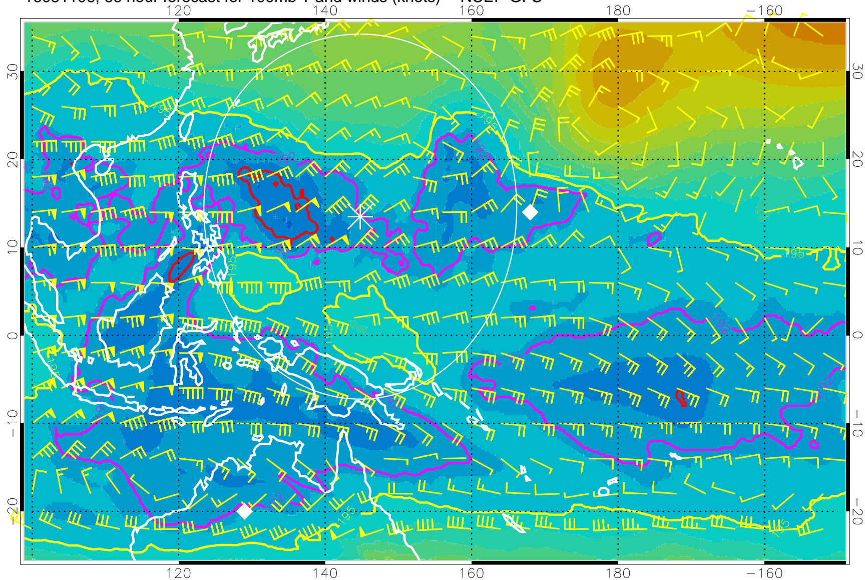
16081106, 66 hour forecast for 100mb T and winds (knots) -- NCEP GFS
