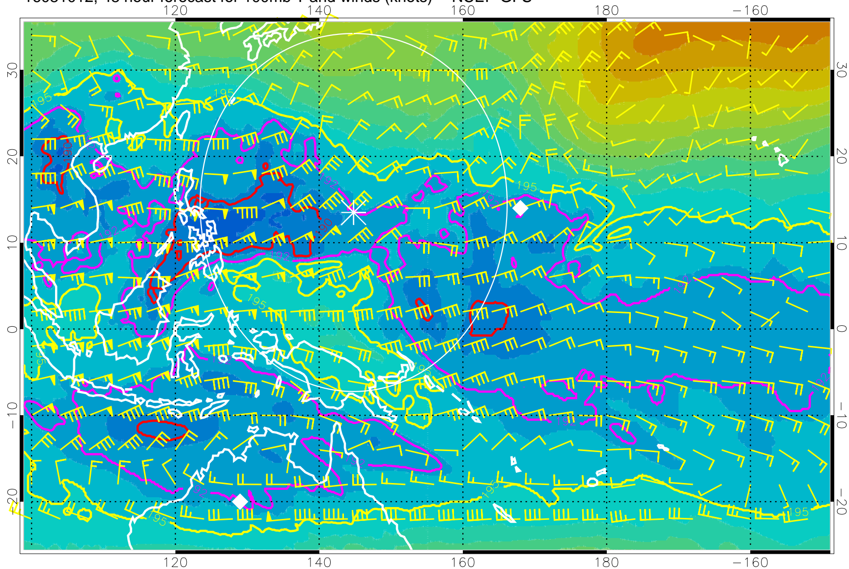
16081012, 48 hour forecast for 100mb T and winds (knots) -- NCEP GFS
