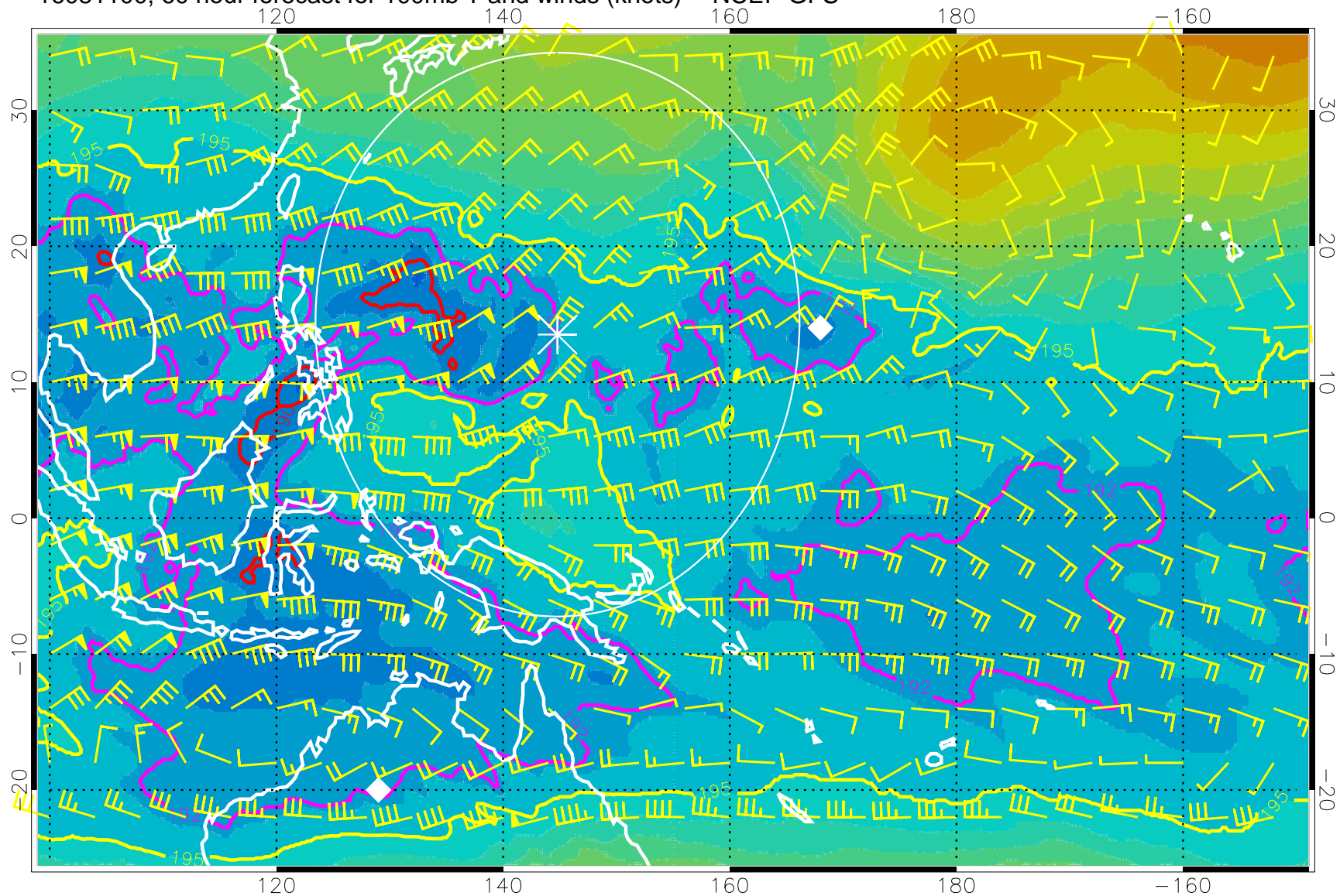
16081100, 60 hour forecast for 100mb T and winds (knots) -- NCEP GFS
