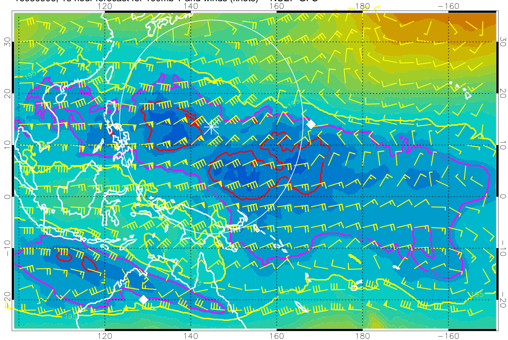
16080906, 18 hour forecast for 100mb T and winds (knots) -- NCEP GFS
