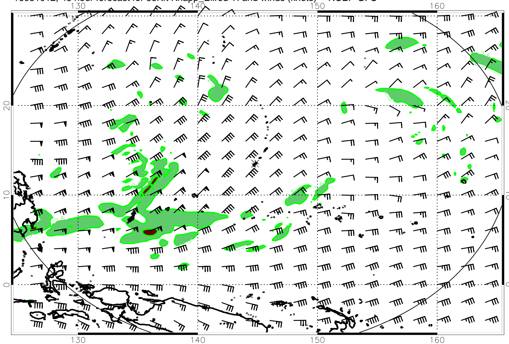
16081012, 48 hour forecast for 53Kft Knapp_Ellrod TI and winds (knots) -- NCEP GFS
