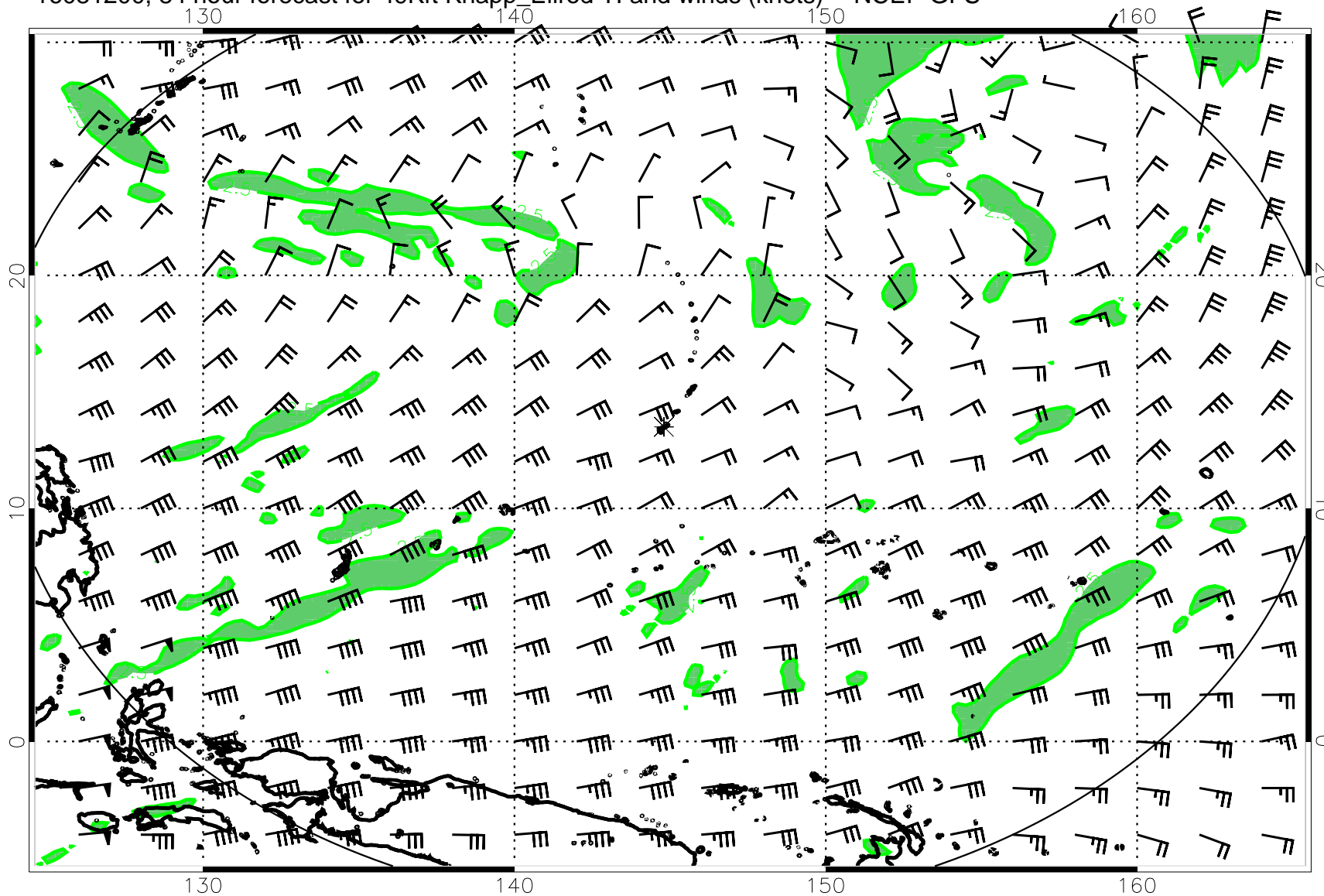
16081200, 84 hour forecast for 49Kft Knapp_Ellrod TI and winds (knots) -- NCEP GFS
