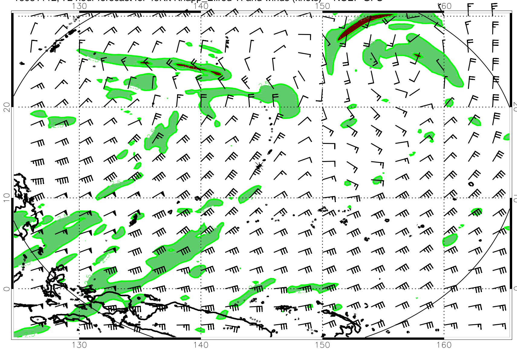
16081112, 72 hour forecast for 49Kft Knapp_Ellrod TI and winds (knots) -- NCEP GFS
