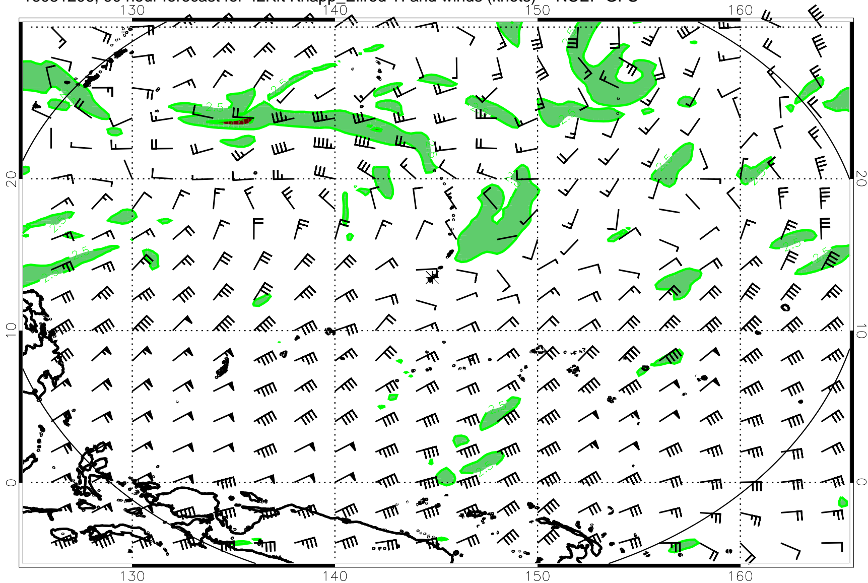
16081206, 90 hour forecast for 42Kft Knapp_Ellrod TI and winds (knots) -- NCEP GFS
