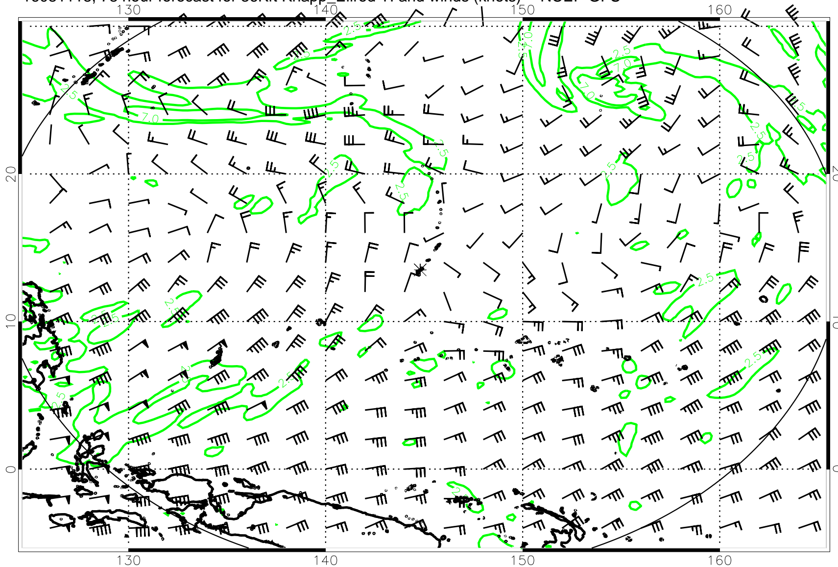
16081118, 78 hour forecast for 36Kft Knapp_Ellrod TI and winds (knots) -- NCEP GFS
