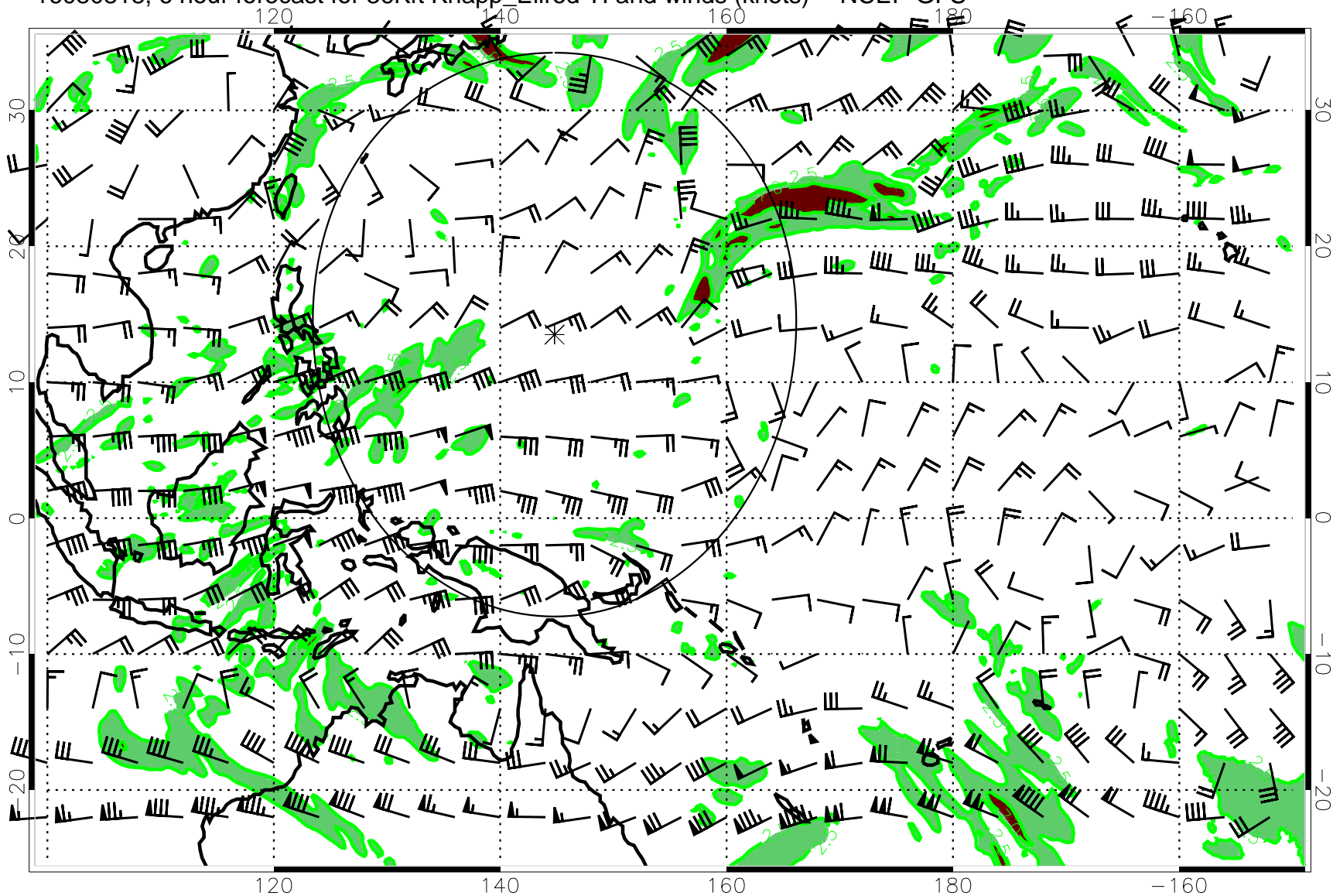
16080818, 6 hour forecast for 36Kft Knapp_Ellrod TI and winds (knots) -- NCEP GFS
