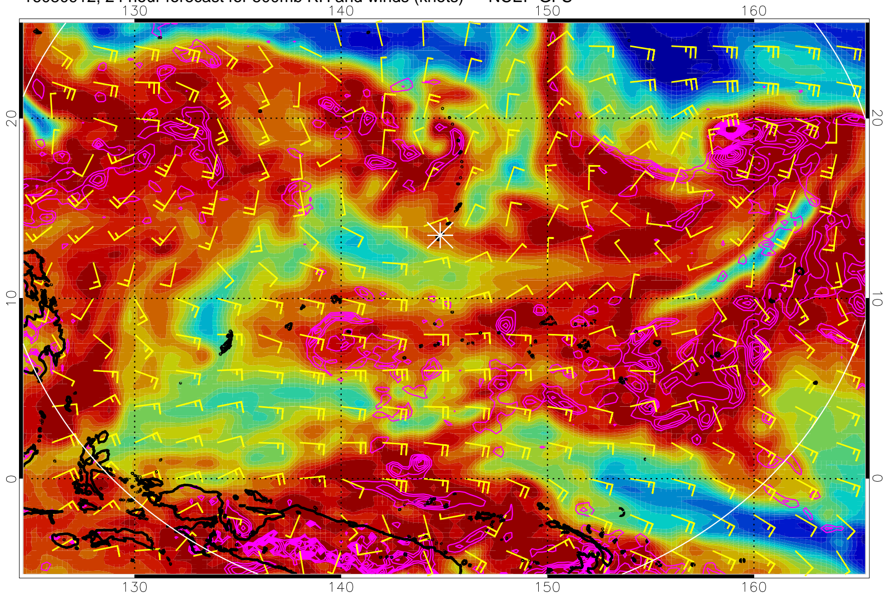
16080912, 24 hour forecast for 500mb RH and winds (knots) -- NCEP GFS
