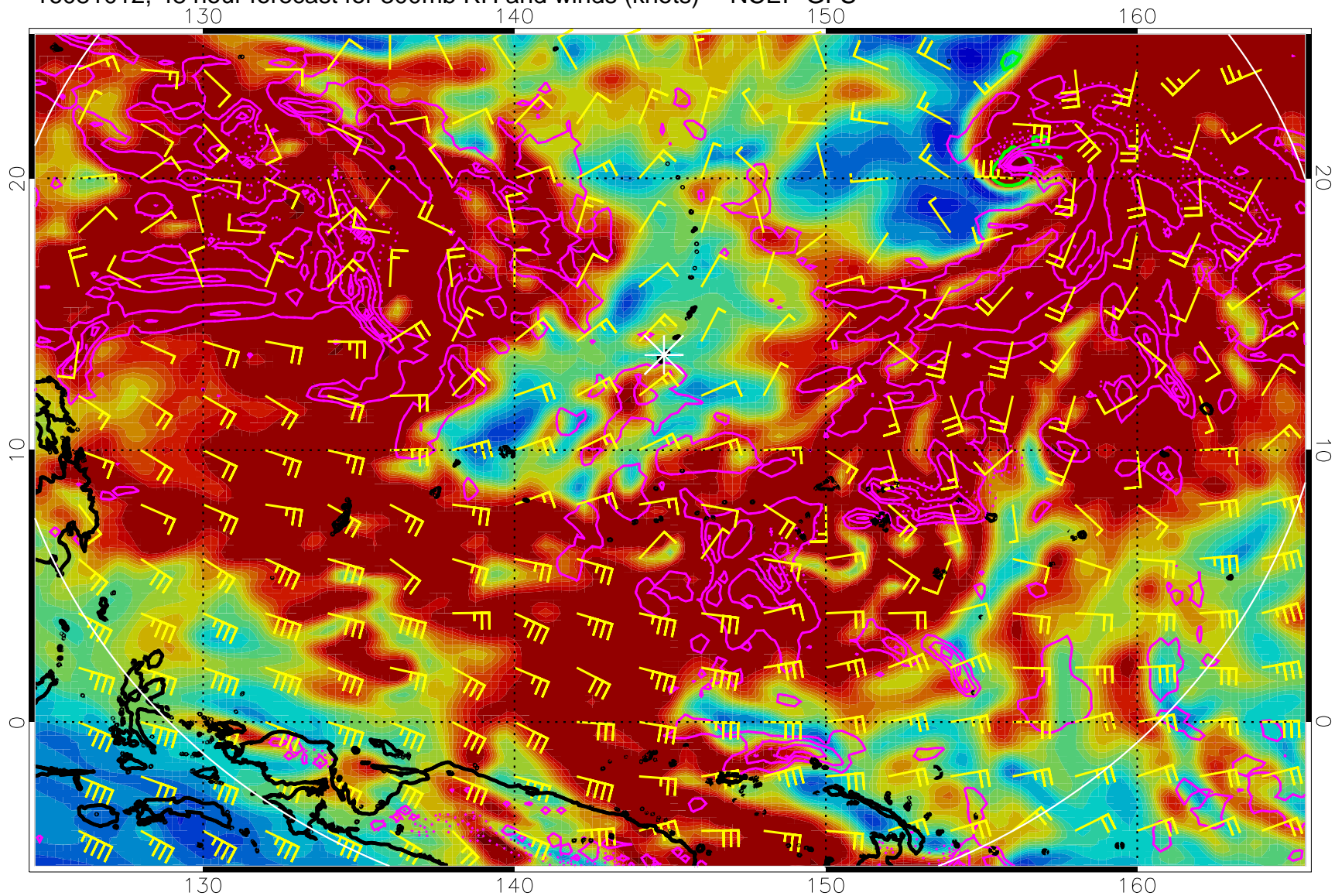
16081012, 48 hour forecast for 300mb RH and winds (knots) -- NCEP GFS
