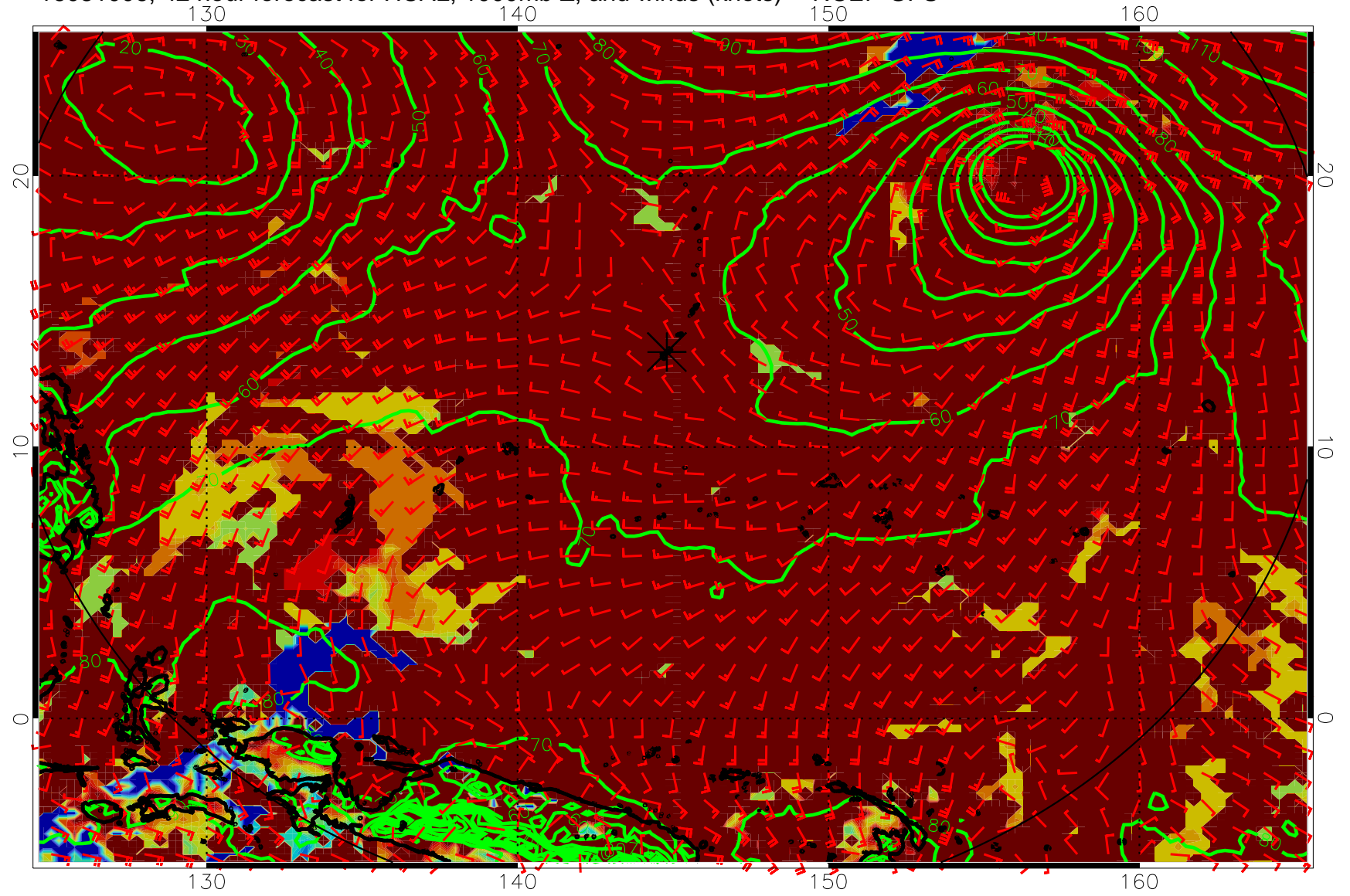
16081006, 42 hour forecast for HCAL, 1000mb Z, and winds (knots) -- NCEP GFS
