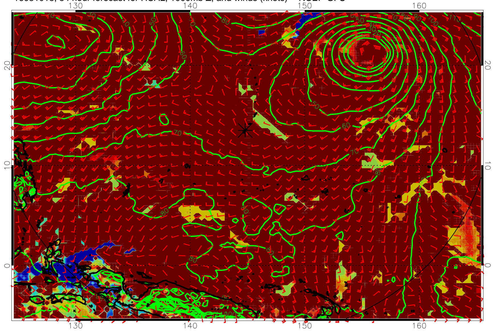
16081018, 54 hour forecast for HCAL, 1000mb Z, and winds (knots) -- NCEP GFS
