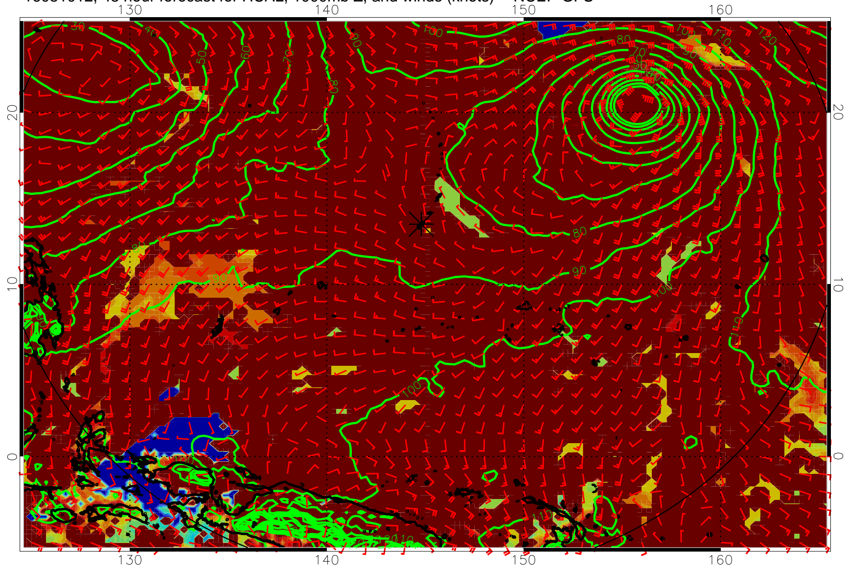
16081012, 48 hour forecast for HCAL, 1000mb Z, and winds (knots) -- NCEP GFS
