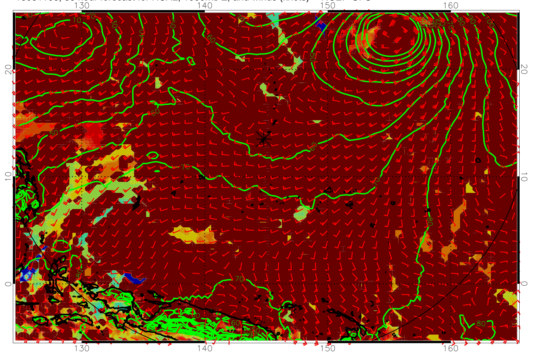
16081106, 66 hour forecast for HCAL, 1000mb Z, and winds (knots) -- NCEP GFS
