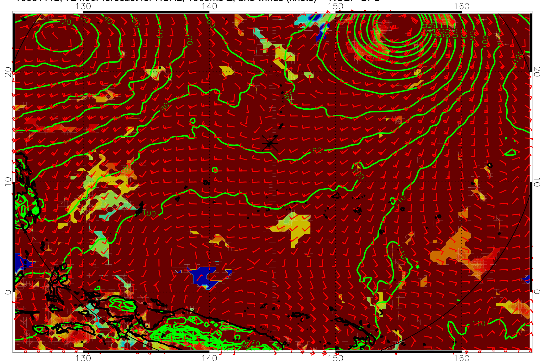
16081112, 72 hour forecast for HCAL, 1000mb Z, and winds (knots) -- NCEP GFS
