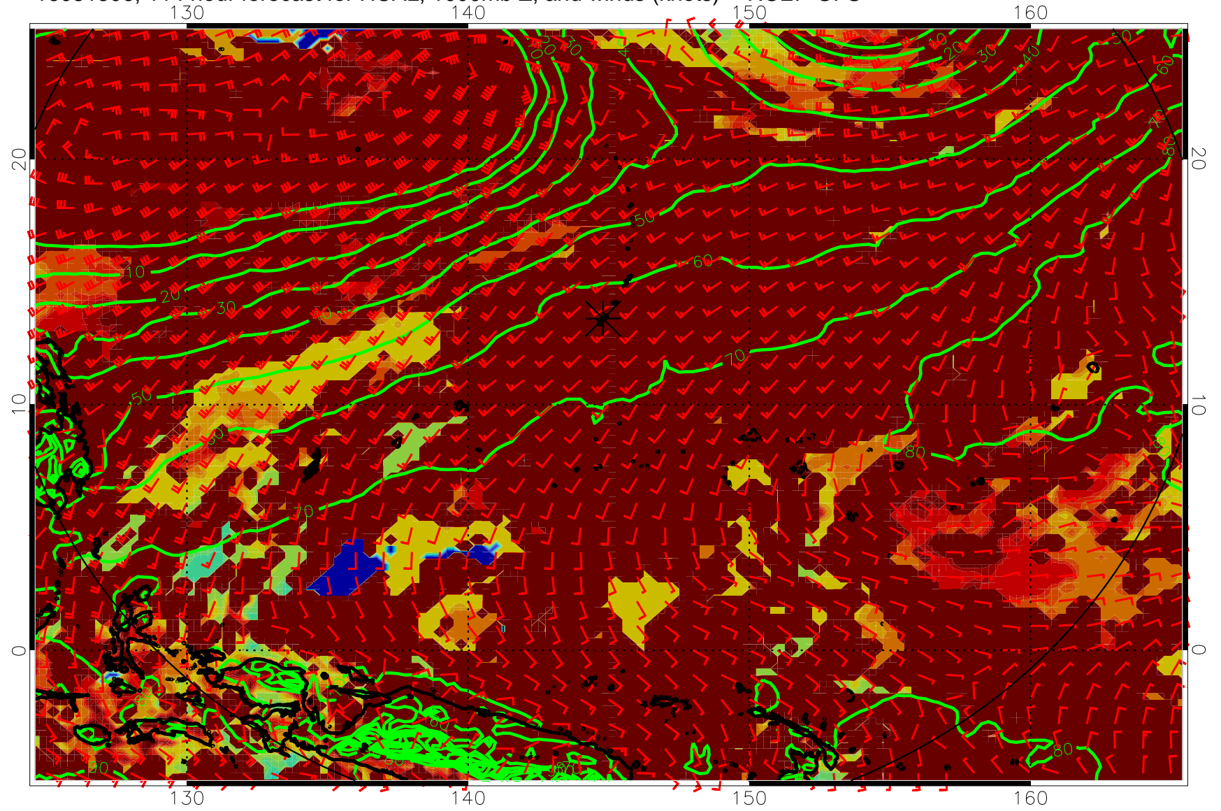
16081306, 114 hour forecast for HCAL, 1000mb Z, and winds (knots) -- NCEP GFS
