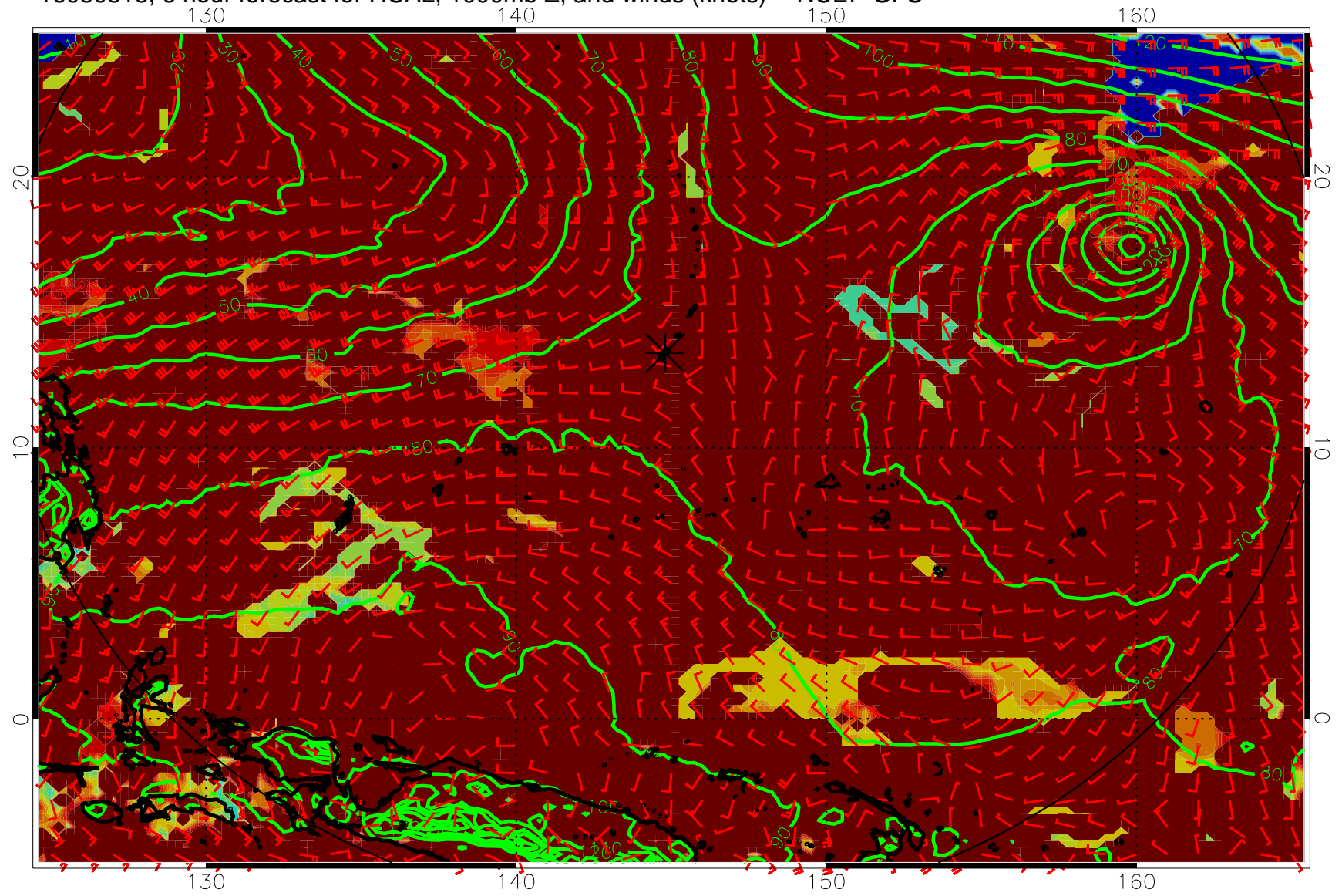
16080818, 6 hour forecast for HCAL, 1000mb Z, and winds (knots) -- NCEP GFS
