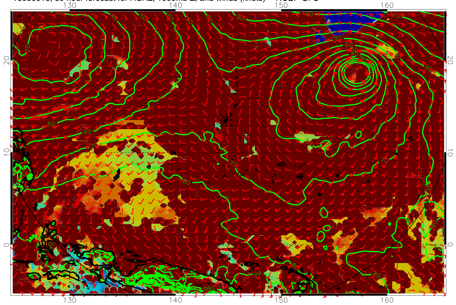
16080918, 30 hour forecast for HCAL, 1000mb Z, and winds (knots) -- NCEP GFS
