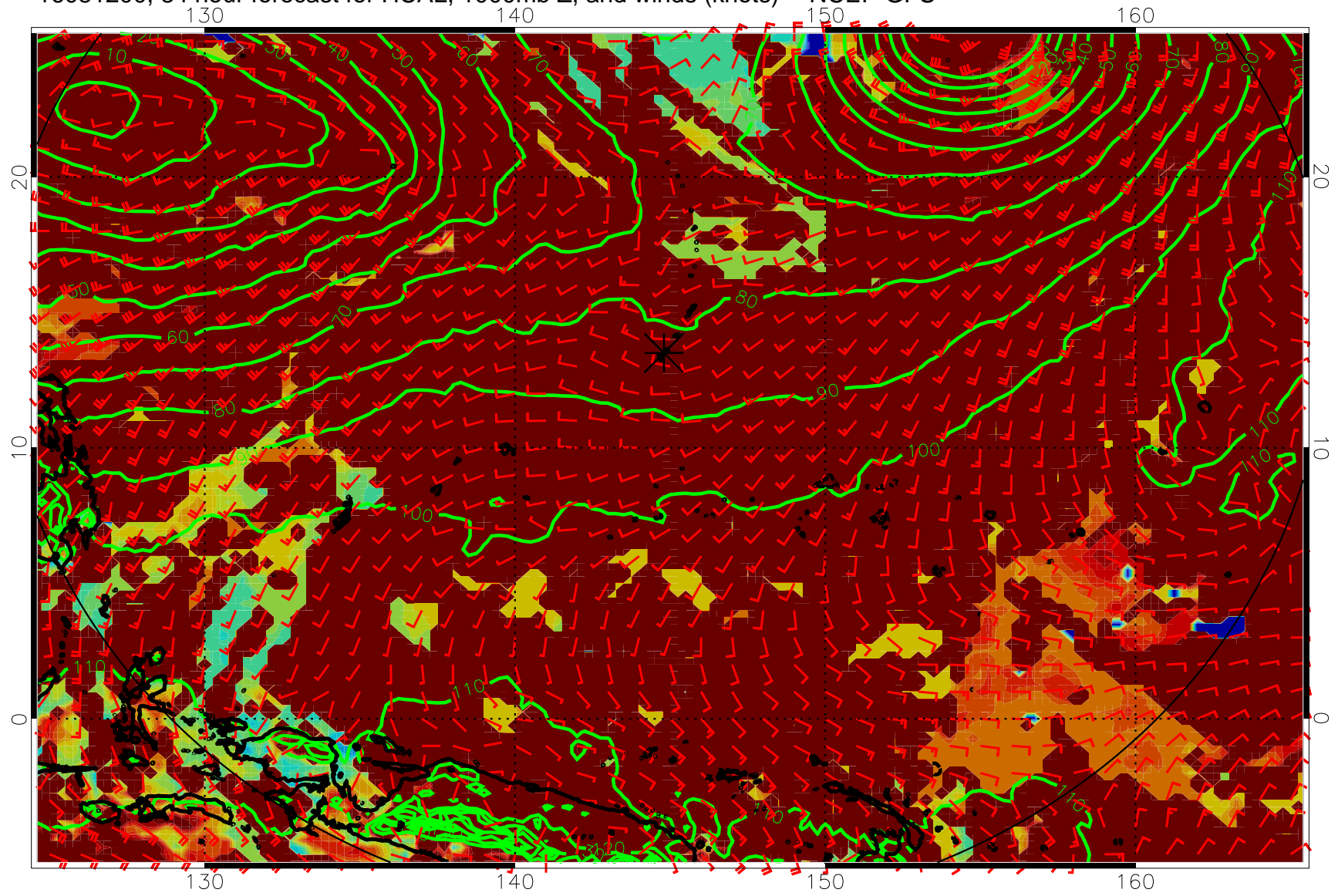
16081200, 84 hour forecast for HCAL, 1000mb Z, and winds (knots) -- NCEP GFS
