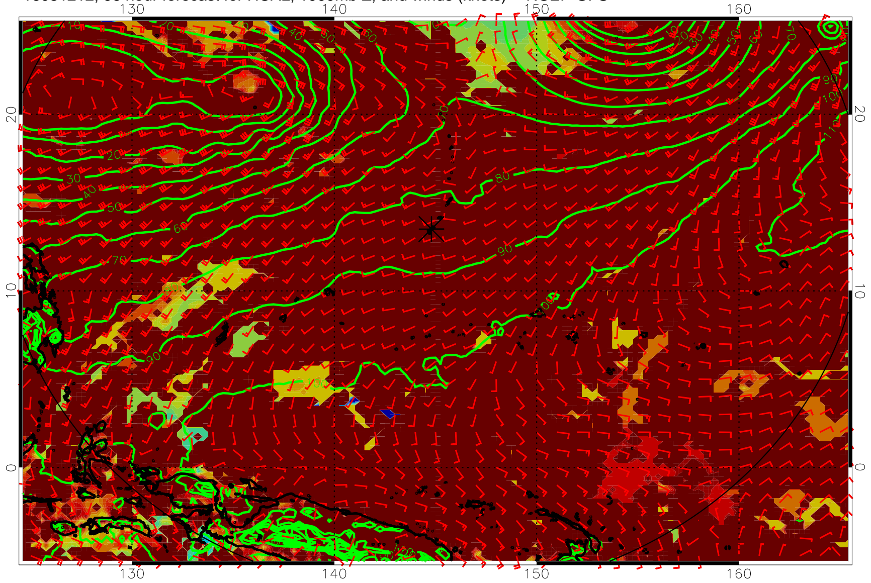
16081212, 96 hour forecast for HCAL, 1000mb Z, and winds (knots) -- NCEP GFS
