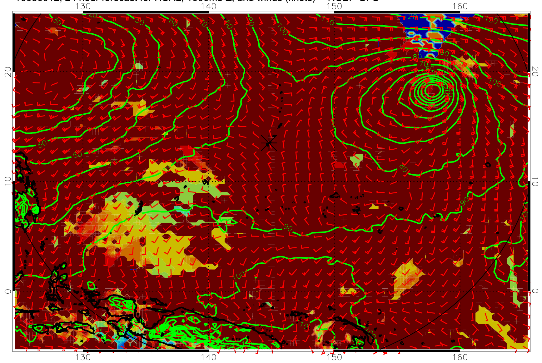
16080912, 24 hour forecast for HCAL, 1000mb Z, and winds (knots) -- NCEP GFS
