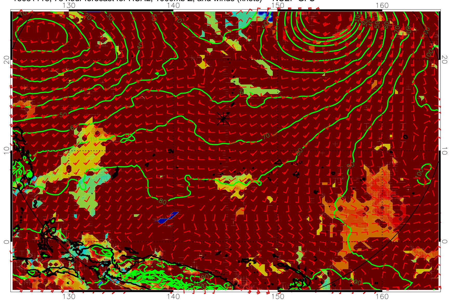
16081118, 78 hour forecast for HCAL, 1000mb Z, and winds (knots) -- NCEP GFS
