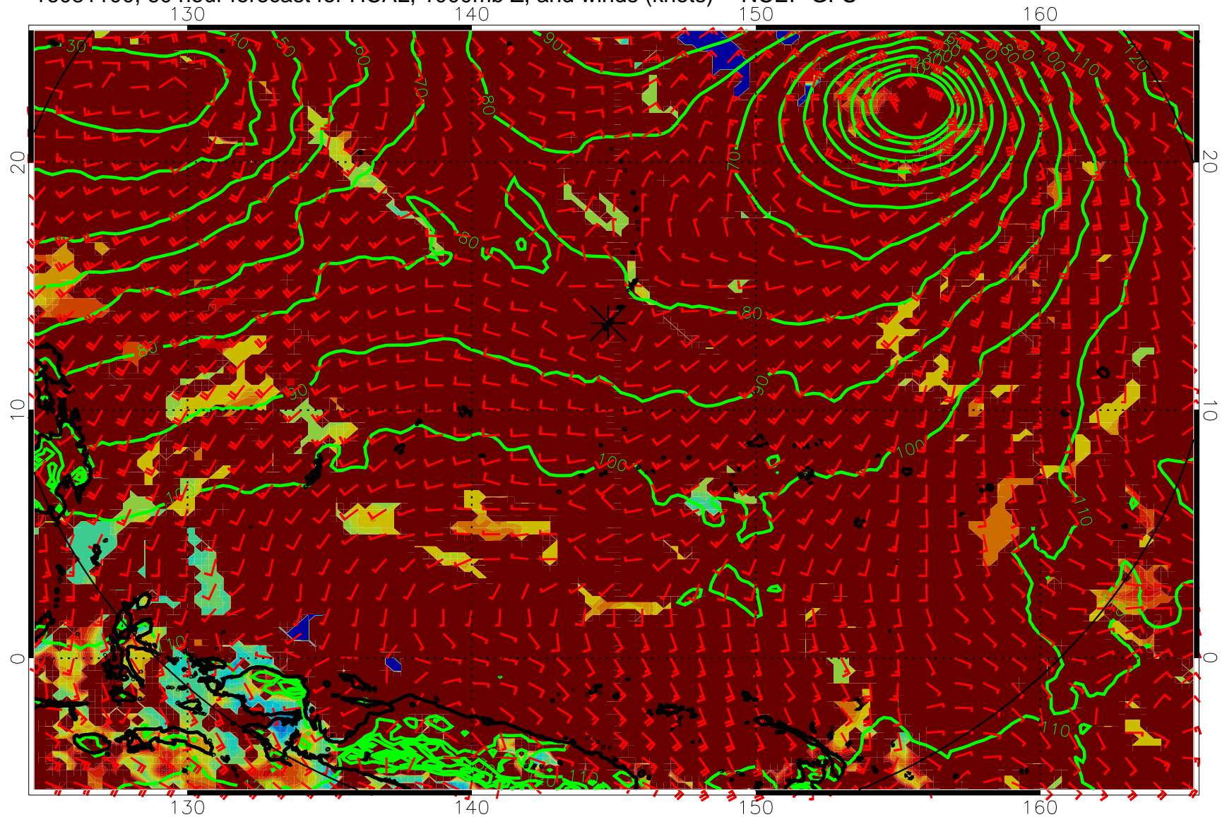
16081100, 60 hour forecast for HCAL, 1000mb Z, and winds (knots) -- NCEP GFS
