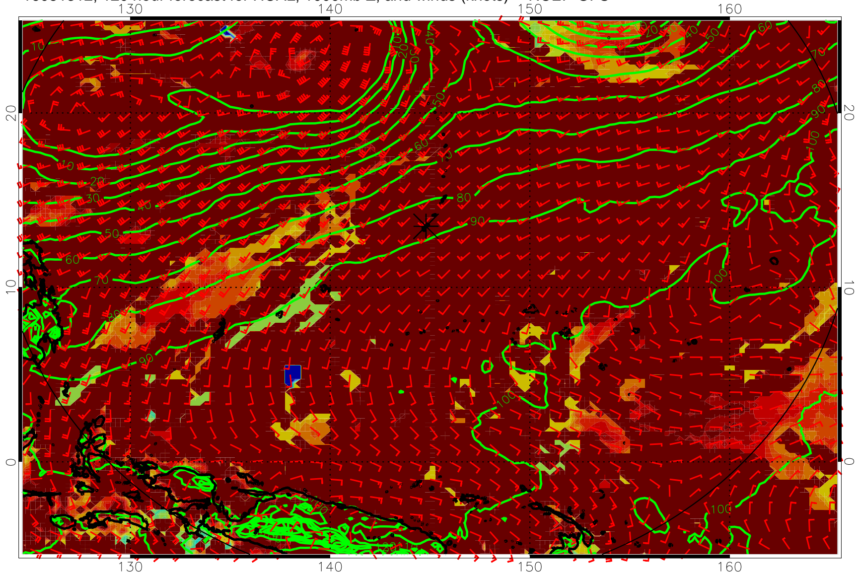
16081312, 120 hour forecast for HCAL, 1000mb Z, and winds (knots) -- NCEP GFS
