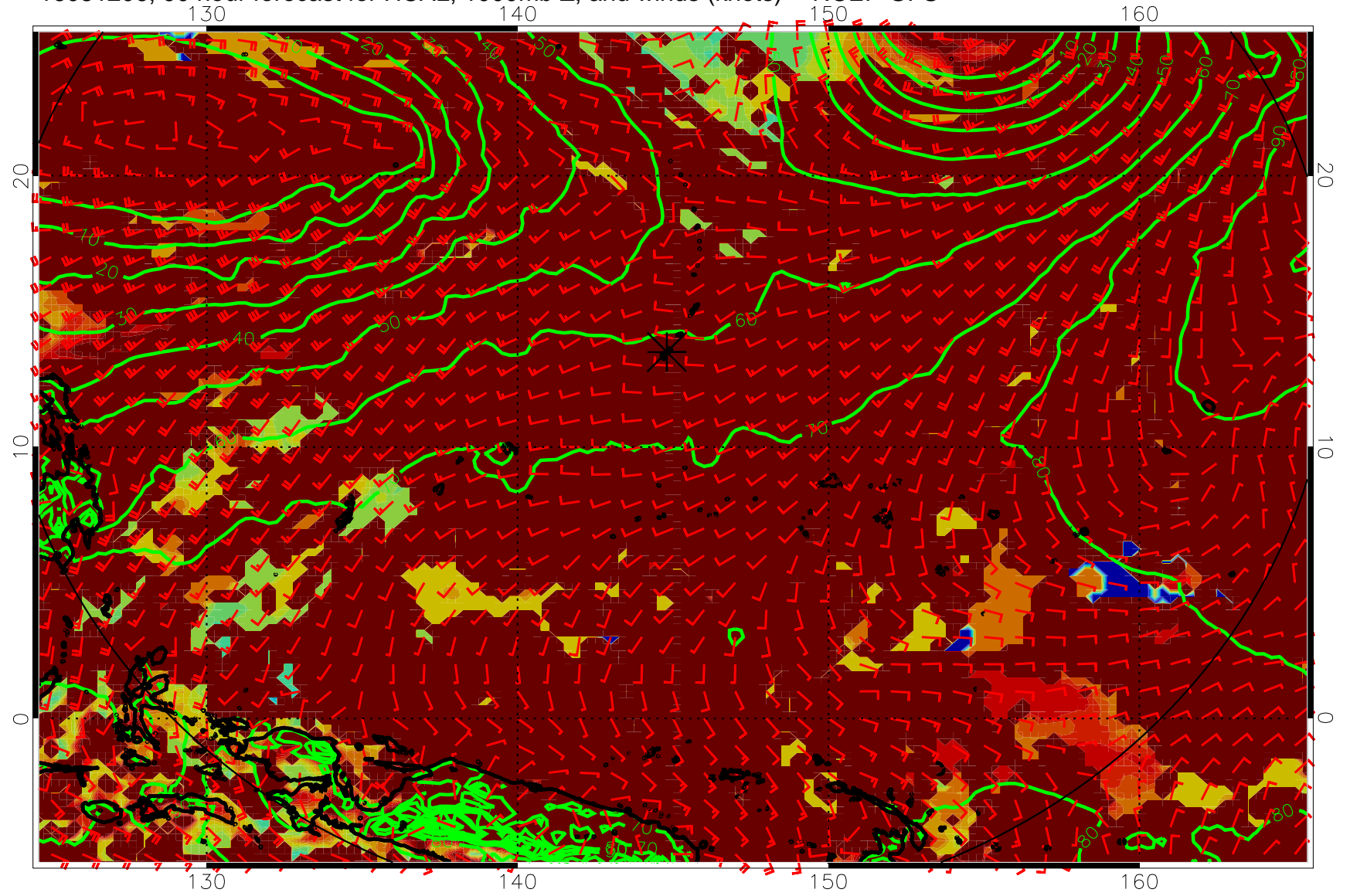
16081206, 90 hour forecast for HCAL, 1000mb Z, and winds (knots) -- NCEP GFS
