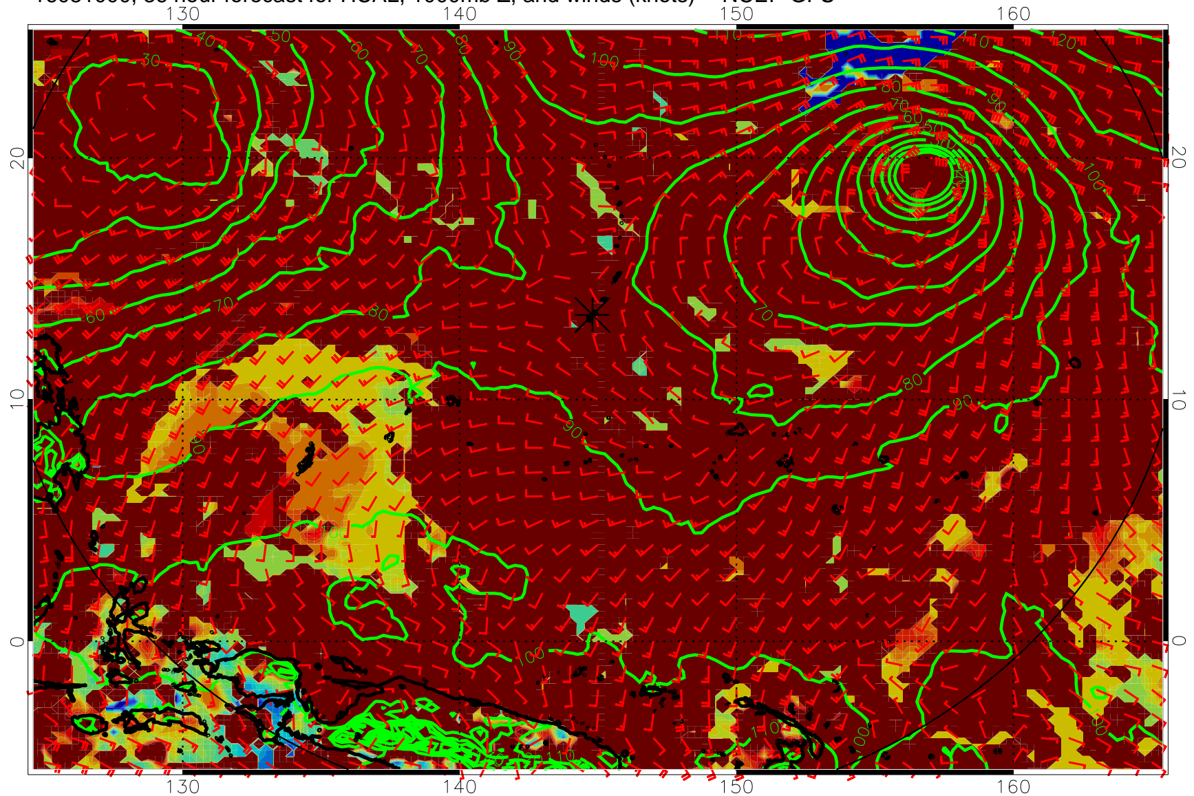
16081000, 36 hour forecast for HCAL, 1000mb Z, and winds (knots) -- NCEP GFS
