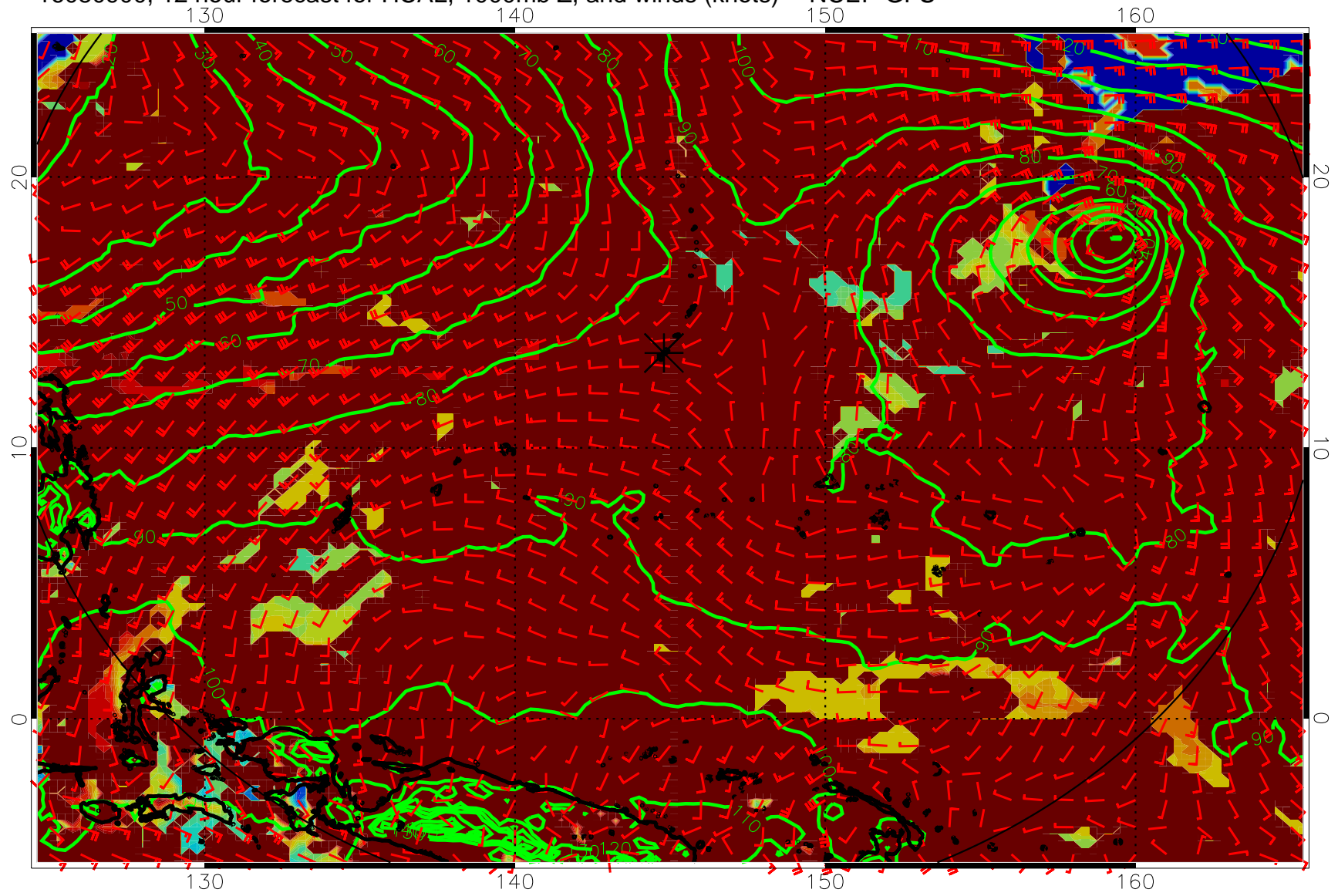
16080900, 12 hour forecast for HCAL, 1000mb Z, and winds (knots) -- NCEP GFS
