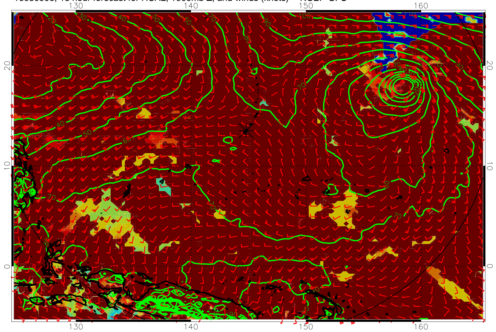
16080906, 18 hour forecast for HCAL, 1000mb Z, and winds (knots) -- NCEP GFS
