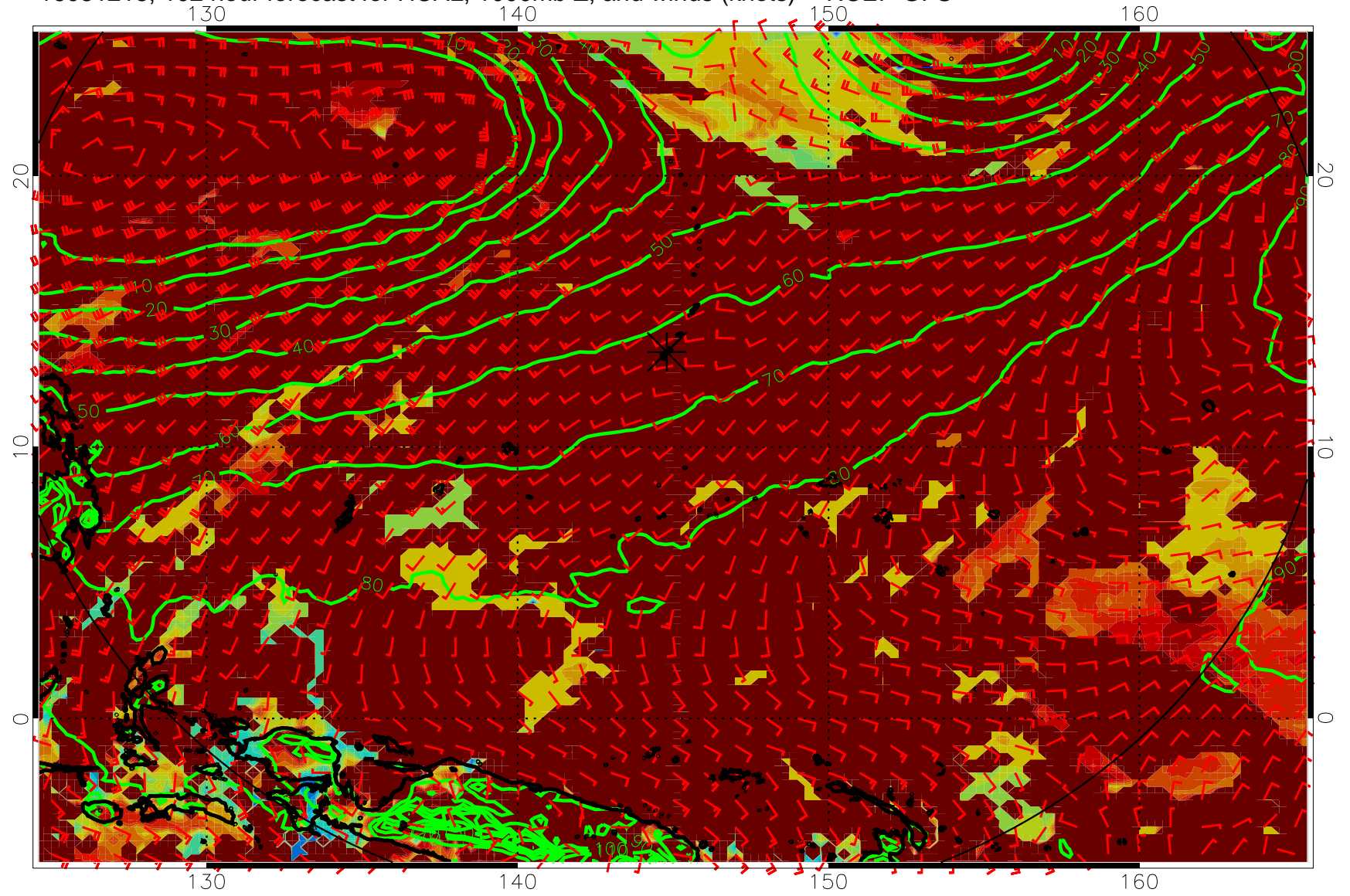
16081218, 102 hour forecast for HCAL, 1000mb Z, and winds (knots) -- NCEP GFS
