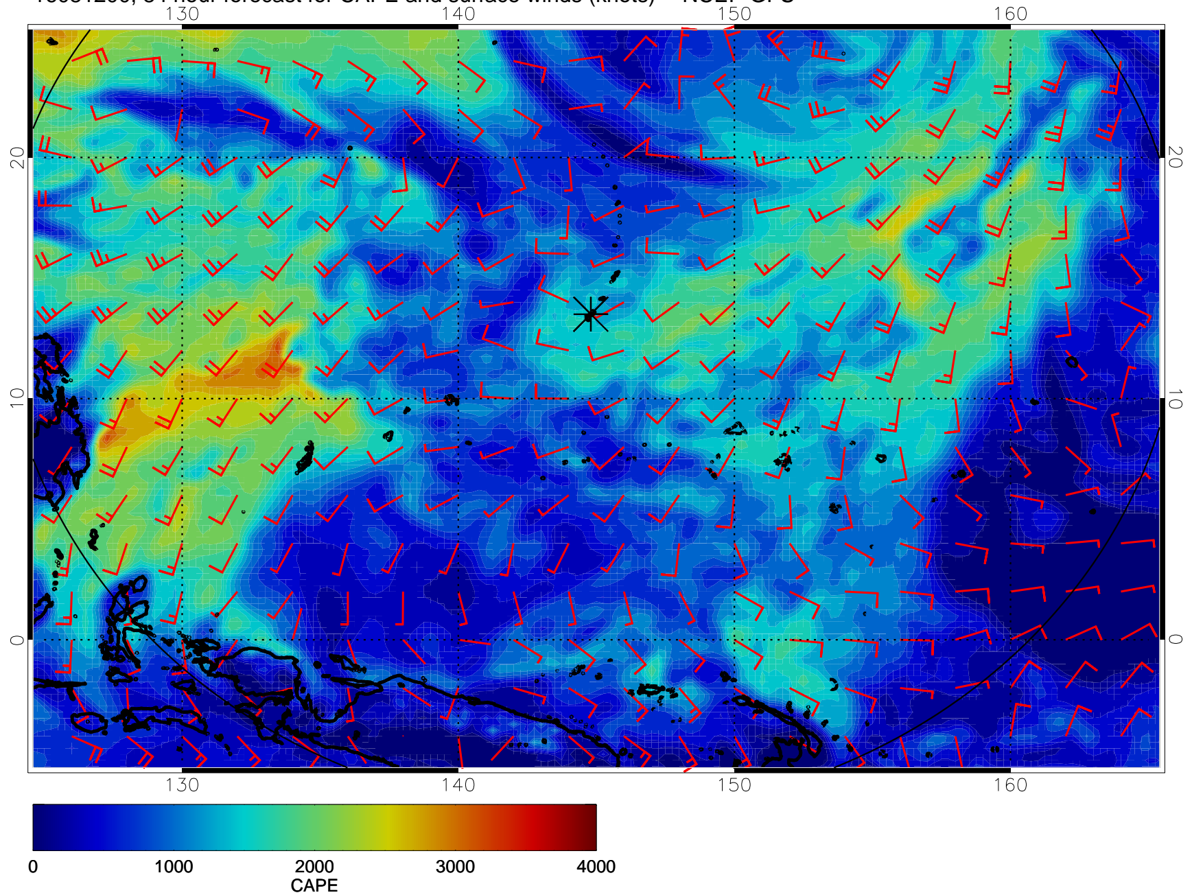
16081200, 84 hour forecast for CAPE and surface winds (knots) -- NCEP GFS
