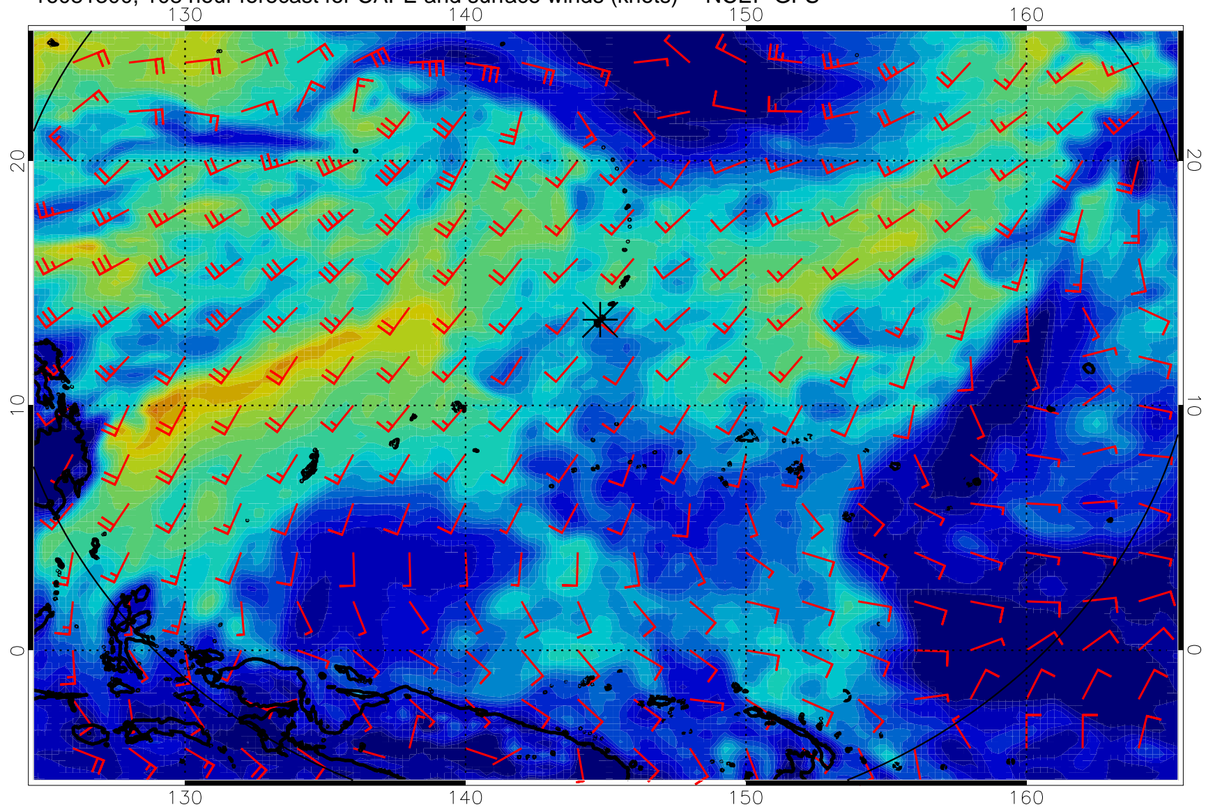
16081300, 108 hour forecast for CAPE and surface winds (knots) -- NCEP GFS
