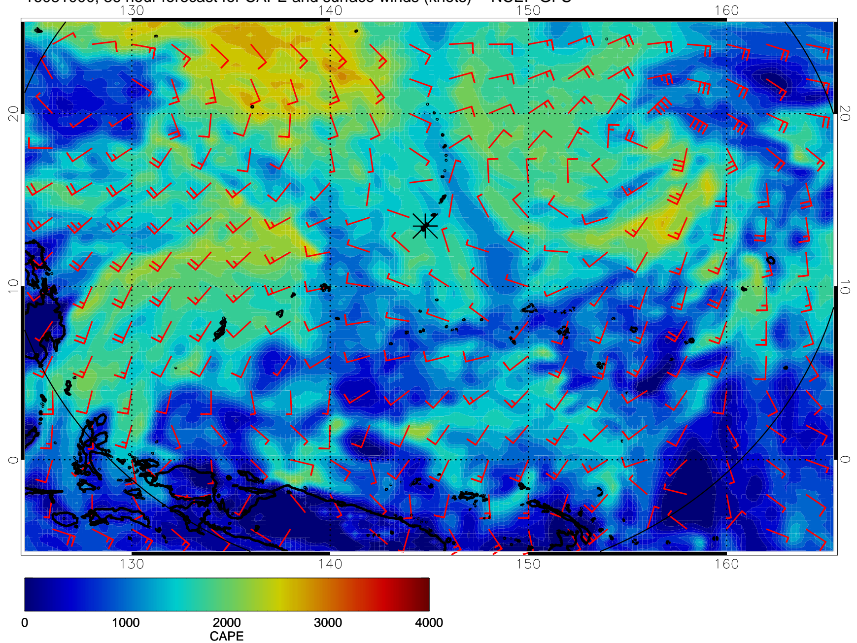
16081000, 36 hour forecast for CAPE and surface winds (knots) -- NCEP GFS
