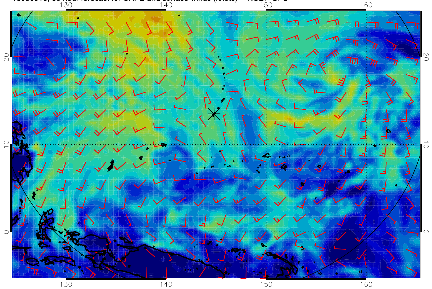
16080918, 30 hour forecast for CAPE and surface winds (knots) -- NCEP GFS
