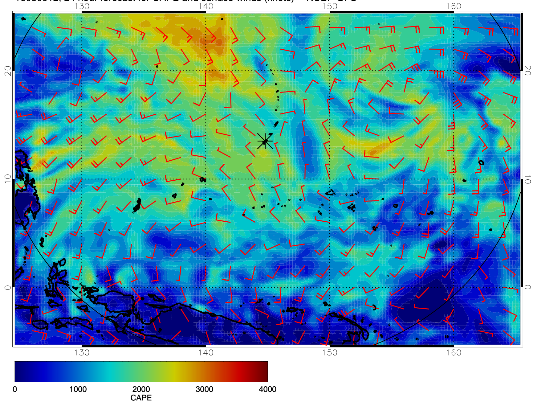
16080912, 24 hour forecast for CAPE and surface winds (knots) -- NCEP GFS
