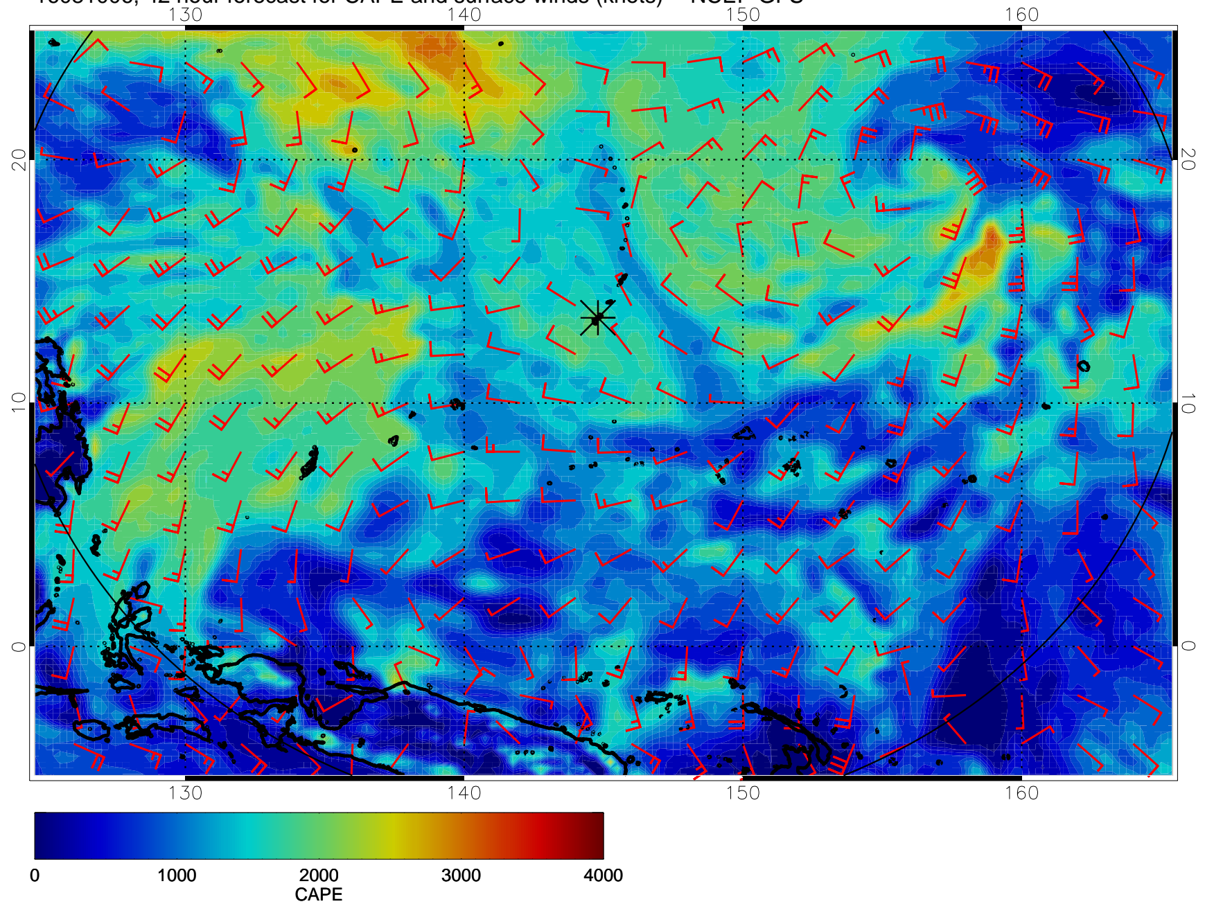
16081006, 42 hour forecast for CAPE and surface winds (knots) -- NCEP GFS
