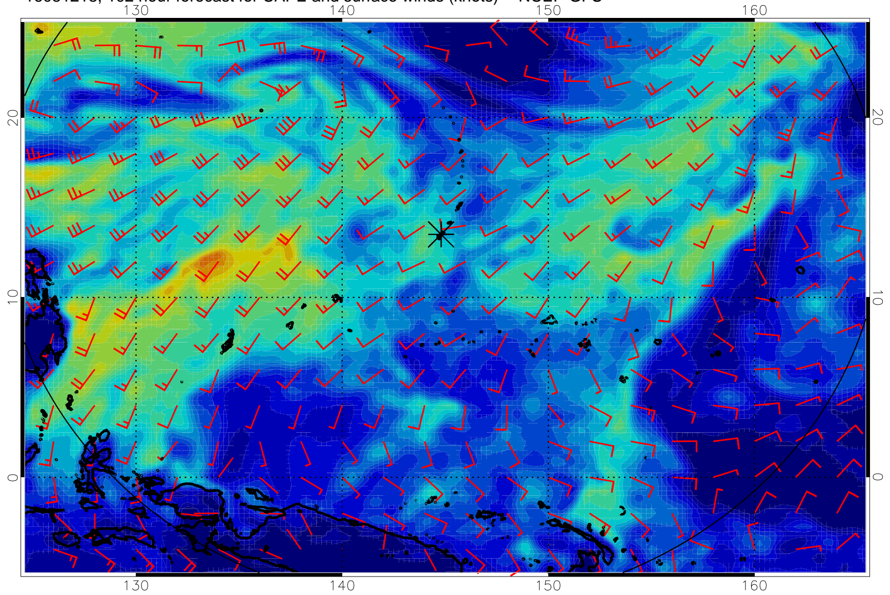
16081218, 102 hour forecast for CAPE and surface winds (knots) -- NCEP GFS
