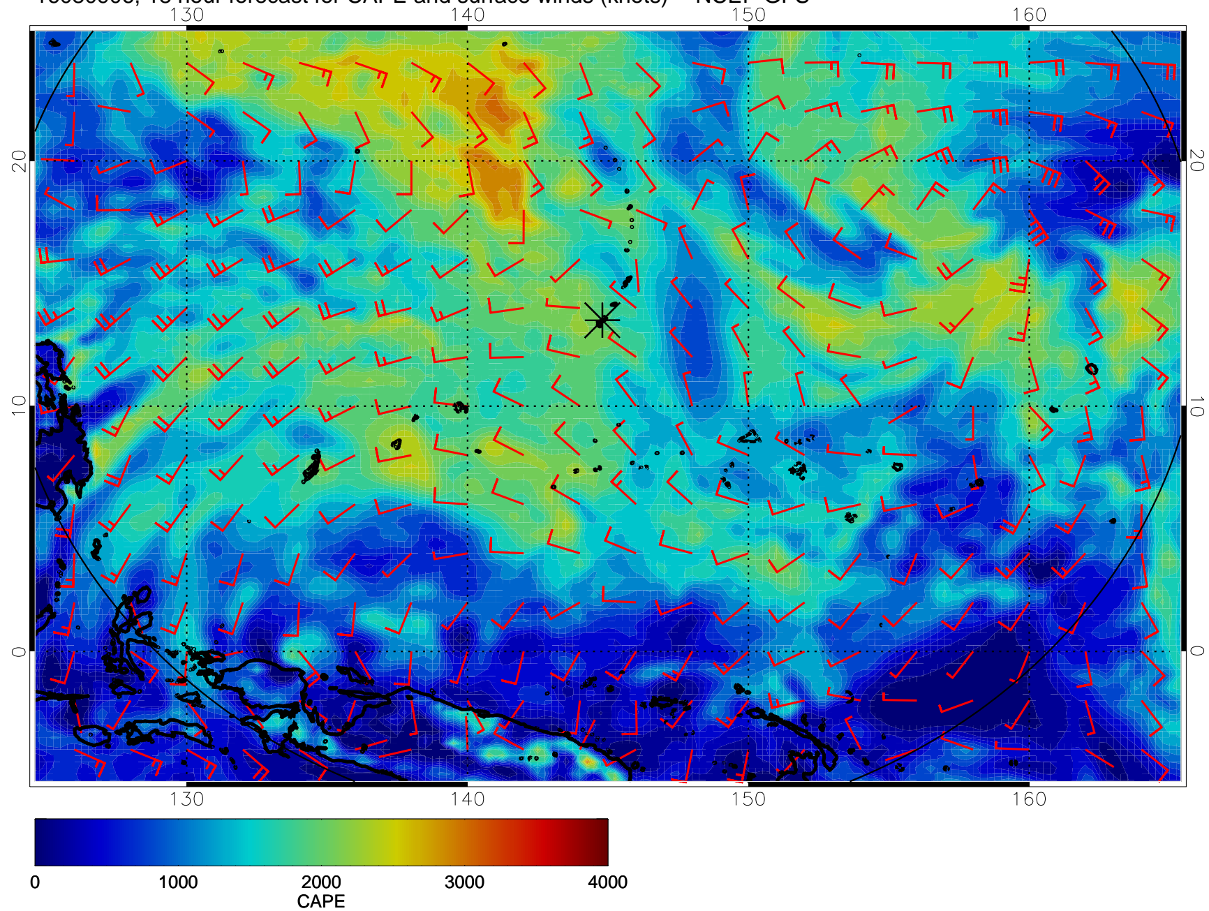
16080906, 18 hour forecast for CAPE and surface winds (knots) -- NCEP GFS
