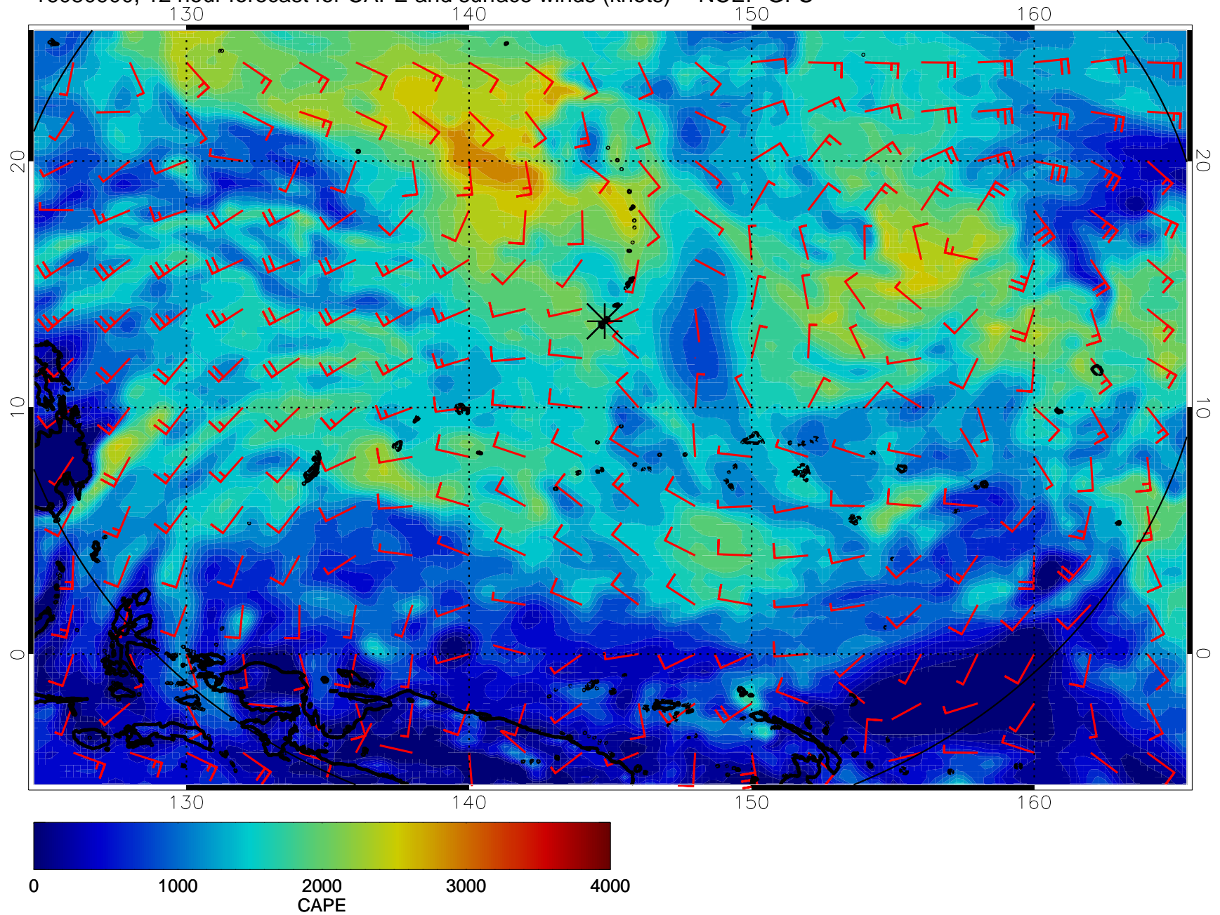
16080900, 12 hour forecast for CAPE and surface winds (knots) -- NCEP GFS
