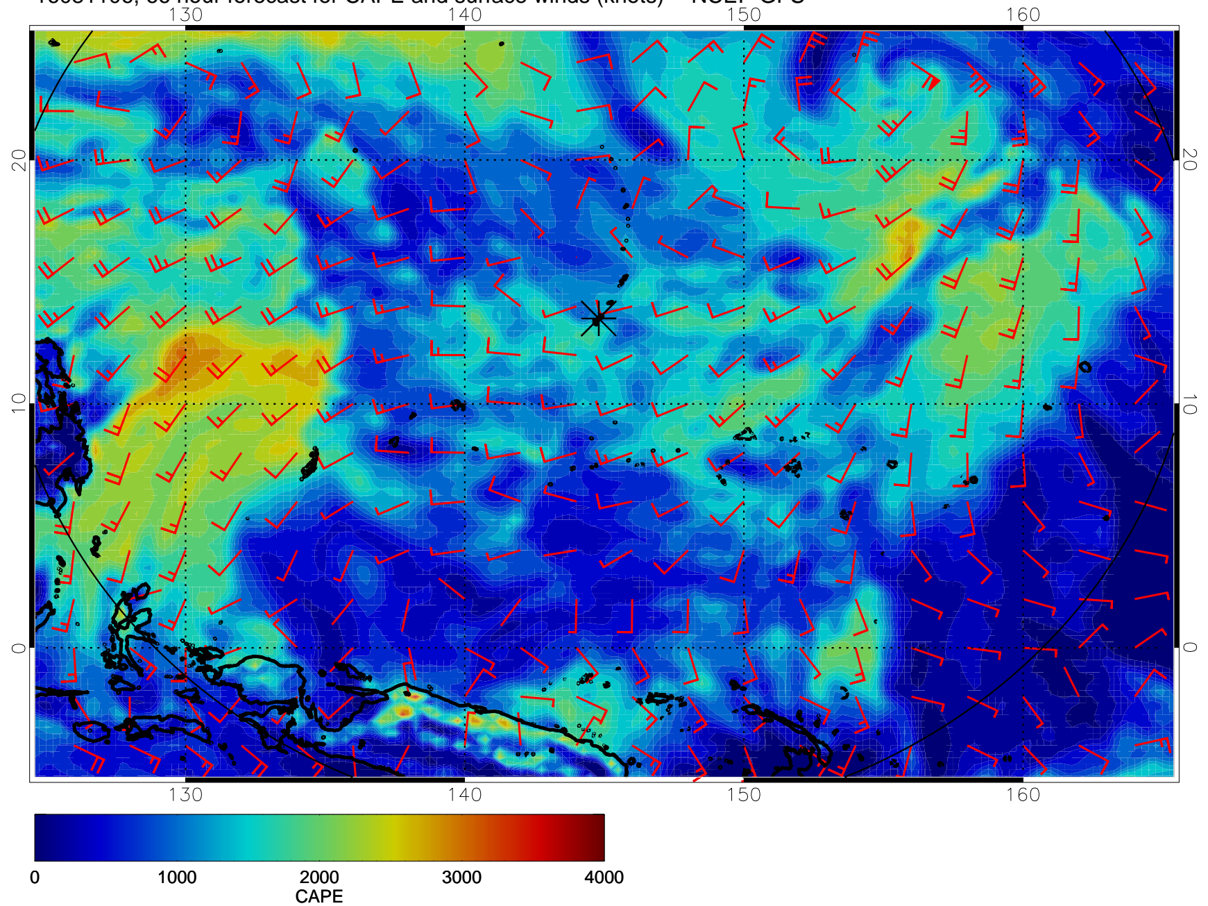
16081106, 66 hour forecast for CAPE and surface winds (knots) -- NCEP GFS
