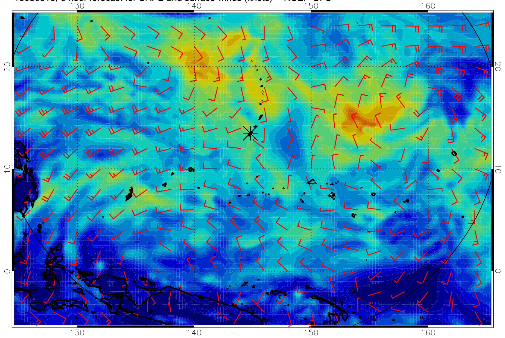
16080818, 6 hour forecast for CAPE and surface winds (knots) -- NCEP GFS
