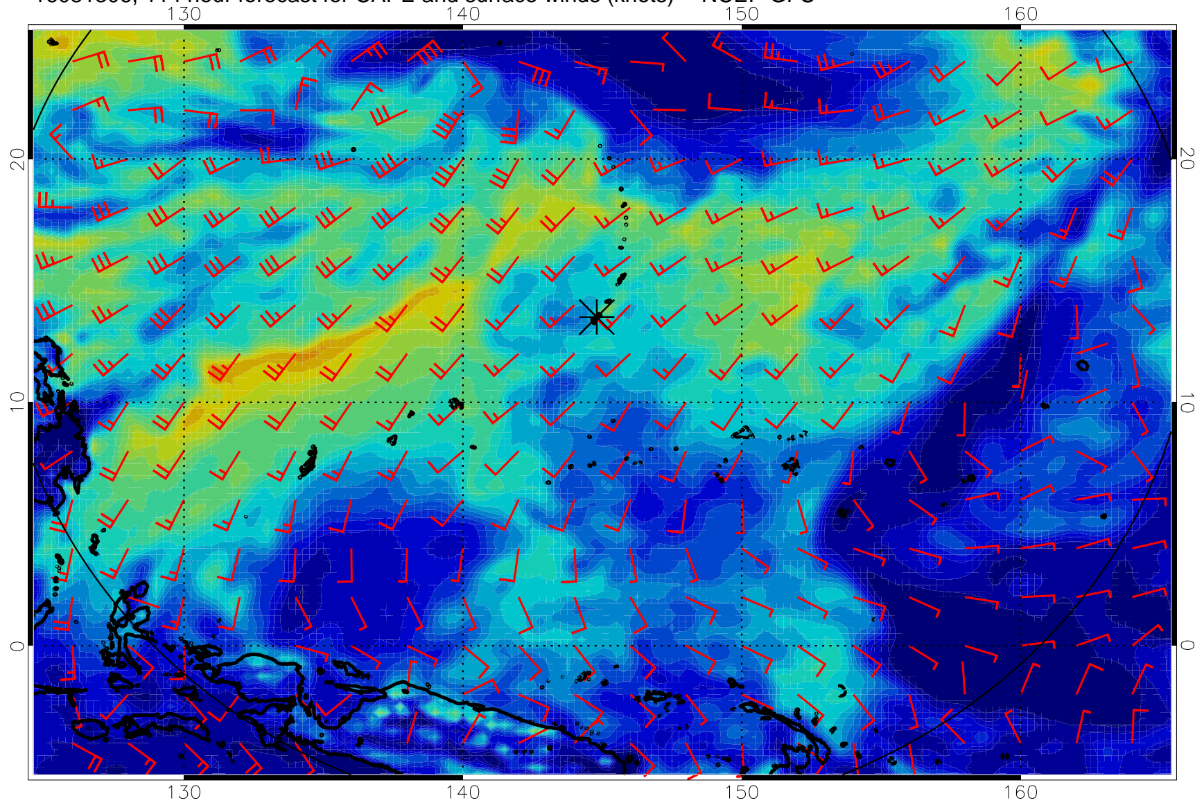
16081306, 114 hour forecast for CAPE and surface winds (knots) -- NCEP GFS
