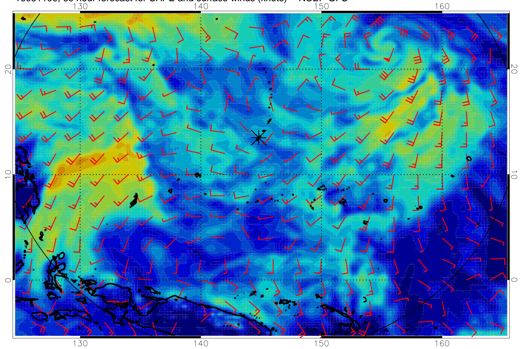
16081100, 60 hour forecast for CAPE and surface winds (knots) -- NCEP GFS
