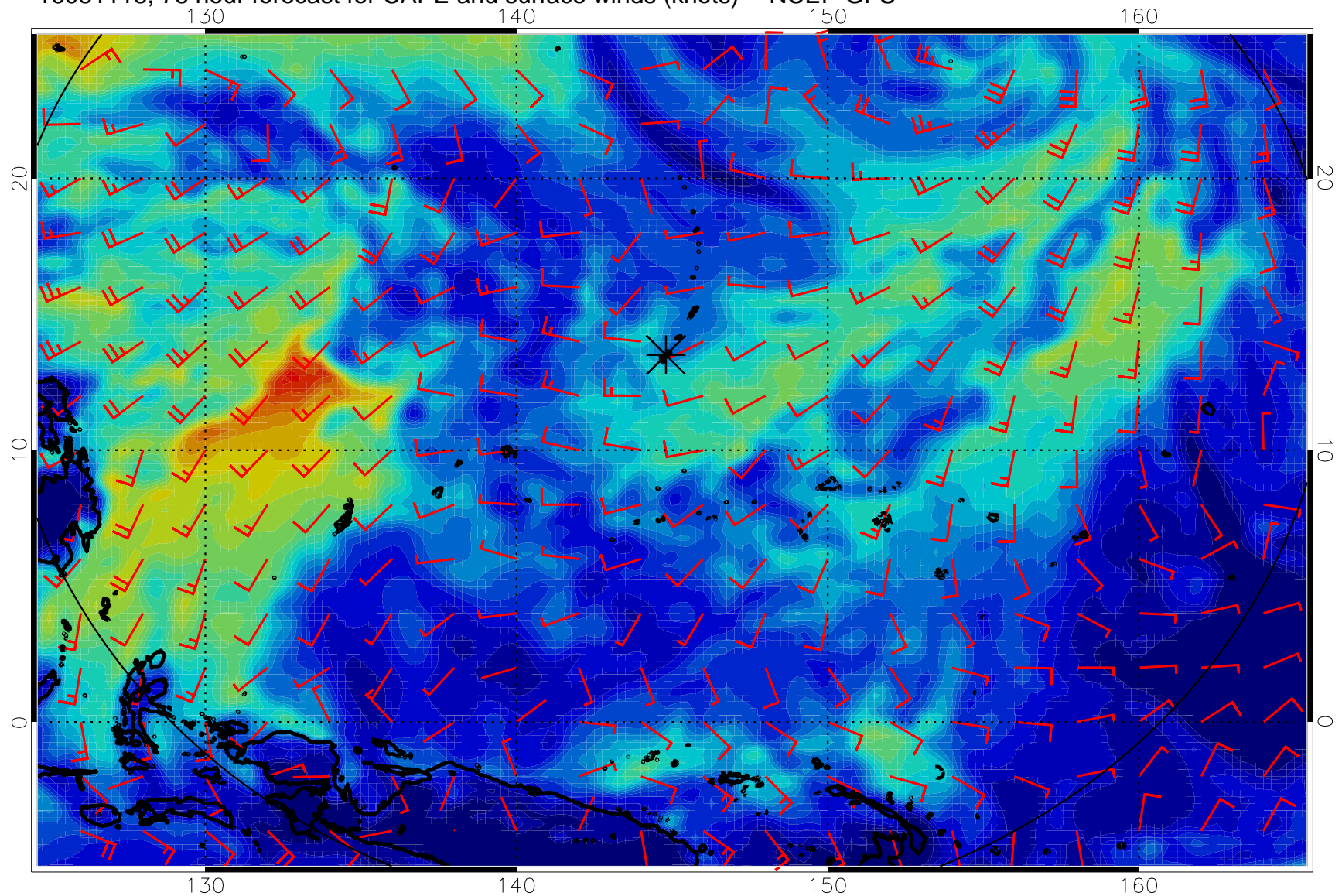
16081118, 78 hour forecast for CAPE and surface winds (knots) -- NCEP GFS
