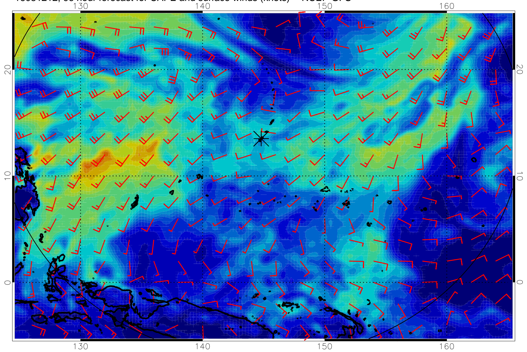
16081212, 96 hour forecast for CAPE and surface winds (knots) -- NCEP GFS
