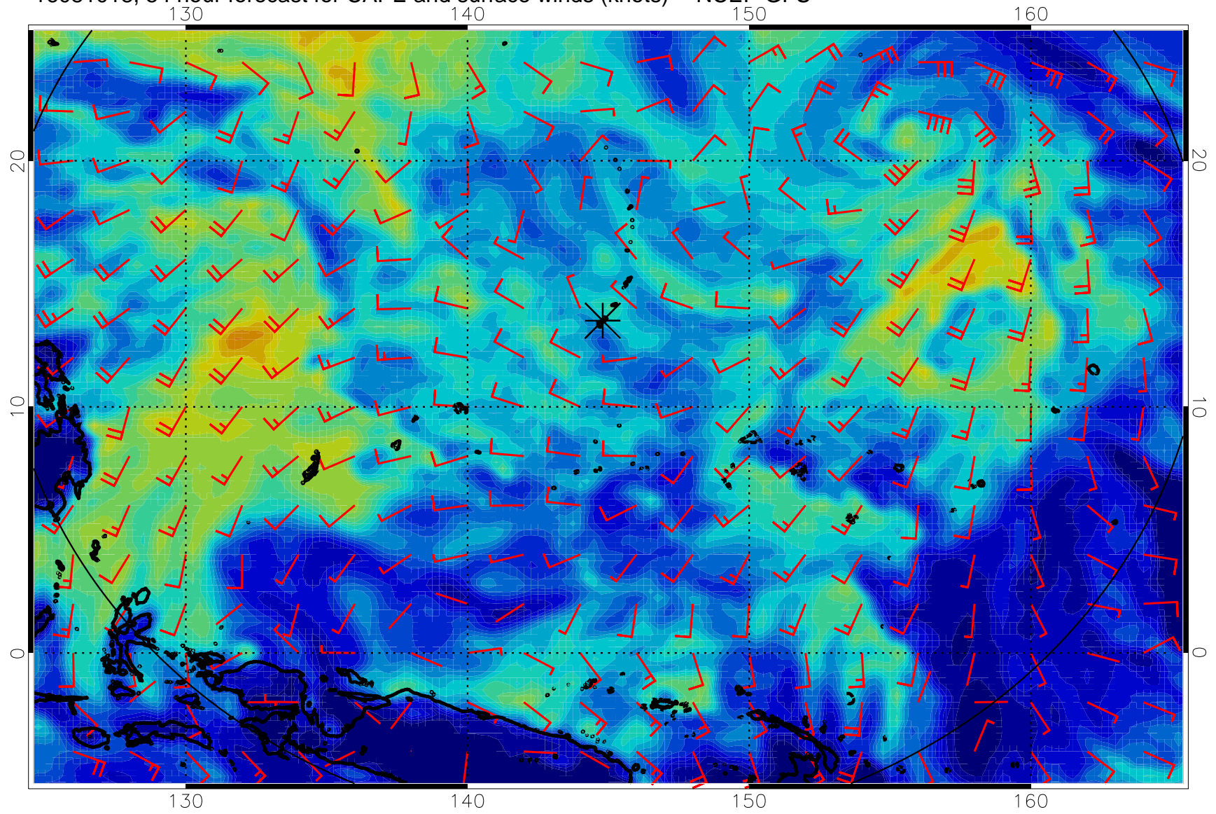
16081018, 54 hour forecast for CAPE and surface winds (knots) -- NCEP GFS
