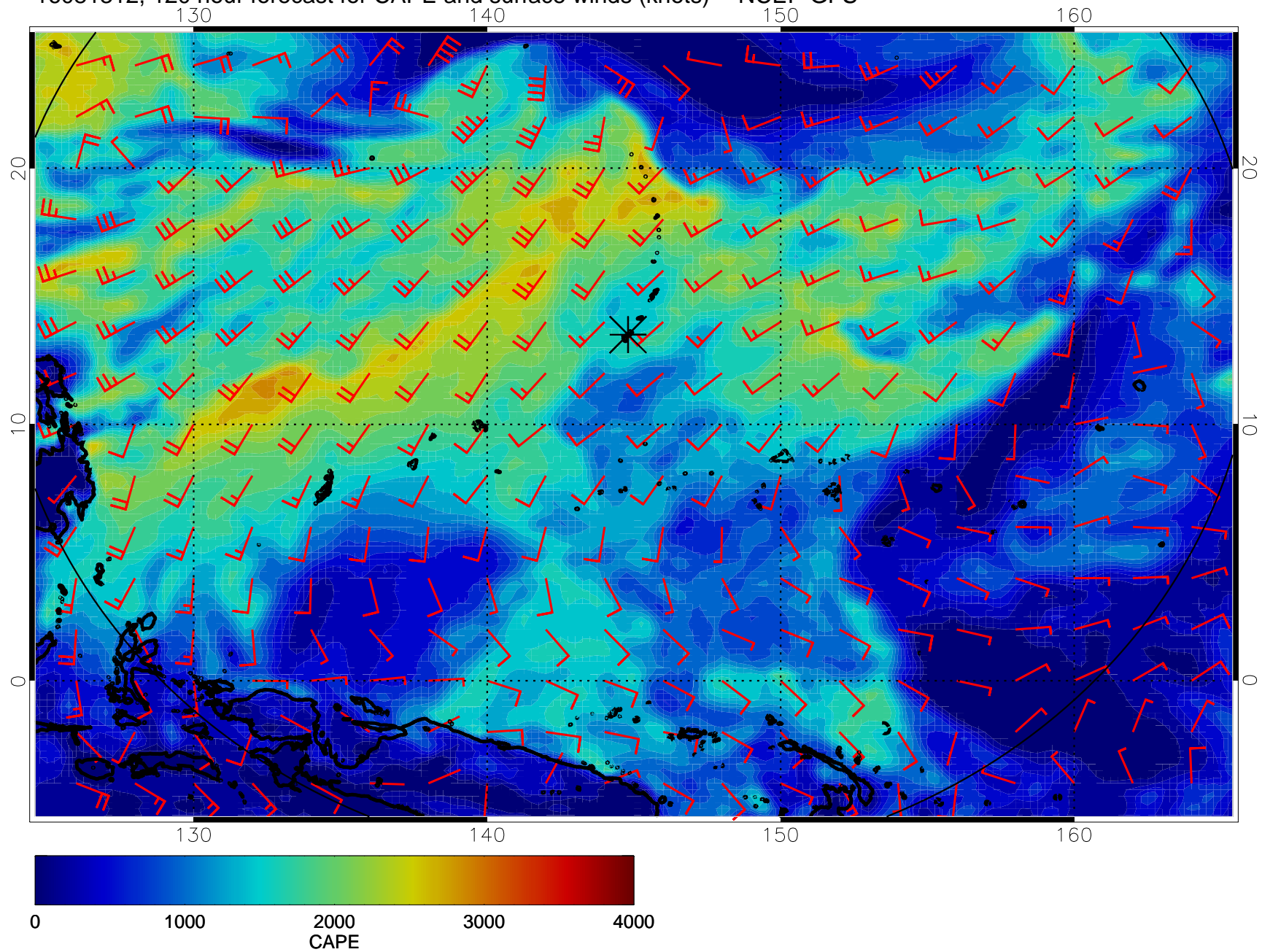
16081312, 120 hour forecast for CAPE and surface winds (knots) -- NCEP GFS
