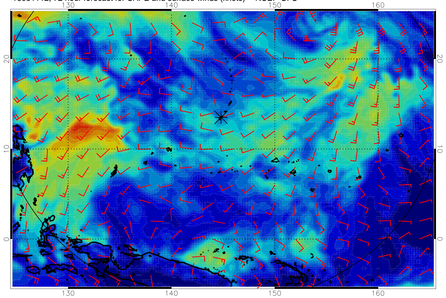
16081112, 72 hour forecast for CAPE and surface winds (knots) -- NCEP GFS
