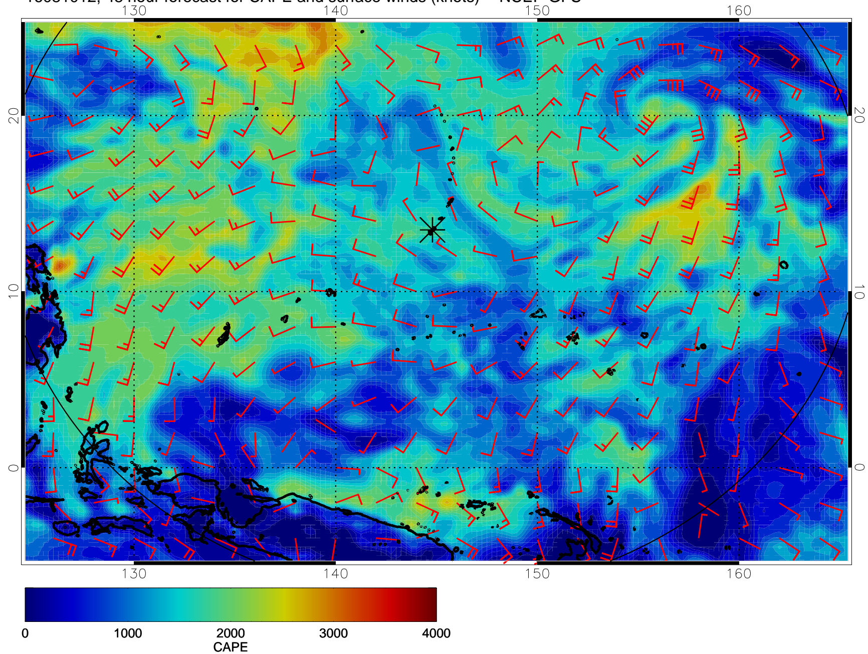
16081012, 48 hour forecast for CAPE and surface winds (knots) -- NCEP GFS
