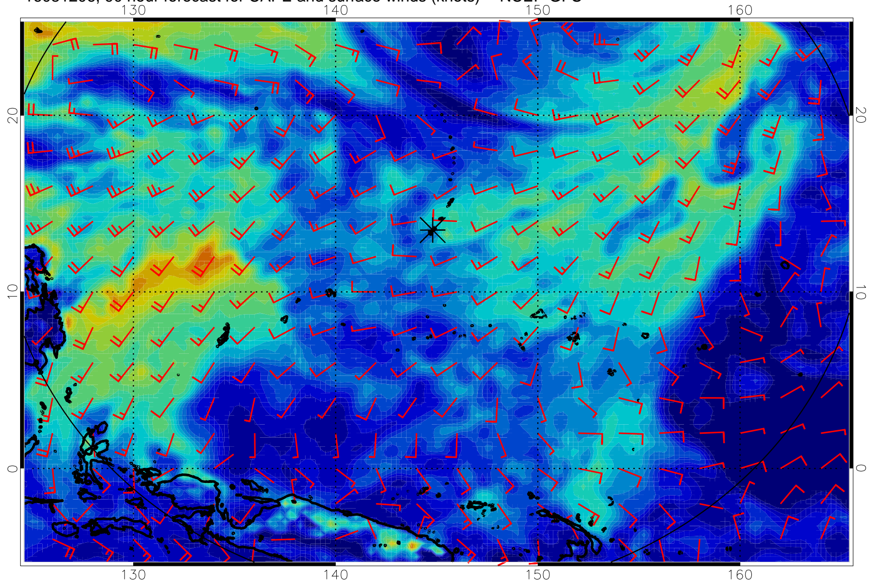
16081206, 90 hour forecast for CAPE and surface winds (knots) -- NCEP GFS
