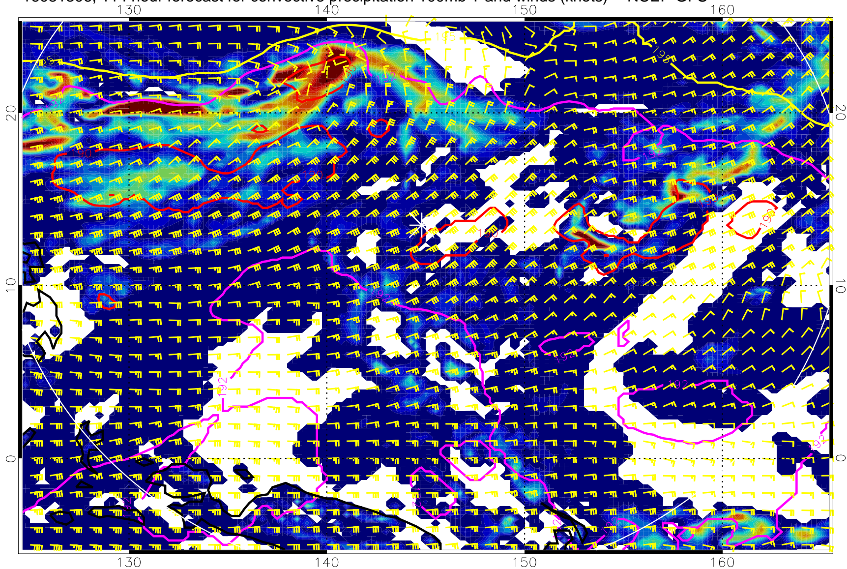
16081306, 114 hour forecast for convective precipitation 100mb T and winds (knots) -- NCEP GFS
