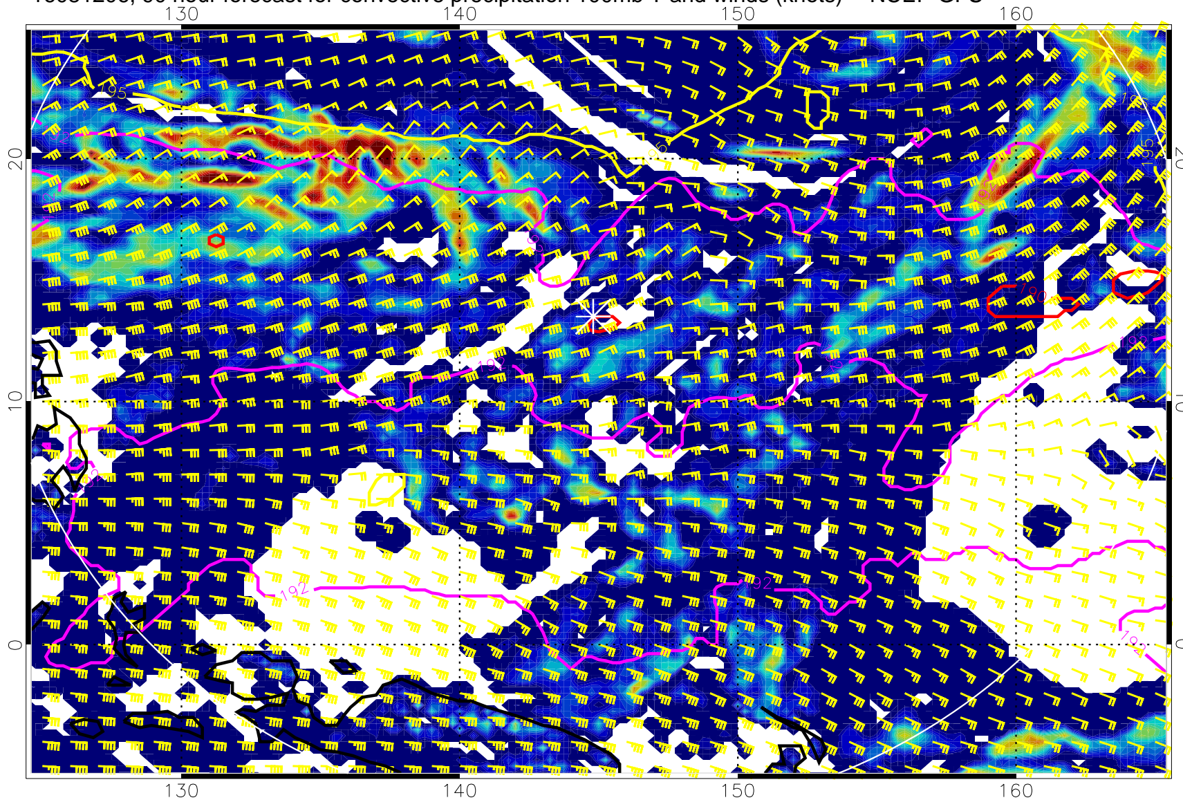
16081206, 90 hour forecast for convective precipitation 100mb T and winds (knots) -- NCEP GFS
