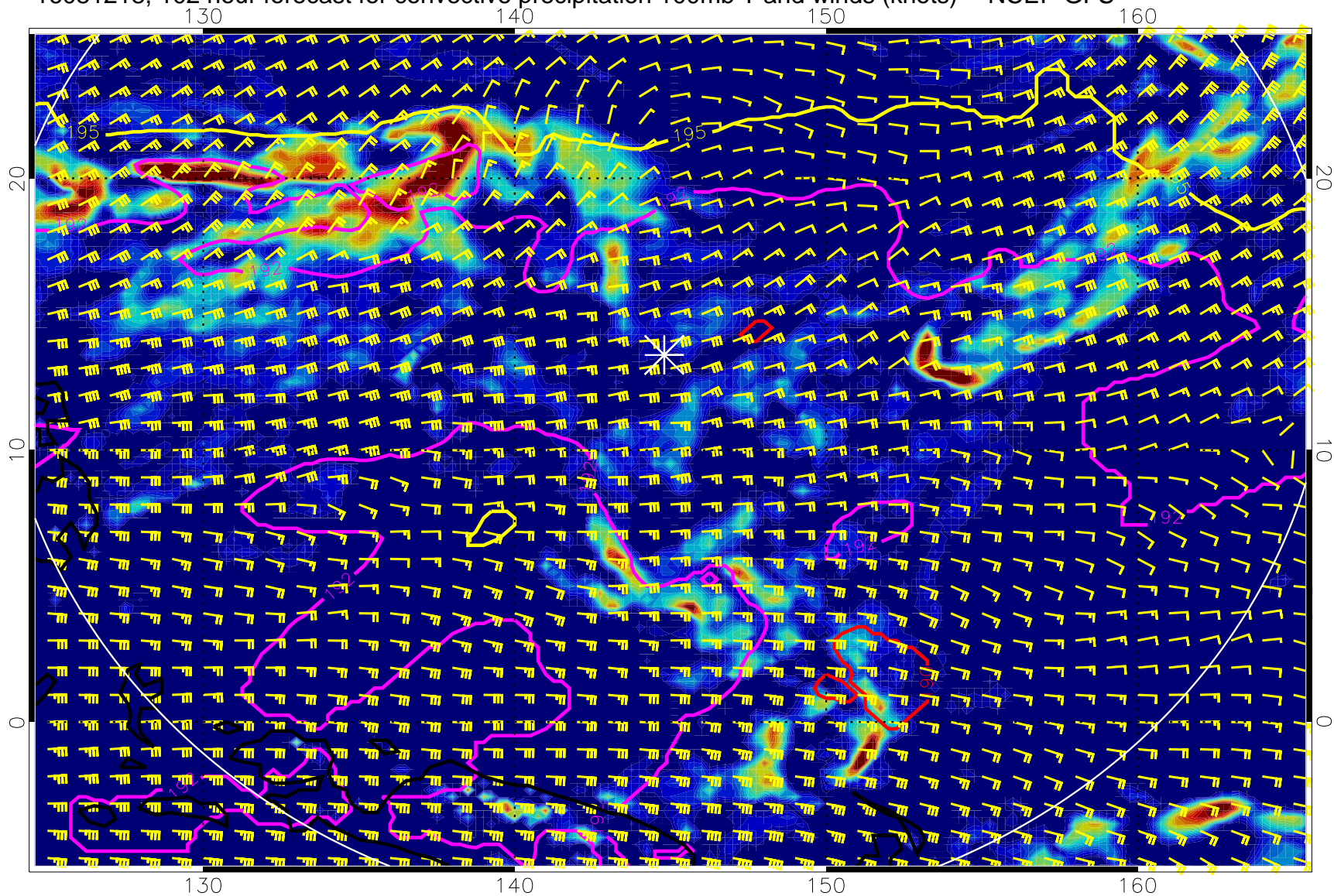
16081218, 102 hour forecast for convective precipitation 100mb T and winds (knots) -- NCEP GFS
