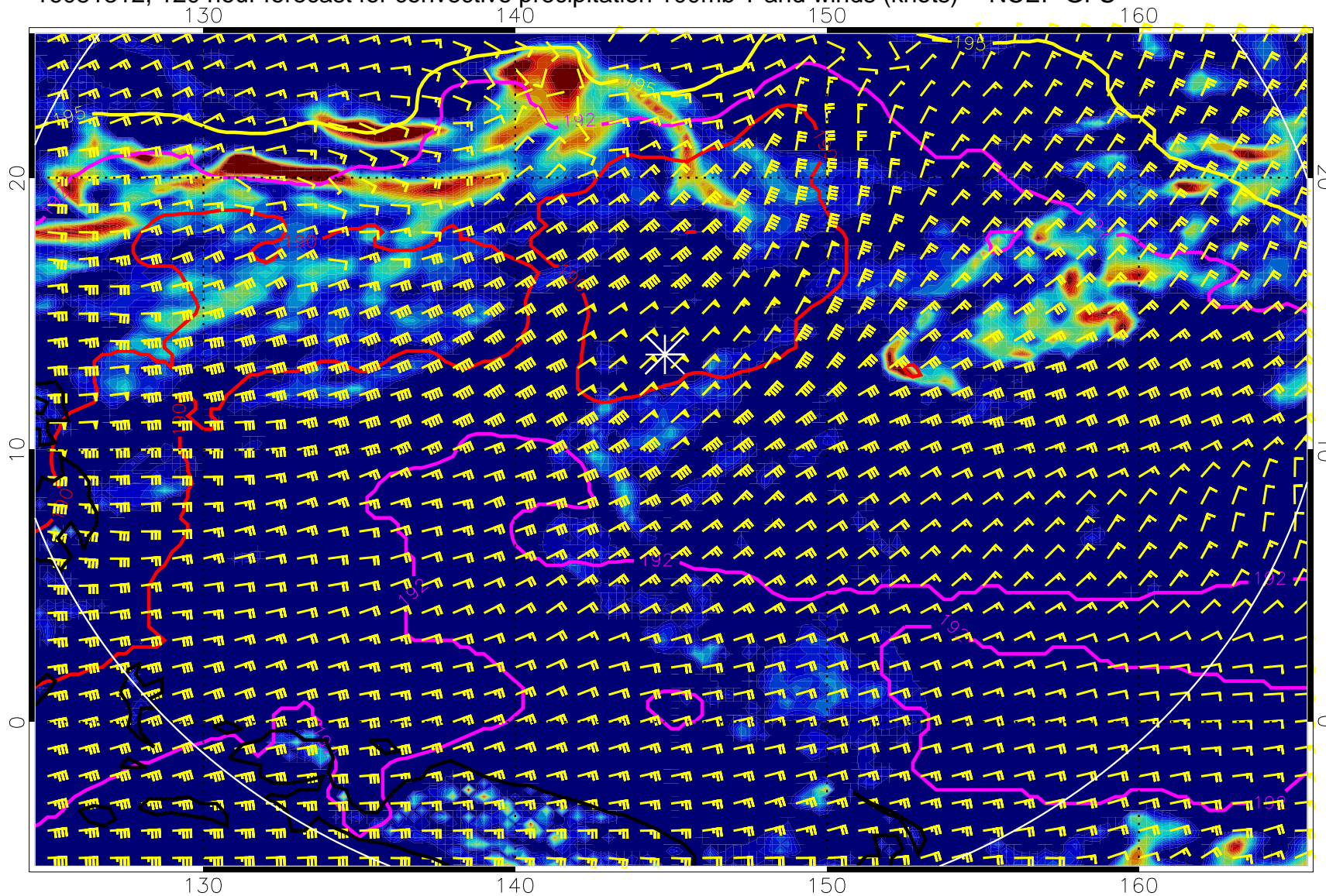
16081312, 120 hour forecast for convective precipitation 100mb T and winds (knots) -- NCEP GFS
