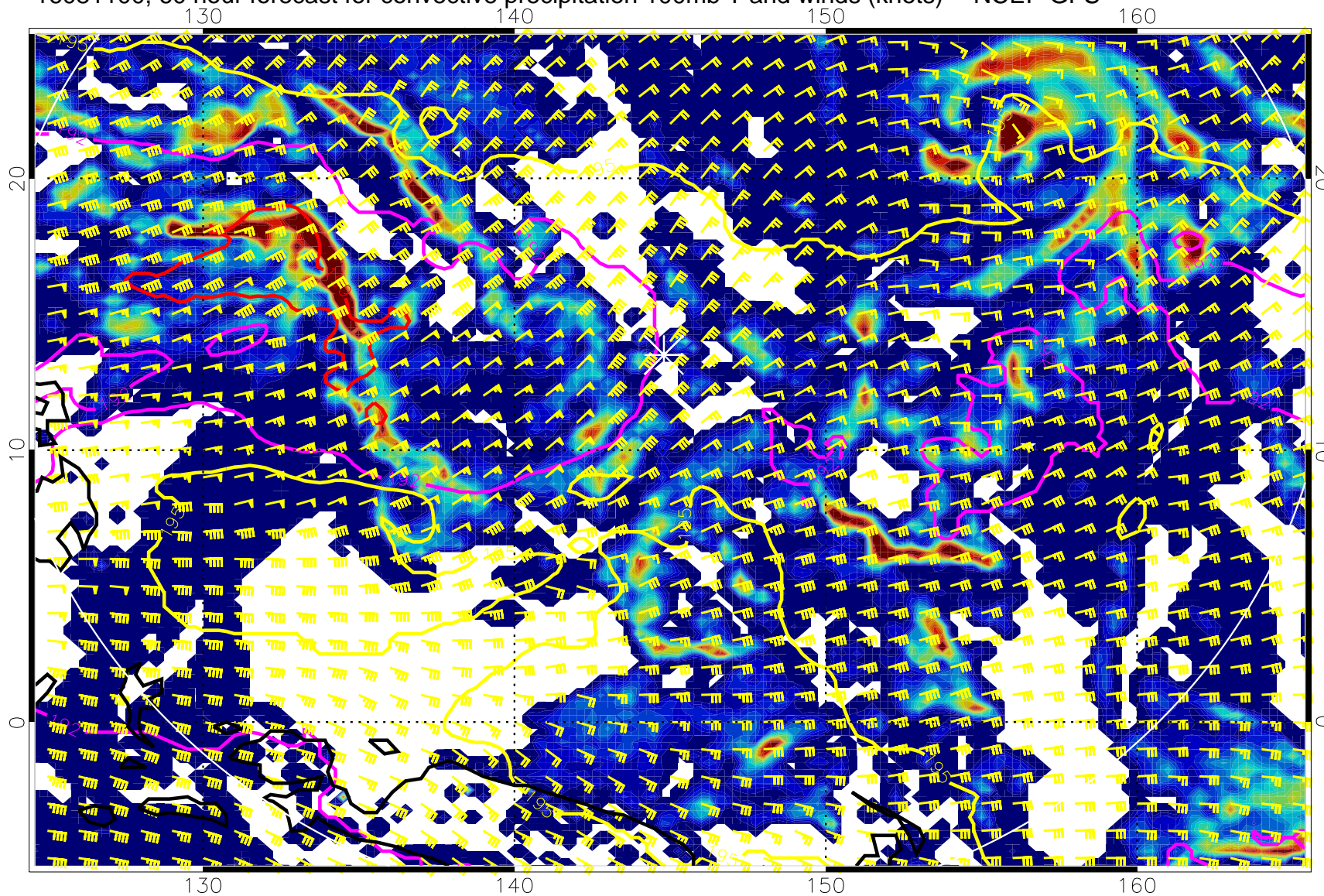
16081100, 60 hour forecast for convective precipitation 100mb T and winds (knots) -- NCEP GFS
