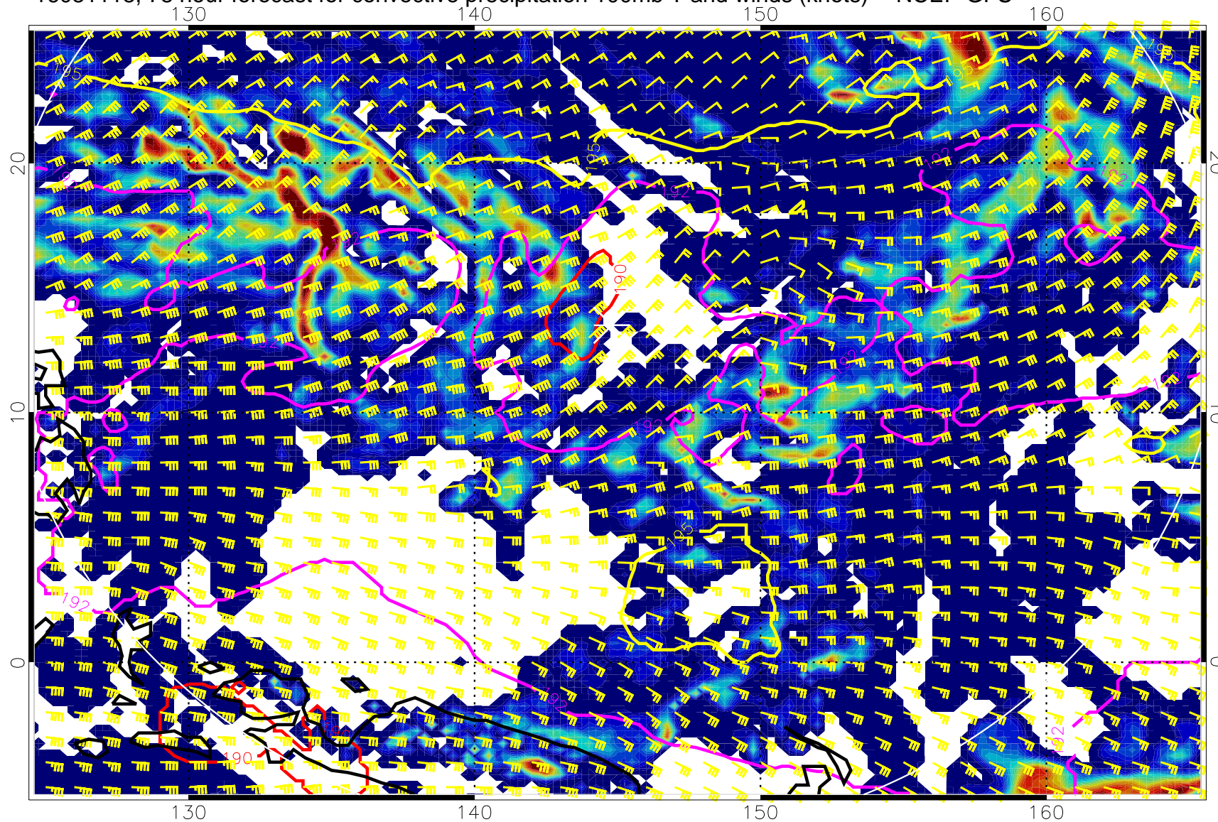
16081118, 78 hour forecast for convective precipitation 100mb T and winds (knots) -- NCEP GFS
