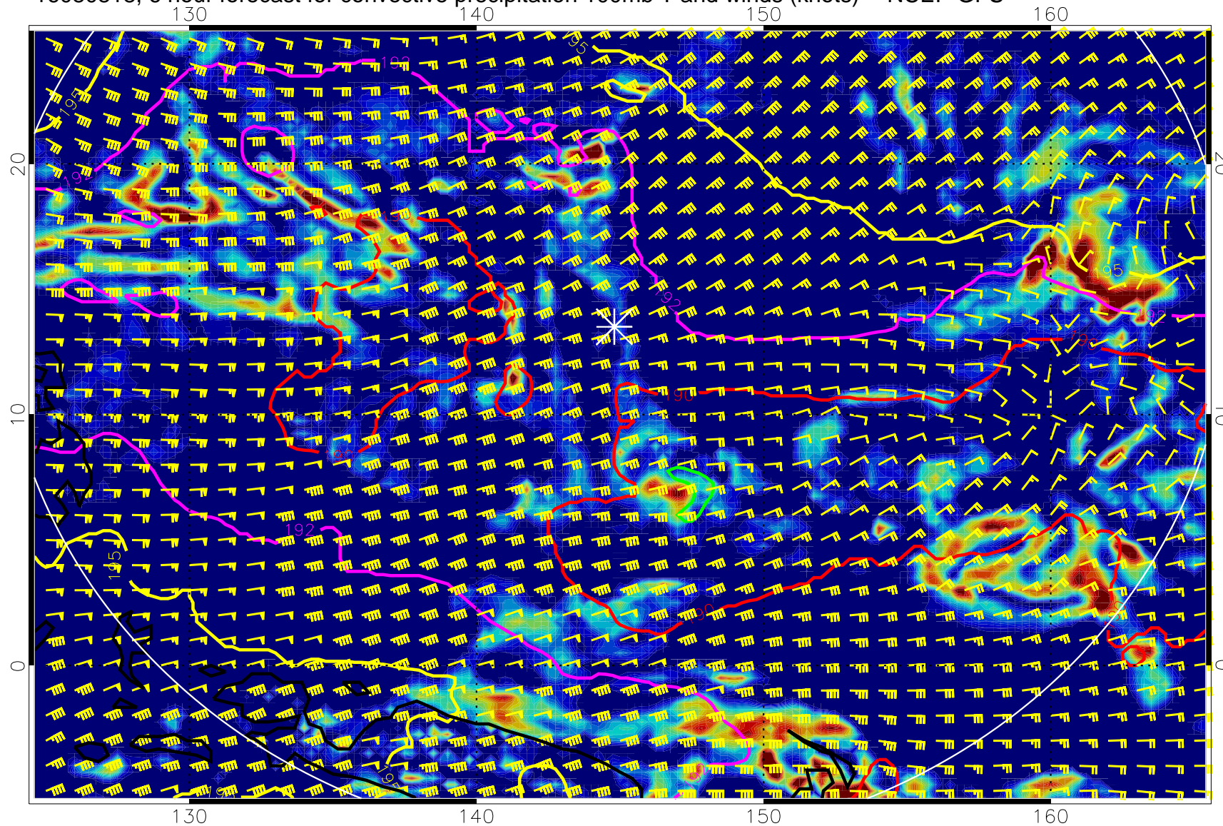
16080818, 6 hour forecast for convective precipitation 100mb T and winds (knots) -- NCEP GFS
