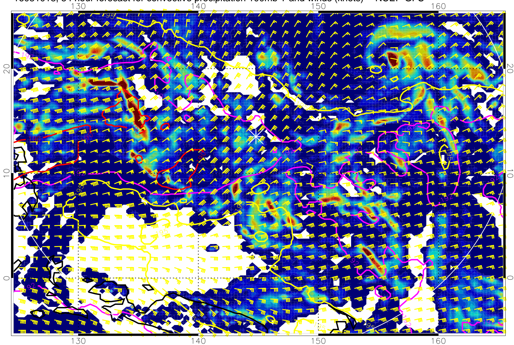
16081018, 54 hour forecast for convective precipitation 100mb T and winds (knots) -- NCEP GFS
