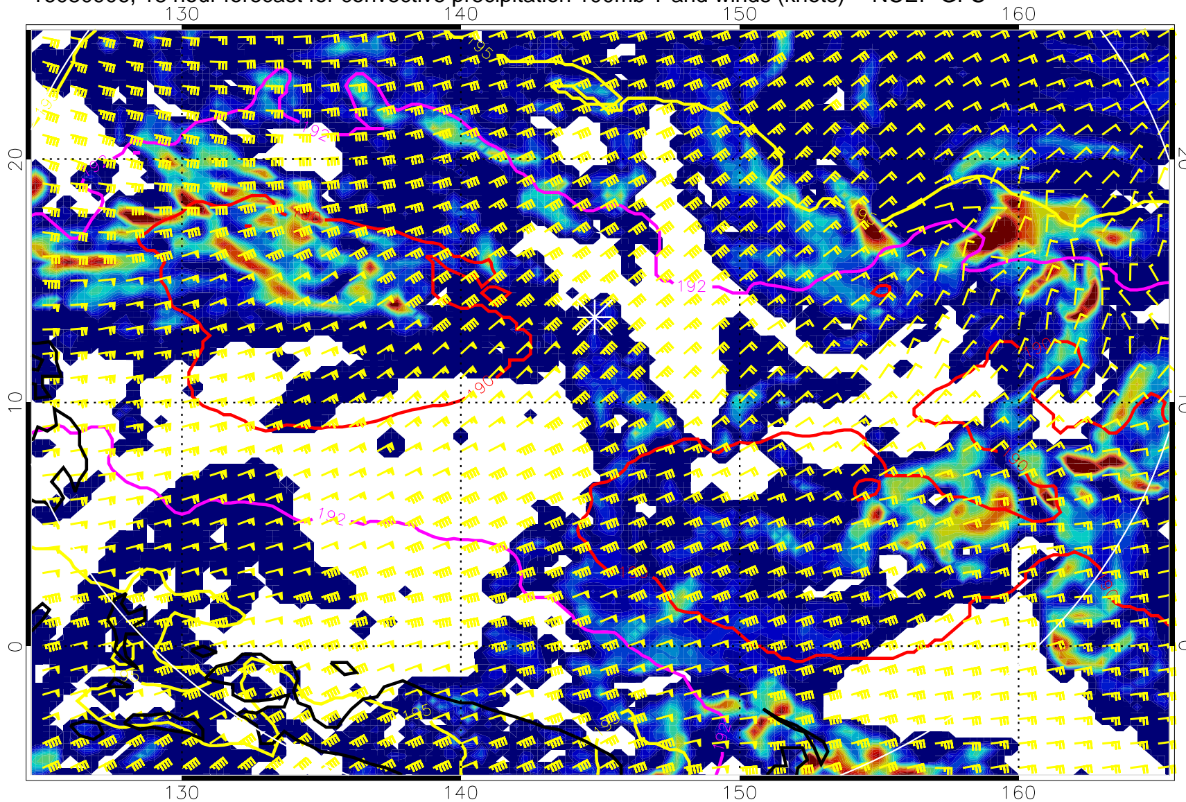
16080906, 18 hour forecast for convective precipitation 100mb T and winds (knots) -- NCEP GFS
