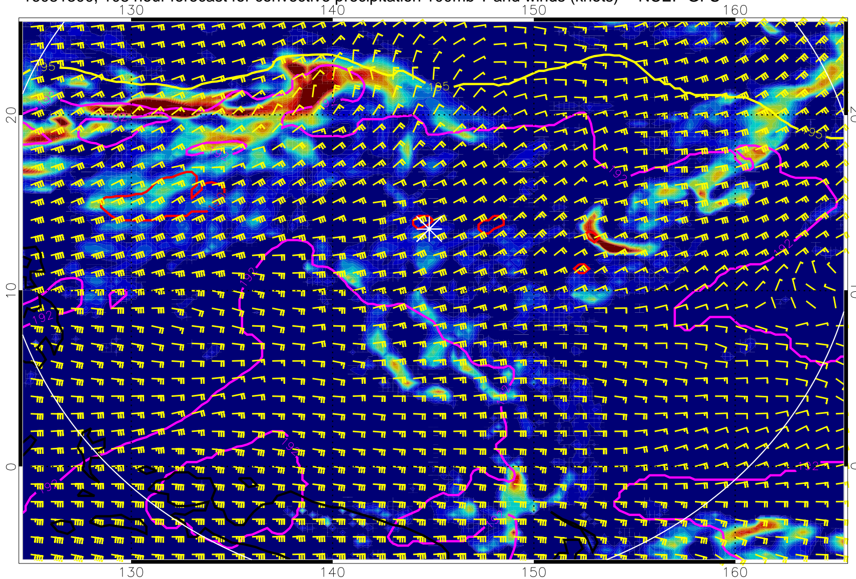
16081300, 108 hour forecast for convective precipitation 100mb T and winds (knots) -- NCEP GFS
