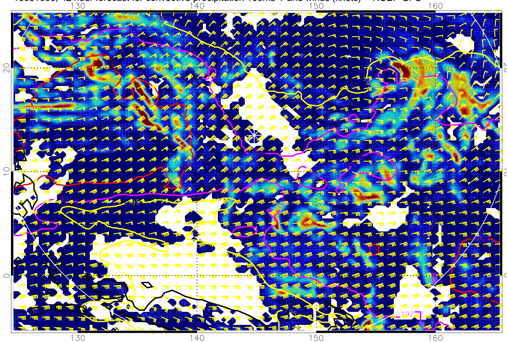
16081006, 42 hour forecast for convective precipitation 100mb T and winds (knots) -- NCEP GFS
