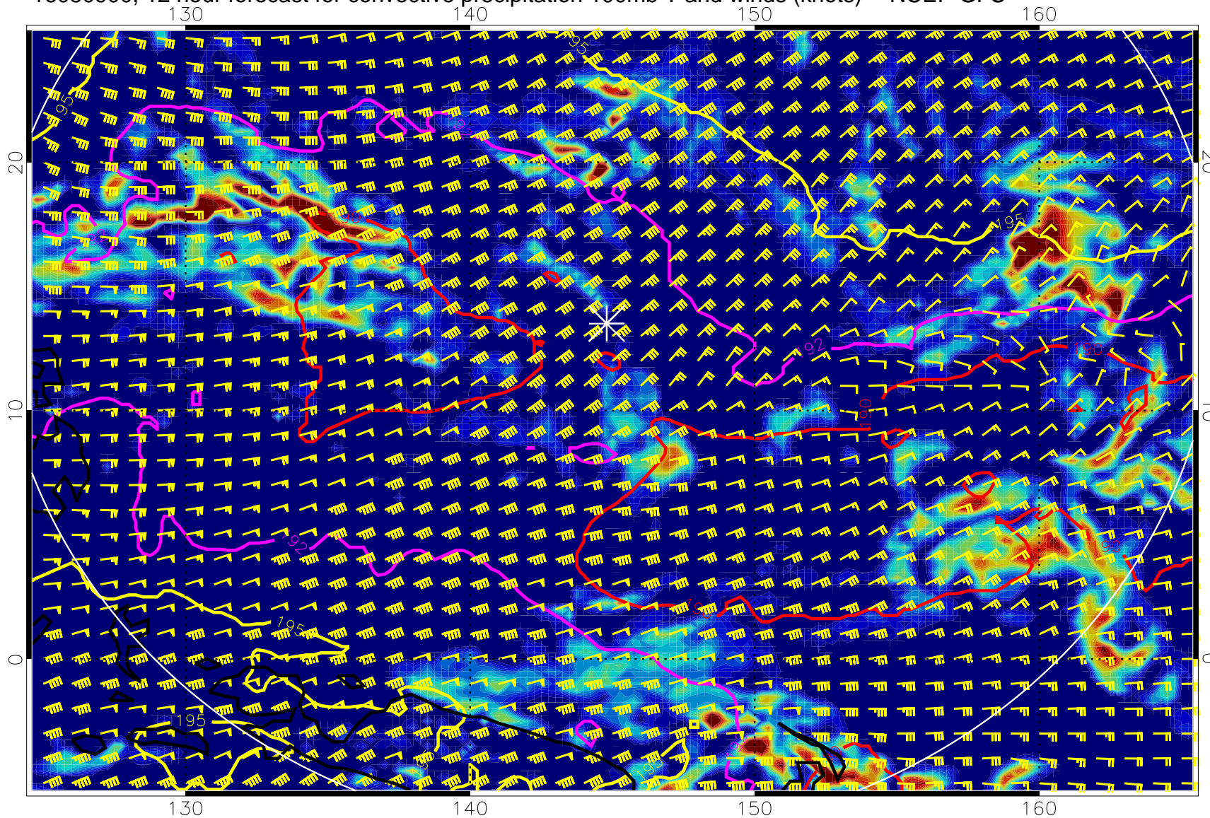
16080900, 12 hour forecast for convective precipitation 100mb T and winds (knots) -- NCEP GFS
