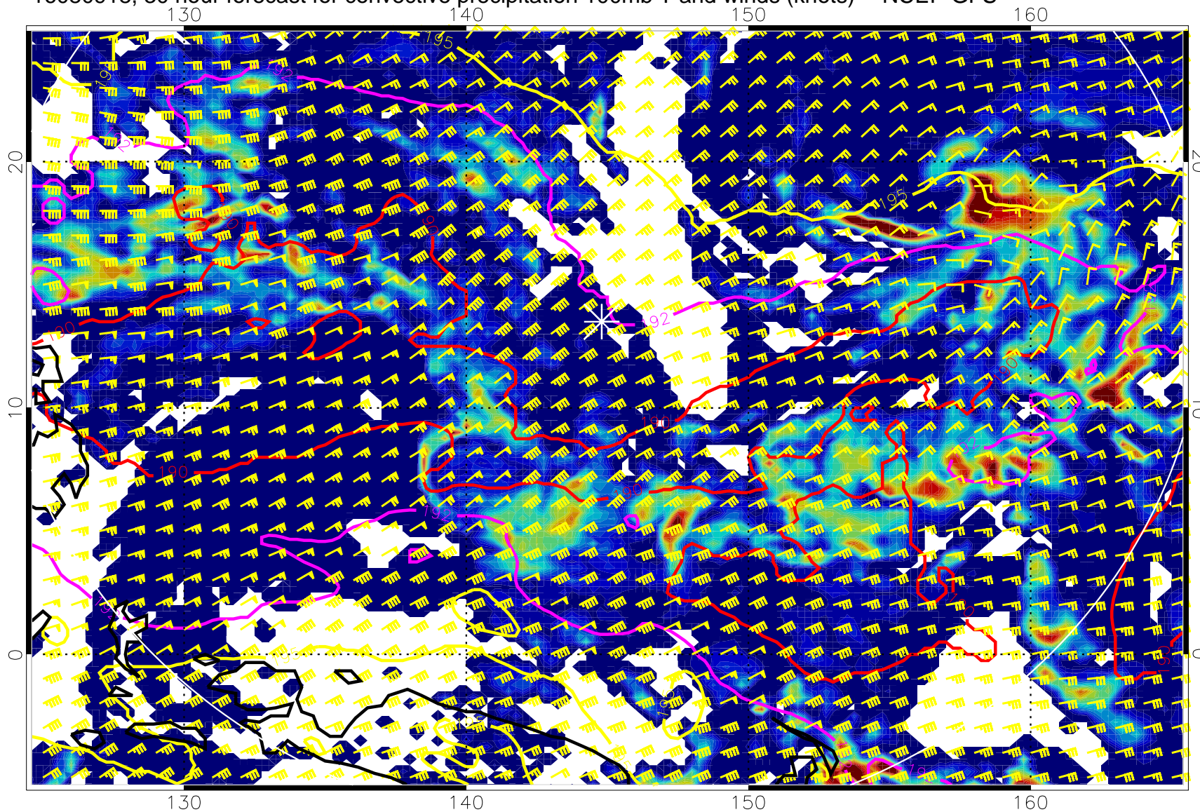
16080918, 30 hour forecast for convective precipitation 100mb T and winds (knots) -- NCEP GFS
