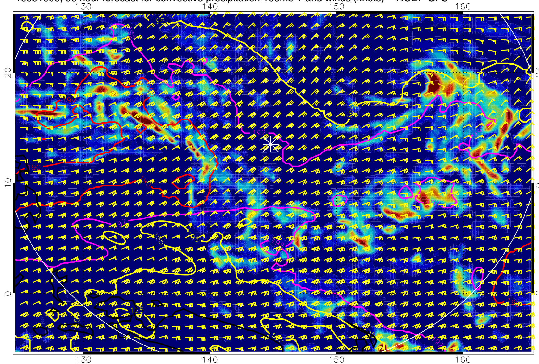
16081000, 36 hour forecast for convective precipitation 100mb T and winds (knots) -- NCEP GFS
