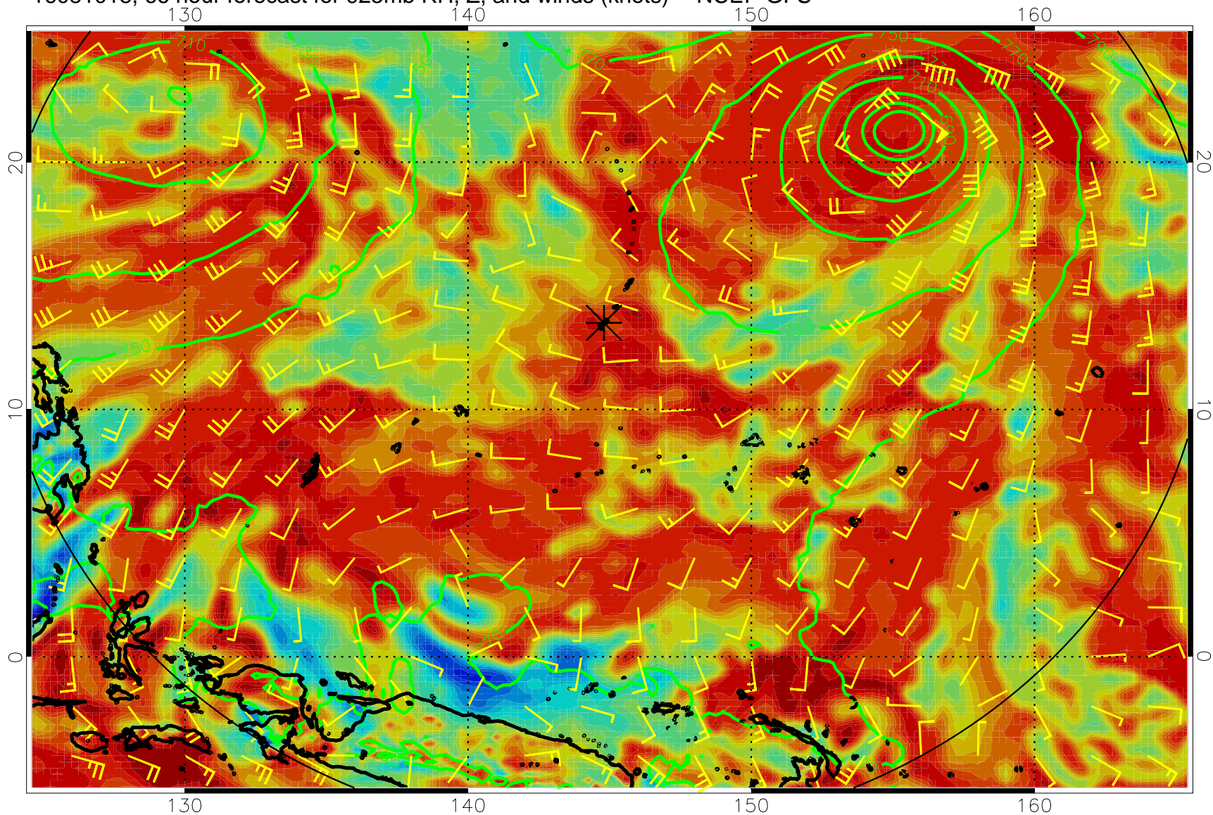
16081018, 66 hour forecast for 925mb RH, Z, and winds (knots) -- NCEP GFS
