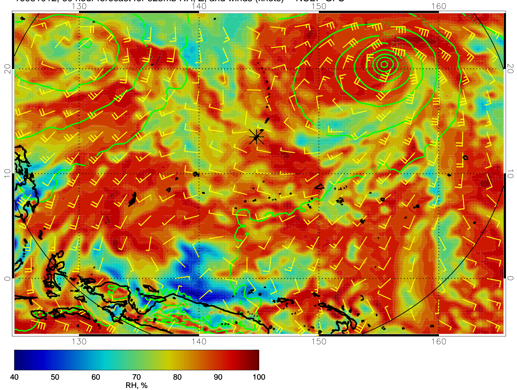
16081012, 60 hour forecast for 925mb RH, Z, and winds (knots) -- NCEP GFS
