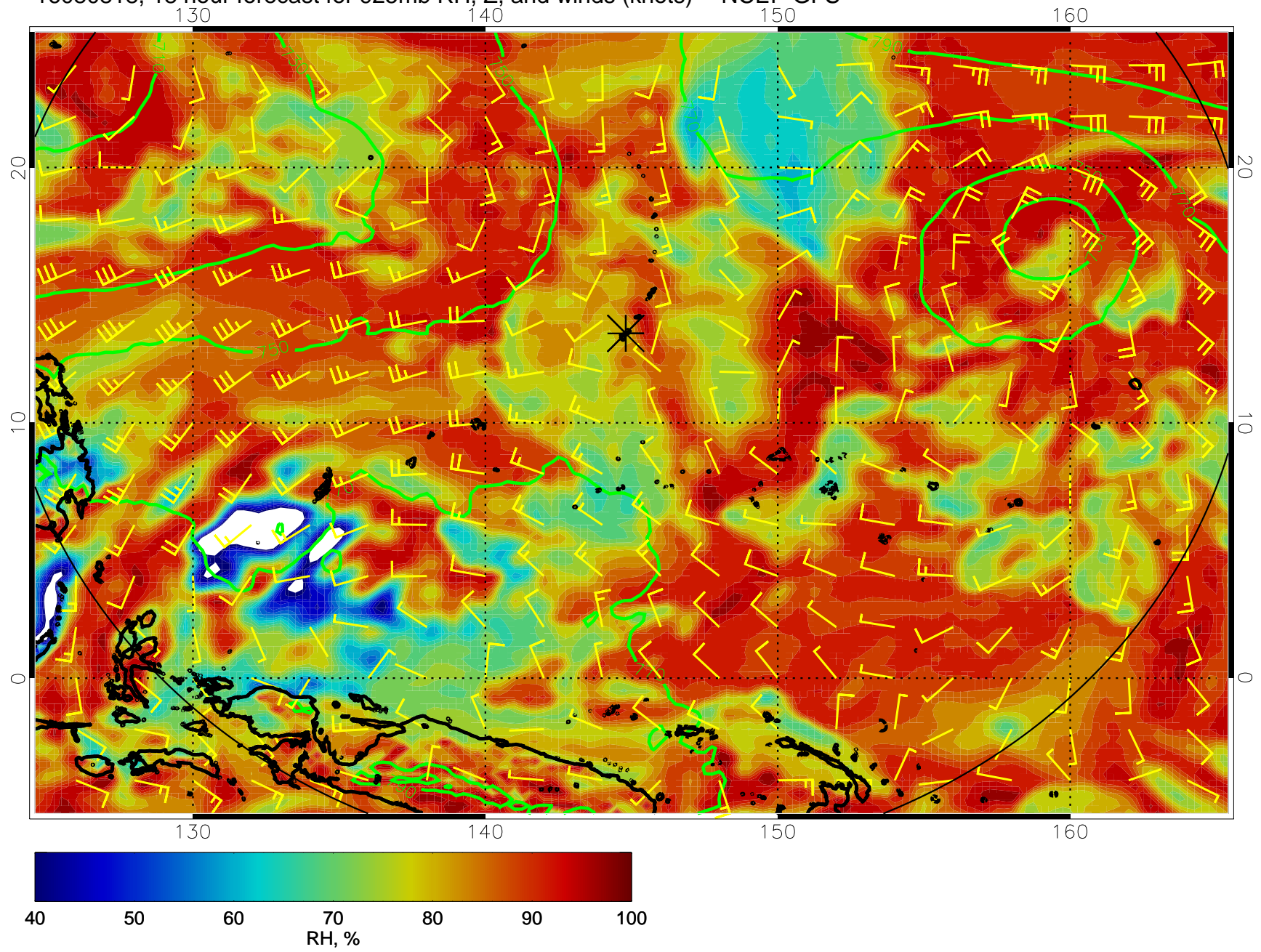
16080818, 18 hour forecast for 925mb RH, Z, and winds (knots) -- NCEP GFS
