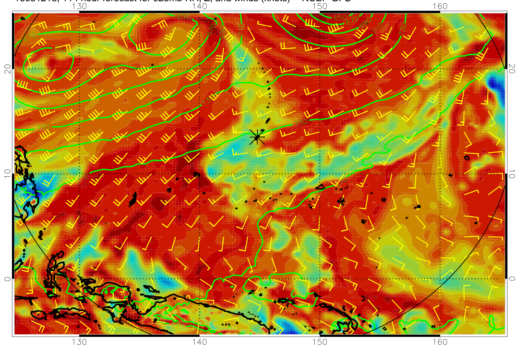
16081218, 114 hour forecast for 925mb RH, Z, and winds (knots) -- NCEP GFS
