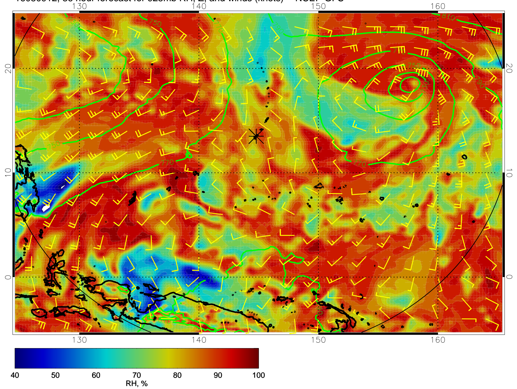
16080912, 36 hour forecast for 925mb RH, Z, and winds (knots) -- NCEP GFS
