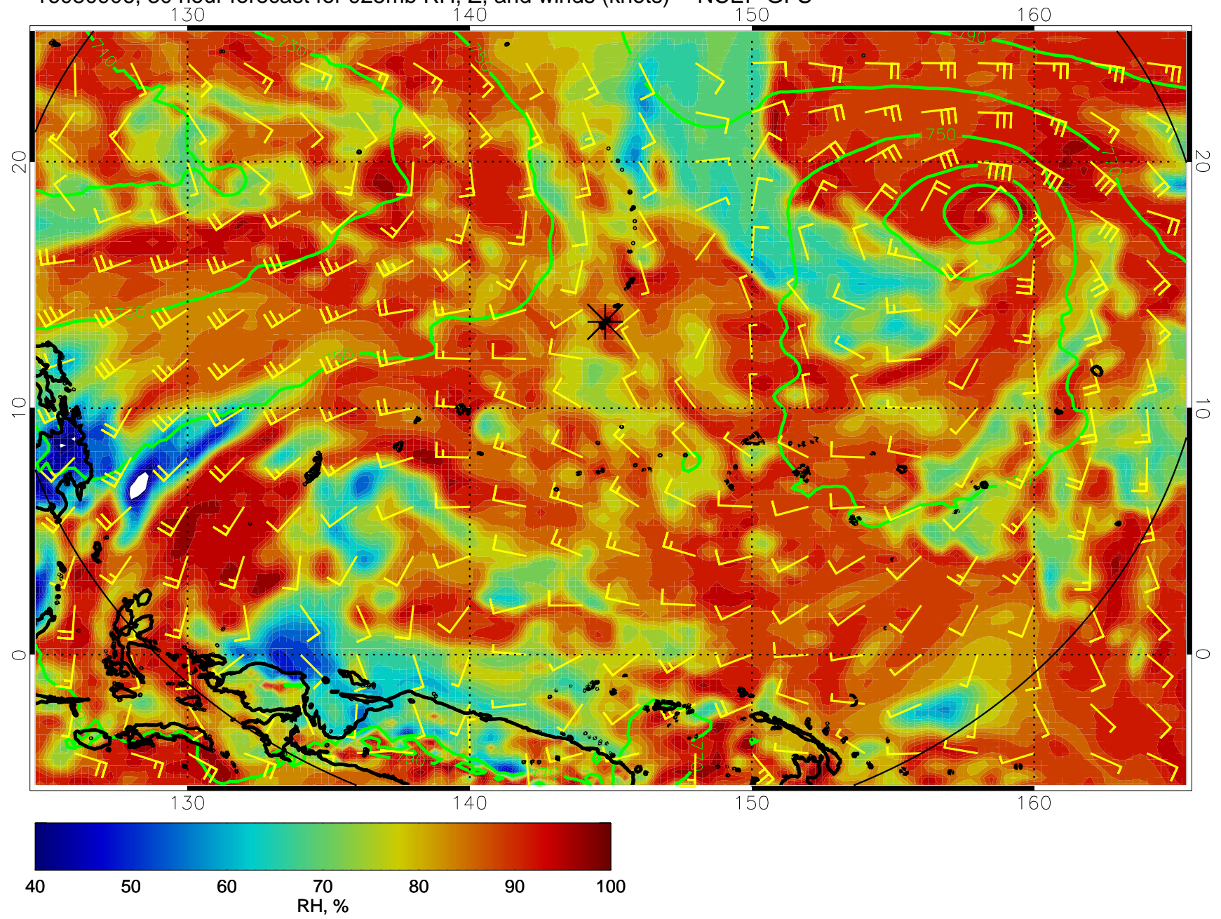
16080906, 30 hour forecast for 925mb RH, Z, and winds (knots) -- NCEP GFS
