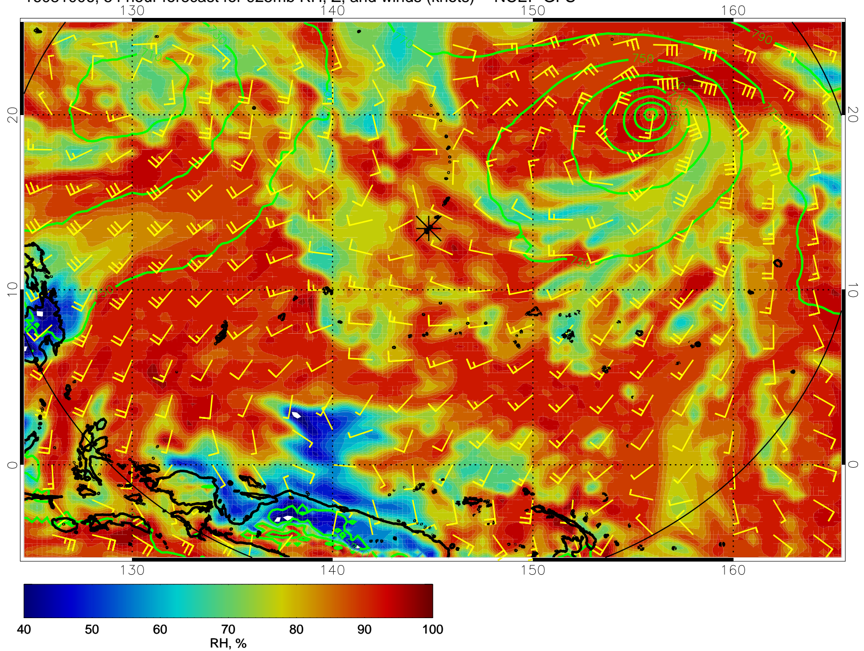
16081006, 54 hour forecast for 925mb RH, Z, and winds (knots) -- NCEP GFS
