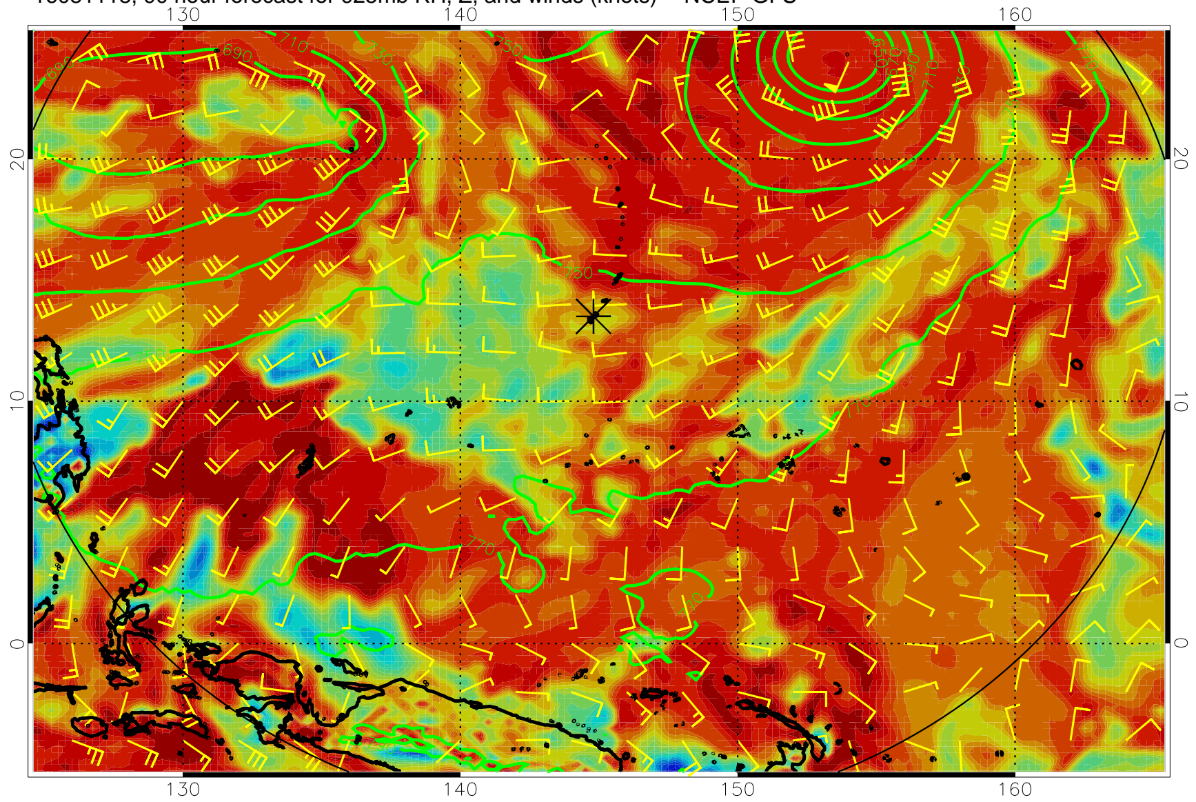
16081118, 90 hour forecast for 925mb RH, Z, and winds (knots) -- NCEP GFS
