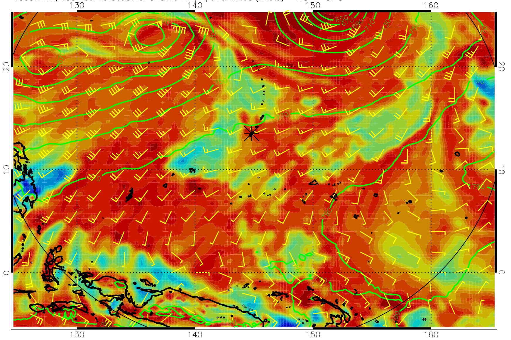
16081212, 108 hour forecast for 925mb RH, Z, and winds (knots) -- NCEP GFS
