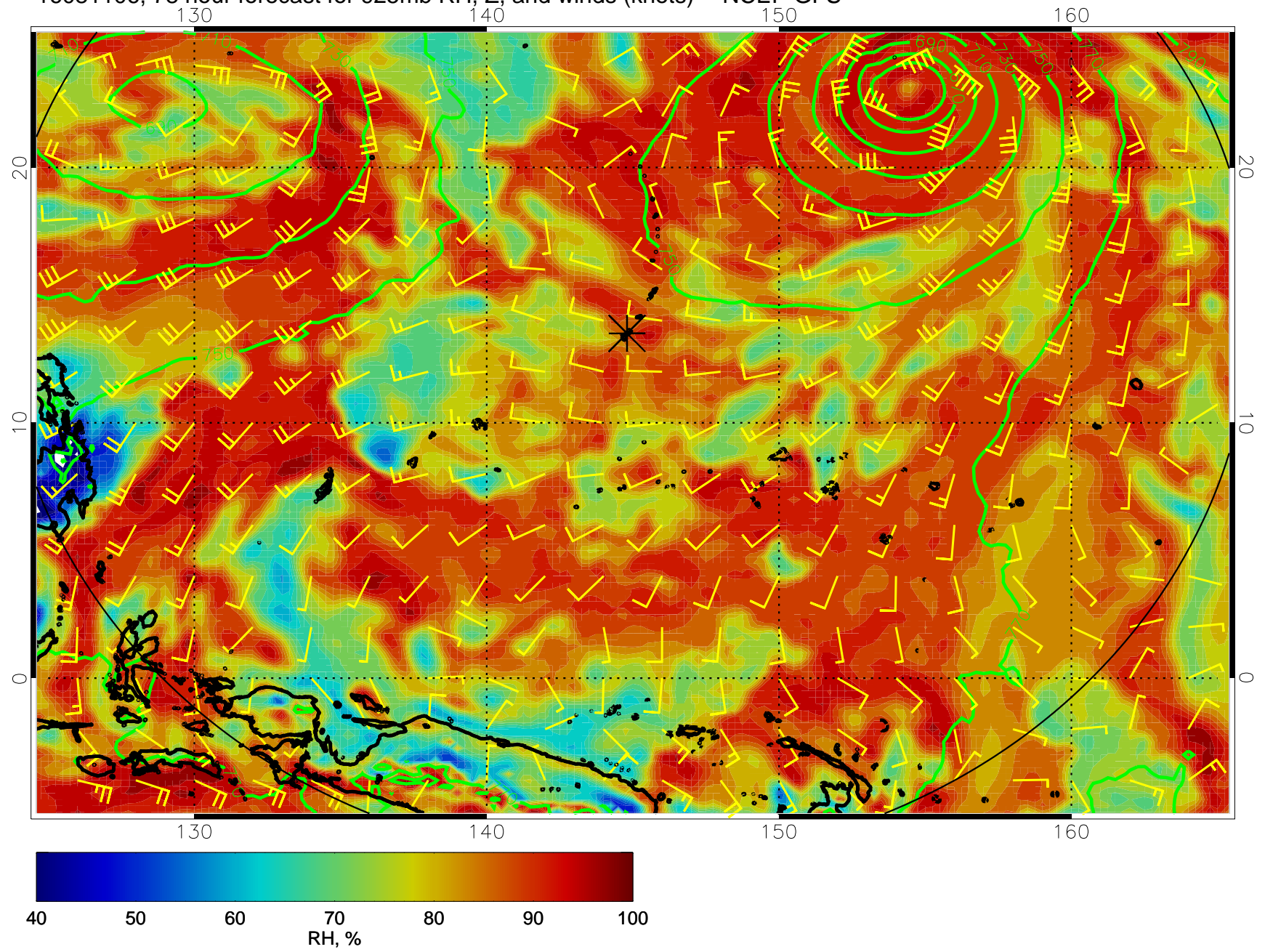
16081106, 78 hour forecast for 925mb RH, Z, and winds (knots) -- NCEP GFS
