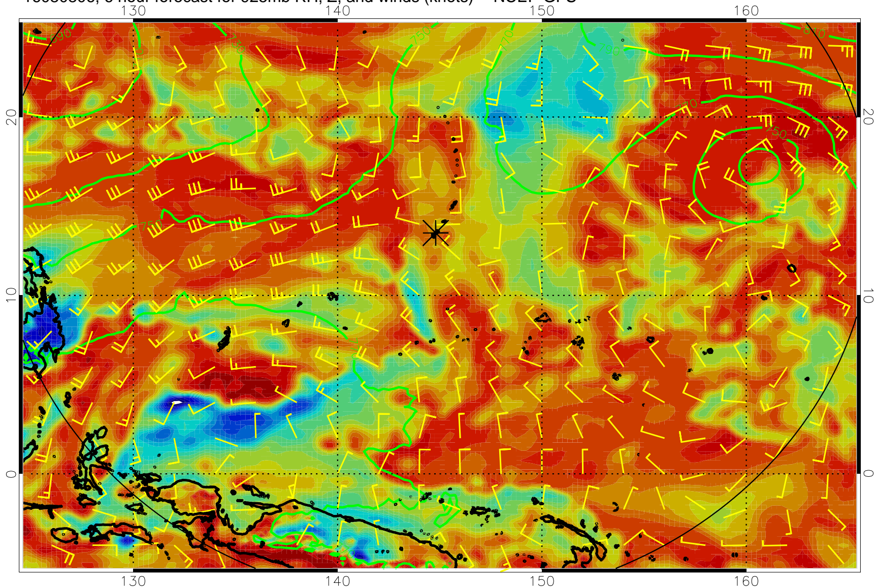
16080806, 6 hour forecast for 925mb RH, Z, and winds (knots) -- NCEP GFS
