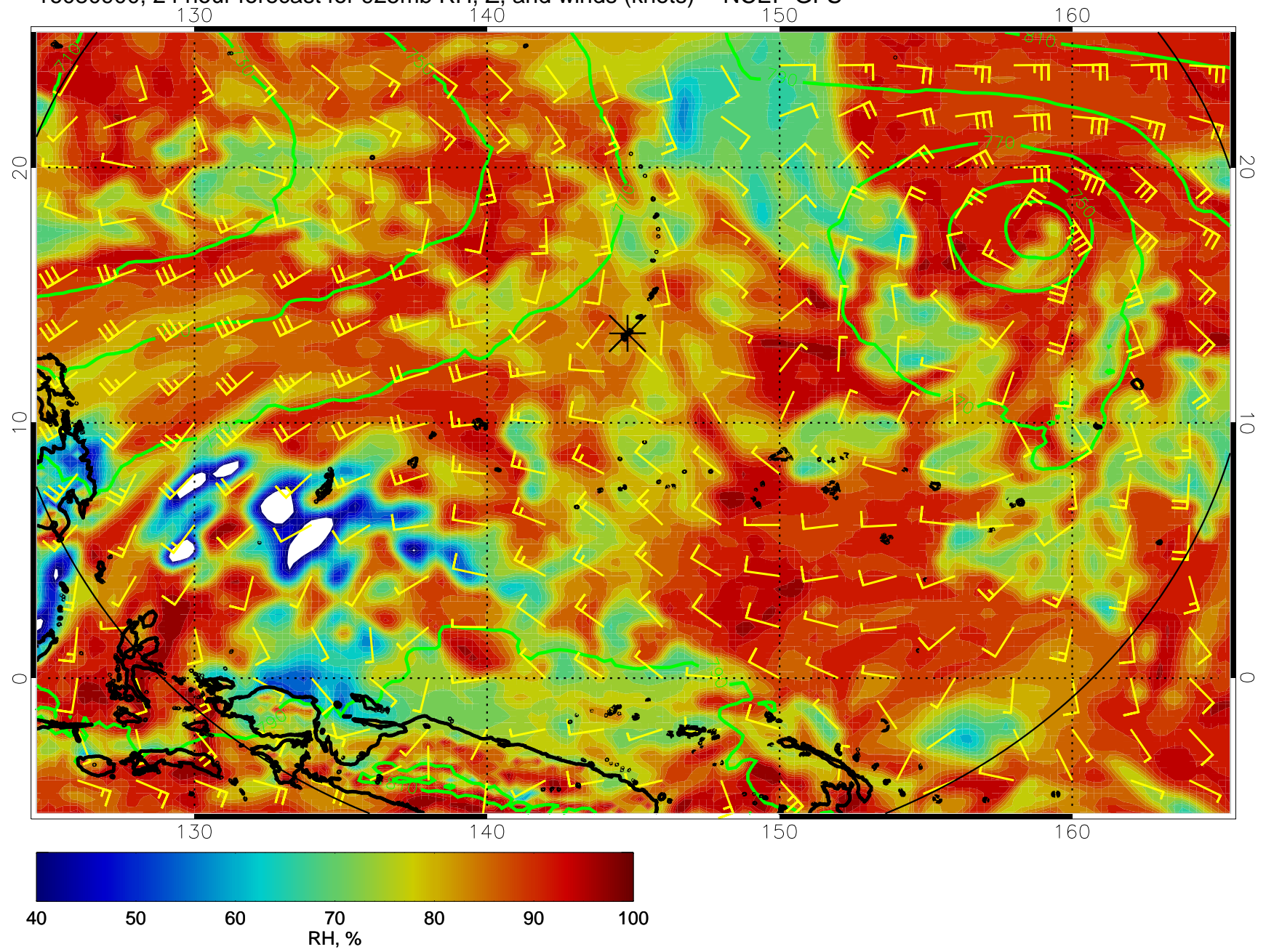
16080900, 24 hour forecast for 925mb RH, Z, and winds (knots) -- NCEP GFS
