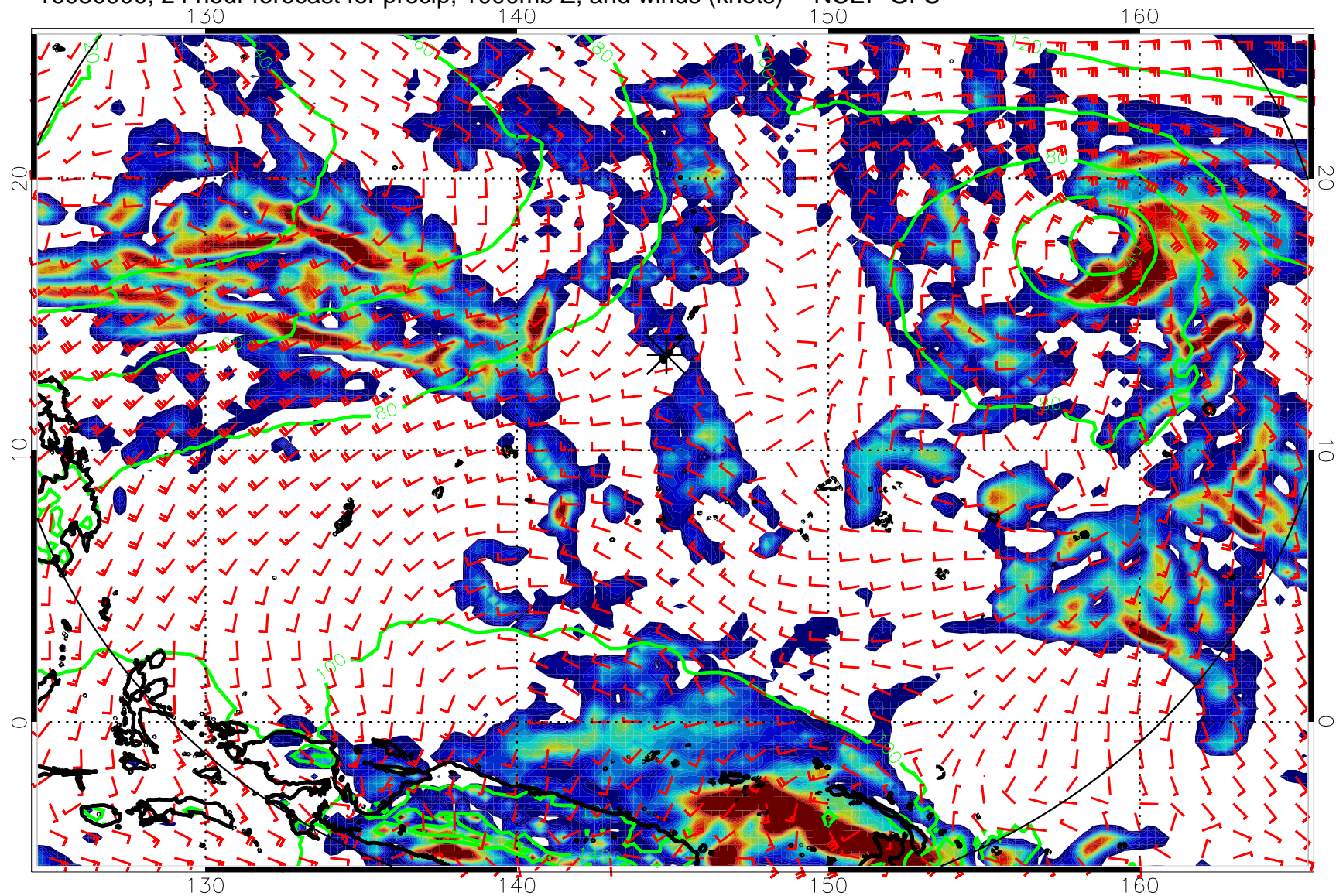
16080900, 24 hour forecast for precip, 1000mb Z, and winds (knots) -- NCEP GFS
