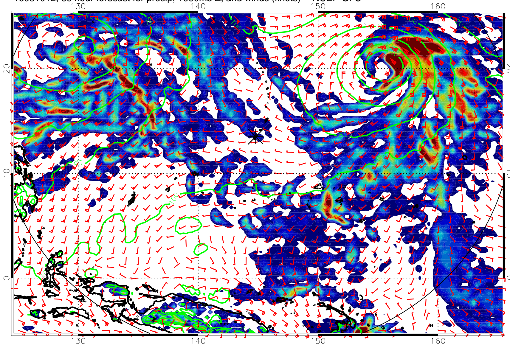
16081012, 60 hour forecast for precip, 1000mb Z, and winds (knots) -- NCEP GFS
