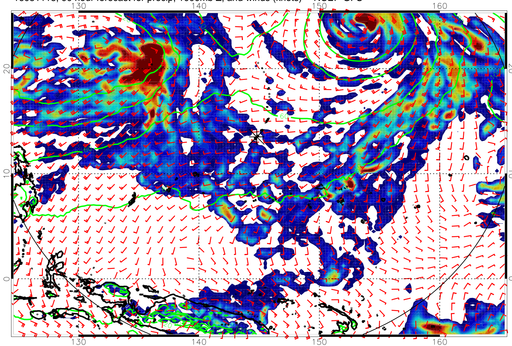
16081118, 90 hour forecast for precip, 1000mb Z, and winds (knots) -- NCEP GFS
