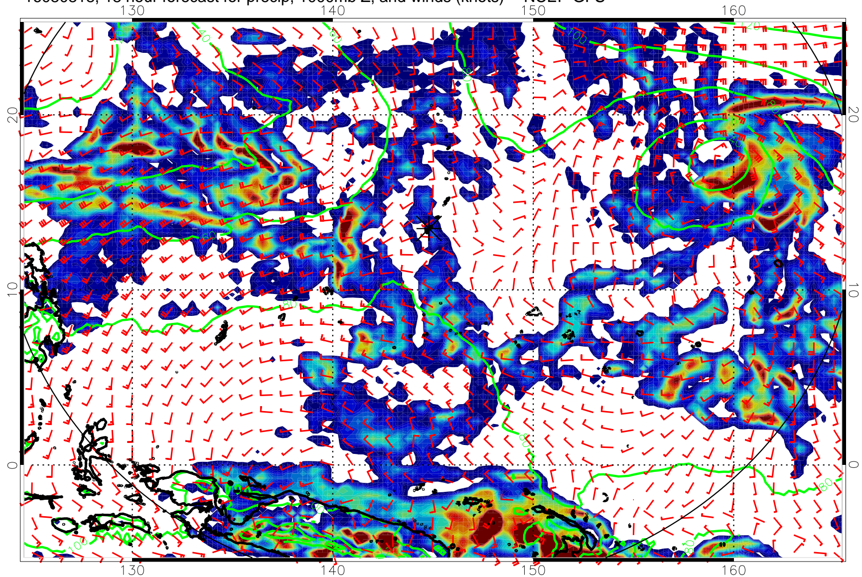
16080818, 18 hour forecast for precip, 1000mb Z, and winds (knots) -- NCEP GFS
