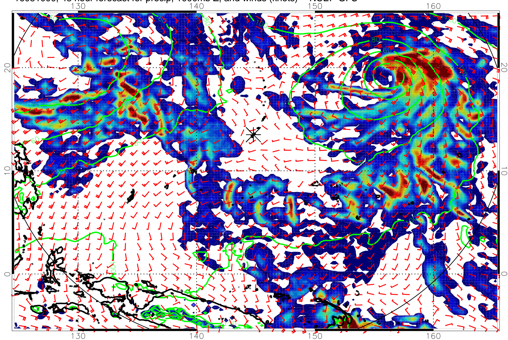
16081000, 48 hour forecast for precip, 1000mb Z, and winds (knots) -- NCEP GFS
