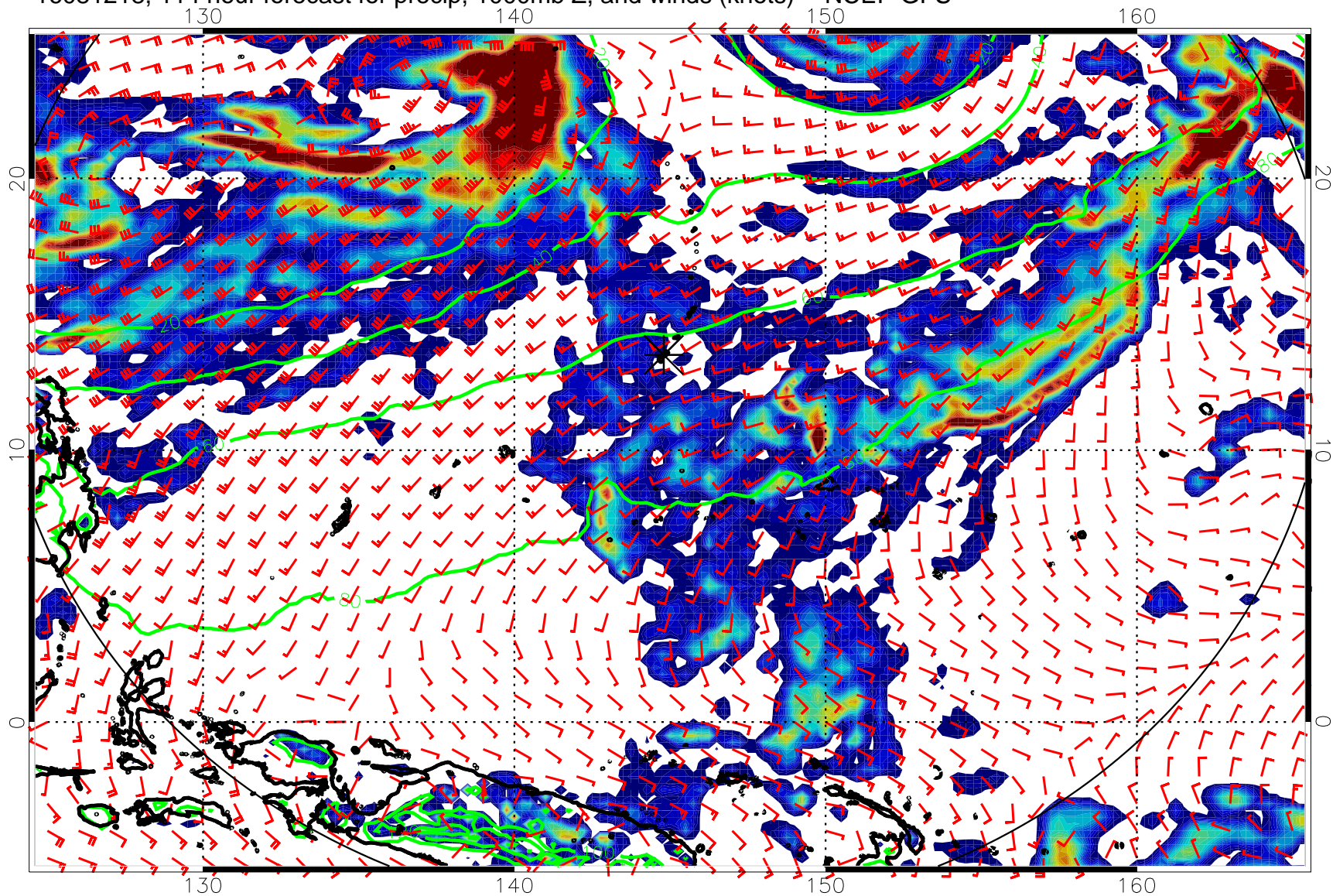
16081218, 114 hour forecast for precip, 1000mb Z, and winds (knots) -- NCEP GFS
