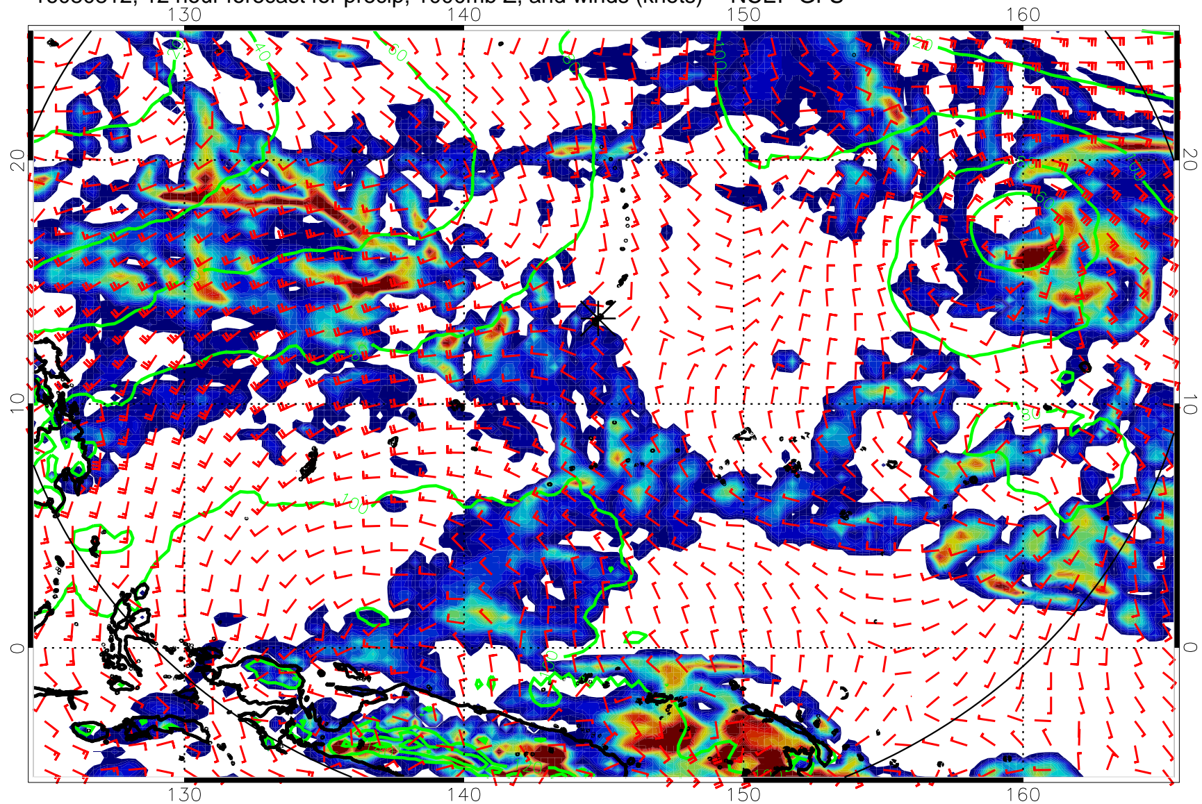
16080812, 12 hour forecast for precip, 1000mb Z, and winds (knots) -- NCEP GFS
