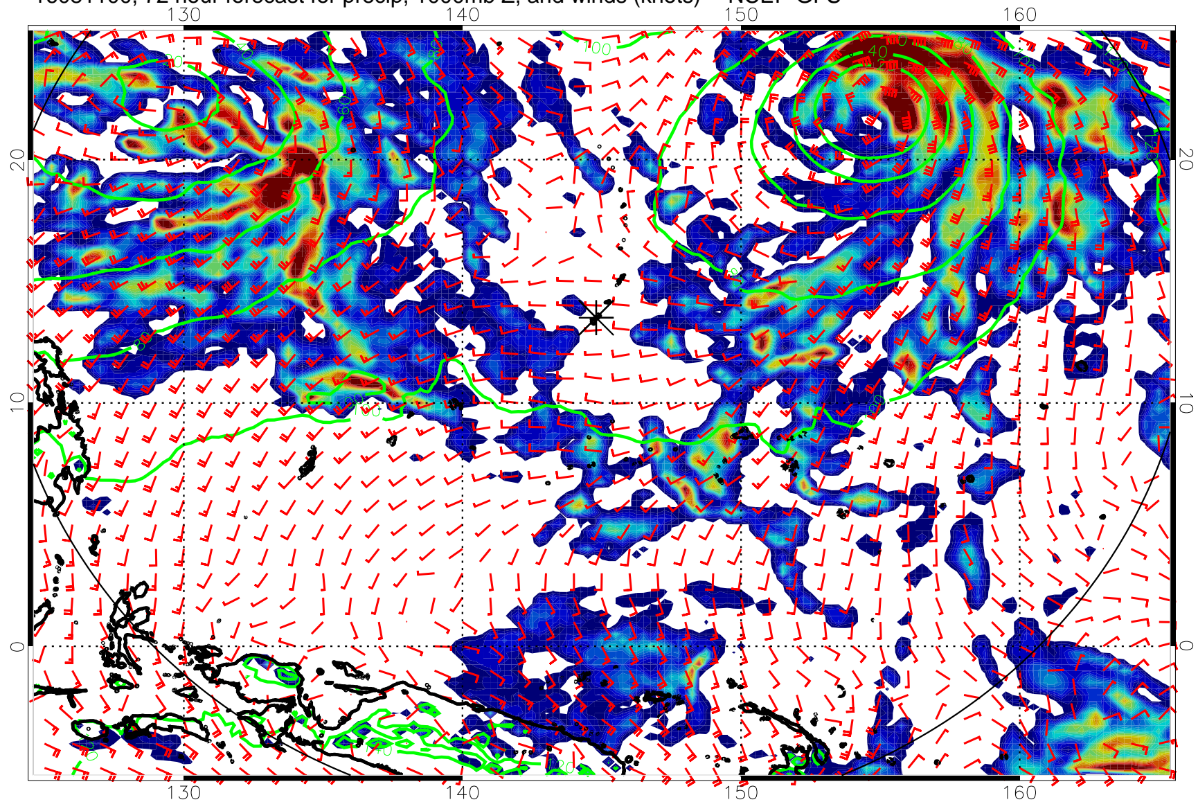
16081100, 72 hour forecast for precip, 1000mb Z, and winds (knots) -- NCEP GFS
