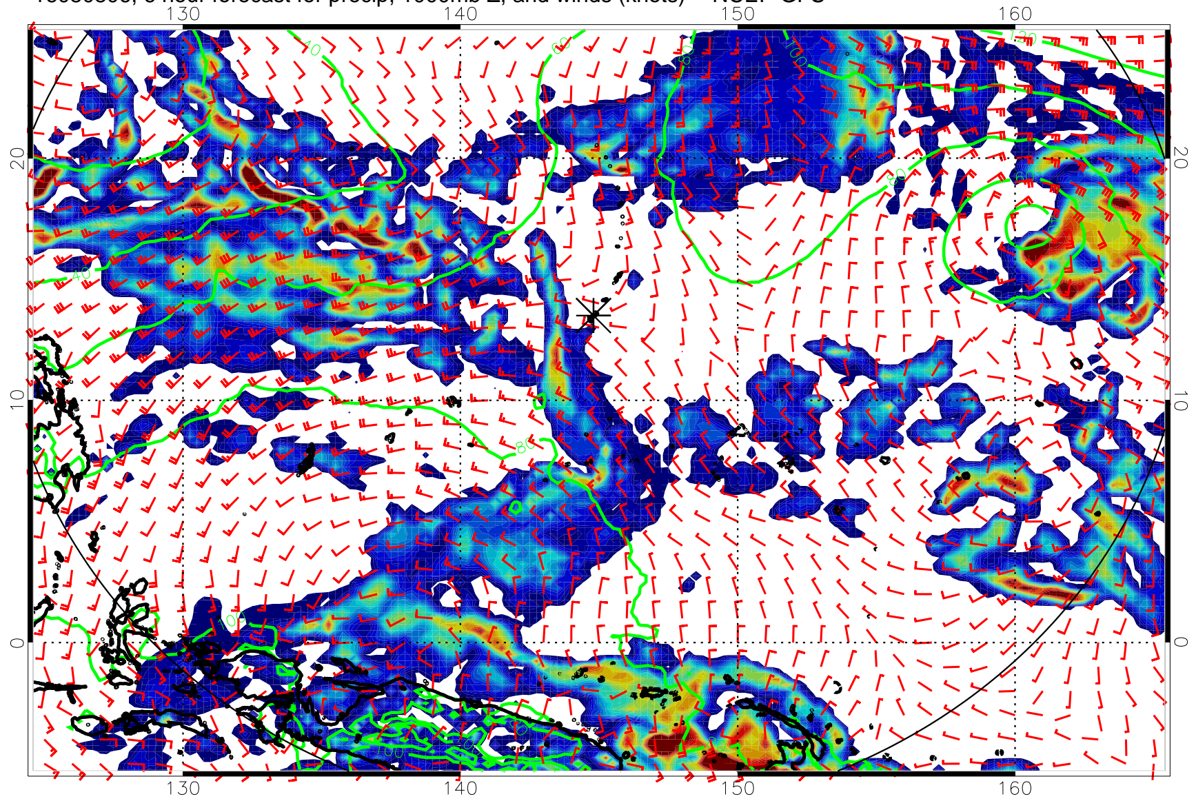
16080806, 6 hour forecast for precip, 1000mb Z, and winds (knots) -- NCEP GFS
