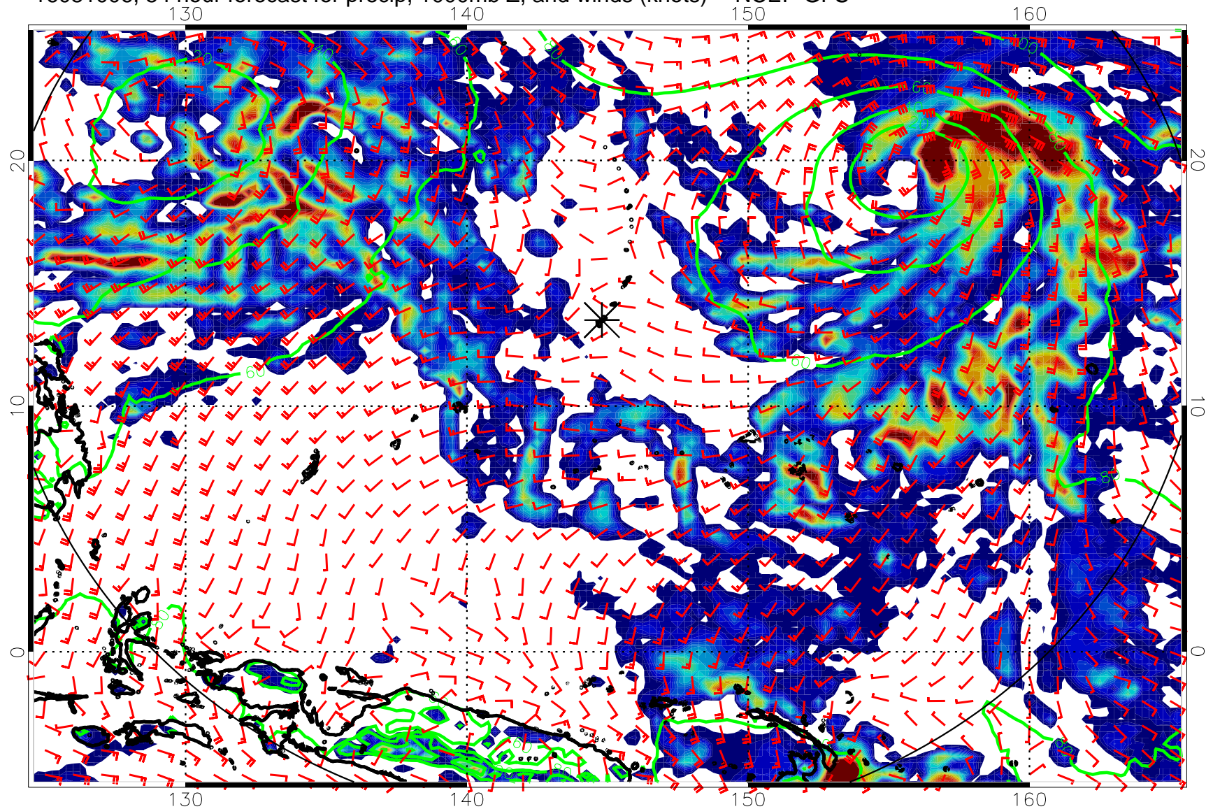
16081006, 54 hour forecast for precip, 1000mb Z, and winds (knots) -- NCEP GFS
