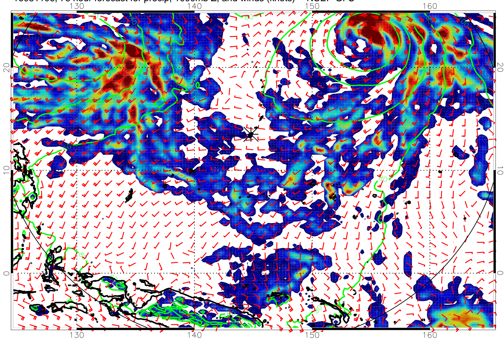
16081106, 78 hour forecast for precip, 1000mb Z, and winds (knots) -- NCEP GFS
