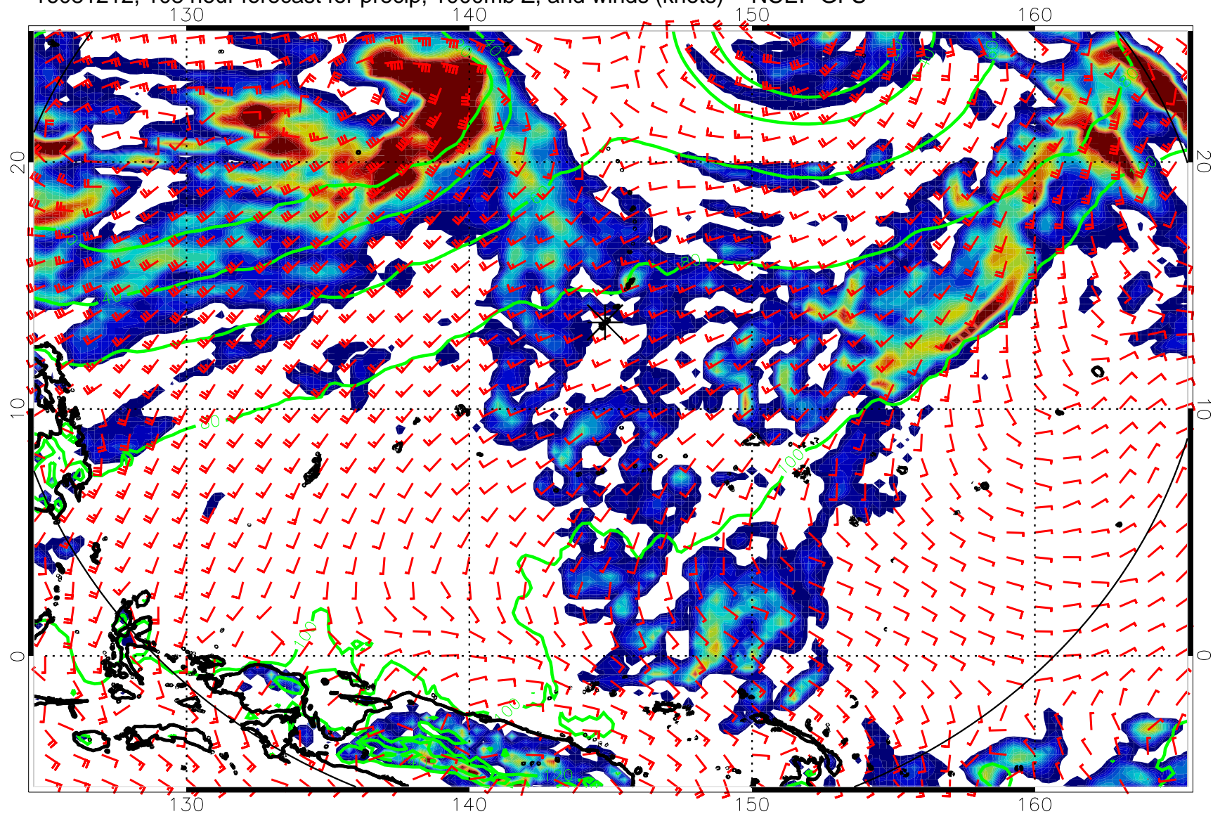
16081212, 108 hour forecast for precip, 1000mb Z, and winds (knots) -- NCEP GFS
