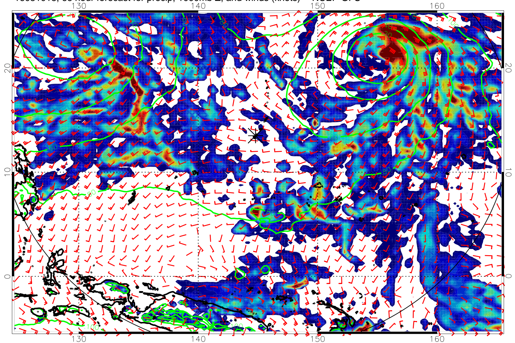
16081018, 66 hour forecast for precip, 1000mb Z, and winds (knots) -- NCEP GFS
