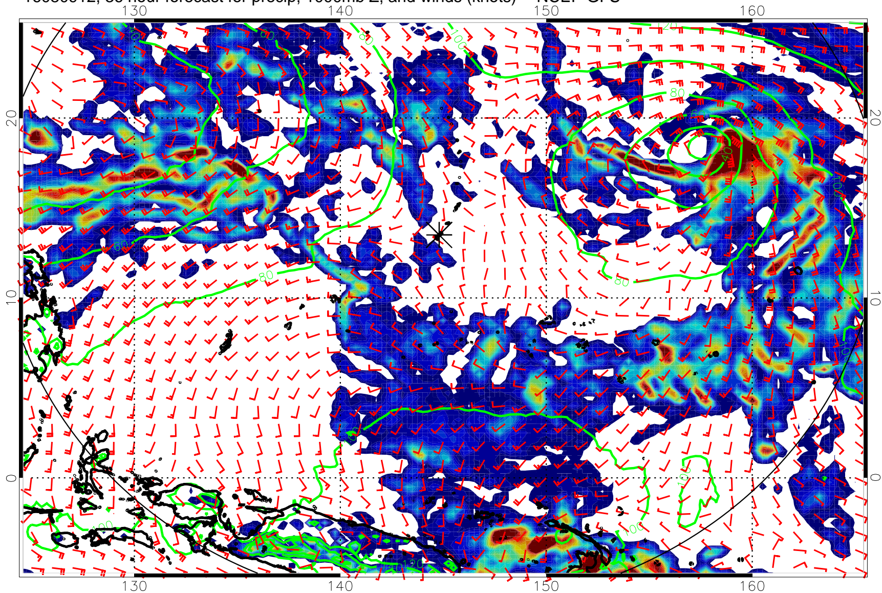
16080912, 36 hour forecast for precip, 1000mb Z, and winds (knots) -- NCEP GFS
