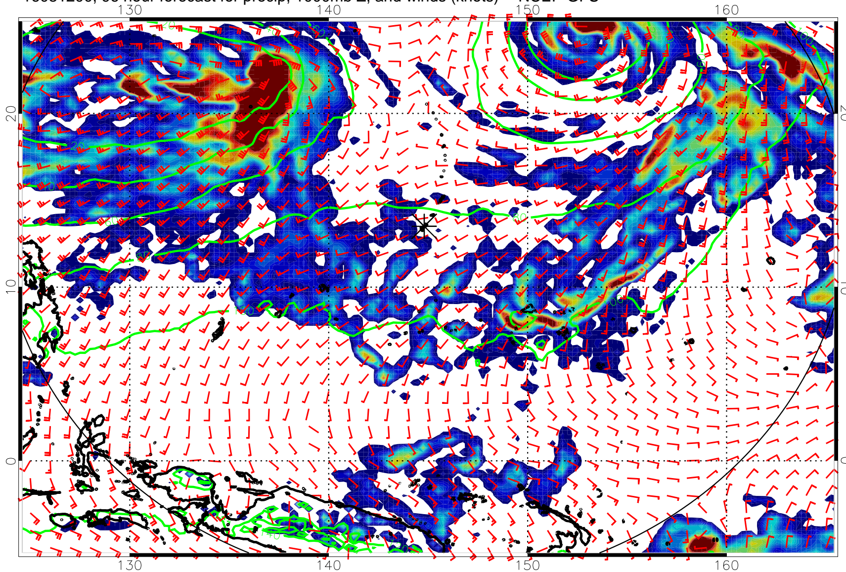
16081200, 96 hour forecast for precip, 1000mb Z, and winds (knots) -- NCEP GFS
