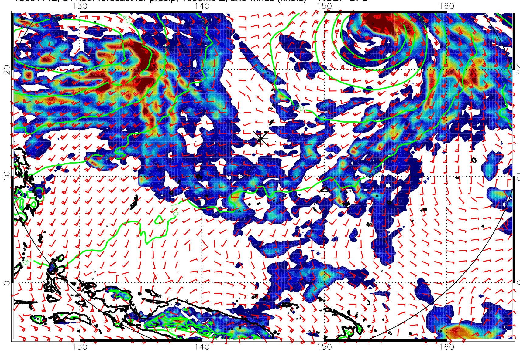
16081112, 84 hour forecast for precip, 1000mb Z, and winds (knots) -- NCEP GFS
