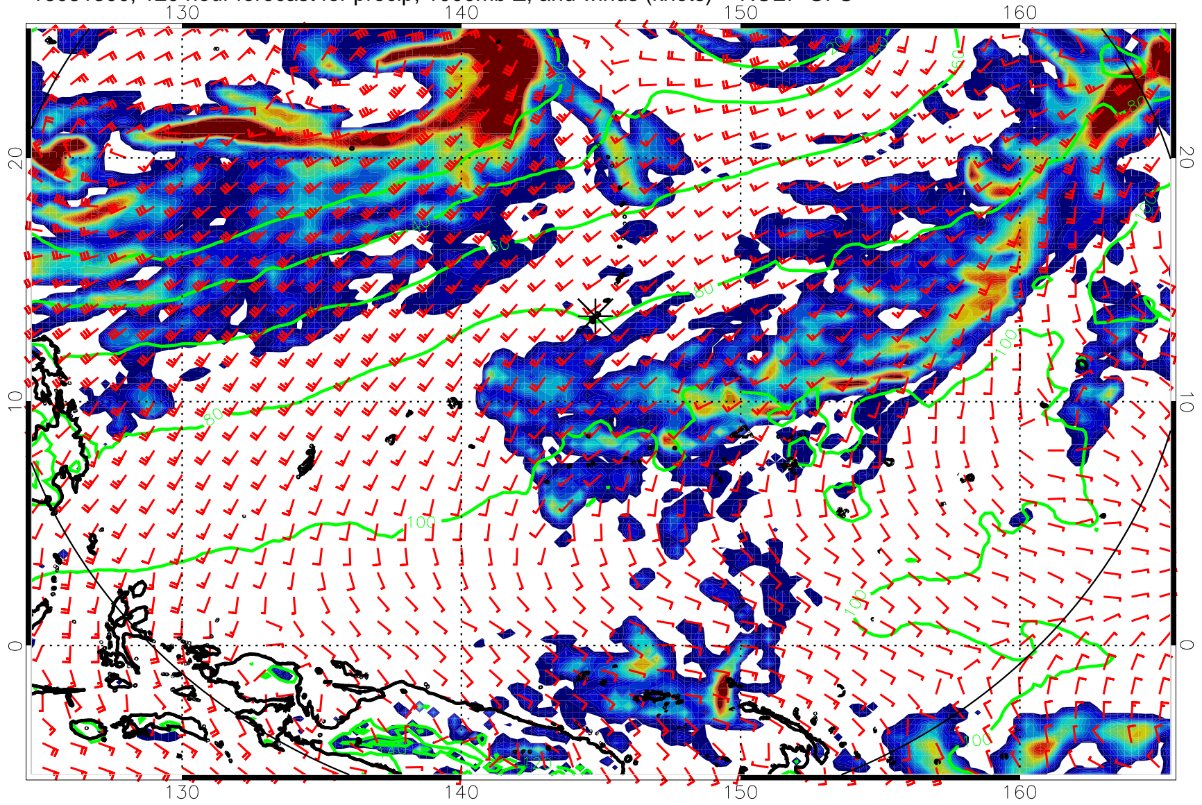
16081300, 120 hour forecast for precip, 1000mb Z, and winds (knots) -- NCEP GFS
