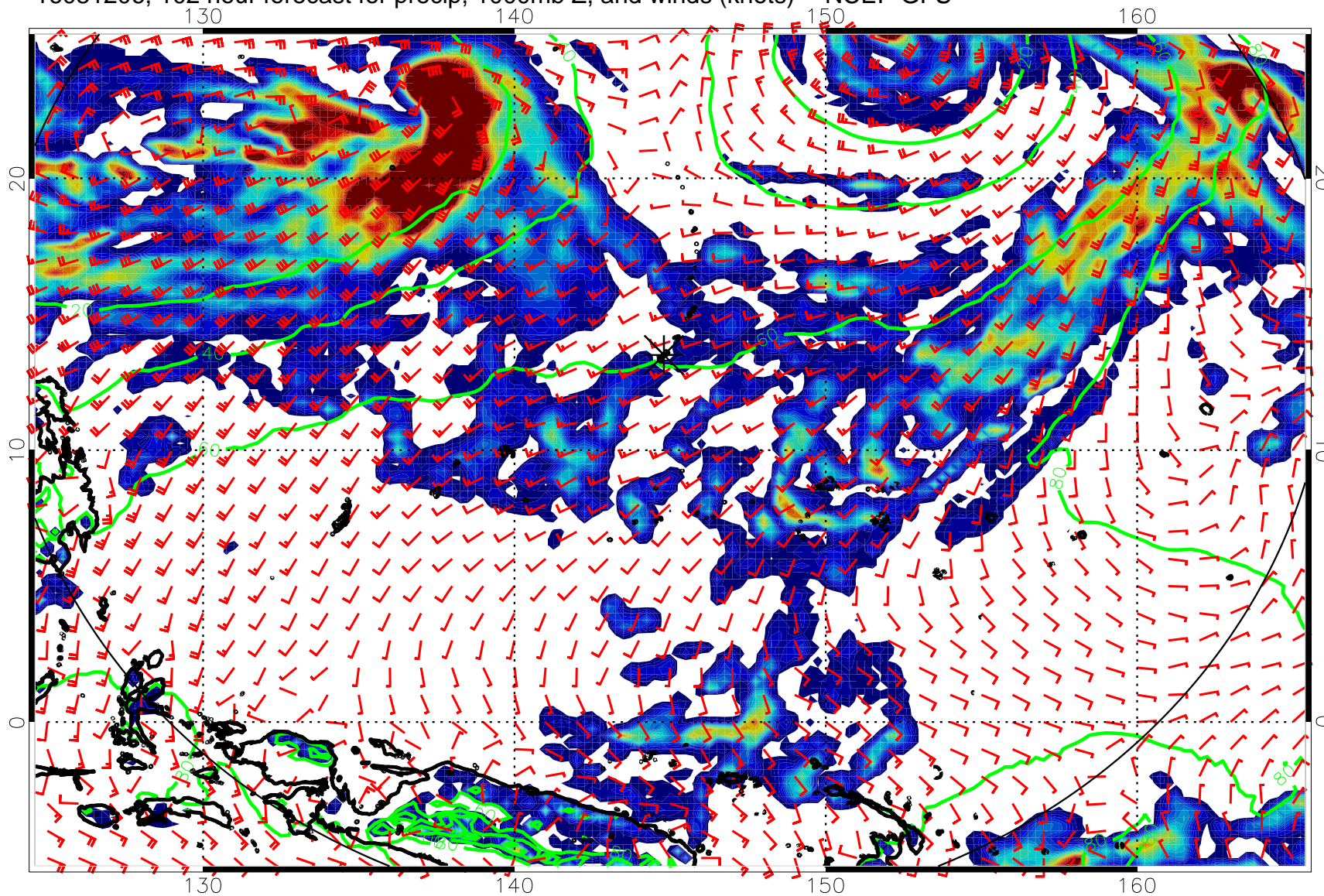
16081206, 102 hour forecast for precip, 1000mb Z, and winds (knots) -- NCEP GFS
