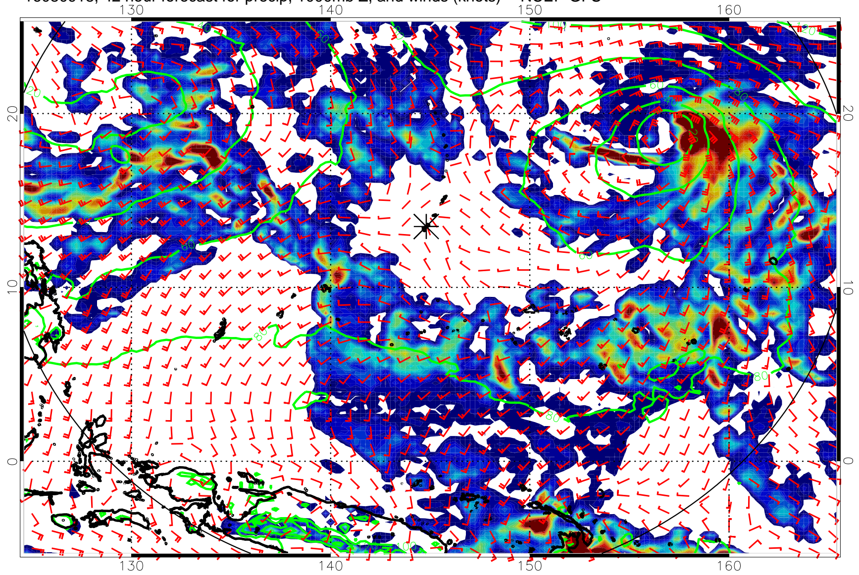
16080918, 42 hour forecast for precip, 1000mb Z, and winds (knots) -- NCEP GFS
