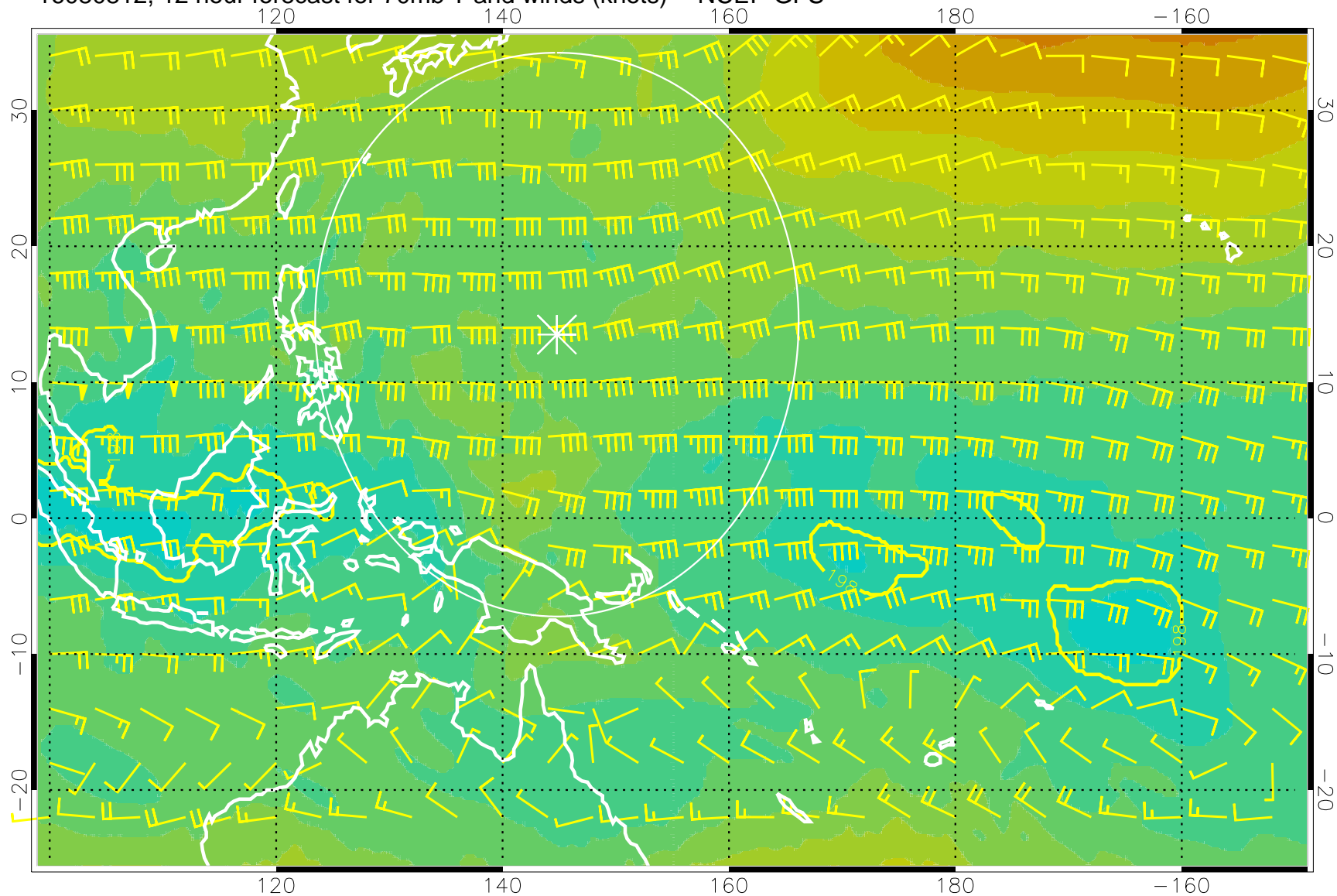
16080812, 12 hour forecast for 70mb T and winds (knots) -- NCEP GFS
