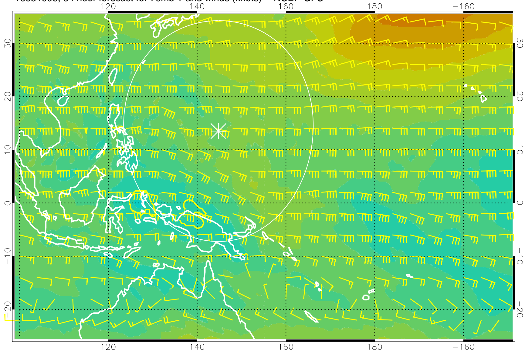
16081006, 54 hour forecast for 70mb T and winds (knots) -- NCEP GFS
