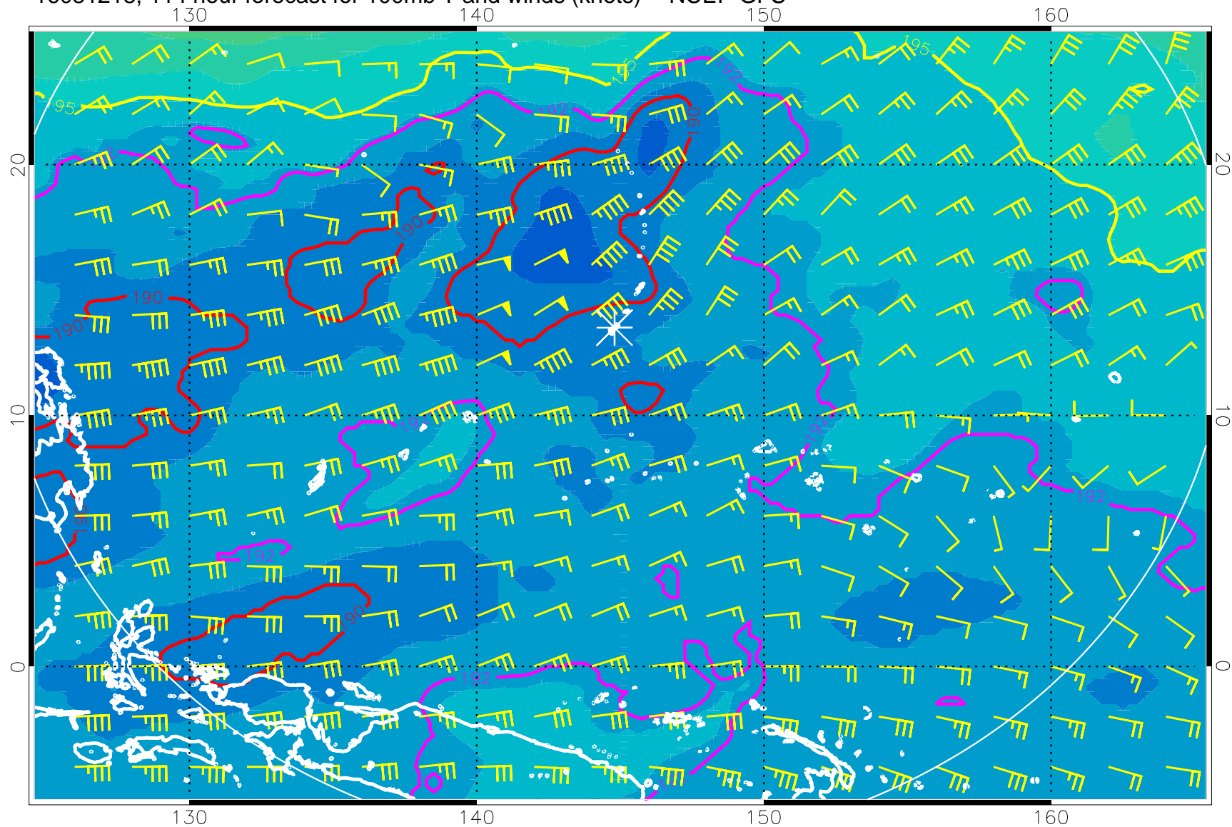
16081218, 114 hour forecast for 100mb T and winds (knots) -- NCEP GFS
