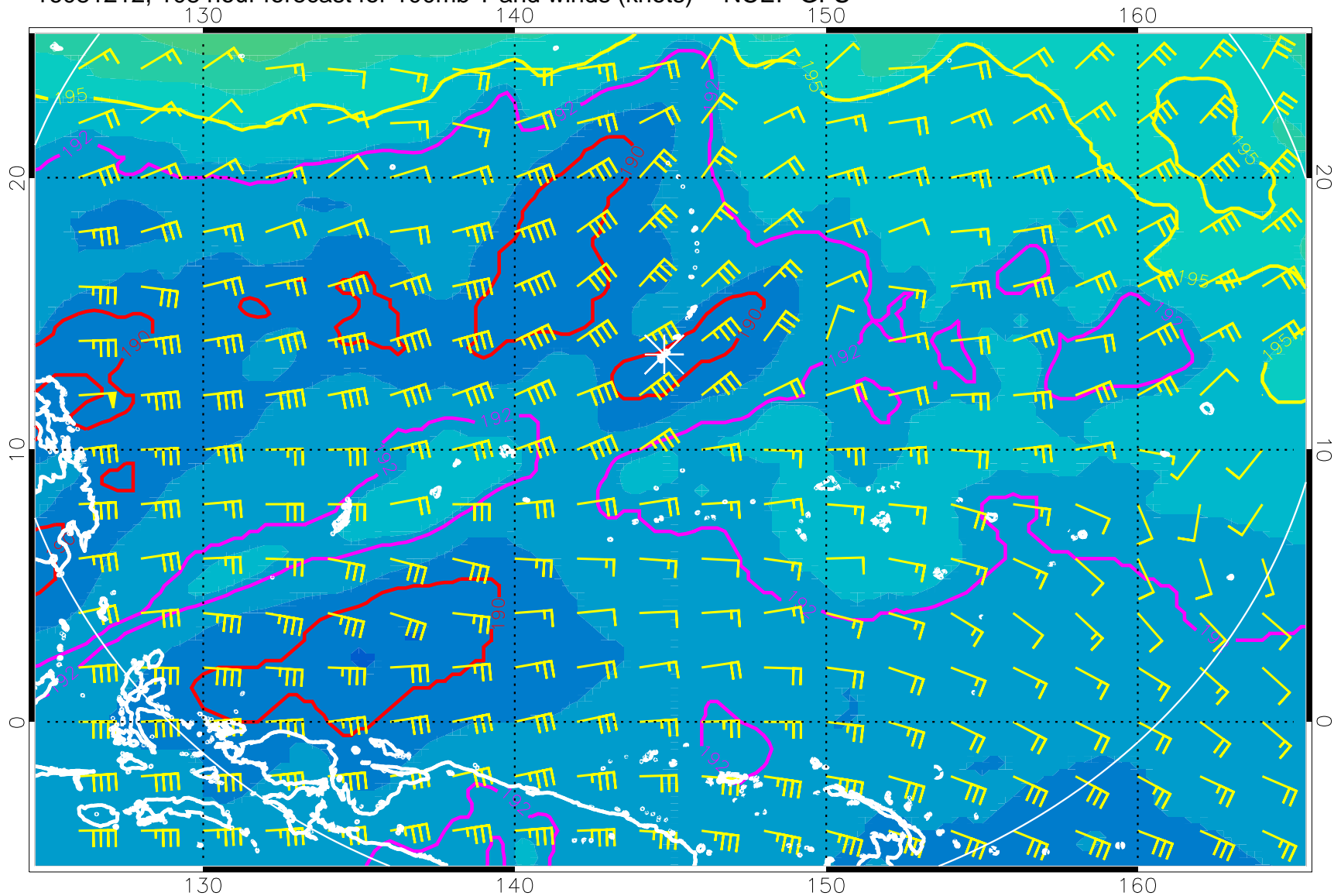
16081212, 108 hour forecast for 100mb T and winds (knots) -- NCEP GFS
