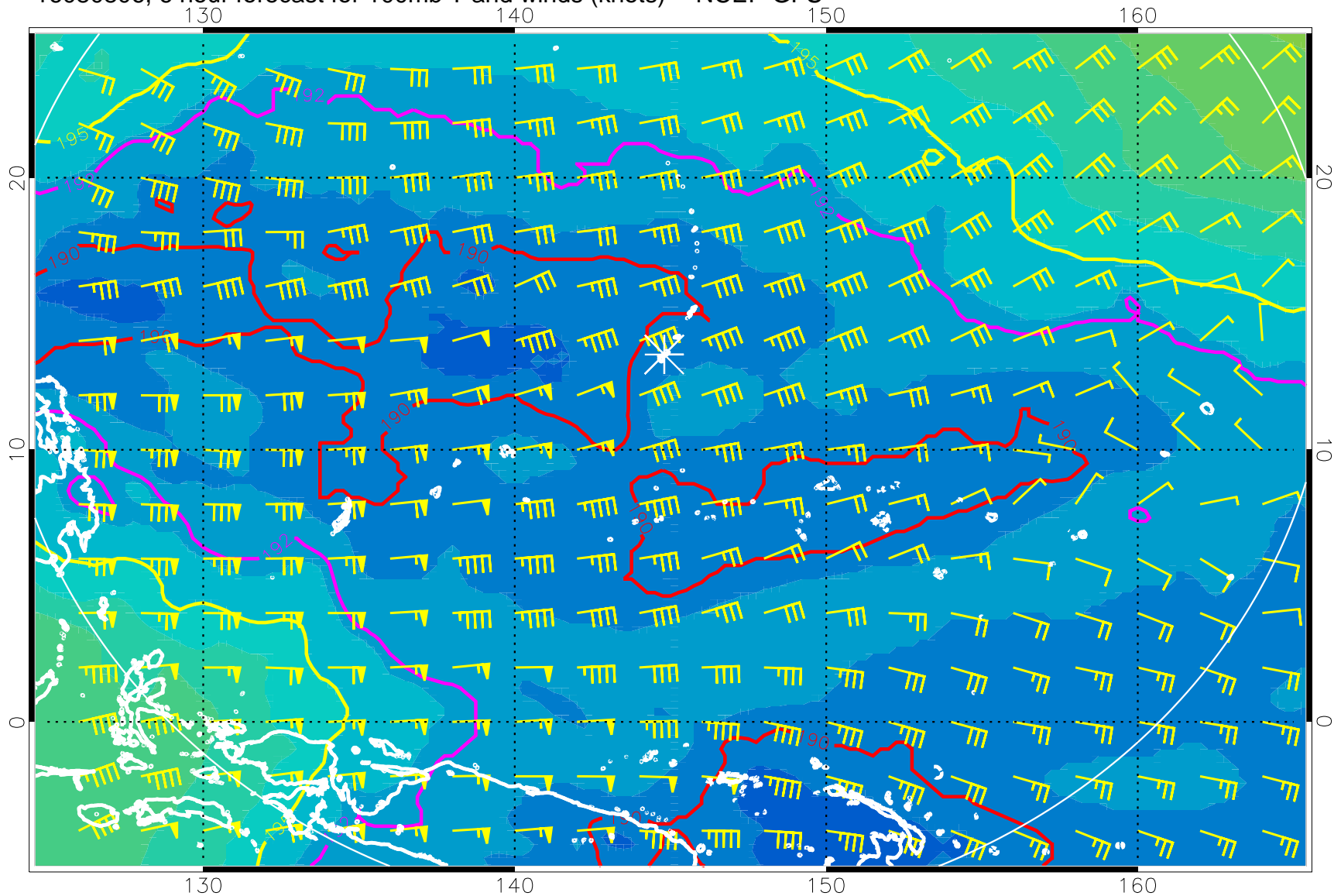
16080806, 6 hour forecast for 100mb T and winds (knots) -- NCEP GFS
