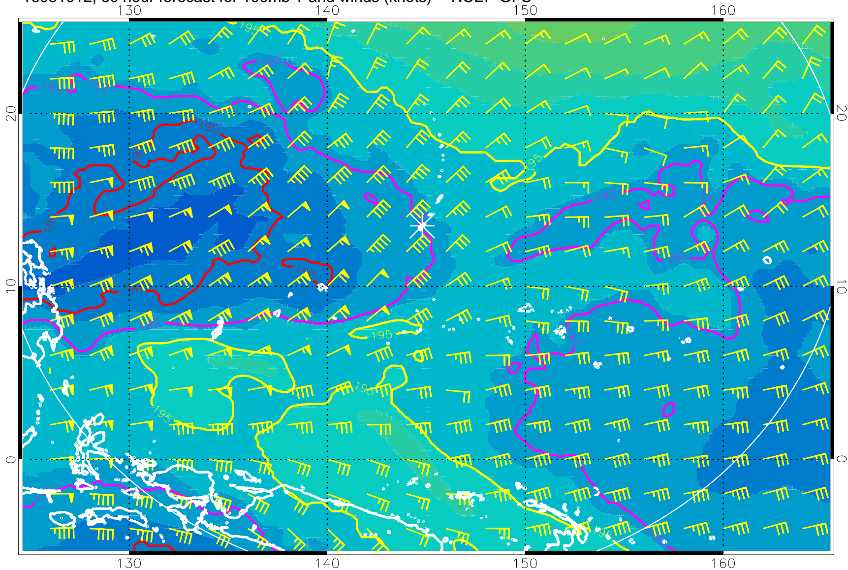
16081012, 60 hour forecast for 100mb T and winds (knots) -- NCEP GFS
