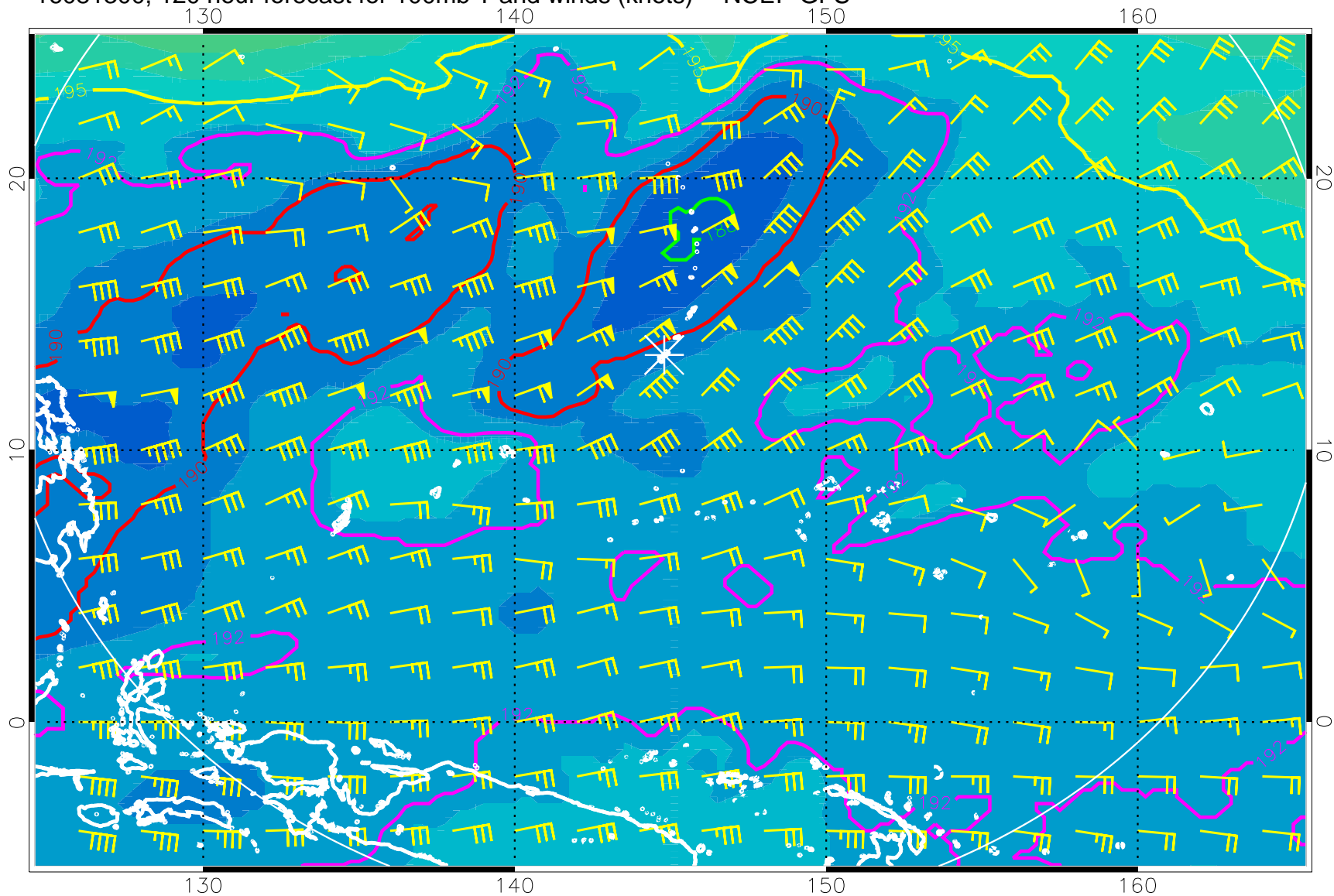
16081300, 120 hour forecast for 100mb T and winds (knots) -- NCEP GFS
