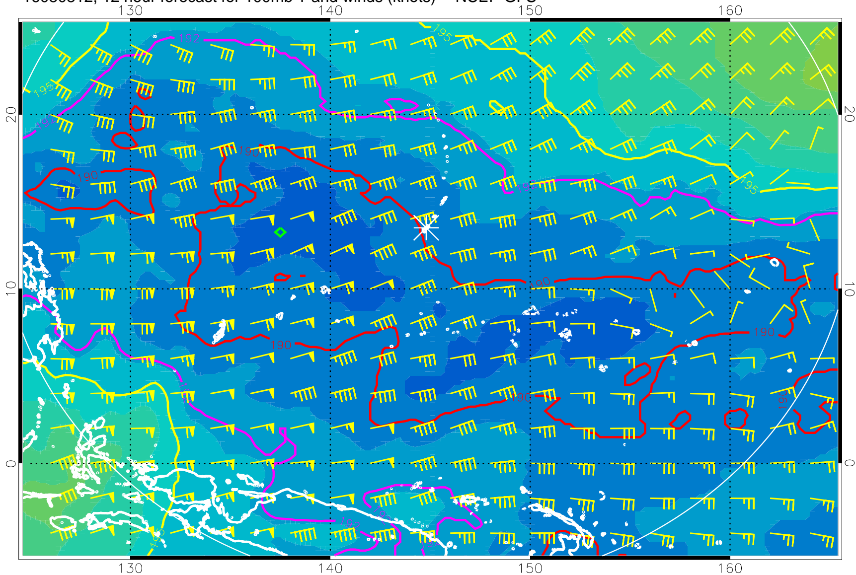
16080812, 12 hour forecast for 100mb T and winds (knots) -- NCEP GFS
