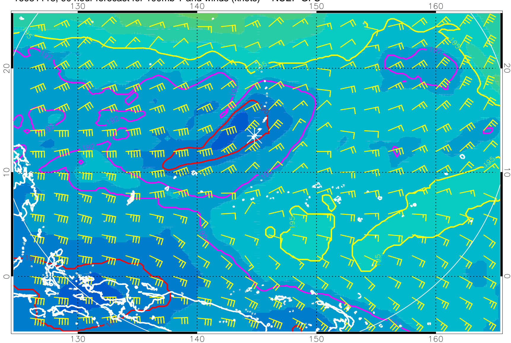
16081118, 90 hour forecast for 100mb T and winds (knots) -- NCEP GFS
