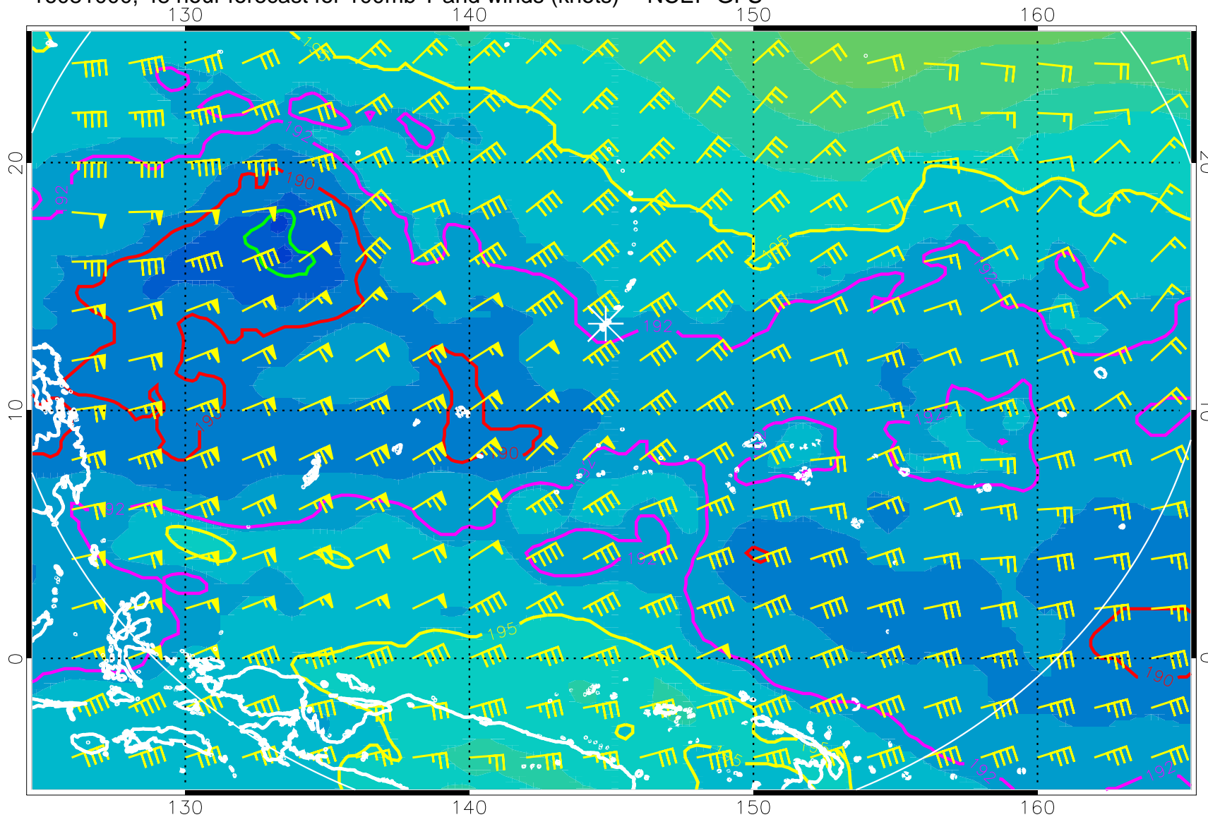
16081000, 48 hour forecast for 100mb T and winds (knots) -- NCEP GFS
