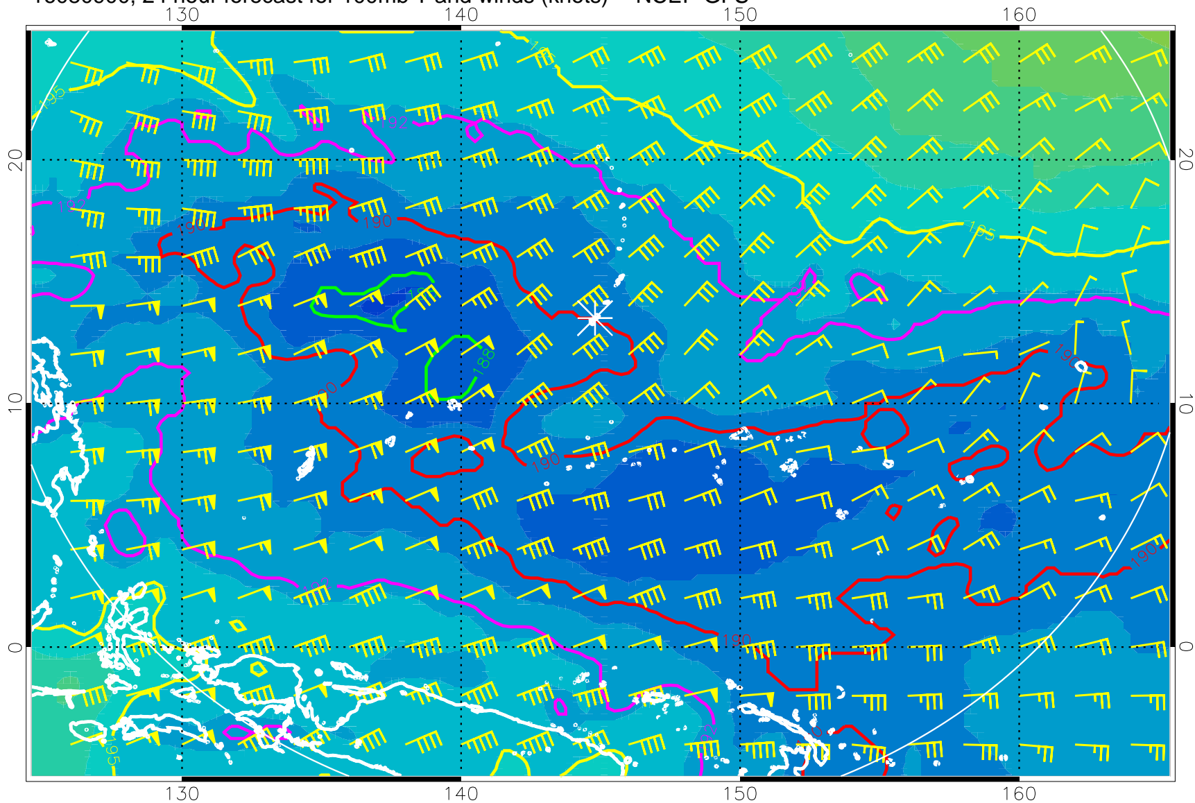
16080900, 24 hour forecast for 100mb T and winds (knots) -- NCEP GFS
