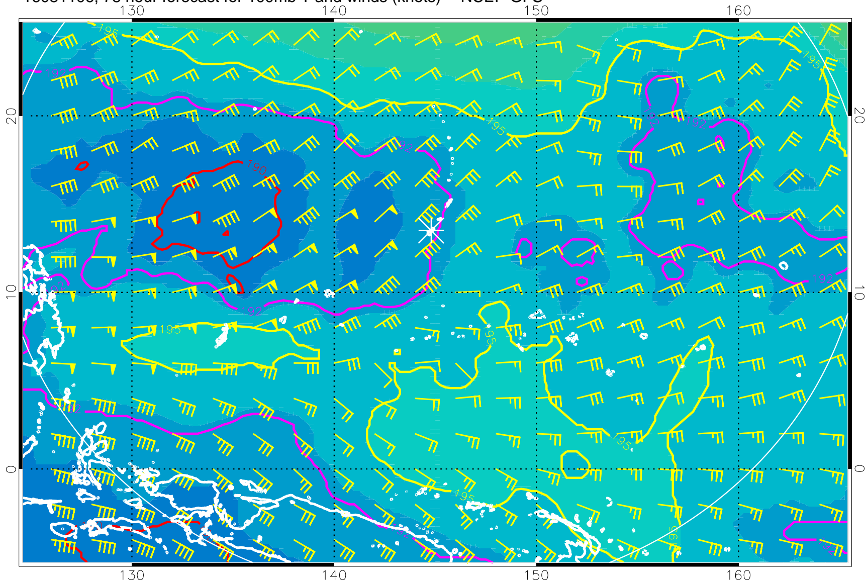
16081106, 78 hour forecast for 100mb T and winds (knots) -- NCEP GFS
