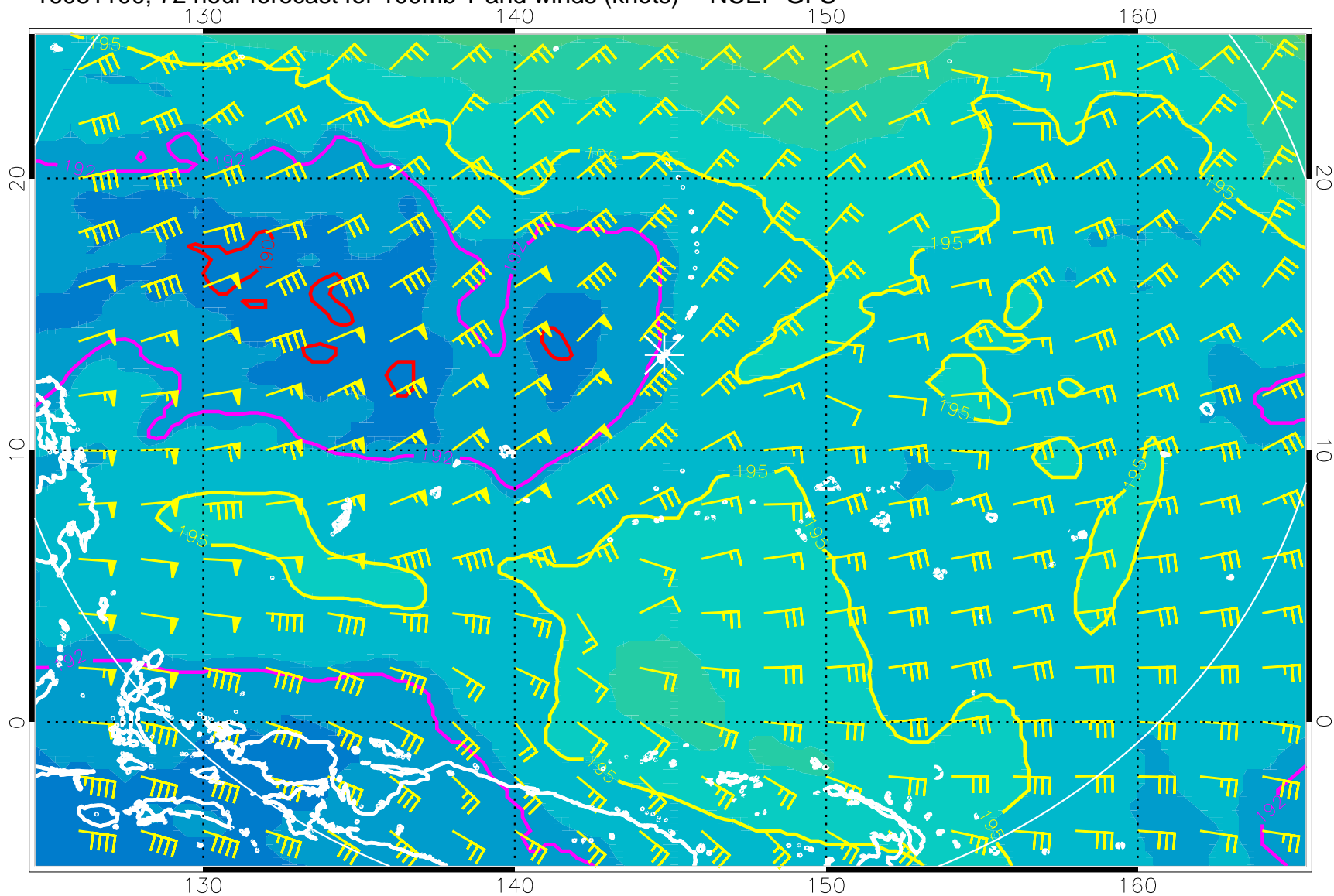
16081100, 72 hour forecast for 100mb T and winds (knots) -- NCEP GFS
