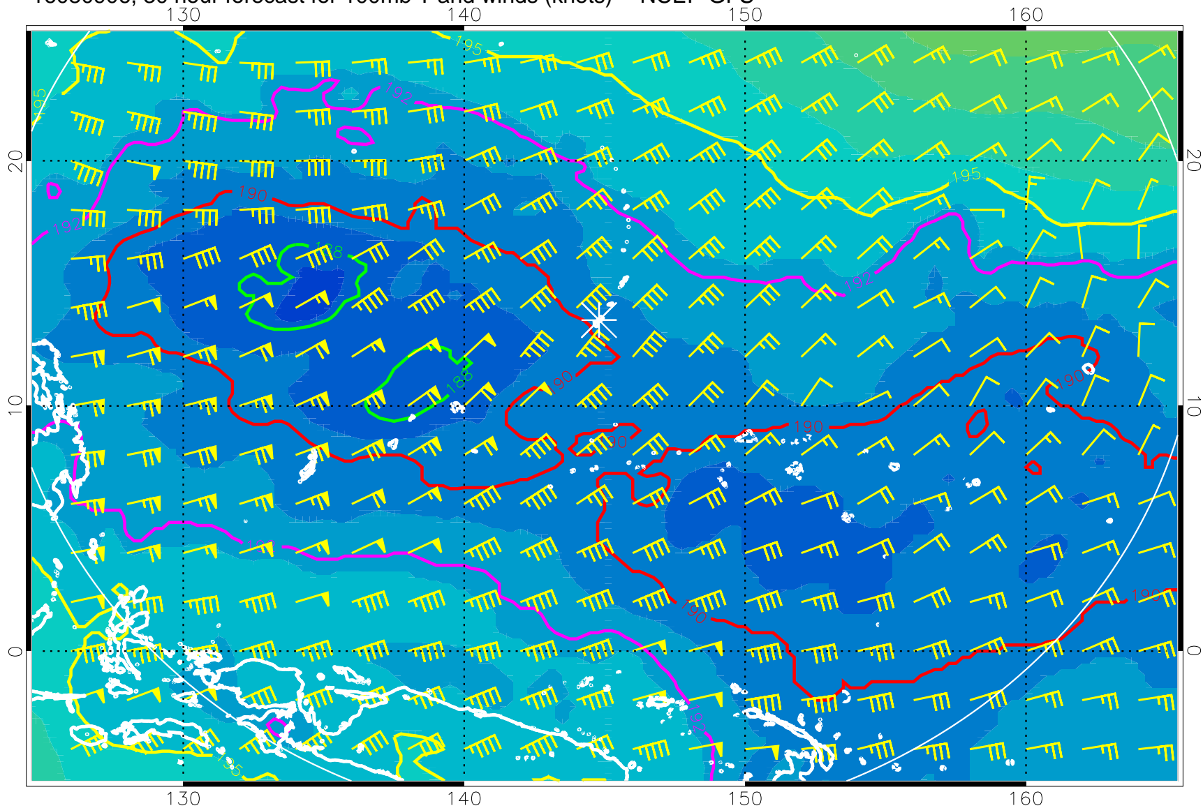
16080906, 30 hour forecast for 100mb T and winds (knots) -- NCEP GFS
