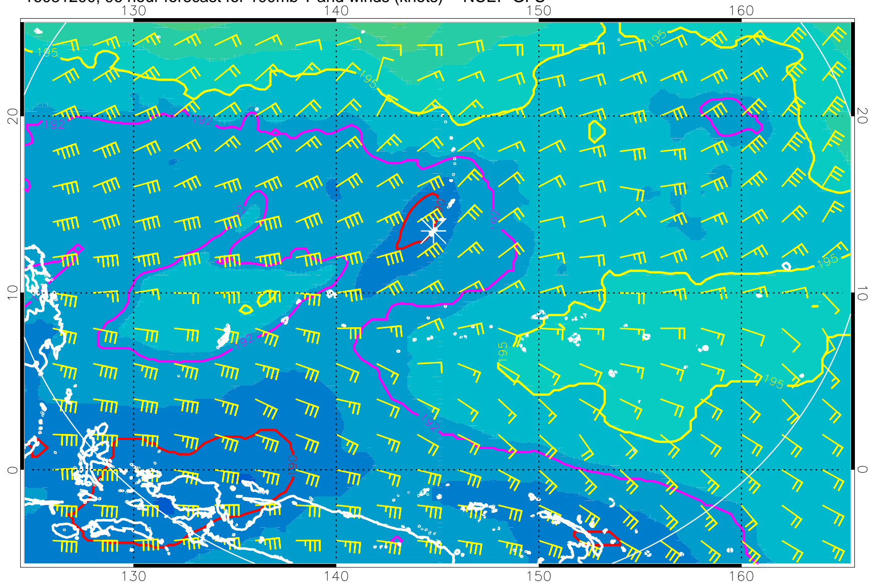
16081200, 96 hour forecast for 100mb T and winds (knots) -- NCEP GFS
