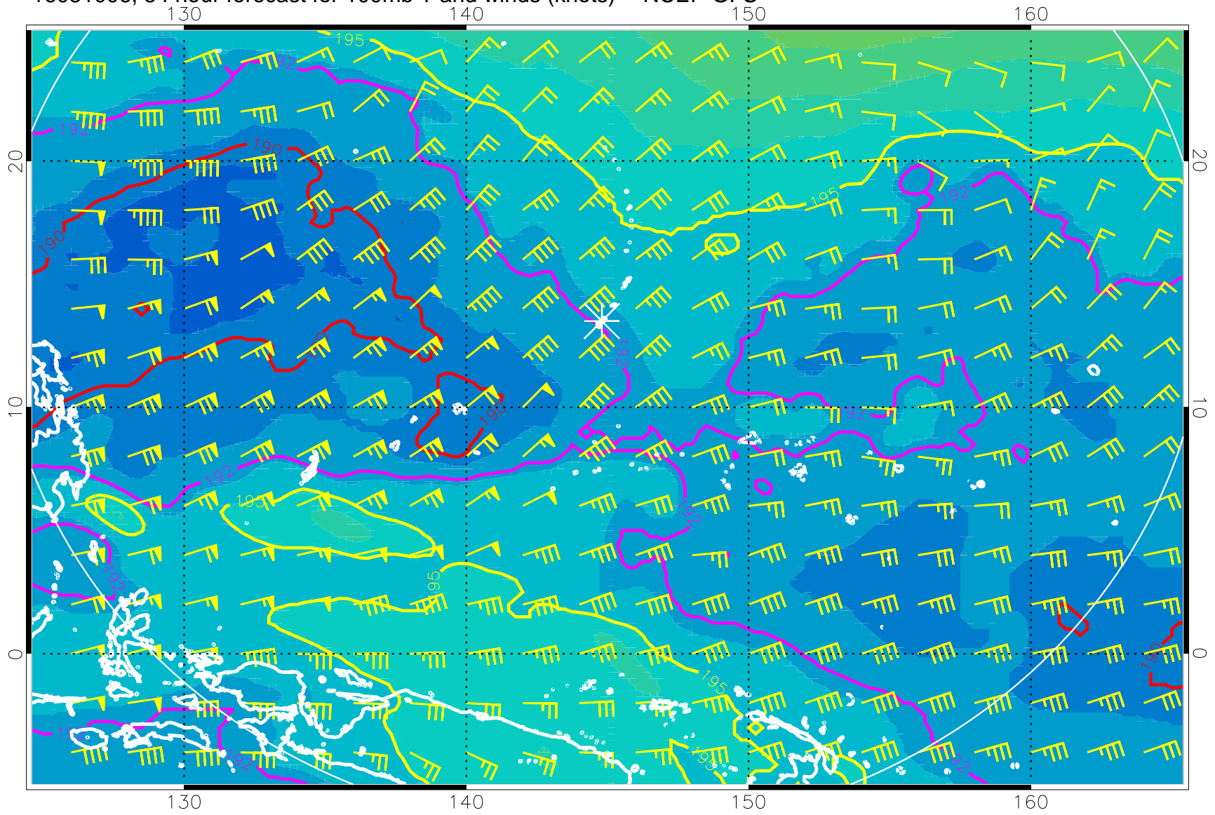
16081006, 54 hour forecast for 100mb T and winds (knots) -- NCEP GFS
