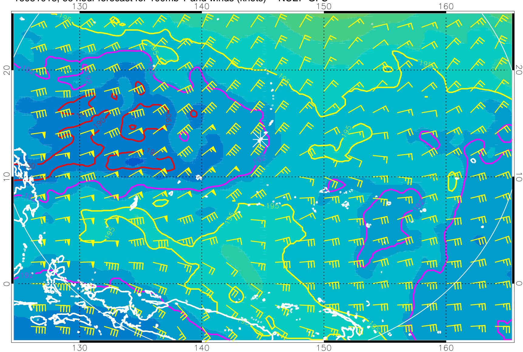
16081018, 66 hour forecast for 100mb T and winds (knots) -- NCEP GFS
