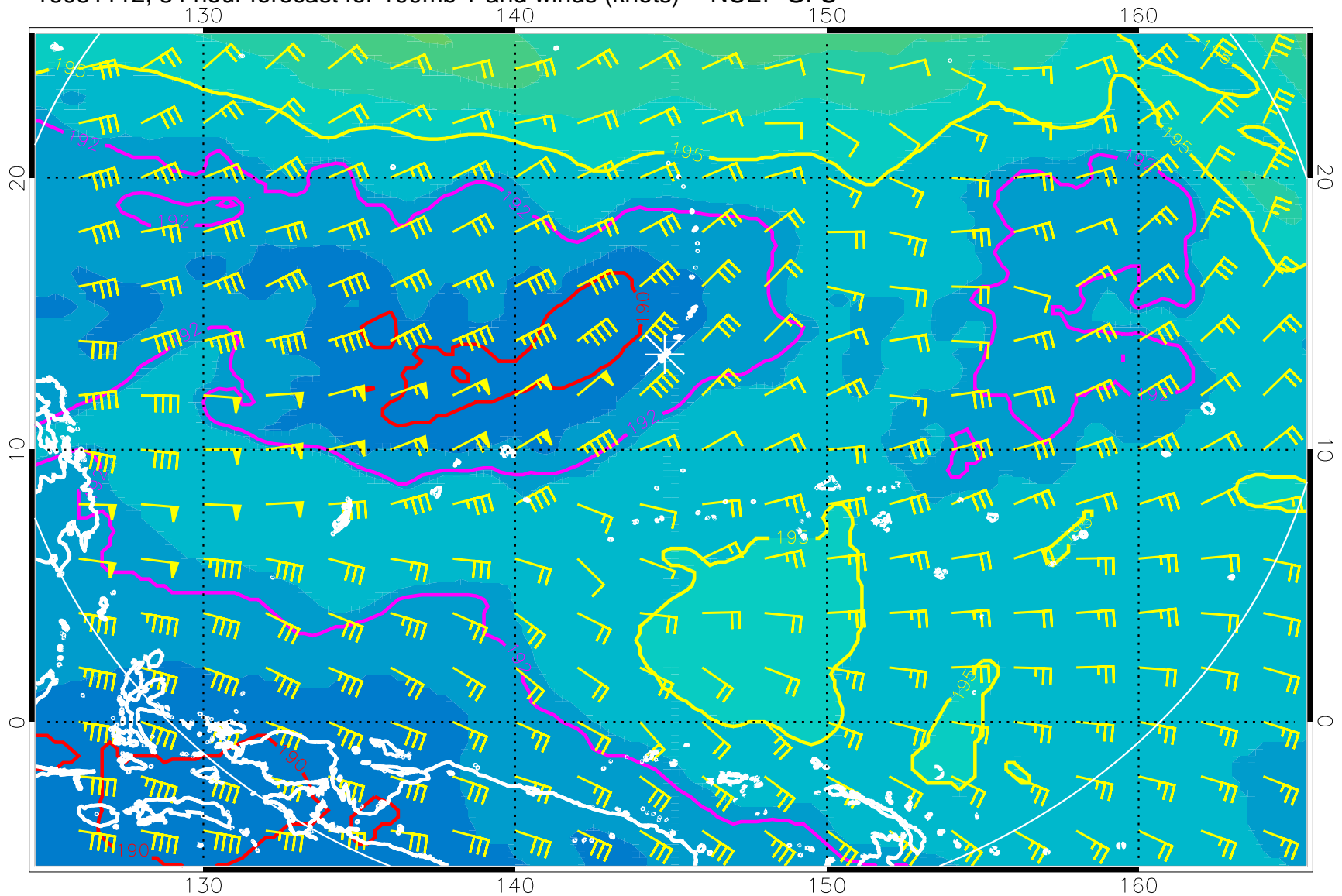
16081112, 84 hour forecast for 100mb T and winds (knots) -- NCEP GFS
