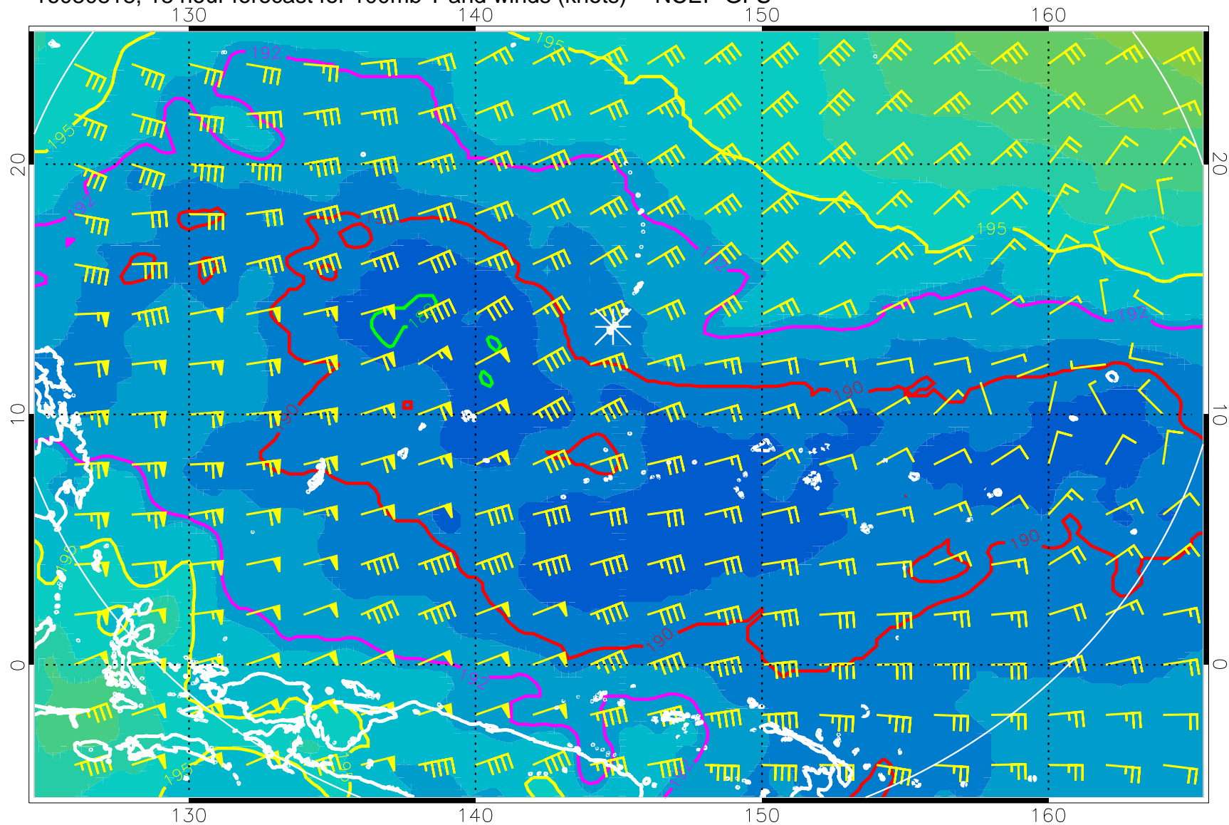
16080818, 18 hour forecast for 100mb T and winds (knots) -- NCEP GFS
