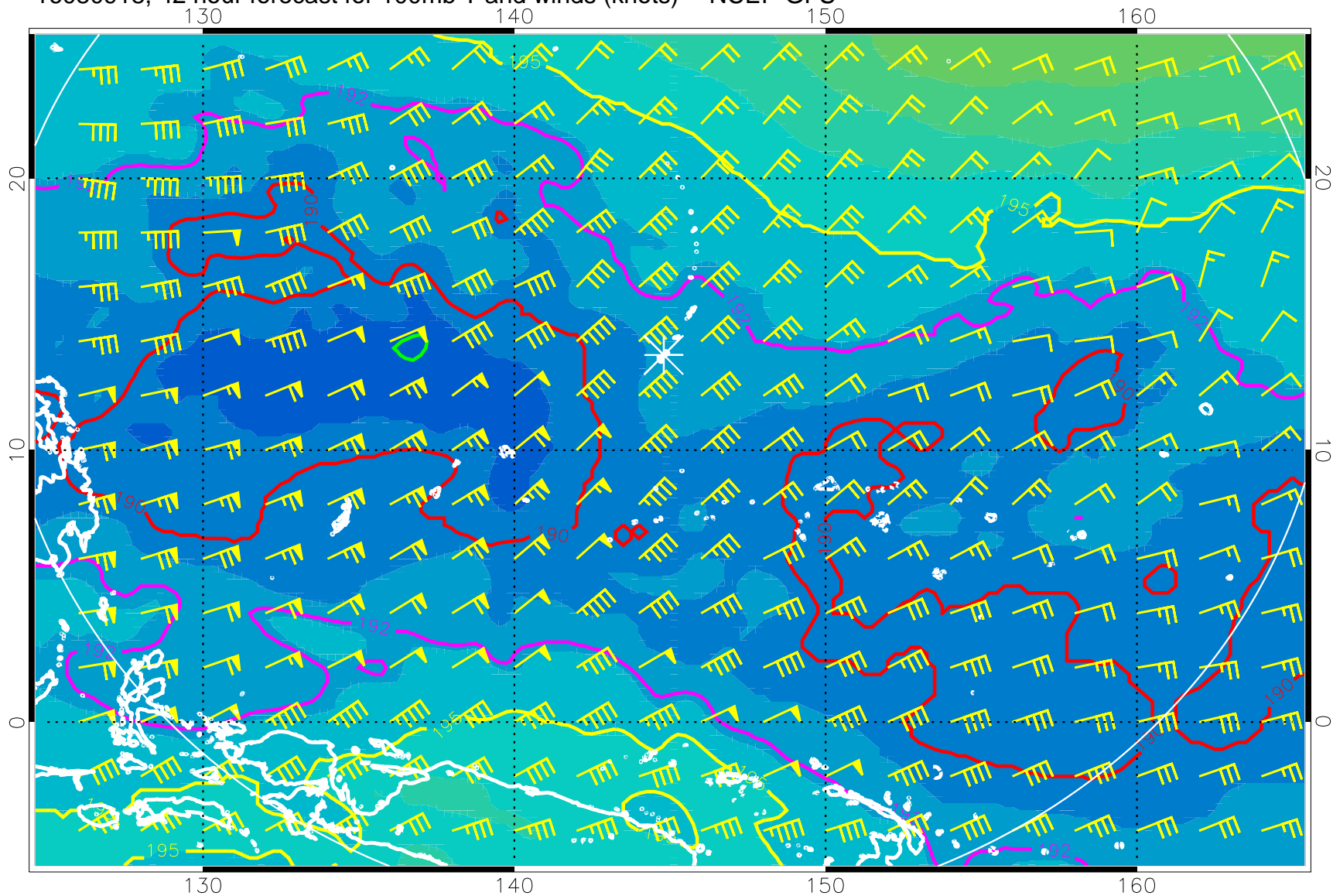
16080918, 42 hour forecast for 100mb T and winds (knots) -- NCEP GFS
