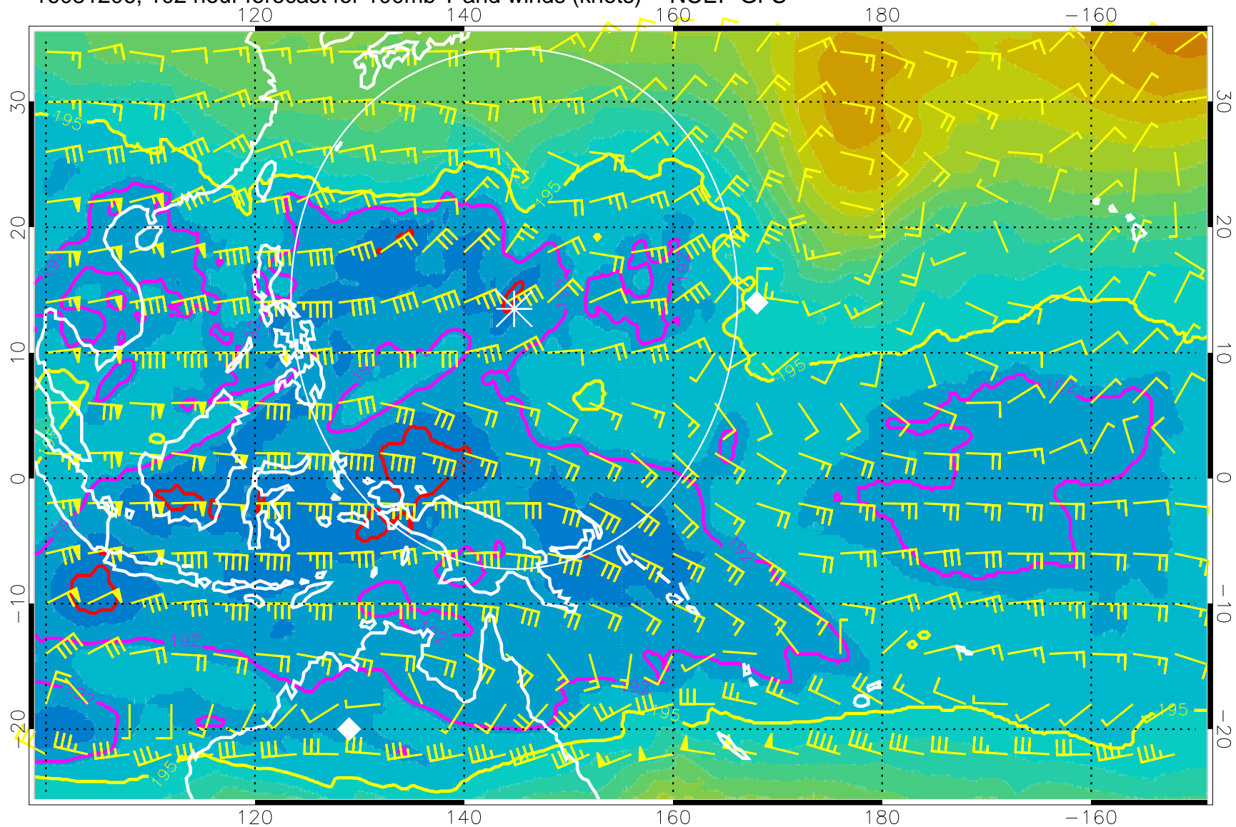
16081206, 102 hour forecast for 100mb T and winds (knots) -- NCEP GFS
