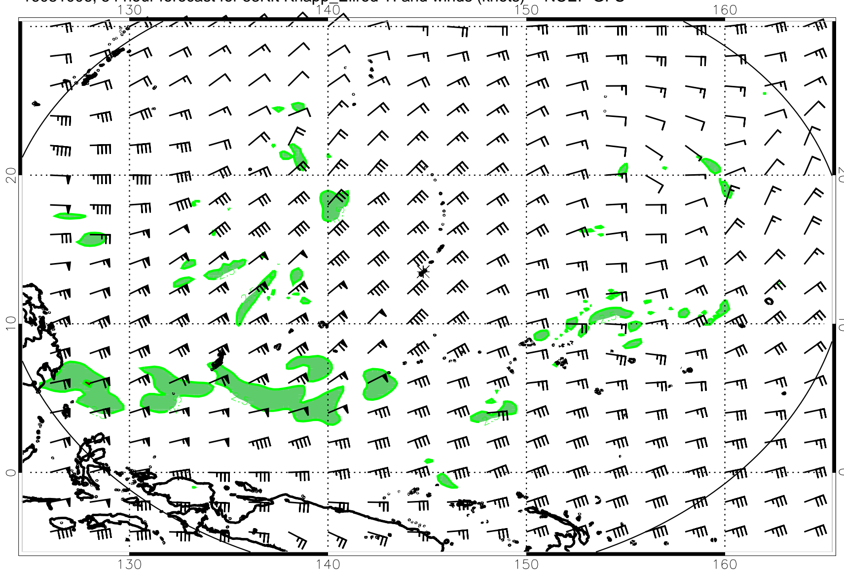
16081006, 54 hour forecast for 53Kft Knapp_Ellrod TI and winds (knots) -- NCEP GFS
