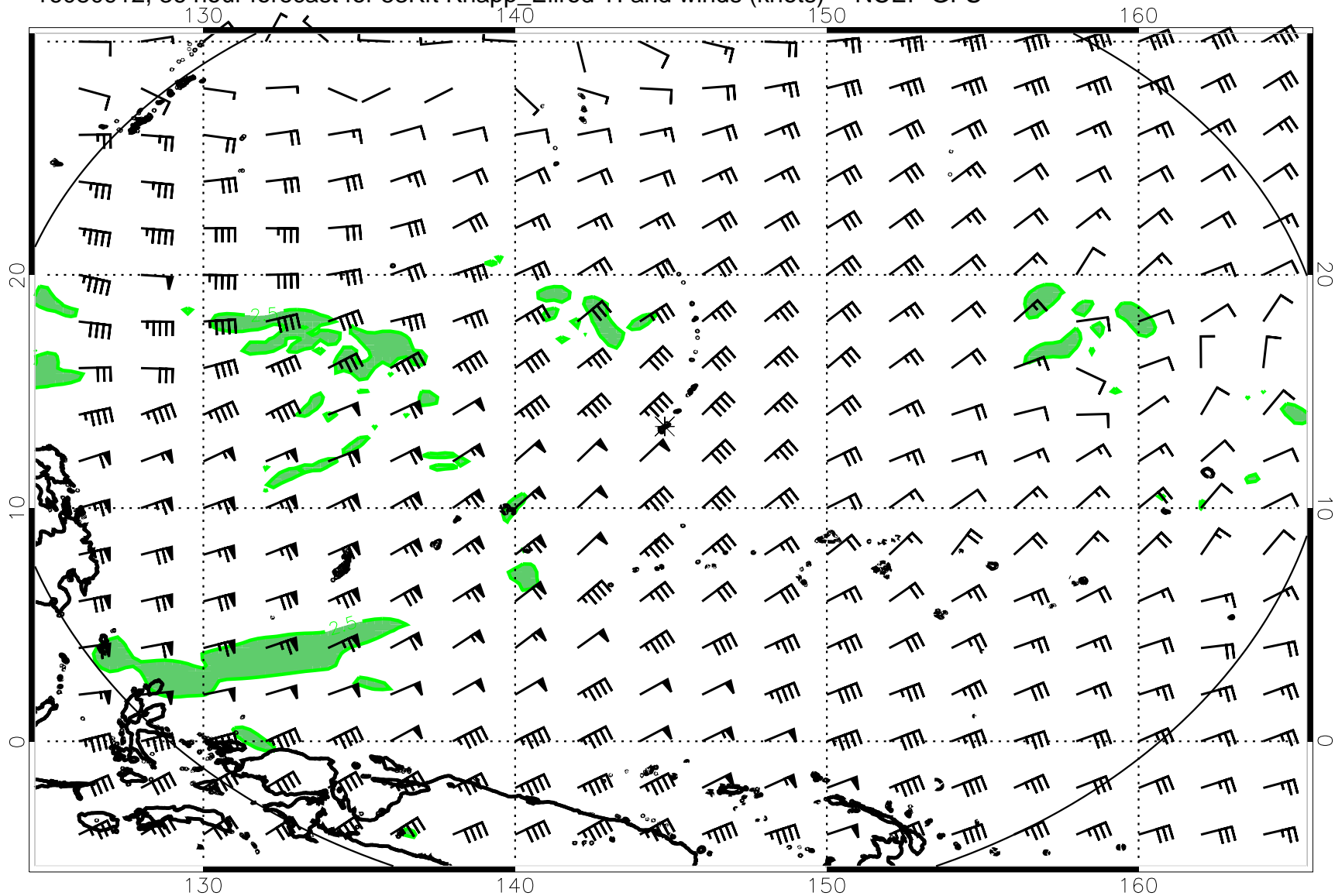
16080912, 36 hour forecast for 53Kft Knapp_Ellrod TI and winds (knots) -- NCEP GFS
