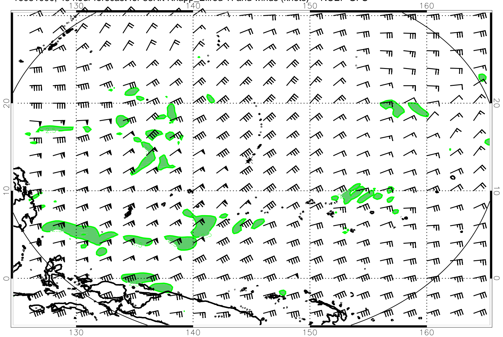
16081000, 48 hour forecast for 53Kft Knapp_Ellrod TI and winds (knots) -- NCEP GFS
