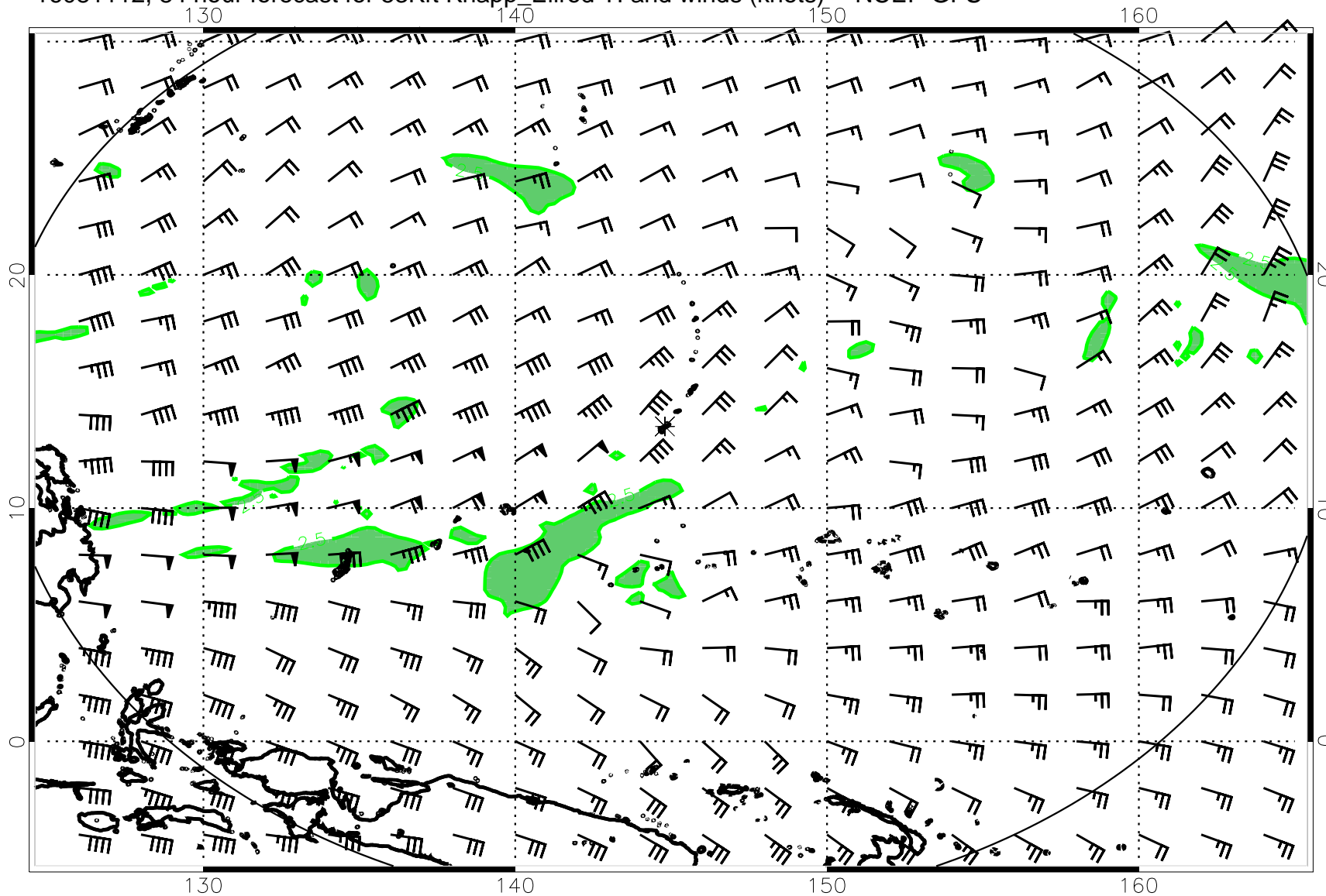
16081112, 84 hour forecast for 53Kft Knapp_Ellrod TI and winds (knots) -- NCEP GFS
