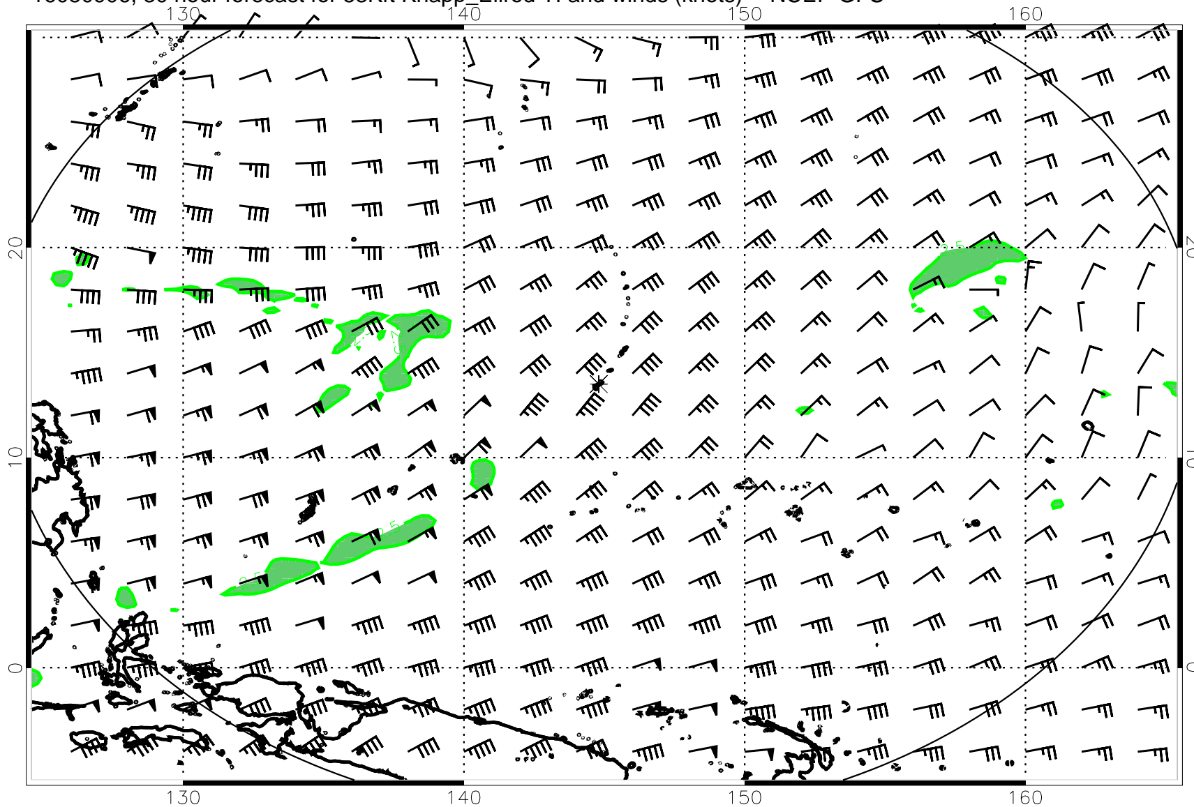
16080906, 30 hour forecast for 53Kft Knapp_Ellrod TI and winds (knots) -- NCEP GFS
