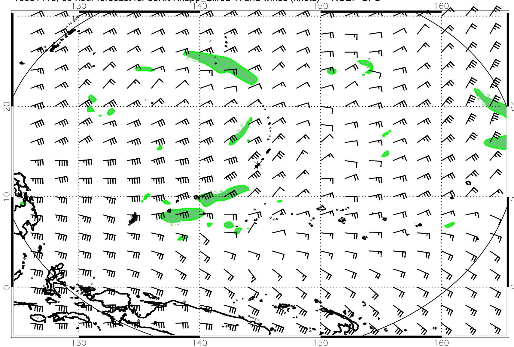
16081118, 90 hour forecast for 53Kft Knapp_Ellrod TI and winds (knots) -- NCEP GFS
