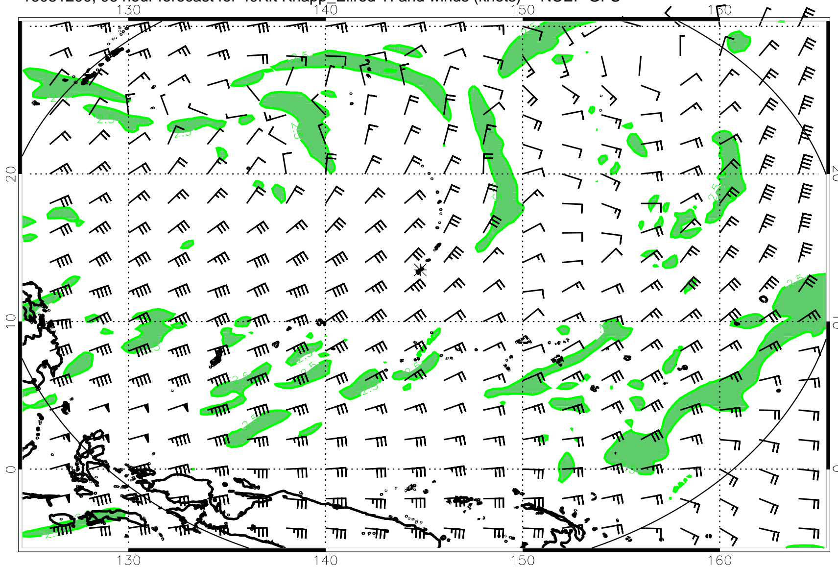
16081200, 96 hour forecast for 49Kft Knapp_Ellrod TI and winds (knots) -- NCEP GFS
