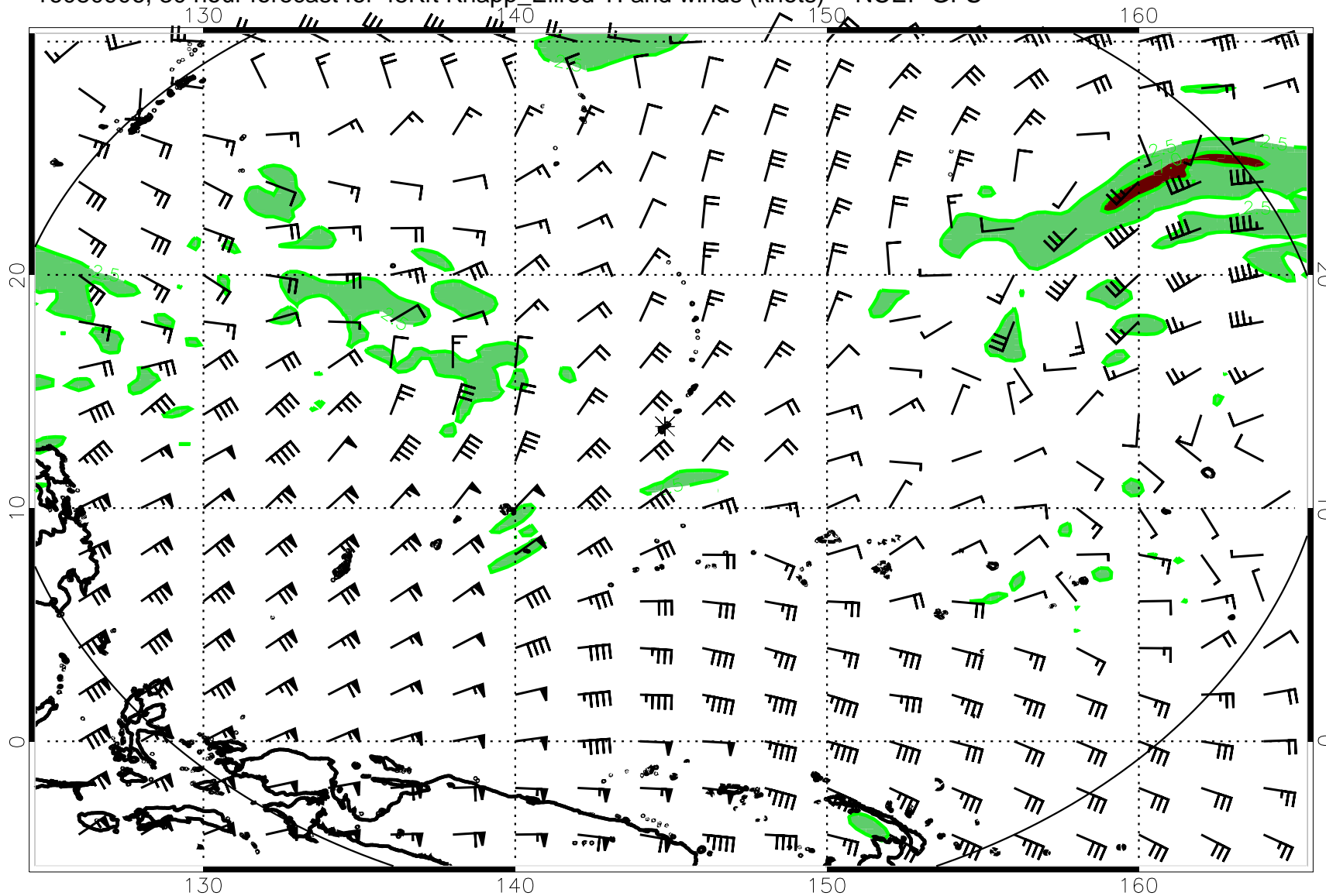
16080906, 30 hour forecast for 45Kft Knapp_Ellrod TI and winds (knots) -- NCEP GFS
