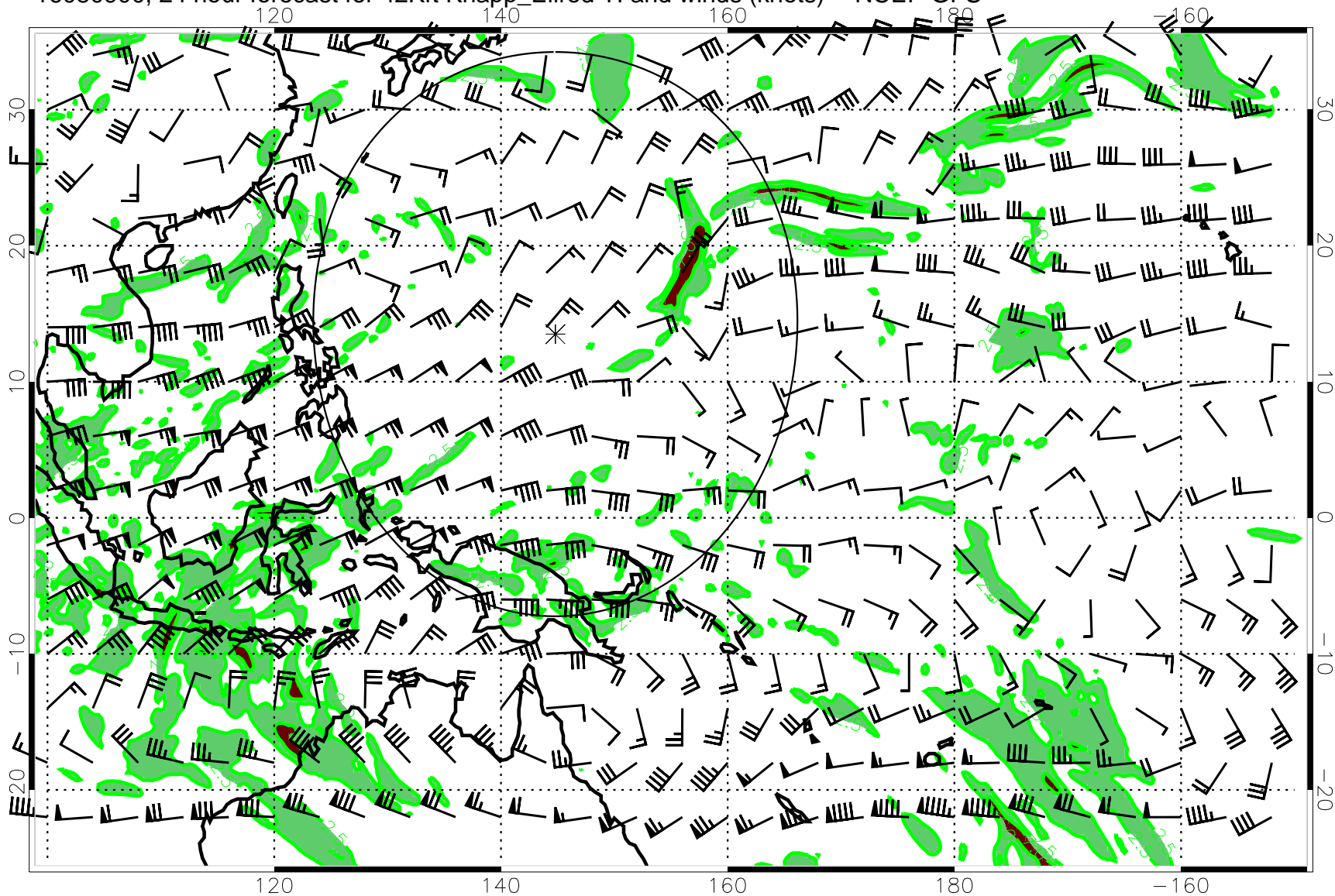
16080900, 24 hour forecast for 42Kft Knapp_Ellrod TI and winds (knots) -- NCEP GFS
