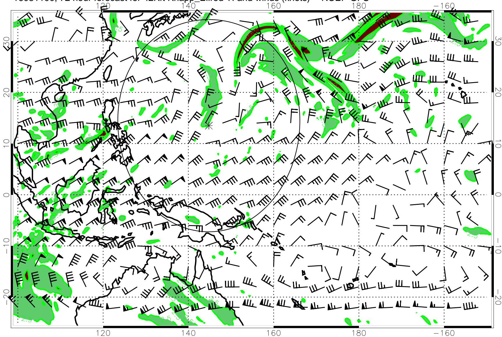
16081100, 72 hour forecast for 42Kft Knapp_Ellrod TI and winds (knots) -- NCEP GFS
