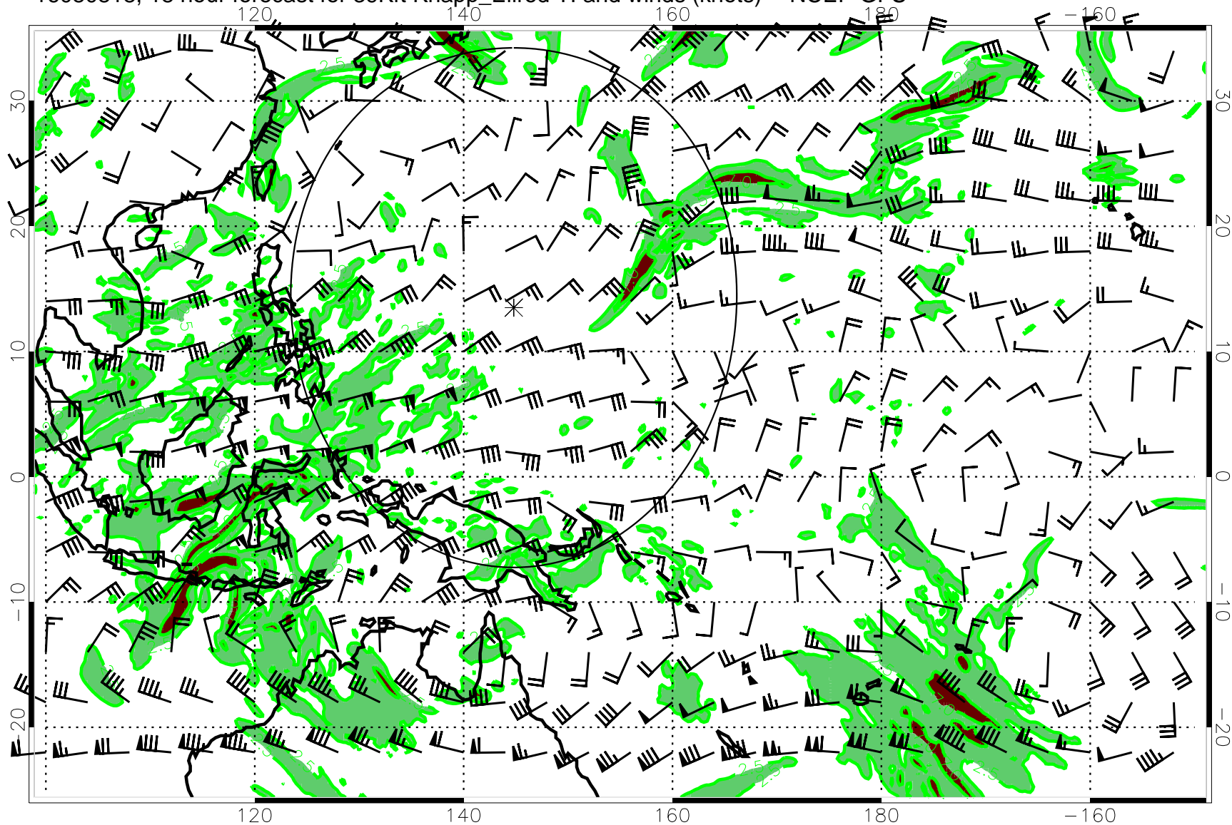
16080818, 18 hour forecast for 39Kft Knapp_Ellrod TI and winds (knots) -- NCEP GFS
