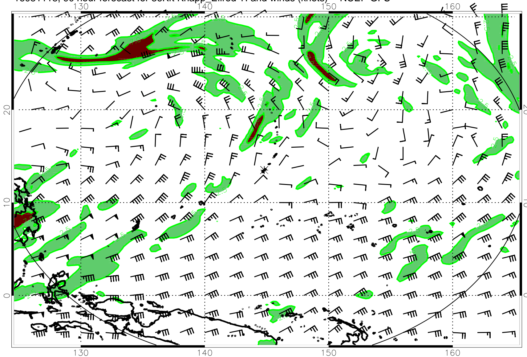
16081118, 90 hour forecast for 36Kft Knapp_Ellrod TI and winds (knots) -- NCEP GFS
