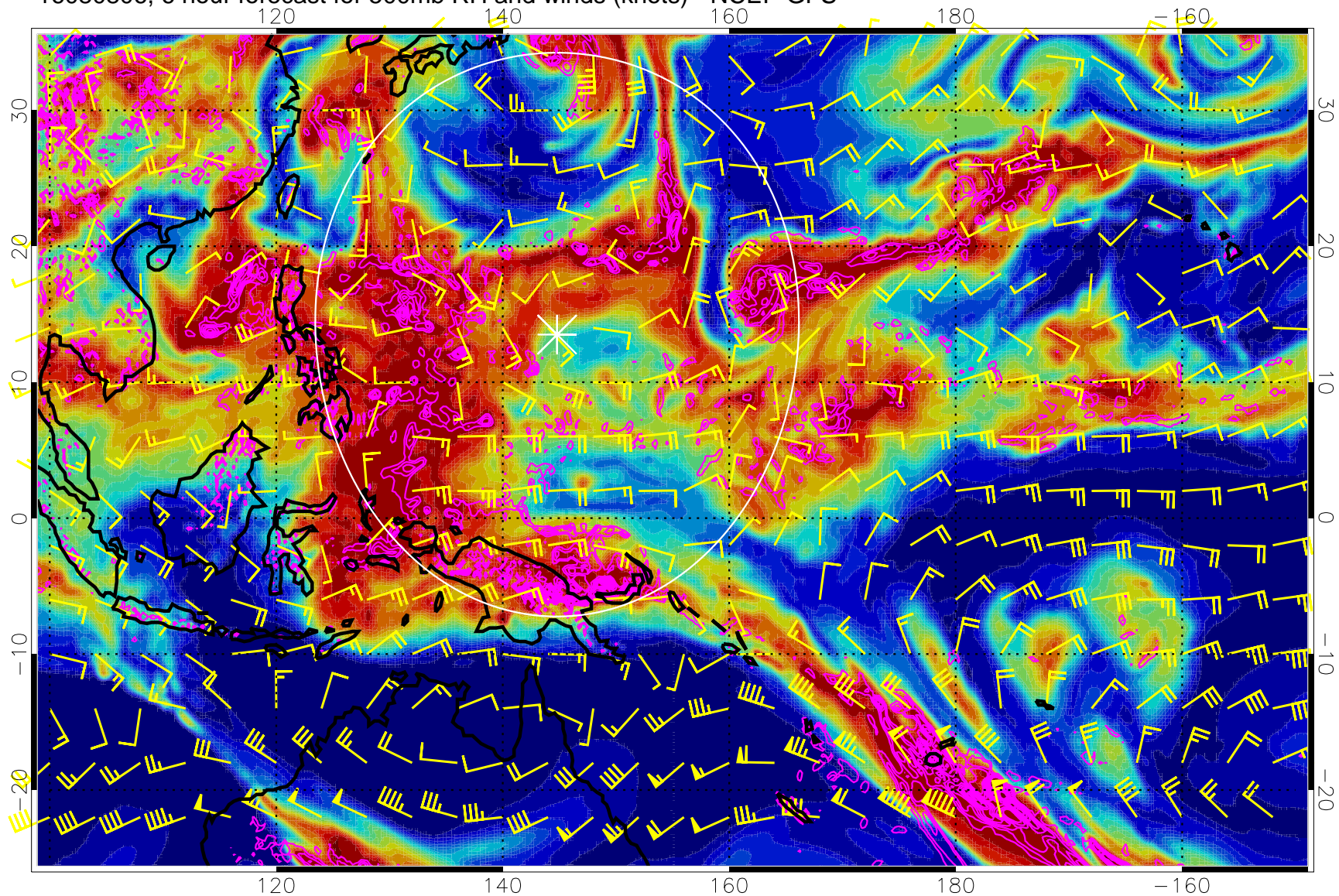
16080806, 6 hour forecast for 500mb RH and winds (knots) - NCEP GFS
