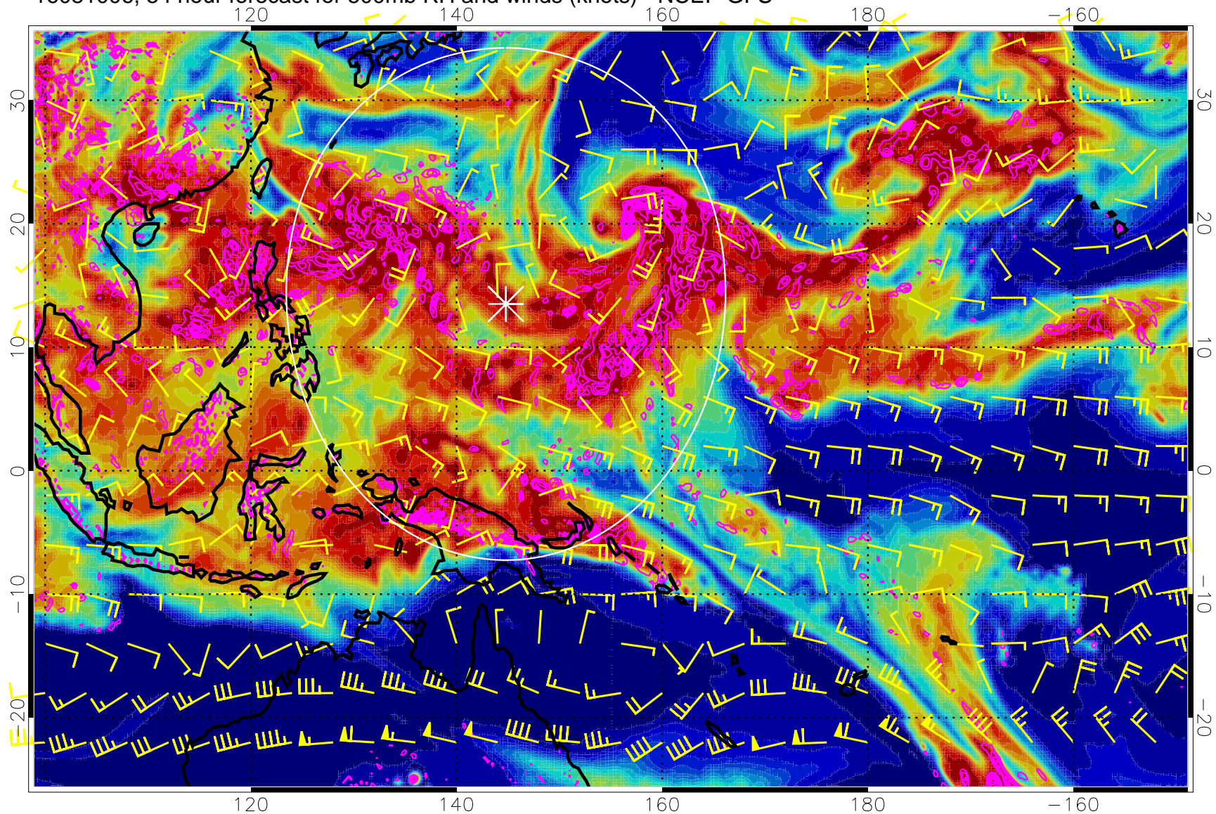
16081006, 54 hour forecast for 500mb RH and winds (knots) - NCEP GFS
